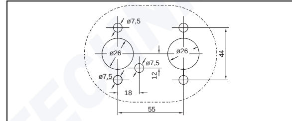
Fig. 3: Hole pattern
