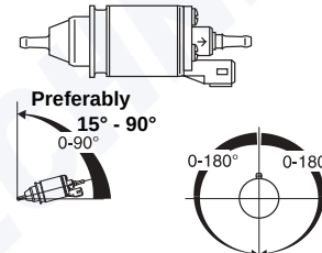
Fig. 15: Metering pump DP 2
