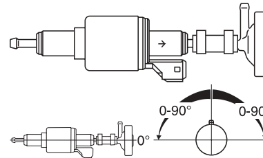
Fig. 16: Metering pump DP 30
