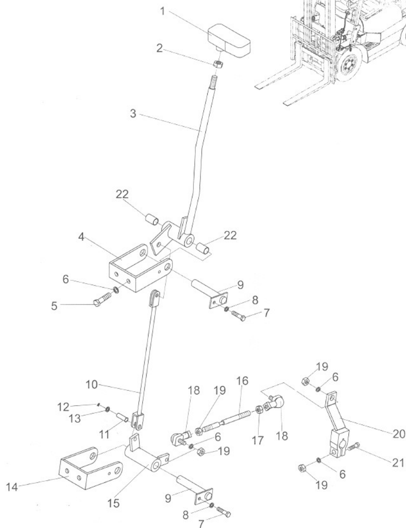
变速箱变速操纵(液力式)/TRANSMISSION CONTROL LINKAGE (TOR-CON TYPE)
