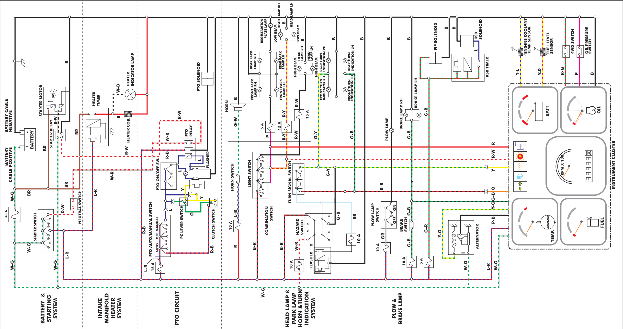
INSTRUMENT CLUSTER CONNECTION DETAILS
