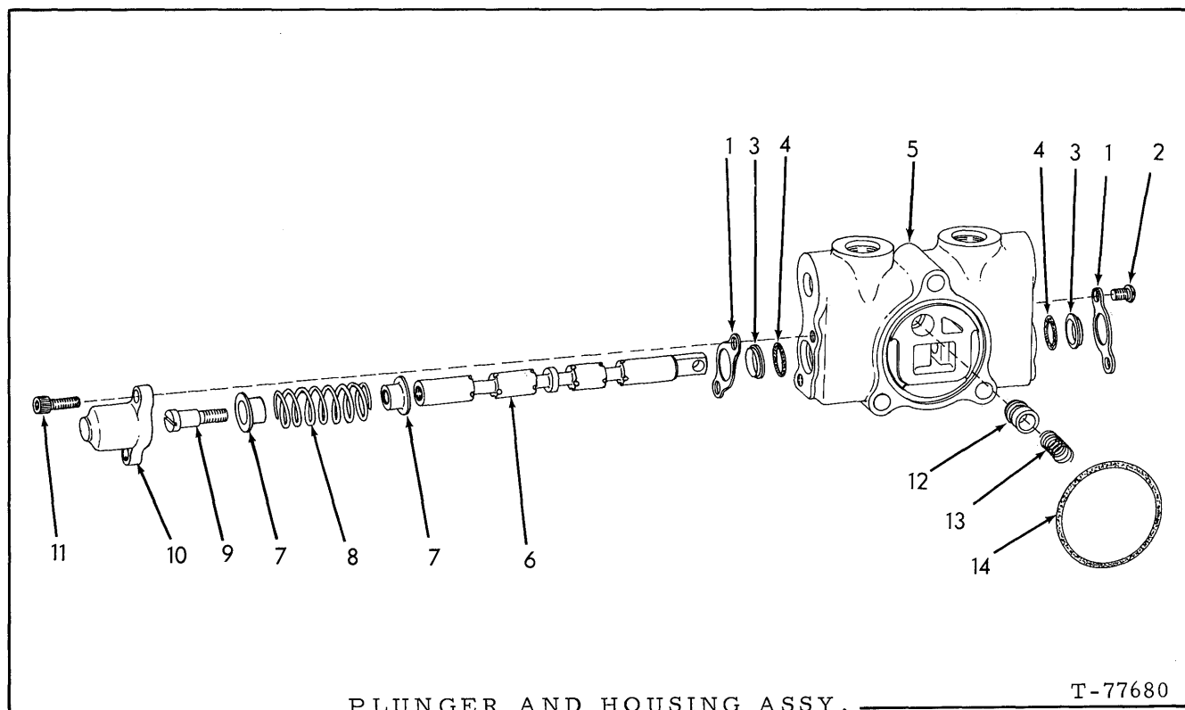
PLUNGER AND HOUSING ASSY.
