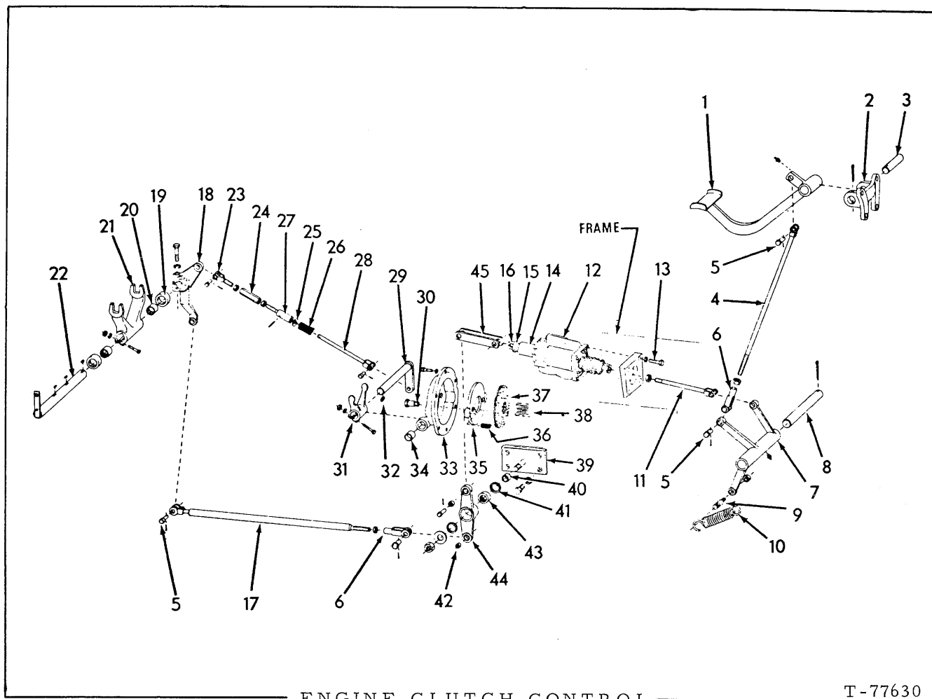
ENGINE CLUTCH CONTROL
