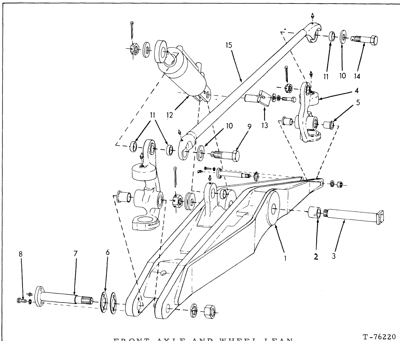
FRONT AXLE AND WHEEL LEAN
