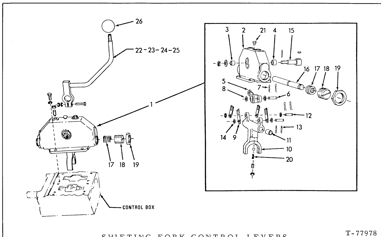
SHIFTING FORK CONTROL LEVERS
