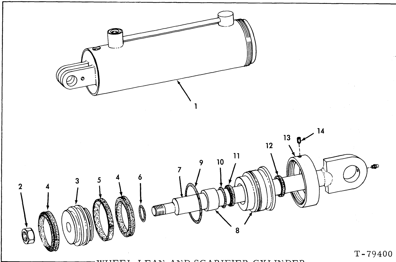
WHEEL LEAN AND SCARIFIER CYLINDER
