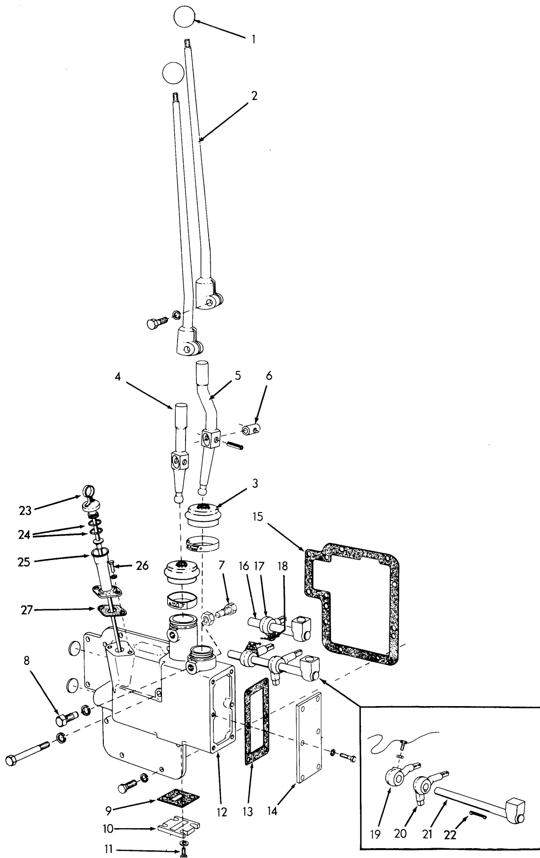
GEAR SHIFT CONTROLS
