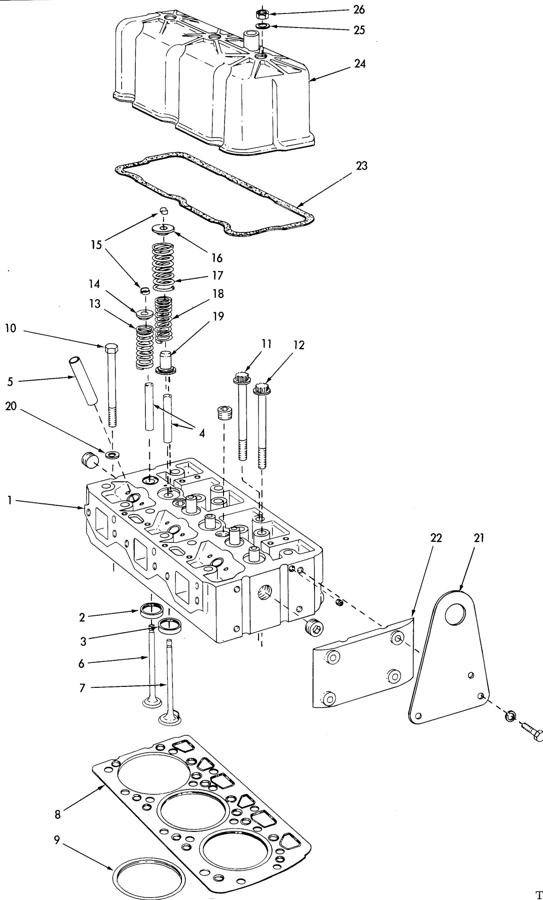
CYLINDER HEAD
