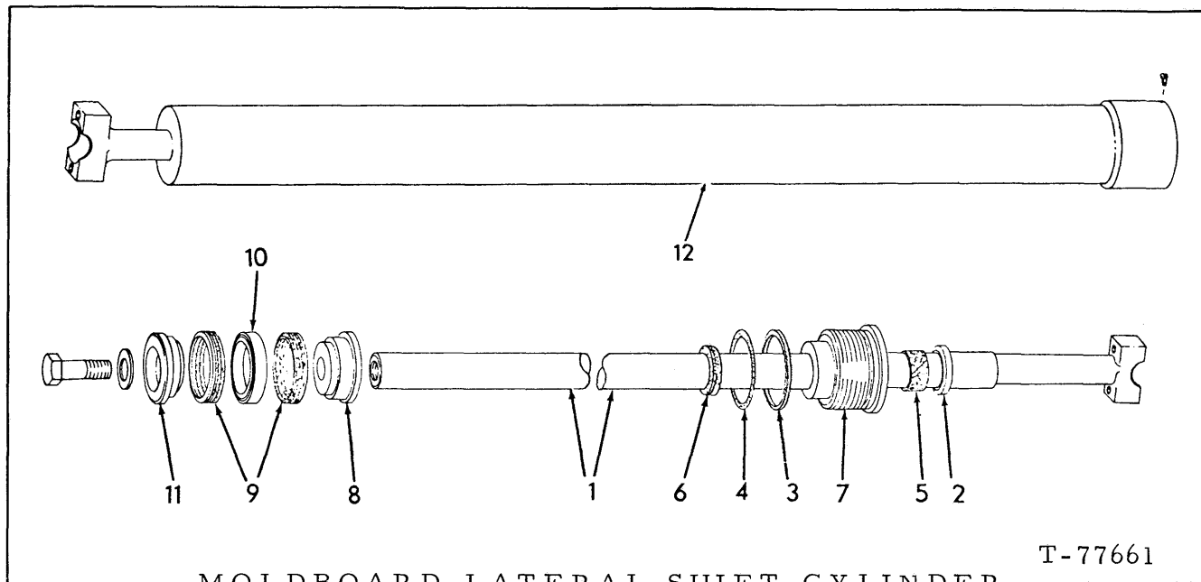
MOLDBOARD LATERAL SHIFT CYLINDER
