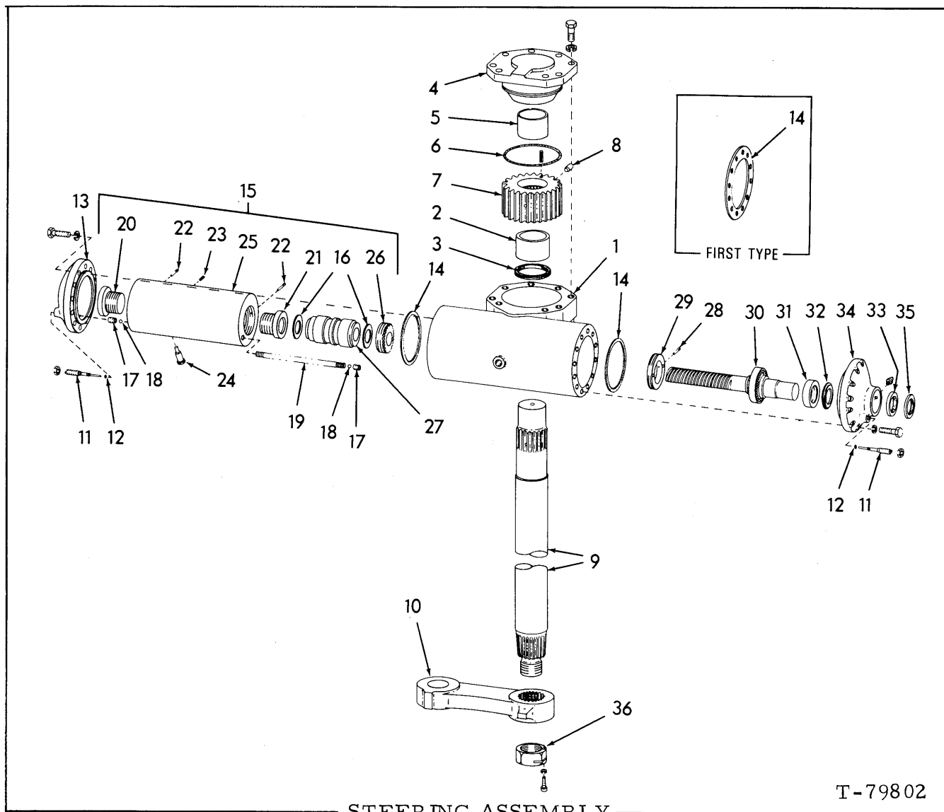
STEERING ASSEMBLY
