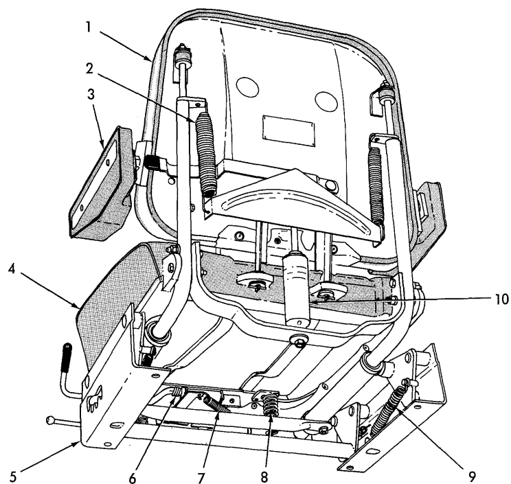
SEAT ASSEMBLY
