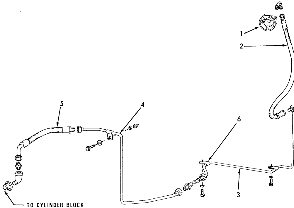
ENGINE OIL PRESSURE GAUGE
