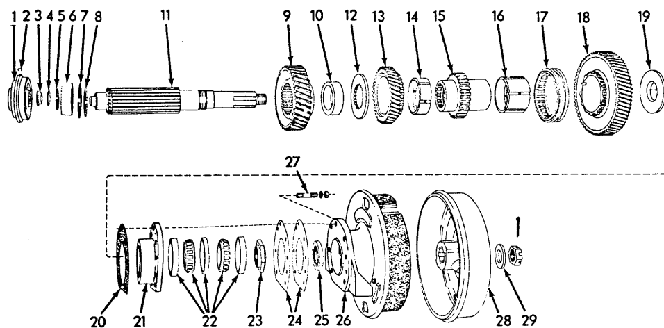
TRANSMISSION BOTTOM SHAFT
