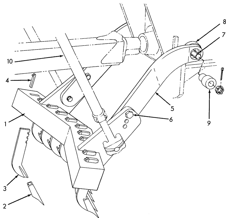
SCARIFIER
