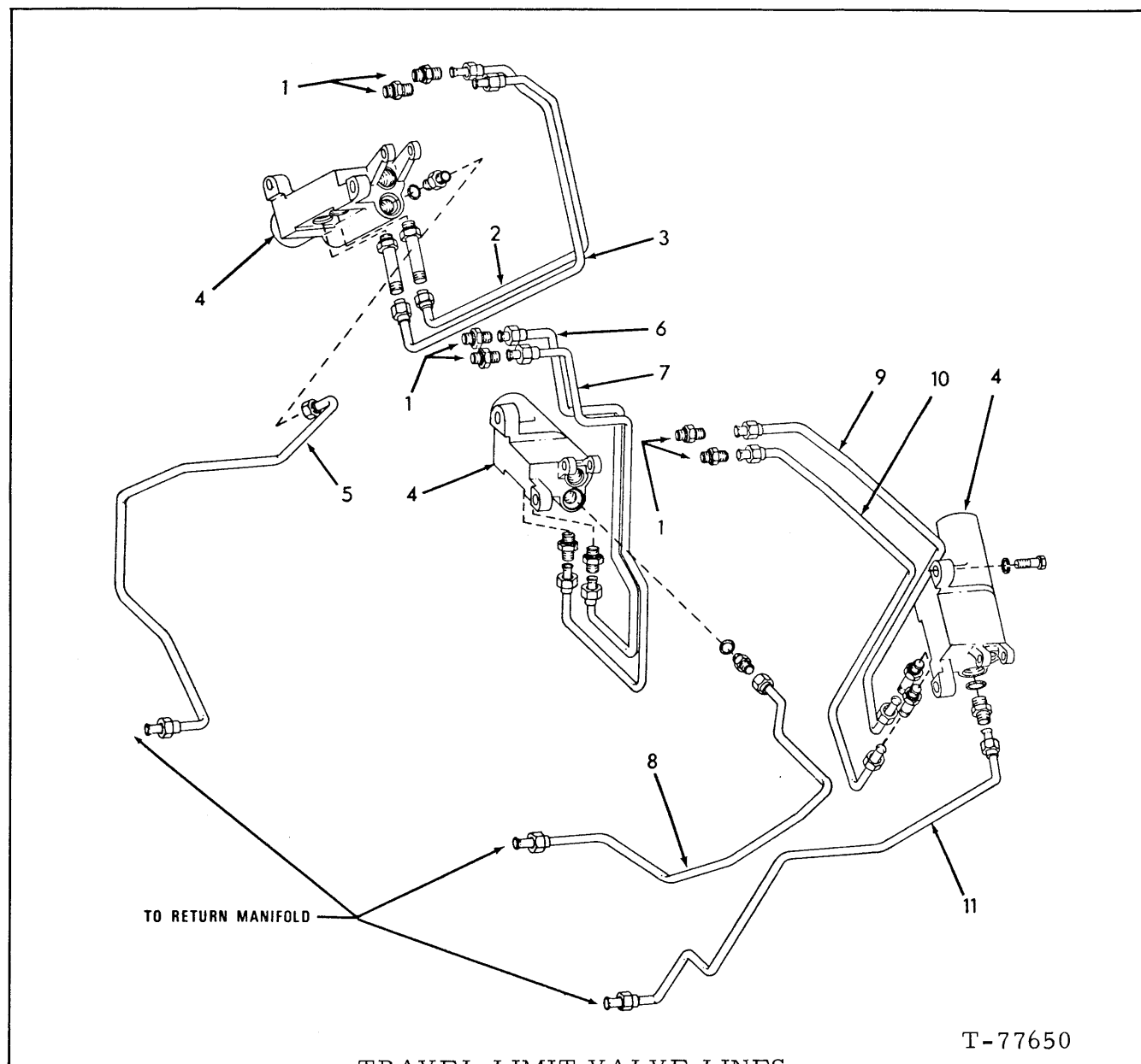
TRAVEL LIMIT VALVE LINES
