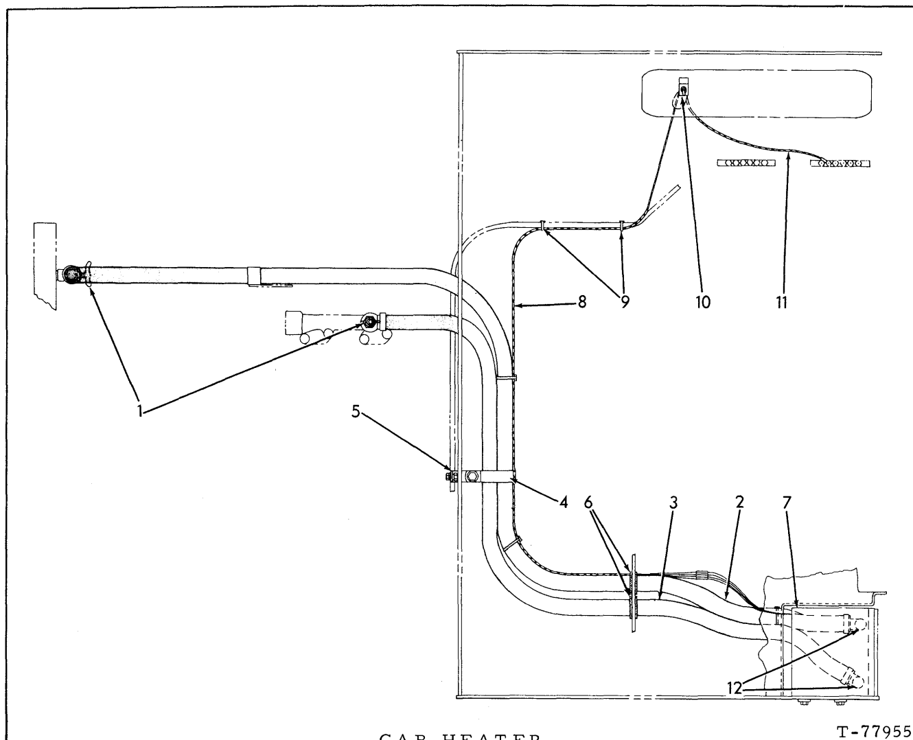
CAB HEATER
