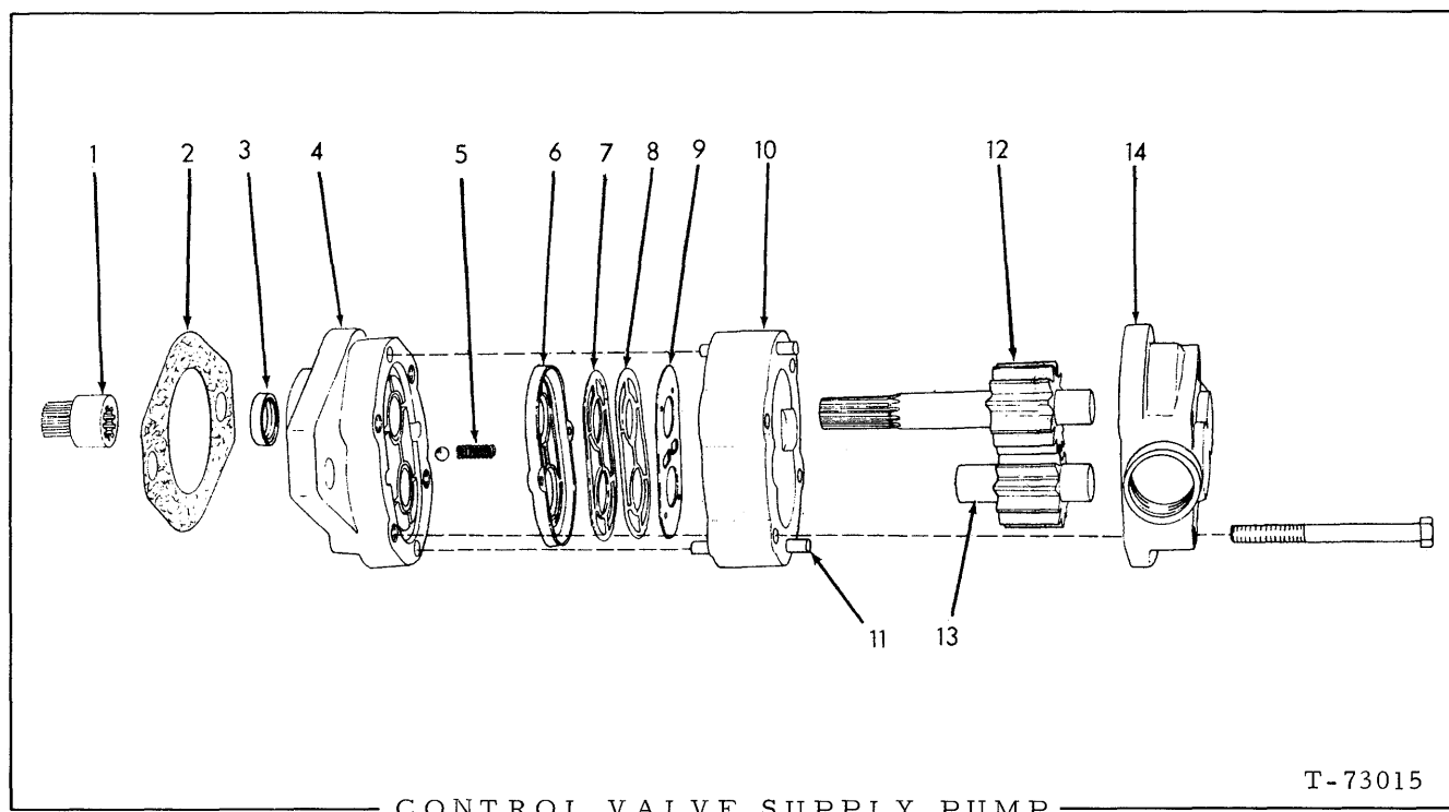
CONTROL VALVE SUPPLY PUMP
