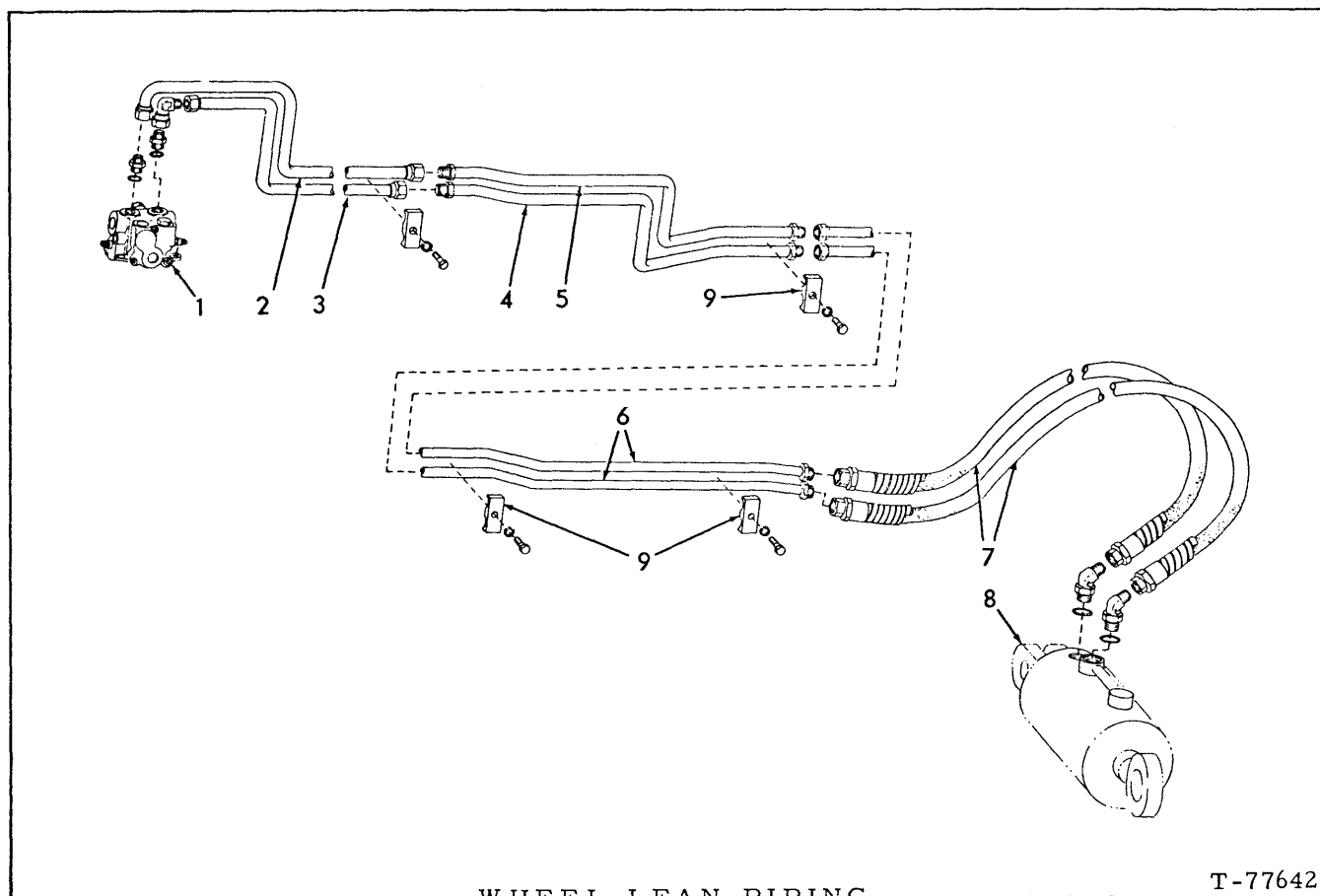
WHEEL LEAN PIPING
