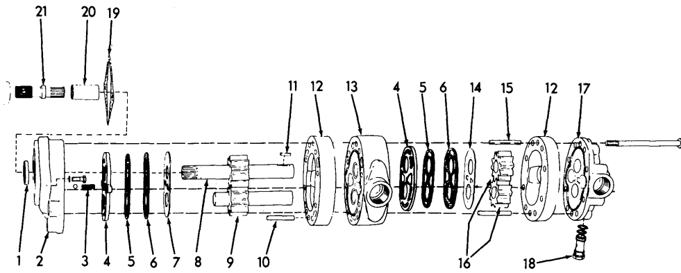
CLUTCH/BRAKE AND STEERING PUMP
