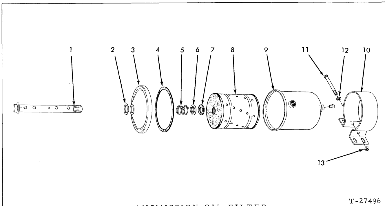
TRANSMISSION OIL FILTER
