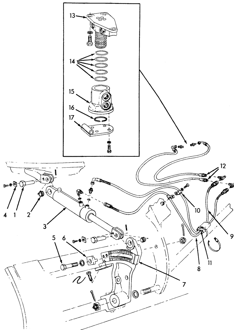
MOLDBOARD PITCH HYDRAULICS
