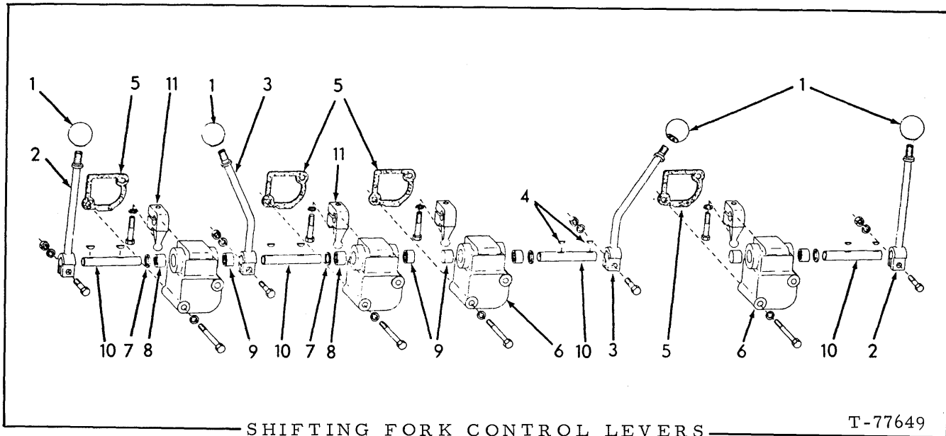
SHIFTING FORK CONTROL LEVERS
