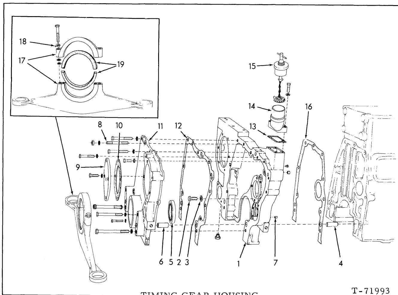
TIMING GEAR HOUSING
