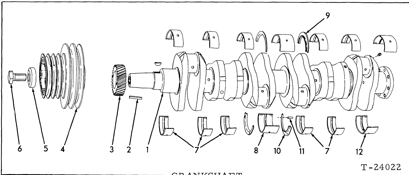
CRANKSHAFT
