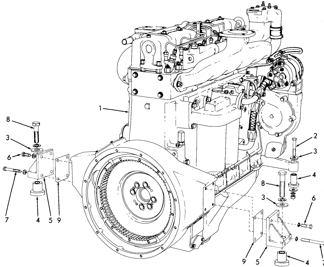
ENGINE AND MOUNTING
