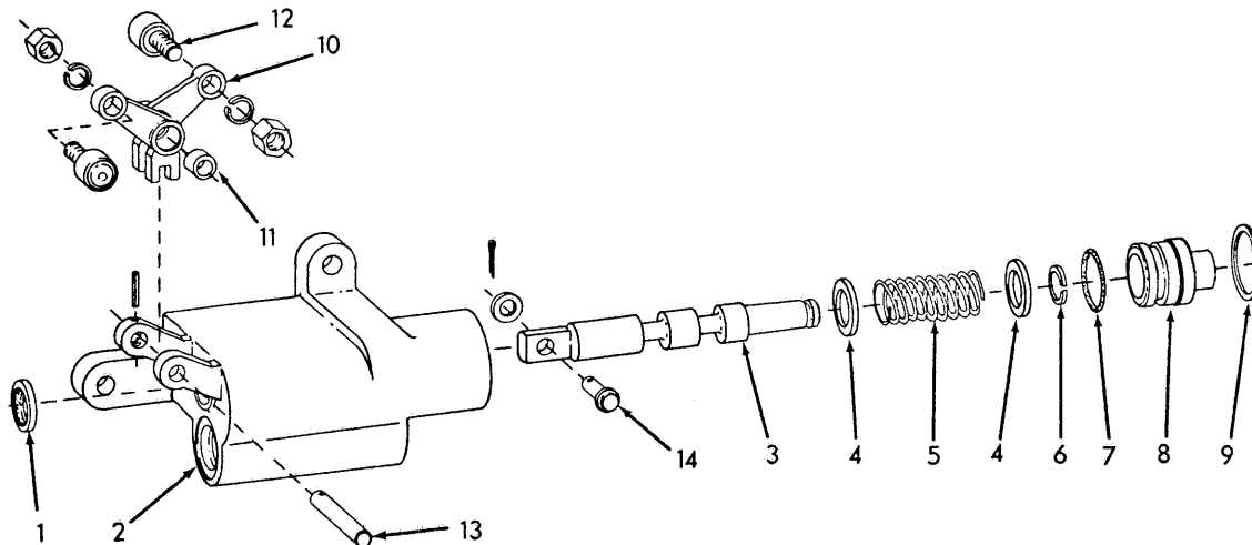
TRAVEL LIMIT VALVE
