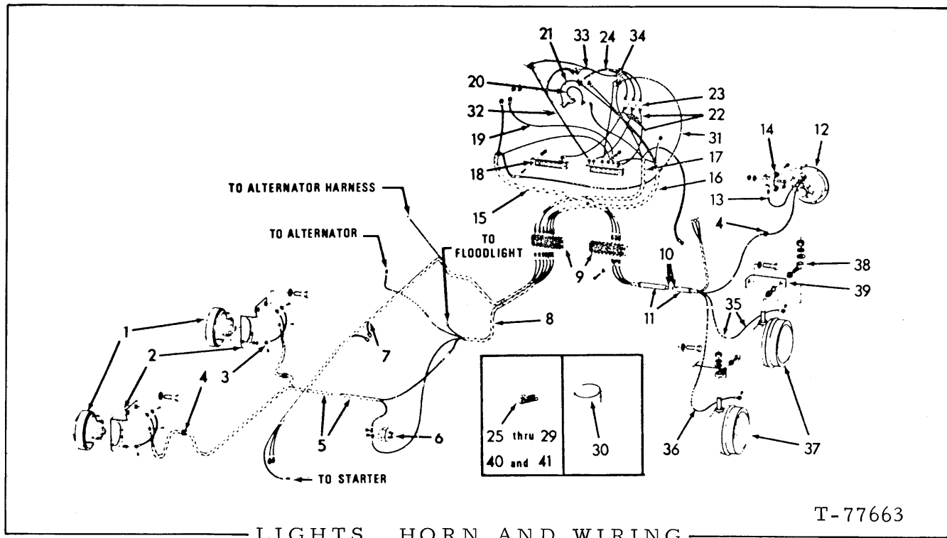
LIGHTS, HORN AND WIRING
