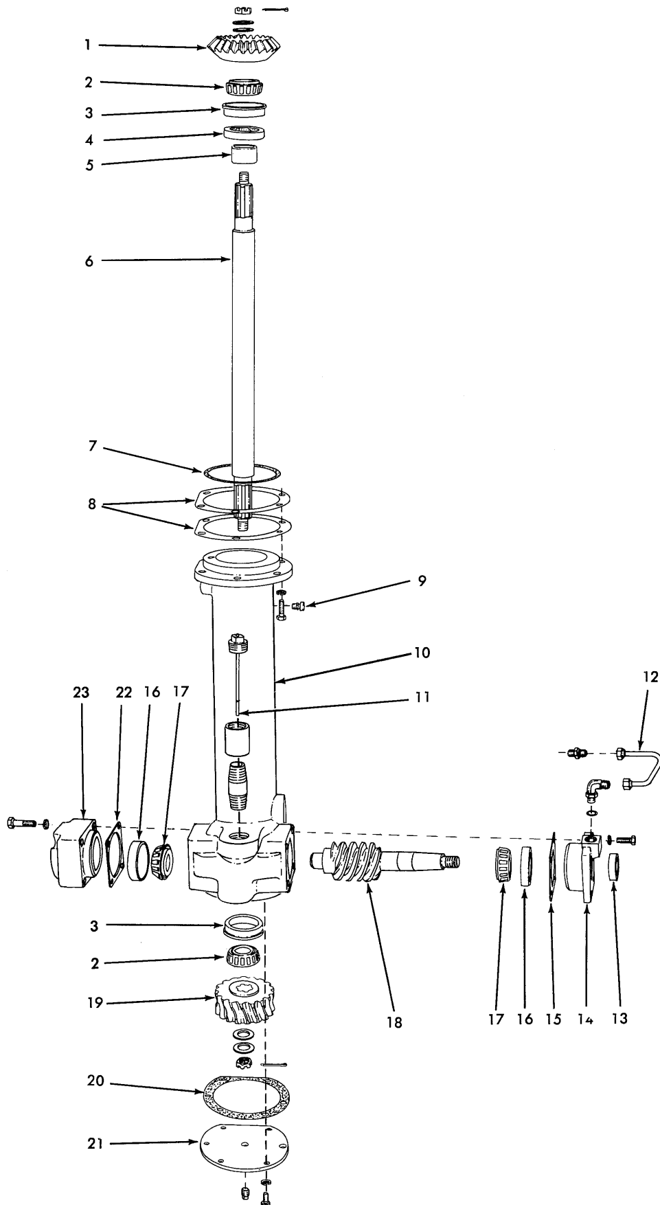
POWER TAKE-OFF VERTICAL DRIVE
