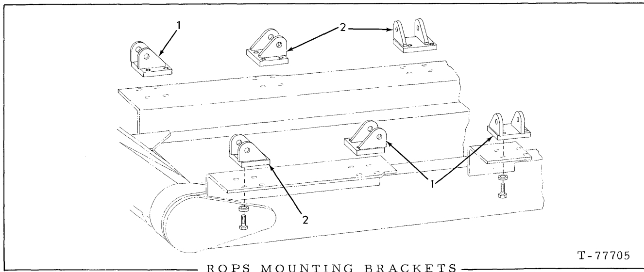
ROPS MOUNTING BRACKETS
