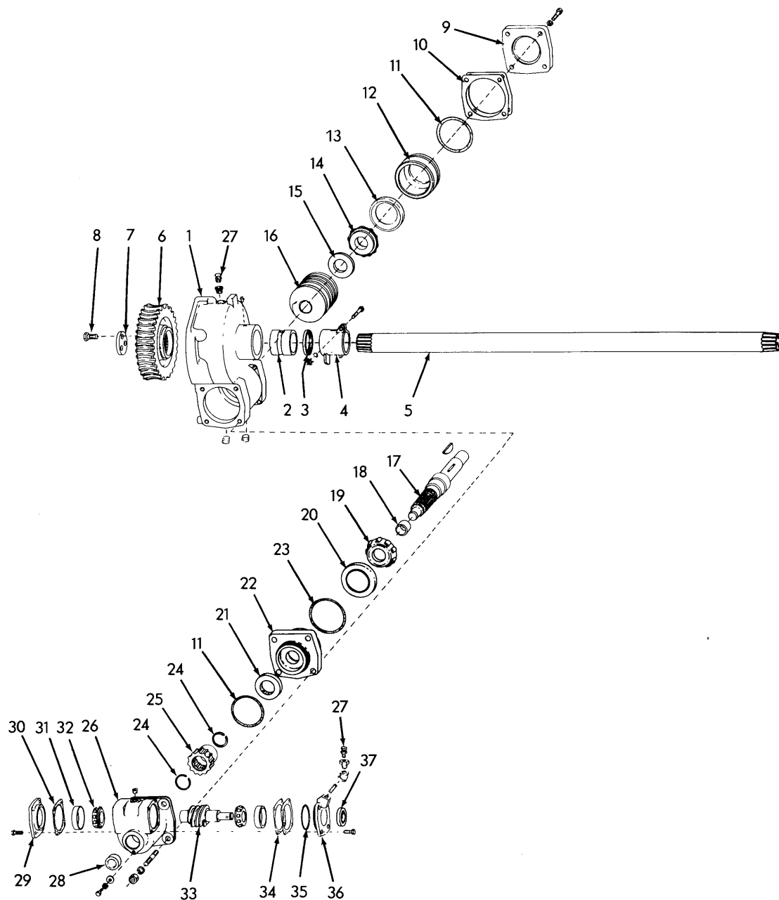
SIDE SHIFT GEAR HOUSING ASSEMBLY
