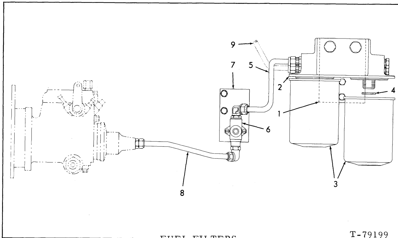
FUEL FILTERS
