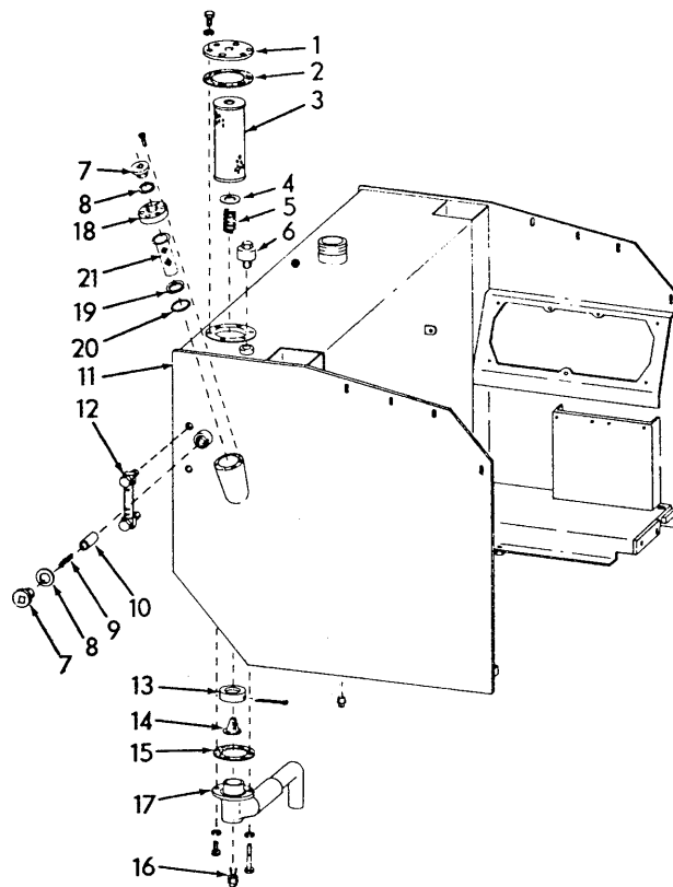
HYDRAULIC TANK
