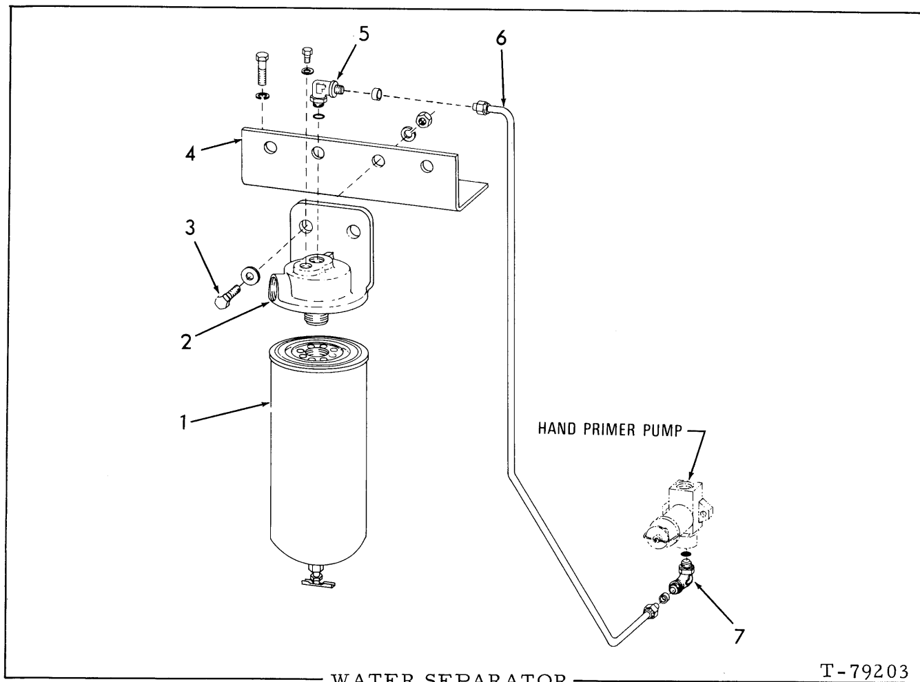
WATER SEPARATOR
