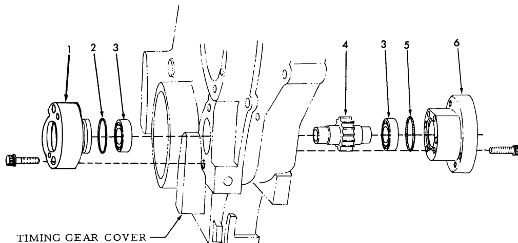
HYDRAULIC PUMP DRIVE
