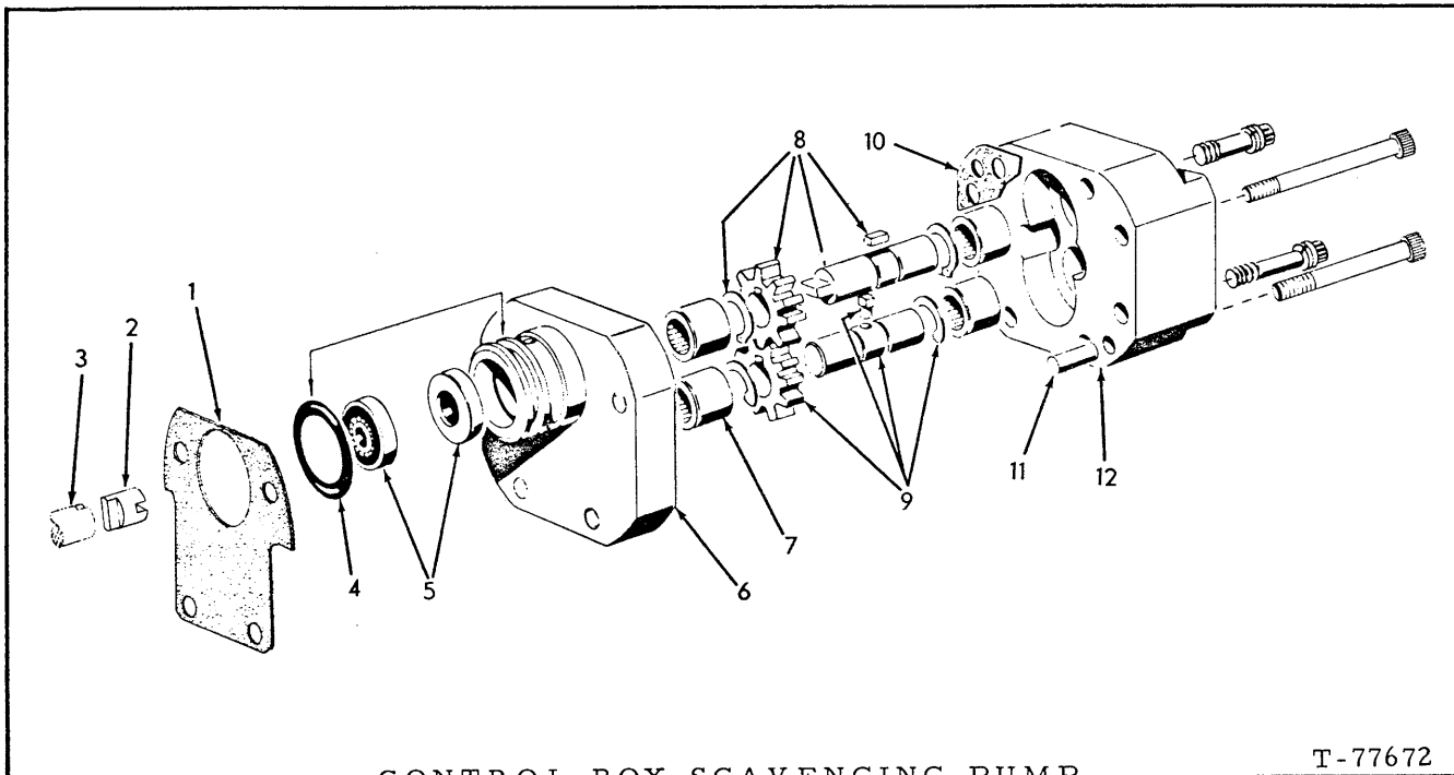
CONTROL BOX SCAVENGING PUMP
