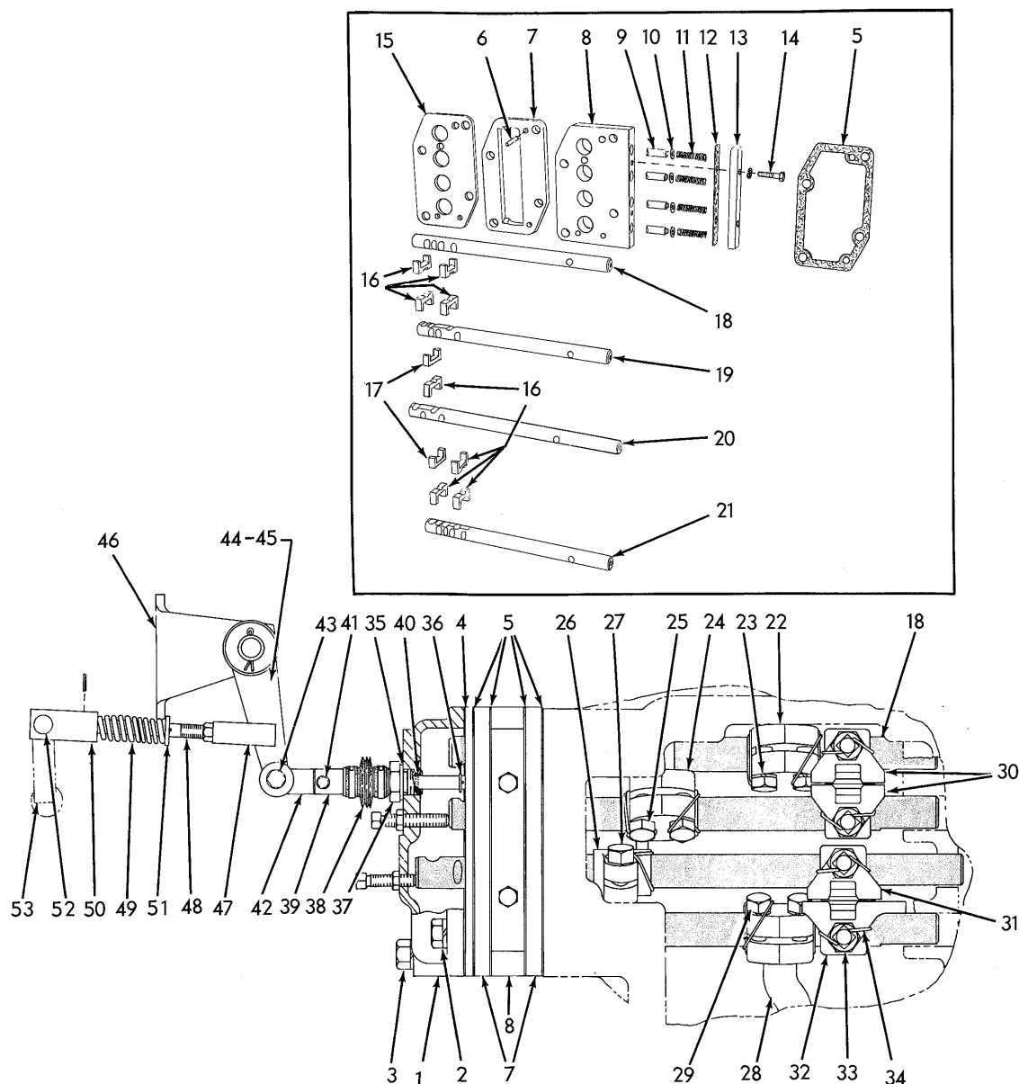
GEAR SHIFT FORKS AND LOCKS
