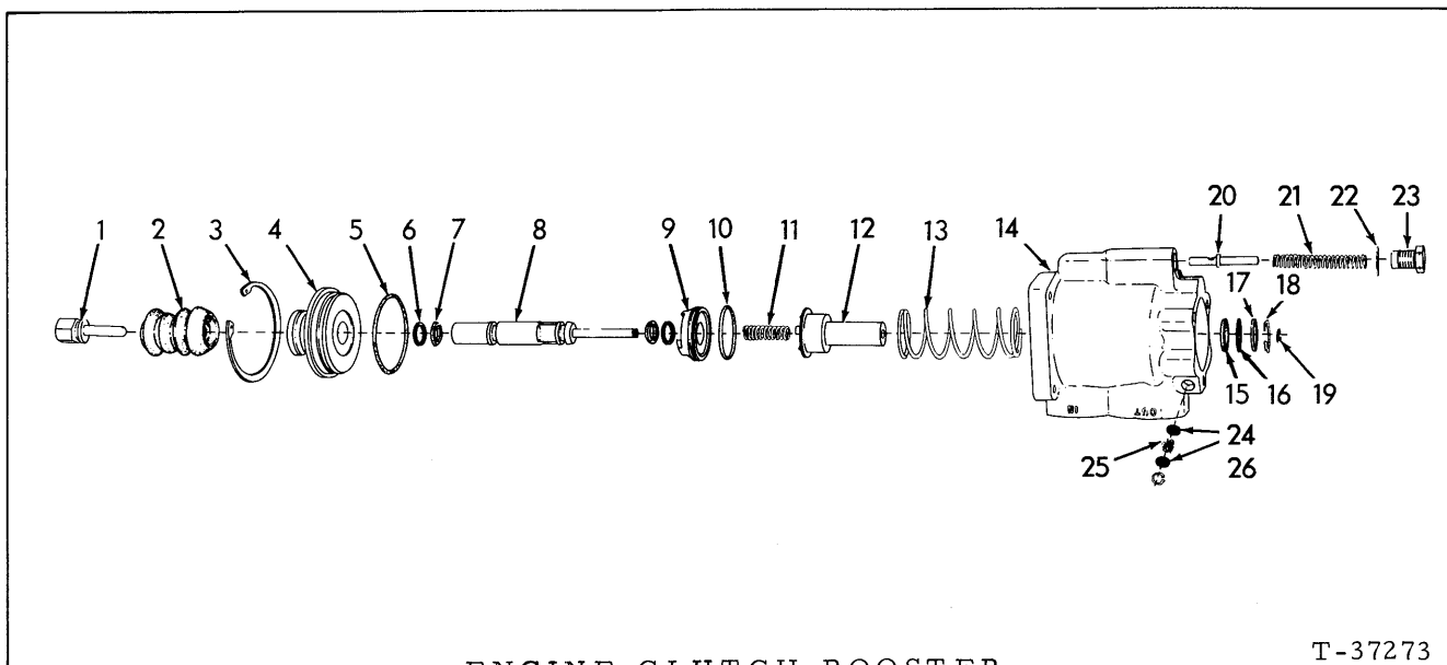
ENGINE CLUTCH BOOSTER
