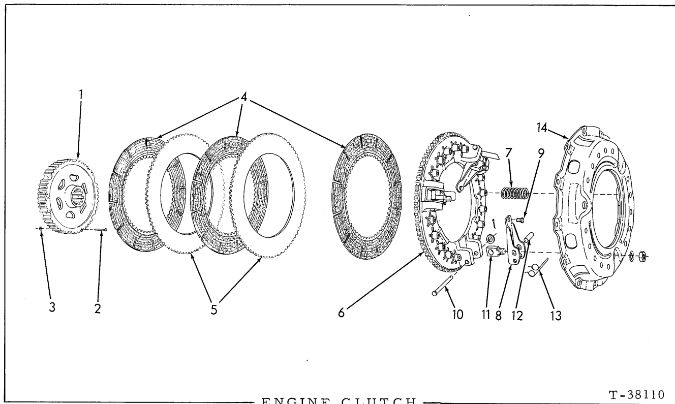
ENGINE CLUTCH
