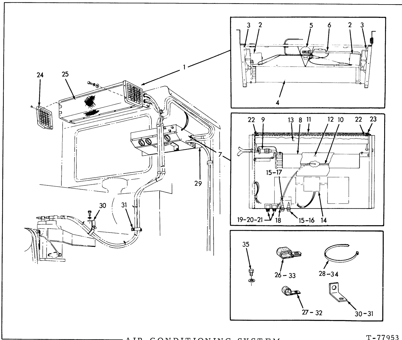
AIR CONDITIONING SYSTEM
