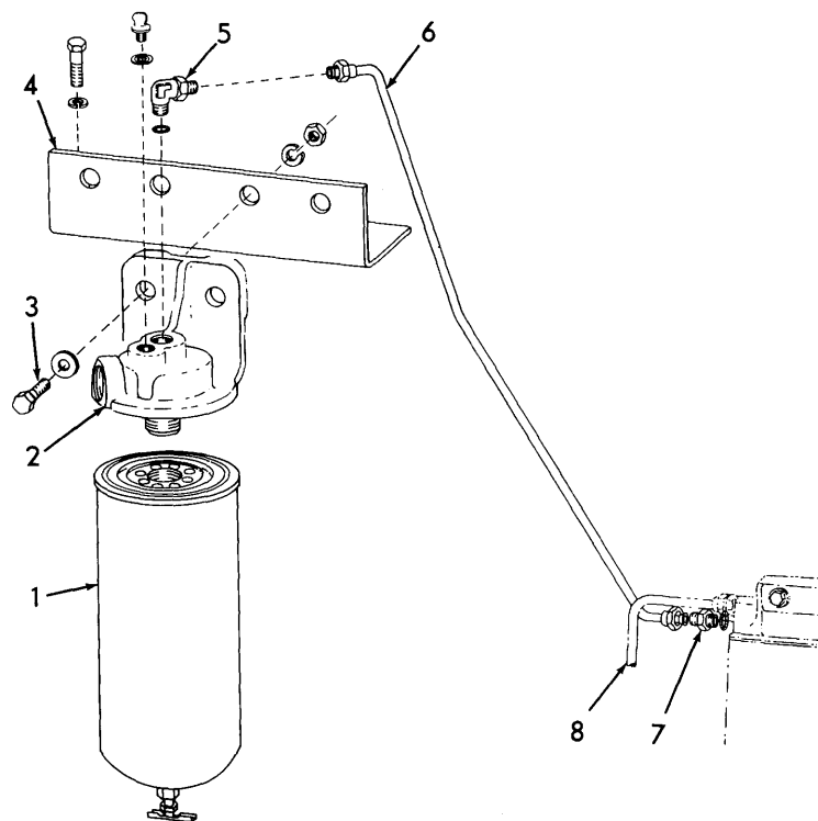
WATER SEPARATOR (Fuel)
