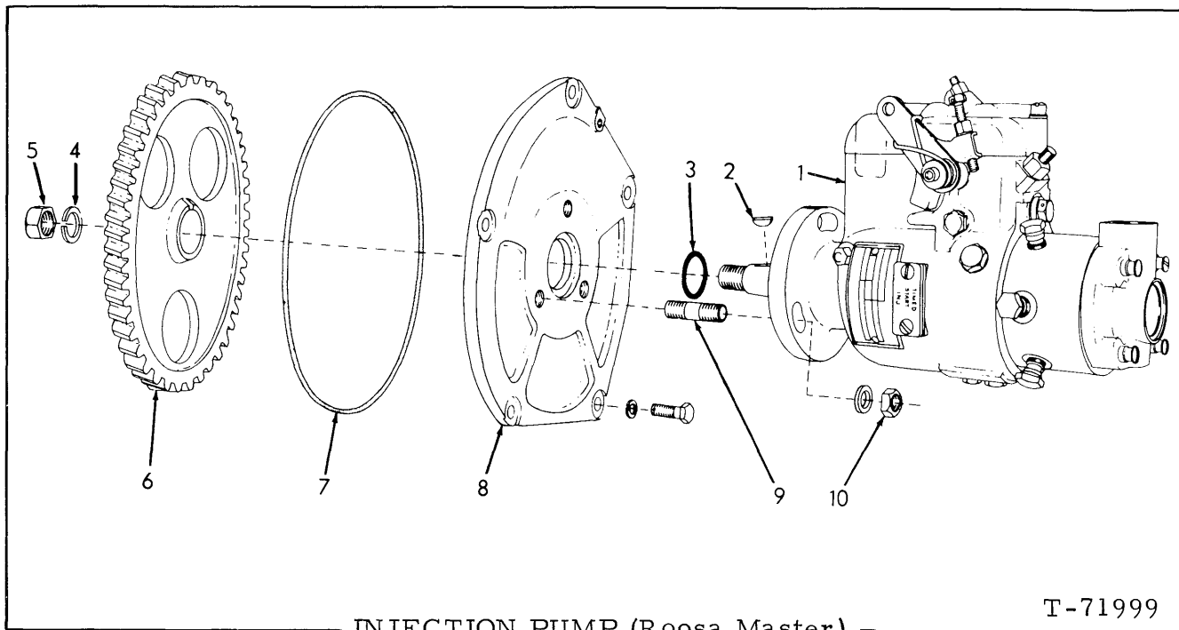
INJECTION PUMP (Roosa Master)
