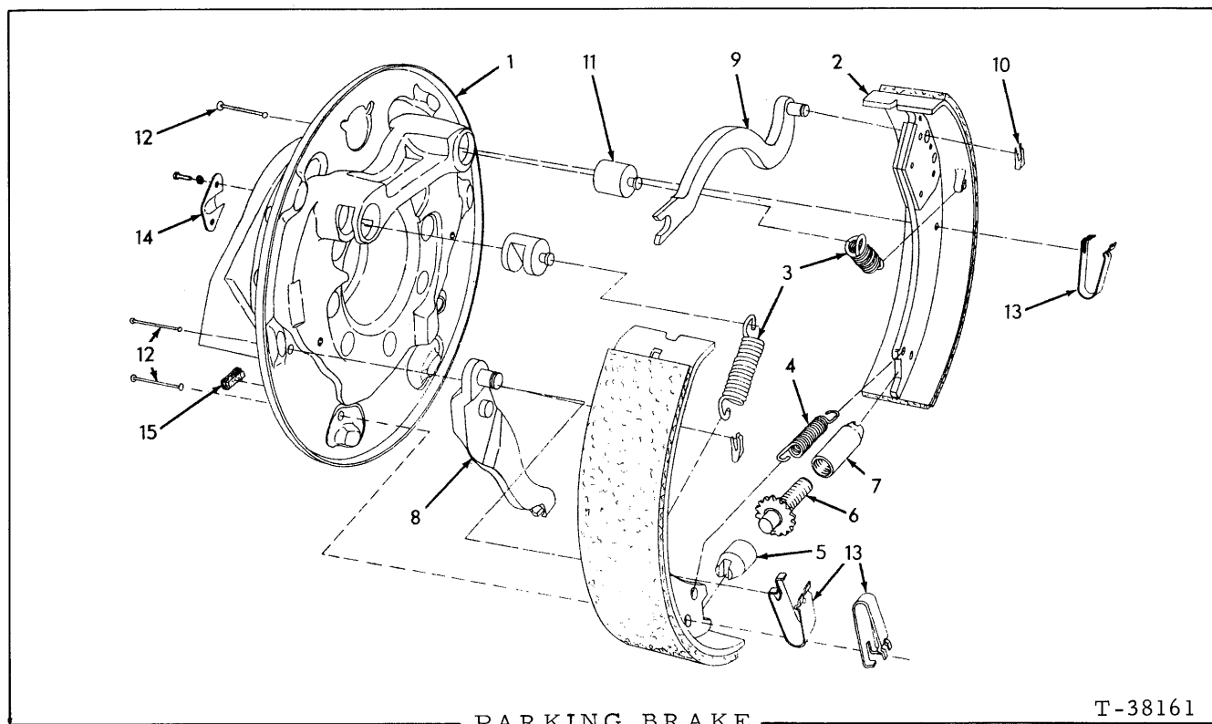
PARKING BRAKE
