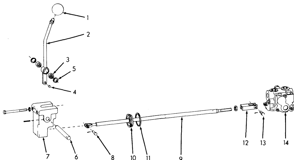
WHEEL LEAN CONTROL
