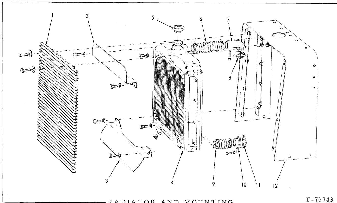
RADIATOR AND MOUNTING
