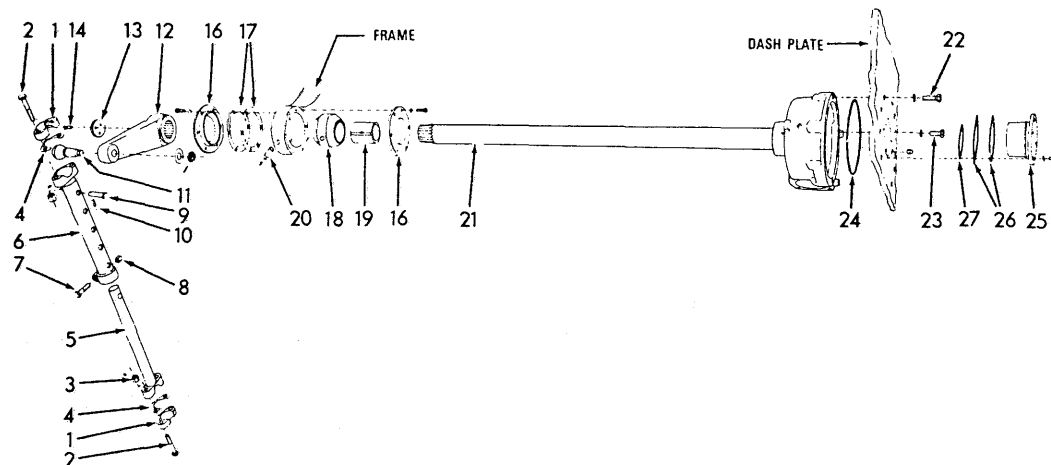
MOLDBOARD LIFT
