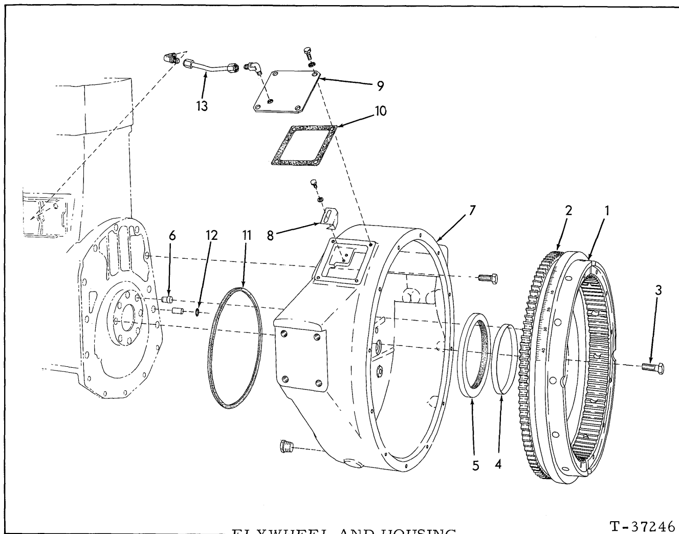
FLYWHEEL AND HOUSING
