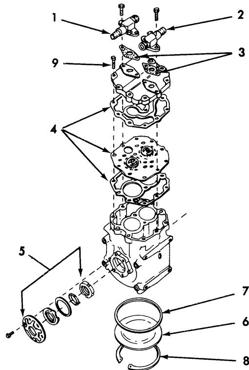
COMPRESSOR
