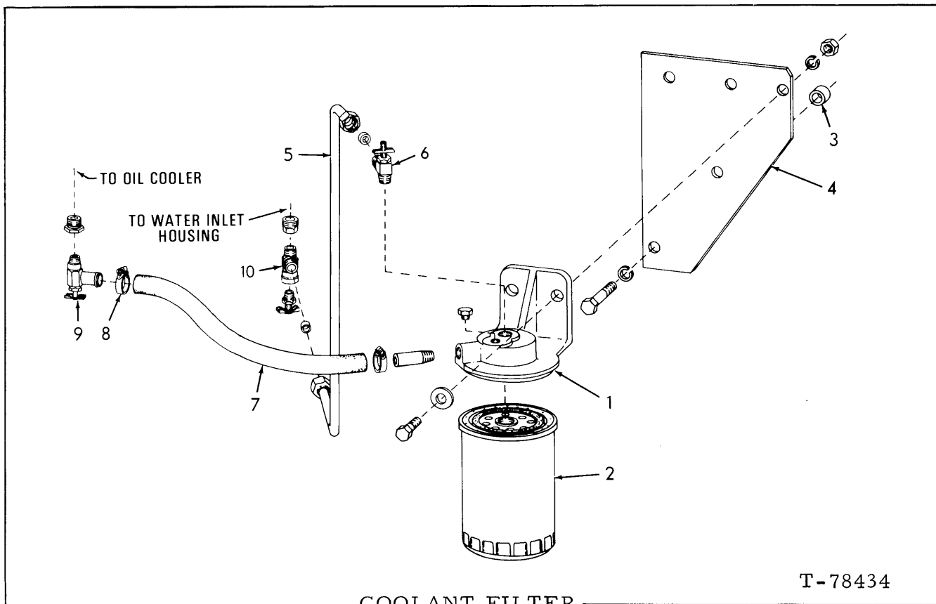
COOLANT FILTER
