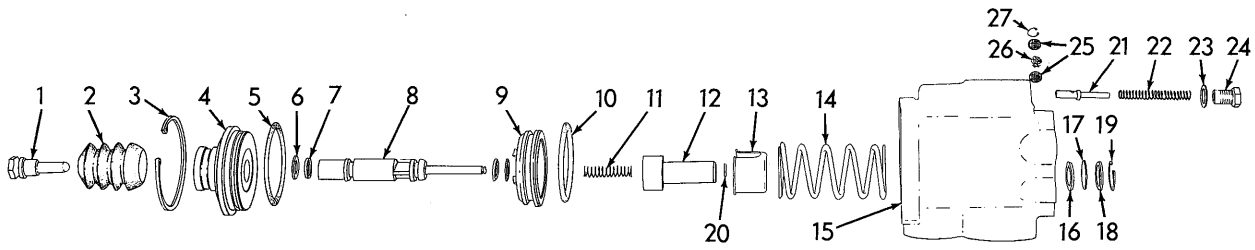
POWER BRAKE BOOSTER
