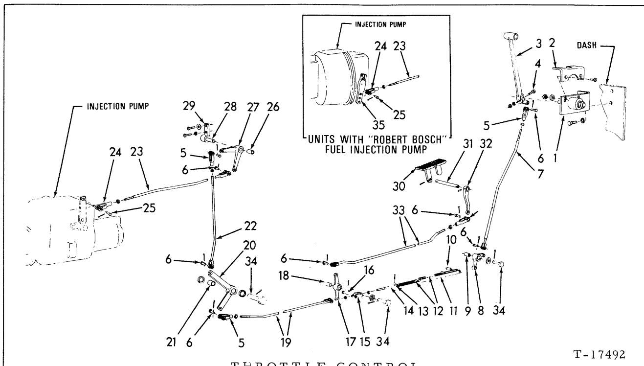
THROTTLE CONTROL
