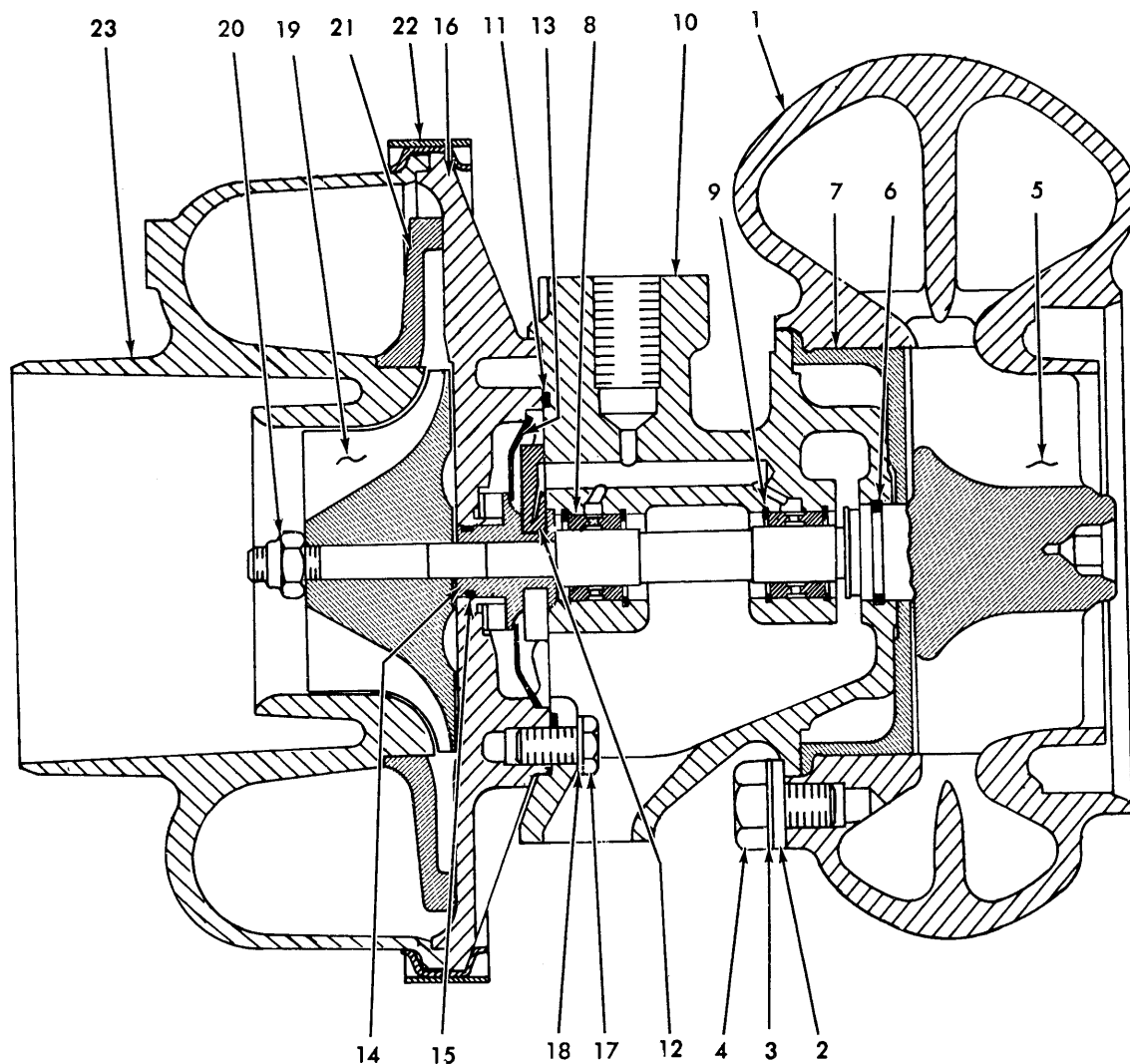
TURBOCHARGER ASSEMBLY
