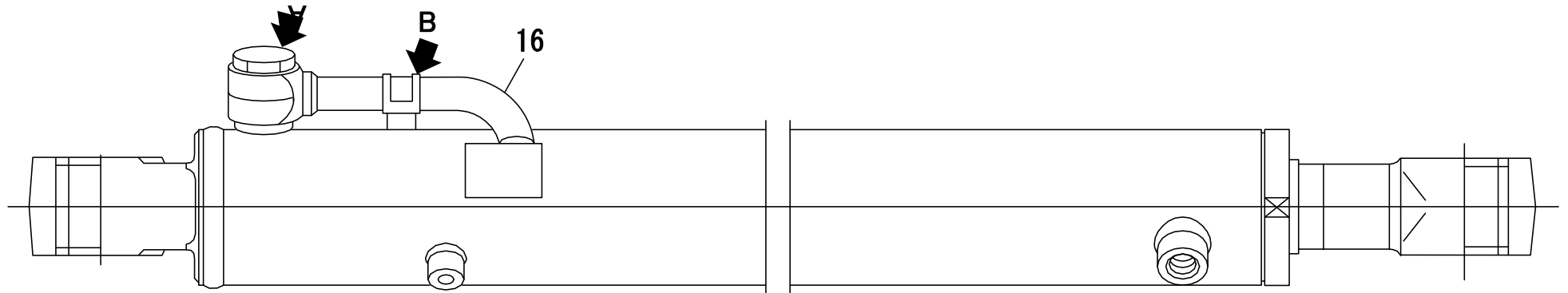
DETAIL "A"
