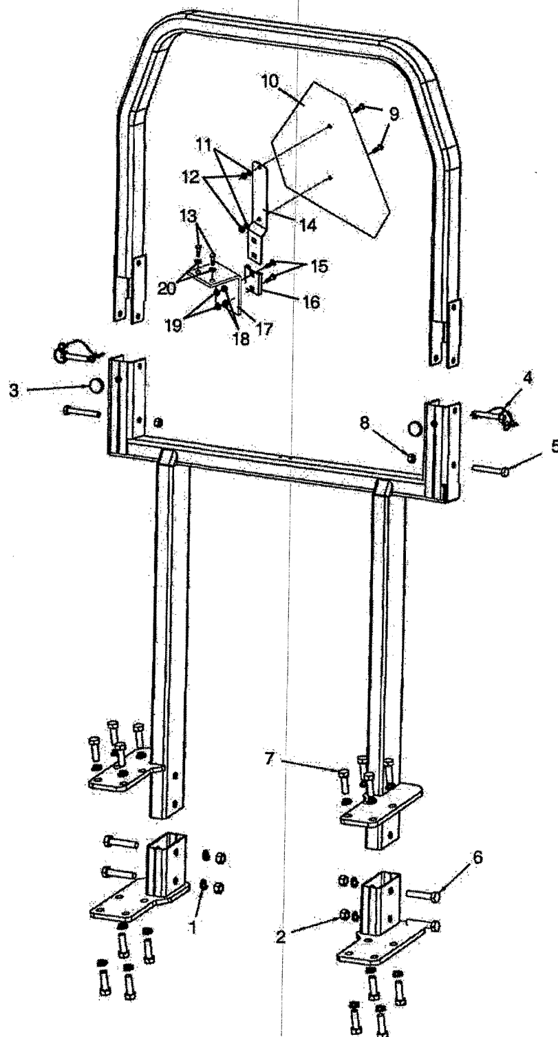
ROLLOVER PROTECTION STRUCTURE & SMV SIGN
