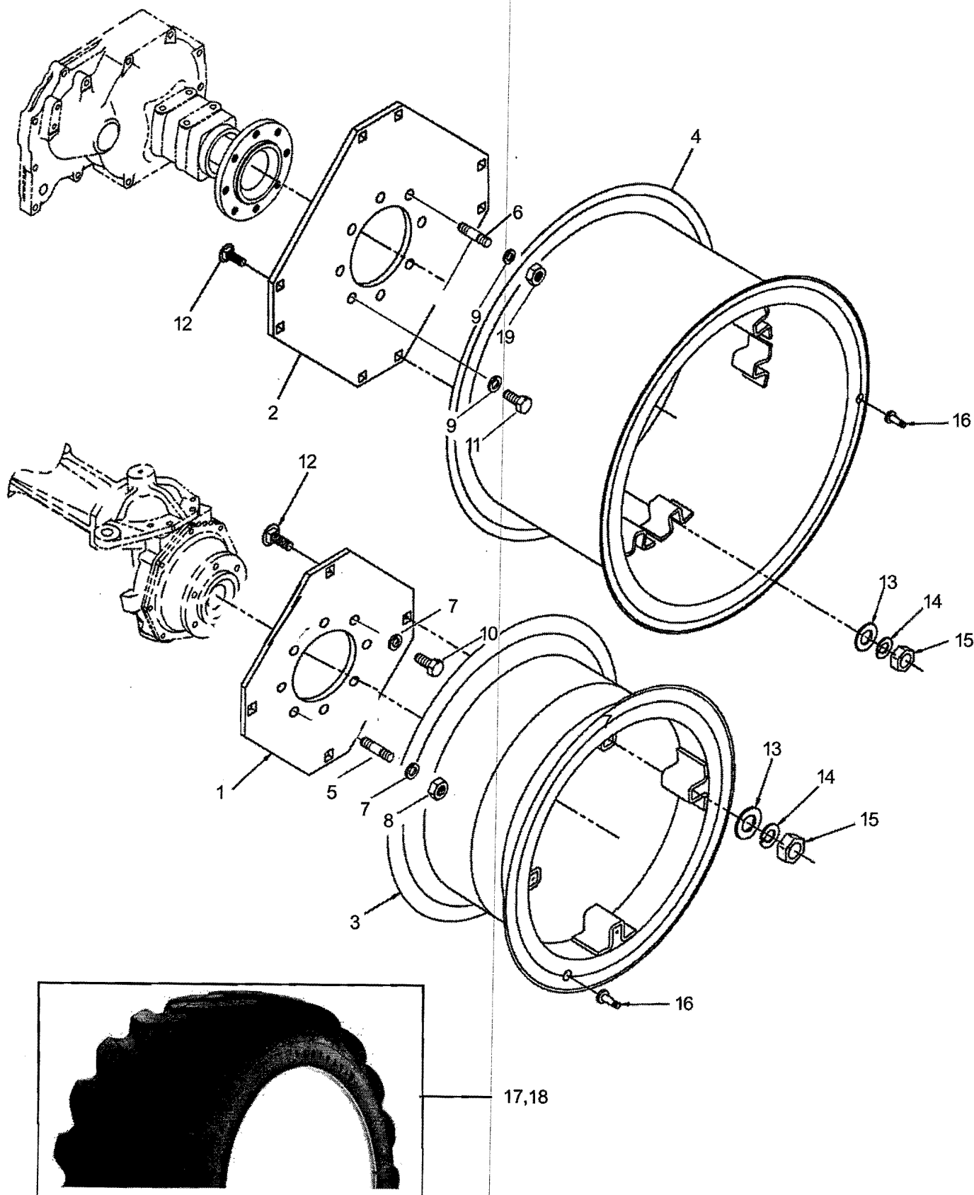
INDUSTRIAL TIRE & RIM ASSEMBLY - 8 HOLE AXLE - 4 WD
