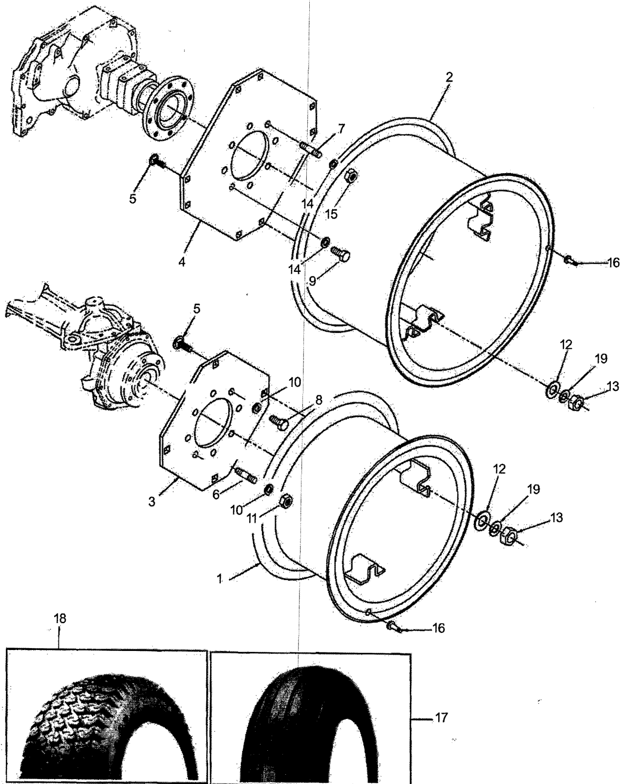
TURF TIRE & RIM ASSEMBLY 1 - 8 HOLE AXLE - 4 WD
