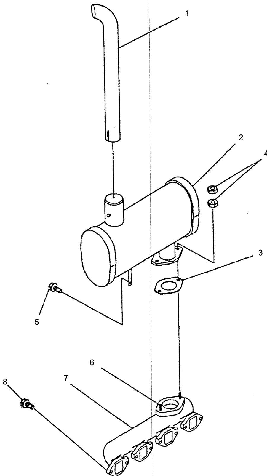
EXHAUST ASSEMBLY
