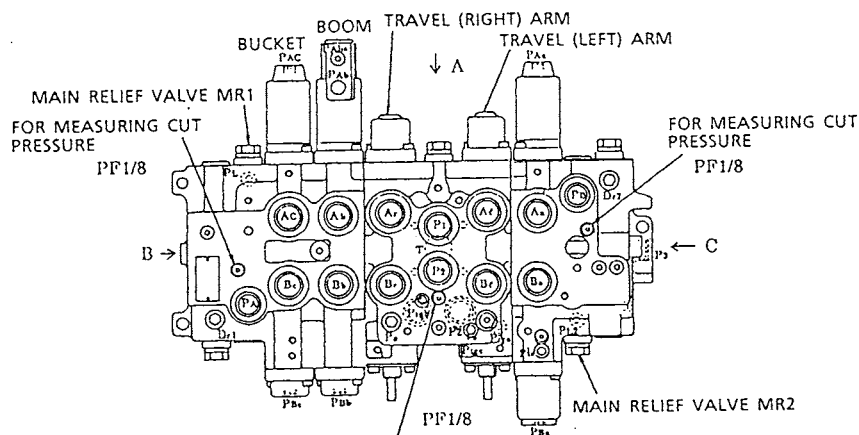
FOR MEASURING PRIORITY PRESSURE Outside view of main control valve
