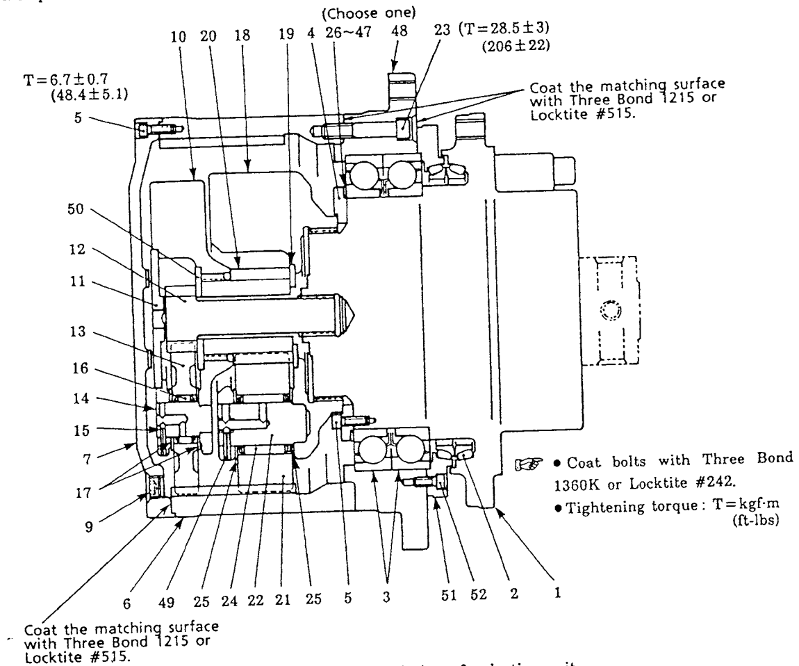
Cross-sectional view of reduction unit.
