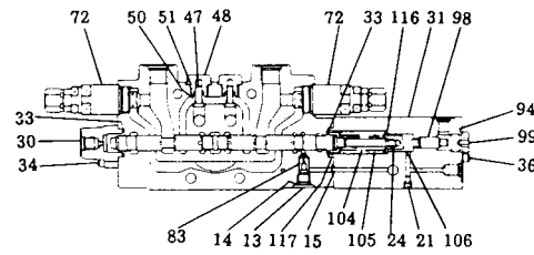
SECTION K - K
