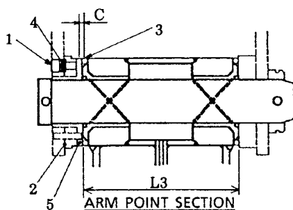
ARM POINT SECTION
