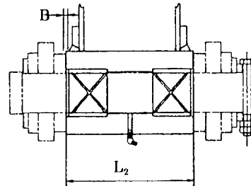
ARM CENTER SECTION
