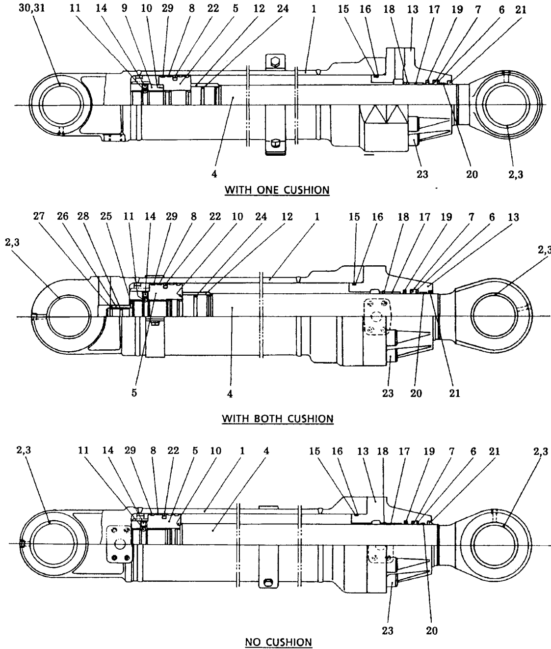
Cross-sectional view of cylinder
