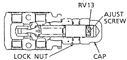
Pilot pressure measuring port and the pilot relief valve for adjustment
