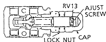
The pilot relief valve for adjustment
