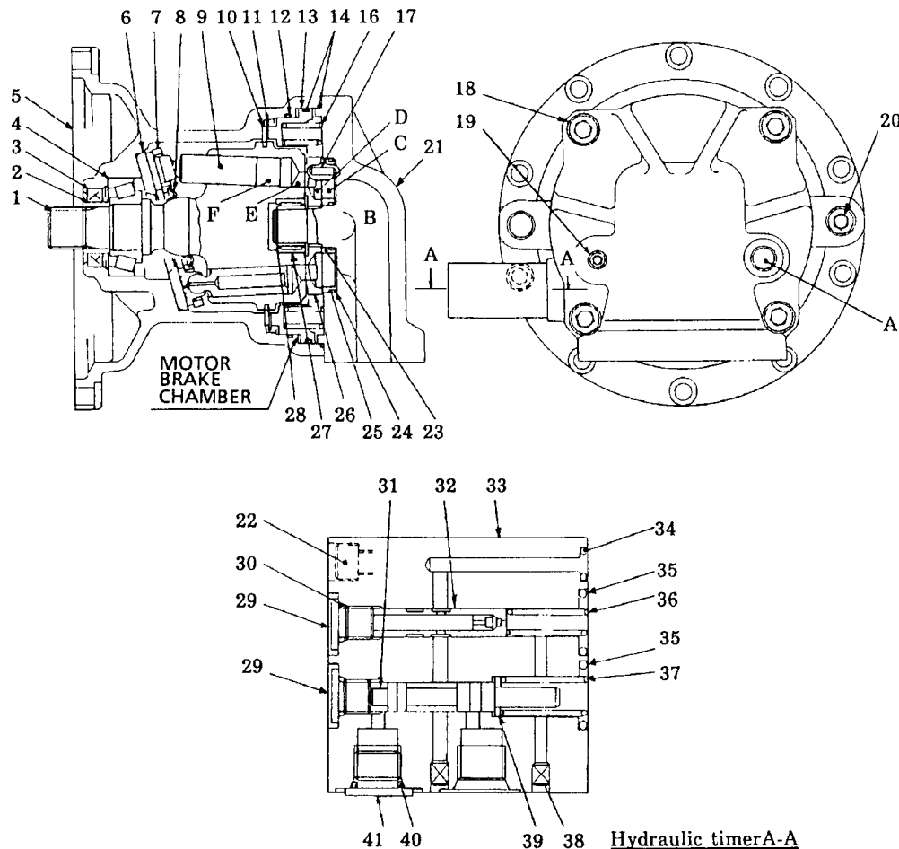
Cross-sectional view of swing motor
