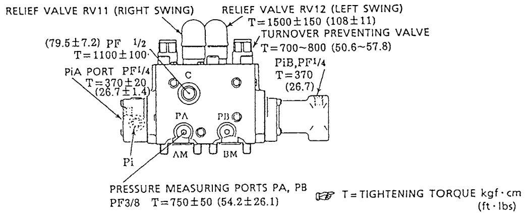
Outside view of swing control valve
