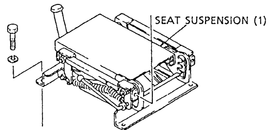
Removing the operator seat
