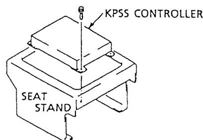
Mounted position of mechatro controller
