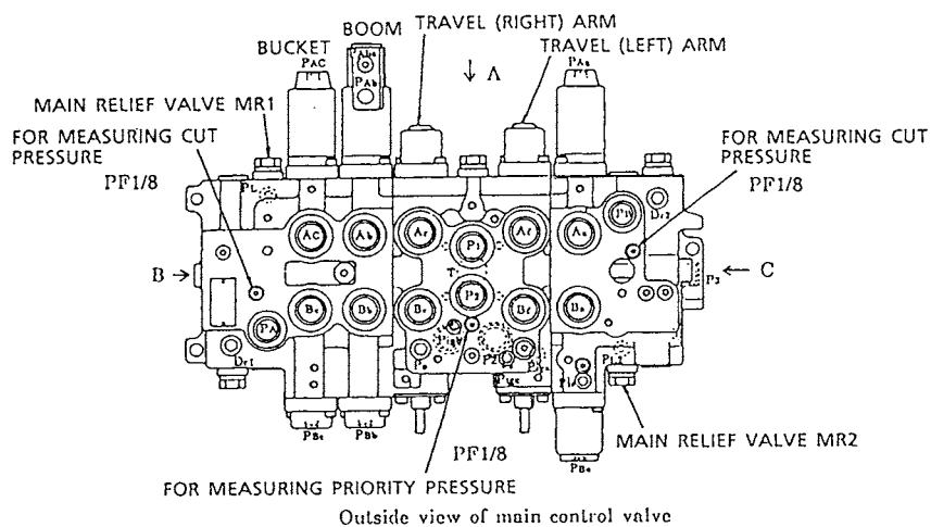
Outside view of main control valve
