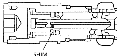
Swing relief valve
