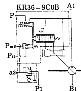
HYDRAULIC CIRCUIT DIAGRAM
