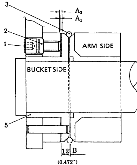
How to adjust clearance B
