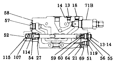
SECTION L - L
