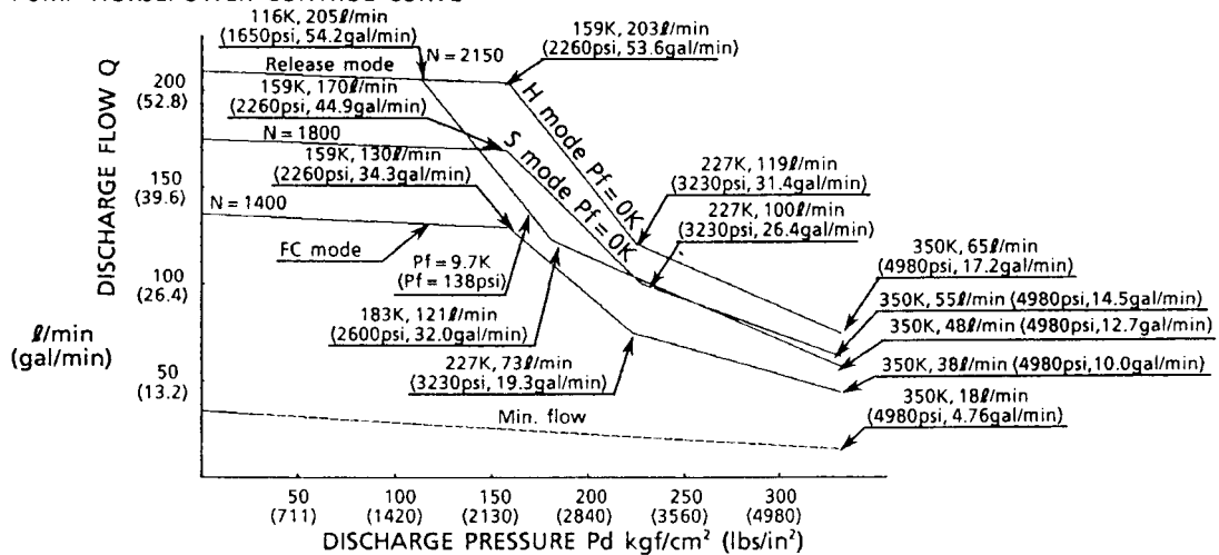
ONE PUMP HORSEPOWER CONTROL CURVE
