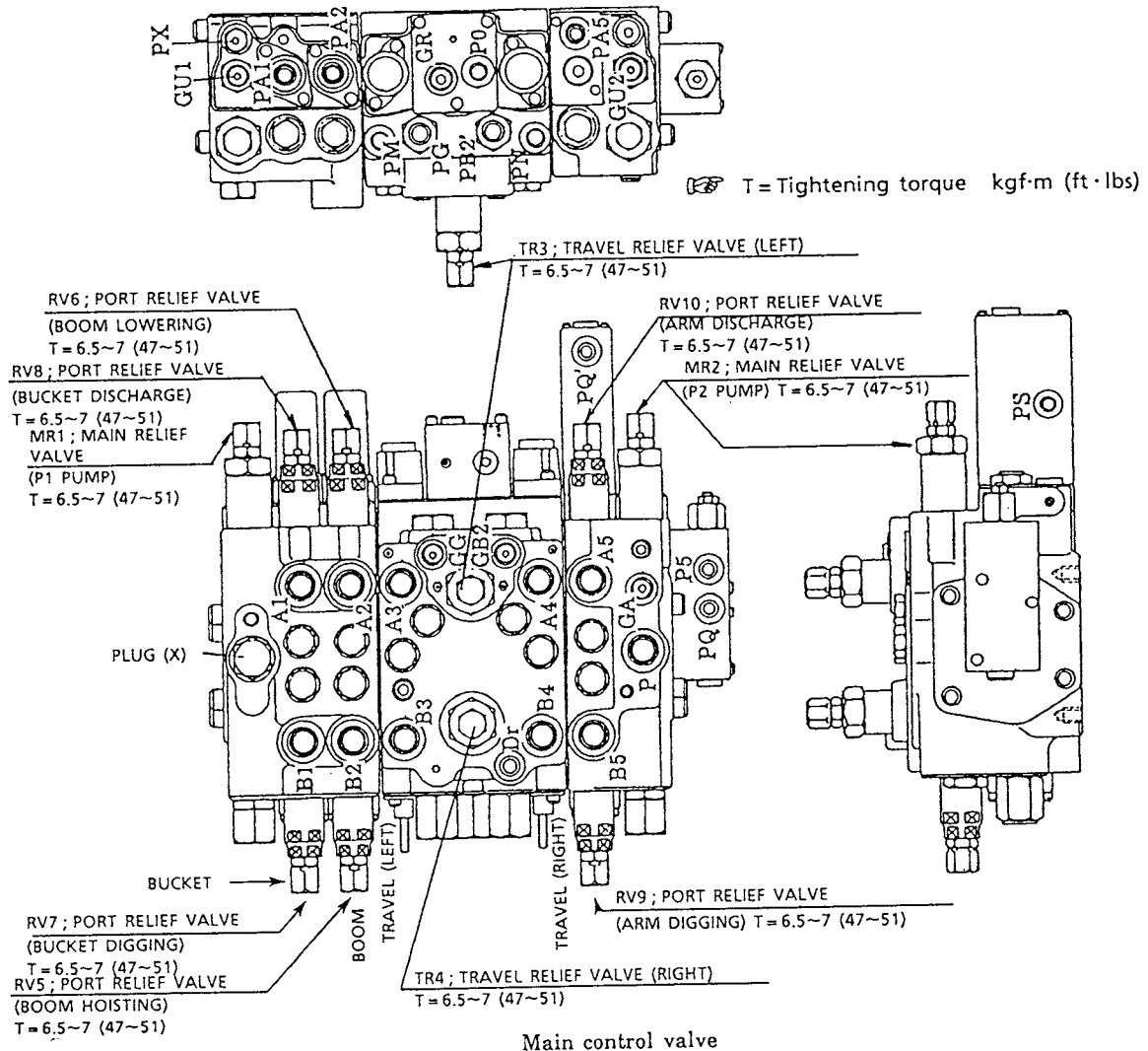
Main control valve
