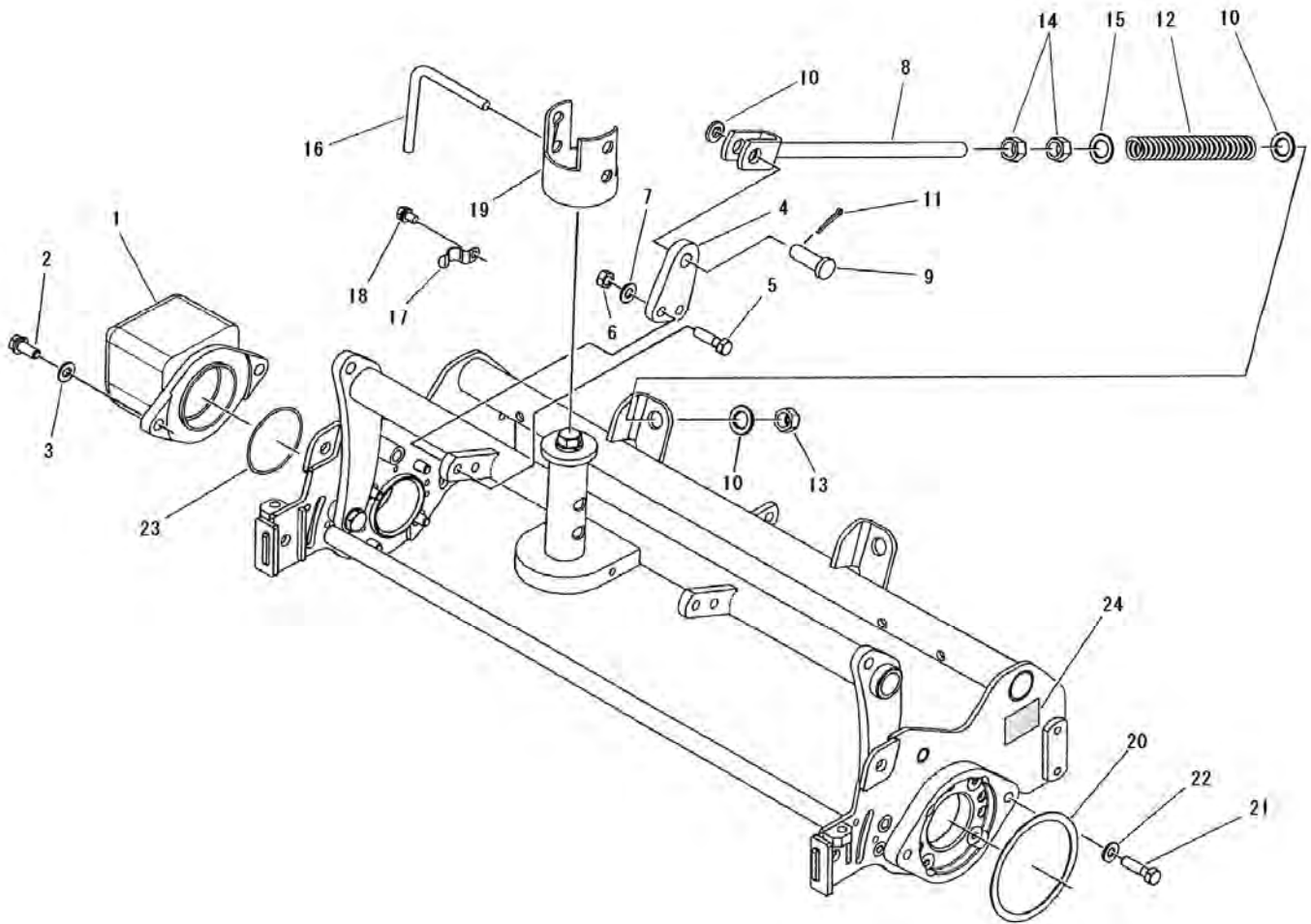
FIG.320 ACCESSORY (F7/FD7) フソクビン (F7/FD7)
