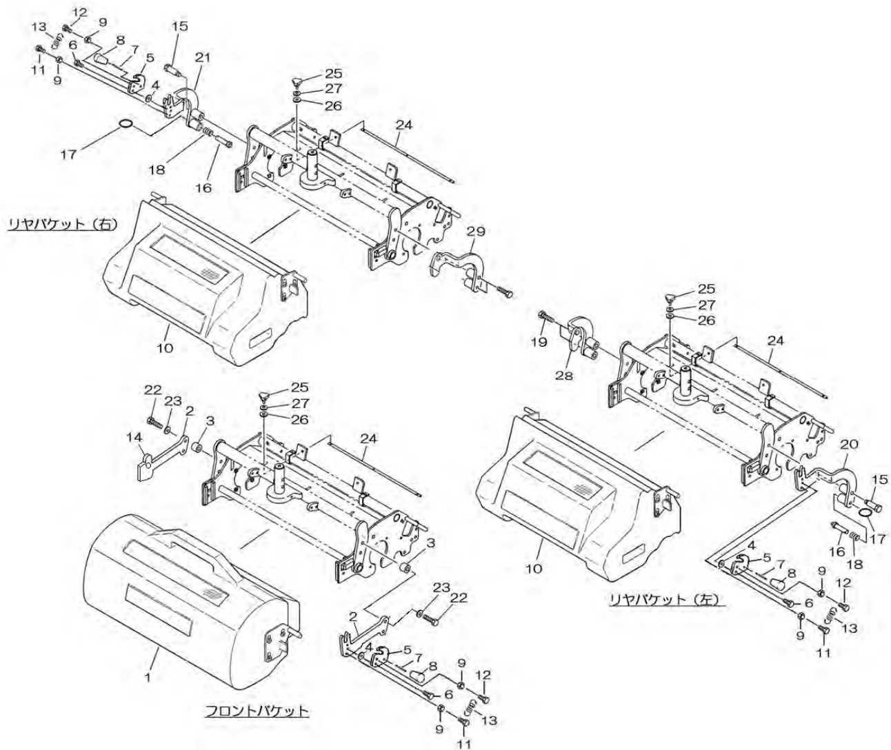
FIG.306 BUCKET ASSY (S7/S9/S11) バケットASSY (S7/S9/S11)
