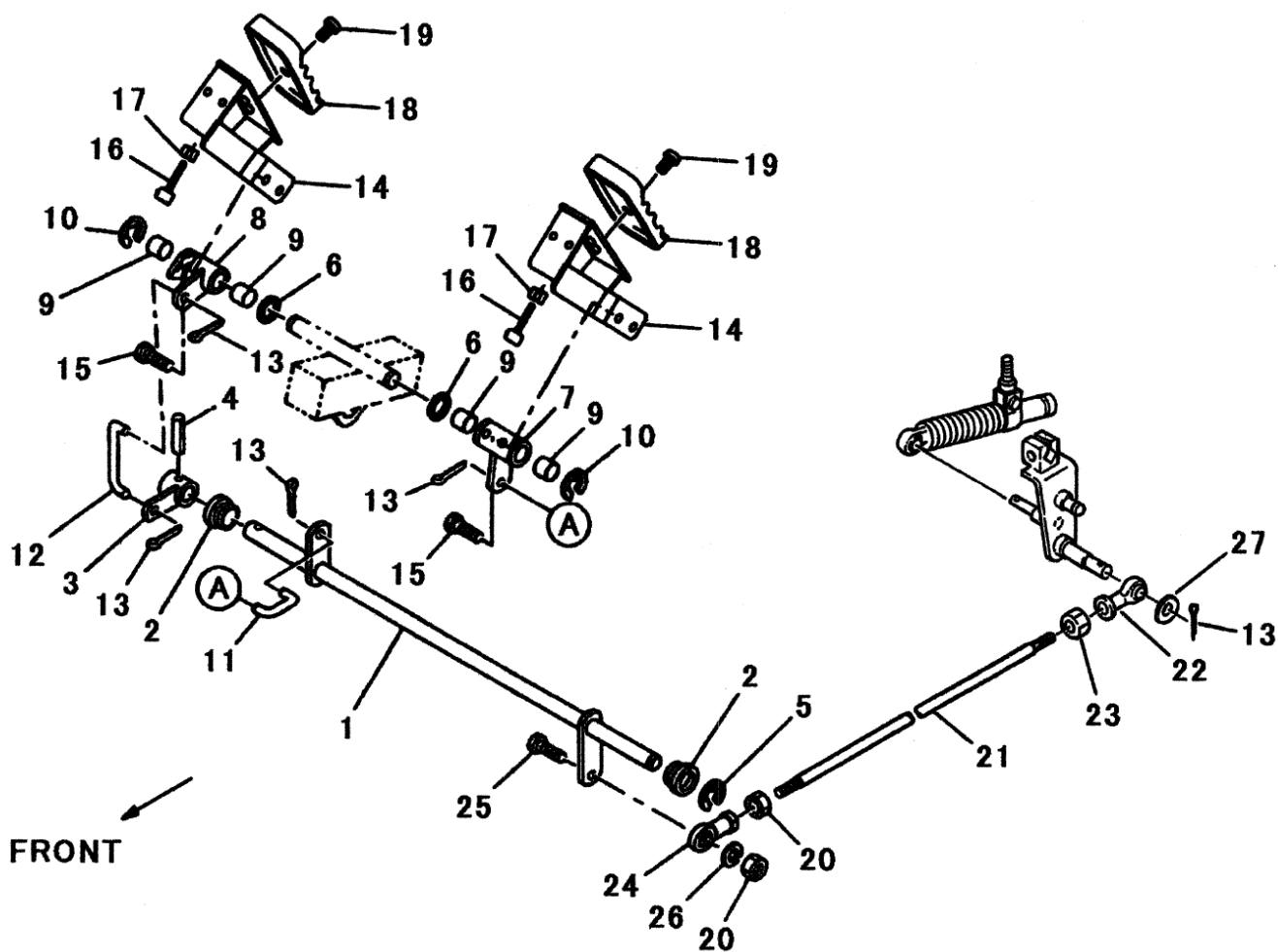
FIG.213 PEDALS, HYDROSTATIC TRANSMISSION H. S. Tペダル
