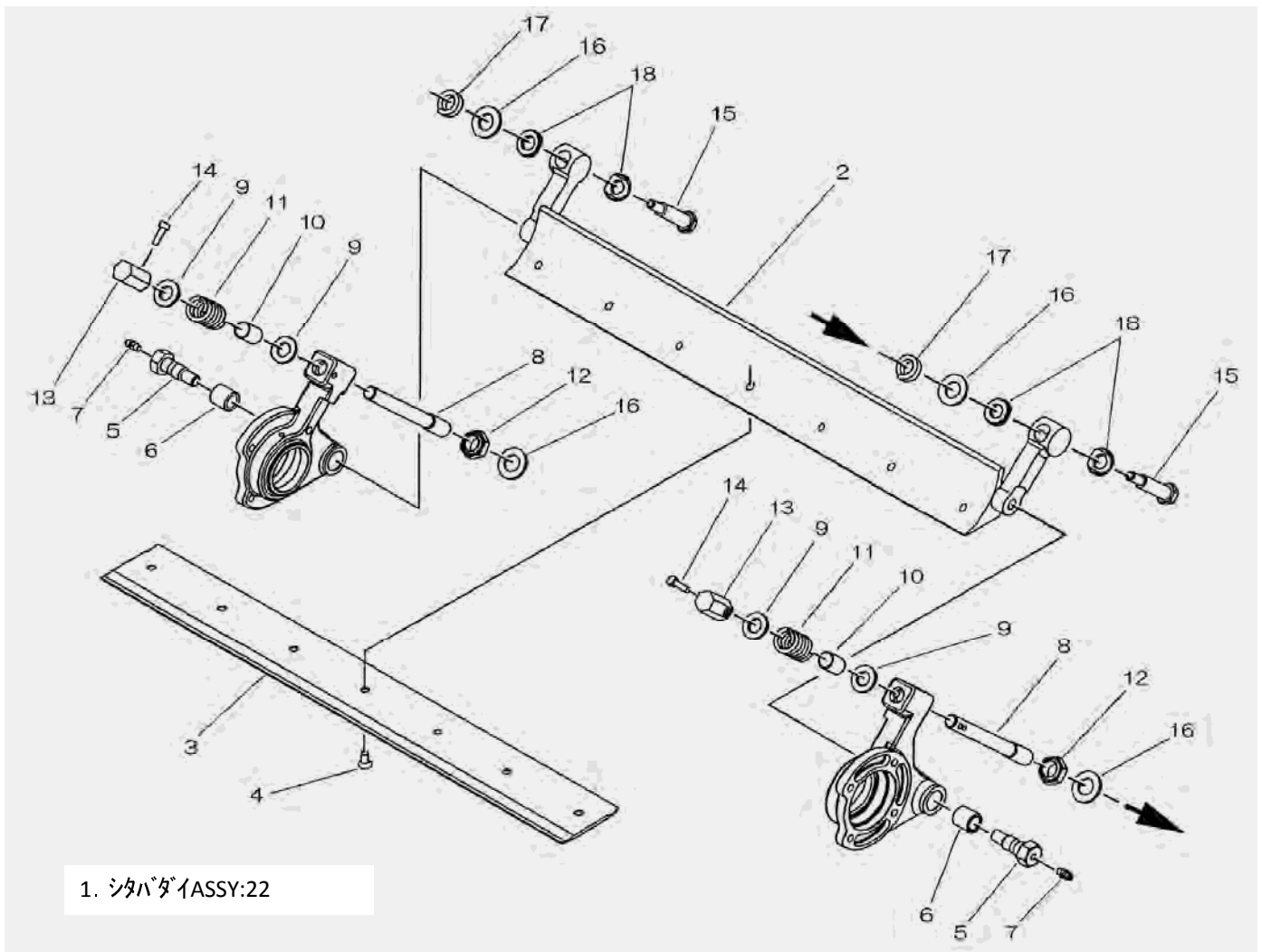
FIG.9 F7 BED KNIFE (F7/FD7) ベッドナイフ (F7/FD7)
