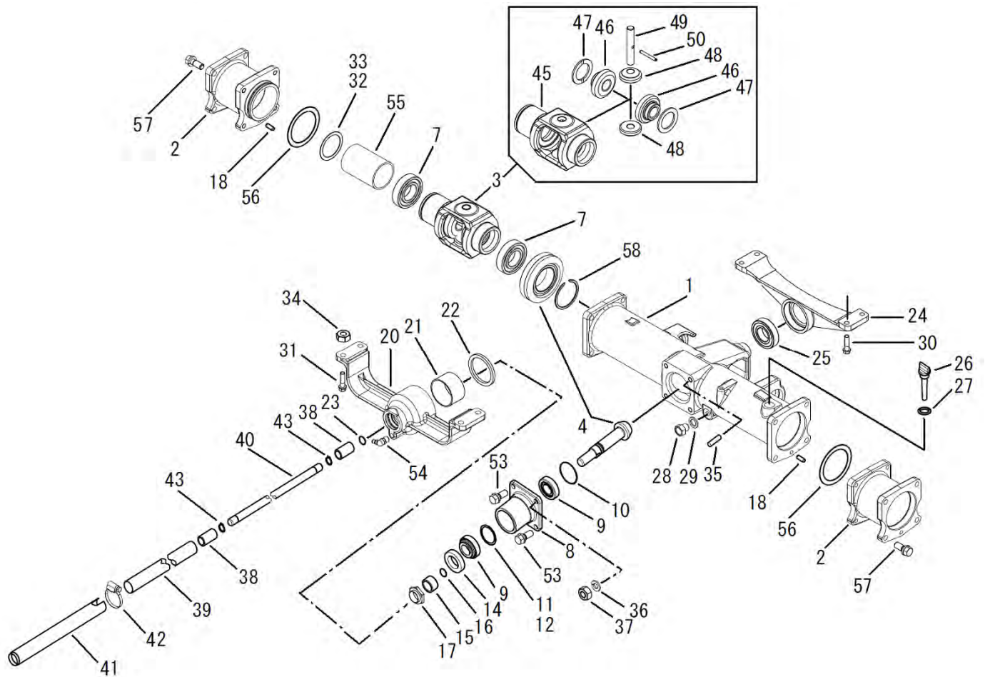
FIG.211-B REAR AXLE, DIFFERENTIAL & HOUSING リヤアクスル、デフ
