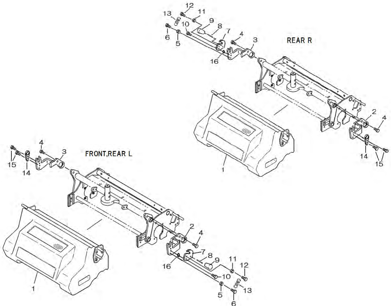
FIG.324 BUCKET ASSY (F7/FD7) バケットASSY (F7/FD7)
