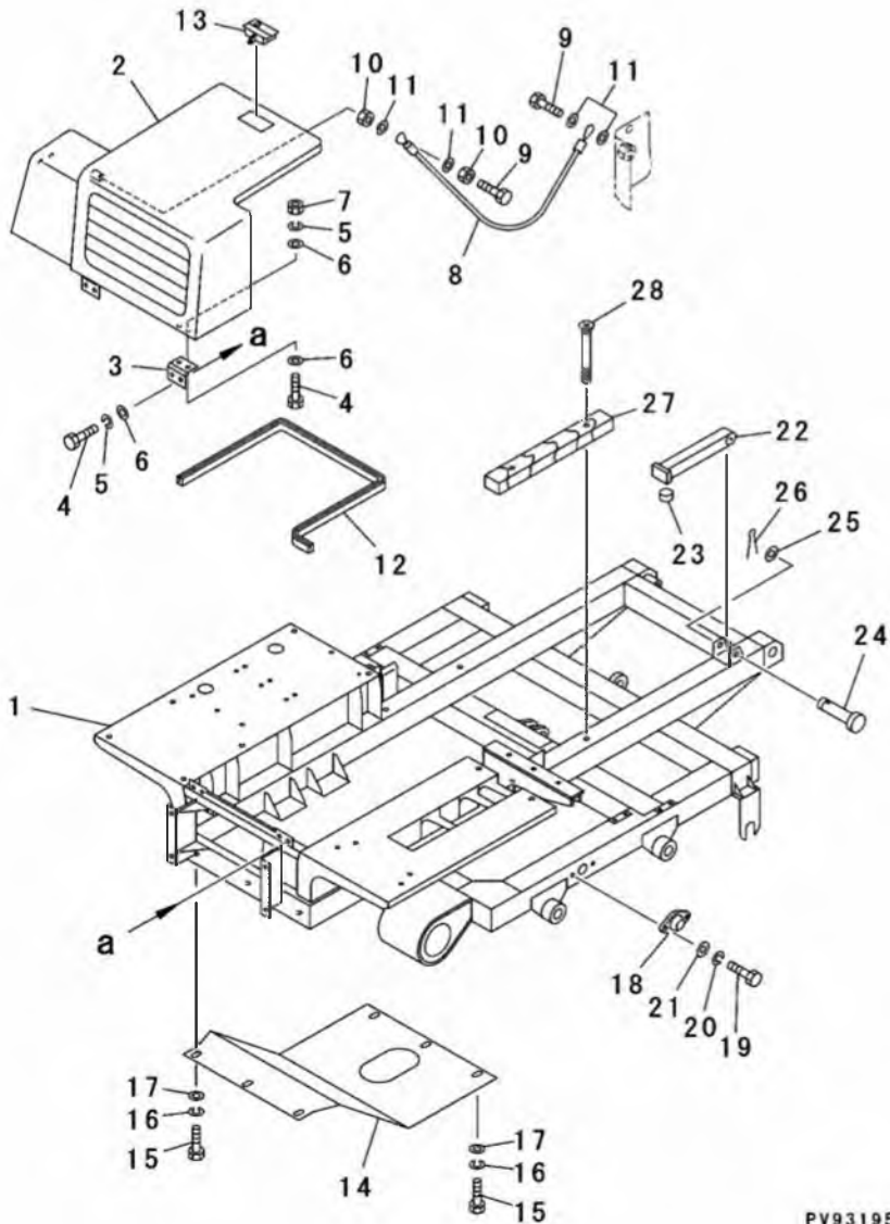
FIG. 201A FRAME RELATED PARTS (1/3) (BONNET AND UNDER COVER) (APPLICABLE TO MST-300VD) (SERIAL NO.3981-)
