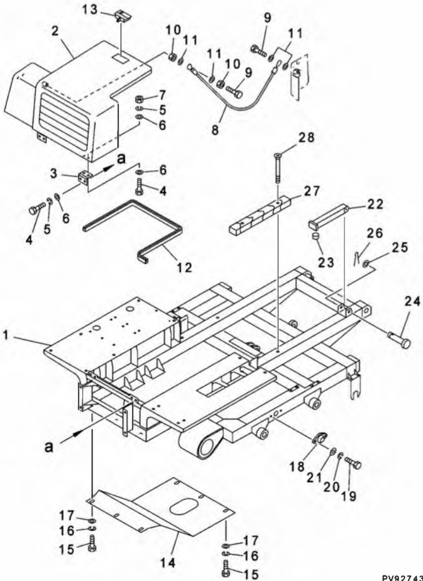
FIG. 201 FRAME RELATED PARTS (1/3) (BONNET AND UNDER COVER) (APPLICABLE TO MST-300VD) (SERIAL NO.3401-3980)
