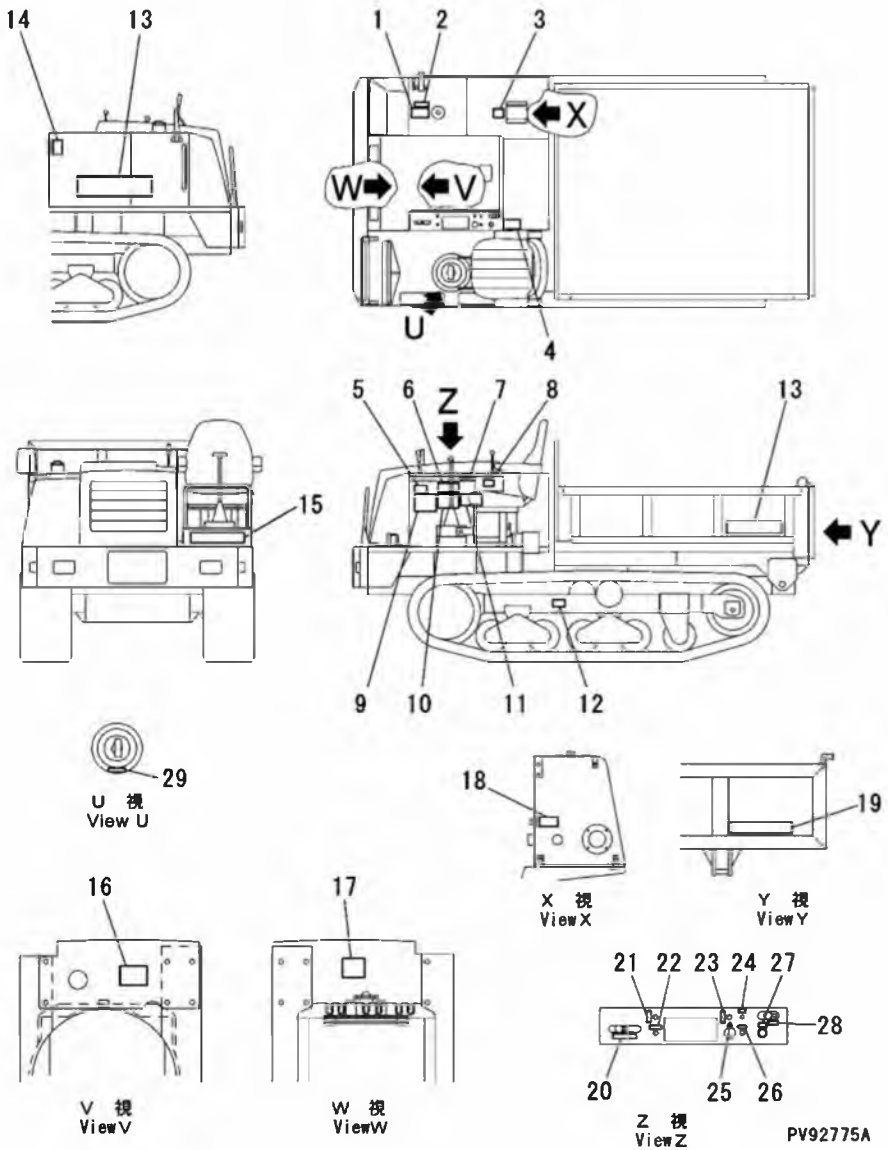
FIG. 801 MARKS AND PLATES (JAPANESE) (SERIAL NO.3401-3980)
