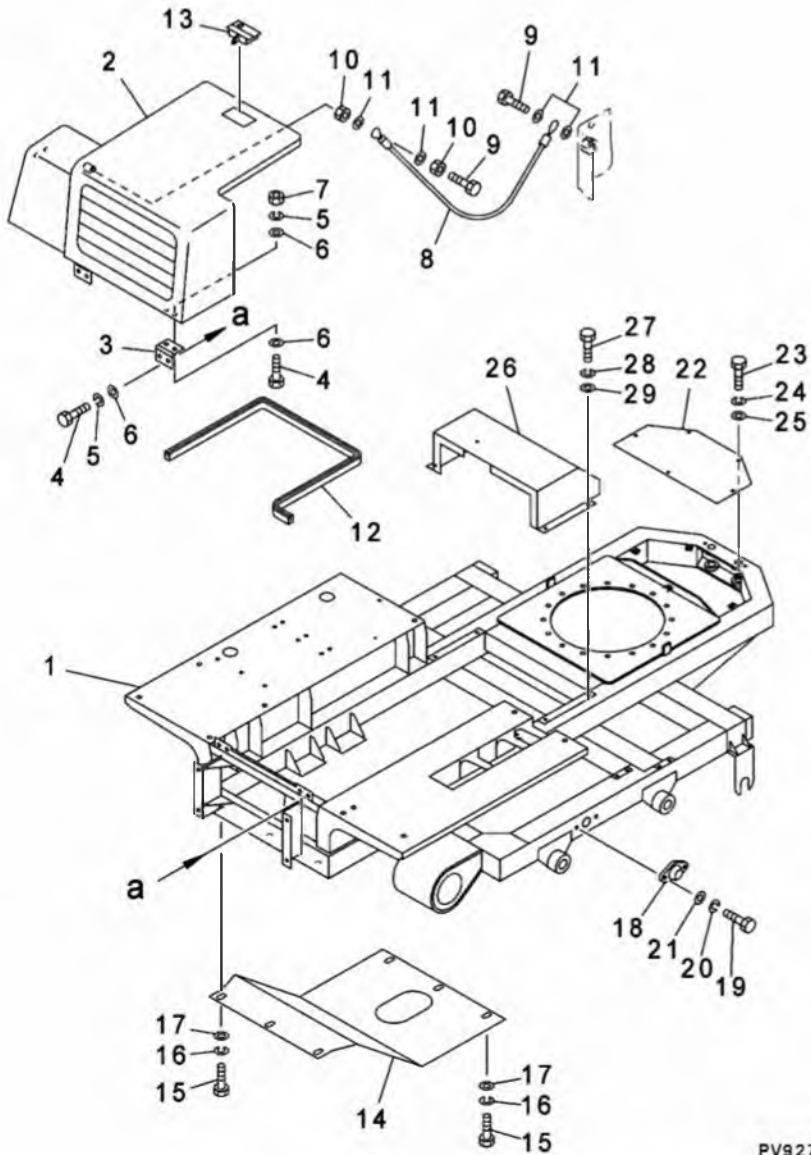
FIG. 202 FRAME RELATED PARTS (1/3) (BONNET AND UNDER COVER) (APPLICABLE TO MST-300VDR) (SERIAL NO.3401-3980)
