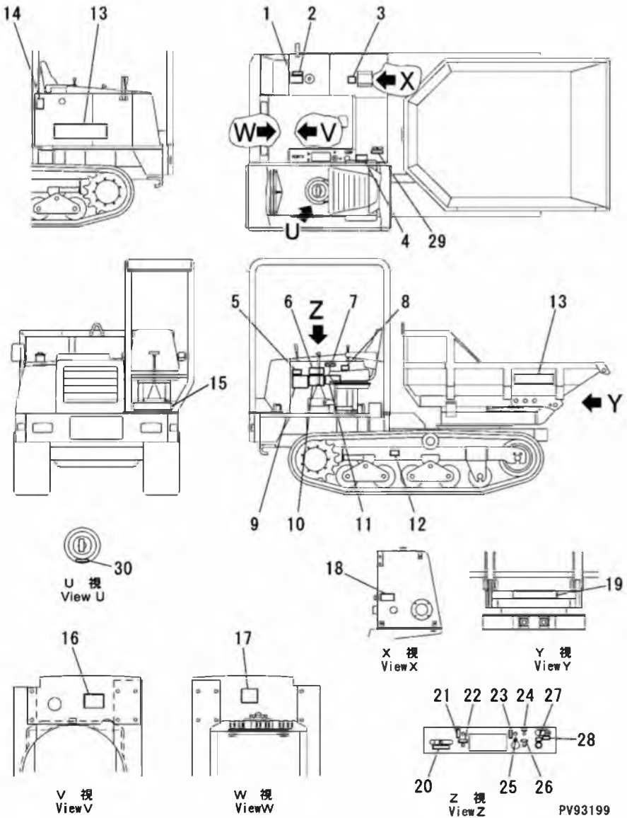
FIG. 802A MARKS AND PLATES (JAPANESE) (APPLICABLE TO MST-300VDR) (SERIAL NO.3981-)
