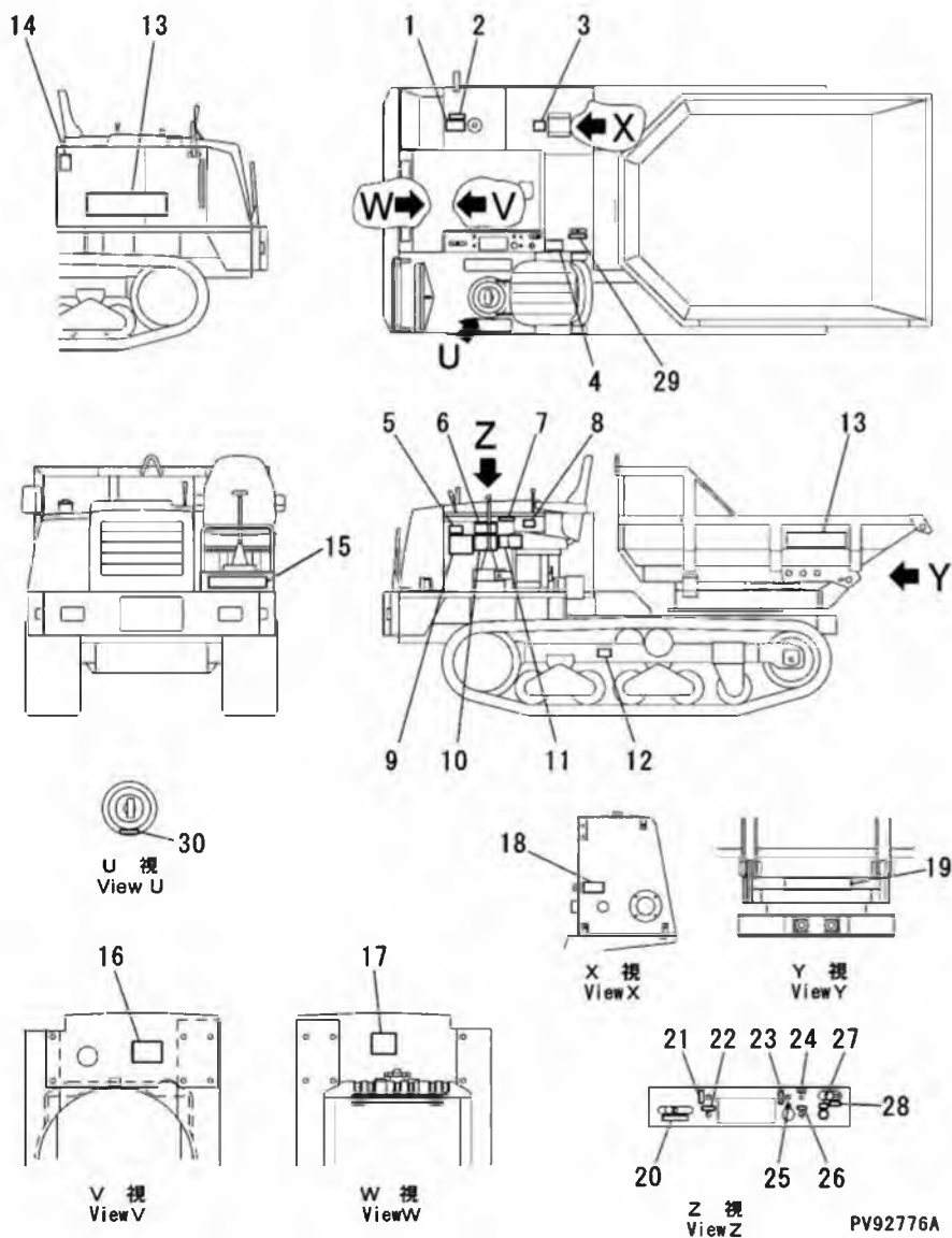
FIG. 802 MARKS AND PLATES (JAPANESE) (APPLICABLE TO MST-300VDR) (SERIAL NO.3401-3980)
