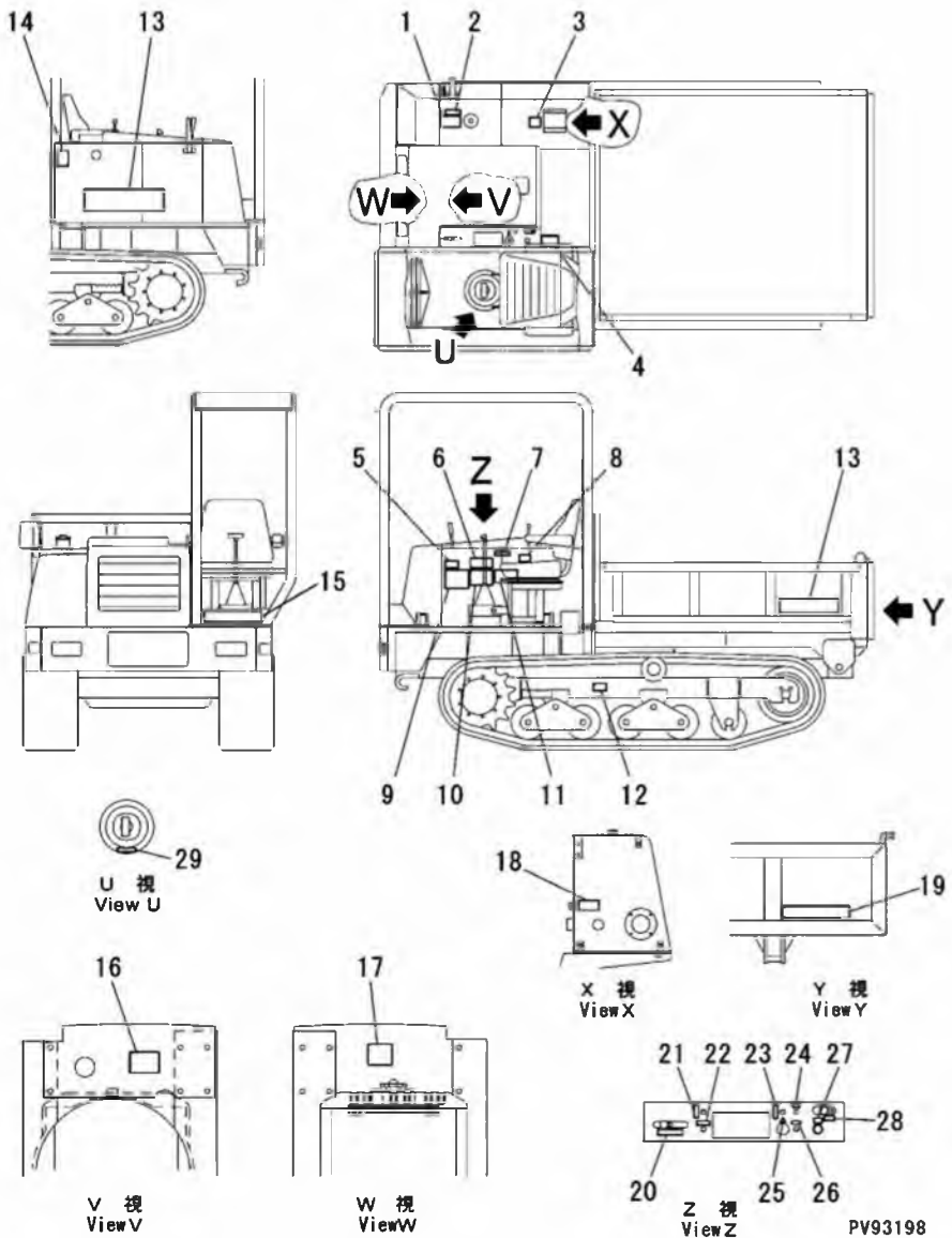
FIG. 801A MARKS AND PLATES (JAPANESE) (SERIAL NO.3981-)
