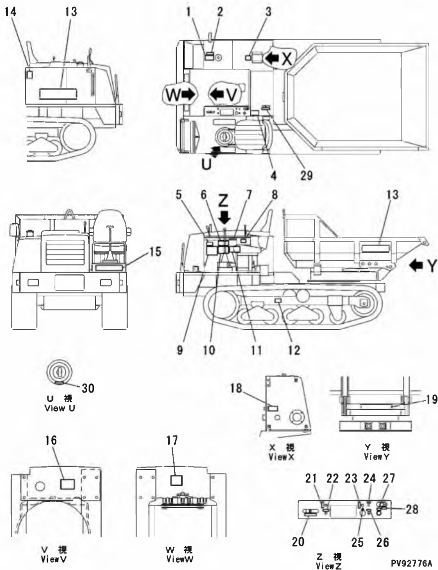
FIG. 812 MARKS AND PLATES (ENGLISH) (APPLICABLE TO MST-300VDR) (SERIAL NO.3401-3980)
