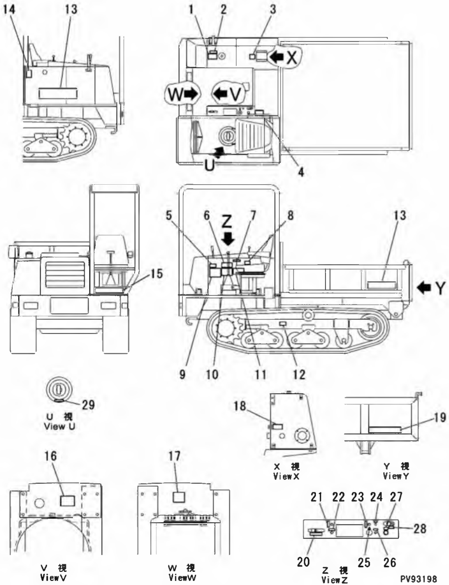
FIG. 811A MARKS AND PLATES (ENGLISH) (APPLICABLE TO MST-300VD) (SERIAL NO.3981-)
