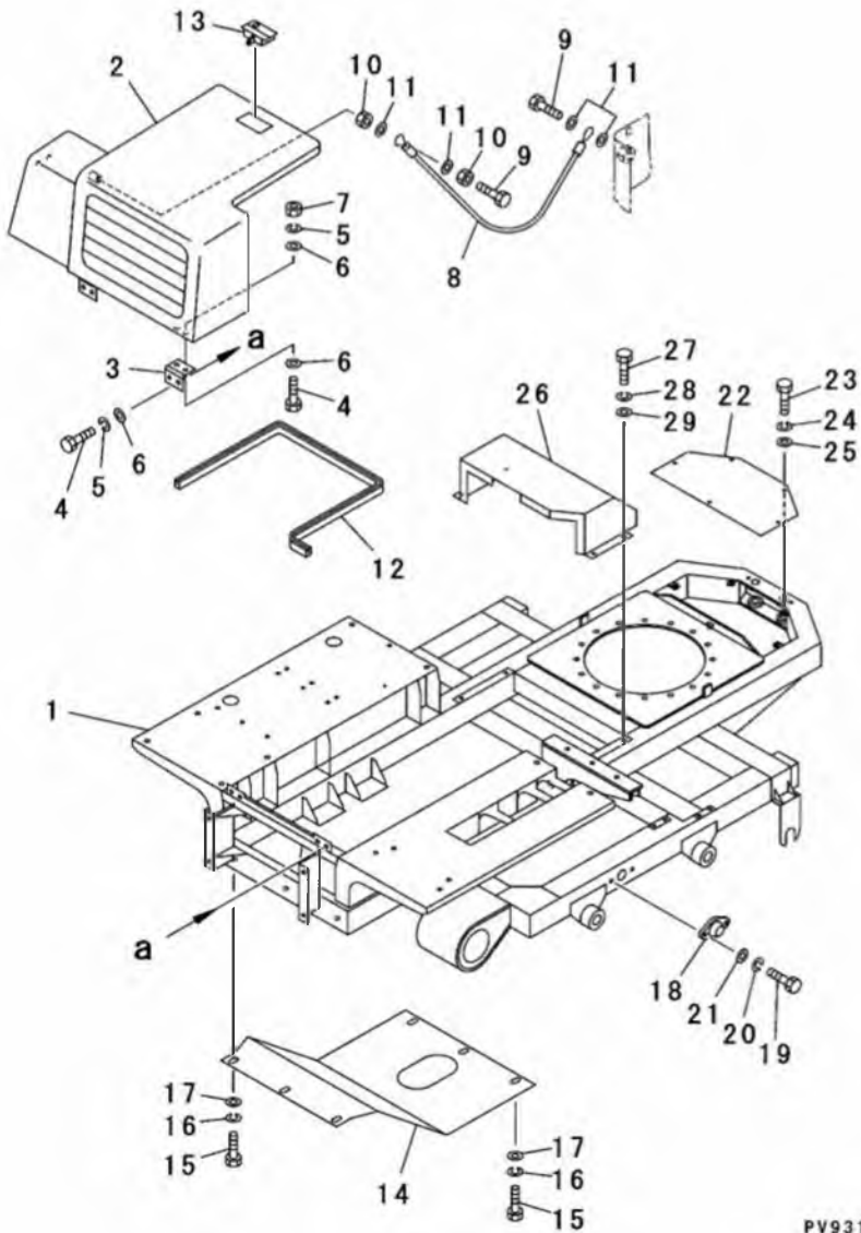
FIG. 202A FRAME RELATED PARTS (1/3) (BONNET AND UNDER COVER) (APPLICABLE TO MST-300VDR) (SERIAL NO.3981-)
