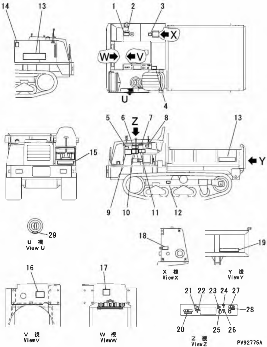
FIG. 811 MARKS AND PLATES (ENGLISH) (APPLICABLE TO MST-300VD) (SERIAL NO.3401-3980)
