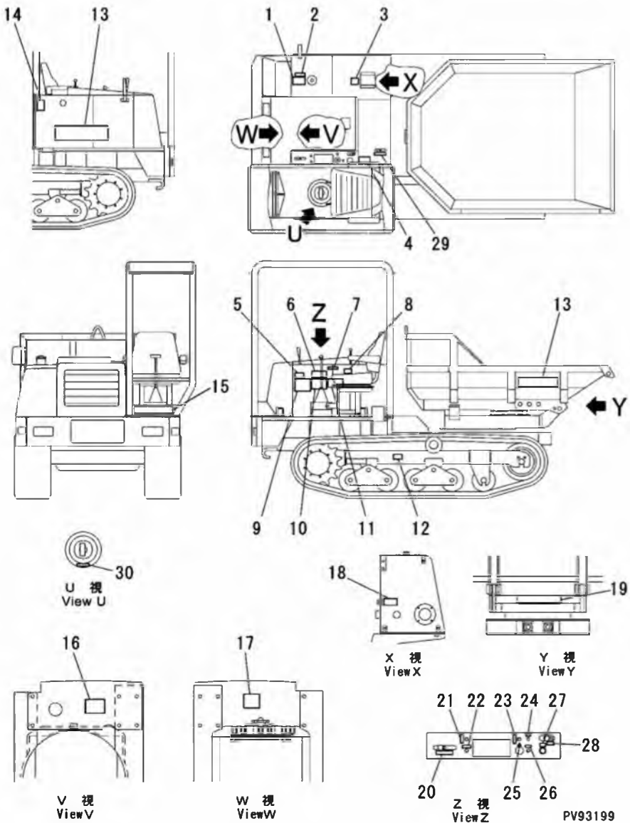
FIG. 812A MARKS AND PLATES (ENGLISH) (APPLICABLE TO MST-300VDR) (SERIAL NO.3981-)
