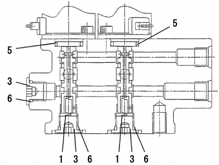
SECTION "X-X"
