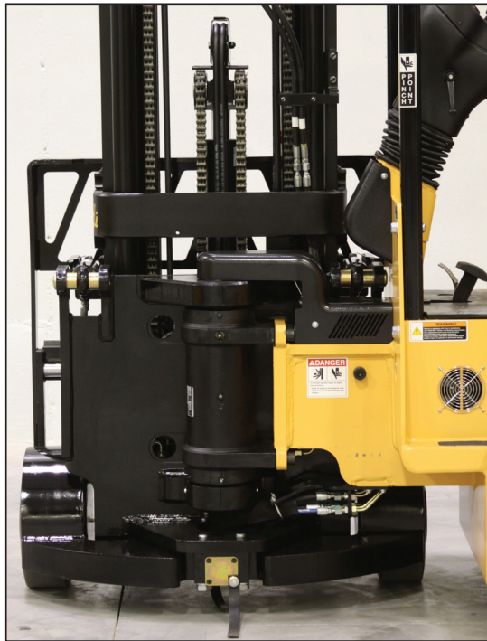
DuraSteer™ Front Wheel Steering *Patented
