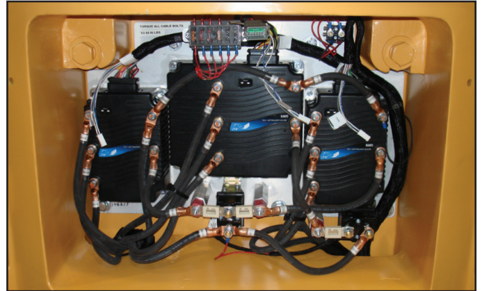
Rear Controller Compartment and Counterweight
