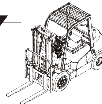
图87/FIG. 87 阀操纵总成（三片 高配）/VALVE CONTROL LINKAGE (THREE-THROW HIGH CONFIGURATION)
