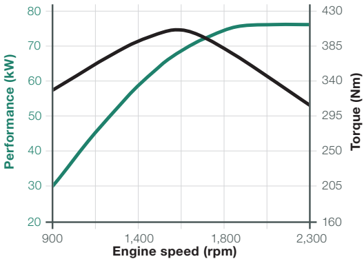
Performance curve of the Deutz TCD 3.6, 74.4 kW, Stage V (option)
