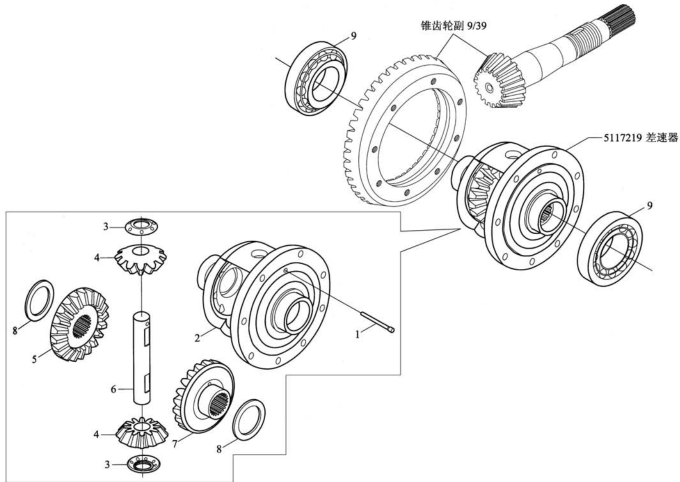
前驱动桥总成 (七) Front Driving Axle Assembly (VII)
