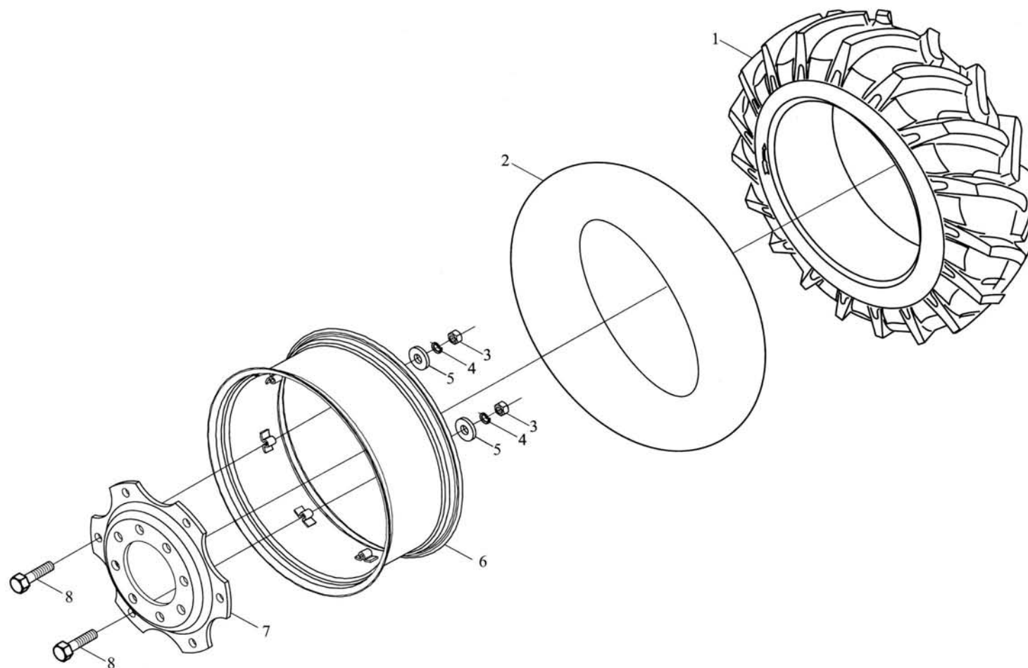
前驱动轮总成 Front Driving Wheel Assembly
