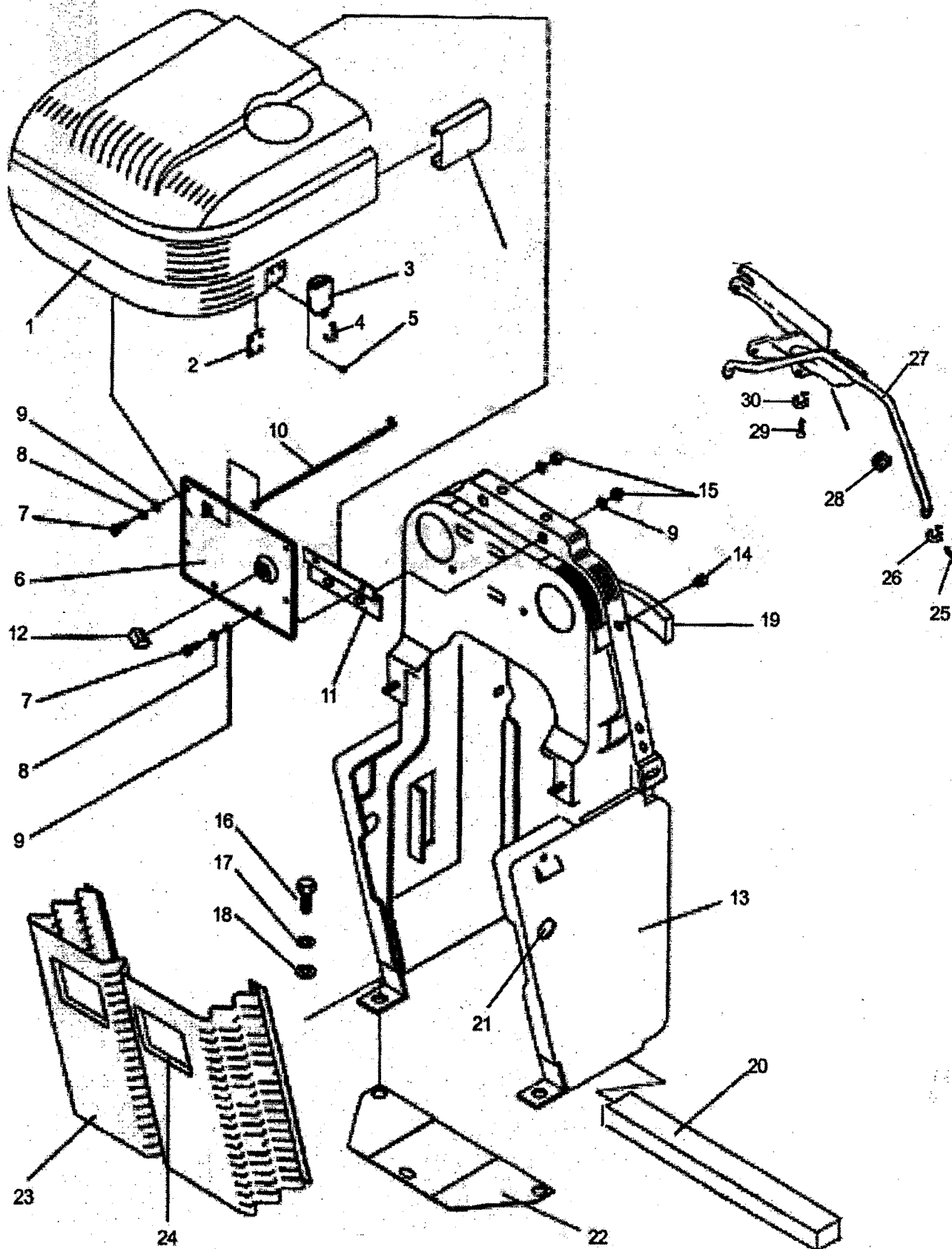
RADIATOR SHELL
