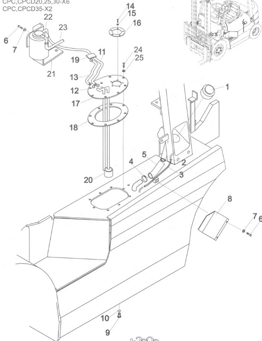
燃油系统/FUEL SYSTEM
