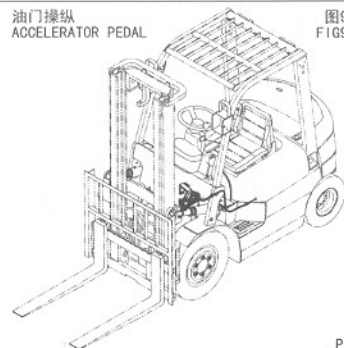
油门操纵 ACCELERATOR PEDAL
