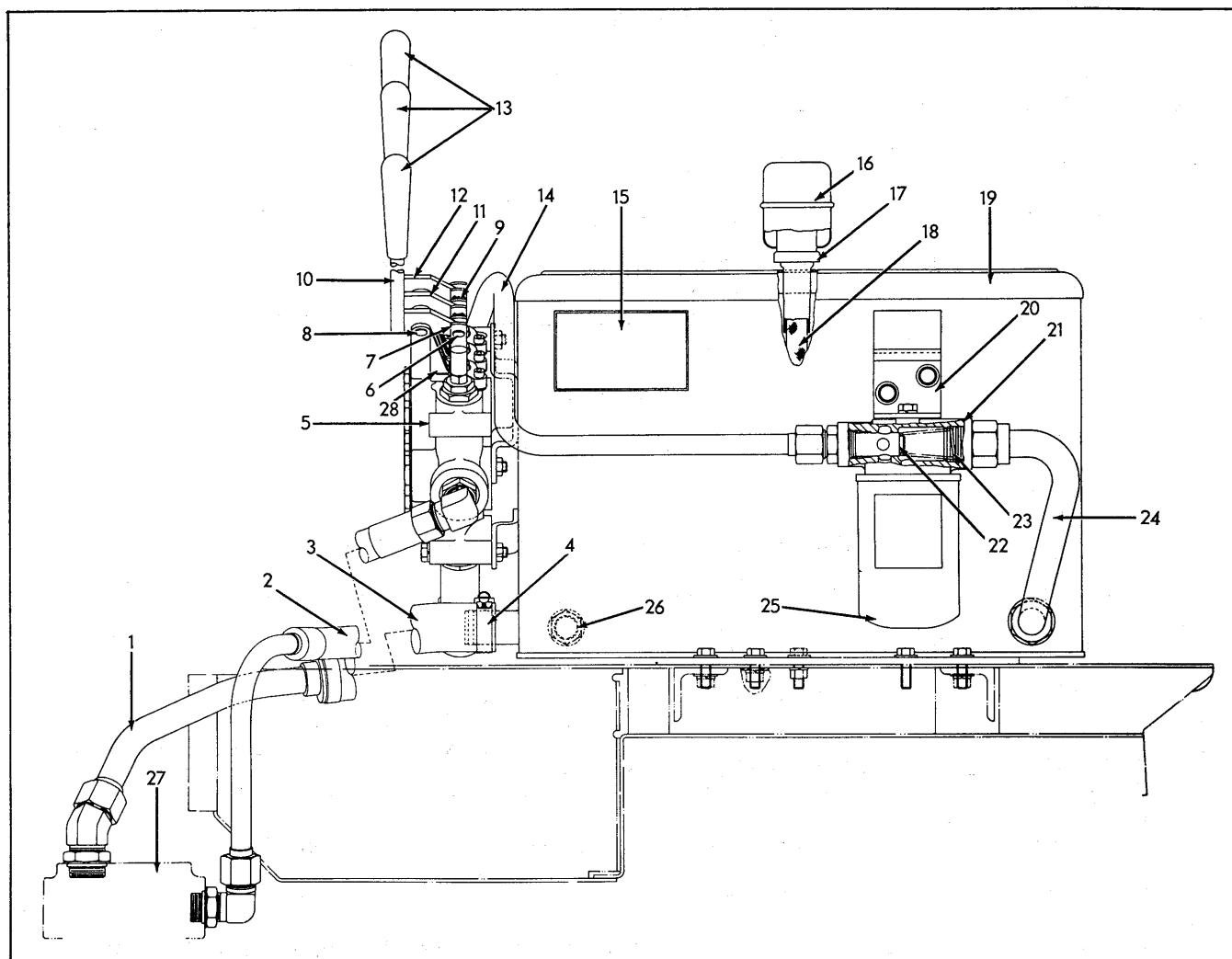
HYDRAULIC SYSTEM W/ Fender Mounted Reservoir
