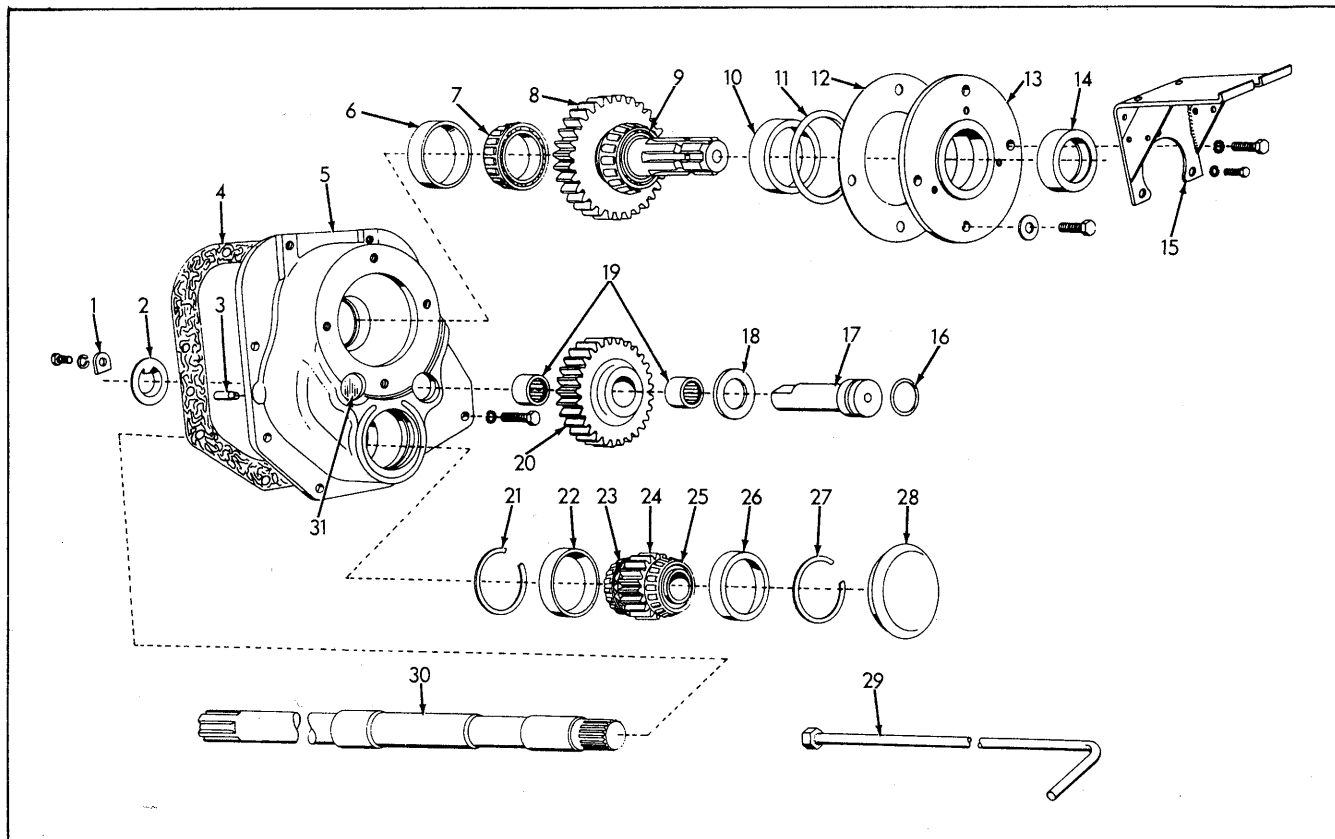
POWER TAKE-OFF H-3 & HD-3 Tractors
