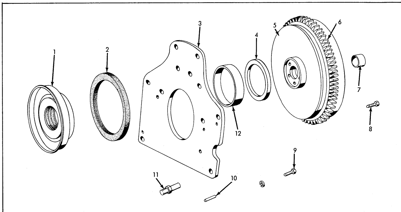
FLYWHEEL & RING GEAR Diesel
