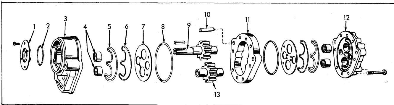
SINGLE HYDRAULIC PUMP (11.5 G.P.M.) Eff. w/Tr. S/N 8694 & Up
