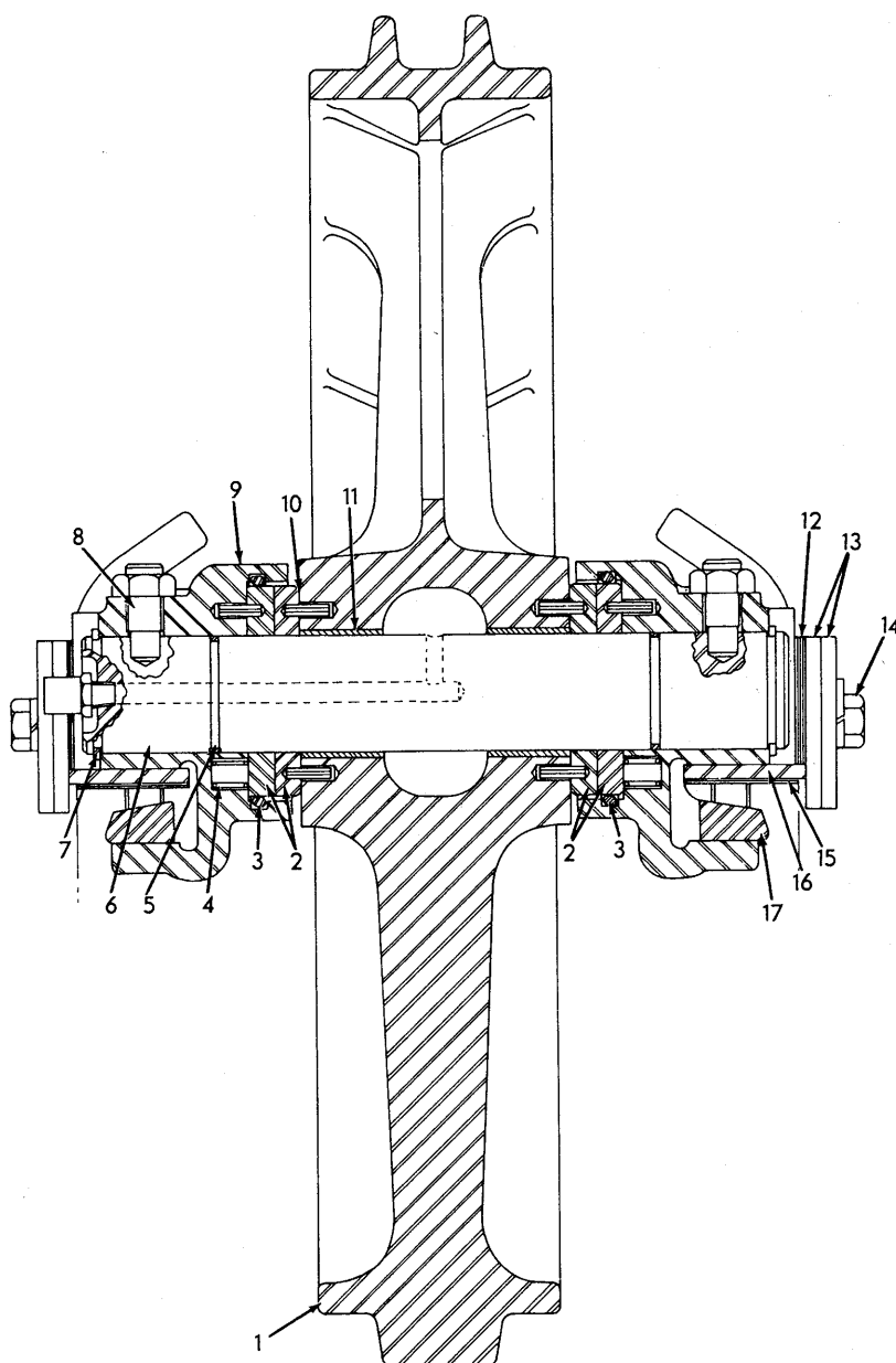
TRACK IDLER Eff. w/Tr. S/N 8298
