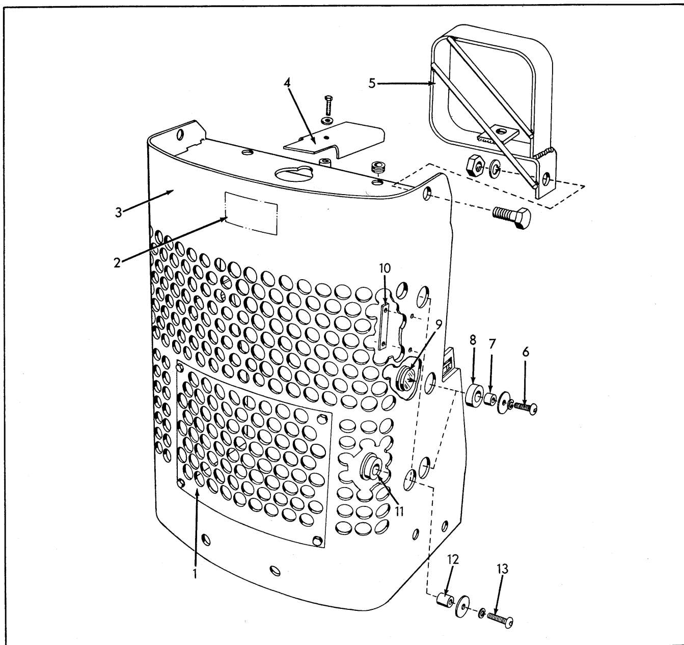
GRILLE - HEAVY DUTY
