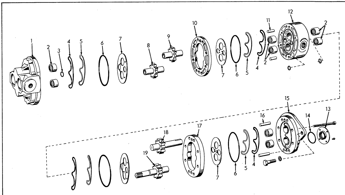
DUAL HYDRAULIC PUMP (25 G.P.M.) Eff. w/Tr. S/N 8694 & Up
