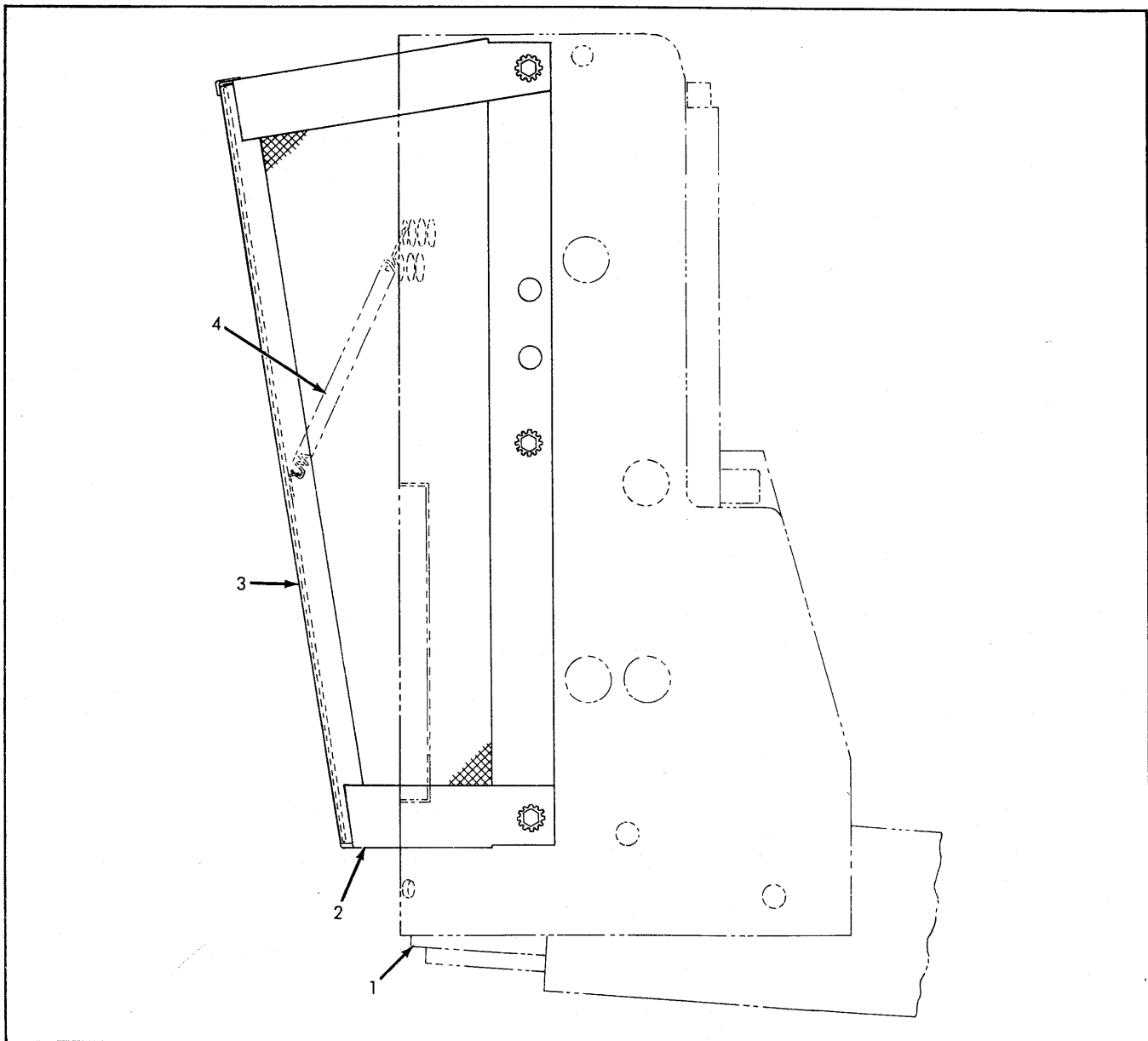
RADIATOR GRILLE SCREEN f/54' Tread Muckland Tractor
