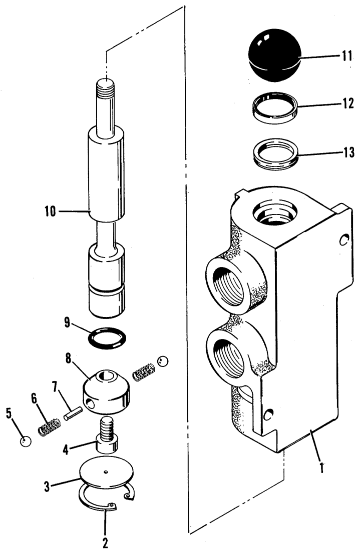
DIVERTER VALVE
