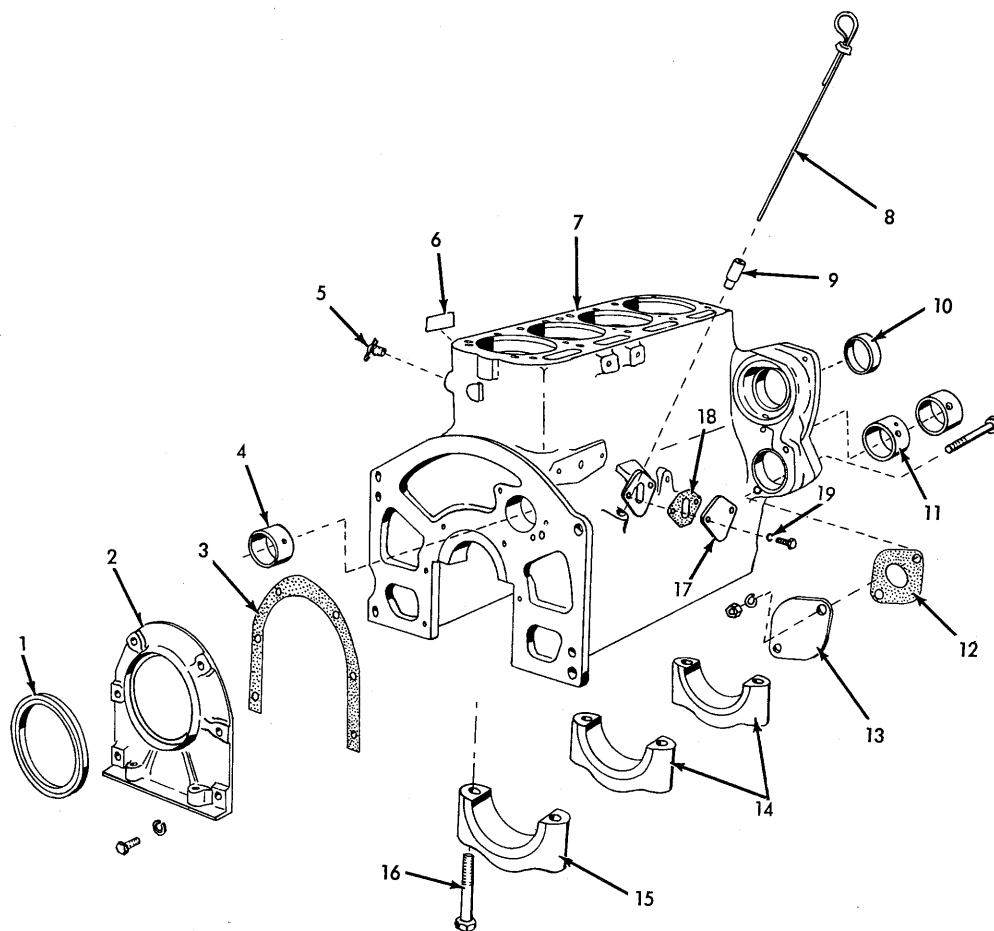
CYLINDER BLOCK Gasoline
