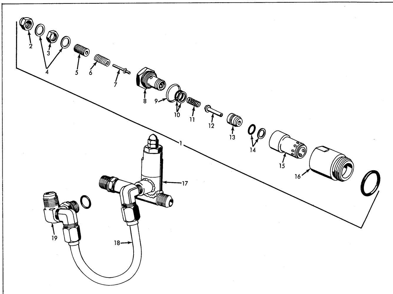
CIRCUIT RELIEF VALVE Used w/1066 Loader
