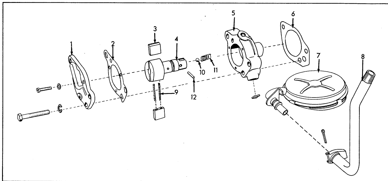
OIL PUMP Gasoline
