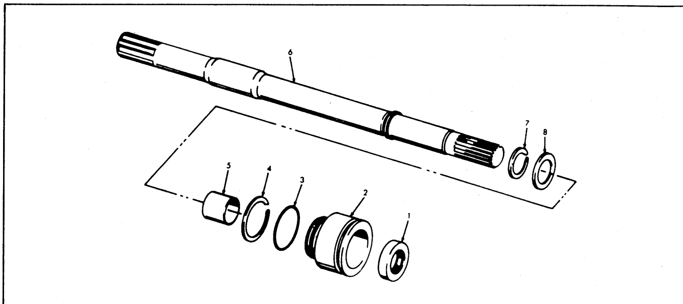
REAR WINCH DRIVE SHAFT
