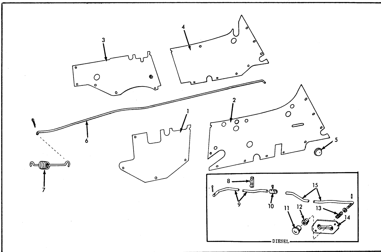
INJECTION PUMP CONTROL, CHOKE CONTROL & SIDE SHEETS Gasoline & Diesel
