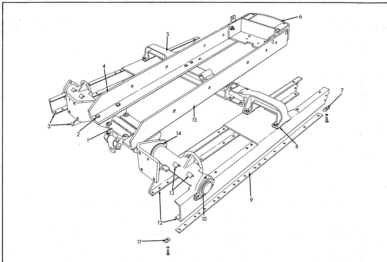
MAIN FRAME, TRUCK FRAME & AXLE
