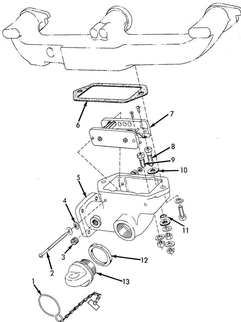
ENGINE AIR HEATER Diesel Used Prior to Eng. S/N 119780
