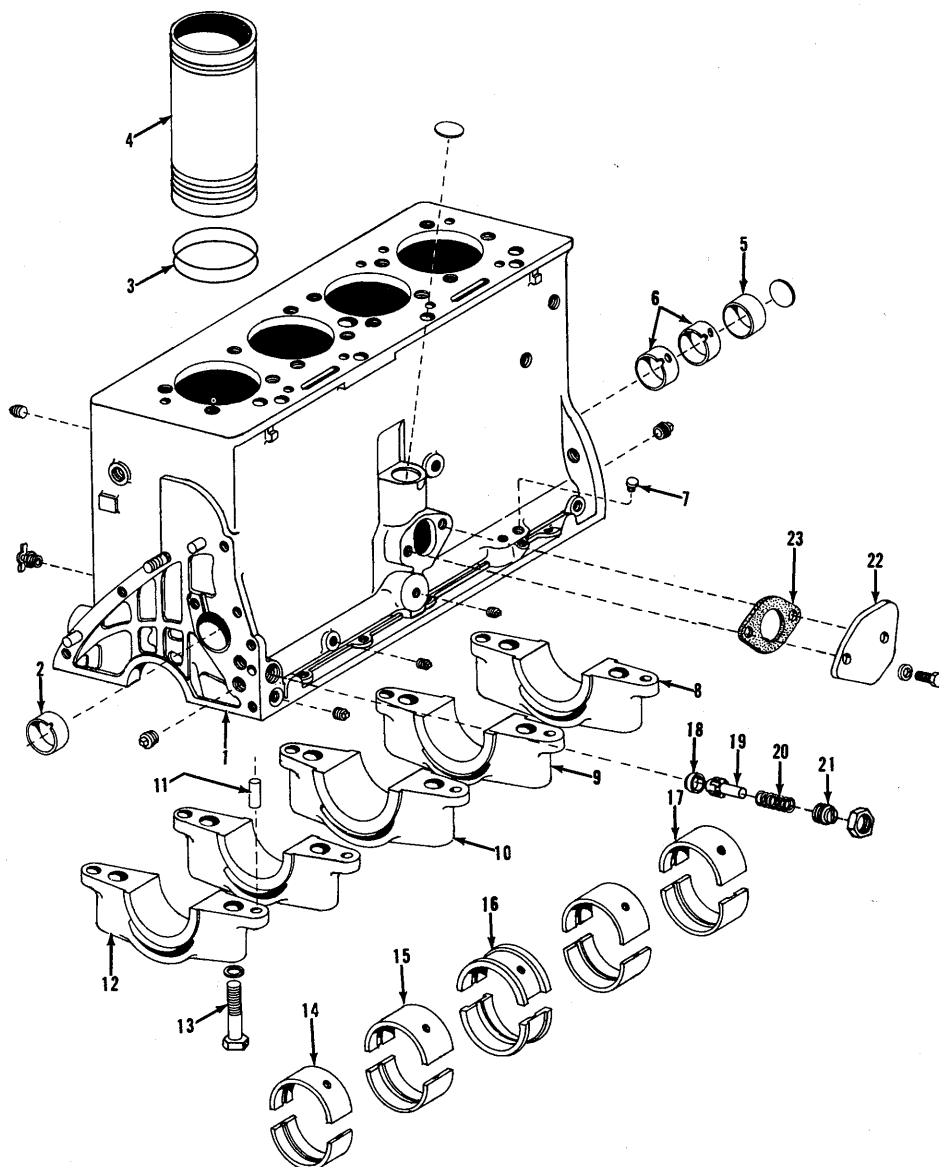
CYLINDER BLOCK Diesel
