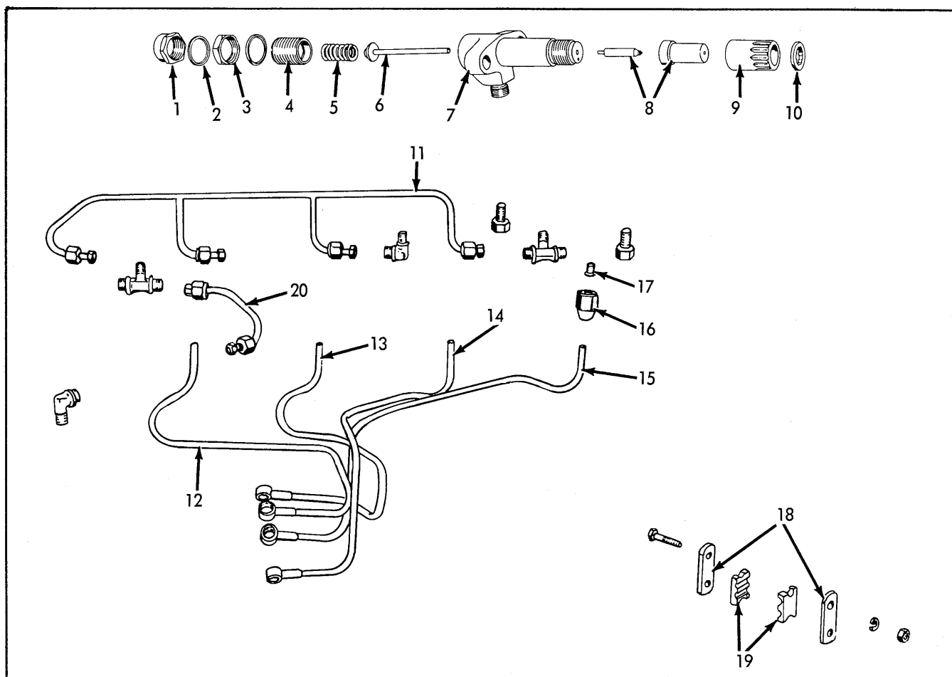
FUEL INJECTION NOZZLES & LINES Diesel
