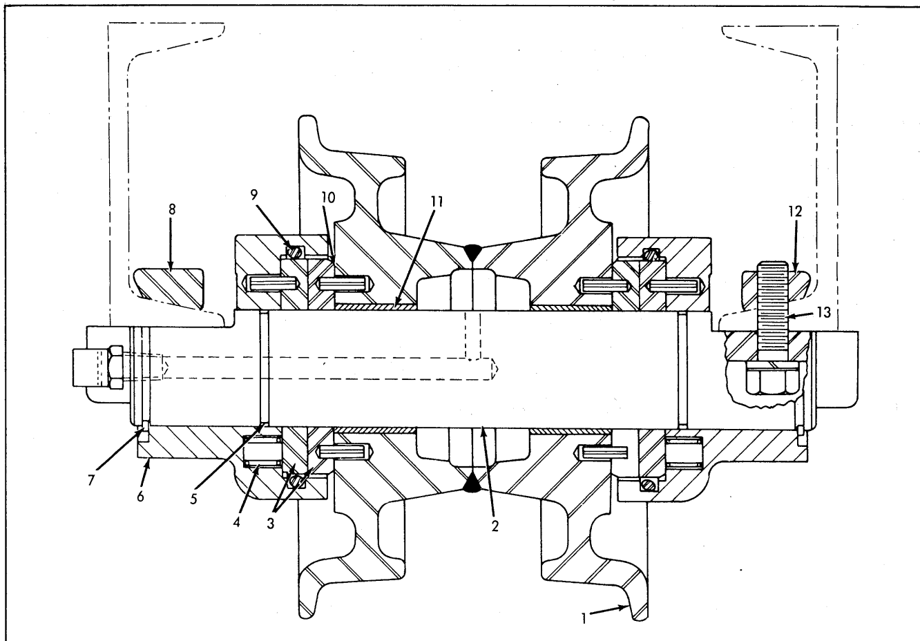
TRUCK WHEEL Eff. w/Tr. S/N 8298 & Up
