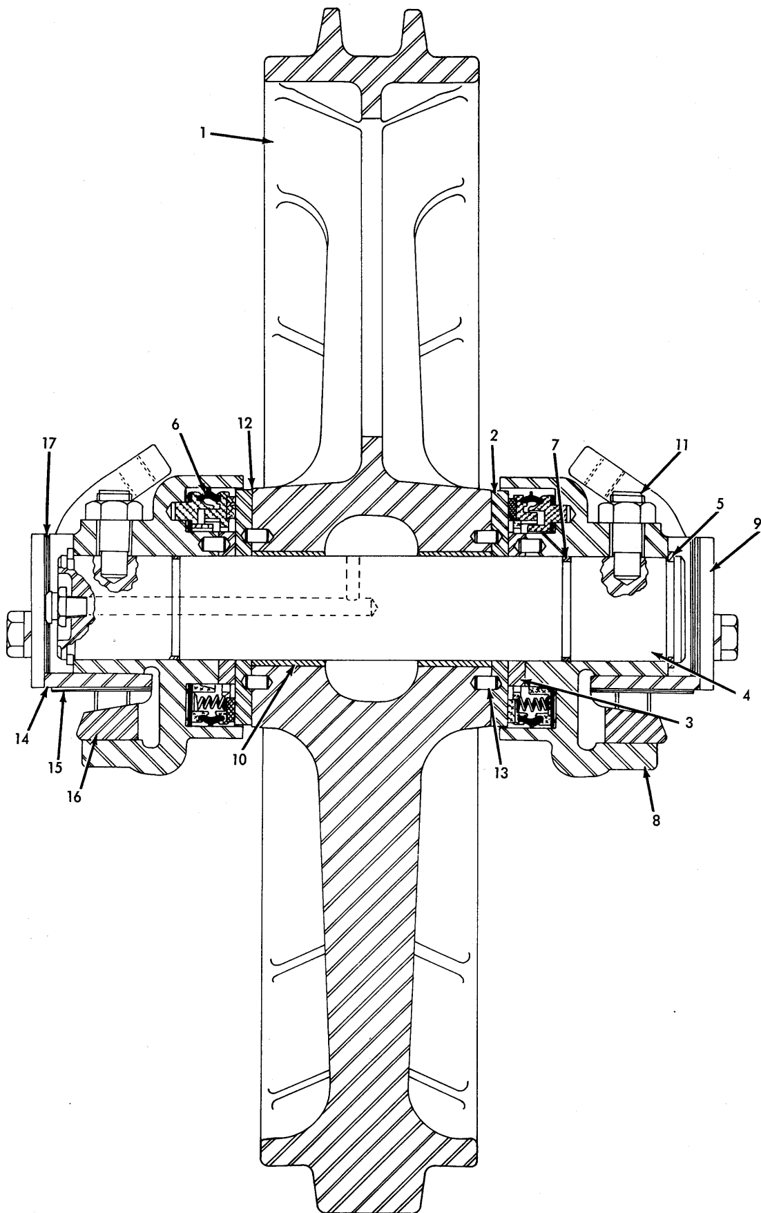
TRACK IDLER (Used Prior to Tr. S/N 8298)
