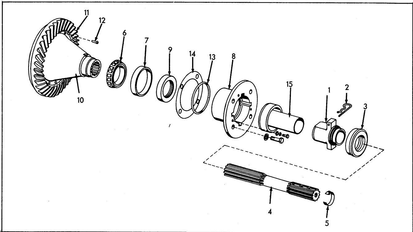
DRIVE SHAFT & RING GEAR R.H. Side Shown
