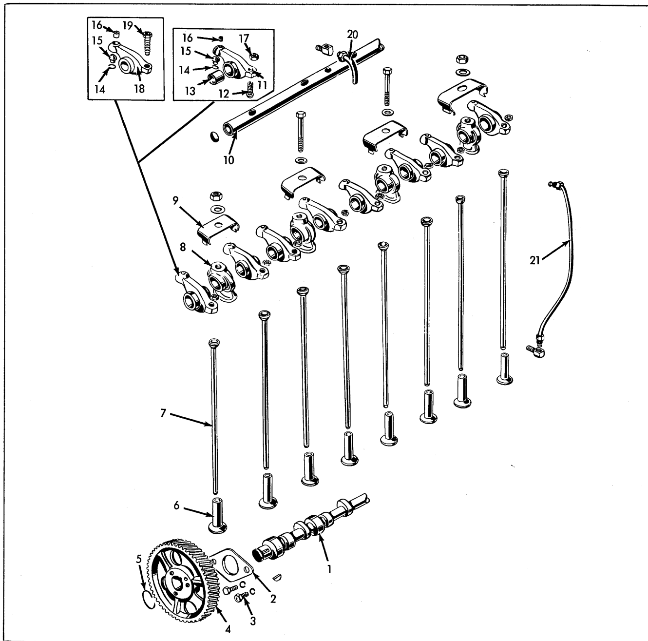
VALVE OPERATING MECHANISM Diesel
