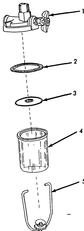
FUEL TANK FILTER Diesel
