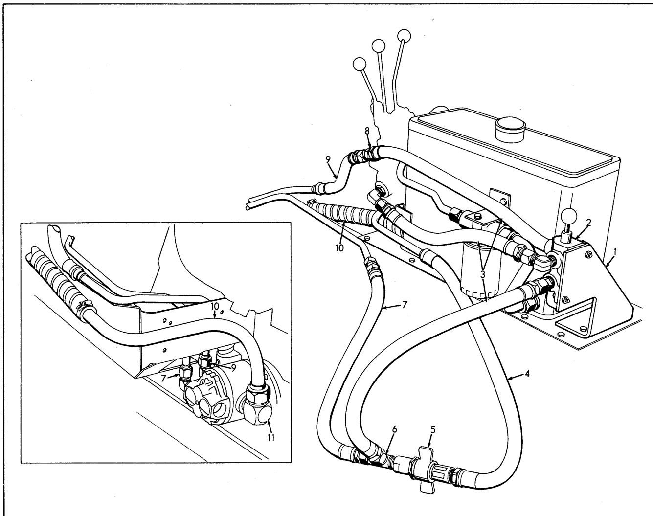
HYDRAULIC LINES Loader & Backhoe Eff. w/Tr. S/N 8694 & Up
