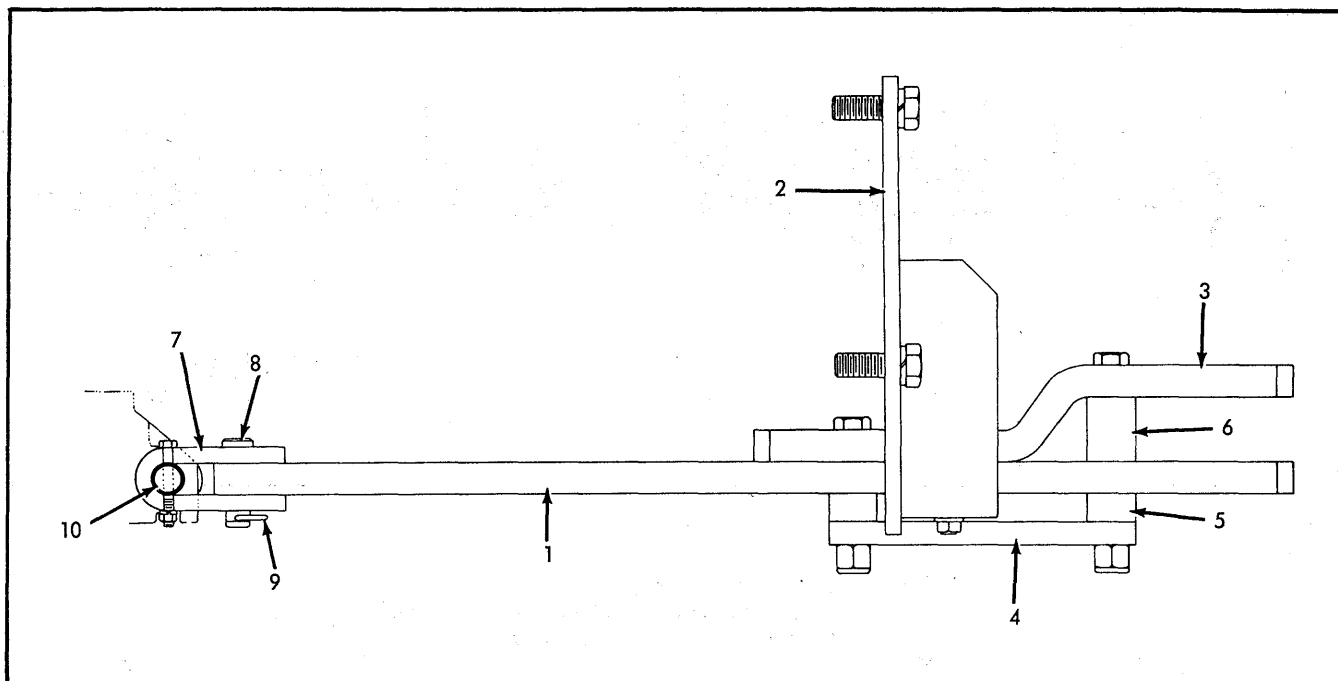
DRAWBAR
