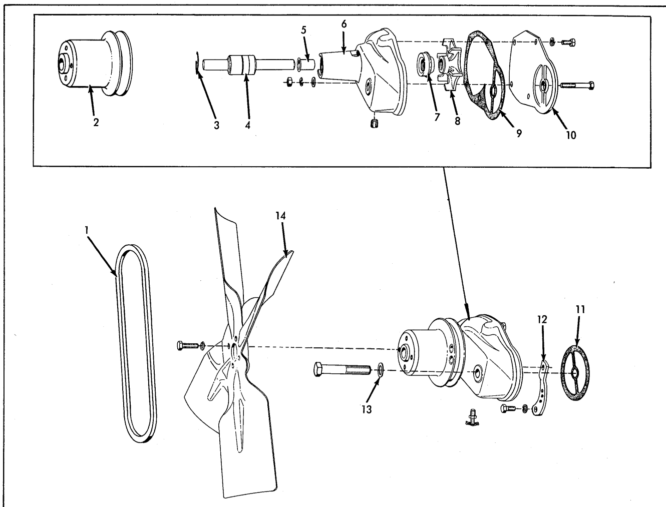
WATER PUMP
