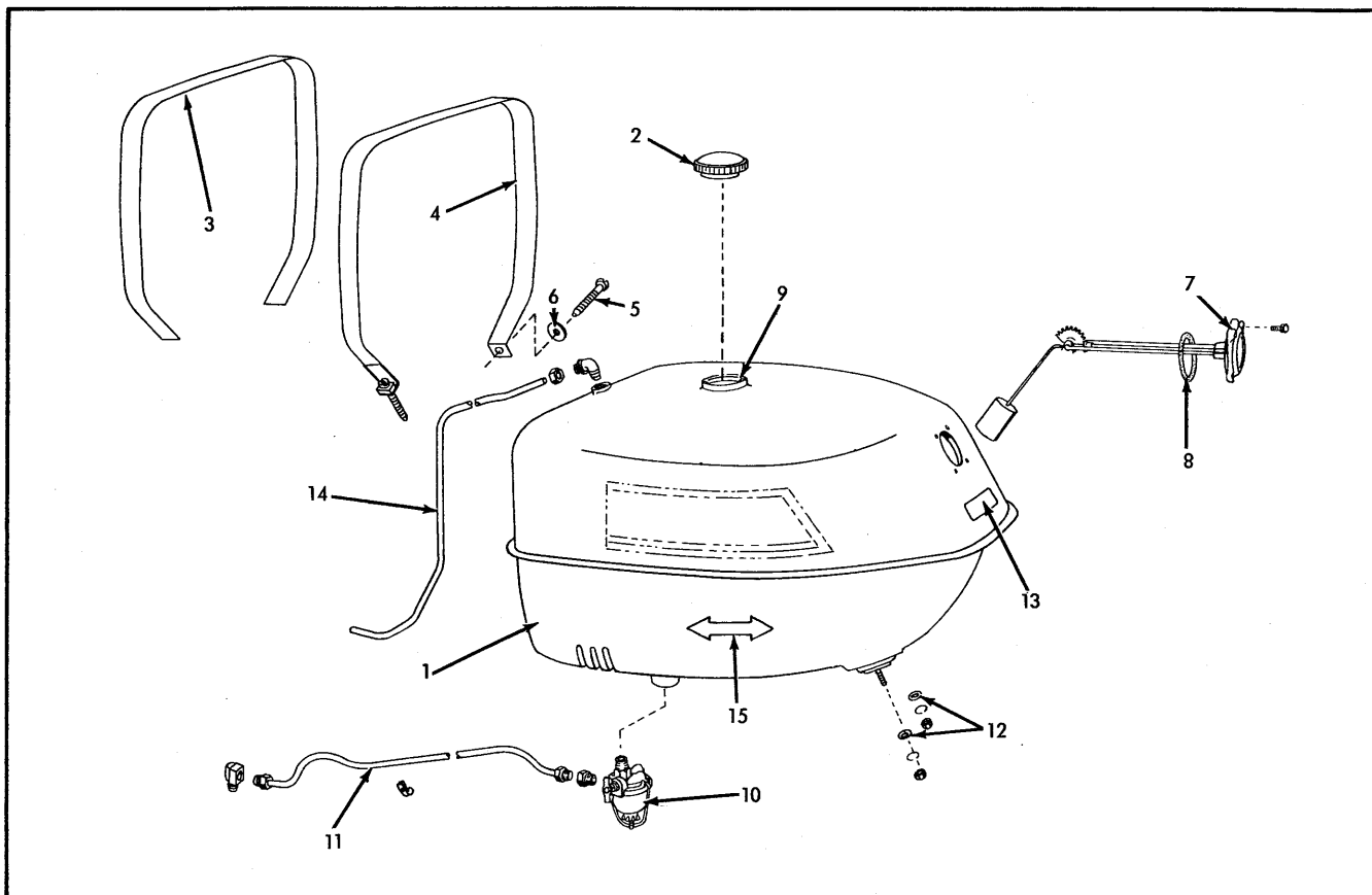
FUEL TANK (Gasoline & Diesel)
