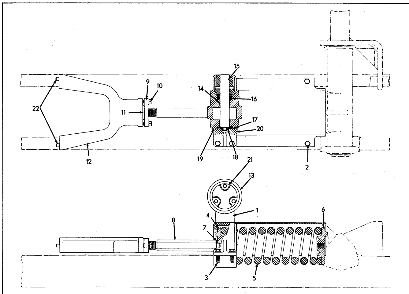
TRACK RELEASE & SUPPORT ROLLER
