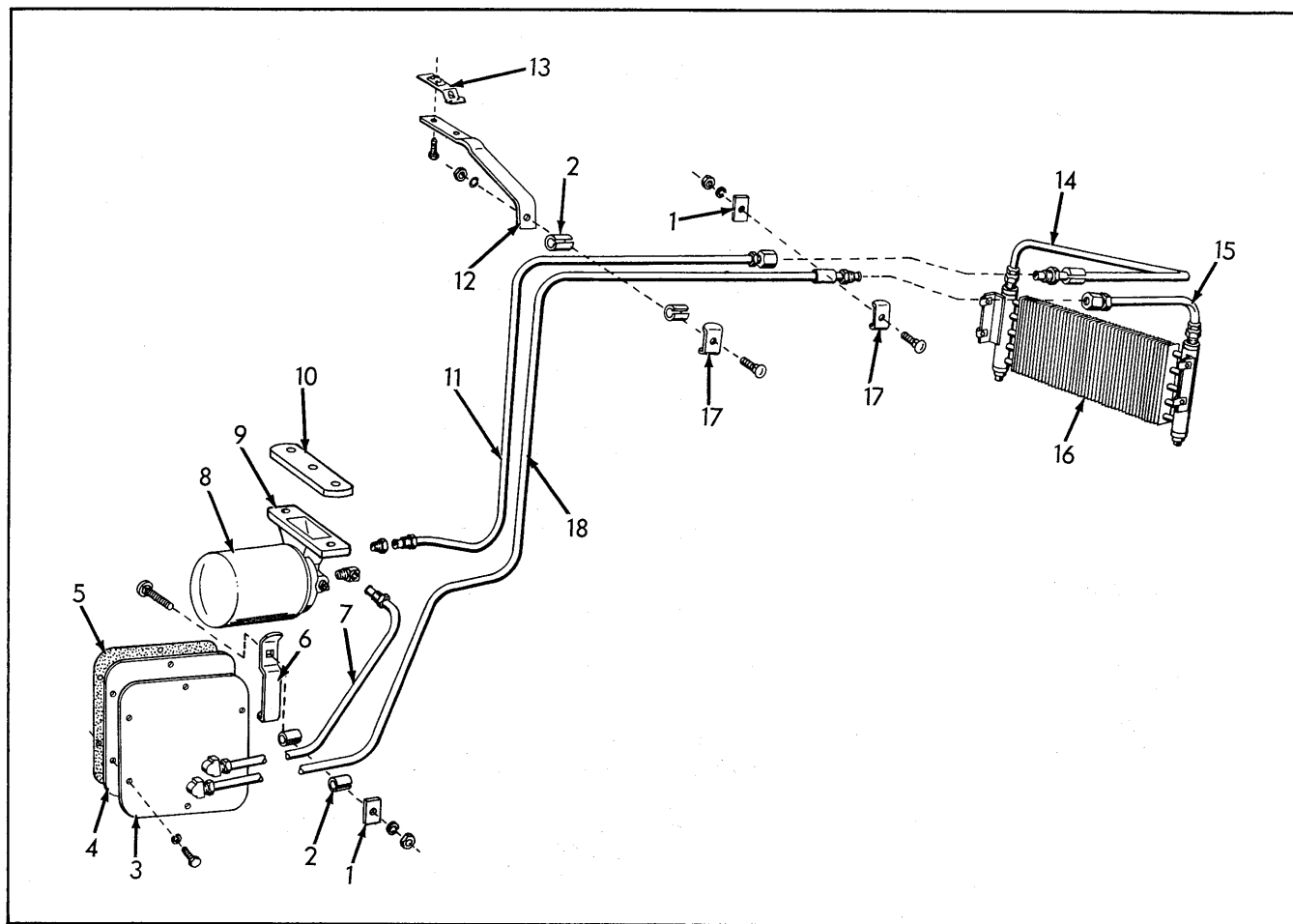
OIL COOLER - POWER DIRECTOR 54" Tread Muckland Tractor
