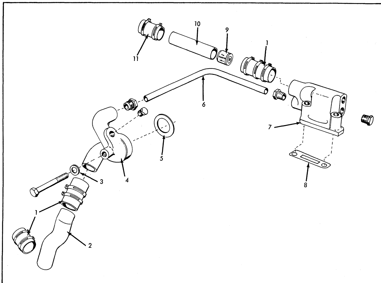
WATER INLET & OUTLET PIPES Diesel
