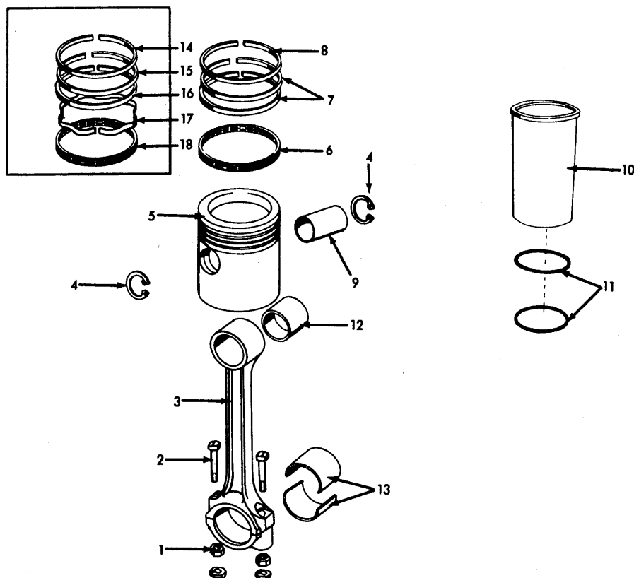
PISTON & CONNECTING ROD Gasoline (160 cu. in. Engine) Eff. w/tr. S/N 6959 & up
