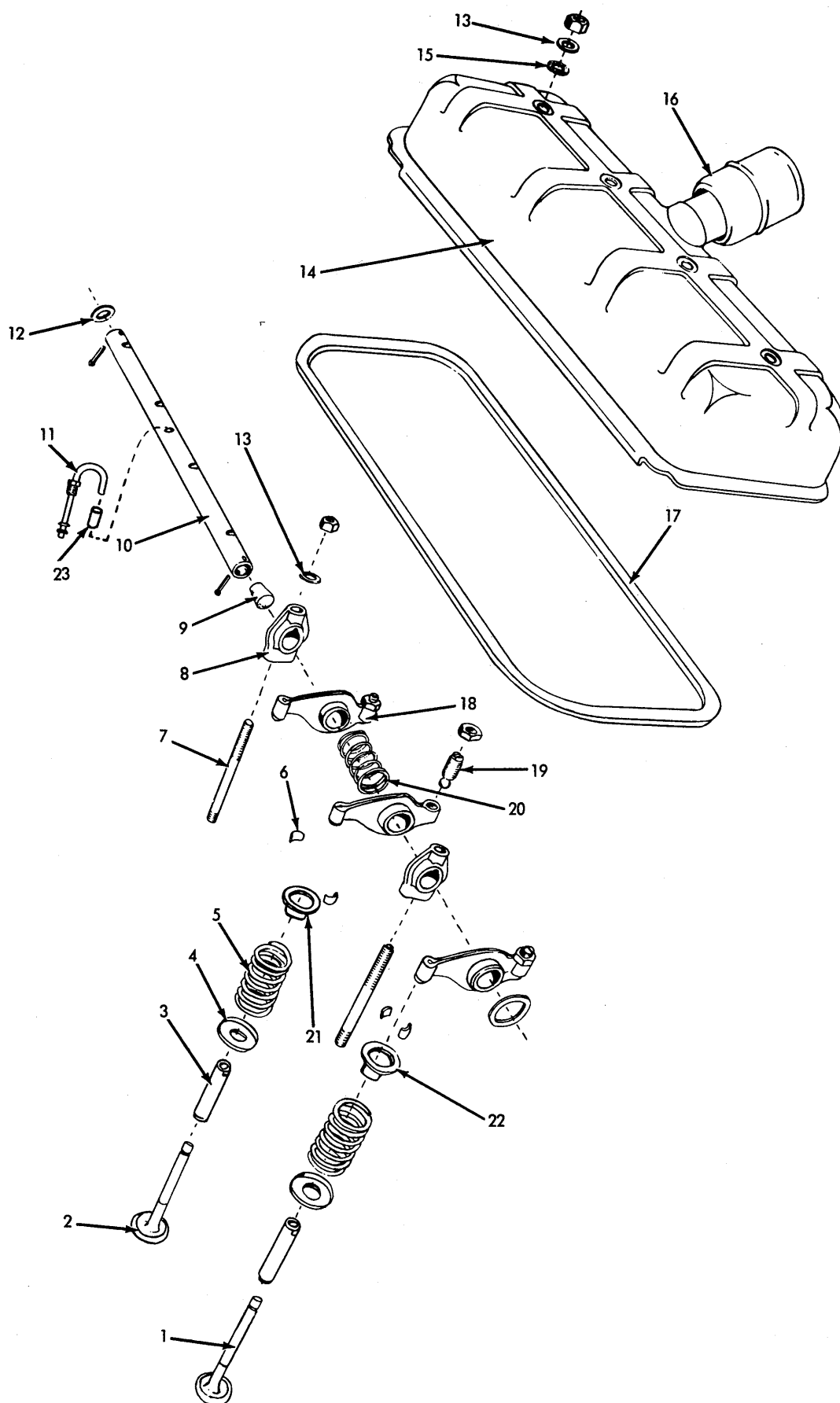
VALVES & ROCKER ARMS
