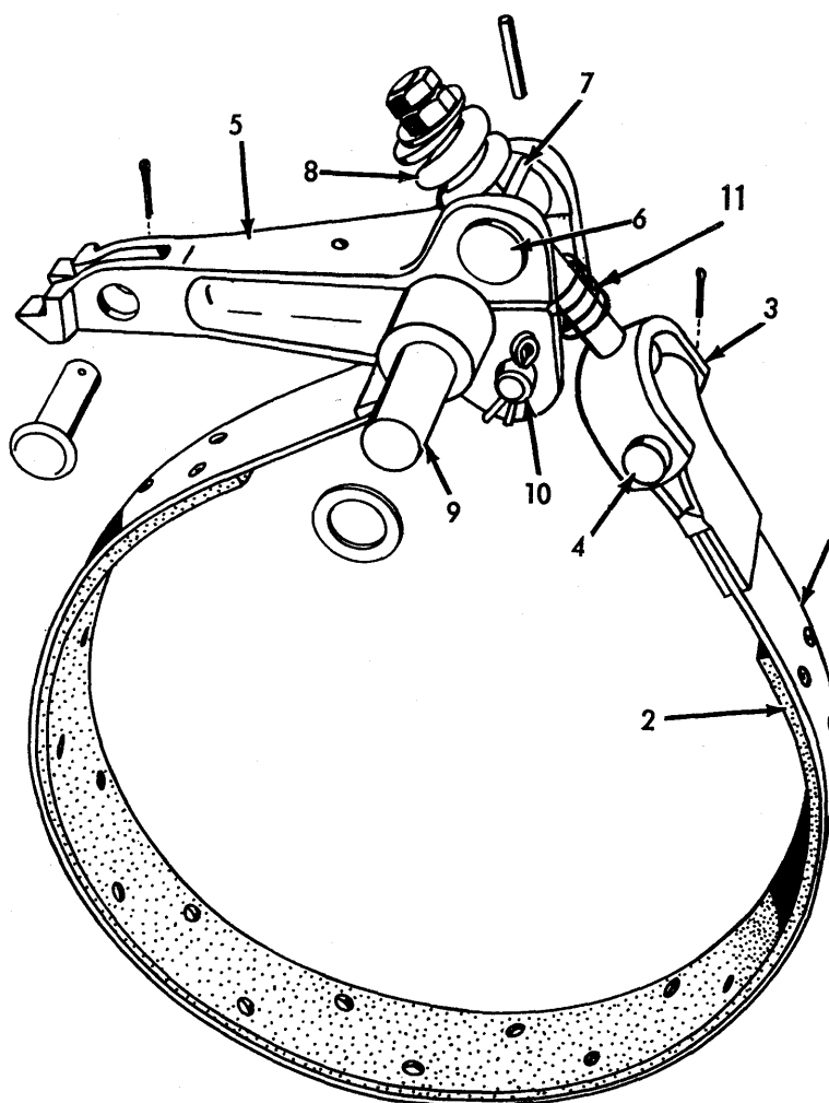
BRAKE BAND & ARM
