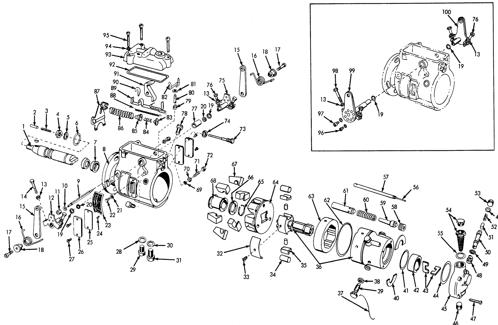
FUEL INJECTION PUMP Used Eng. S/N 117742 Thru D-08499 Eff. w/Eng. S/N D-08500 Muckland Tractor Eff. w/Eng. S/N D-03548
