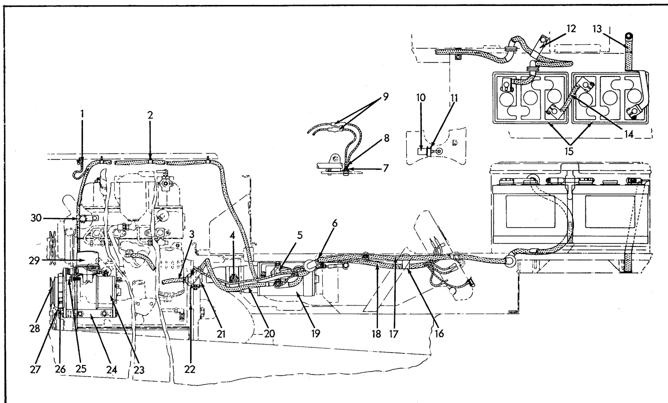
ELECTRICAL SYSTEM Diesel
