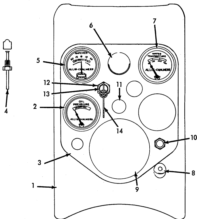
INSTRUMENT PANEL Gasoline & Diesel
