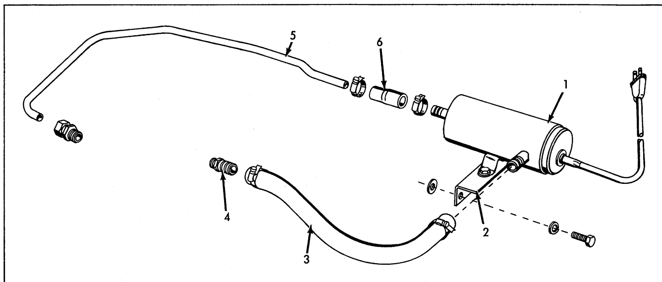
ENGINE WATER HEATER Diesel Tractor Optional Equip.
