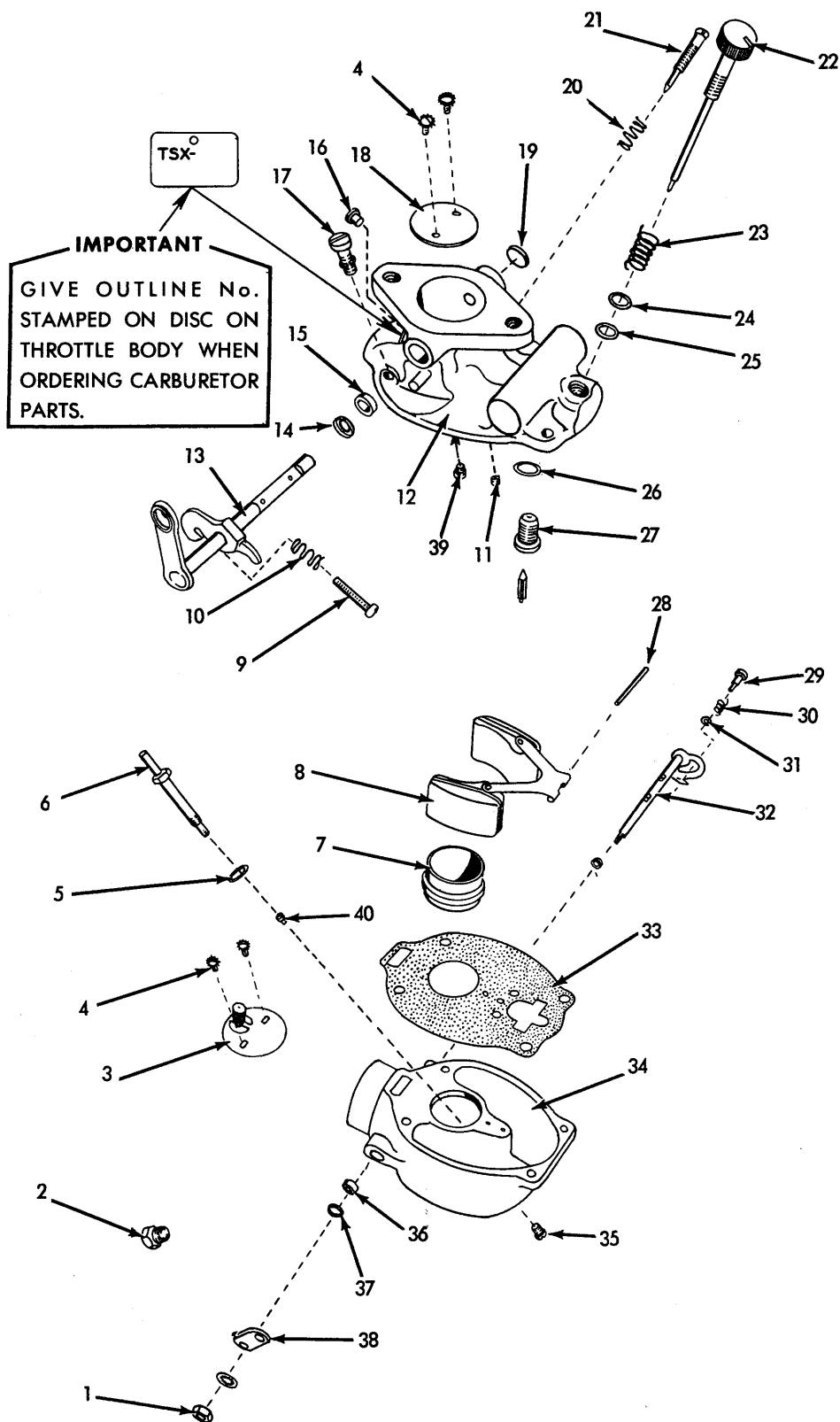
CARBURETOR (Eff. w/Tr. S/N 6959 & up)
