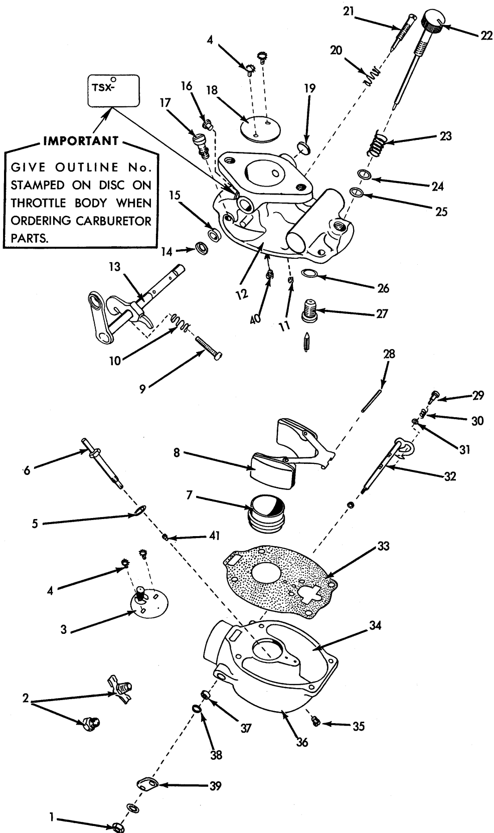
CARBURETOR (Used Prior to Tr. S/N 6959)
