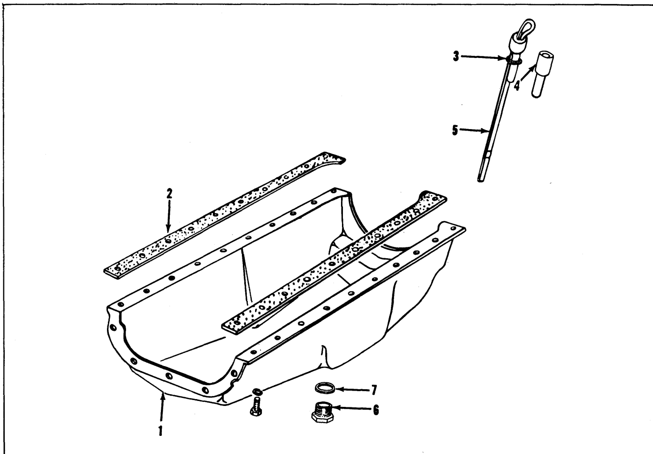
OIL PAN Diesel
