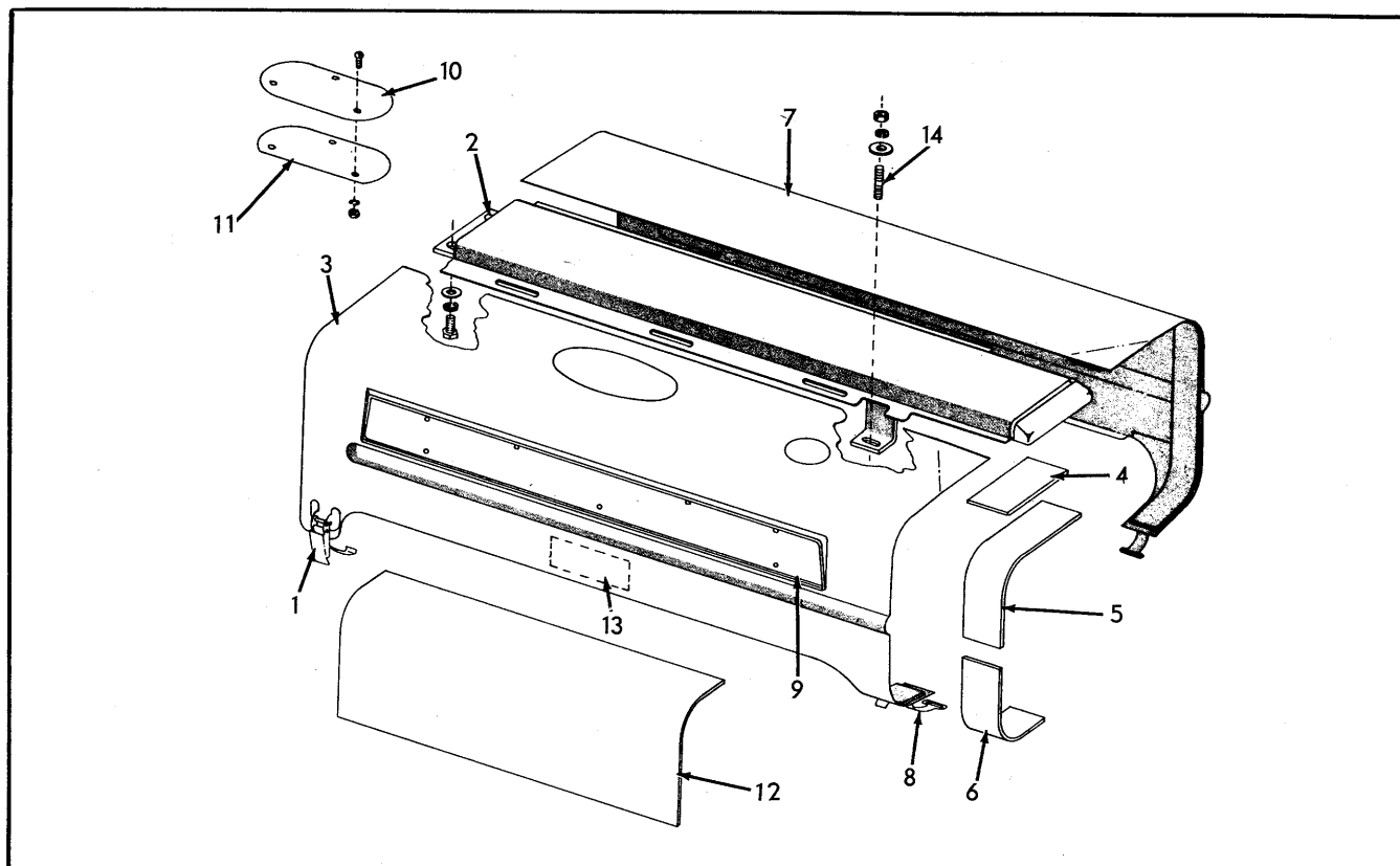
HOOD (Gasoline & Diesel)
