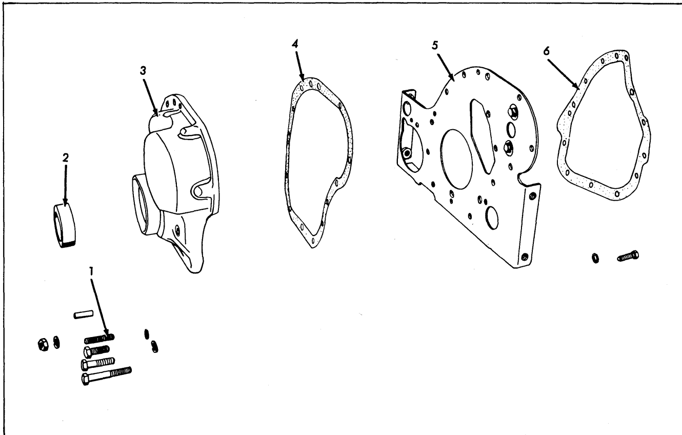
GEAR COVER Diesel
