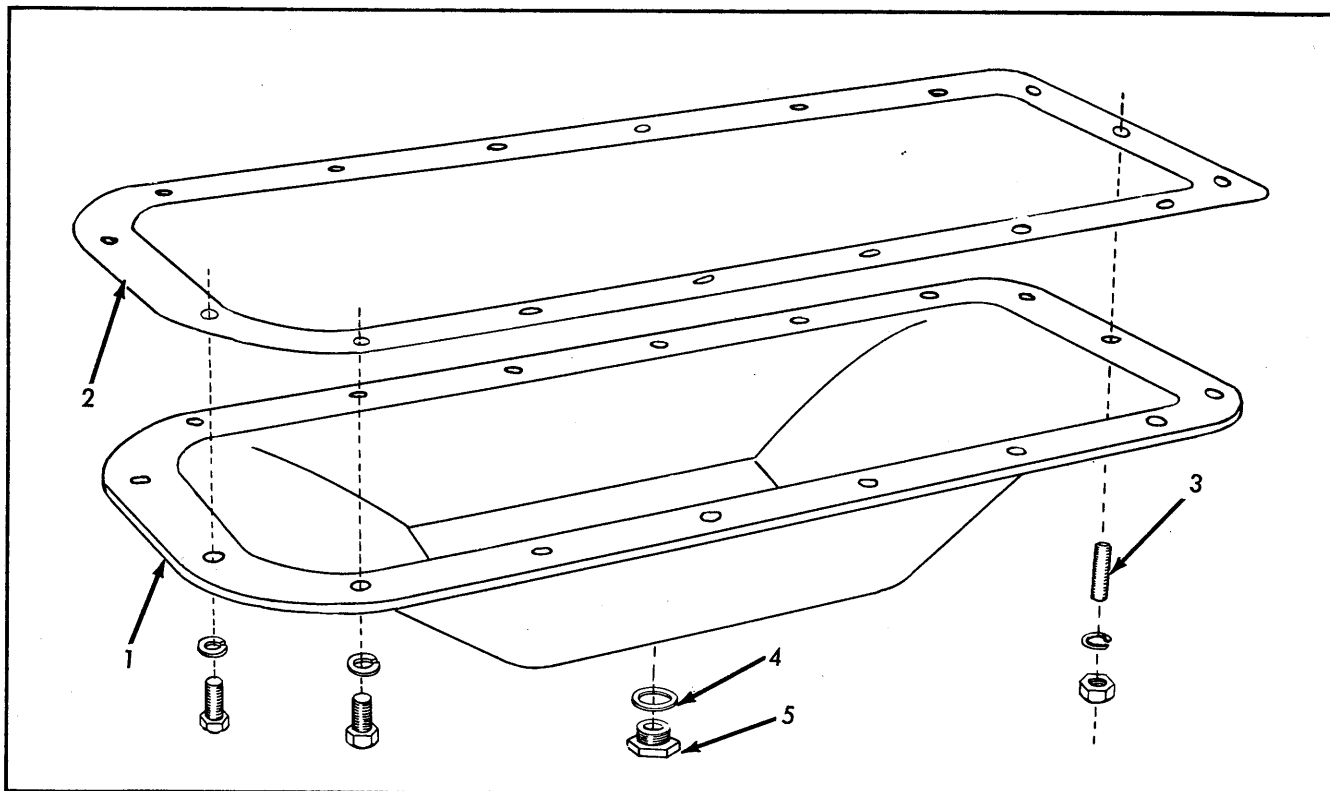
OIL SUMP Gasoline
