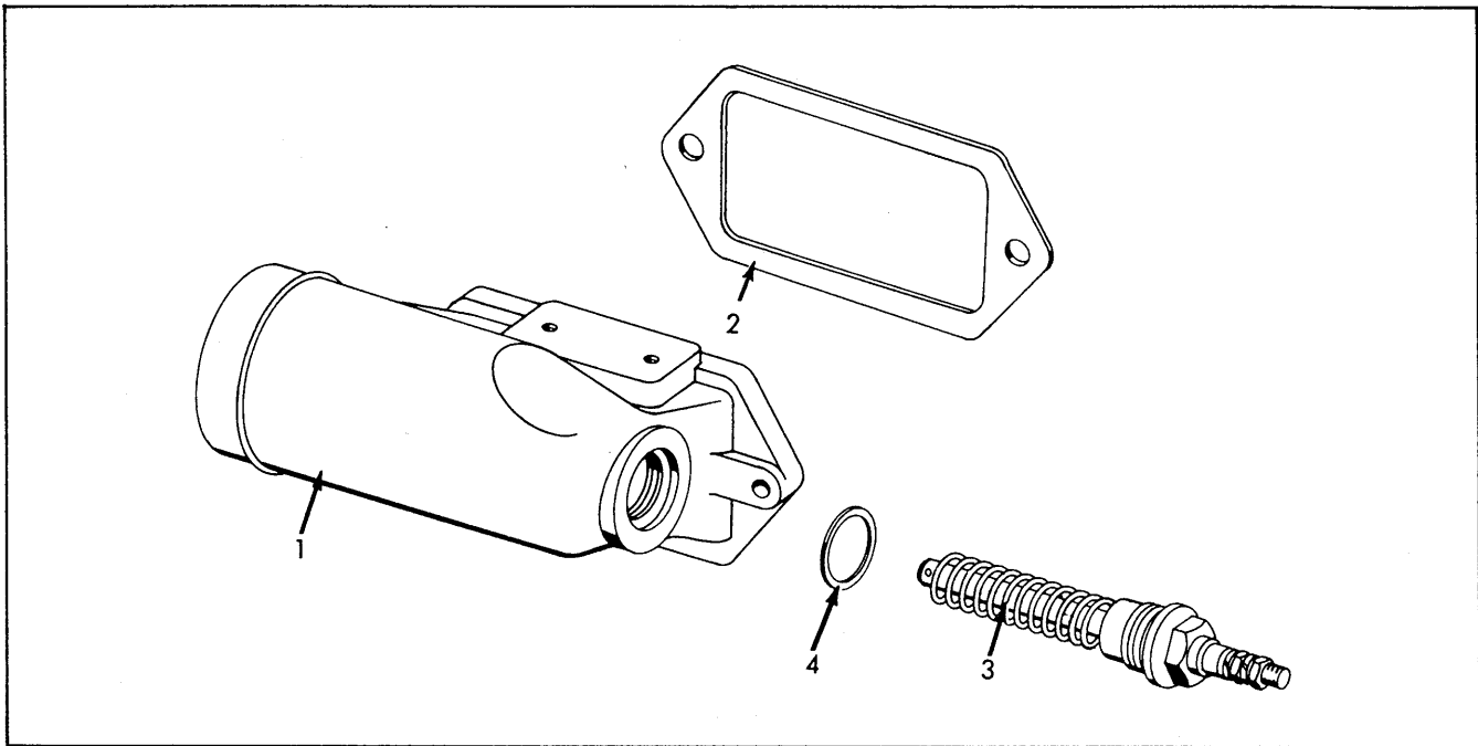
AIR HEATER Eff. w/ Eng. S/N 119780
