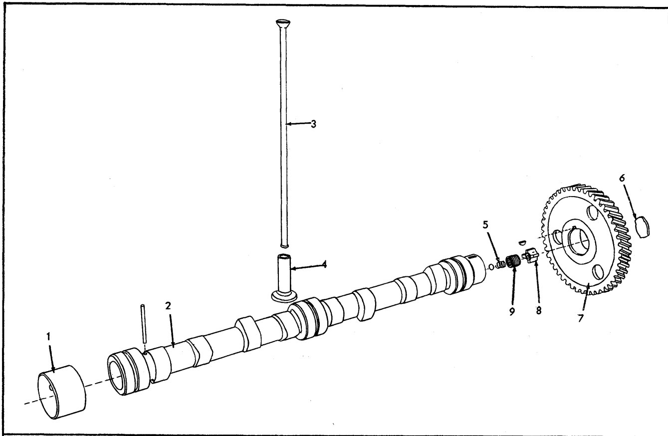
CAMSHAFT Gasoline
