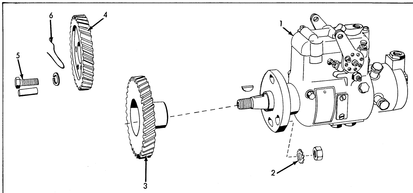
FUEL INJECTION PUMP Diesel
