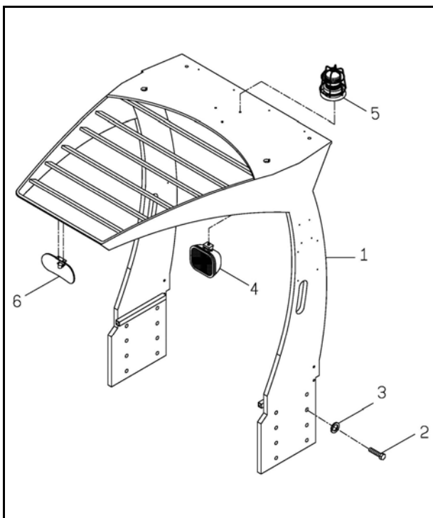
A352-3 OVERHEAD GUARD
