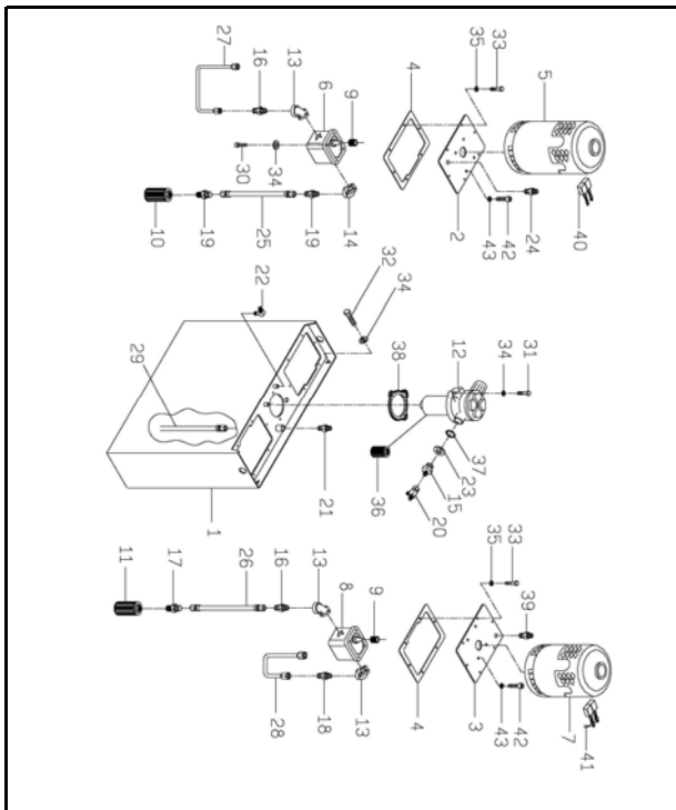
A353-1 OIL TANK MODULE
