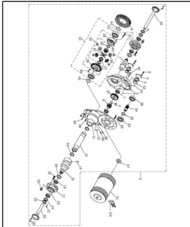
A351-2 AXLE AND TRANSMISSION ASSEMBLY
