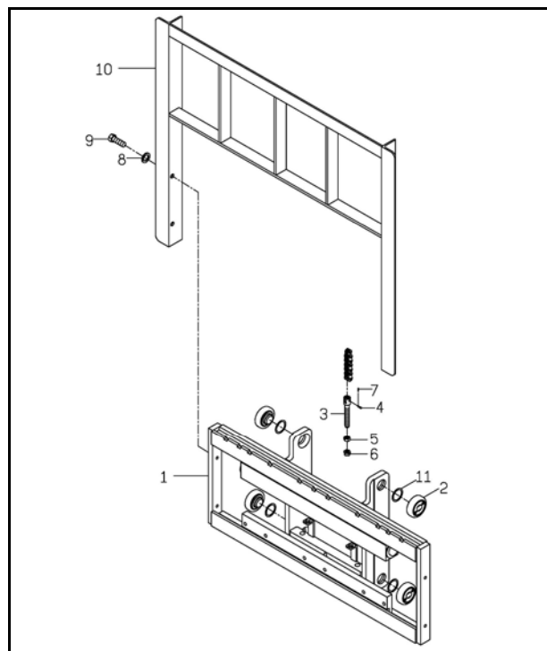
A356-4 NARROW AISLE FORK CARRIAGE ASSEMBLY
