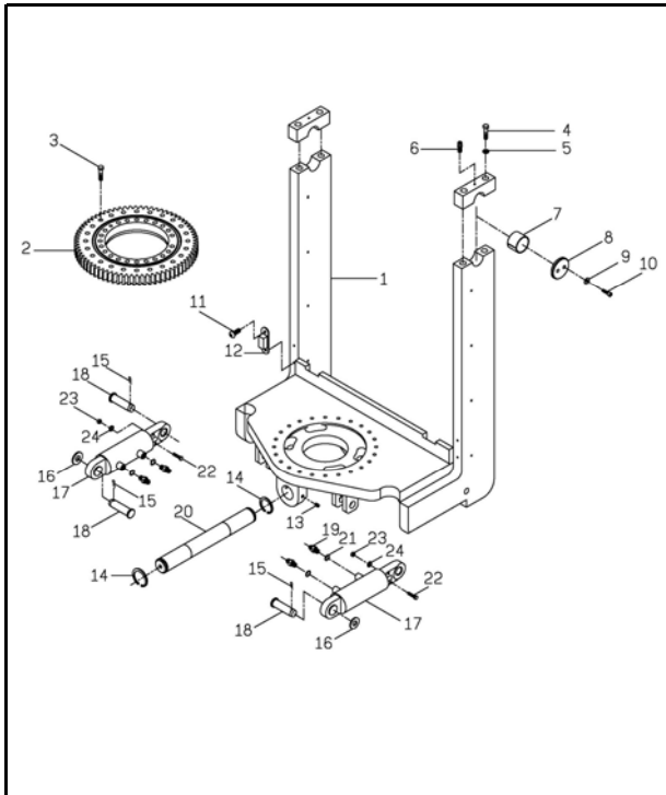
A356-1 MAST SUPPORT ASSEMBLY
