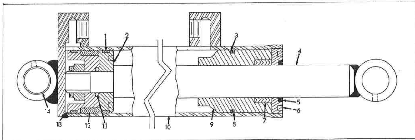
LIFT CYLINDER 1066 Loader Eff. April 1966 (w/Threaded Piston)
