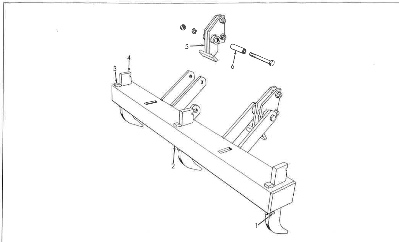
BAR & TOOTH Scarifier
