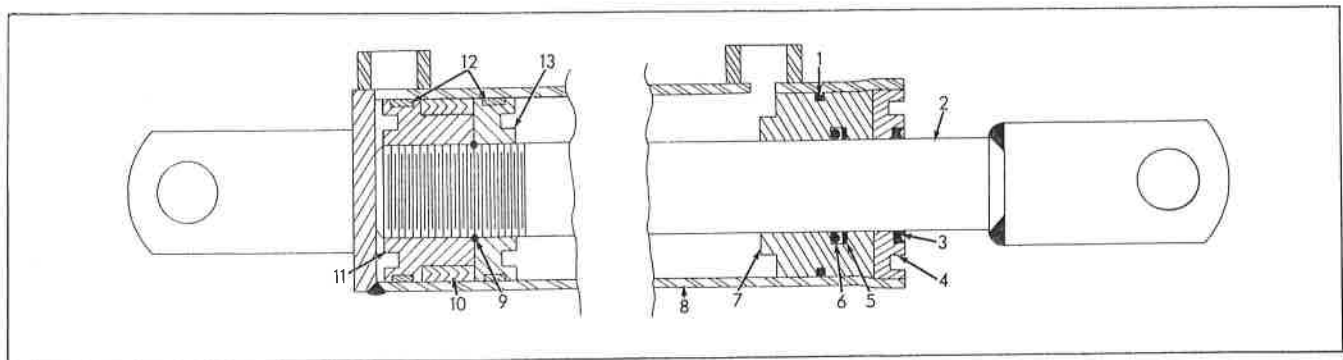
CYLINDER Grapple & Tower, Scarifier & 3-Point Hitch (w/Threaded Piston) (Eff. March 1962)
