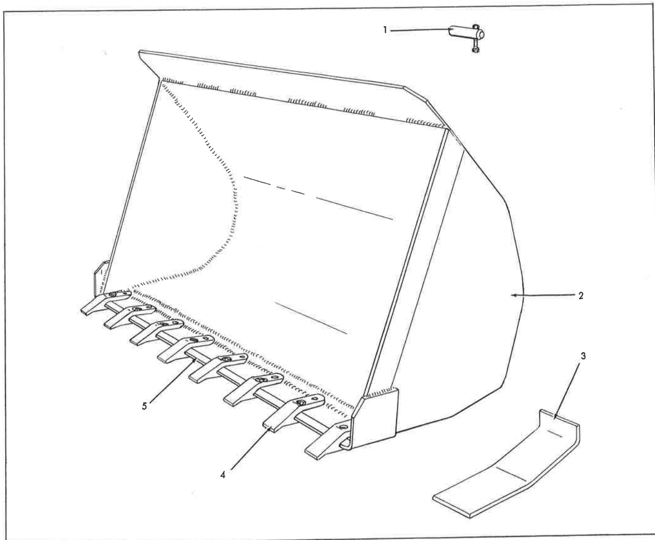
60" BUCKET W/TEETH No. 1066 Loader
