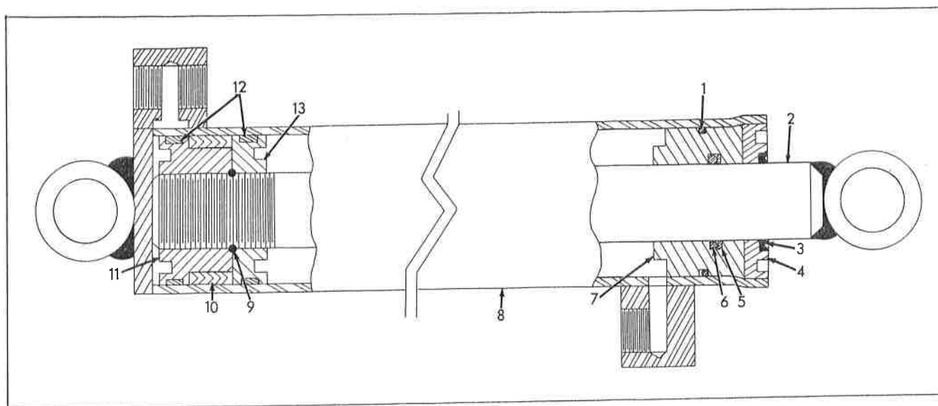
TILT CYLINDER f/No. 1066 Loader Eff. Jan. 1962 Thru March 1966 (w/Threaded Piston)
