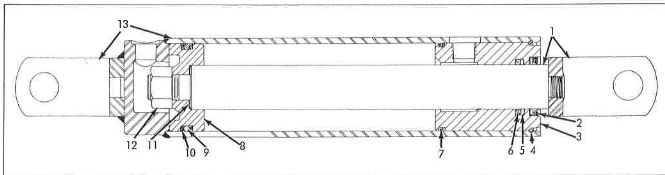
RAM Grapple & Tower f/Scarifier (Eff. June 1961 thru August 1961)
