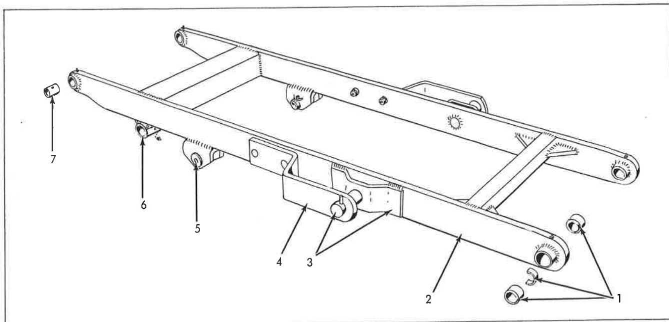
BOOM No. 1066 Loader (Used Prior to June 1965)
