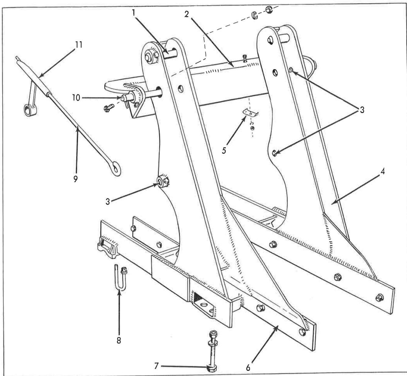
SIDE FRAMES (R. H. & L. H.) No. 1066 Loader (Used Prior to June 1965)
