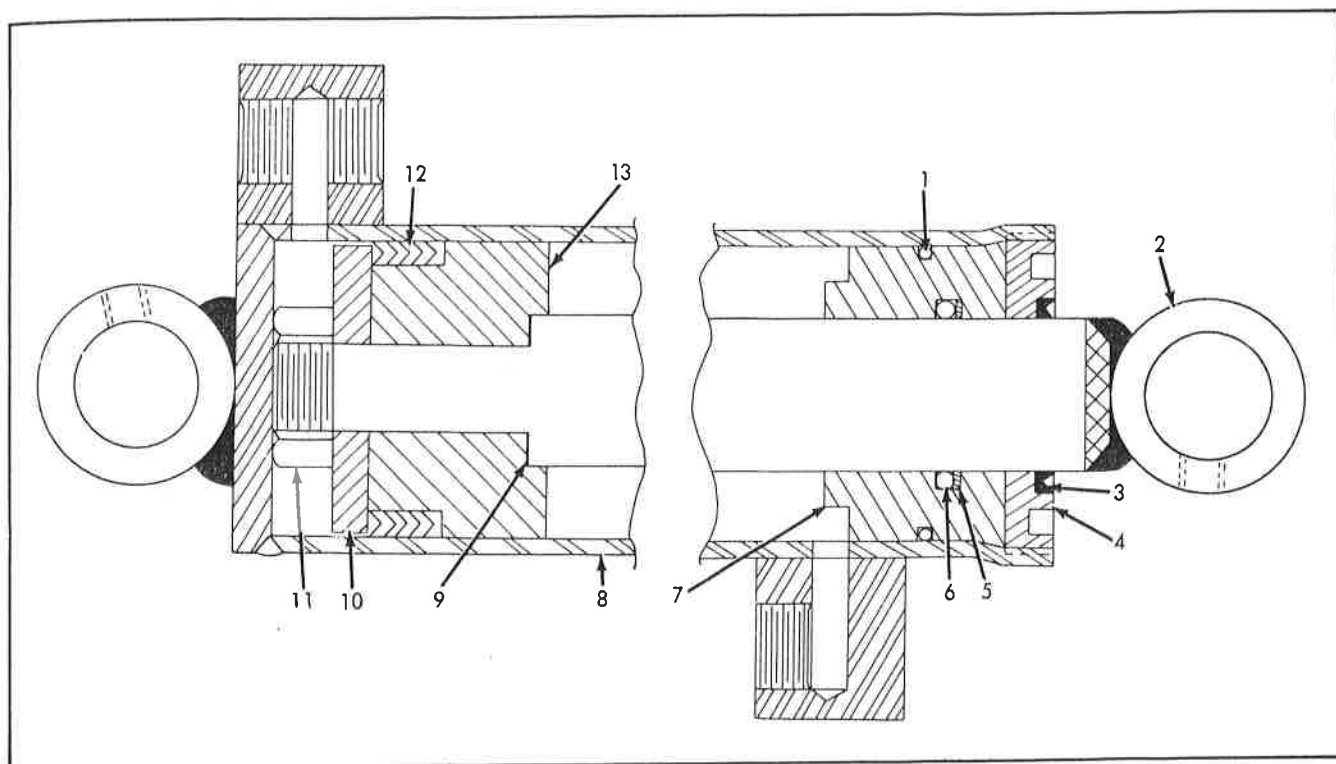
TILT CYLINDER No. 1066 Loader (W/Un-Threaded Piston)
