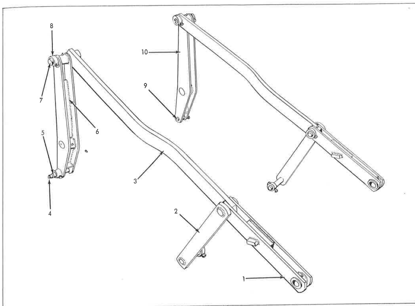
BELLCRANKS & LINKS No. 1066 Loader
