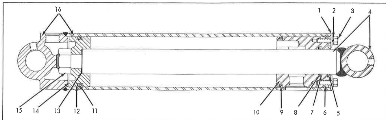
TILT CYLINDER No. 1066 Loader Used Prior To Jan. 1962
