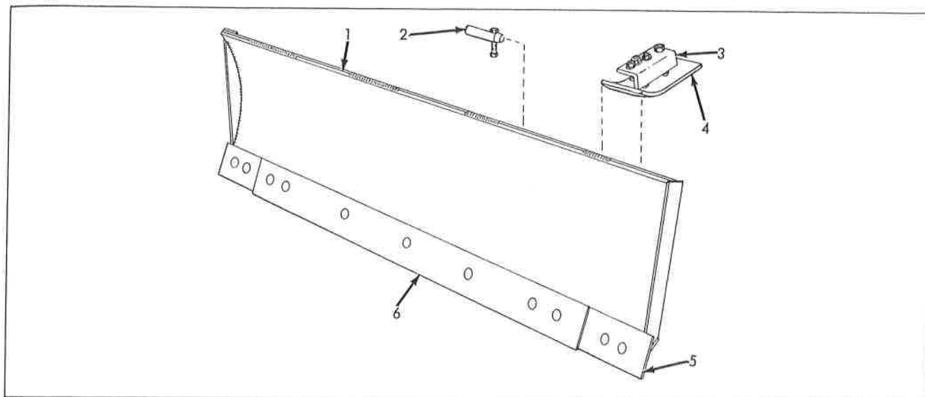
80" DOZER BLADE No. 1066 Loader Attachment
