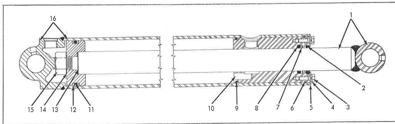
LIFT CYLINDER No. 1066 Loader Used Prior To Jan. 1962
