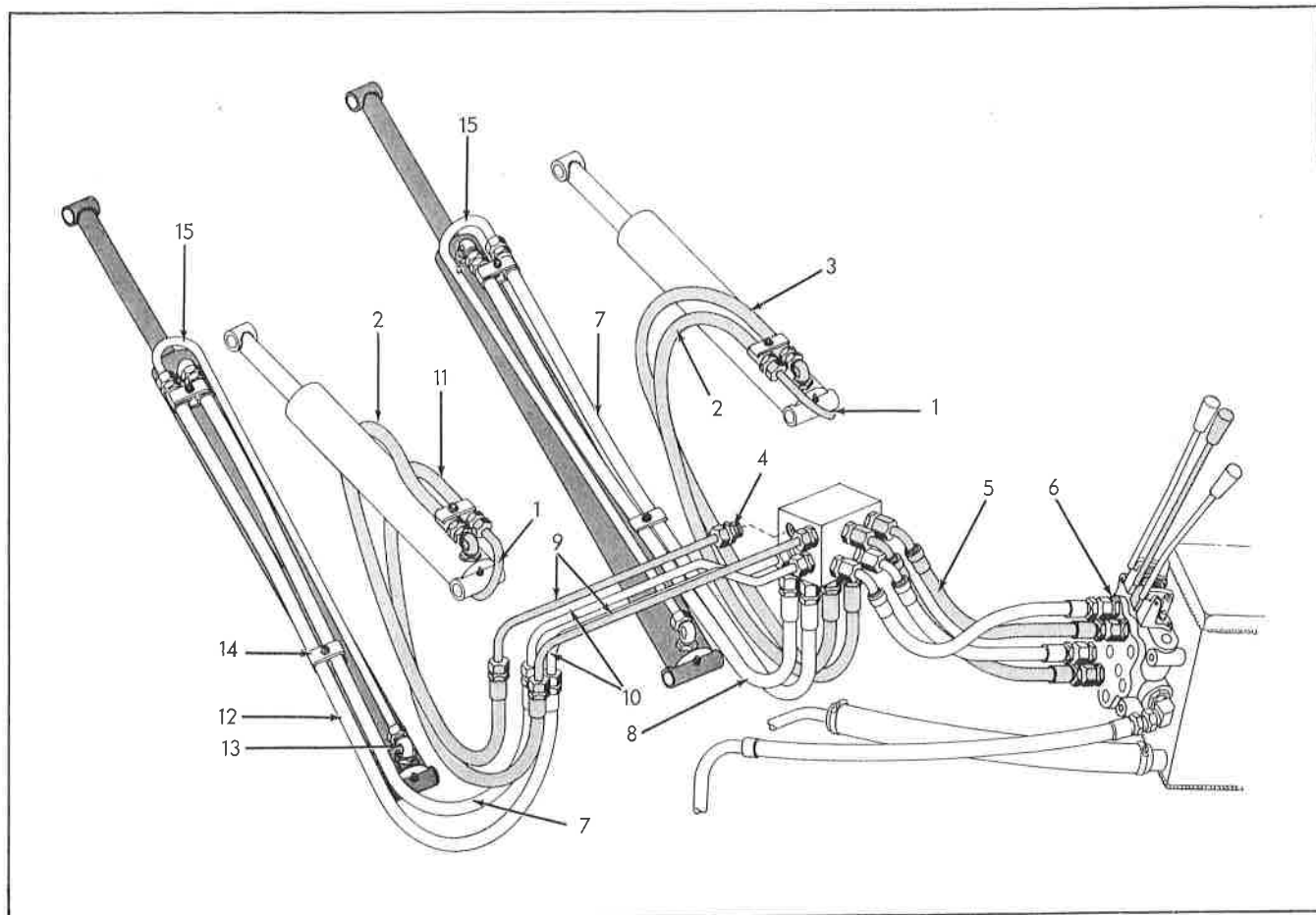
HOSES & TUBES No. 1066 Loader
