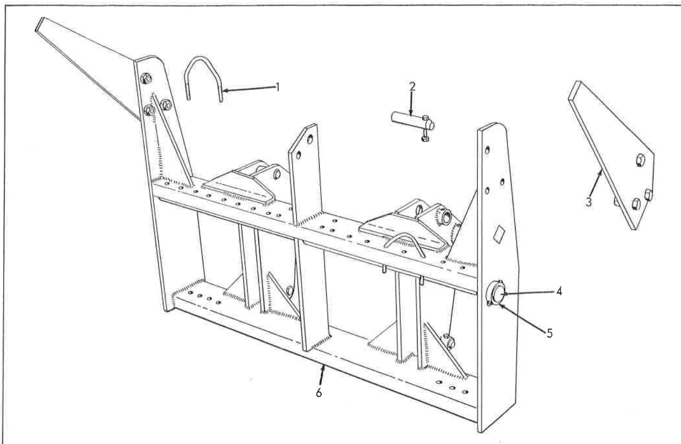
CARRIAGE No. 1066 Loader Attachment
