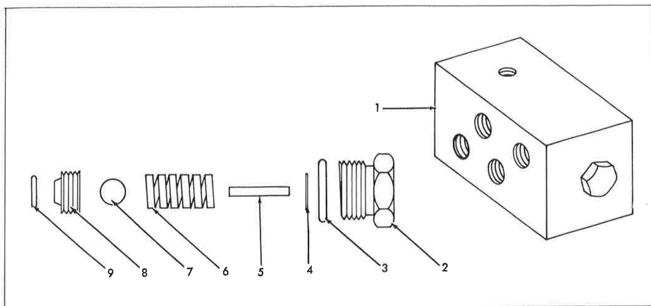
MANIFOLD No. 1066 Loader
