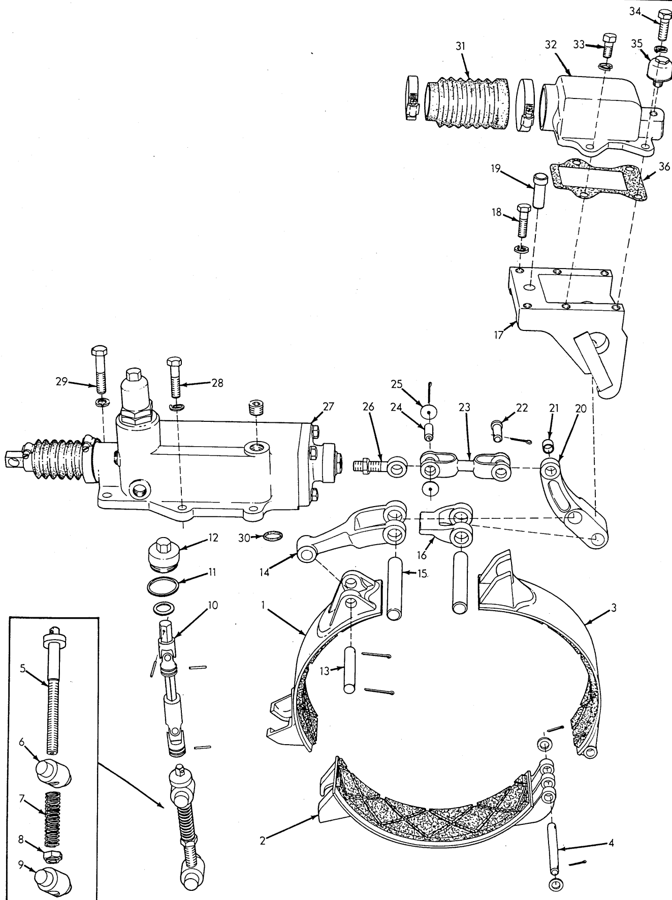
BRAKES (First type)
