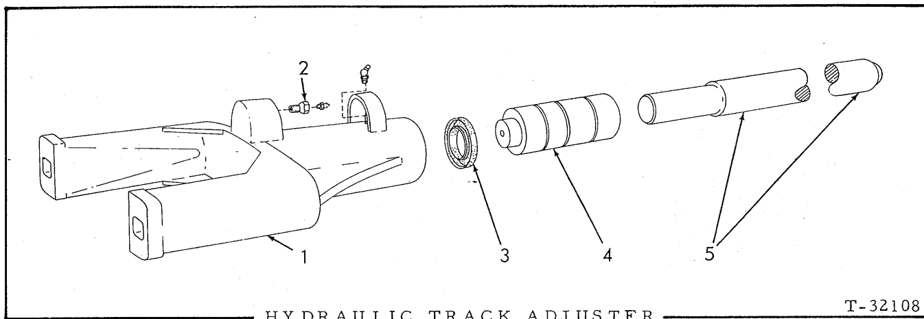
HYDRAULIC TRACK ADJUSTER
