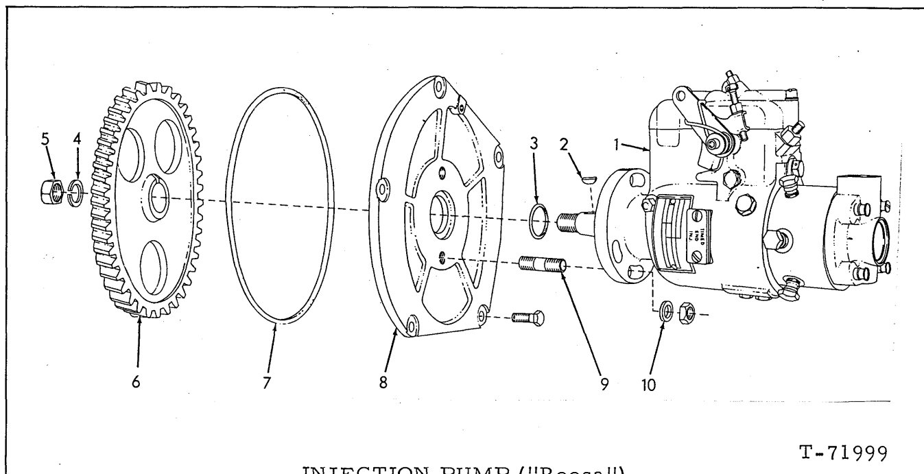
INJECTION PUMP ("Roosa")
