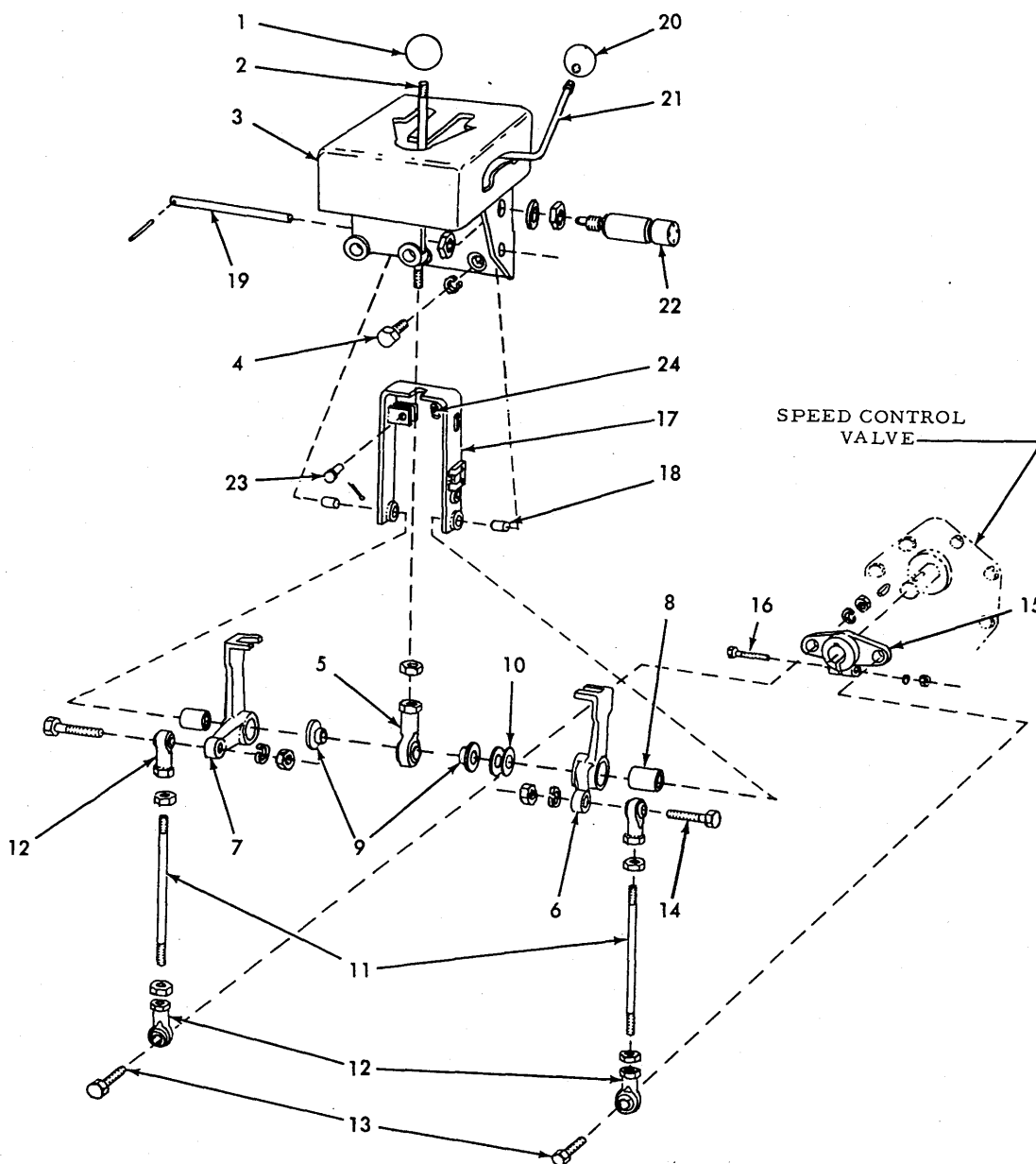
SPEED CONTROL LINKAGE
