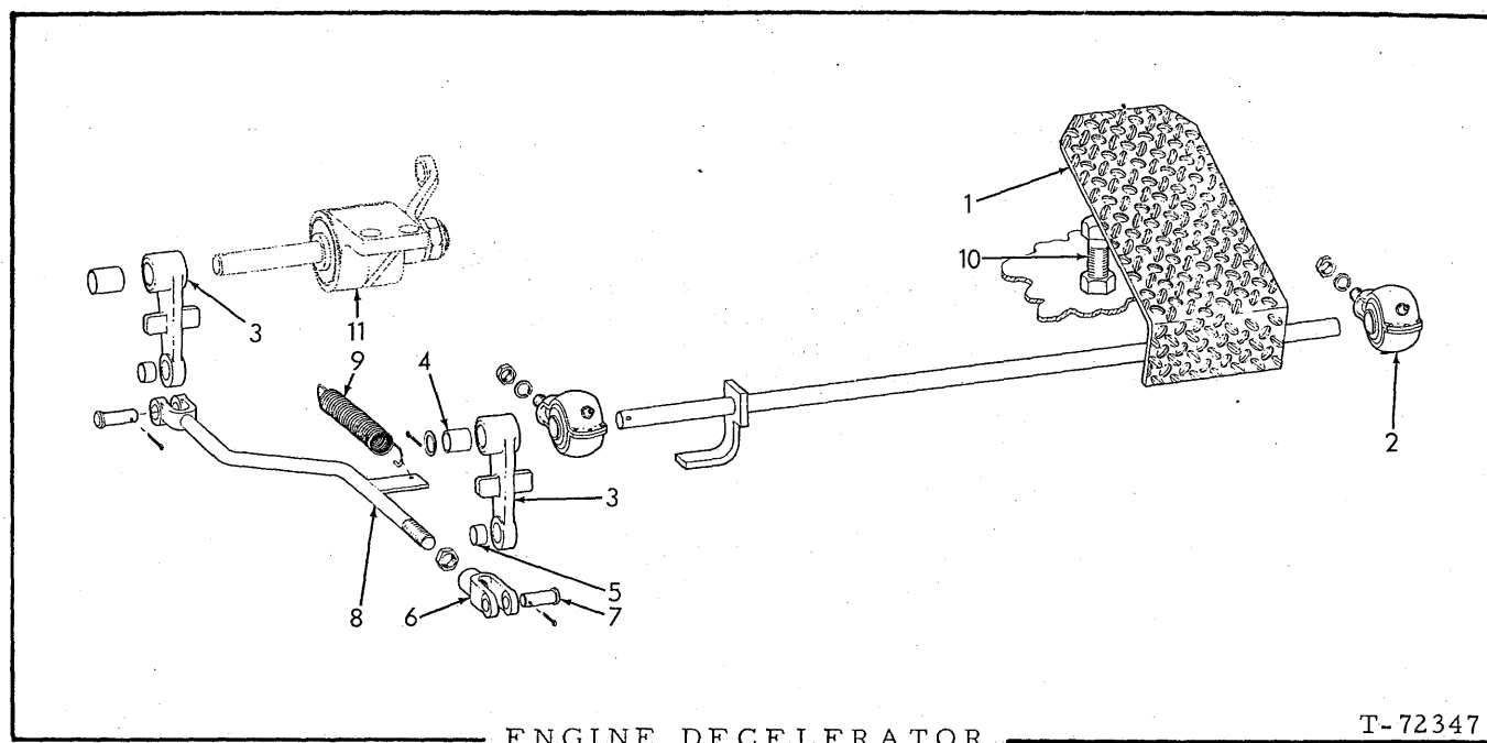
ENGINE DECELERATOR
