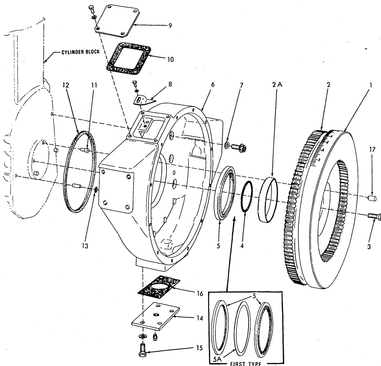
FLYWHEEL AND HOUSING
