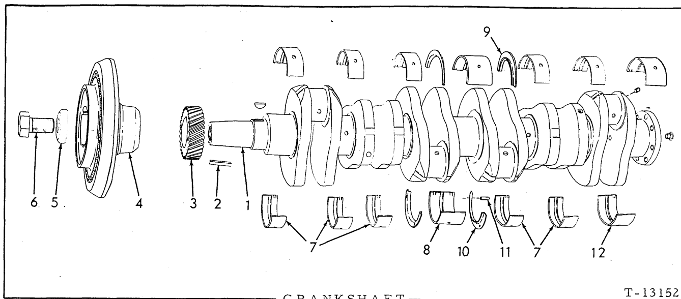
CRANKSHAFT
