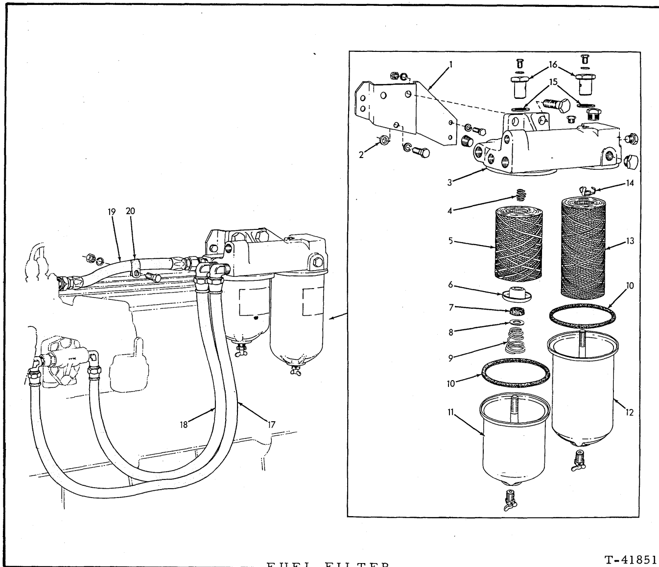
FUEL FILTER
