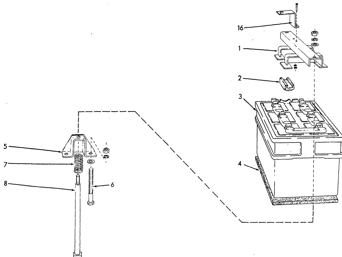
BATTERIES AND CABLES (First type)
