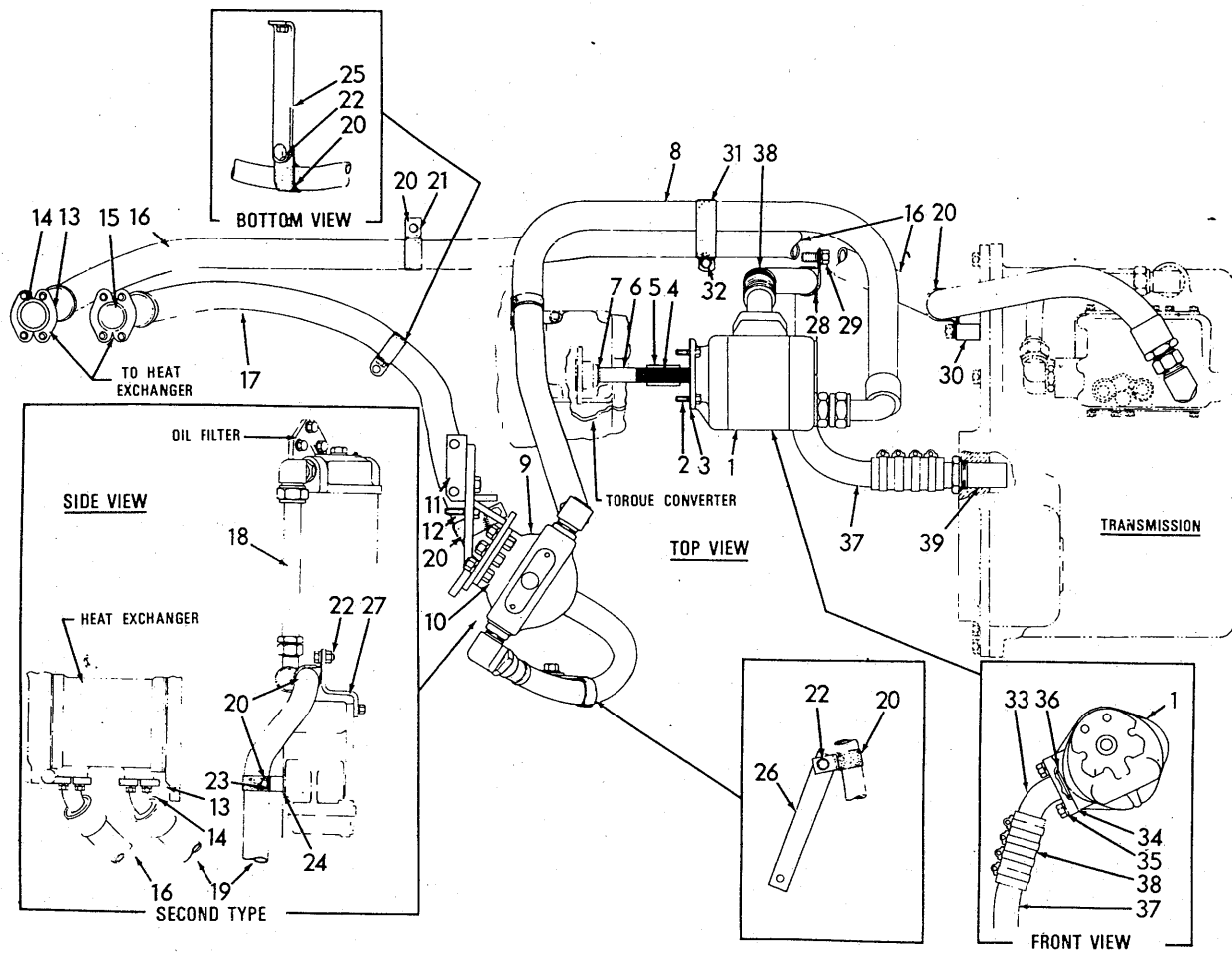
TRANSMISSION OIL PUMP AND FILTER (Second type)
