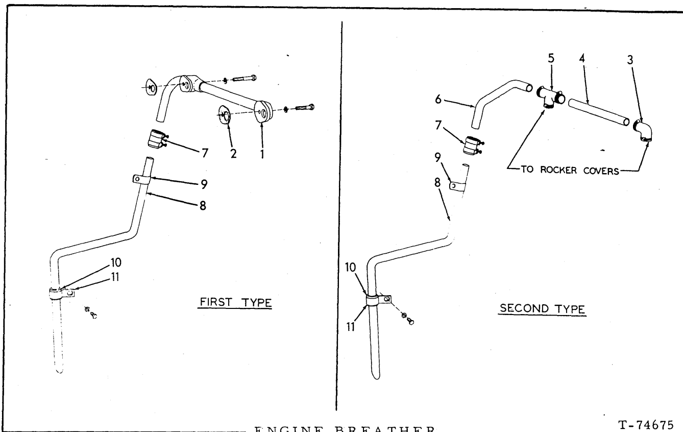
ENGINE BREATHER
