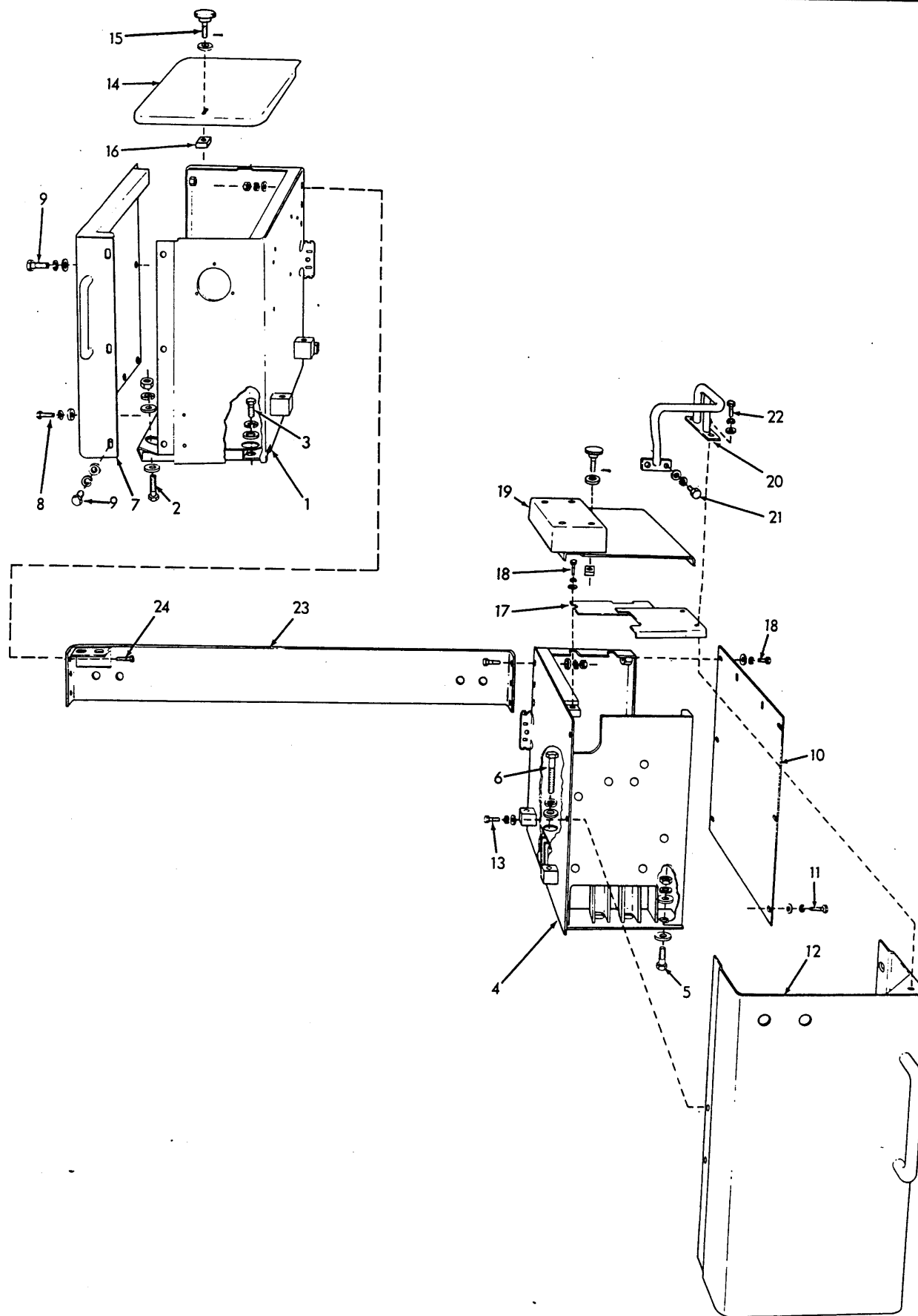
BATTERY BOXES (First type)
