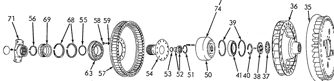
TURBINE AND IMPELLER WHEEL
