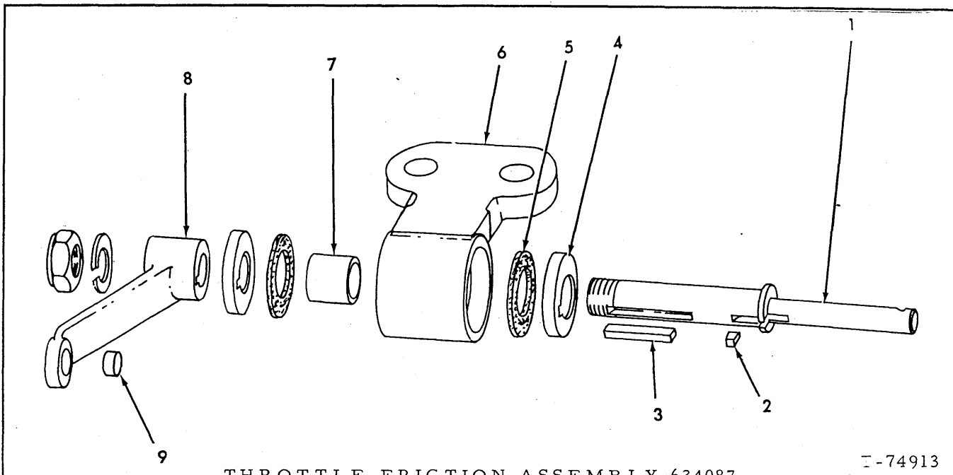
THROTTLE FRICTION ASSEMBLY 634087
