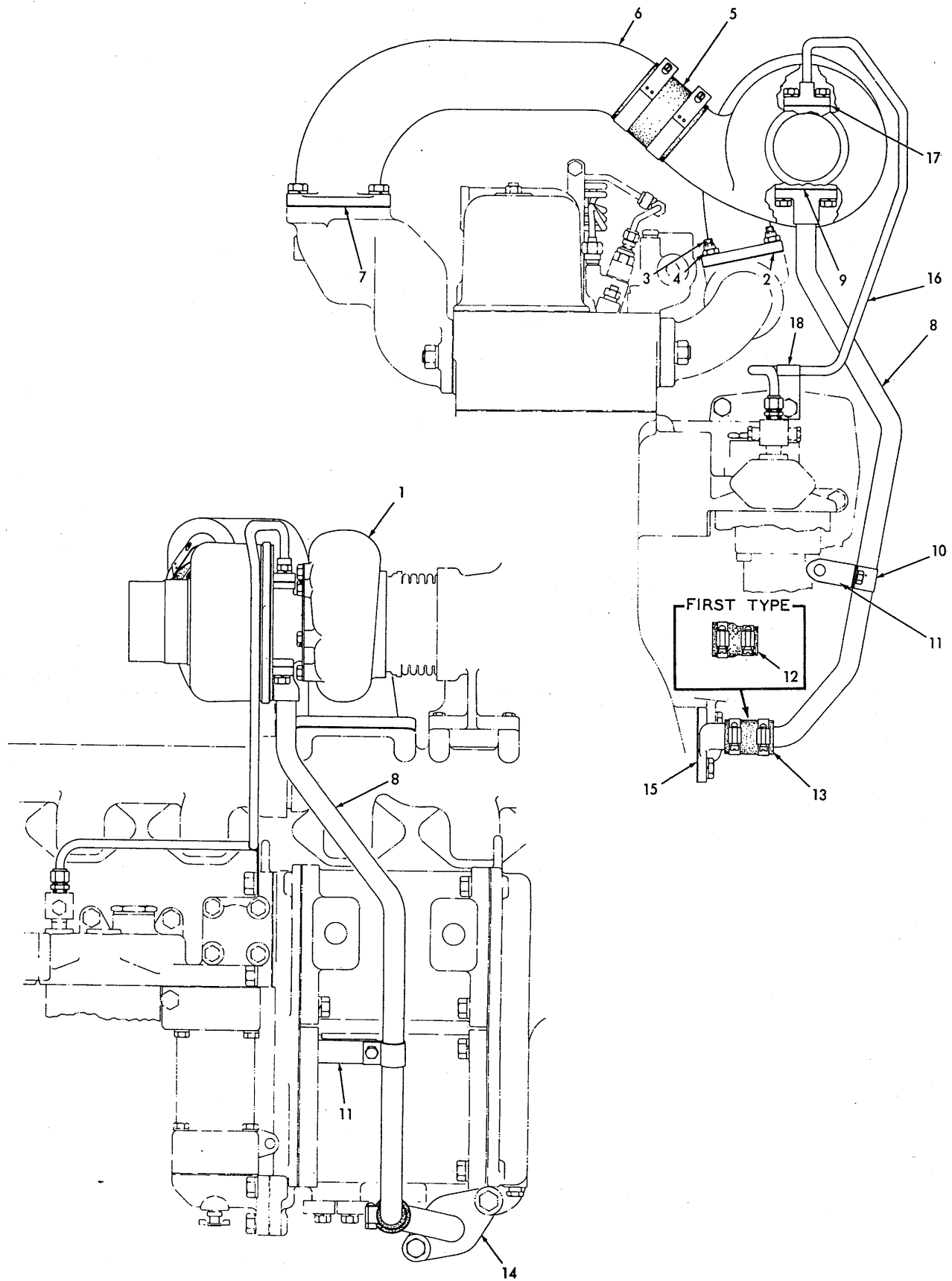
TURBOCHARGER
