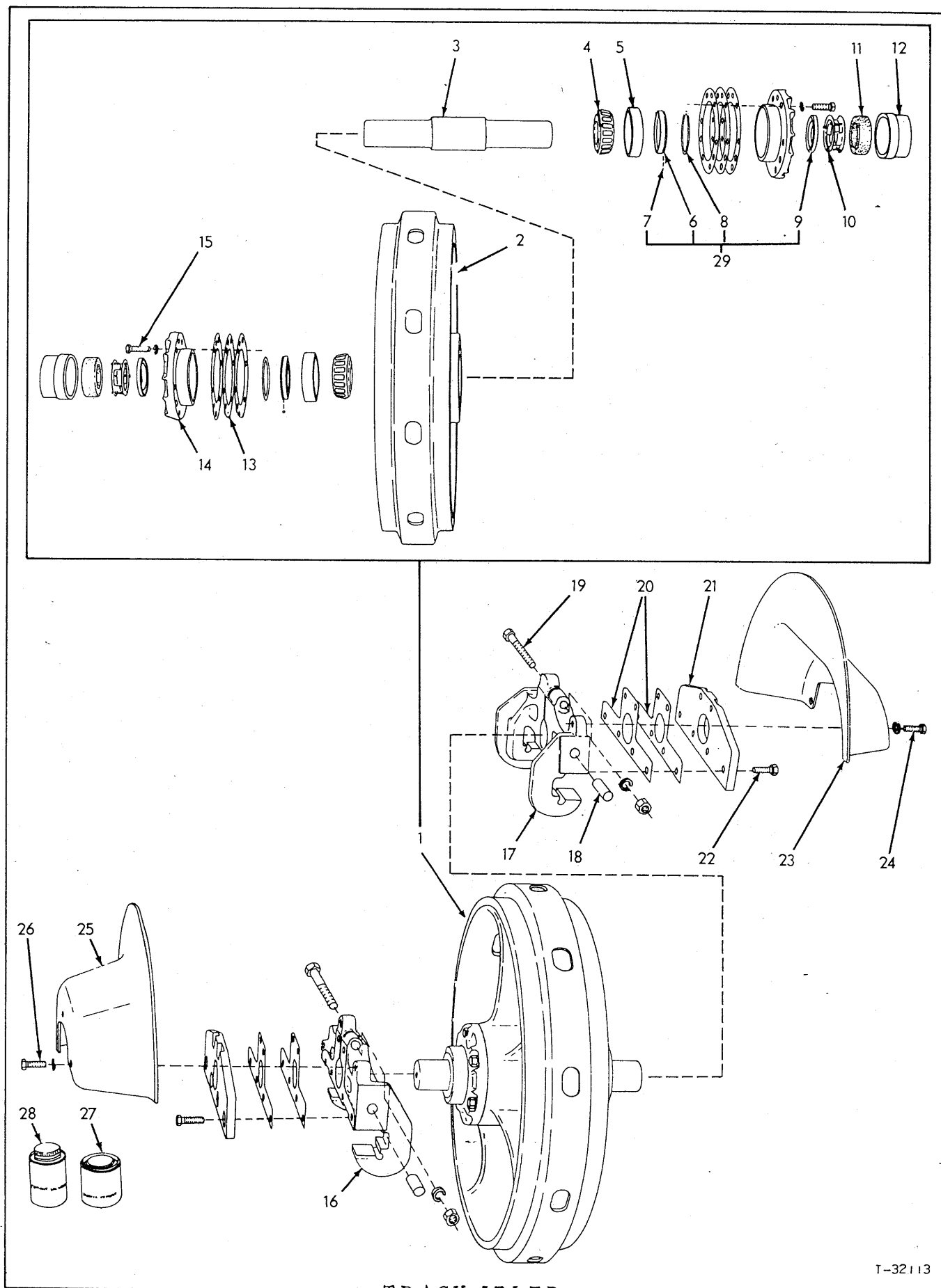
TRACK IDLER
