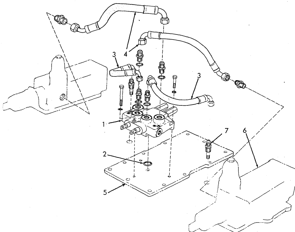
CONTROL VALVE AND LINES
