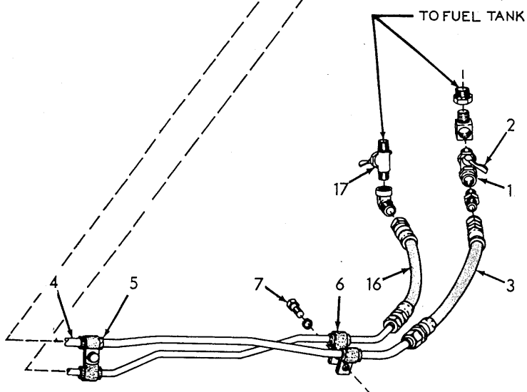
FUEL LINES (First type)
