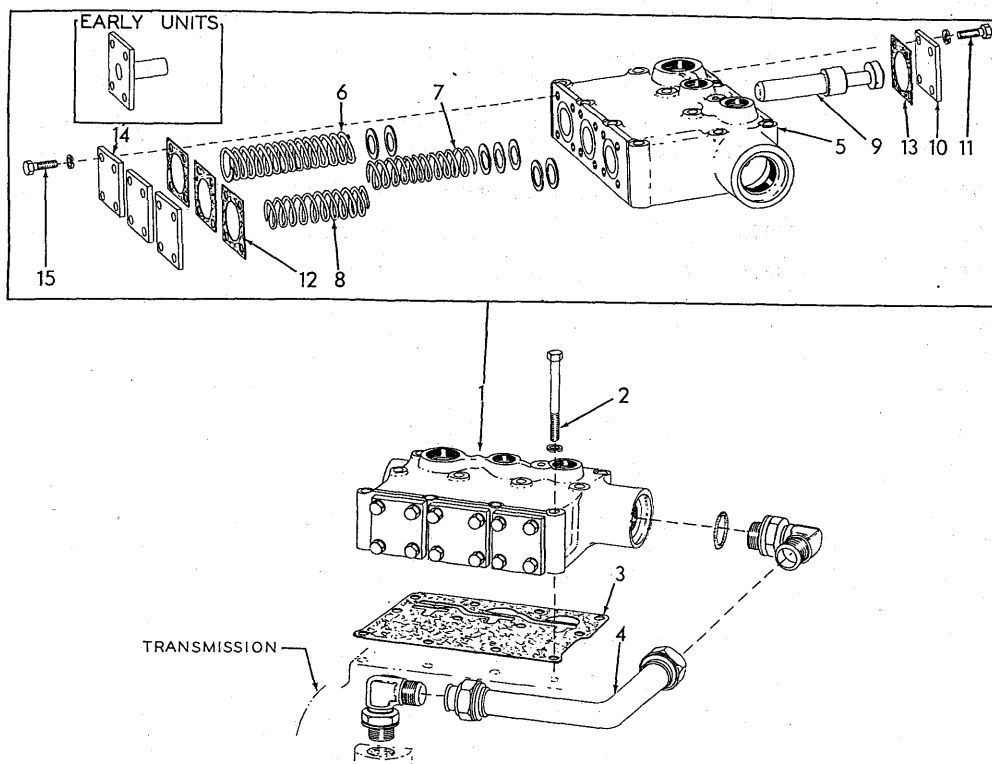
TRANSMISSION PRESSURE RELIEF VALVE
