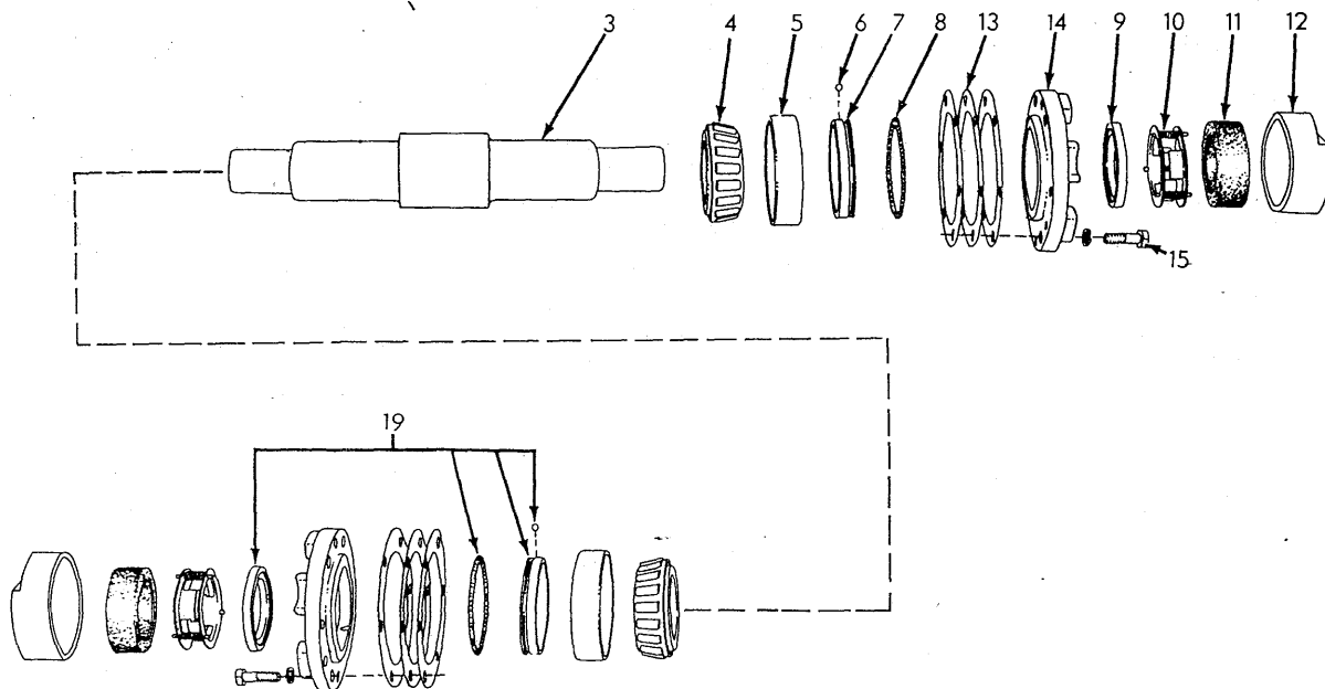
TRACK ROLLER (First type)
