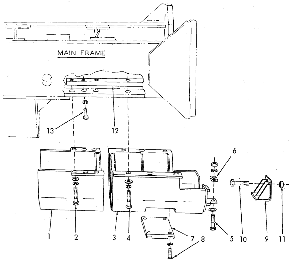
TRANSMISSION GUARDS
