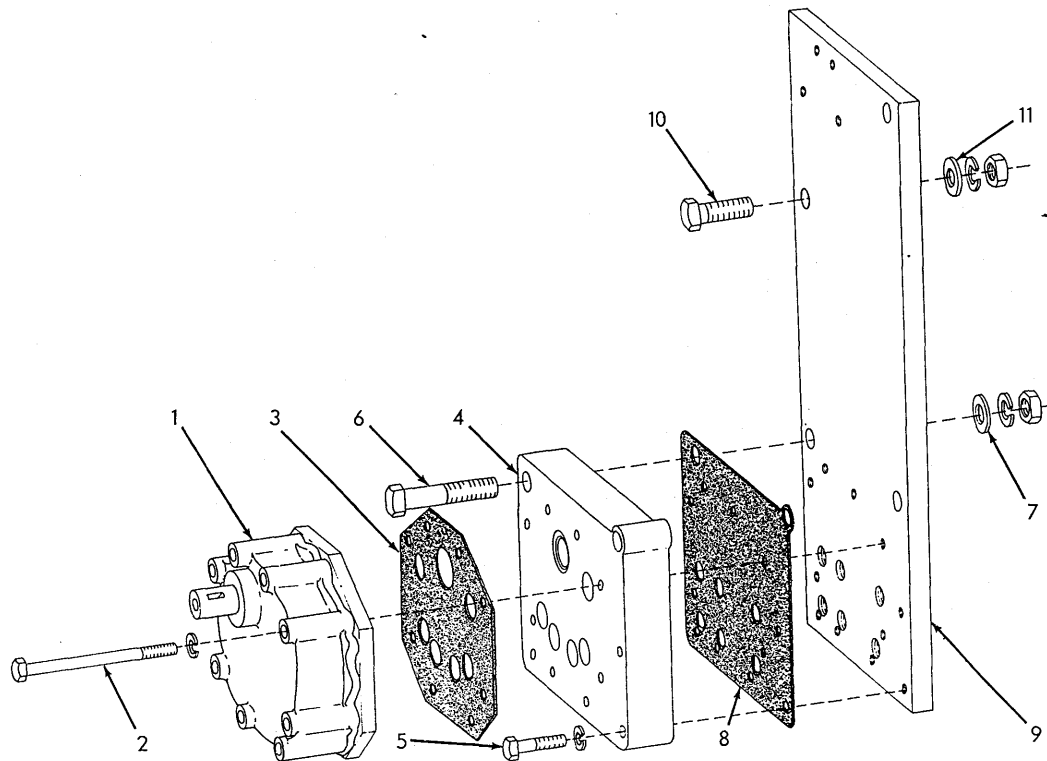
SPEED CONTROL VALVE
