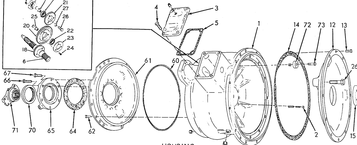
HOUSING
