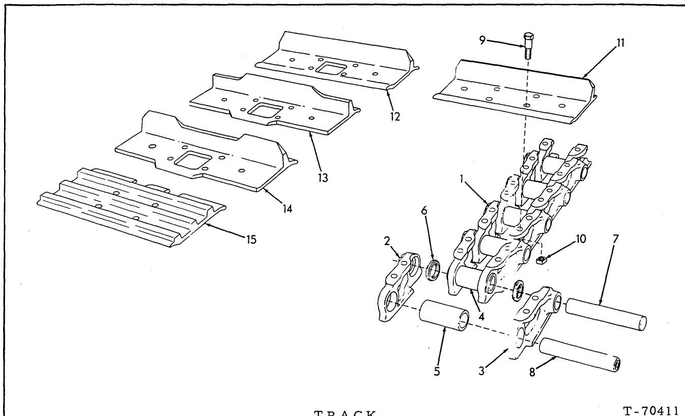
TRACK
