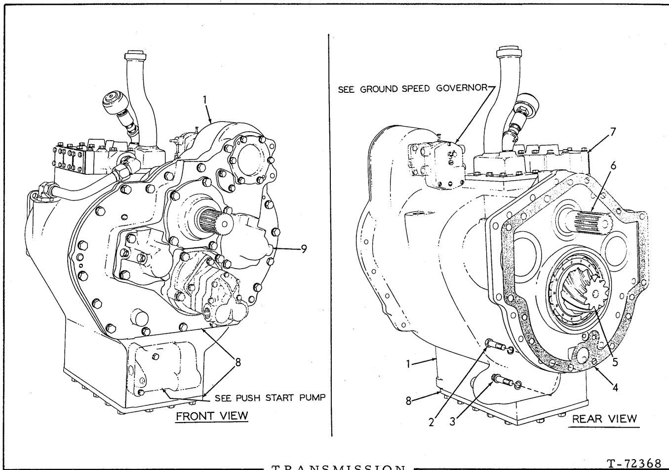
TRANSMISSION
