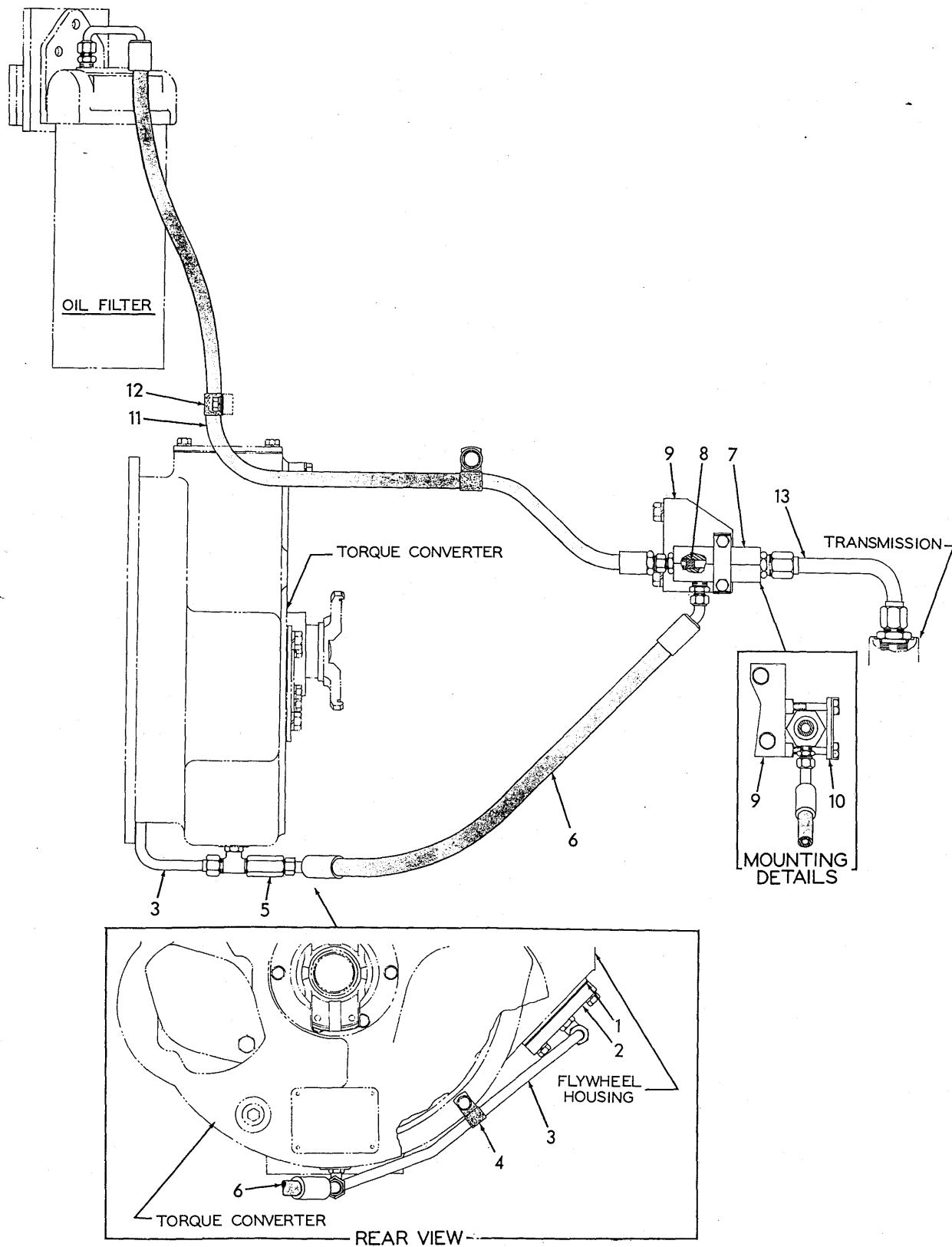
TORQUE CONVERTER AND FLYWHEEL HOUSING DRAIN T-74883
