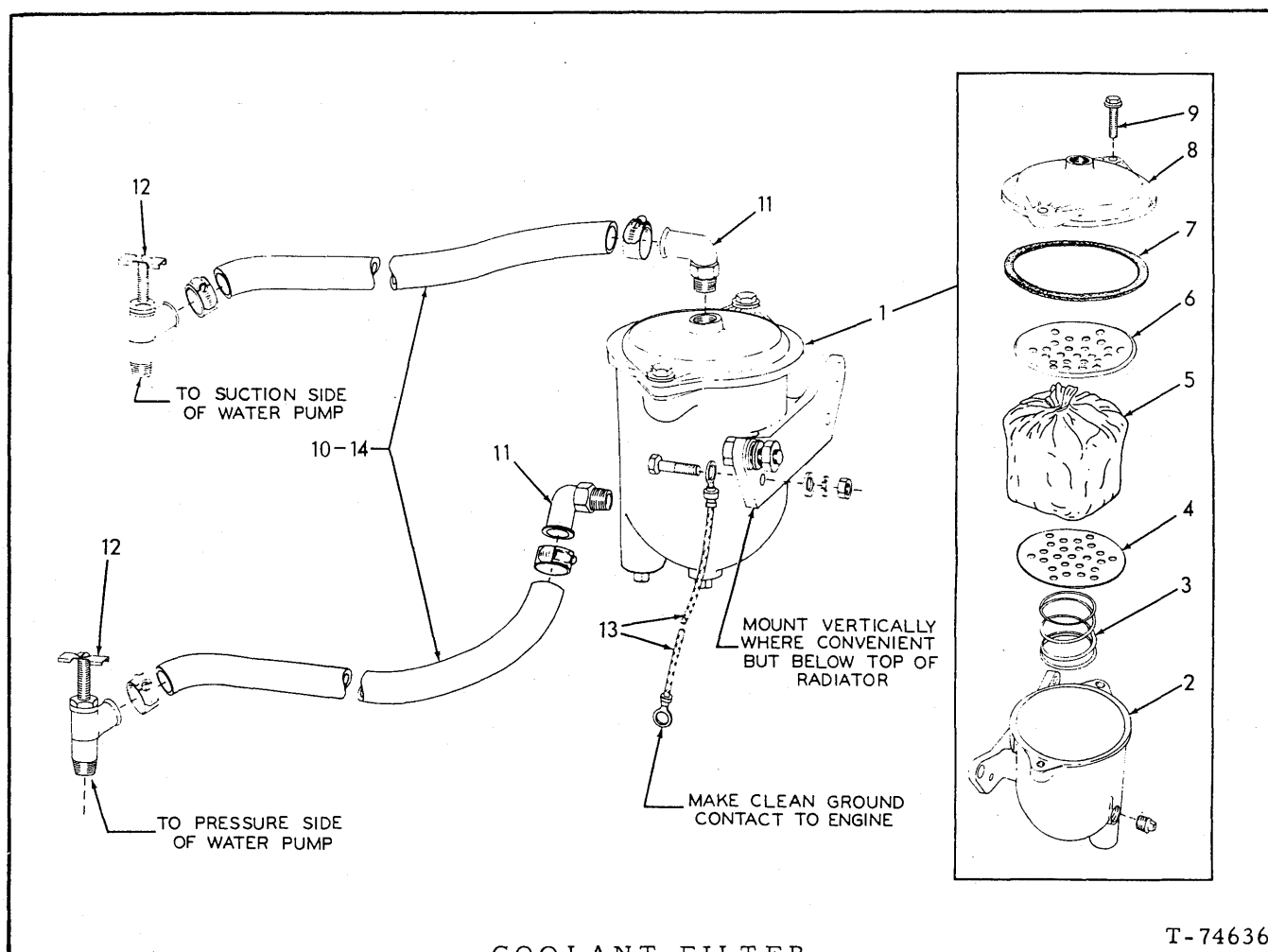
COOLANT FILTER
