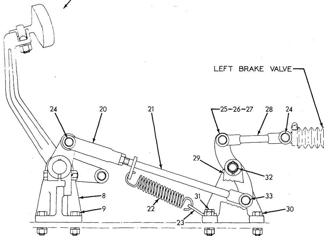
— BRAKE CONTROL (First type) —
