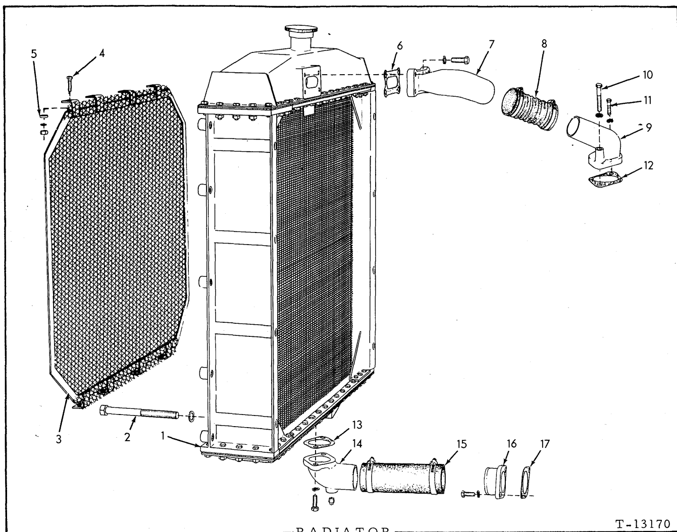
RADIATOR
