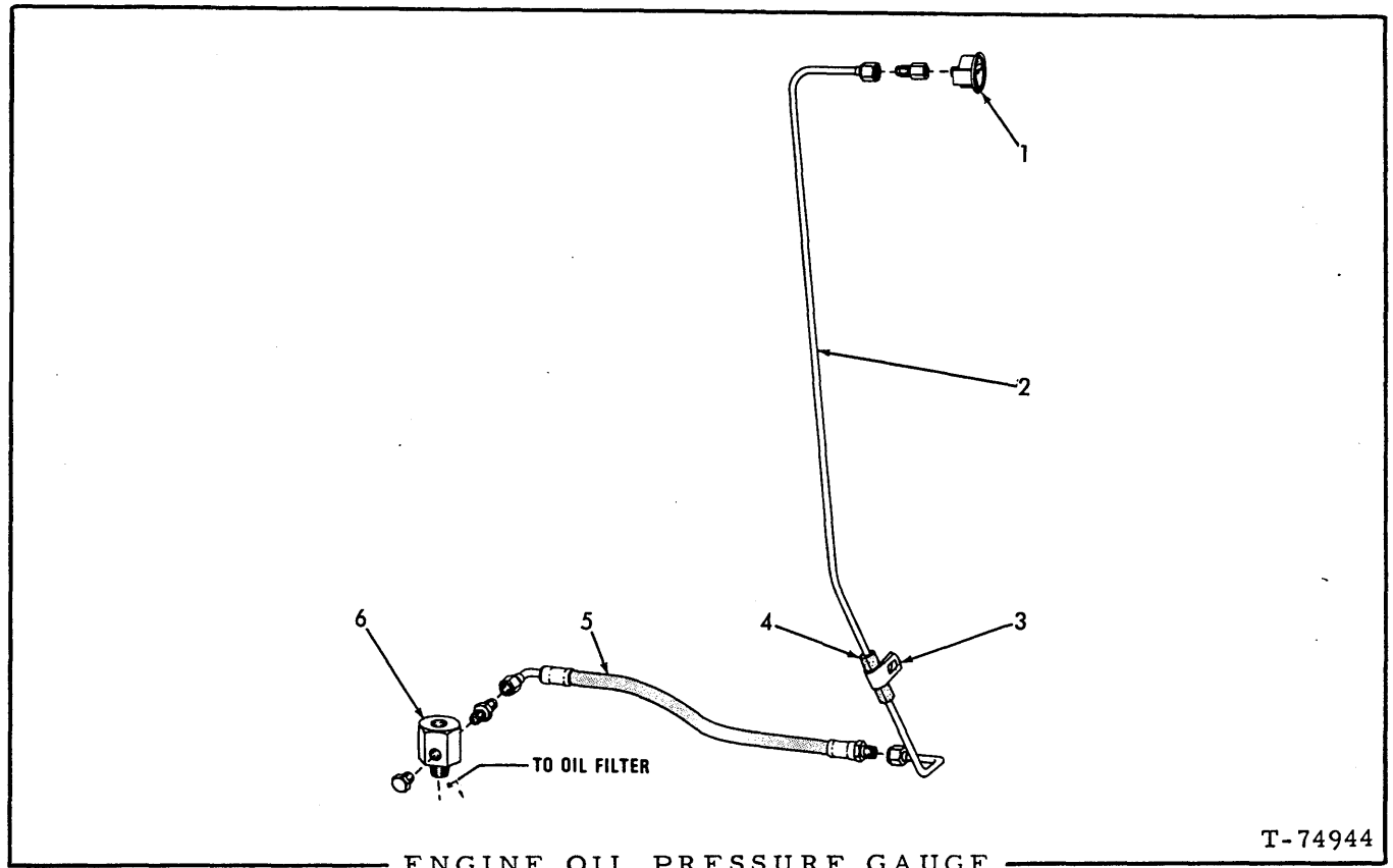
ENGINE OIL PRESSURE GAUGE
