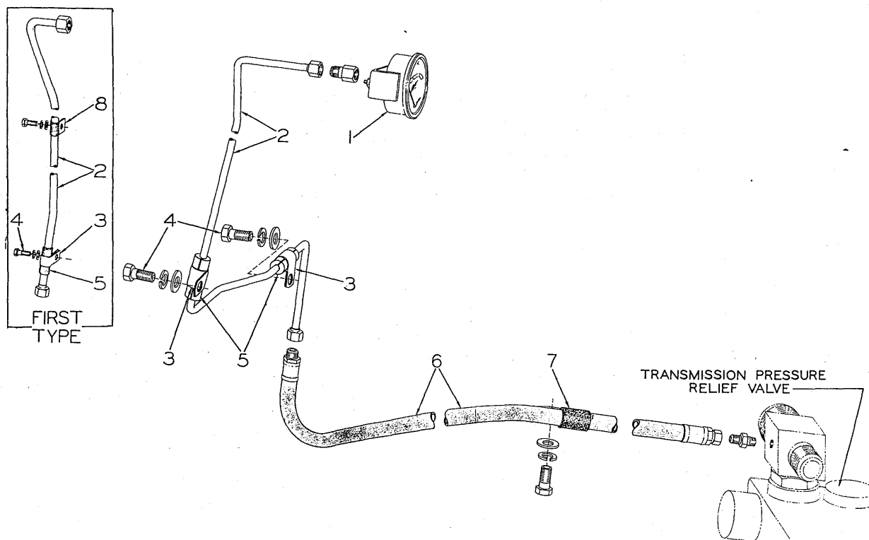
TRANSMISSION LUBRICATING OIL PRESSURE GAUGE T-41935
