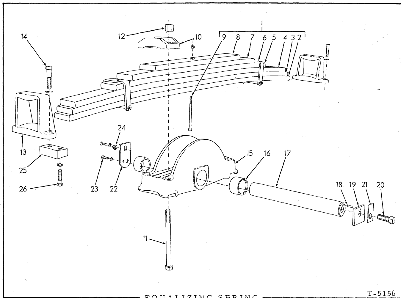
EQUALIZING SPRING
