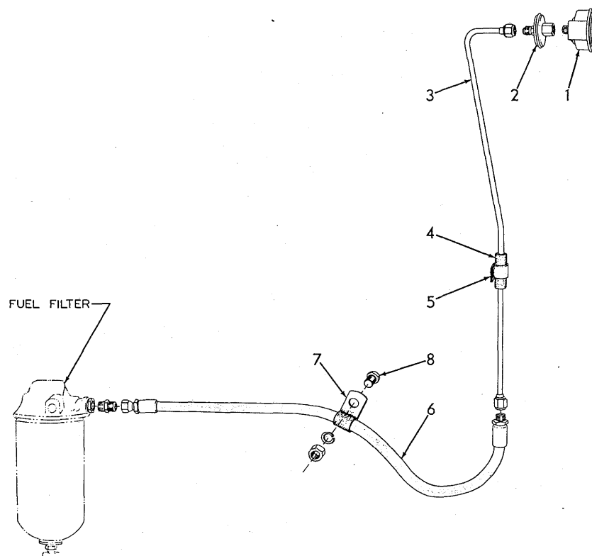
FUEL PRESSURE GAUGE
