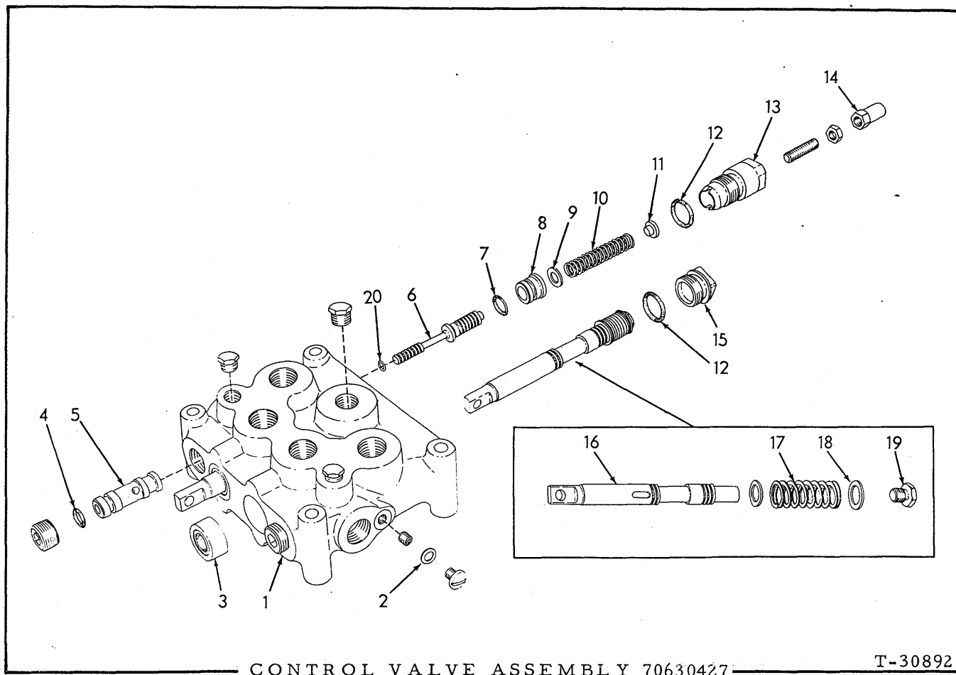
CONTROL VALVE ASSEMBLY 70630427
