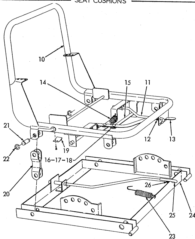
SEAT ASSEMBLY 70632053
