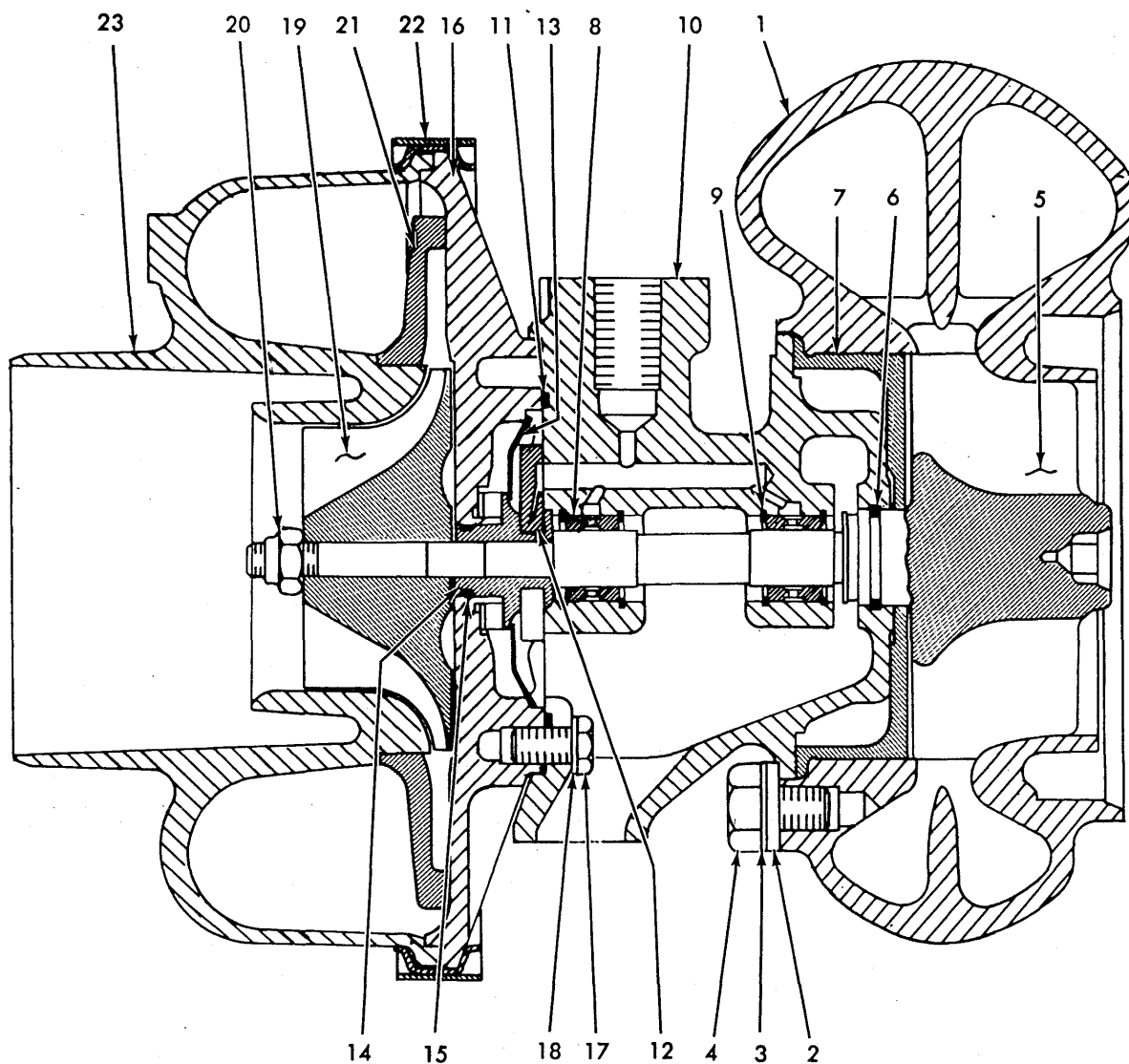
TURBOCHARGER ASSEMBLY
