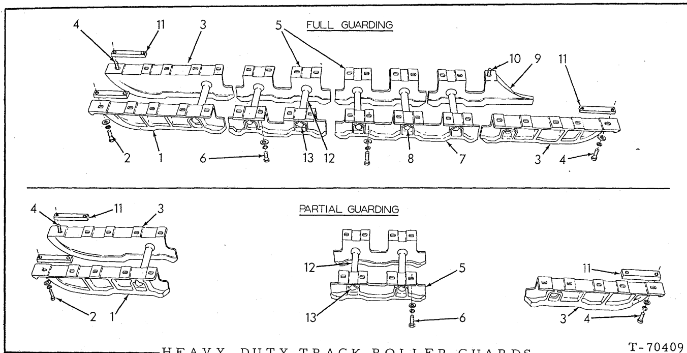
HEAVY-DUTY TRACK ROLLER GUARDS
