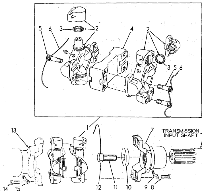
UNIVERSAL JOINT
