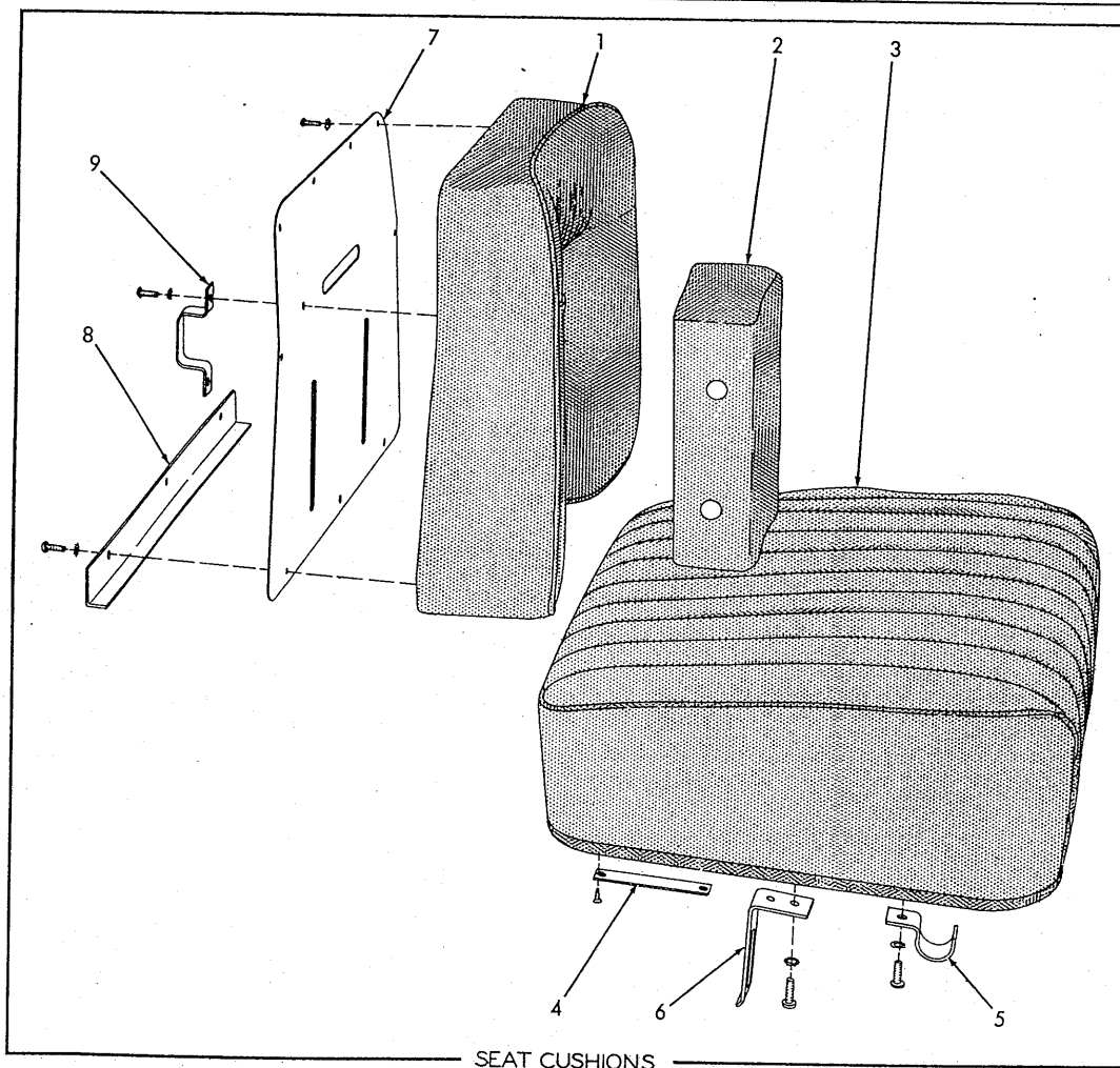
SEAT CUSHIONS
