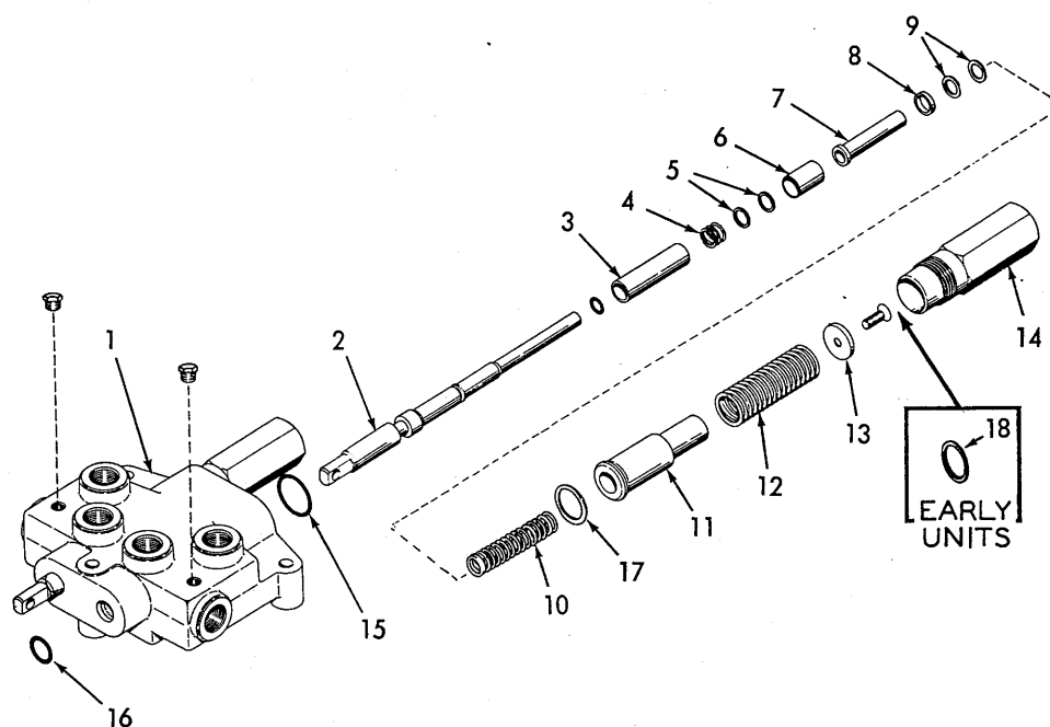
CONTROL VALVE ASSEMBLY 70651432
