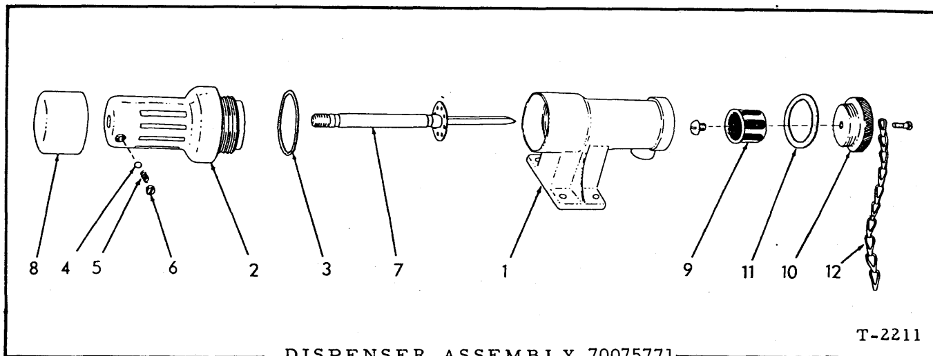
DISPENSER ASSEMBLY 70075771
