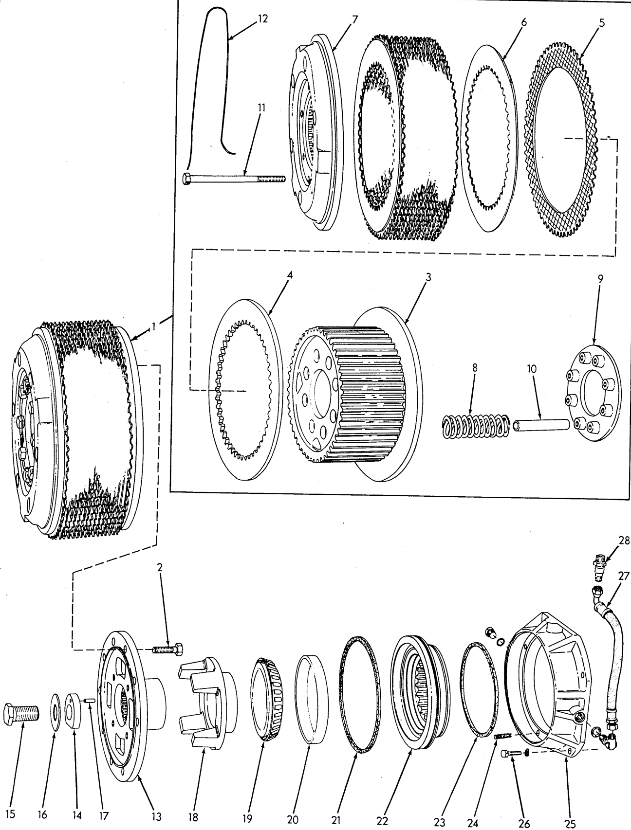
STEERING CLUTCHES
