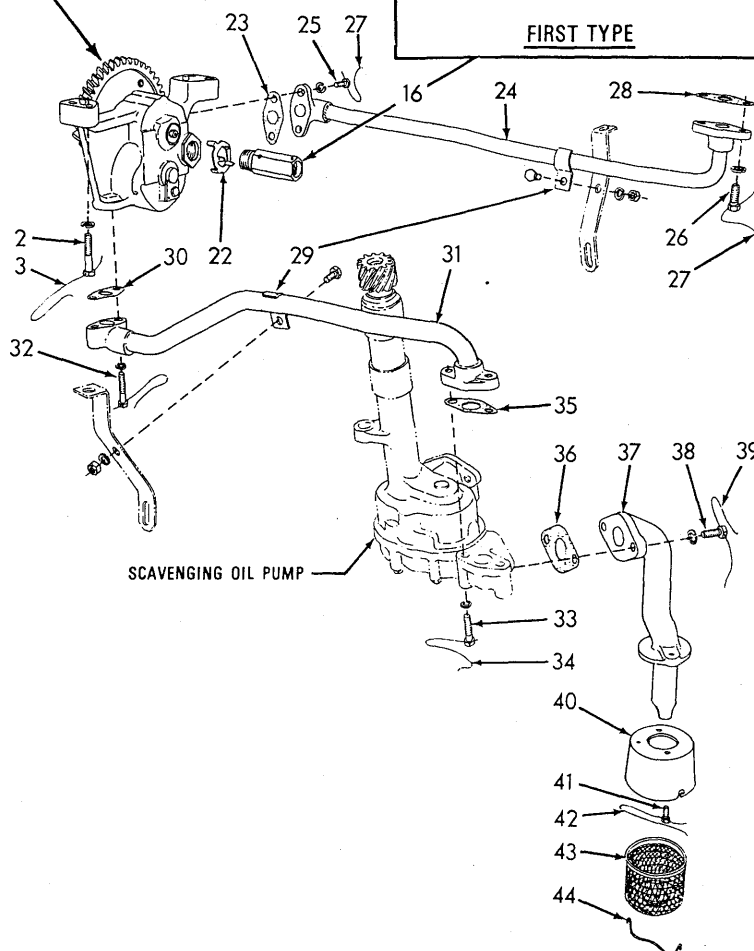
PRESSURE OIL PUMP
