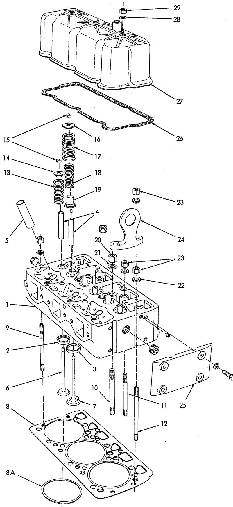
CYLINDER HEAD
