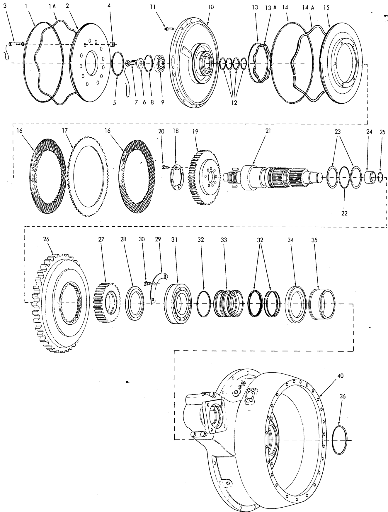
TORQUE CONVERTER PARTS (Front section)
