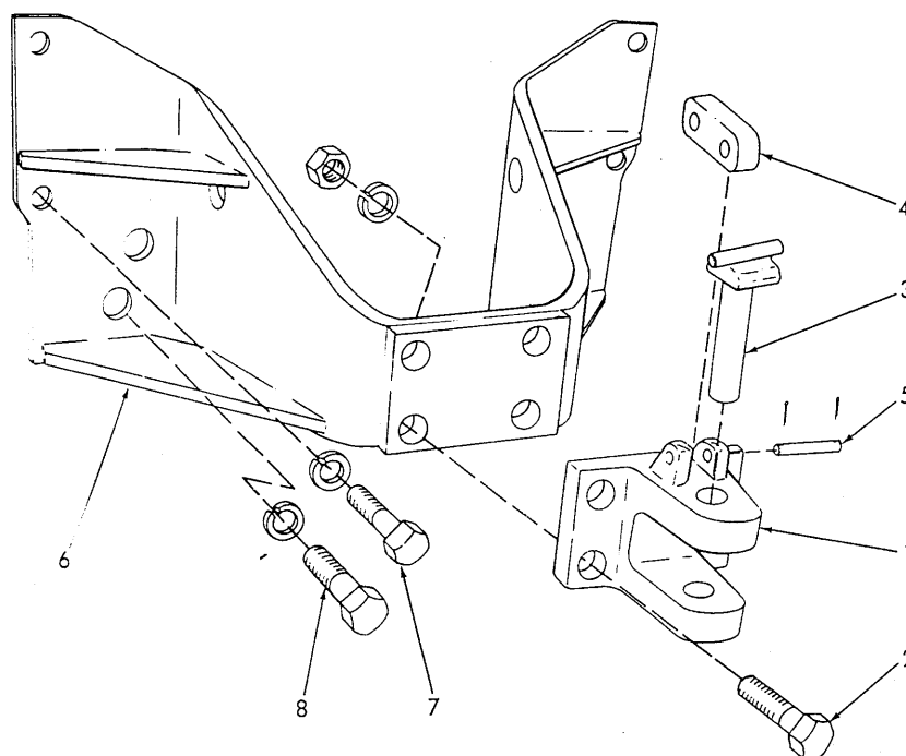
DRAWBAR (Fixed-type)
