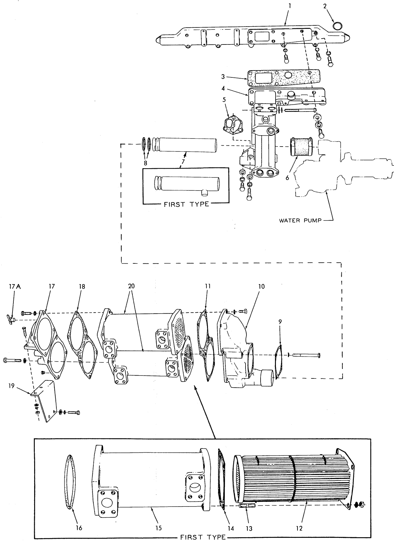
— WATER INLET MANIFOLD AND HEAT EXCHANGER —
