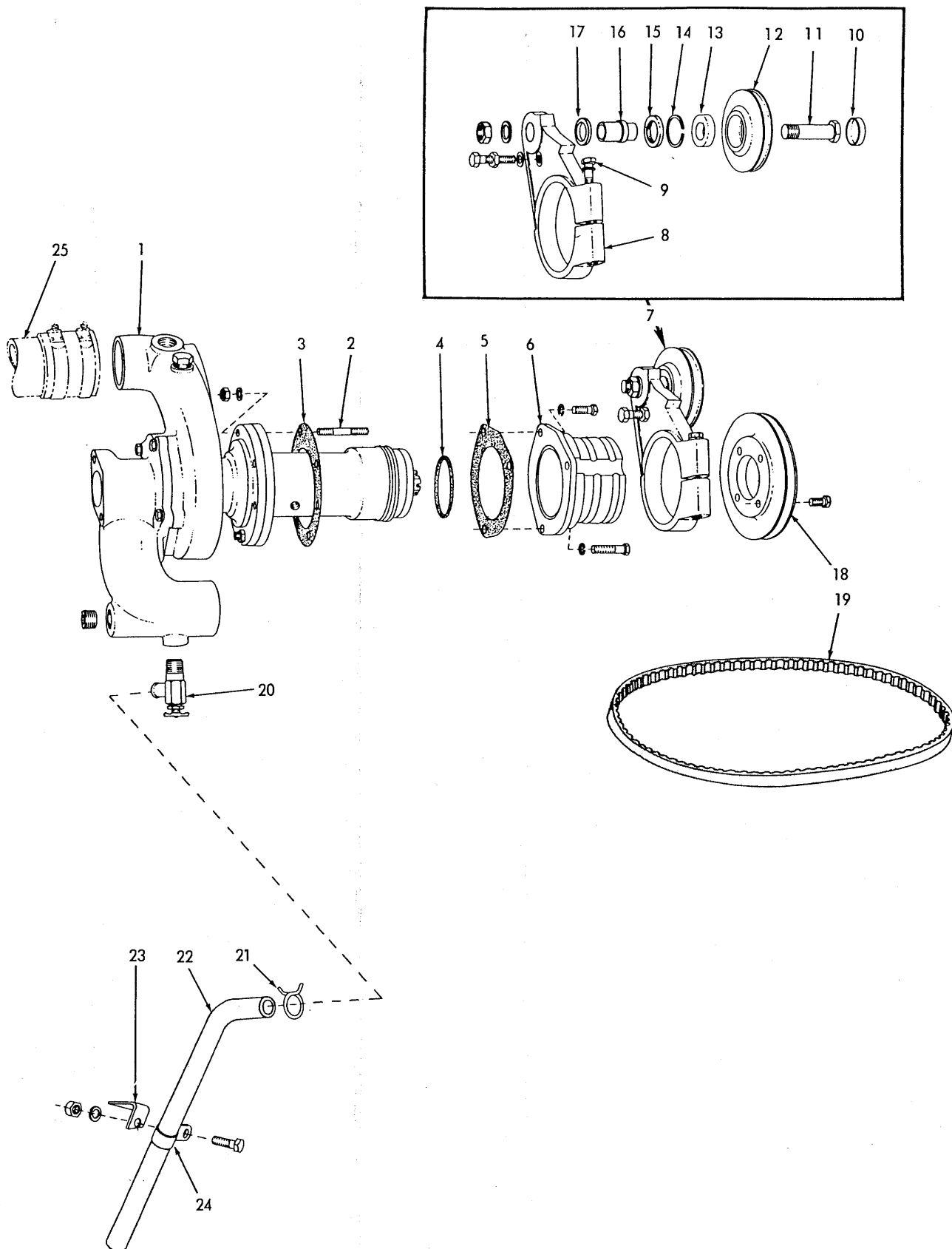
WATER PUMP (Second type)
