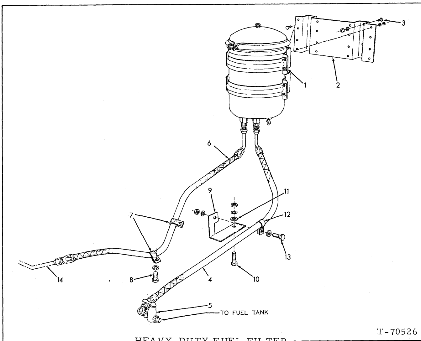
HEAVY-DUTY FUEL FILTER
