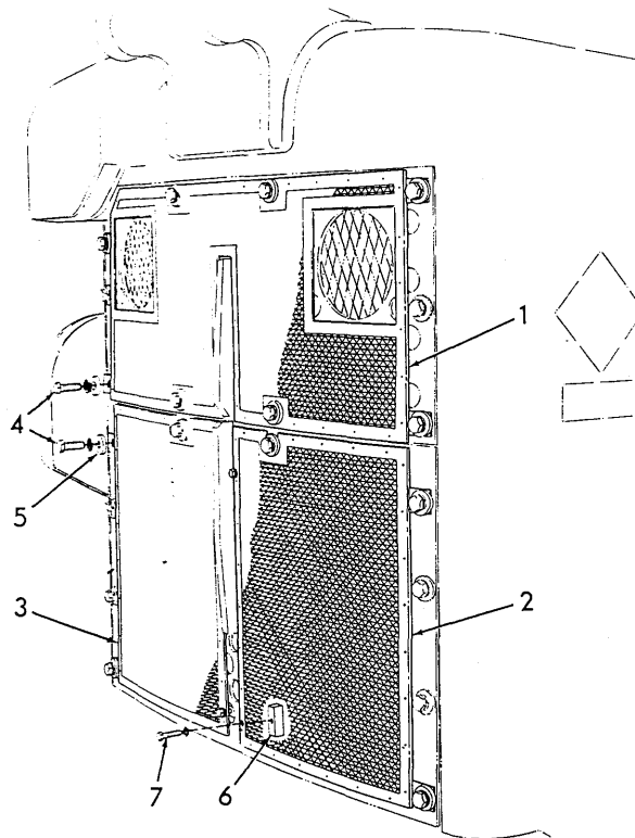
GRILLE SCREEN (For Cable Guard)
