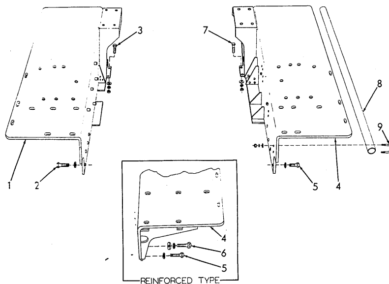
REAR FENDERS
