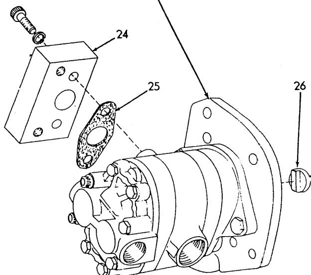
STEERING PUMP ASSEMBLY 70654180 ("Cessna")
