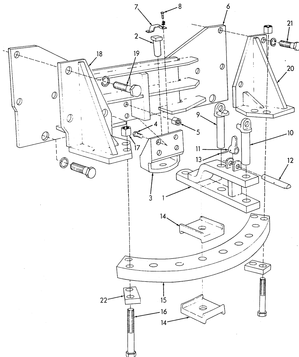
DRAWBAR (Swing-type)
