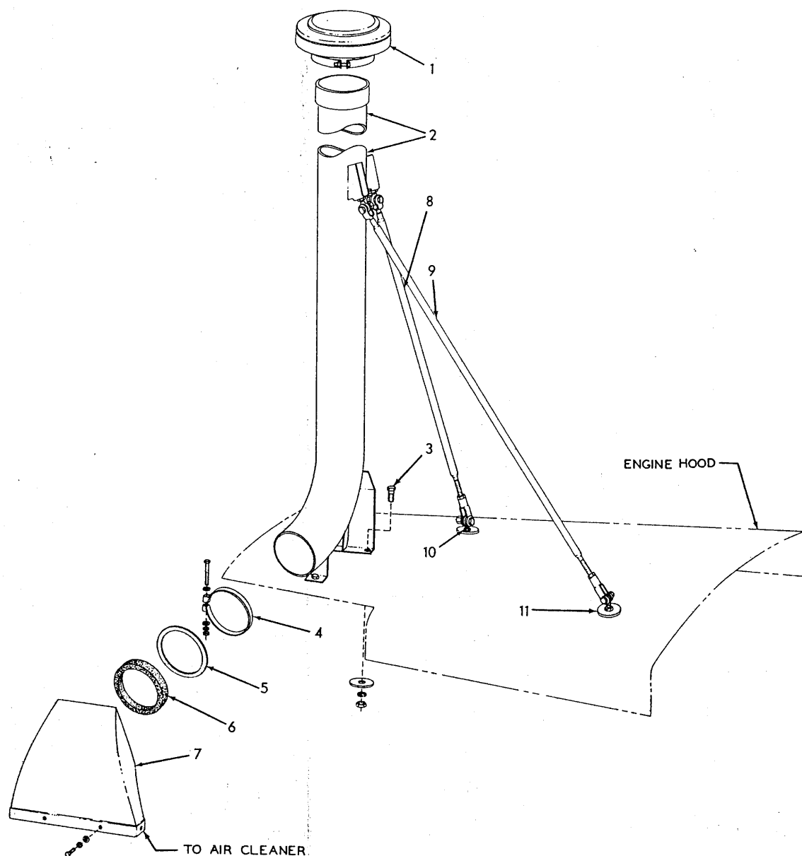
AIR INTAKE EXTENSION
