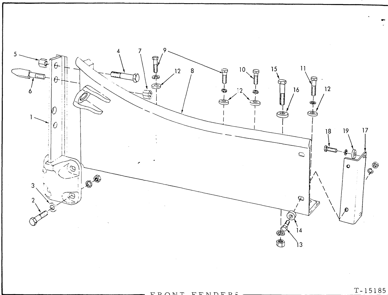
FRONT FENDERS
