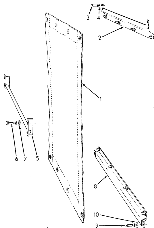
RADIATOR CURTAIN
