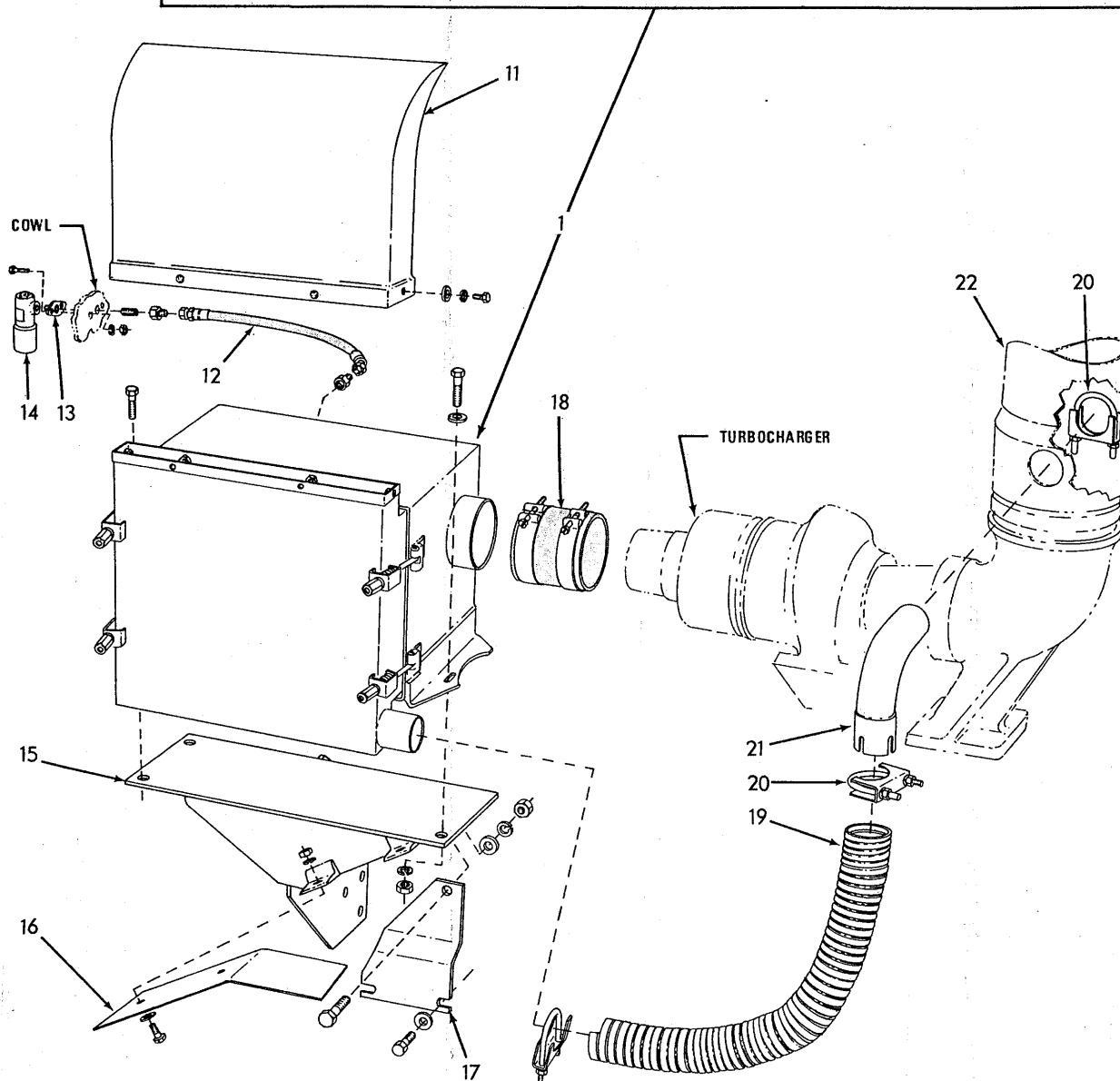
AIR CLEANER ("Farr")(Turbocharged units)
