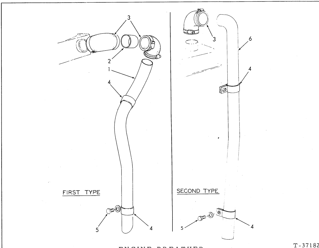
ENGINE BREATHER
