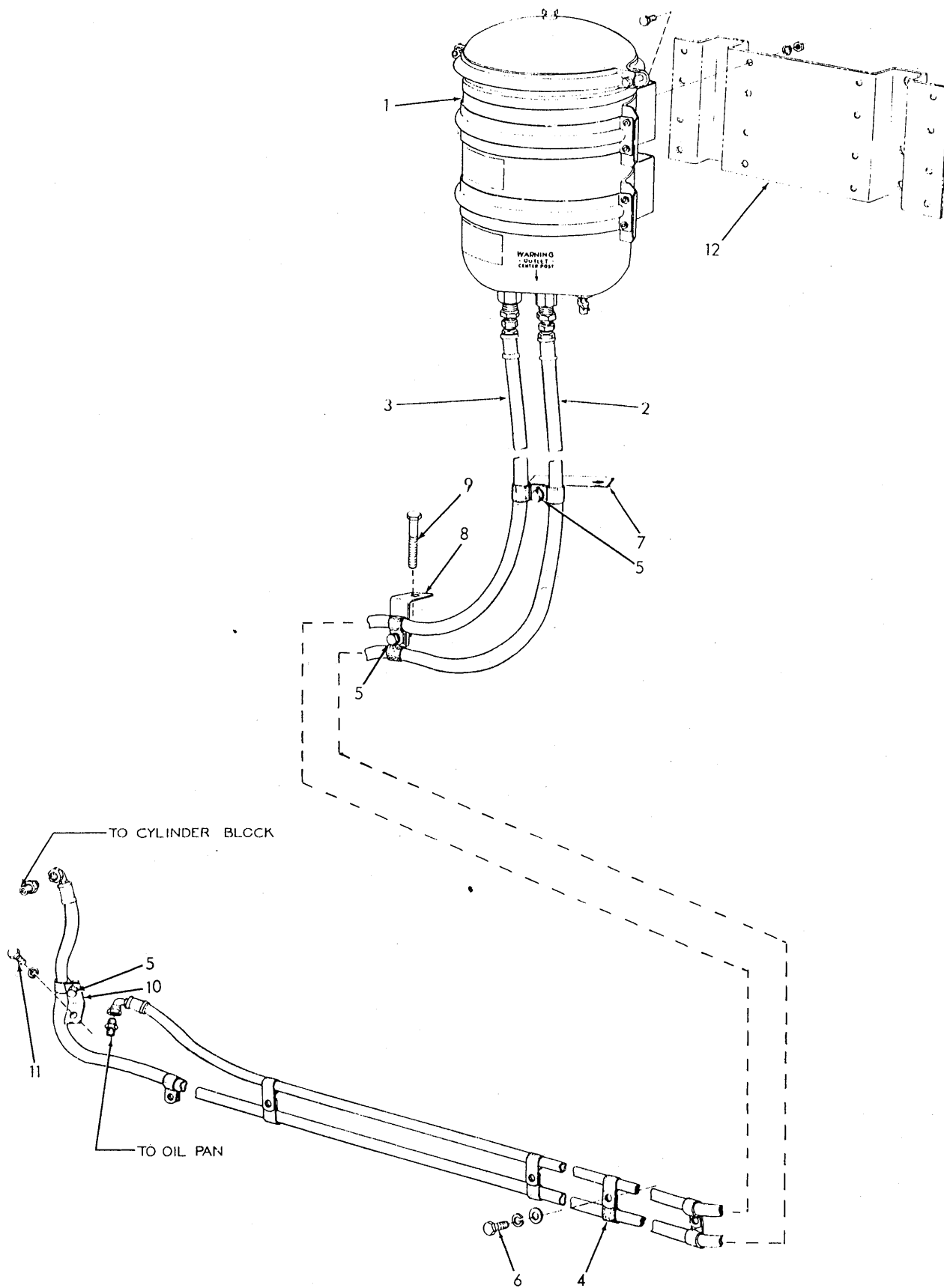
HEAVY-DUTY OIL FILTER
