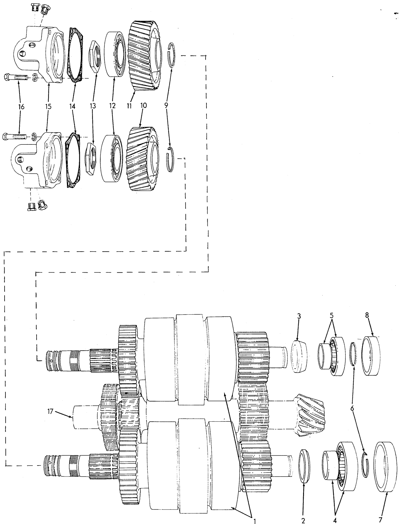
TRANSMISSION CLUTCH SHAFTS
