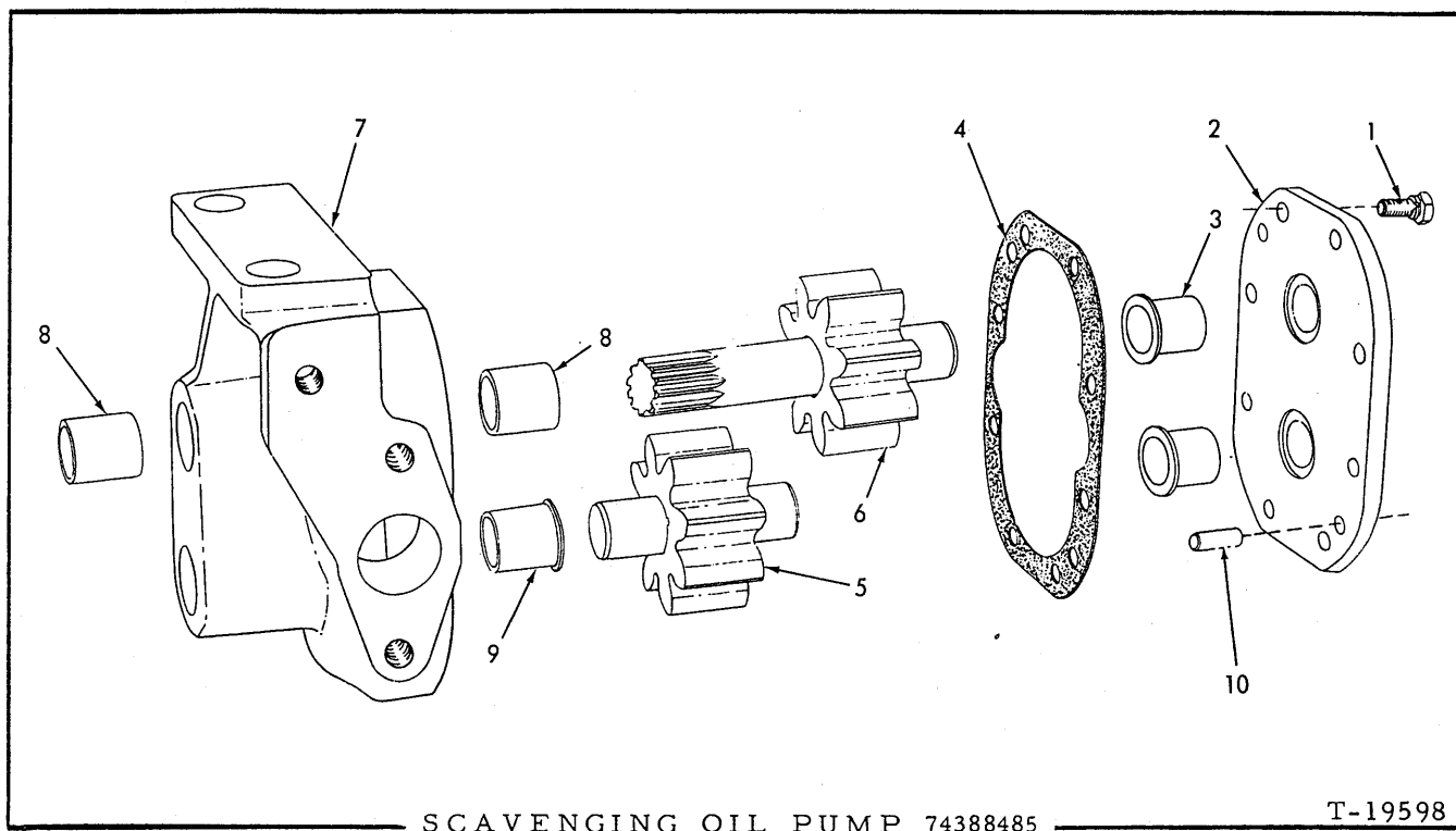
SCAVENGING OIL PUMP 74388485
