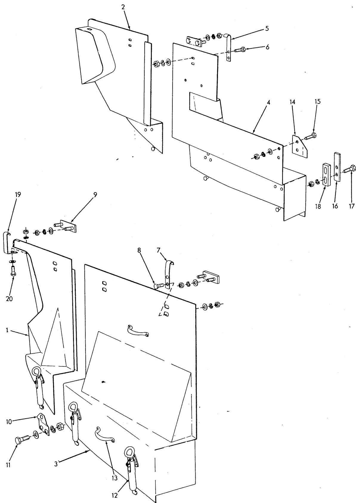
HOOD SIDE PLATES (Tractors with hydraulic radiator guard)
