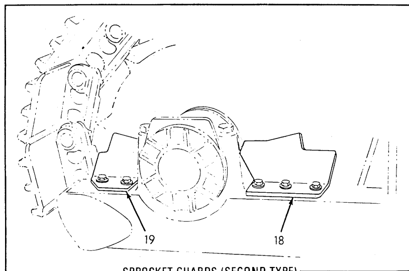
SPROCKET GUARDS (SECOND TYPE)
