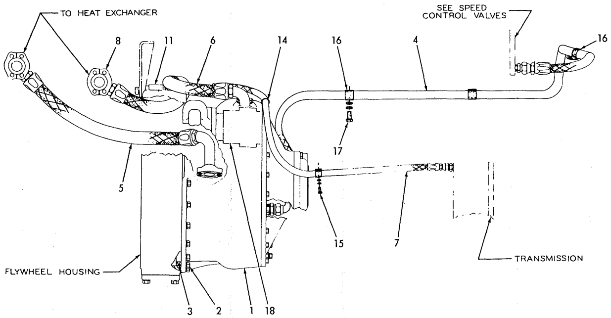
SIDE VIEW
