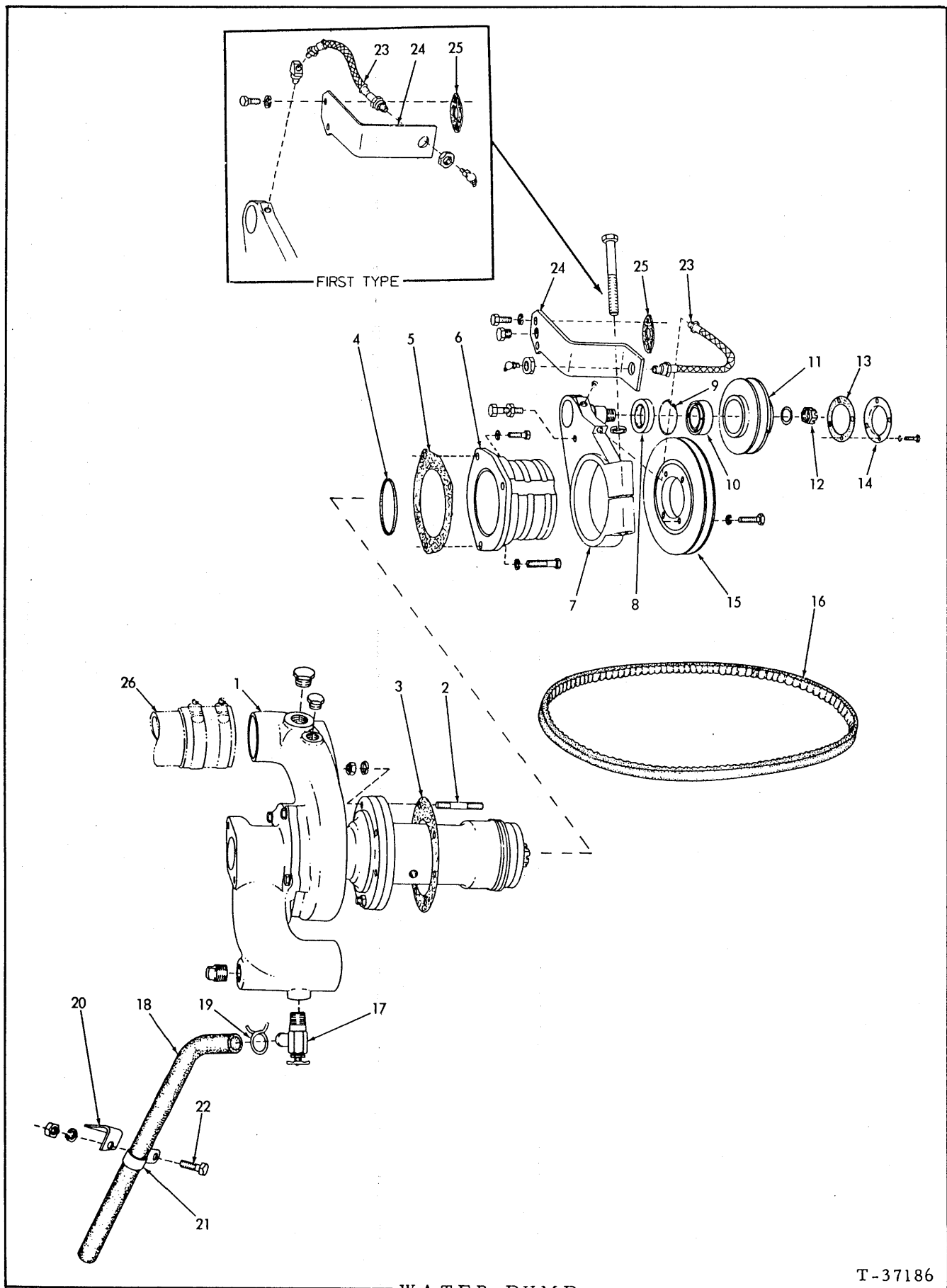
WATER PUMP
