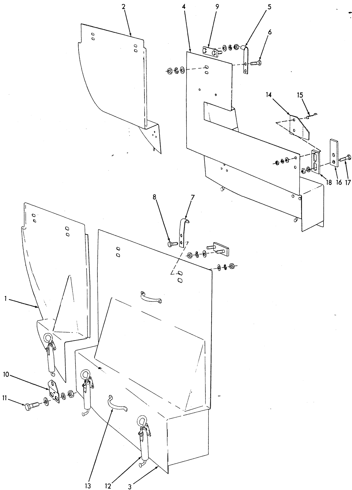
HOOD SIDE PLATES (Tractors with standard or cable radiator guard)
