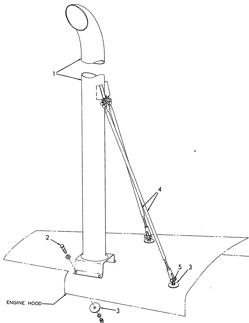
EXHAUST EXTENSION
