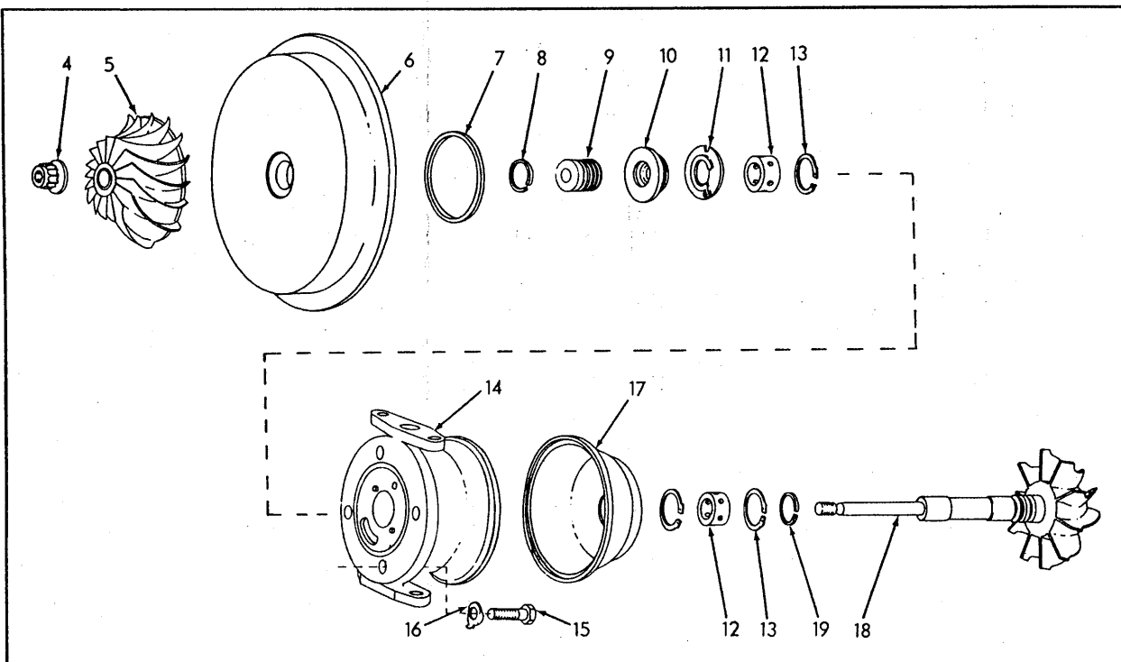
TURBOCHARGER ASSEMBLY
