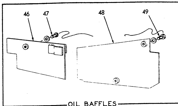
OIL BAFFLES
