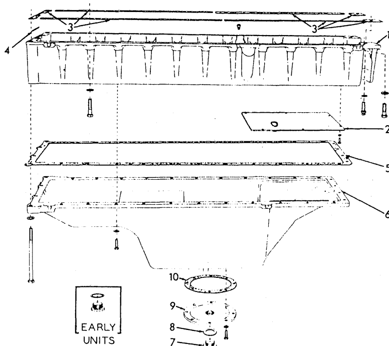
OIL PAN
