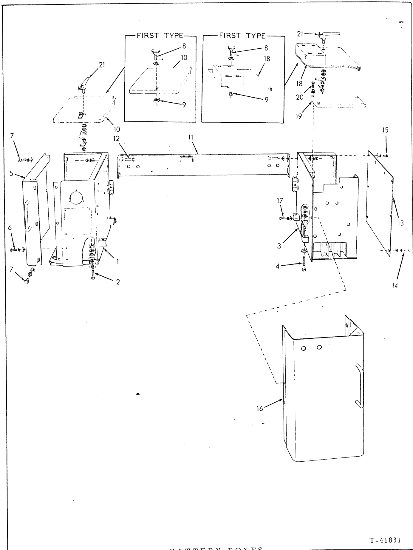
BATTERY BOXES
