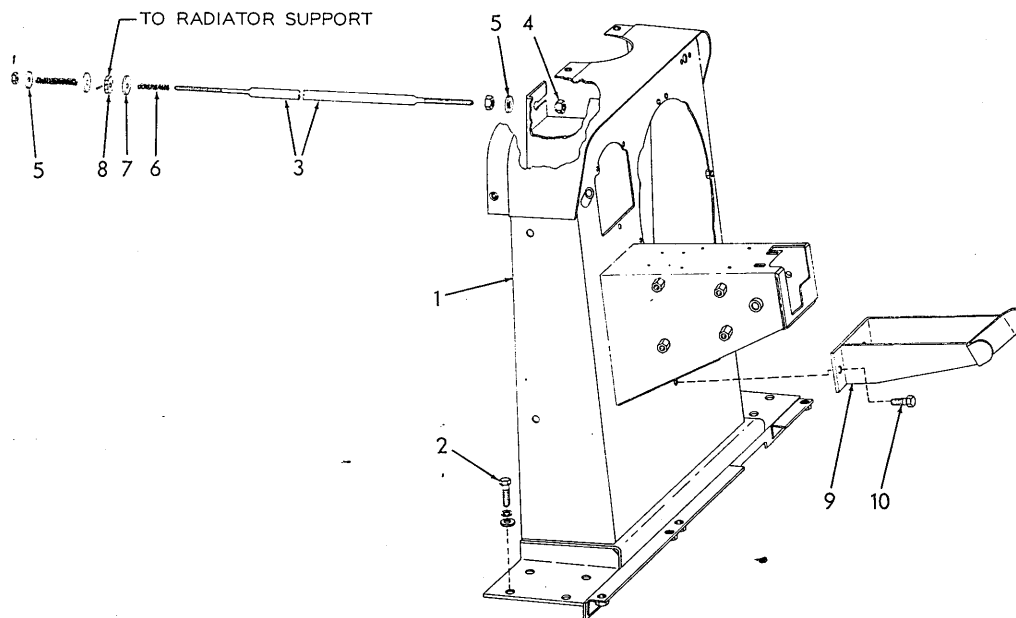
COWL
