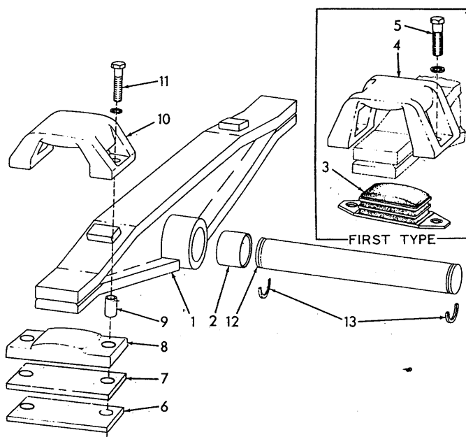
EQUALIZING BEAM
