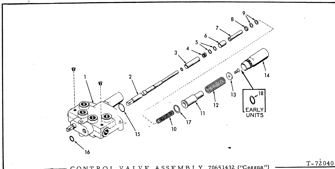
CONTROL VALVE ASSEMBLY 70651432 ("Cessna")
