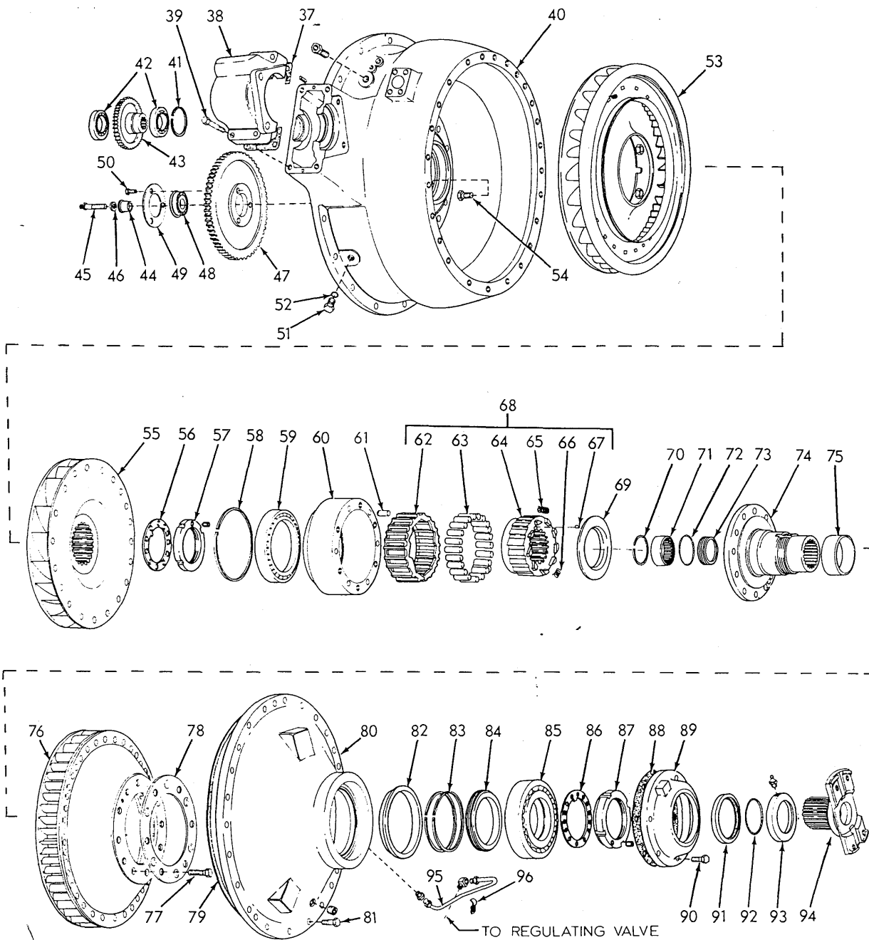
TORQUE CONVERTER PARTS (Rear section)
