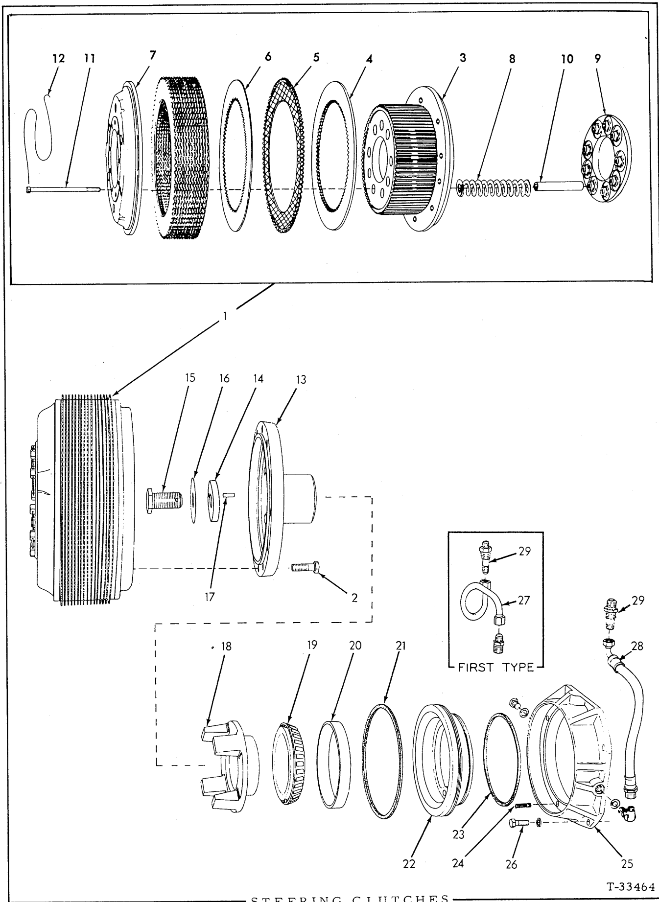
STEERING CLUTCHES
