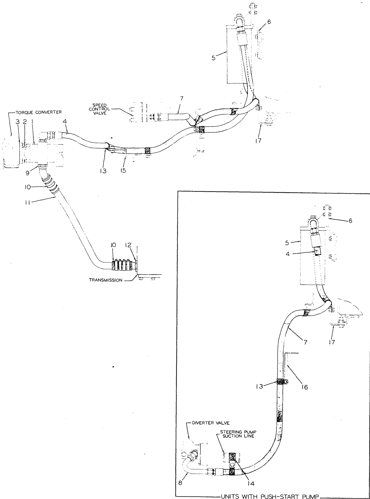
TRANSMISSION OIL PUMP AND FILTER (Third type)
