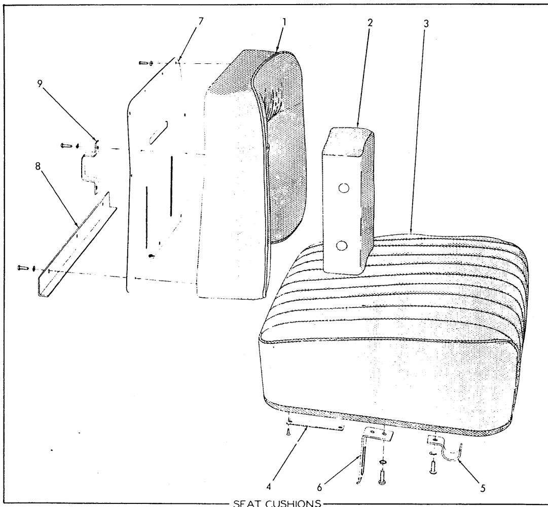
SEAT CUSHIONS
