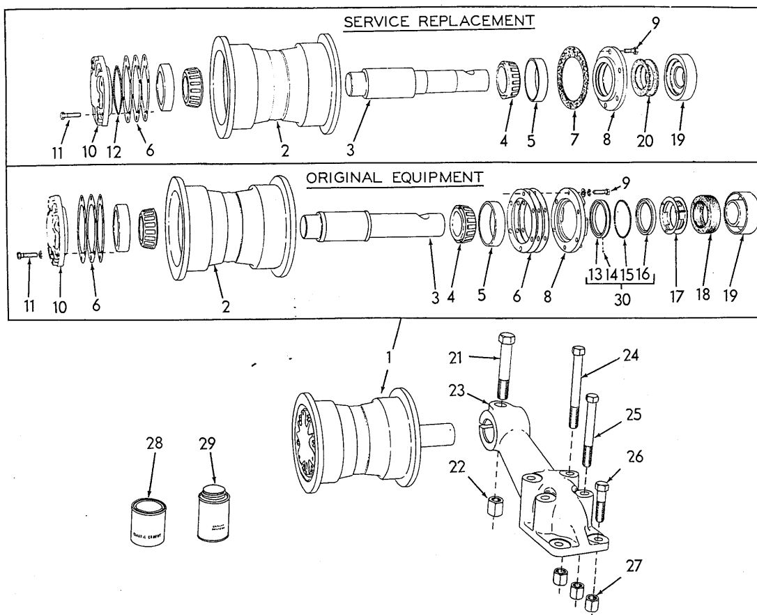
TRACK CARRIER ROLLER
