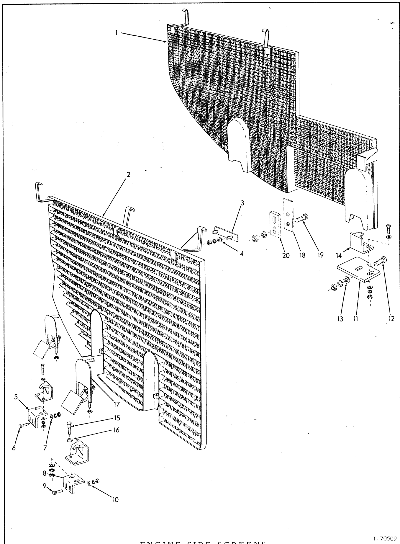
ENGINE SIDE SCREENS
