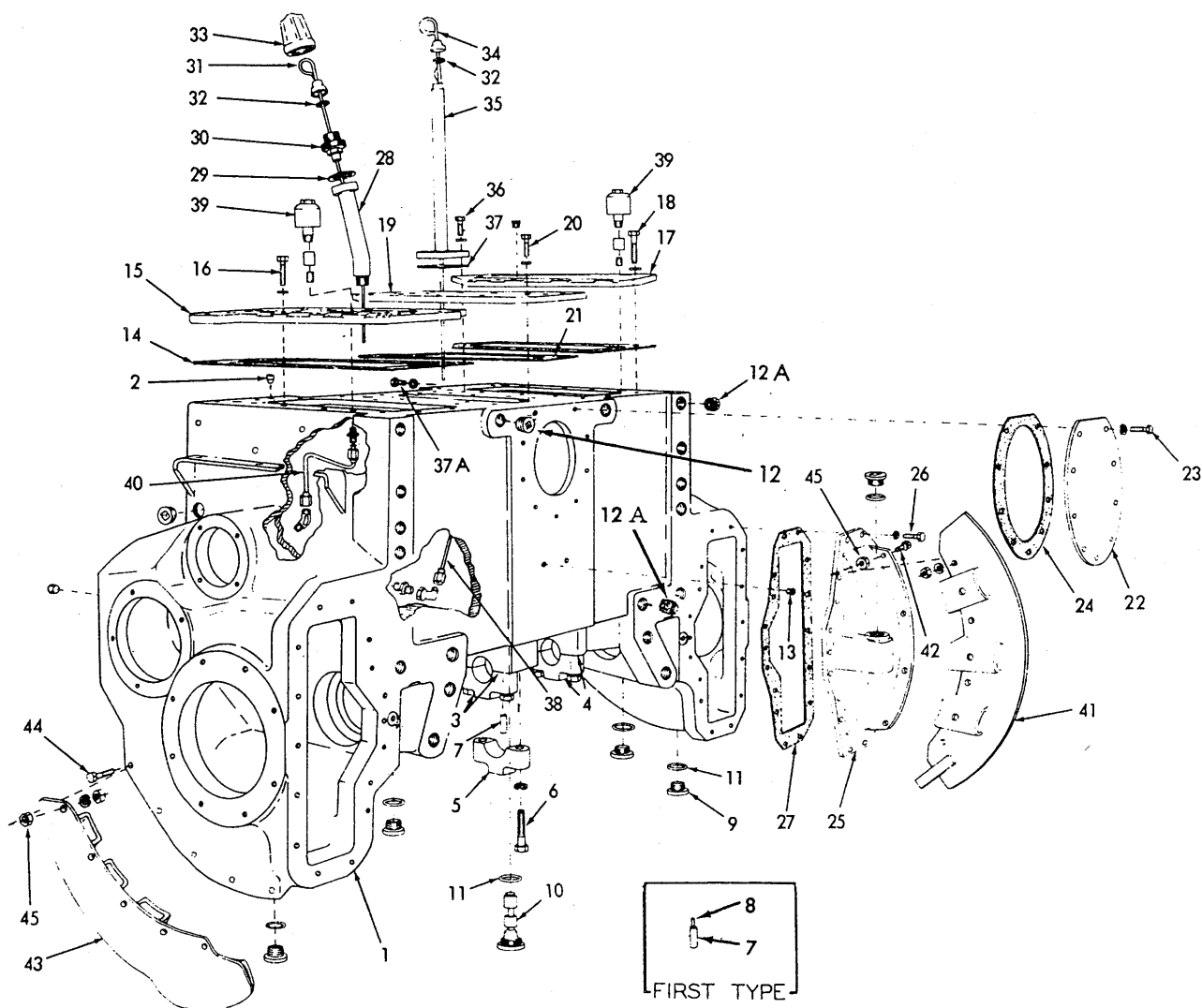
OIL BAFFLES
