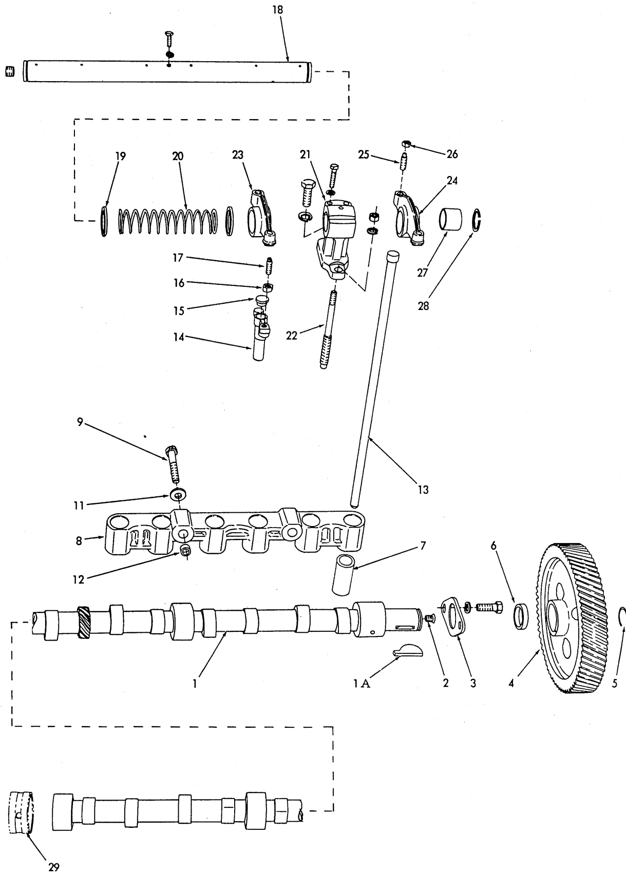
VALVE OPERATING MECHANISM
