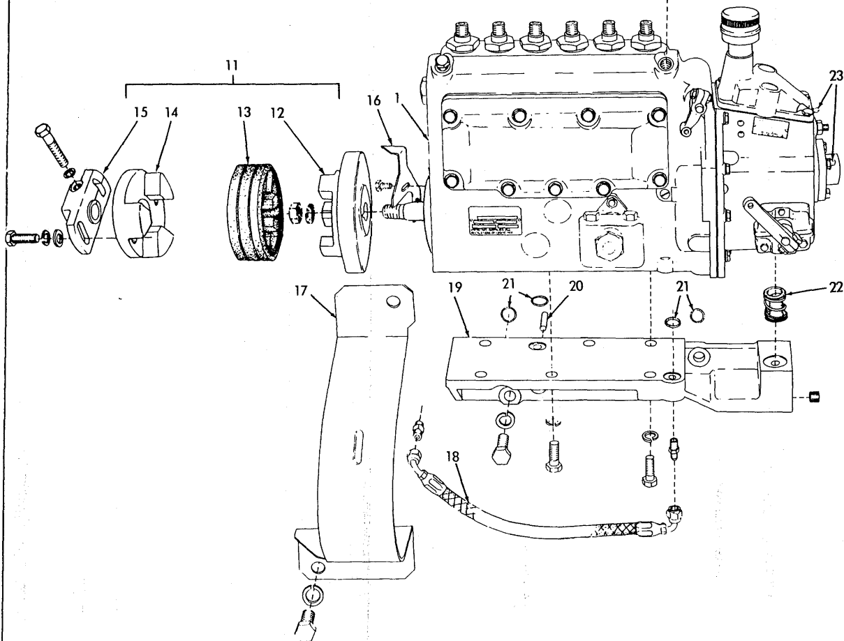
FUEL INJECTION PUMP
