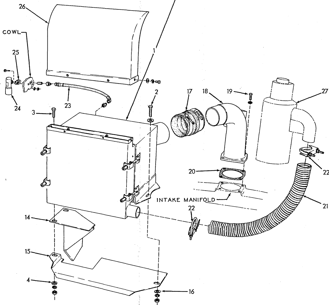
AIR CLEANER (Second type)(Units without turbocharger)
