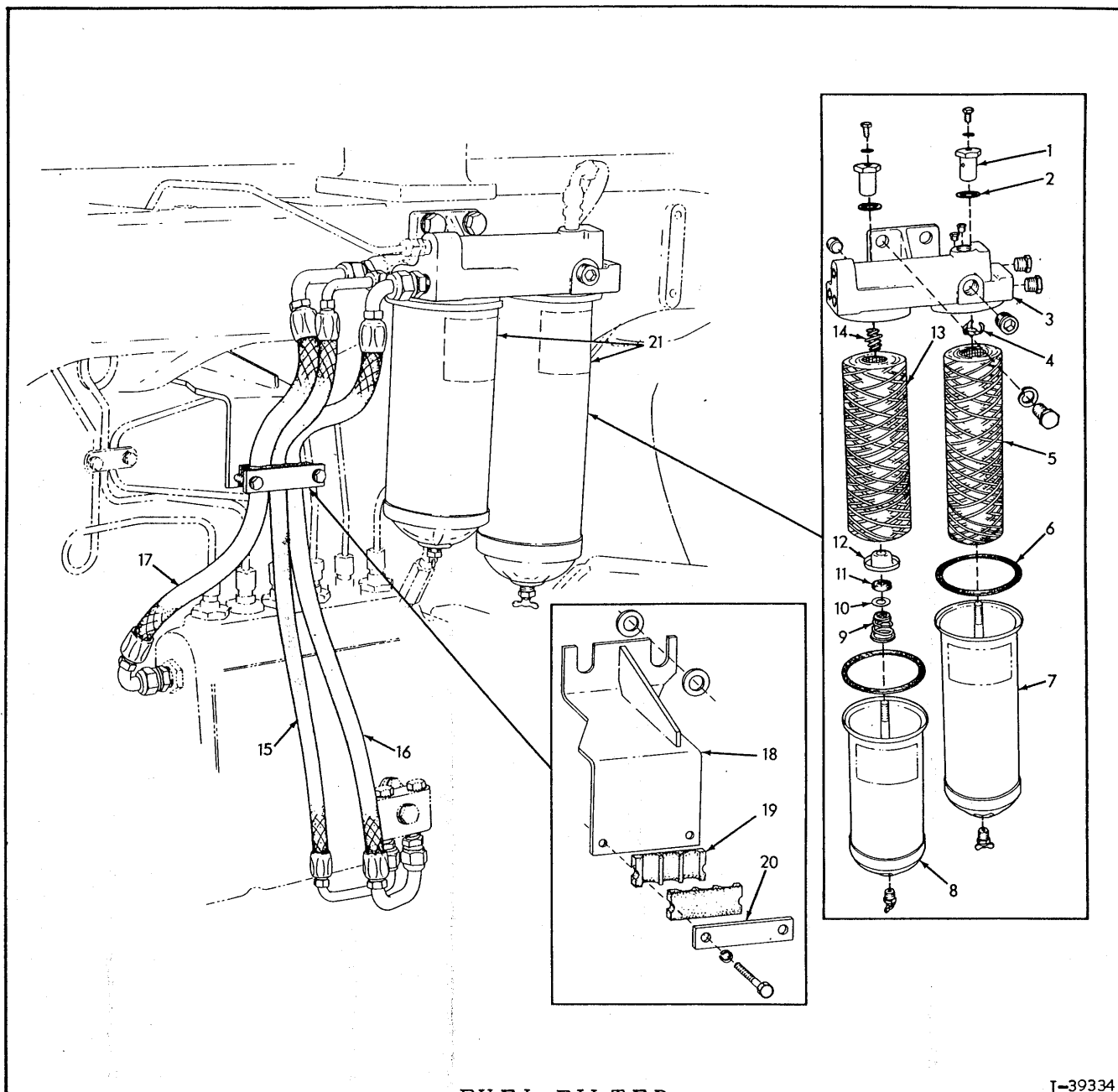
FUEL FILTER
