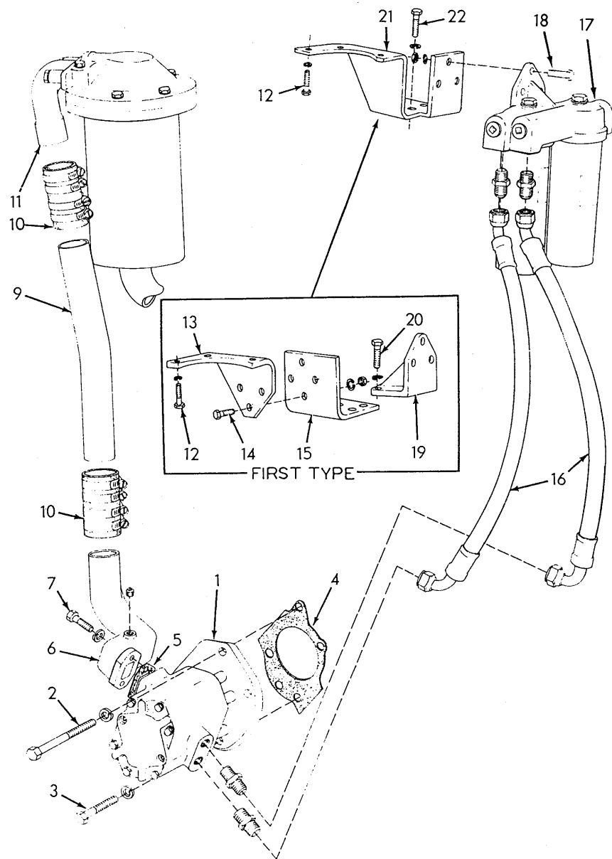
STEERING PUMP AND FILTERS (First type)
