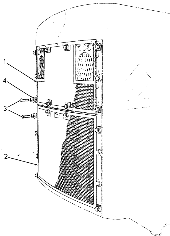
GRILLE SCREEN (For Standard Guard)
