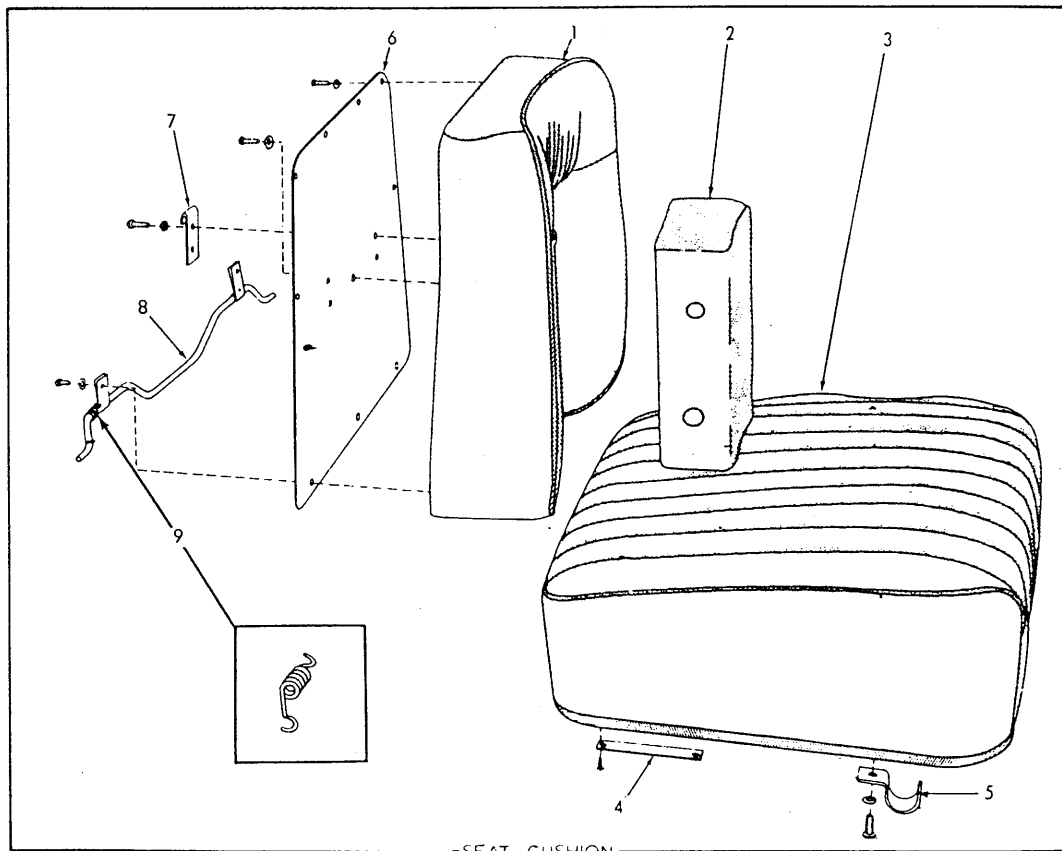
SEAT CUSHION SEAT ASSEMBLY 70659093
