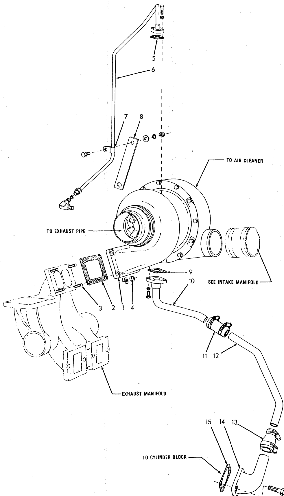
TURBOCHARGER CONNECTIONS
