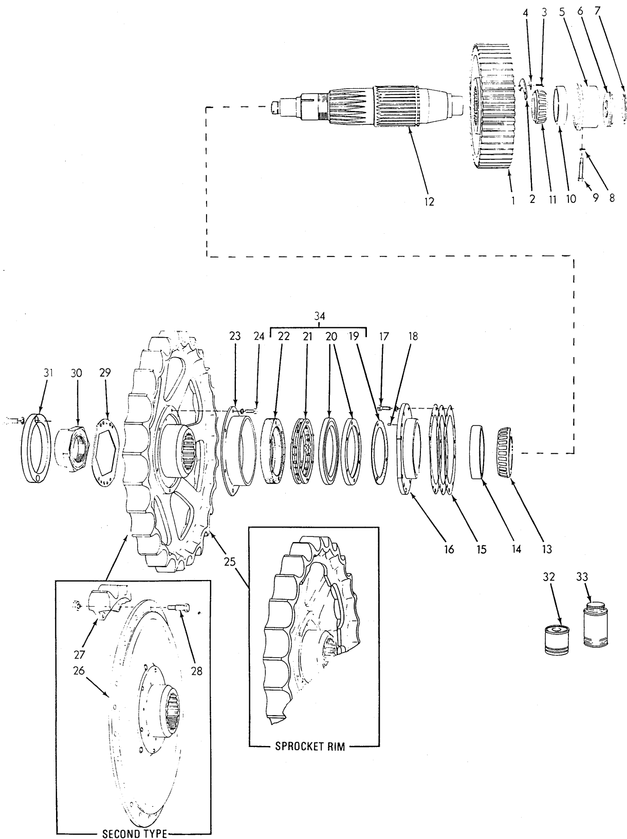
FINAL DRIVE SPROCKET, SHAFT AND GEAR
