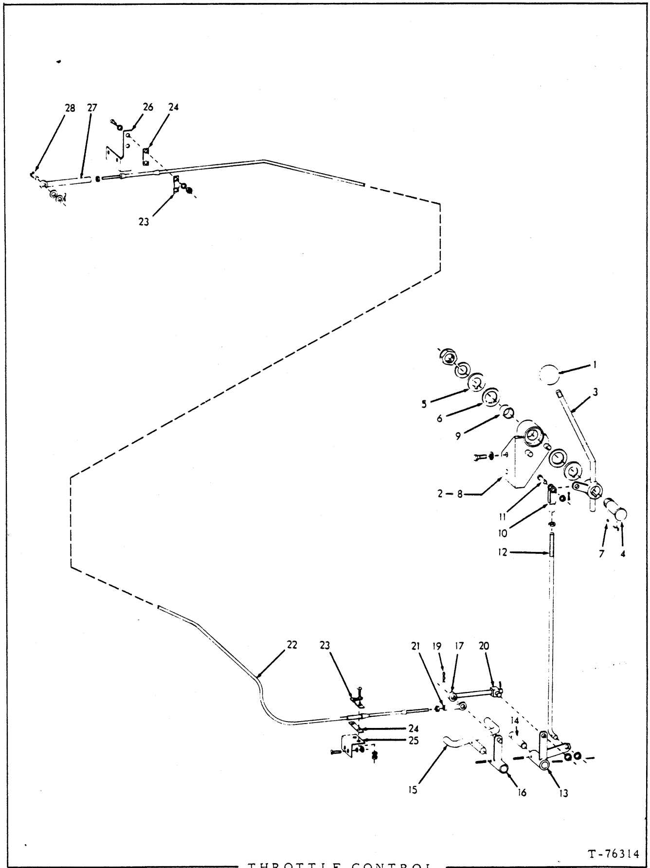
THROTTLE CONTROL
