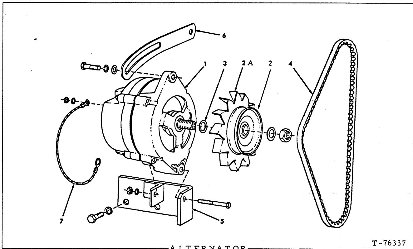
ALTERNATOR
