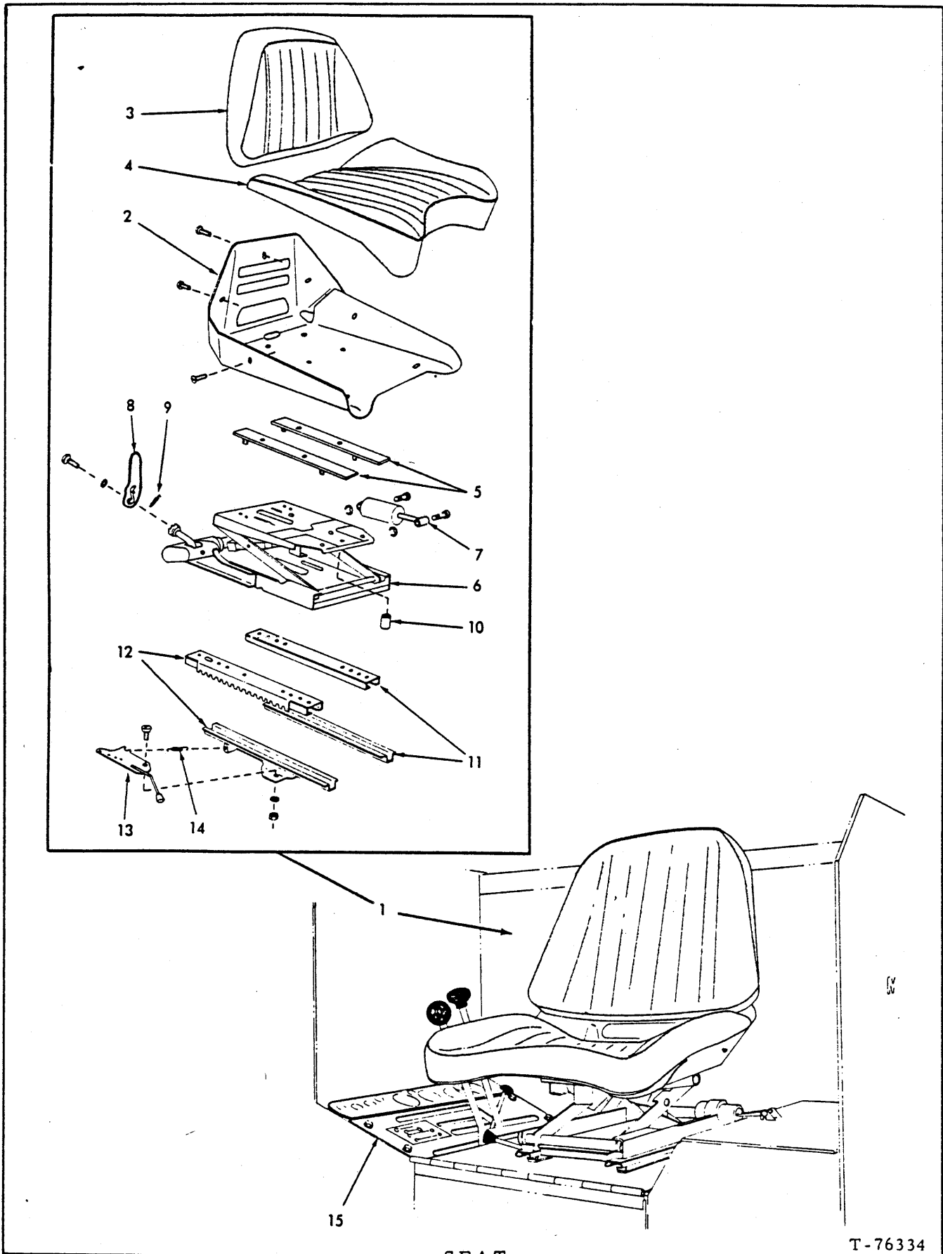
SEAT
