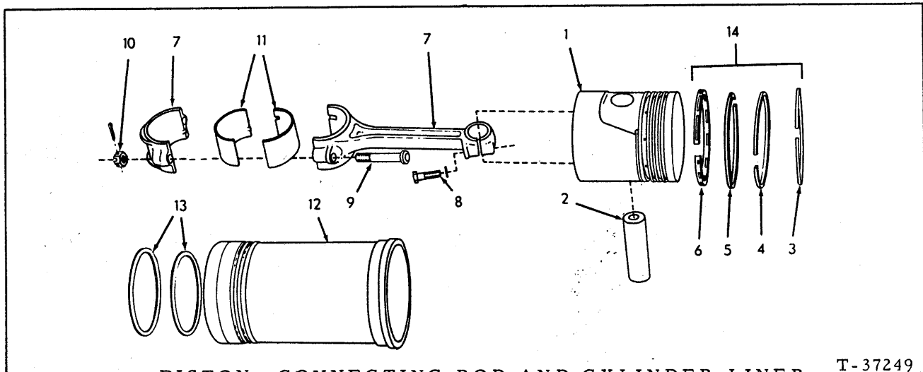
PISTON, CONNECTING ROD AND CYLINDER LINER T-37249
