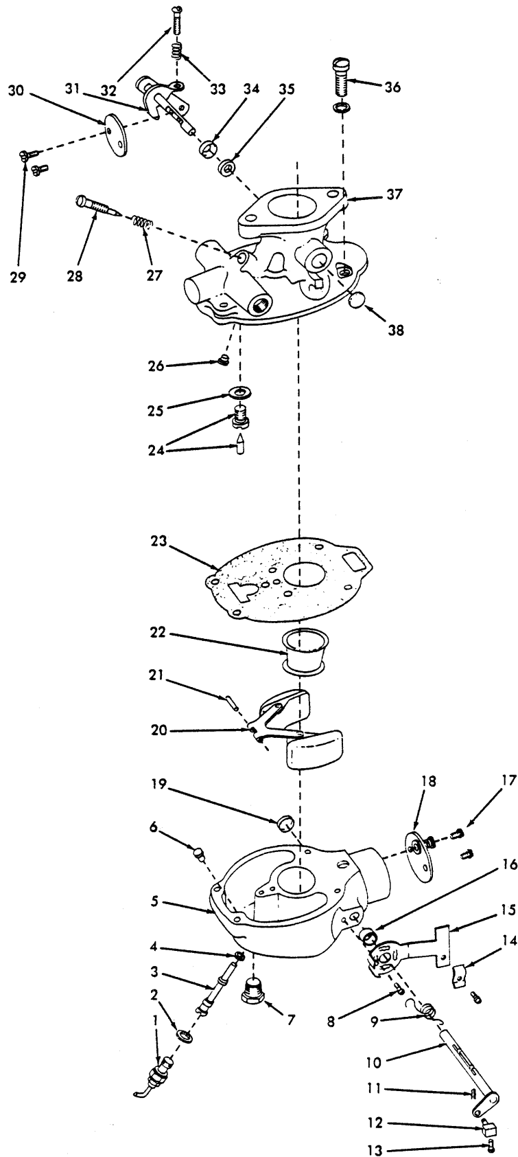
CARBURETOR ASSEMBLY 70239961
