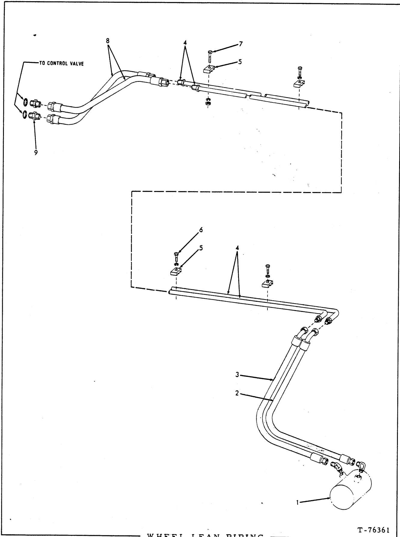
WHEEL LEAN PIPING
