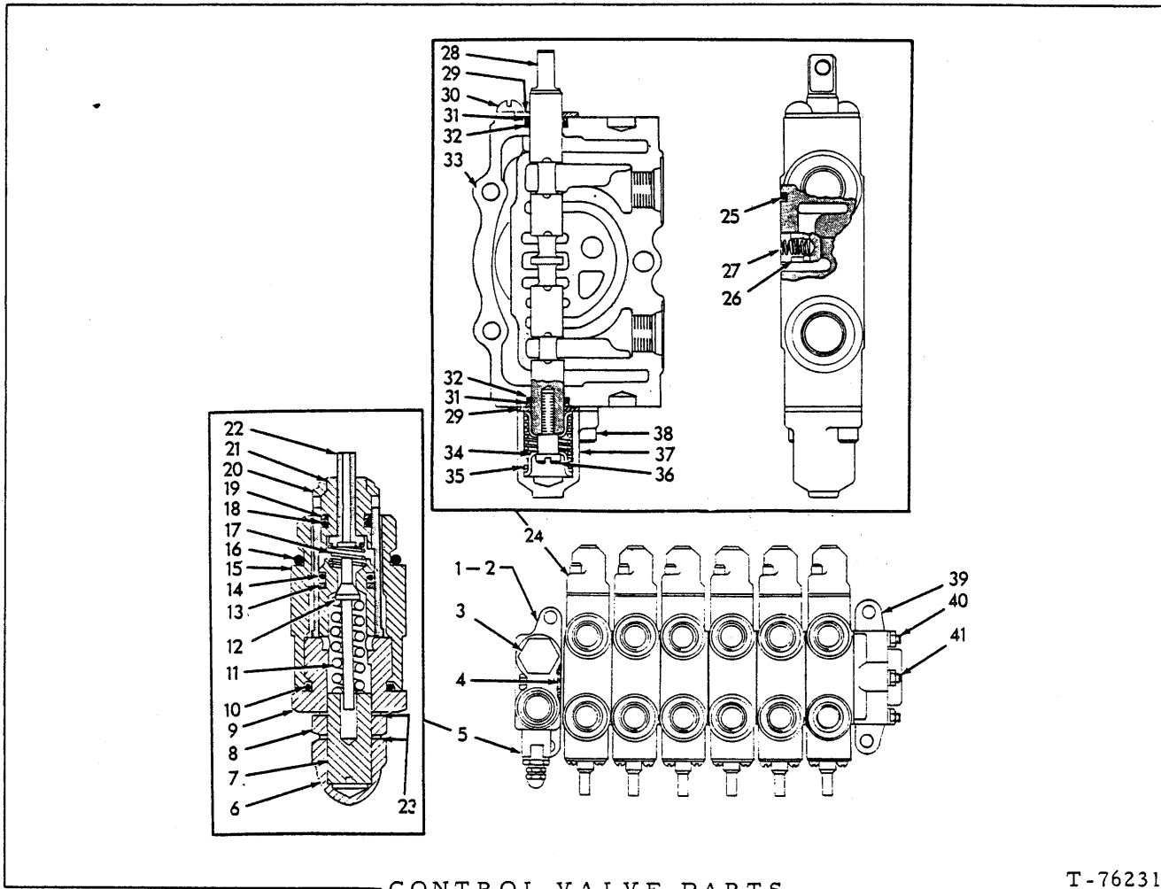
CONTROL VALVE PARTS
