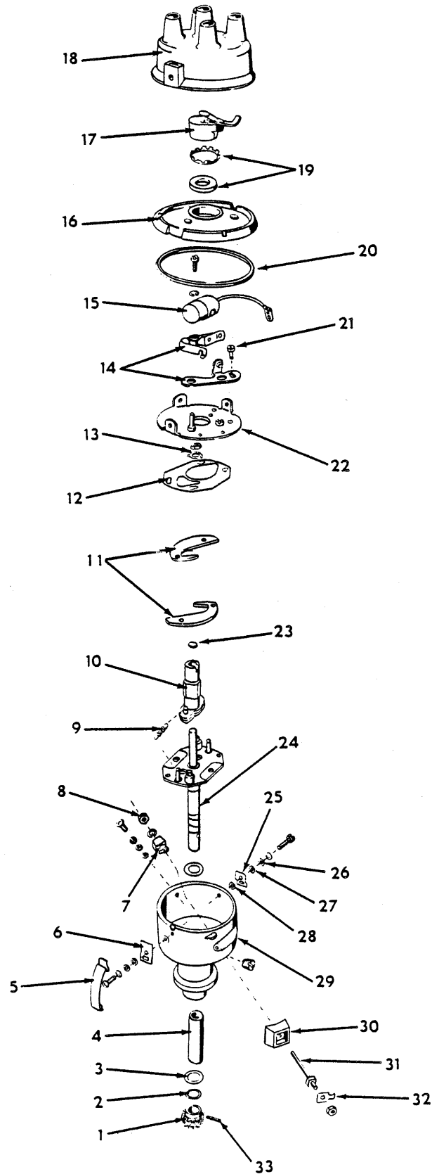
DISTRIBUTOR
