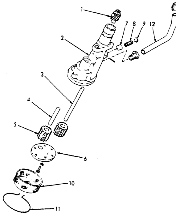
OIL PUMP
