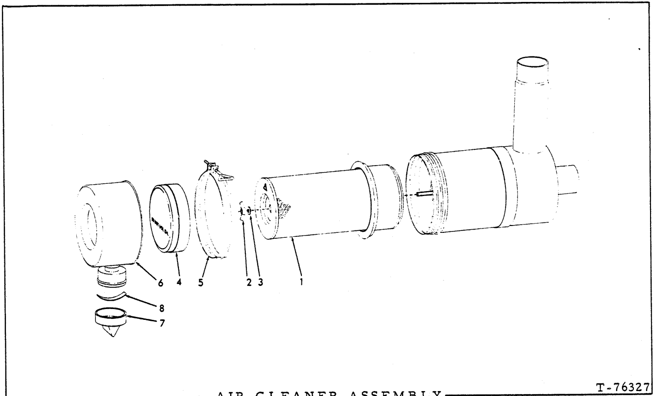
AIR CLEANER ASSEMBLY (Dry-type)
