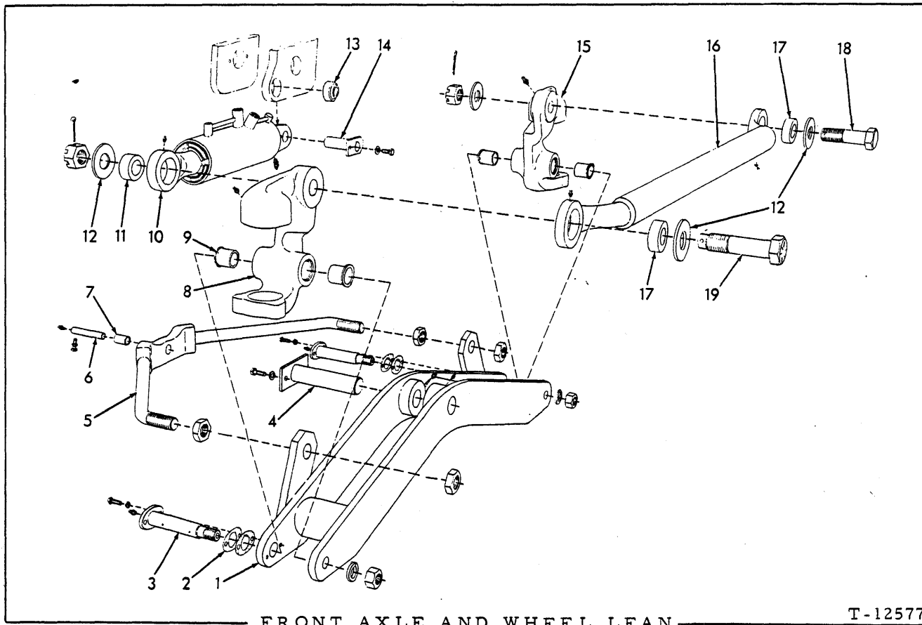
FRONT AXLE AND WHEEL LEAN
