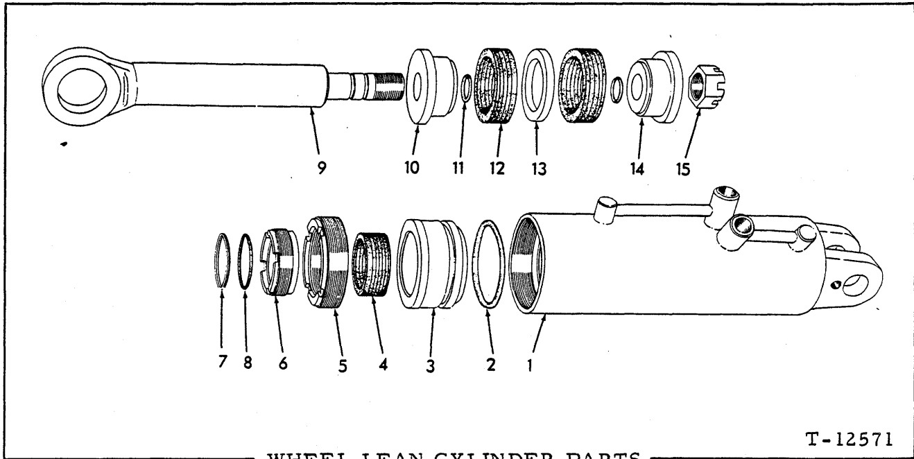
WHEEL LEAN CYLINDER PARTS
