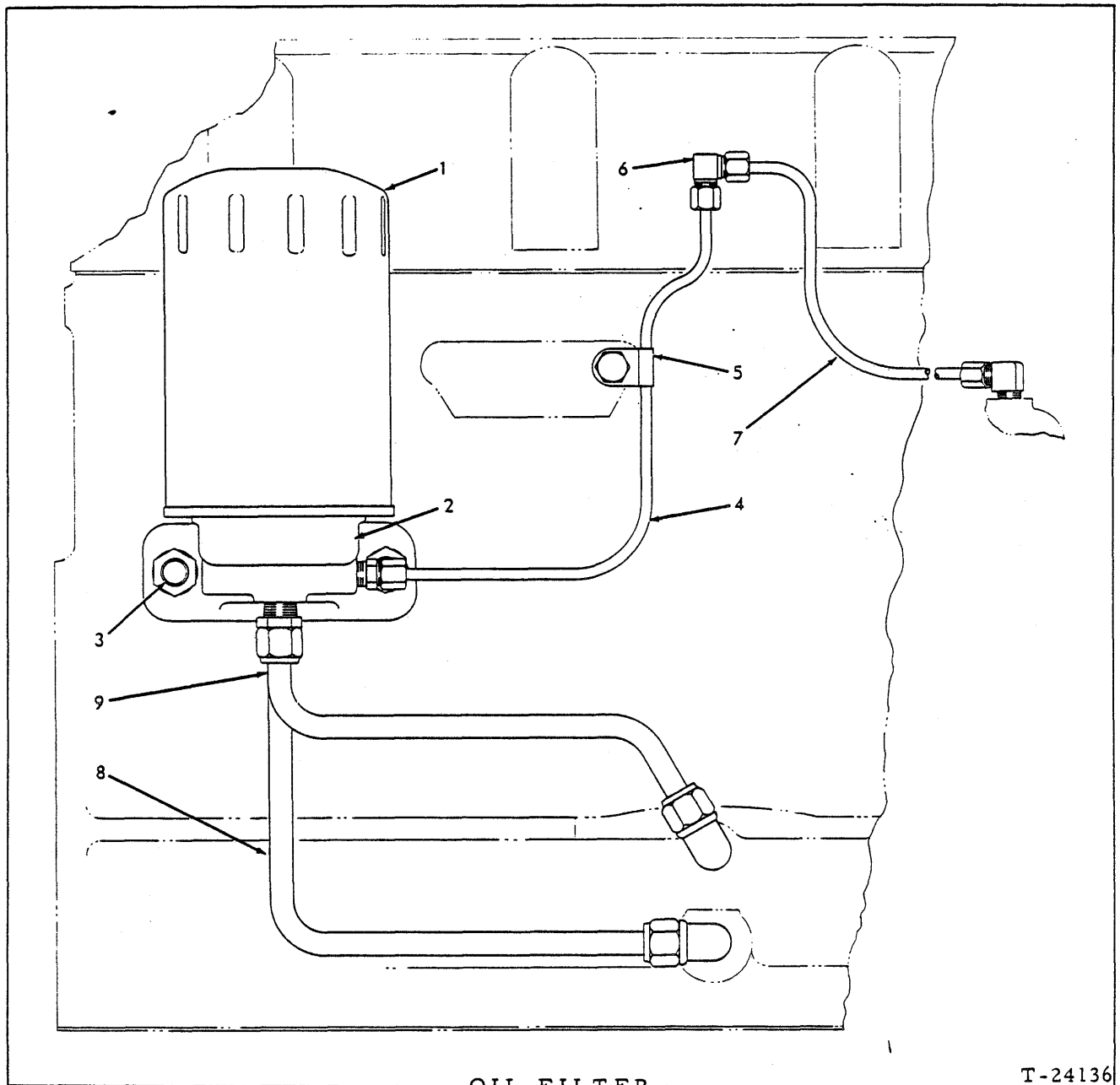
OIL FILTER
