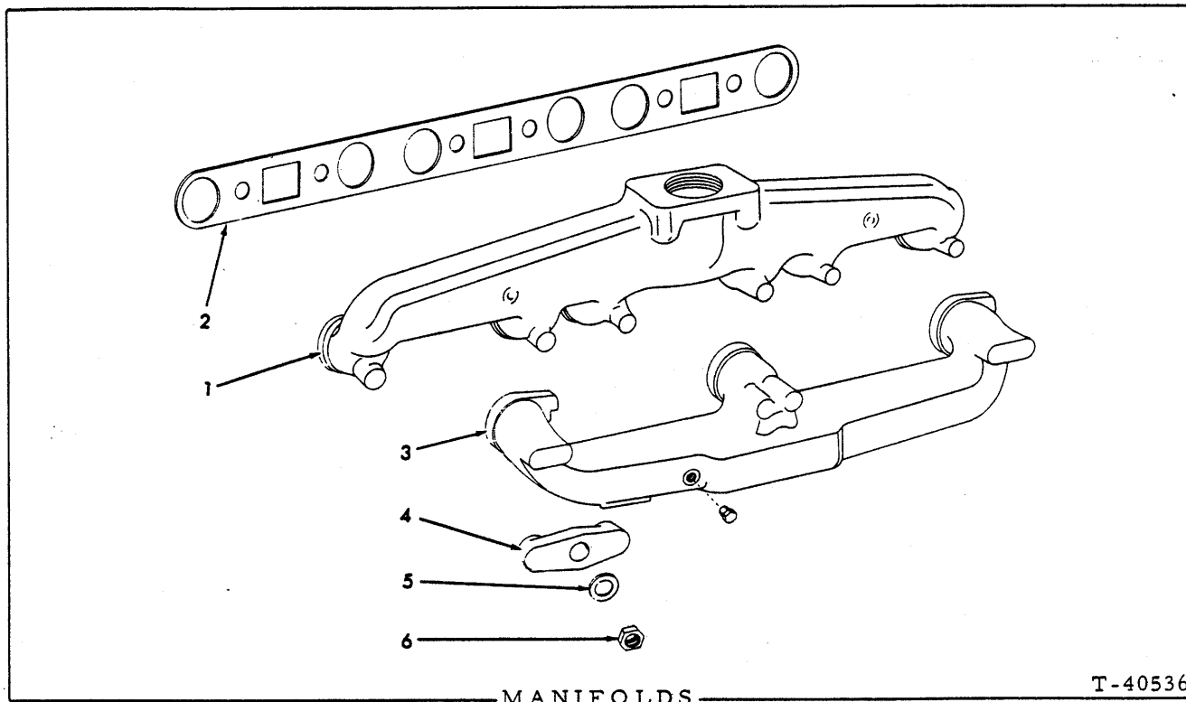
MANIFOLDS
