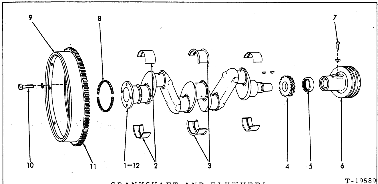
CRANKSHAFT AND FLYWHEEL
