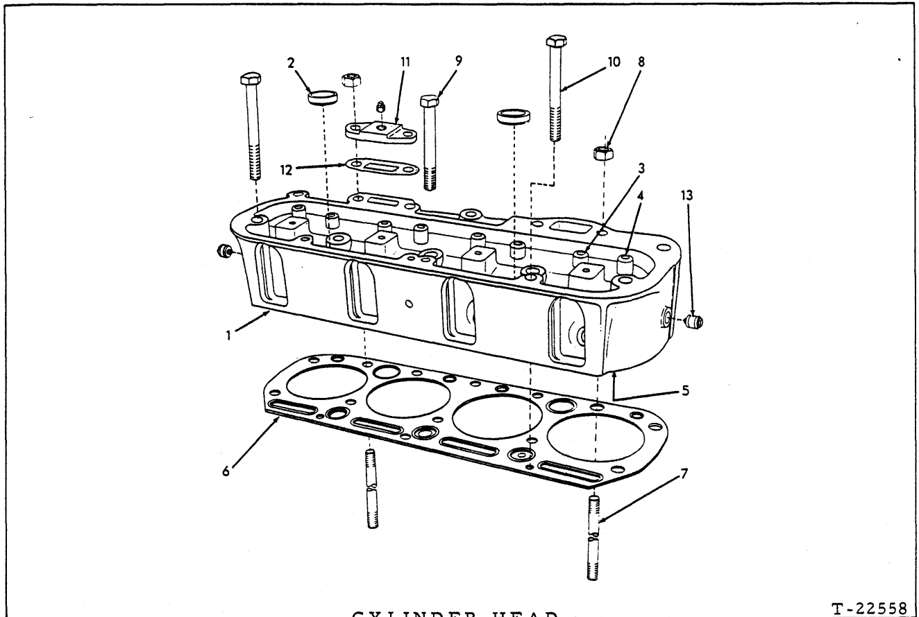
CYLINDER HEAD
