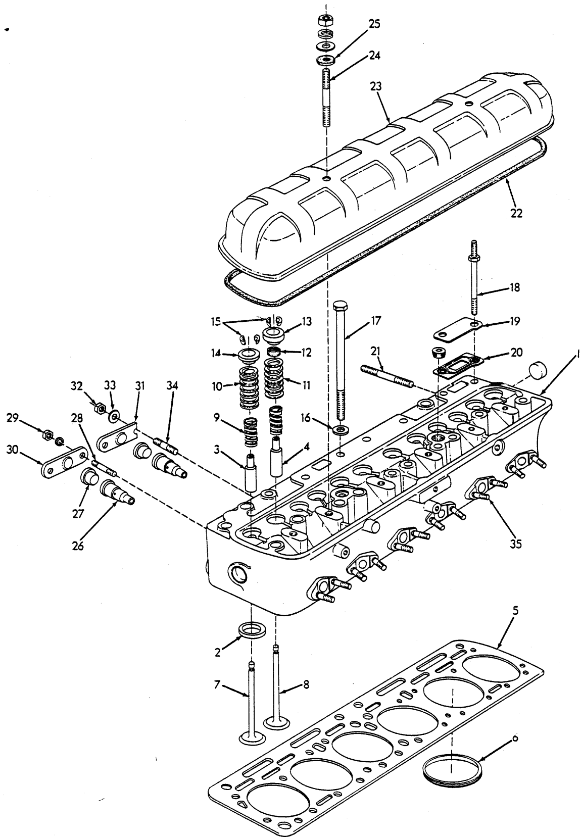
CYLINDER HEAD AND VALVES
