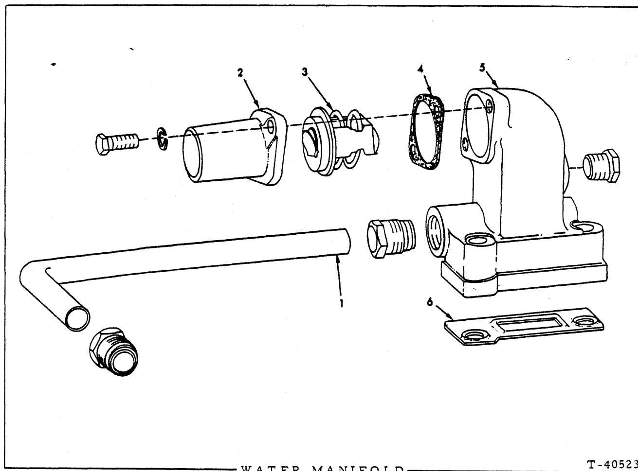
WATER MANIFOLD
