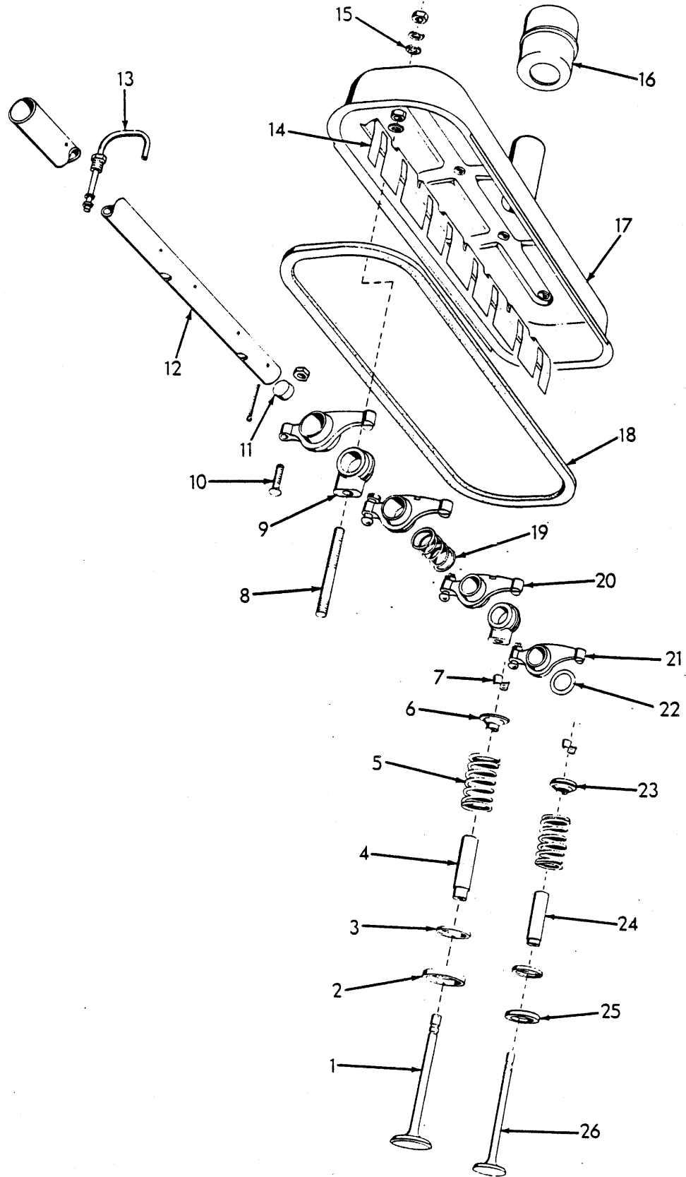
VALVES AND ROCKER ARMS
