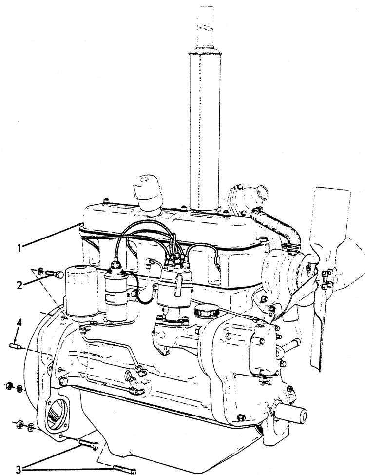
ENGINE ASSEMBLY (Model 17)
