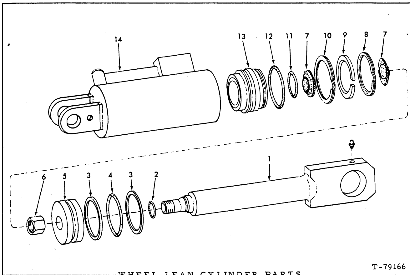
WHEEL LEAN CYLINDER PARTS
