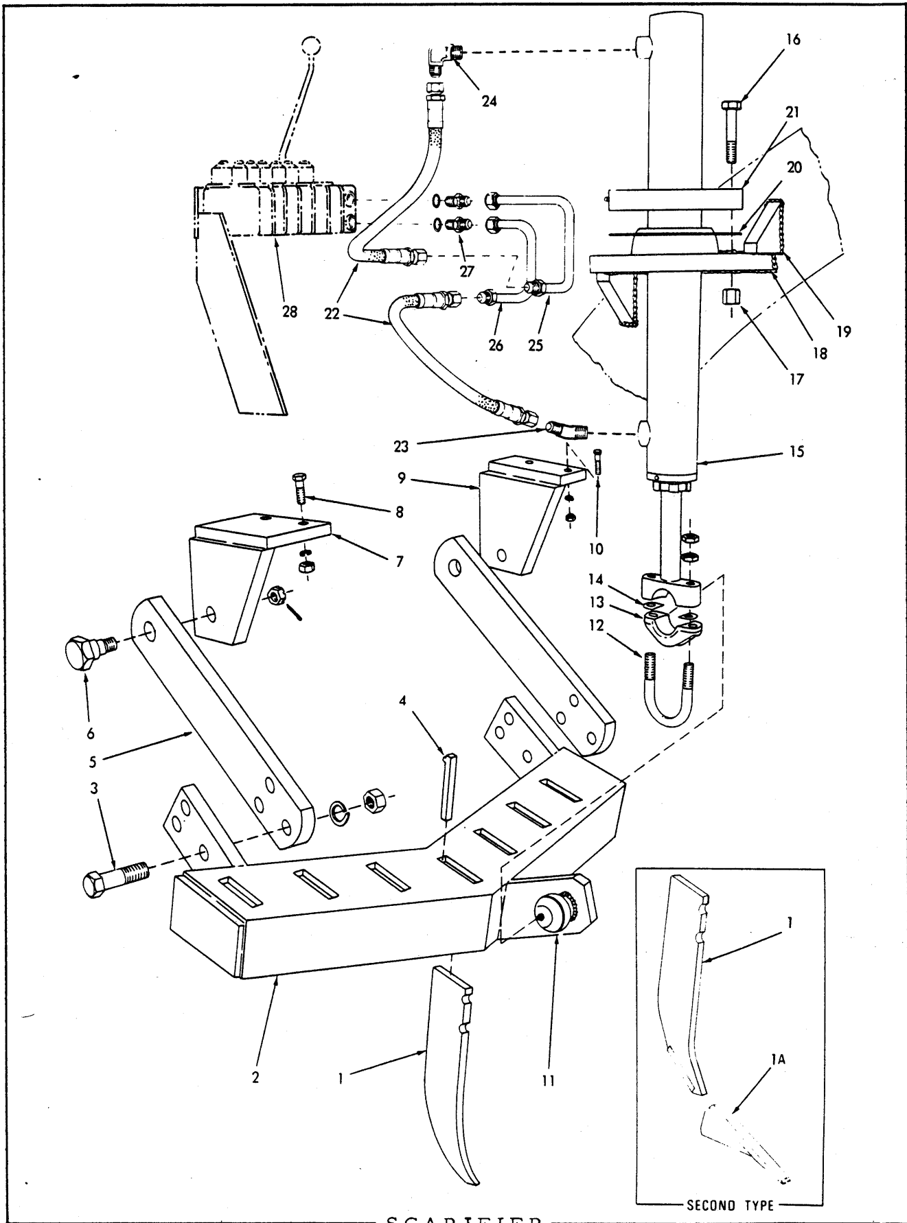
SCARIFIER
