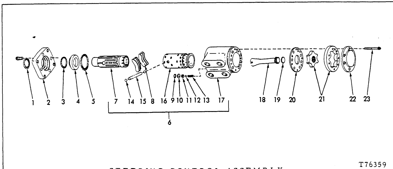
STEERING CONTROL ASSEMBLY
