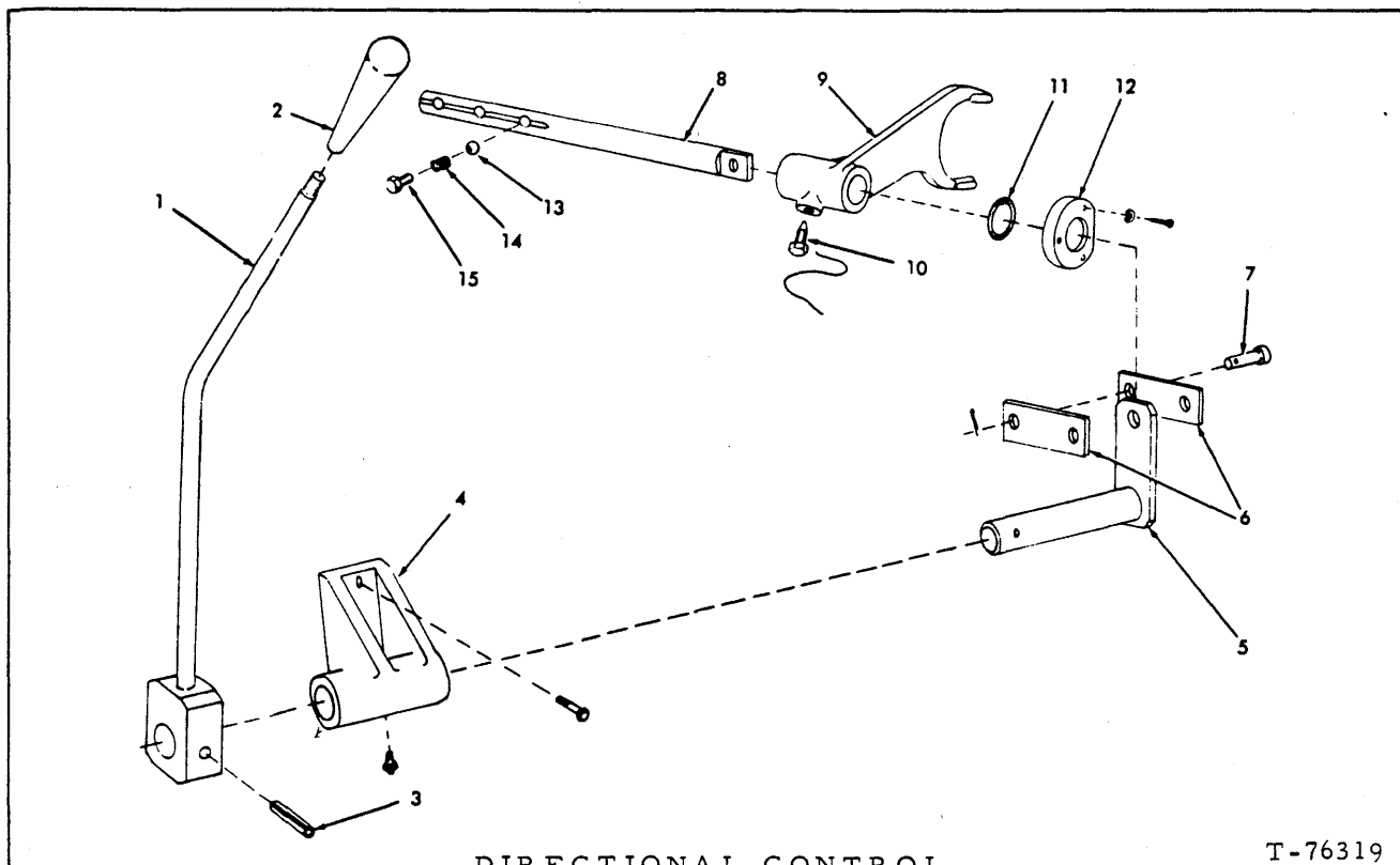
DIRECTIONAL CONTROL
