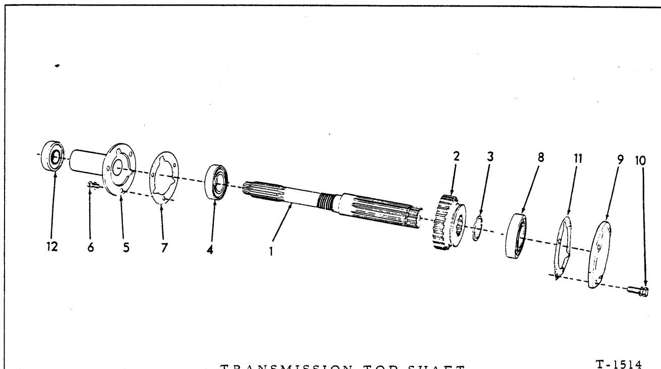
TRANSMISSION TOP SHAFT
