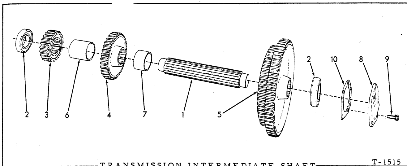
TRANSMISSION INTERMEDIATE SHAFT
