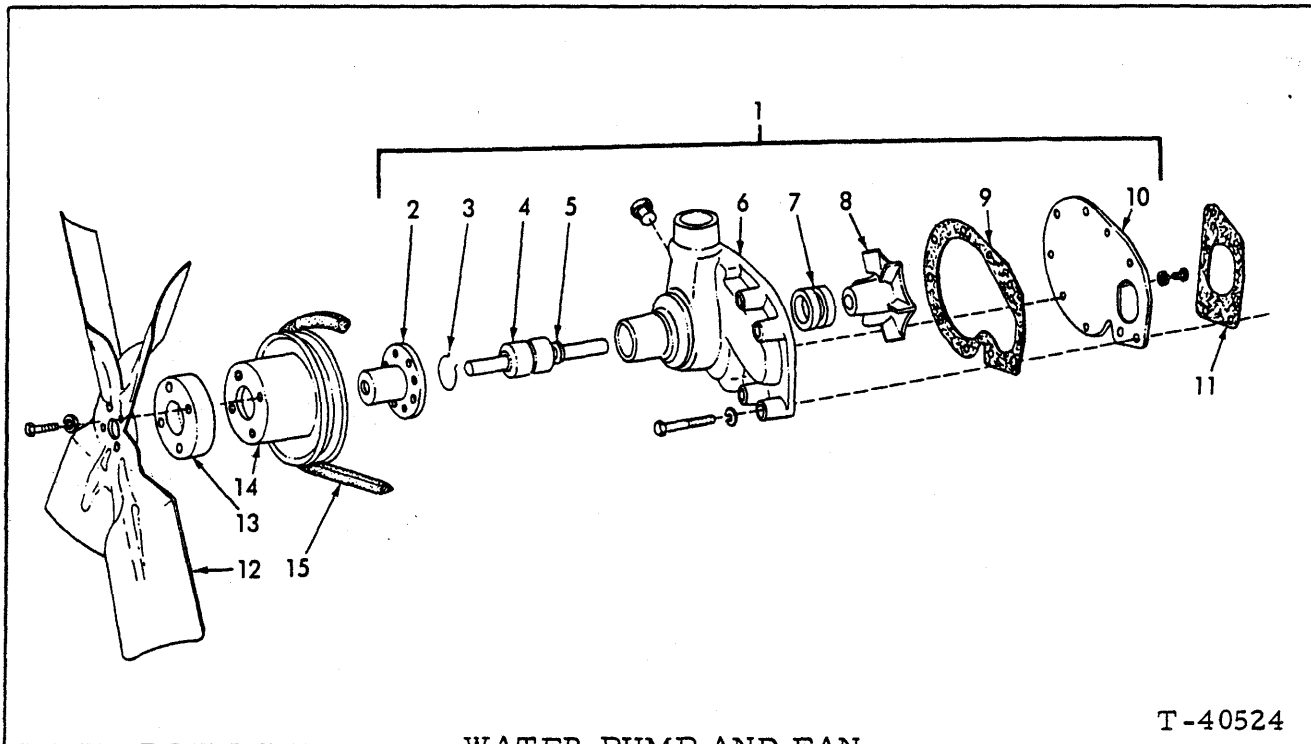
WATER PUMP AND FAN
