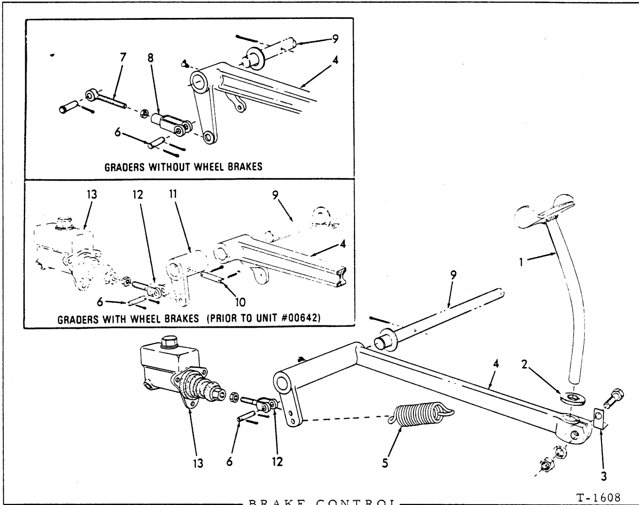
BRAKE CONTROL
