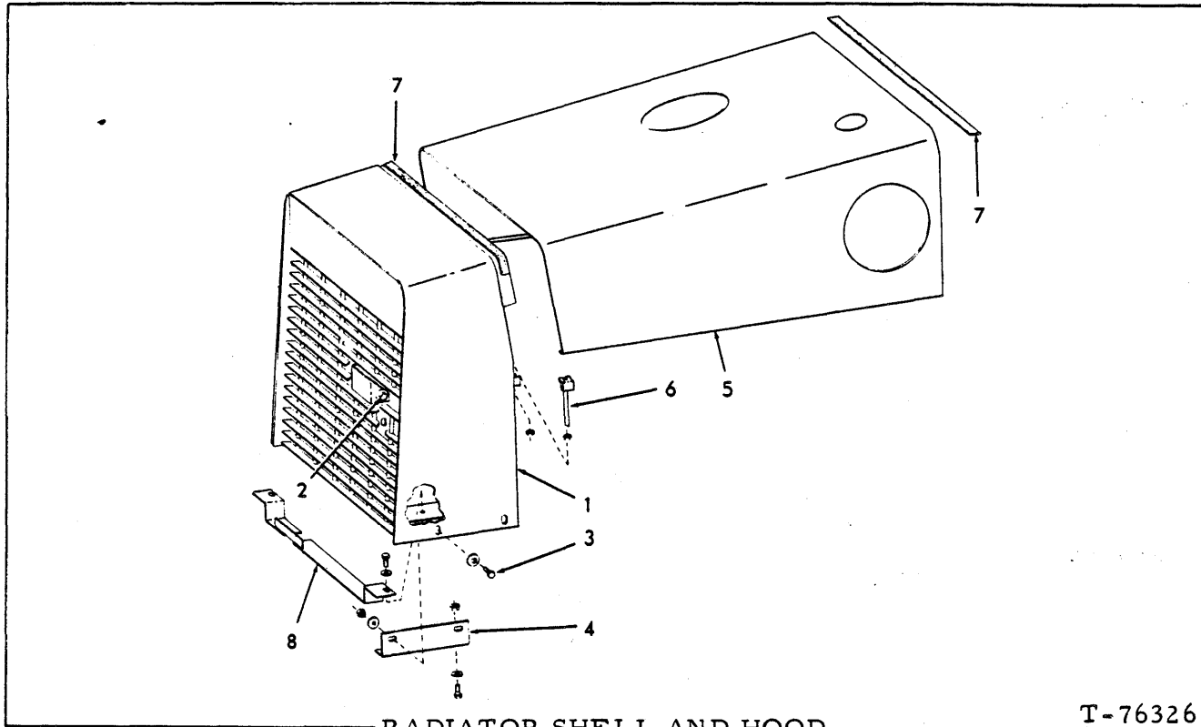
RADIATOR SHELL AND HOOD
