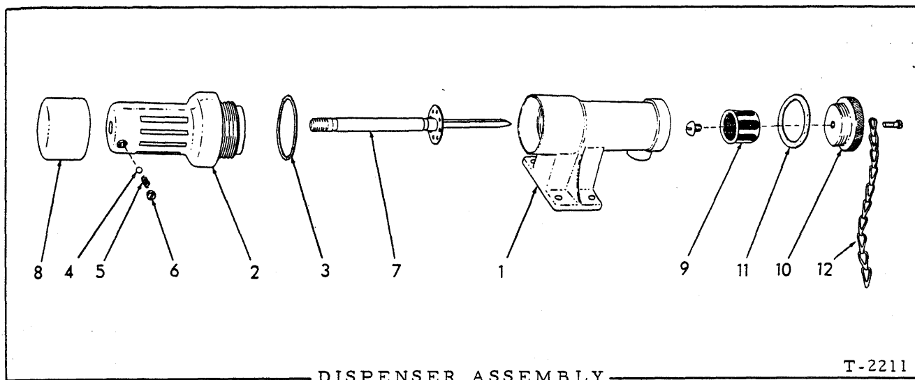
DISPENSER ASSEMBLY
