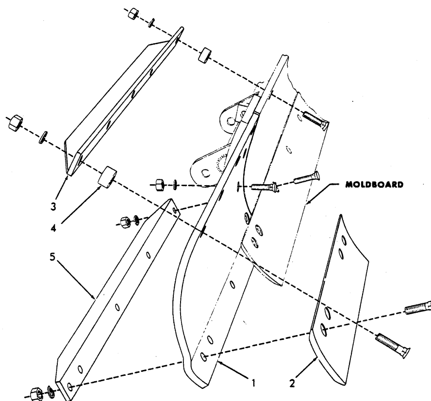
MOLDBOARD EXTENSIONS
