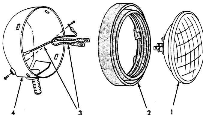
LIGHT ASSEMBLY
