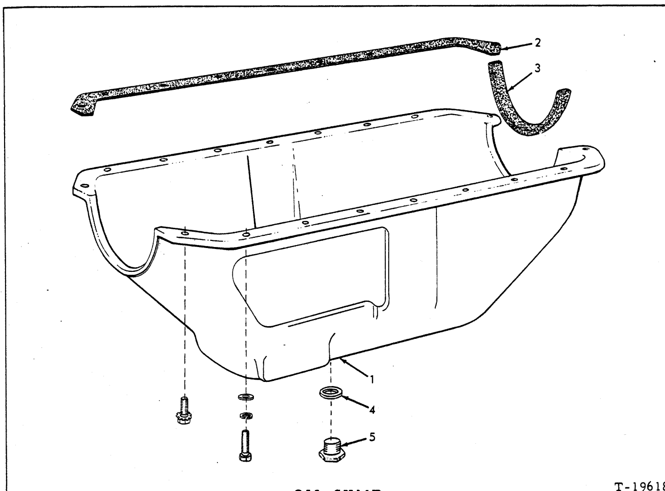
OIL SUMP
