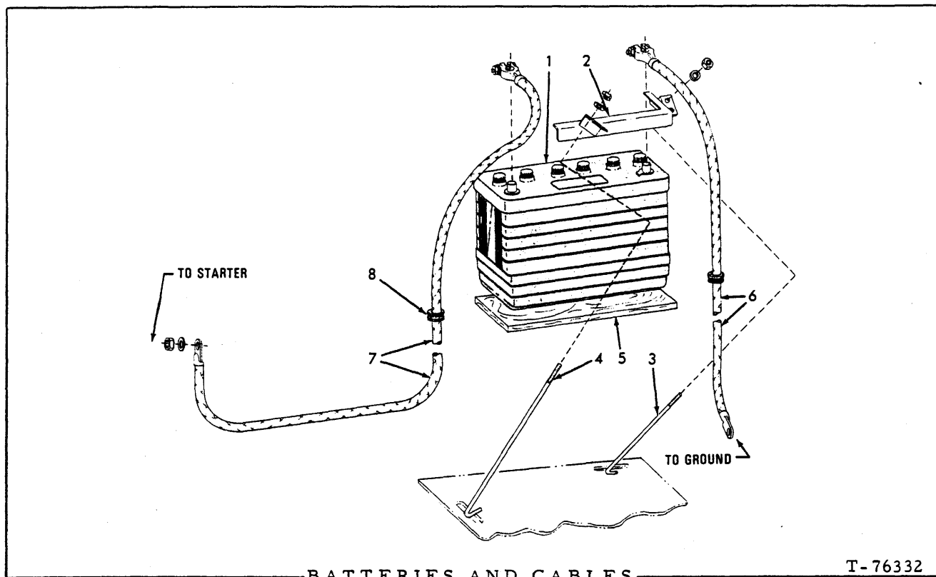
BATTERIES AND CABLES
