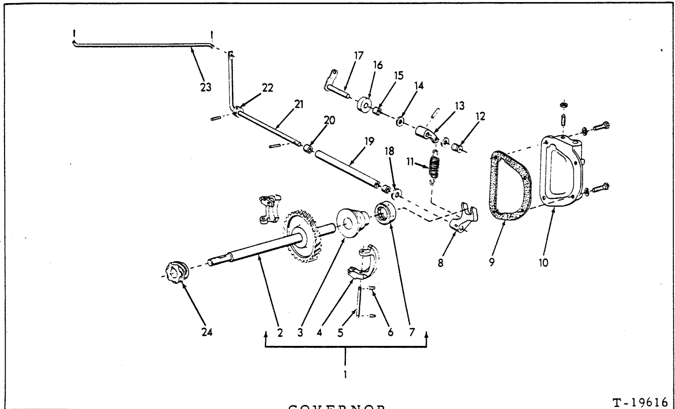
GOVERNOR
