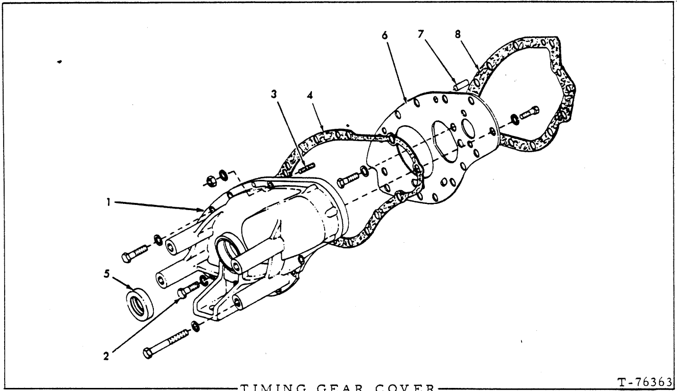
TIMING GEAR COVER
