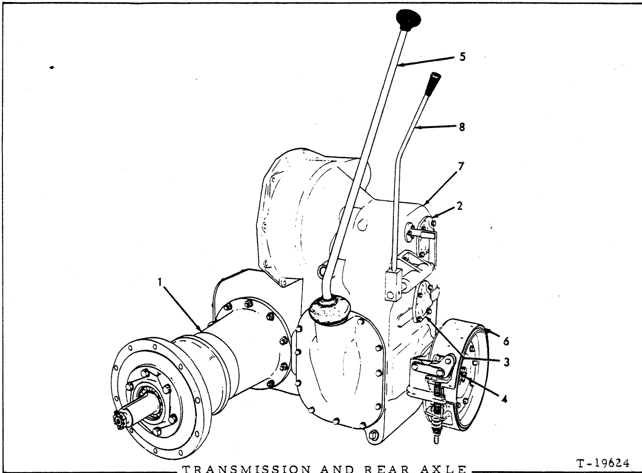
TRANSMISSION AND REAR AXLE
