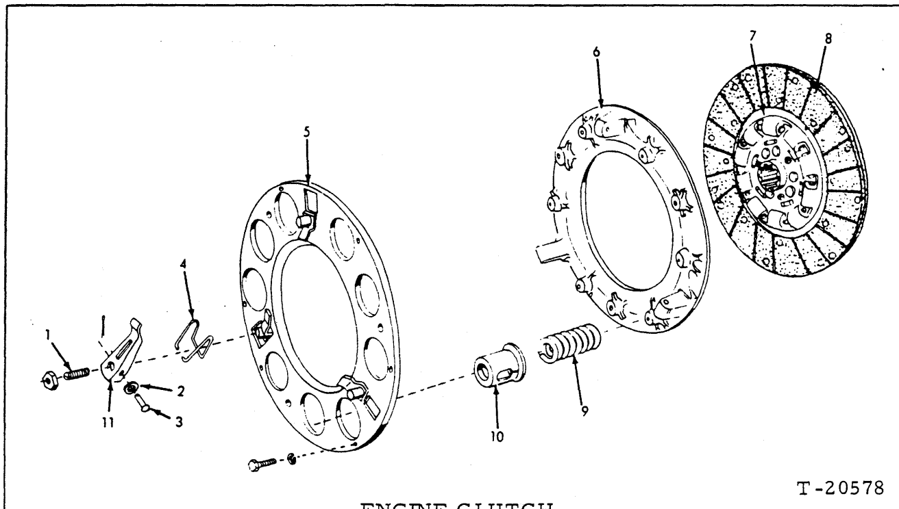
ENGINE CLUTCH (Rockford)
