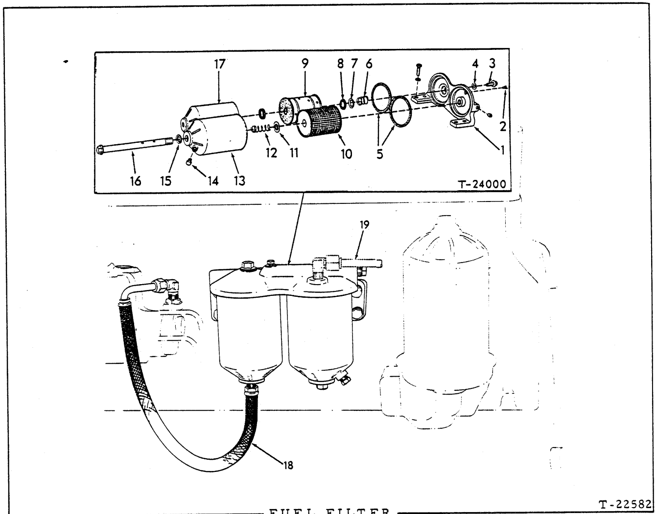
FUEL FILTER
