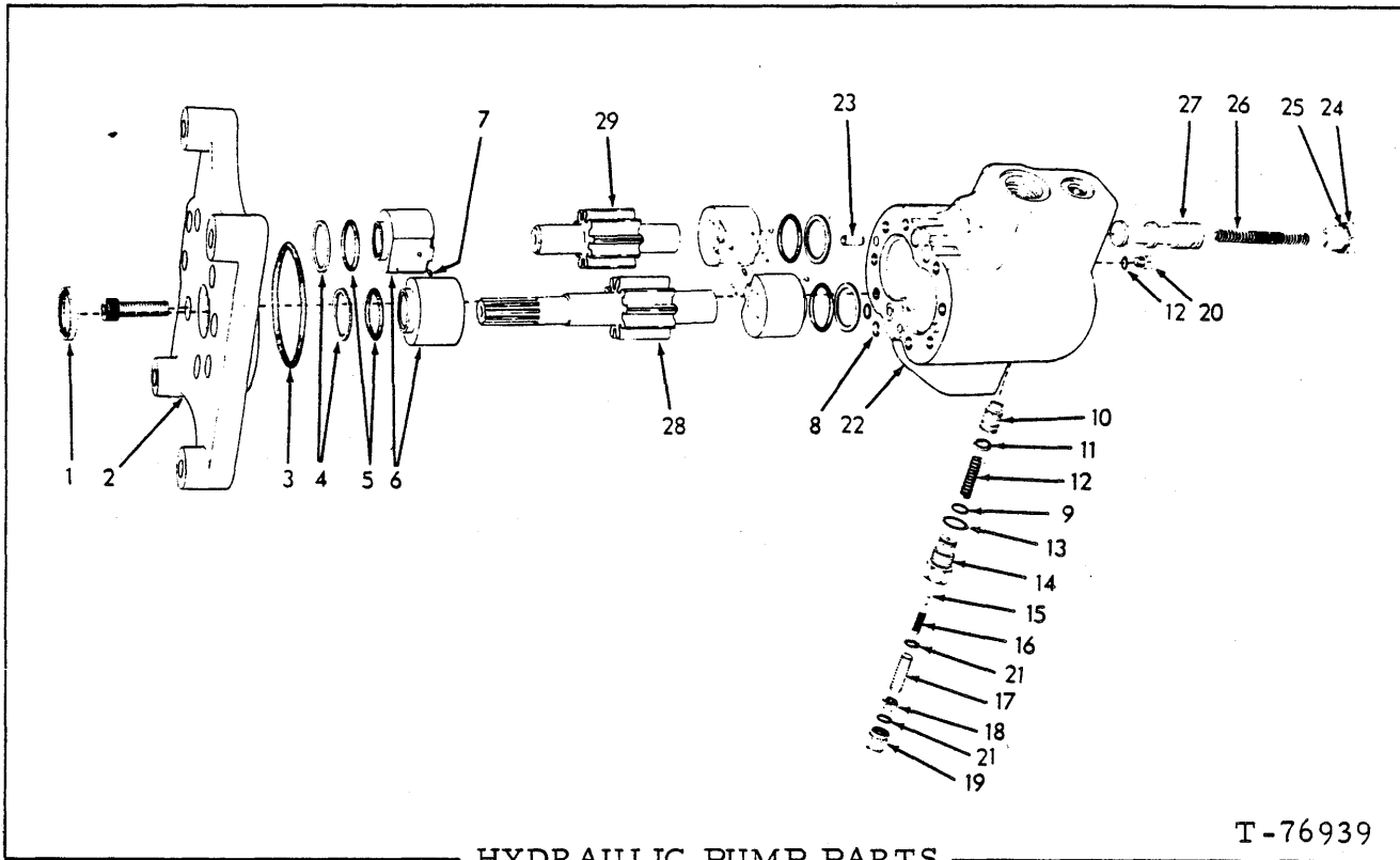
HYDRAULIC PUMP PARTS
