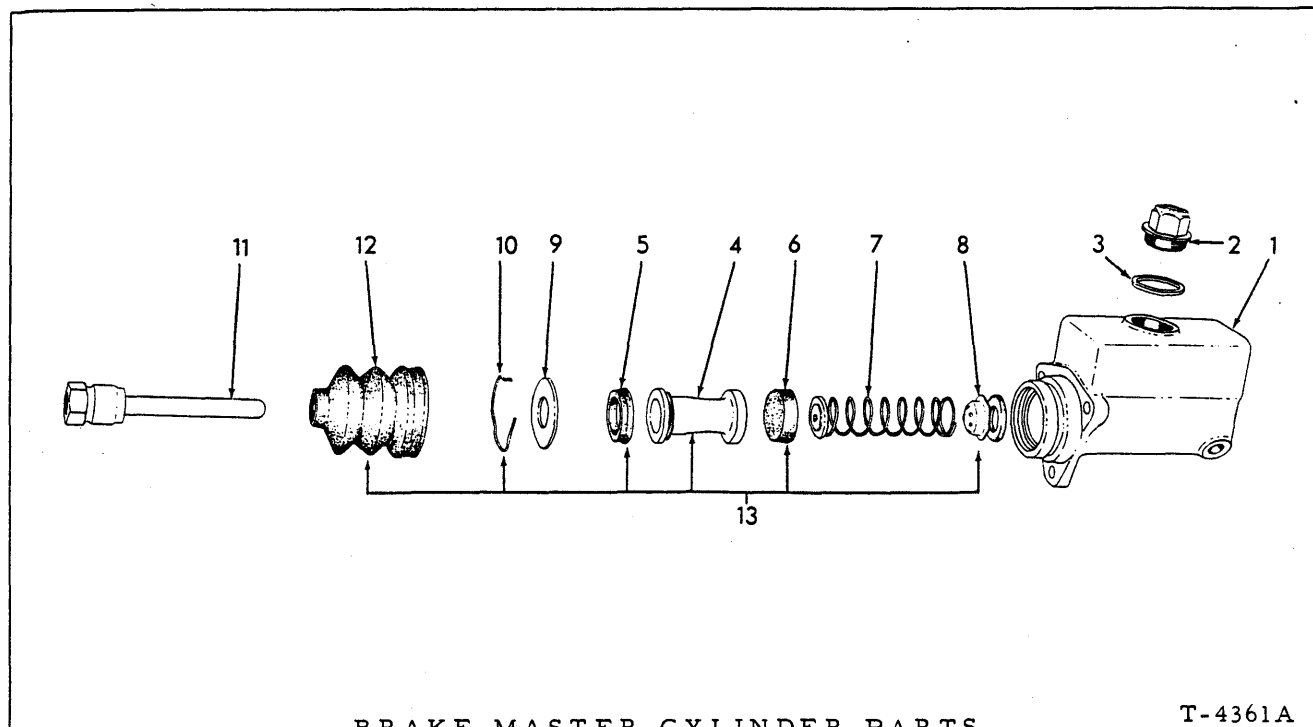
BRAKE MASTER CYLINDER PARTS
