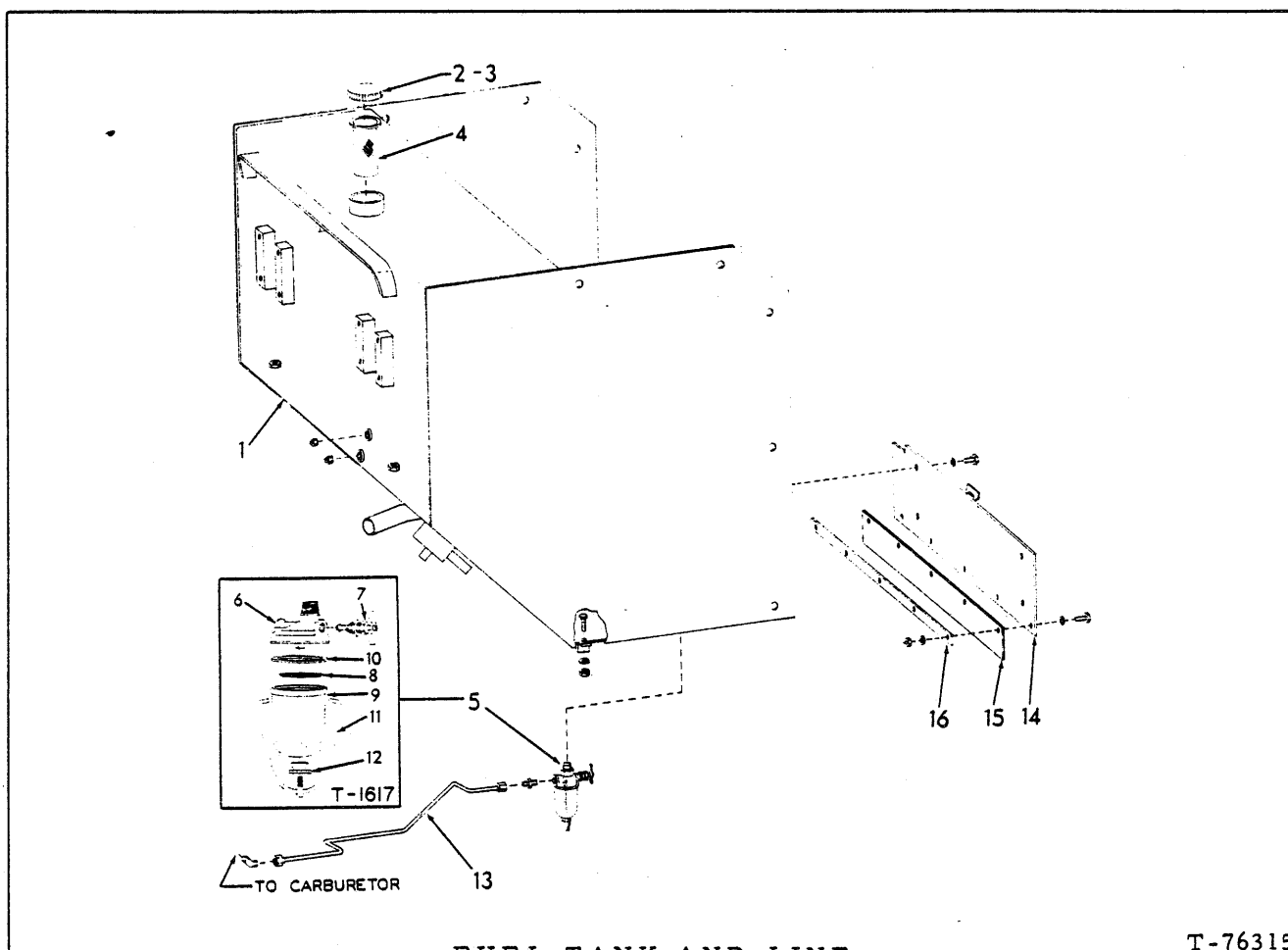
FUEL TANK AND LINE
