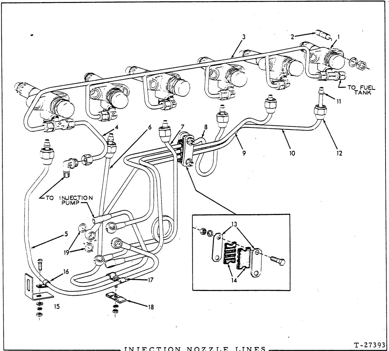
INJECTION NOZZLE LINES
