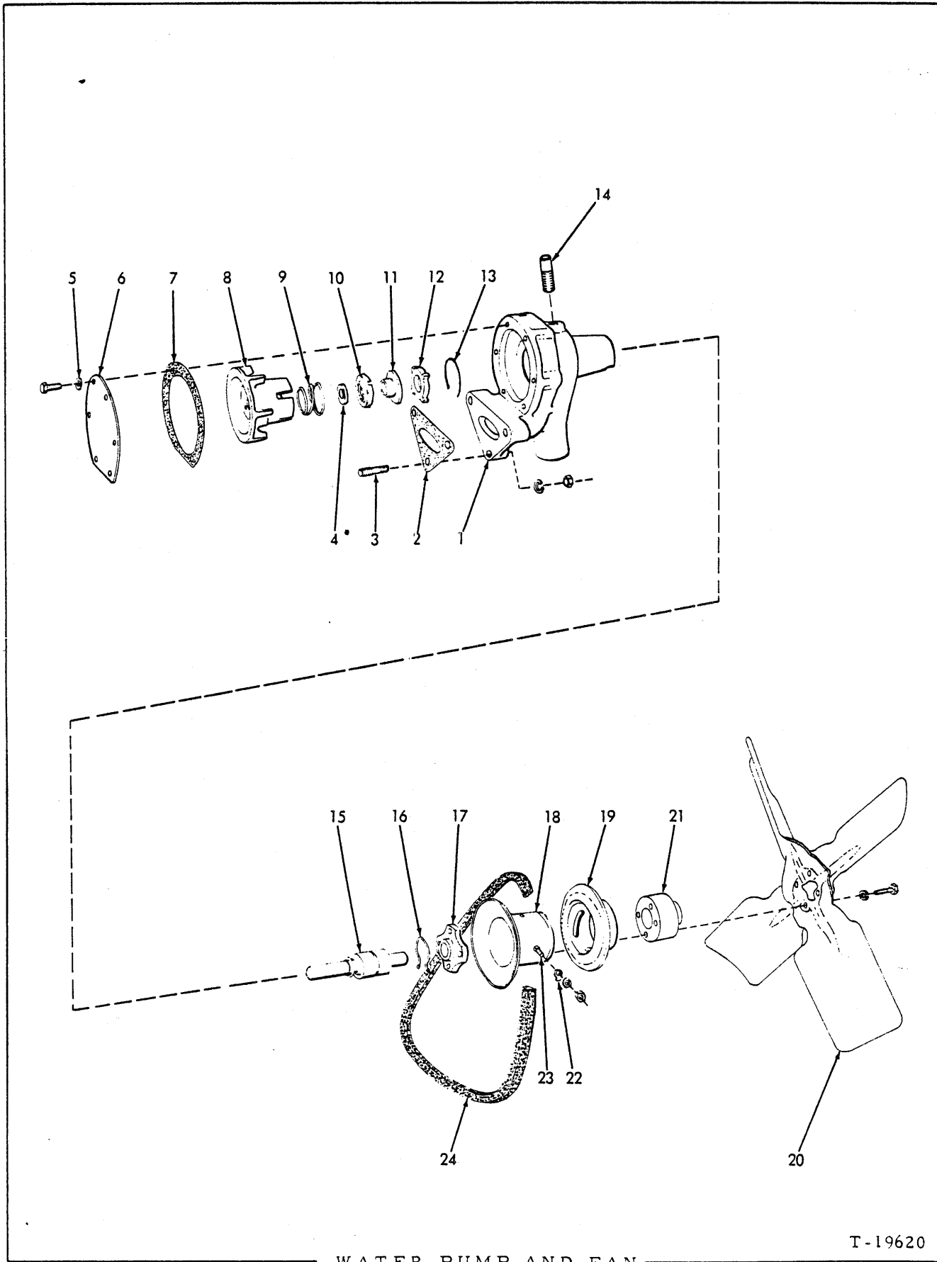
WATER PUMP AND FAN
