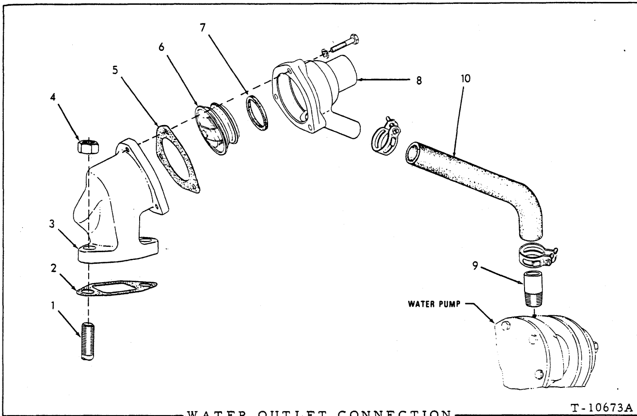
WATER OUTLET CONNECTION
