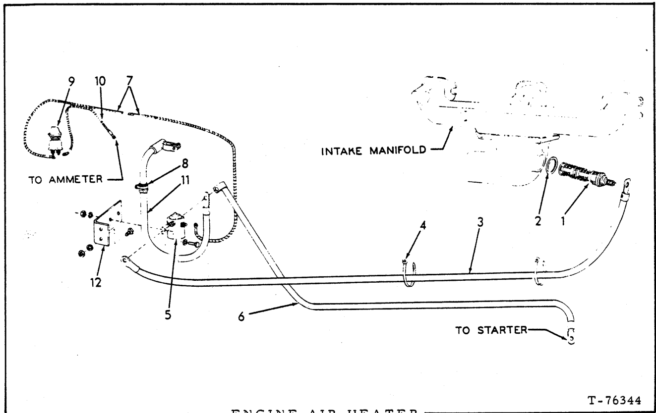
ENGINE AIR HEATER
