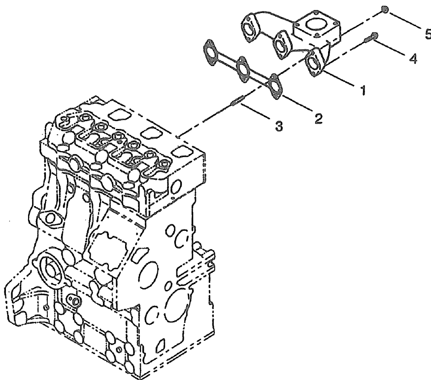
EXHAUST MANIFOLD
