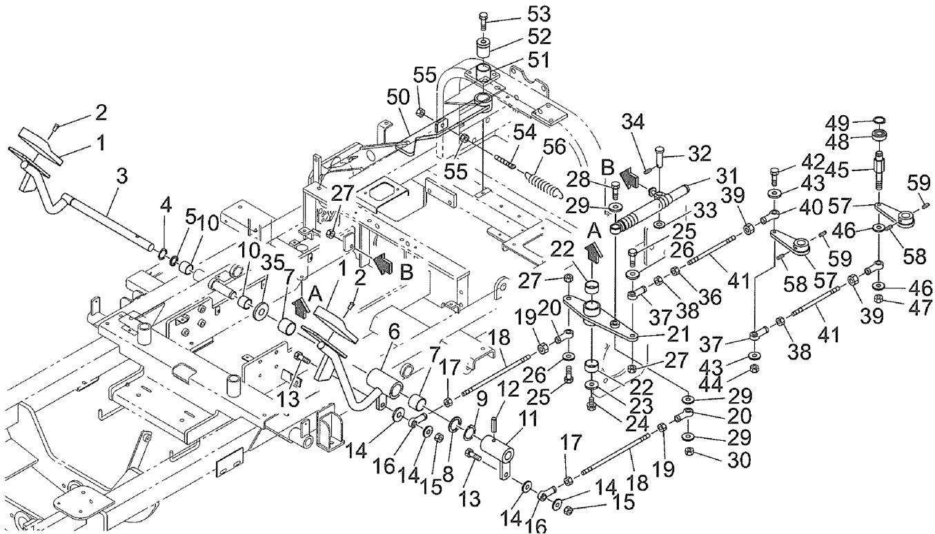
FIG.209 H.S.T CONTROL
