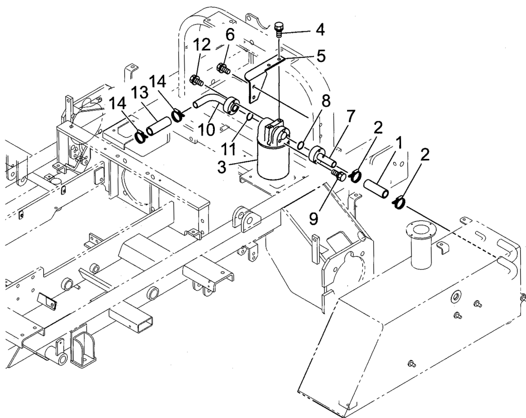
FIG.224 FILTER
