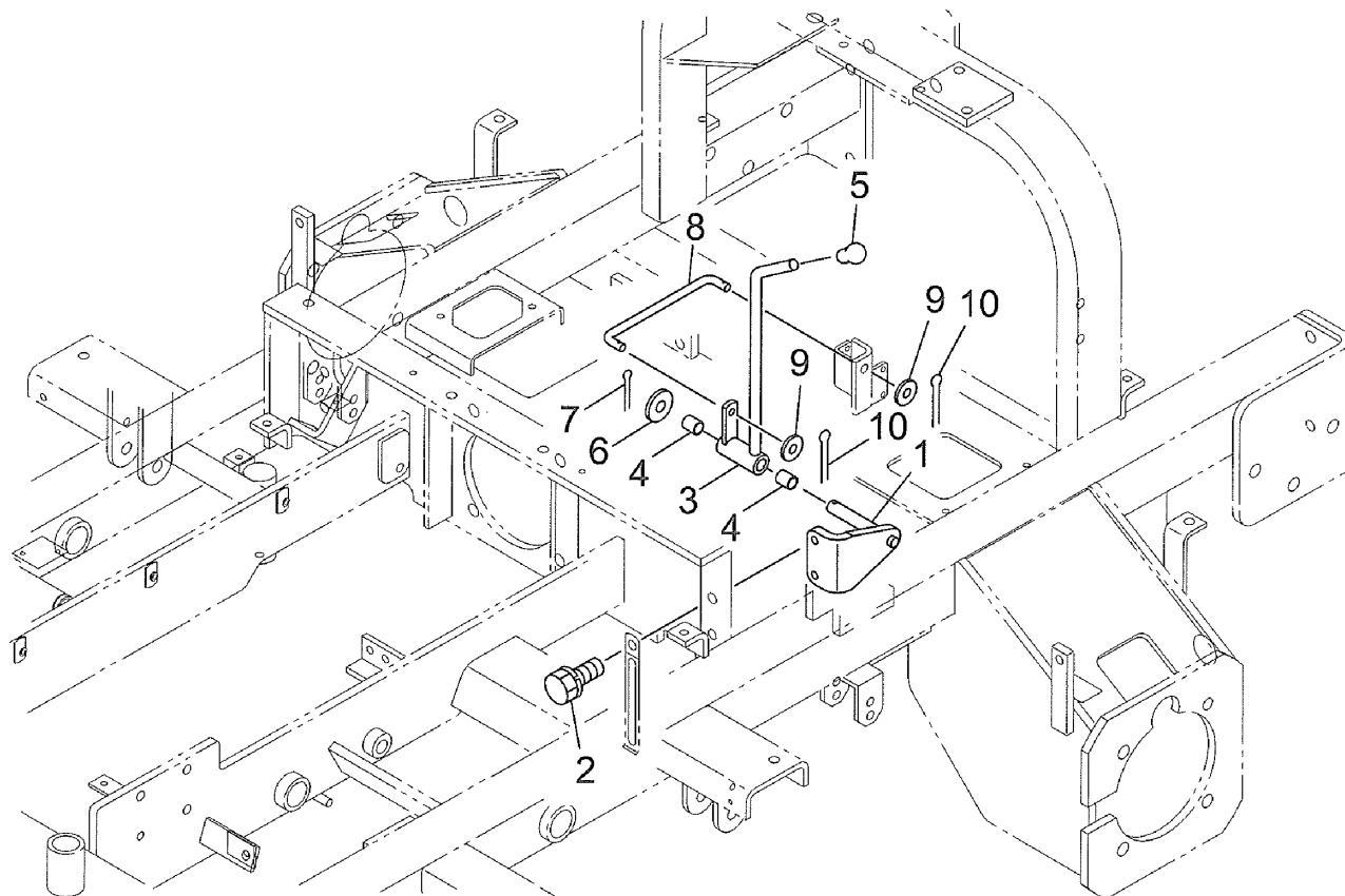
2/4WD VALVE LEVER
