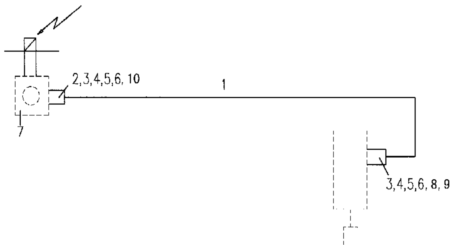
C10-9 4×2 PNEUMATIC DIFFER ENTIAL LOCK FOR STEYR AXLE/单桥轮间差速锁操纵管路 Fig.C10-9
