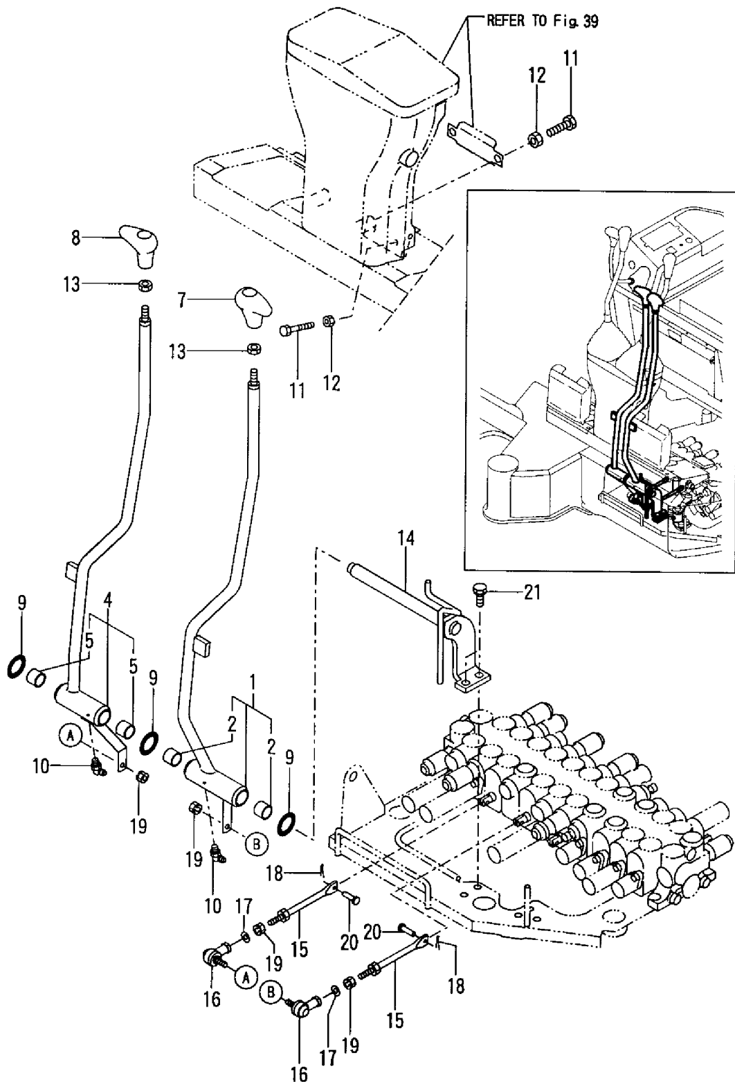
Fig. 40 操纵装置(走行) CONTROL EQUIPMENT(DRIVE)
