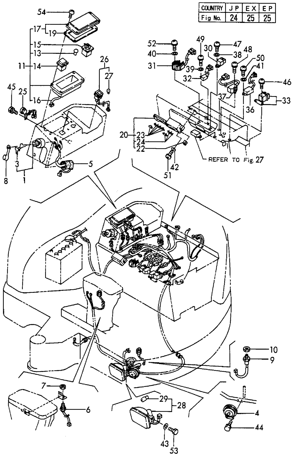
Fig. 25 電装品(機器)(EX, EP) ELECTRIC PART(EQUIPMENT)(EX, EP)
