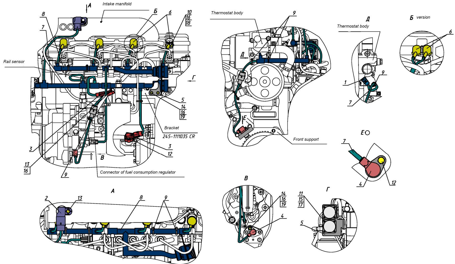
Fig. 17 Installation of electrical equipment.
