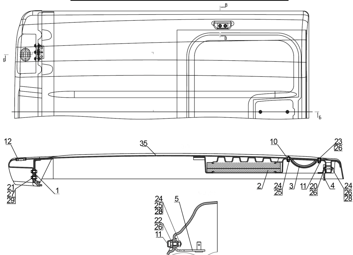
Fig. 67.2. Roof
