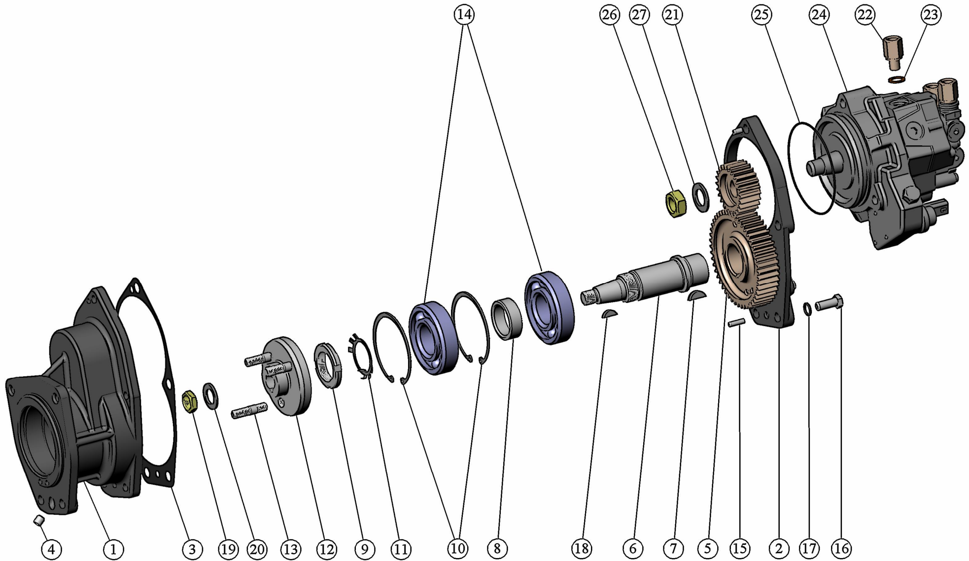
Fig. 8 Fuel pump. Reduction gear unit.
