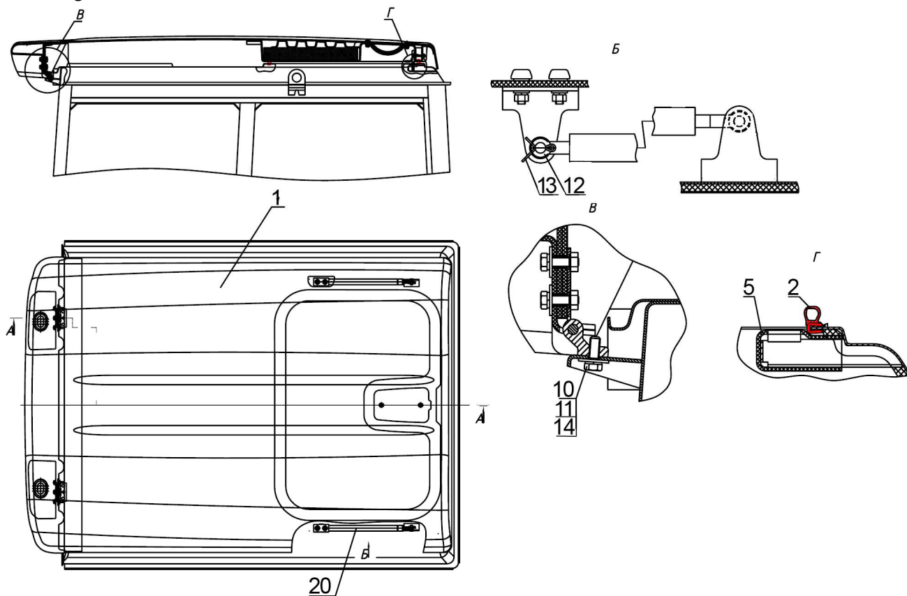
Fig. 67.2. Roof
