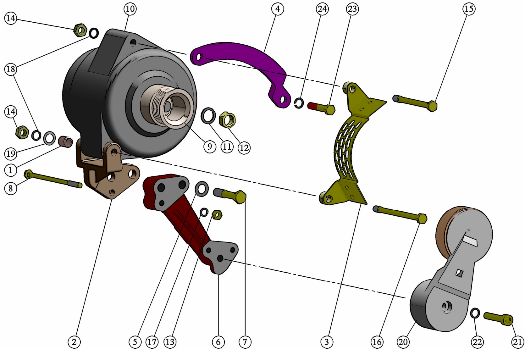
Fig. 18 Alternator installation.
