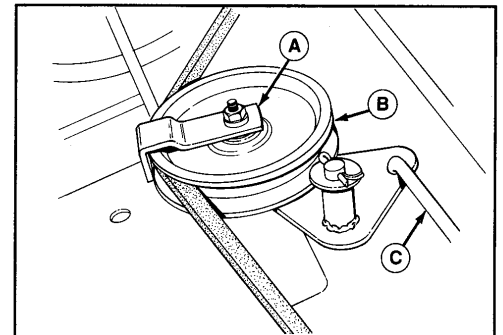
Figure 31. A. Belt Guide B. Idler Pulley C. Clutch Rod
