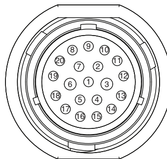
Engine Harness (J2)
