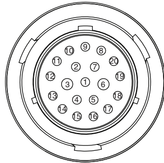
Mower Harness ( J2 )
