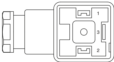
Parking Brake Solenoid (SOL16)
