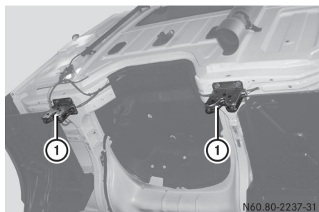
U 20 cab tilt lock
