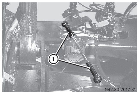
Ball sockets for ALB controller, U 300/400/500
