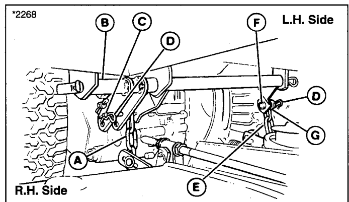
Figure 6. Mower With Electric Lift
