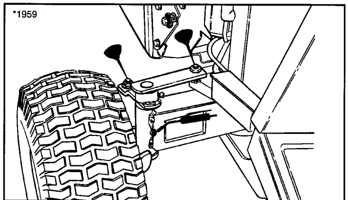
Figure 18. Front Axle Lubrication Points
