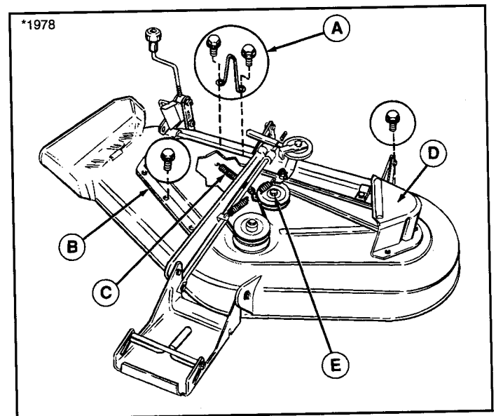
Figure 39. Mower Deck A. Upstop D. L.H. Arbor Cover B. R.H. Arbor Cover E. Capscrew C. Spring
