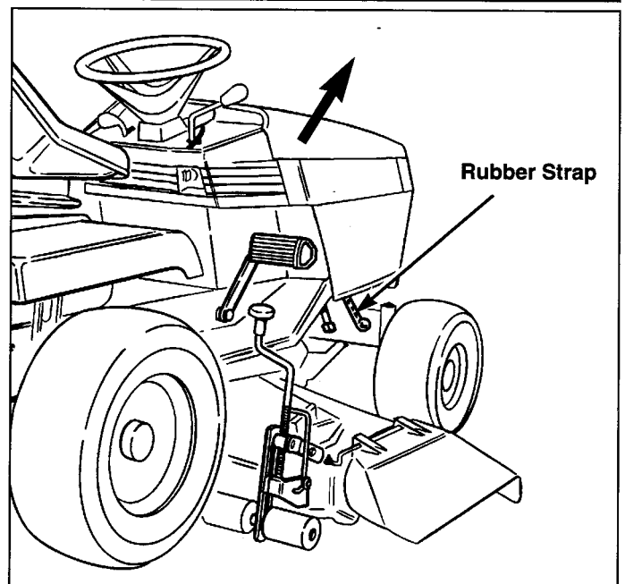
Figure 12. Raising the hood.
