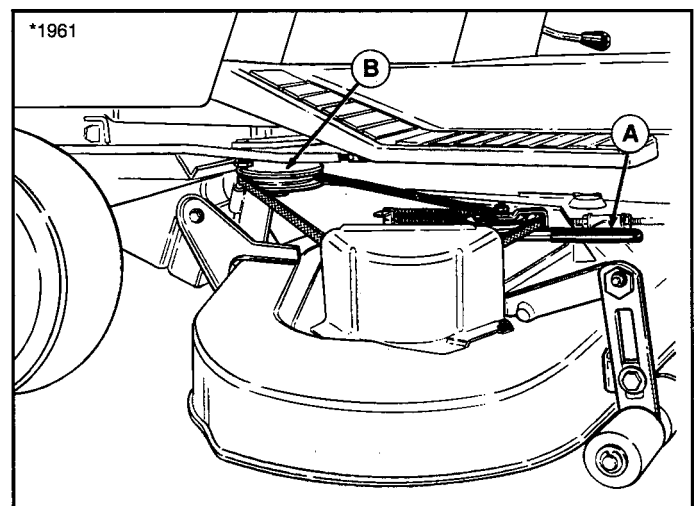
Figure 7. Installing Belt
