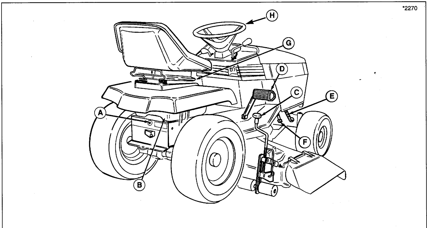
Figure 3. Tractor & Mower Features
