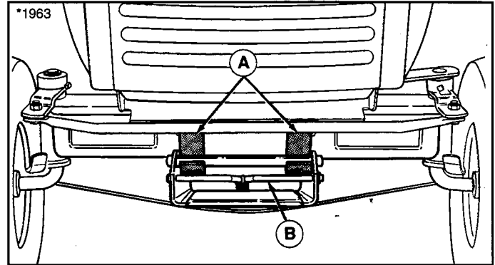
Figure 5. Mower Hitch
