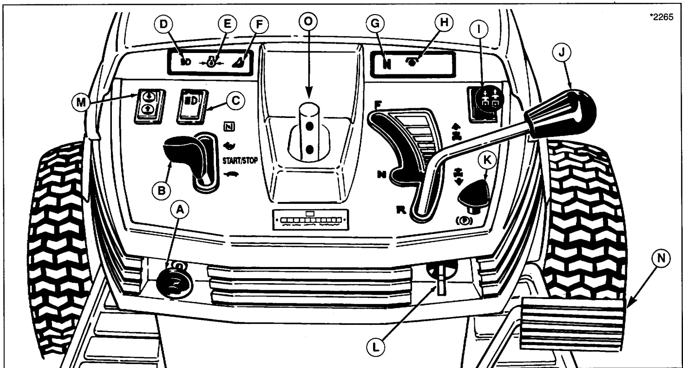
Figure 9. Tractor Controls
