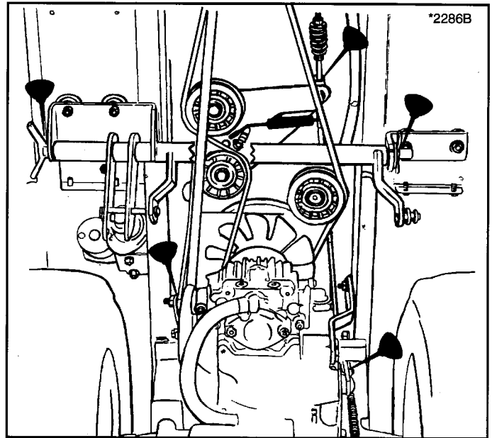
Figure 17. Tractor Lubrication Points - Rear Half
