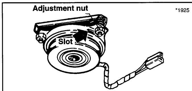
Figure 31. PTO Clutch Adjustment
