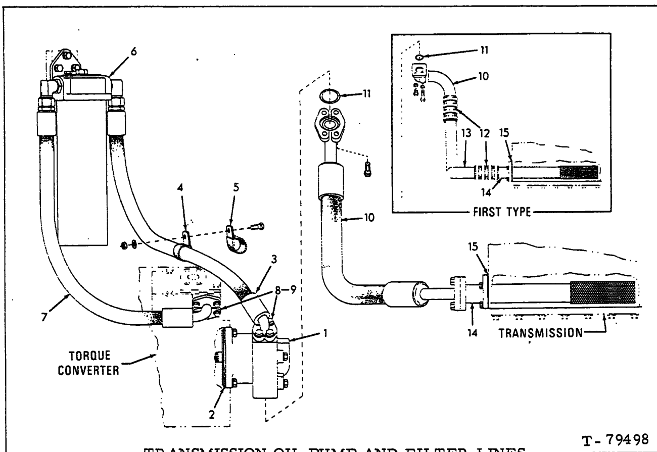
TRANSMISSION OIL PUMP AND FILTER LINES
