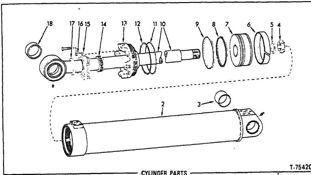
CYLINDER PARTS
