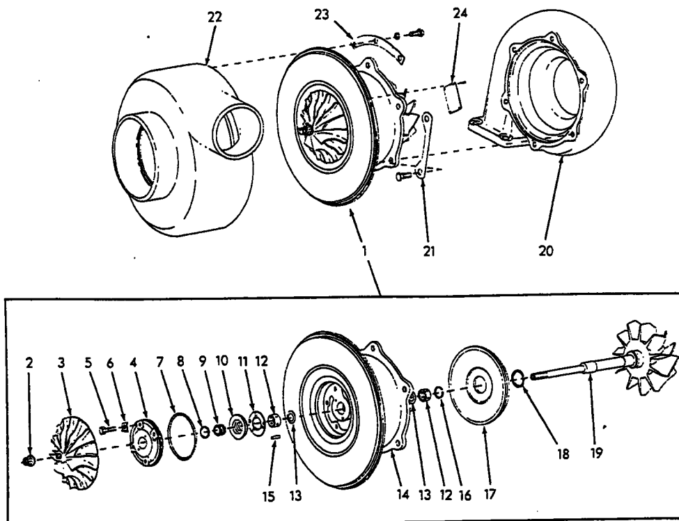
TURBOCHARGER ASSEMBLY
