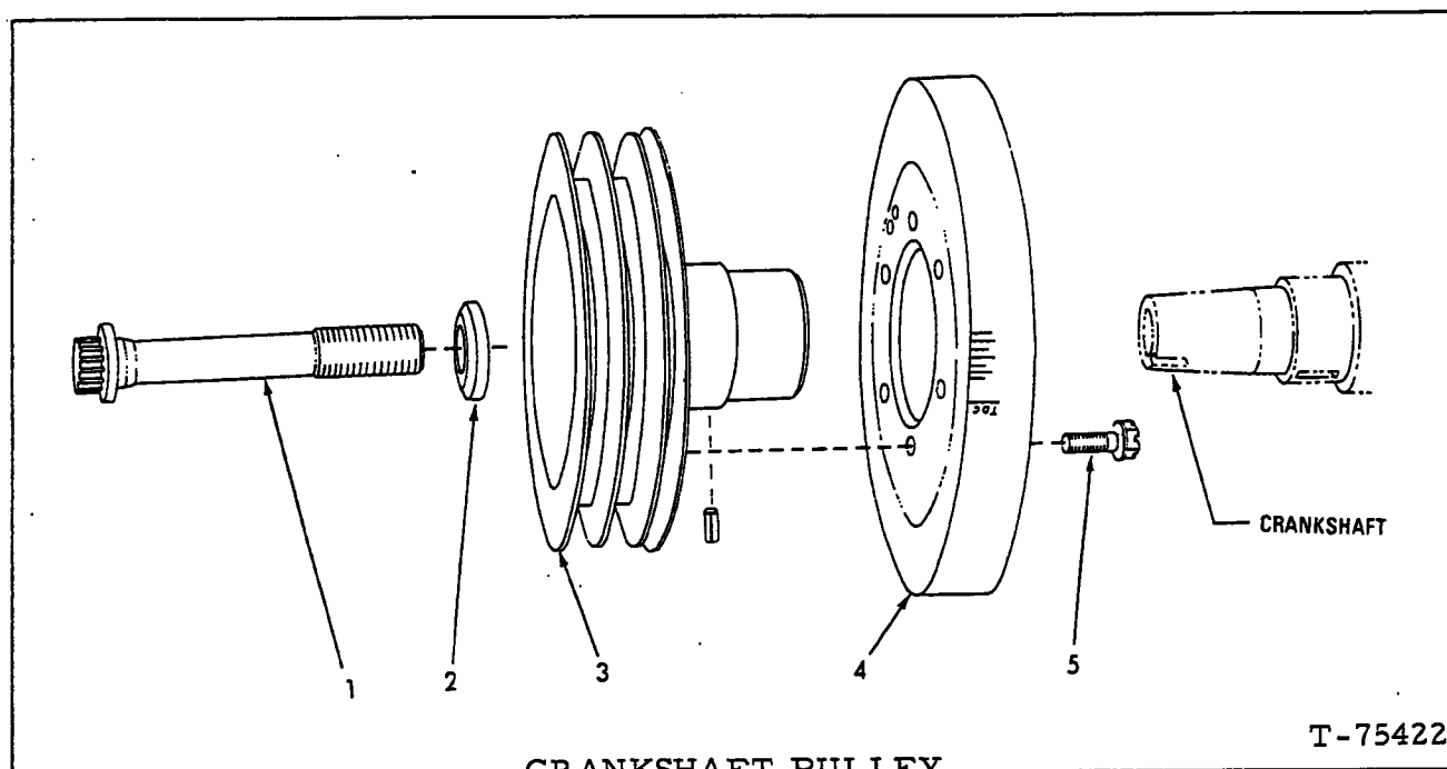
CRANKSHAFT PULLEY
