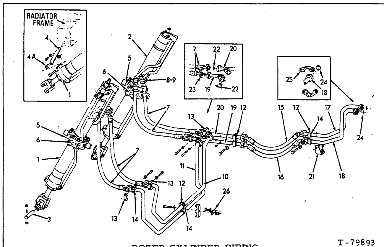
DOZER CYLINDER PIPING
