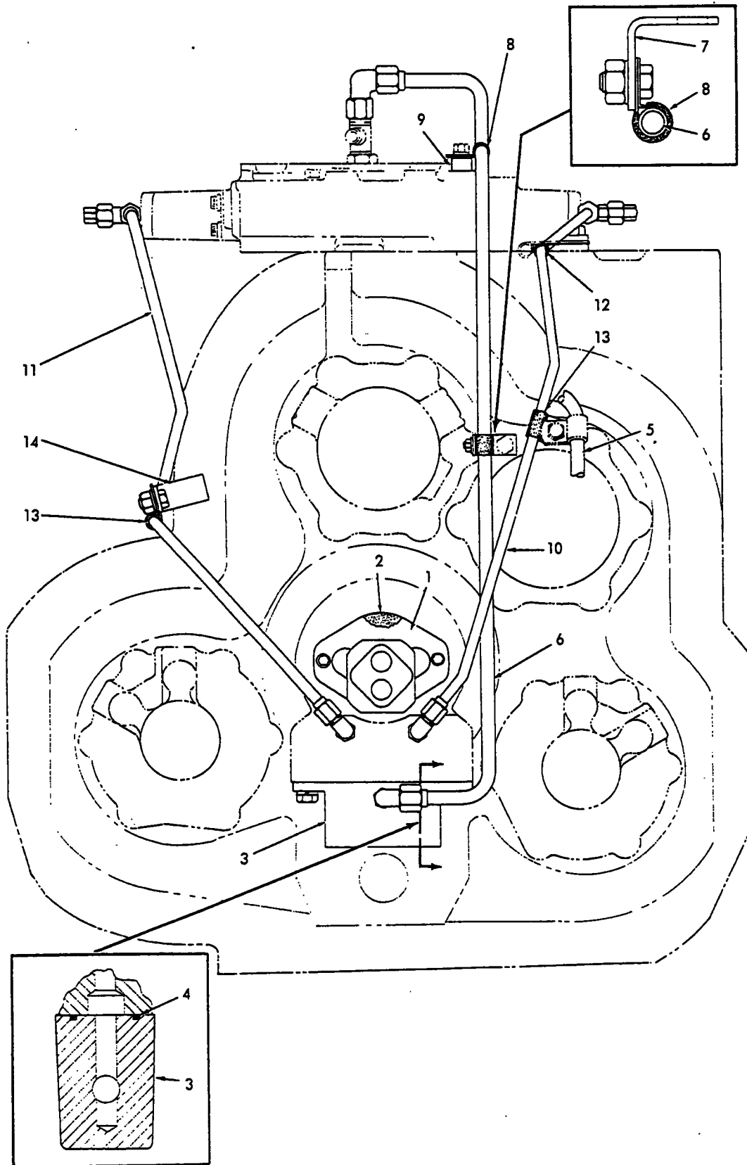
SHIFT INHIBITING PUMP LINES
