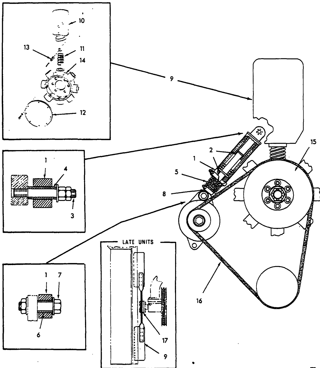
FAN AND BELT TIGHTENER
