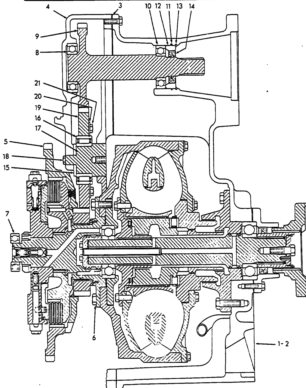
TORQUE CONVERTER ASSEMBLY 73113159
