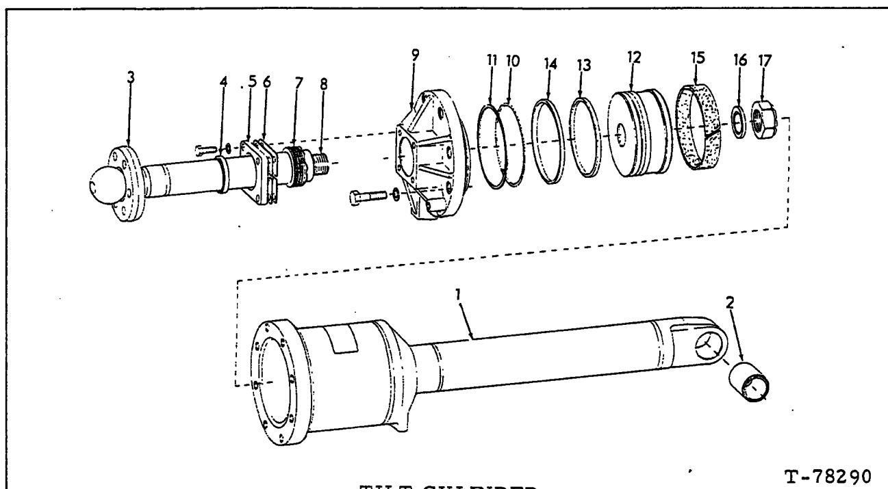
TILT CYLINDER
