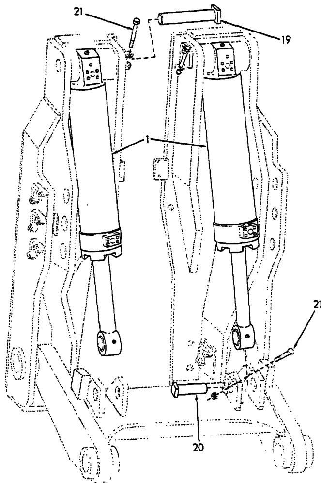
CYLINDER PARTS
