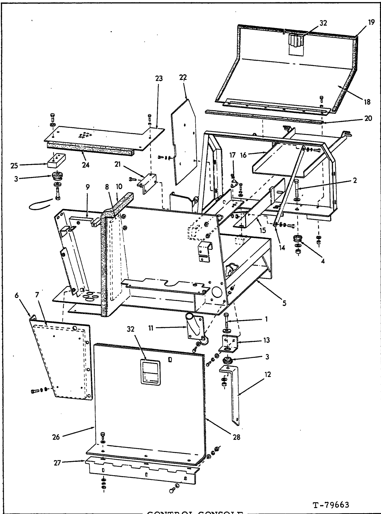
CONTROL CONSOLE
