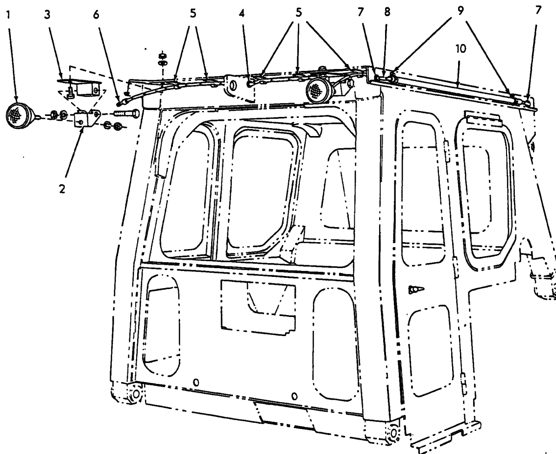
CAB FRONT HEADLIGHTS
