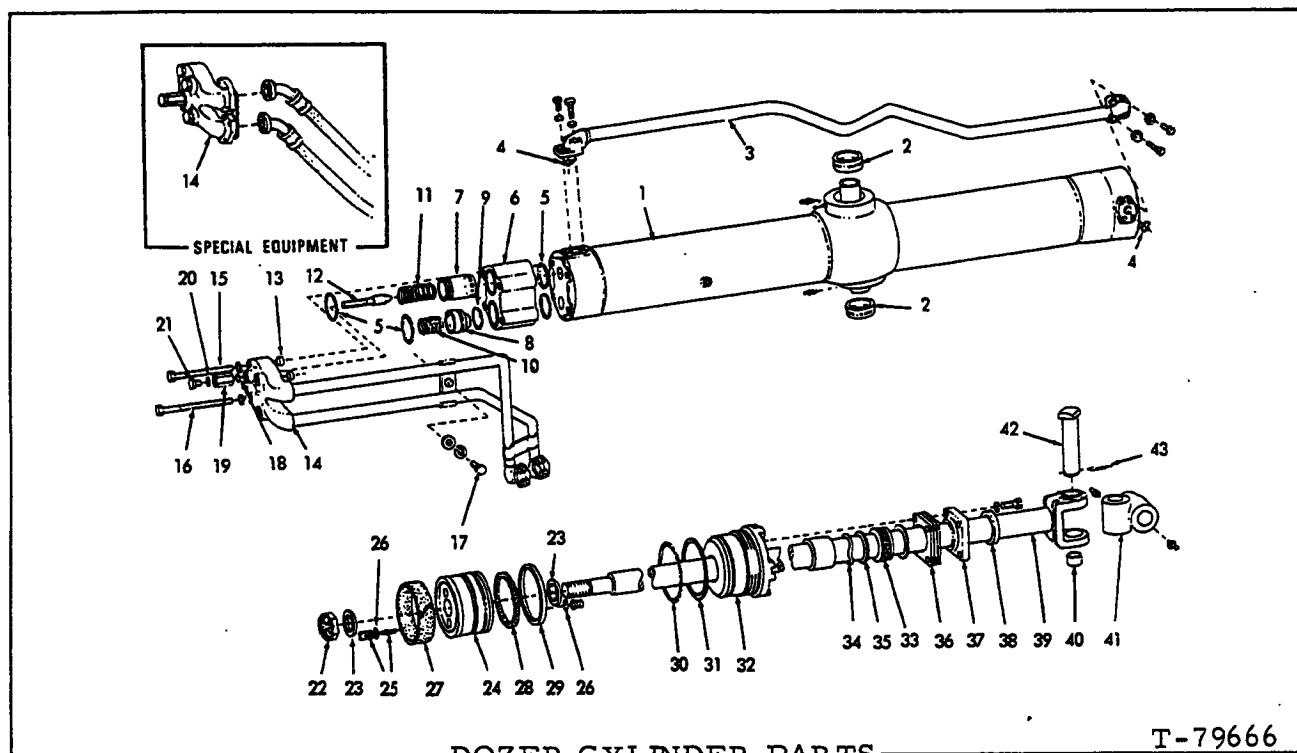
DOZER CYLINDER PARTS
