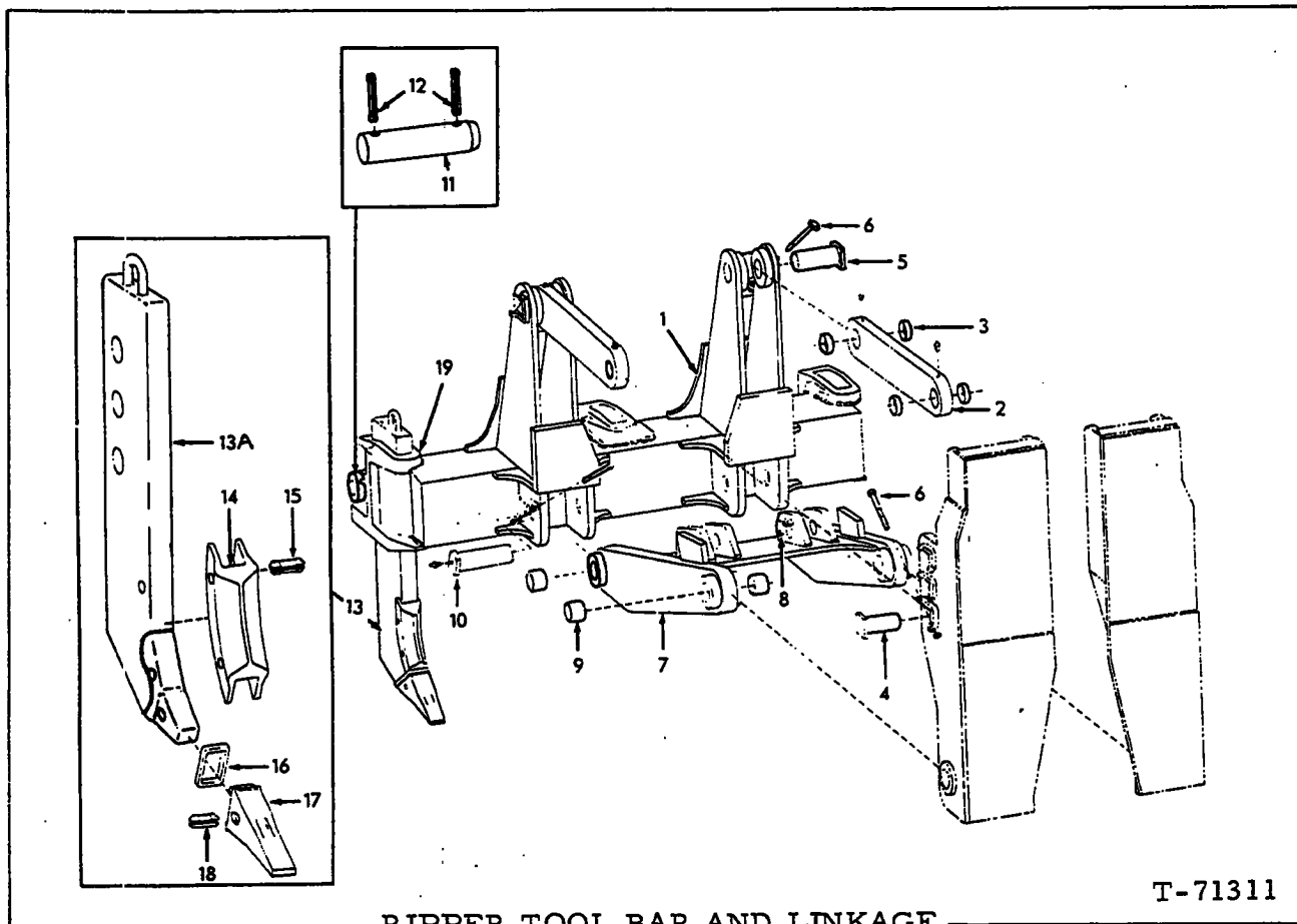
RIPPER TOOL BAR AND LINKAGE
