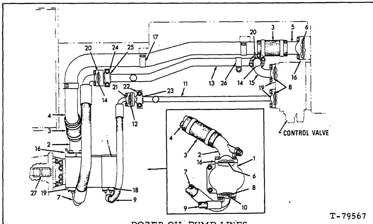
DOZER OIL PUMP LINES
