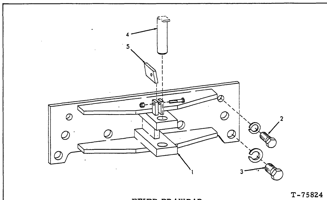
FIXED DRAWBAR
