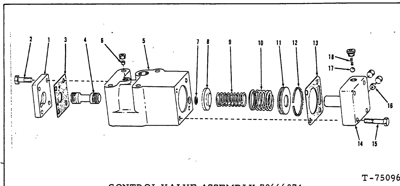
CONTROL VALVE ASSEMBLY 70666074
