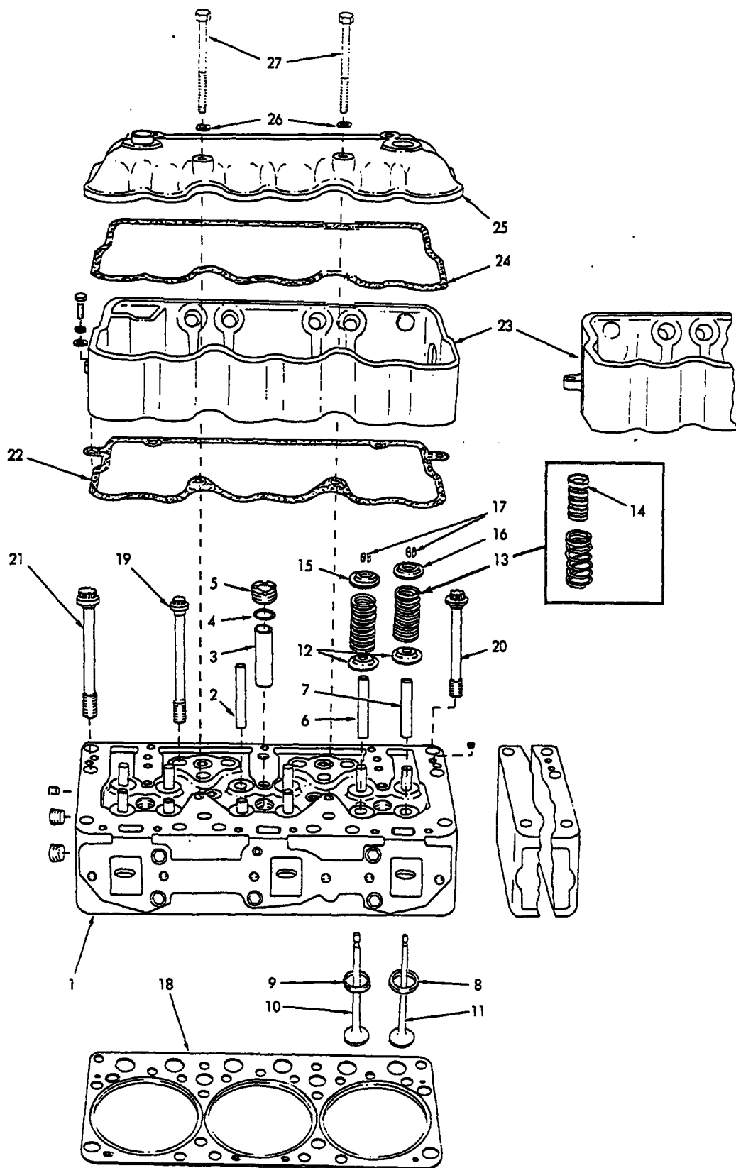
CYLINDER HEAD
