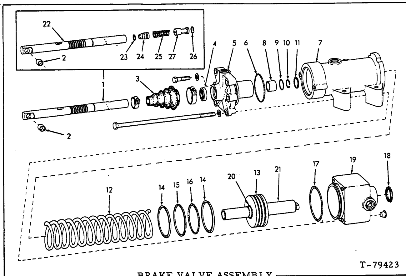
BRAKE VALVE ASSEMBLY
