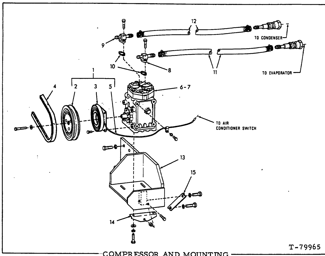
COMPRESSOR AND MOUNTING
