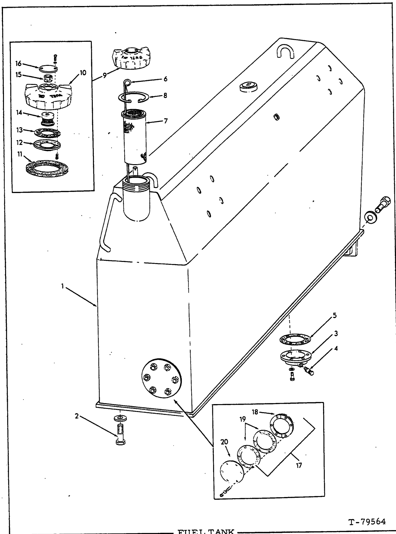
FUEL TANK
