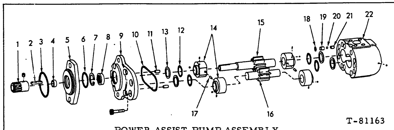
POWER ASSIST PUMP ASSEMBLY
