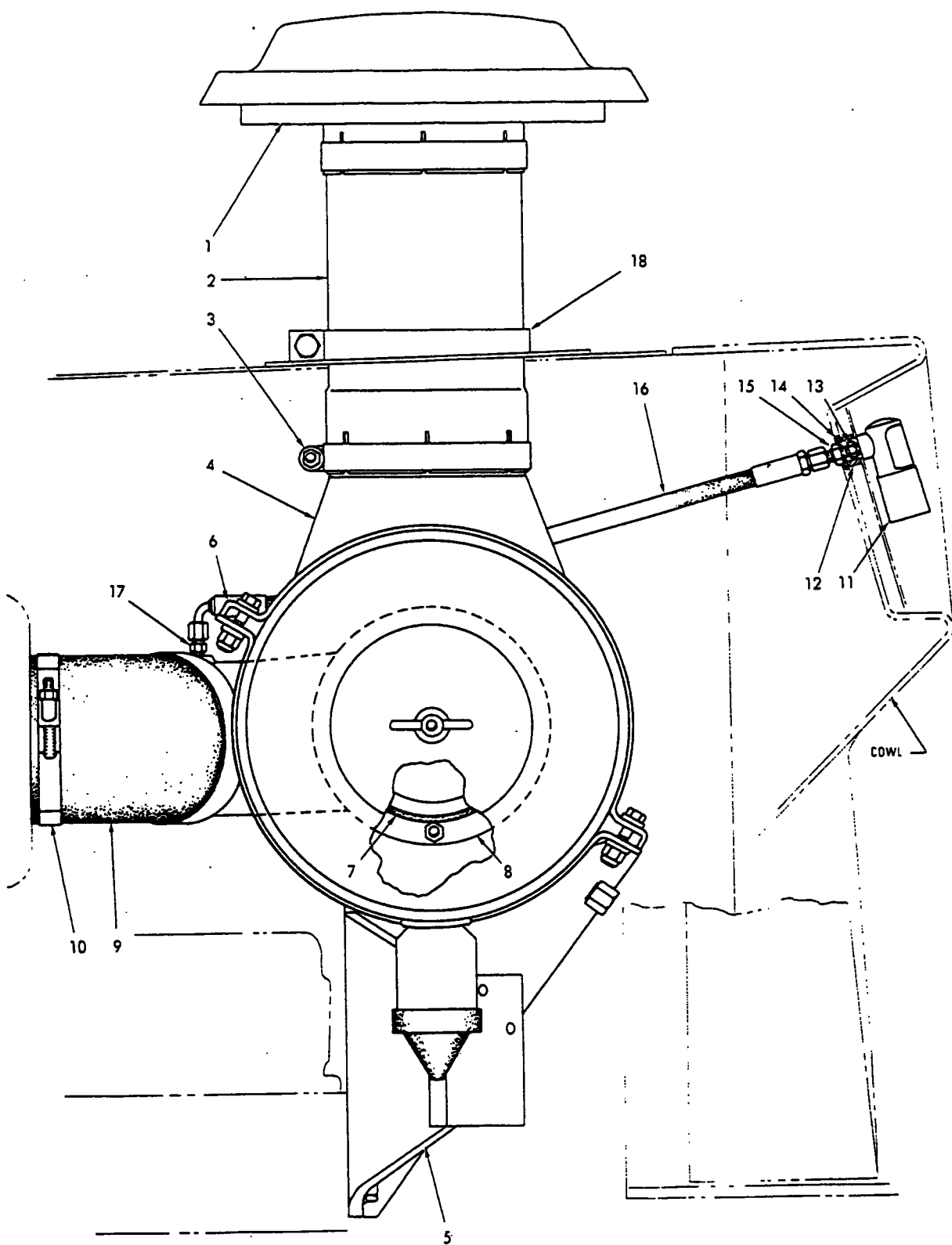
AIR CLEANER
