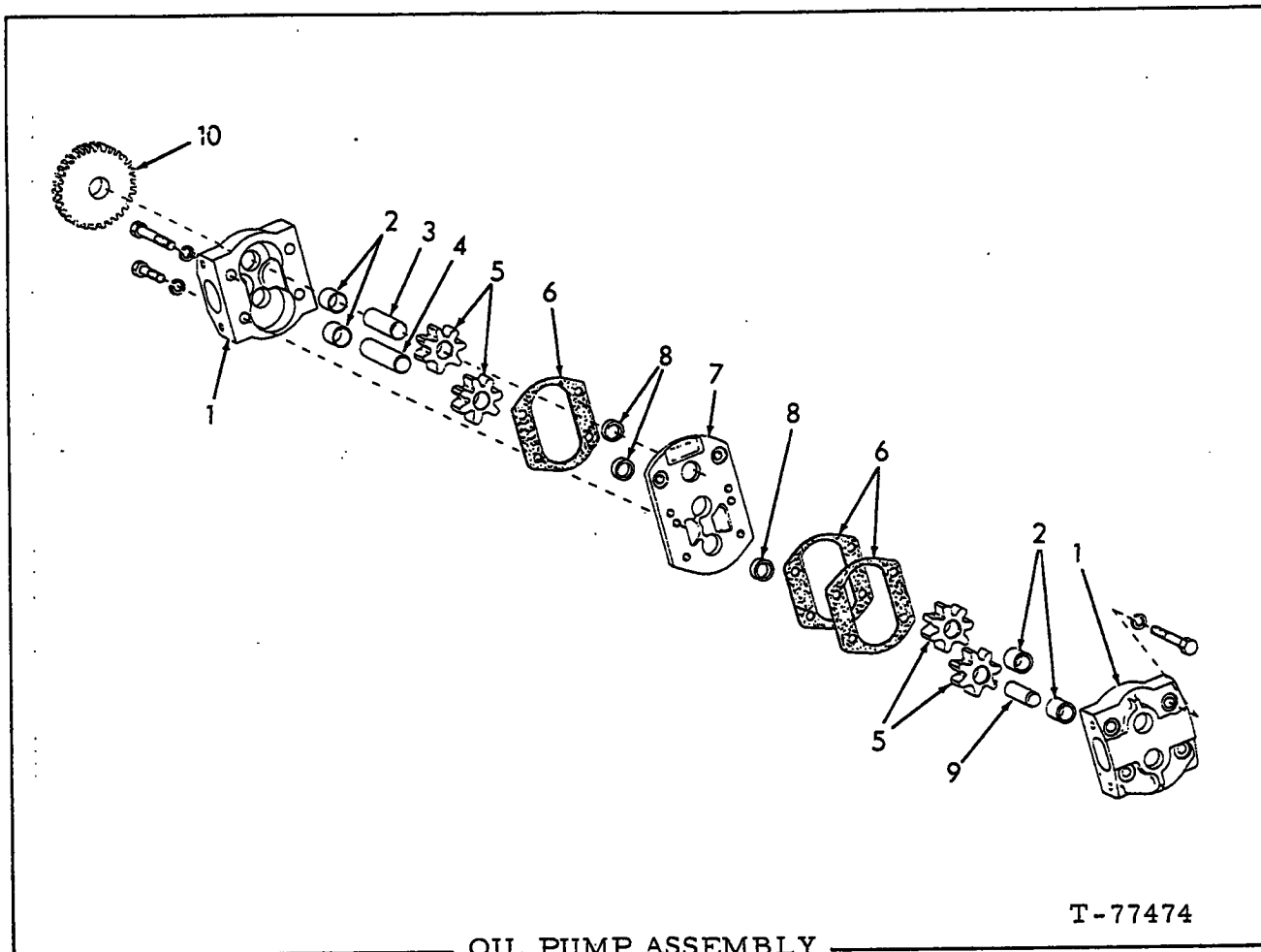
OIL PUMP ASSEMBLY
