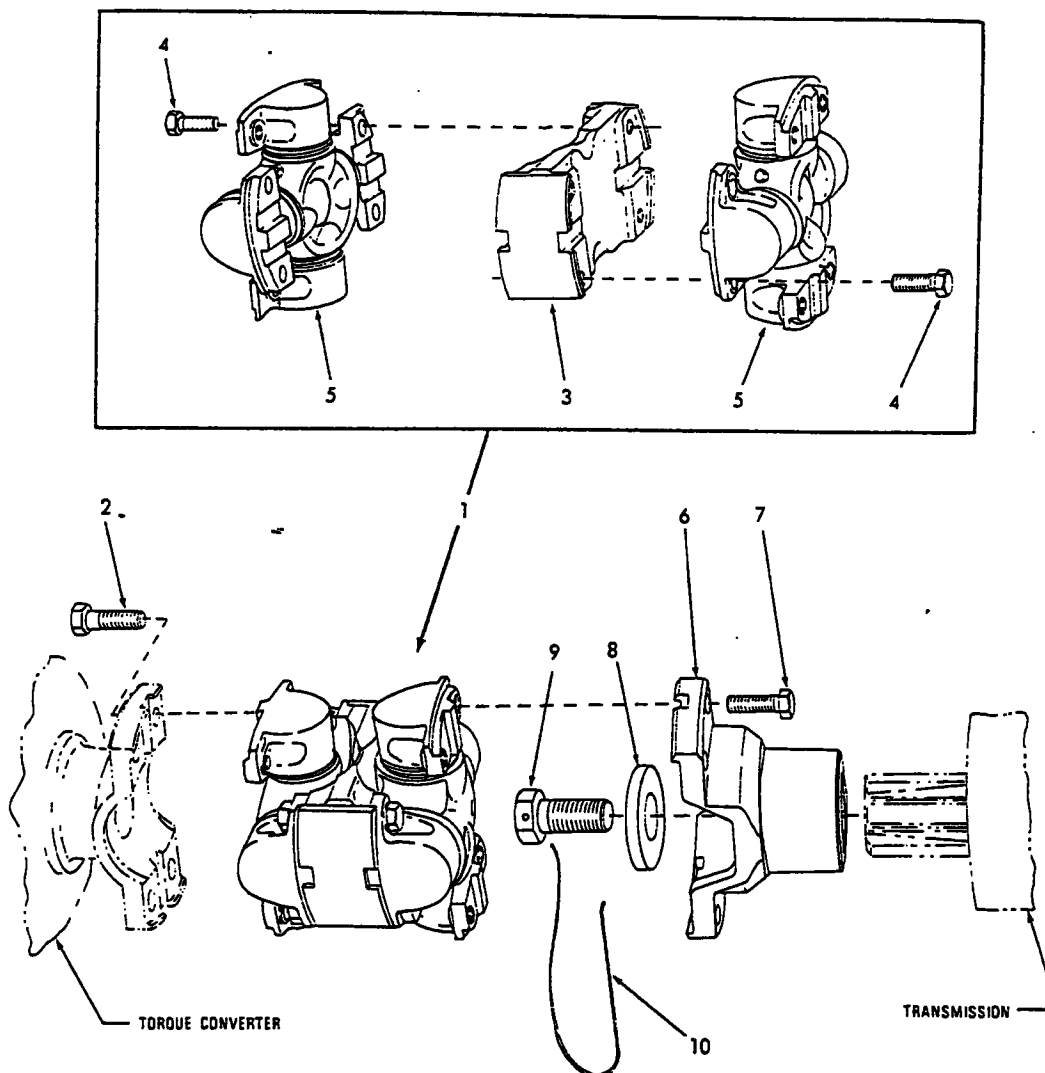
UNIVERSAL JOINT
