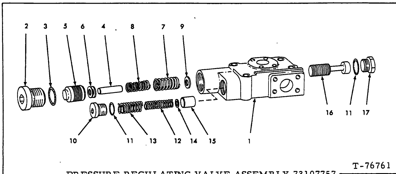
PRESSURE REGULATING VALVE ASSEMBLY 73107757
