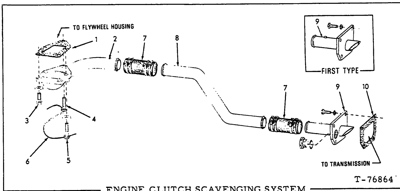
ENGINE CLUTCH SCAVENGING SYSTEM
