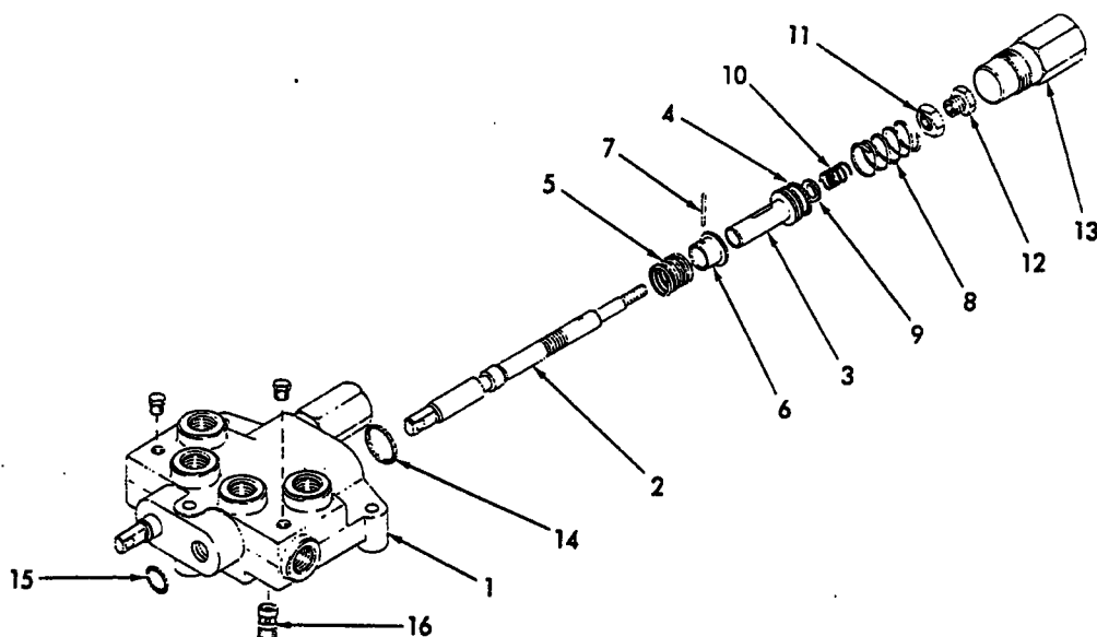
STEERING CONTROL VALVE ASSEMBLY
