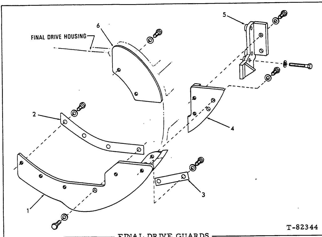
FINAL DRIVE GUARDS
