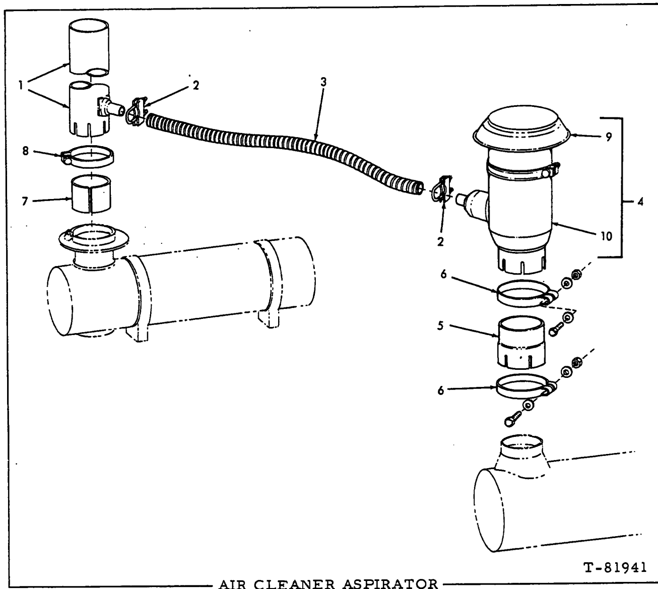
AIR CLEANER ASPIRATOR
