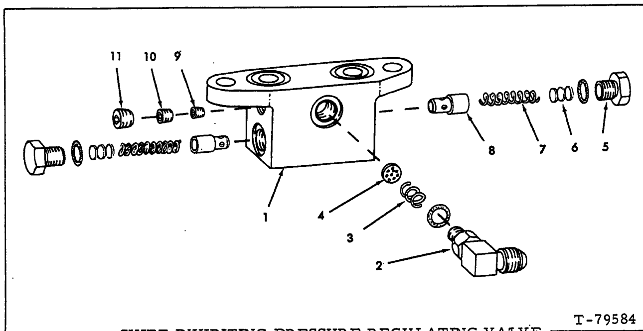
SHIFT INHIBITING PRESSURE REGULATING VALVE
