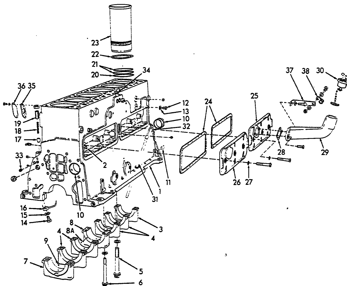
— CYLINDER BLOCK —
