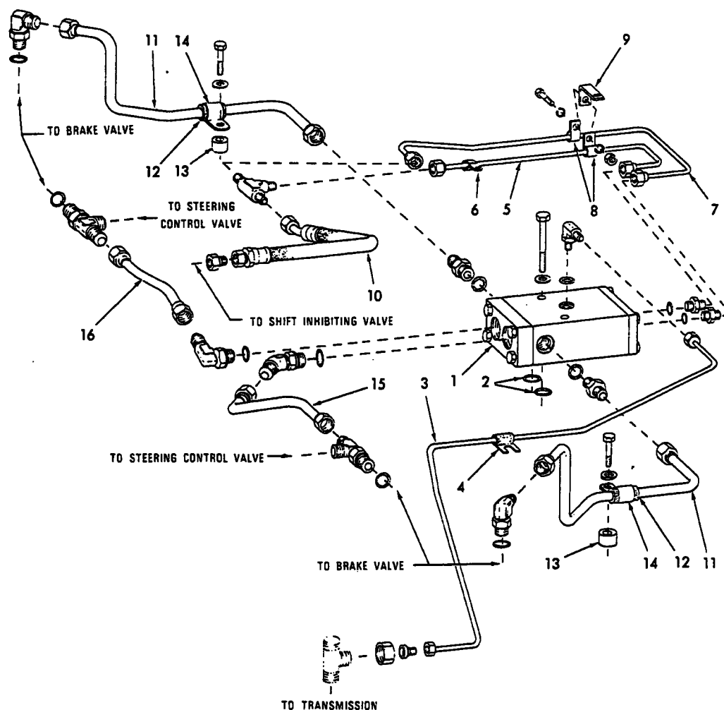
BRAKE REGULATOR VALVE AND LINES
