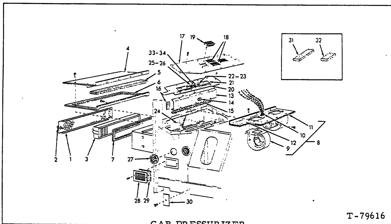
CAB PRESSURIZER
