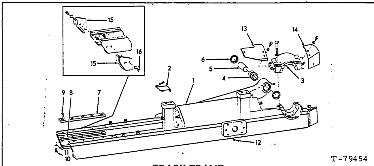
— TRACK FRAME —
