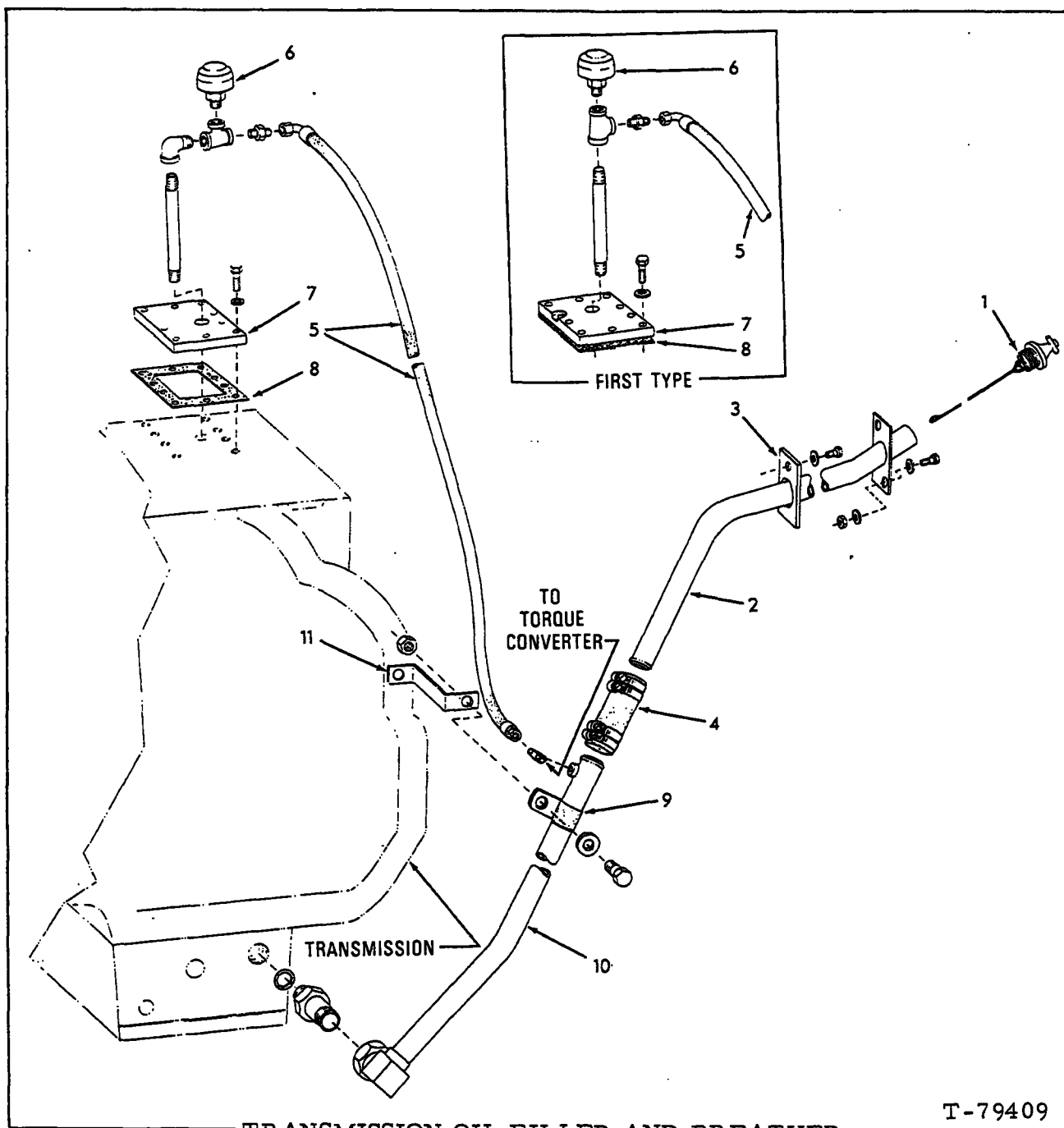
TRANSMISSION OIL FILLER AND BREATHER
