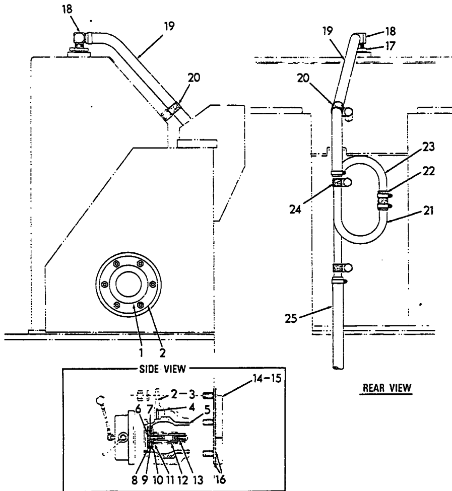
QUICK FUELING
