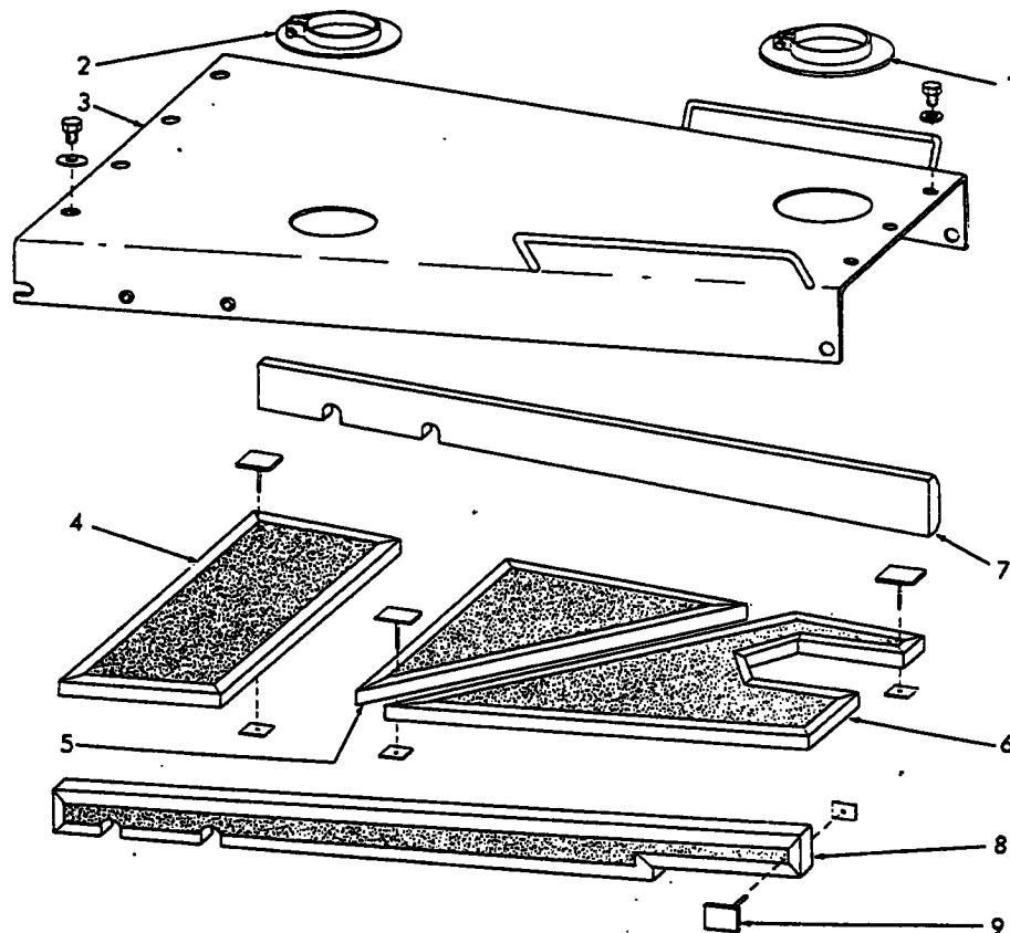
HOOD
