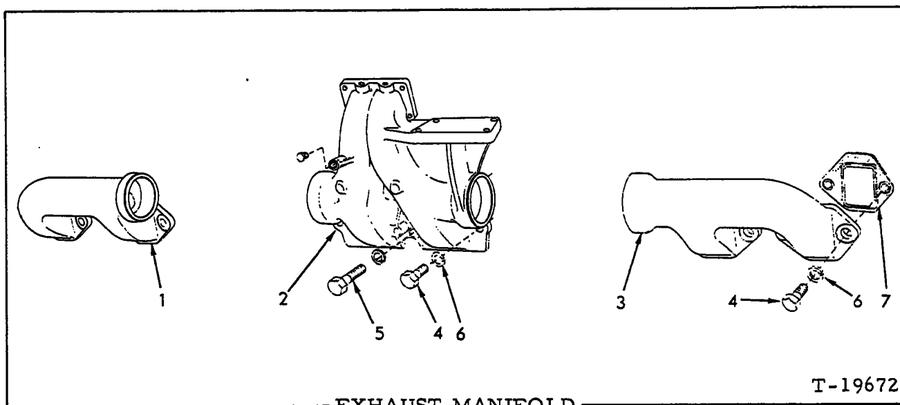
EXHAUST MANIFOLD
