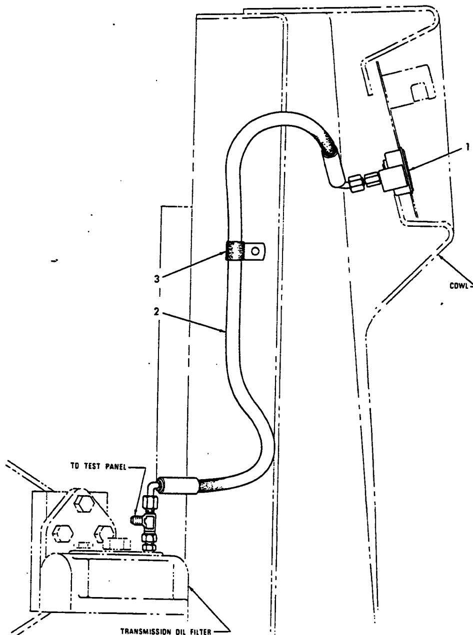
TRANSMISSION OIL PRESSURE GAUGE
