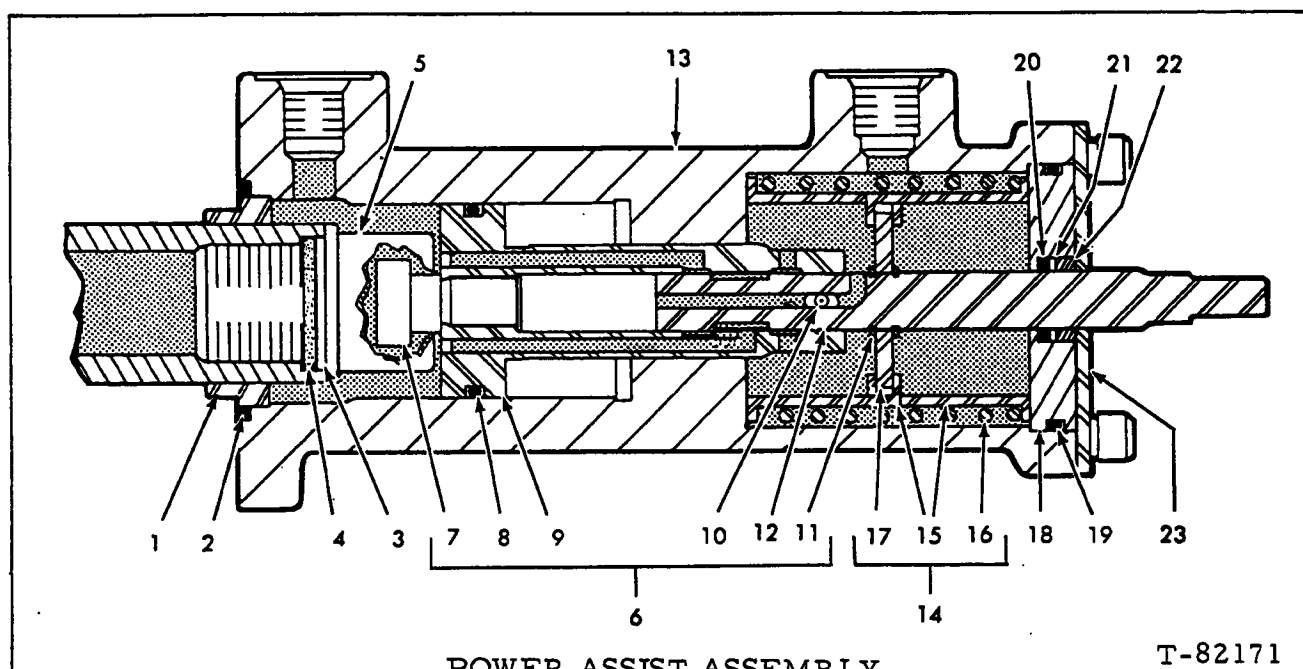
POWER ASSIST ASSEMBLY
