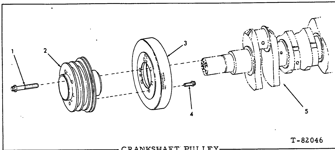
CRANKSHAFT PULLEY
