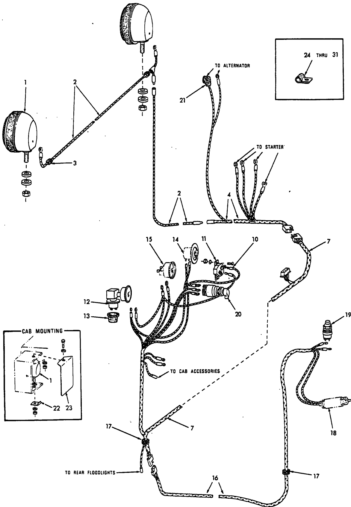
LIGHTS AND WIRING
