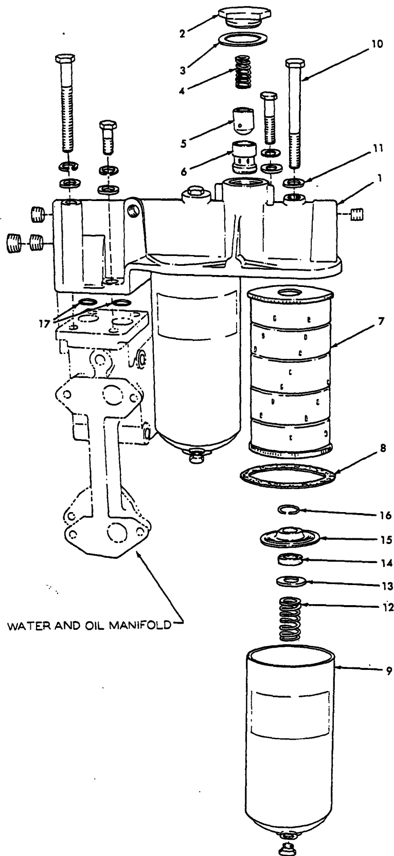
OIL FILTER (Full-flow type)
