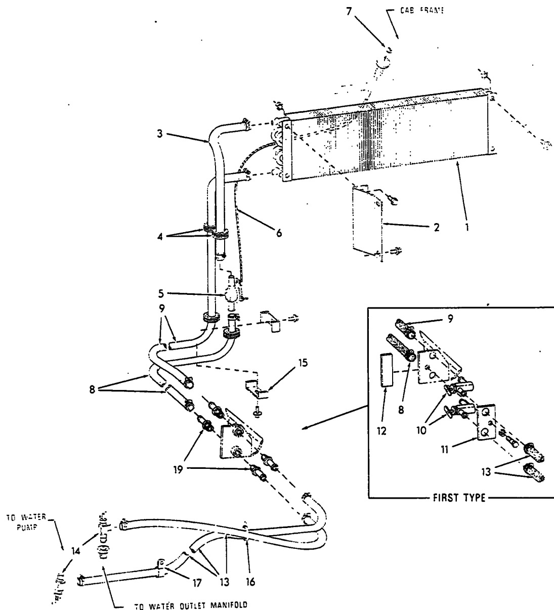
CAB HEATER
