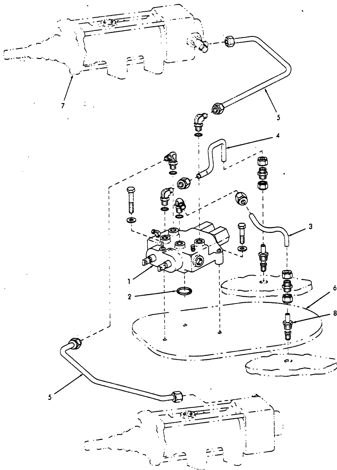
STEERING CONTROL VALVE AND LINES
