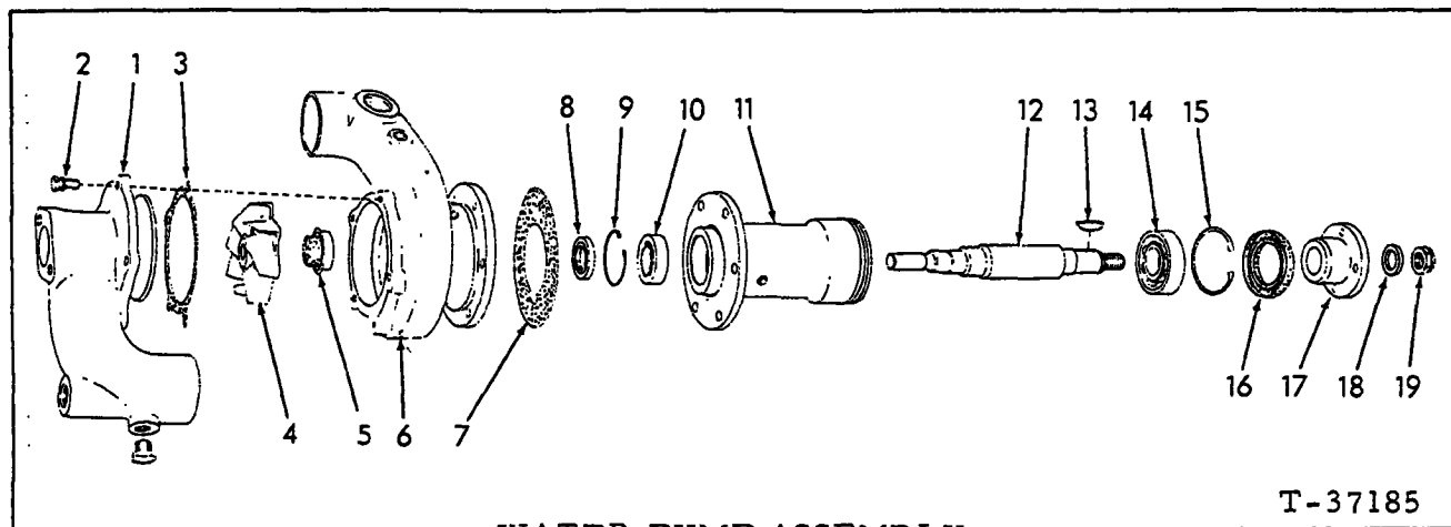
WATER PUMP ASSEMBLY
