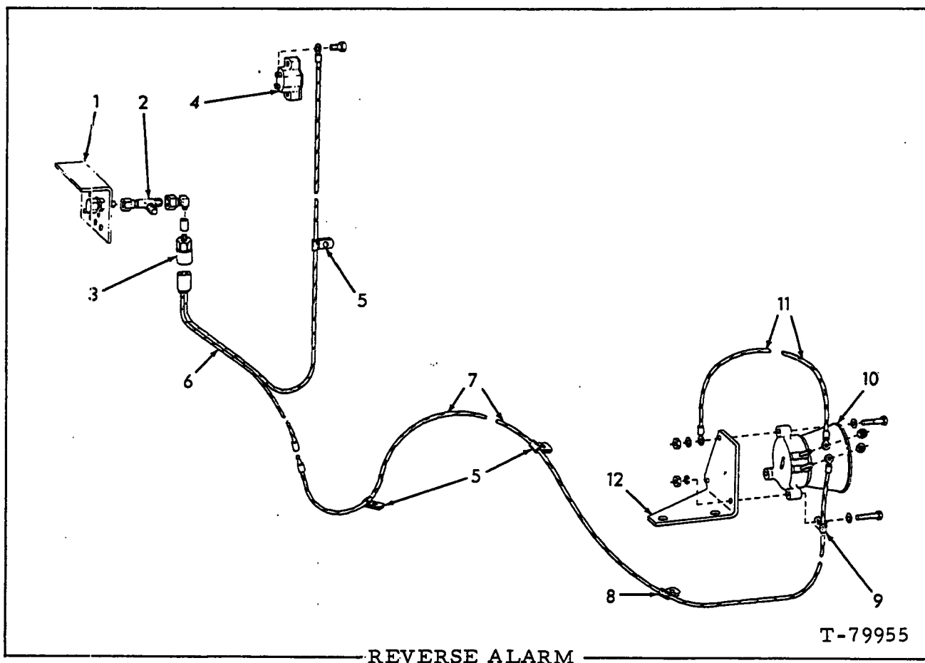
REVERSE ALARM
