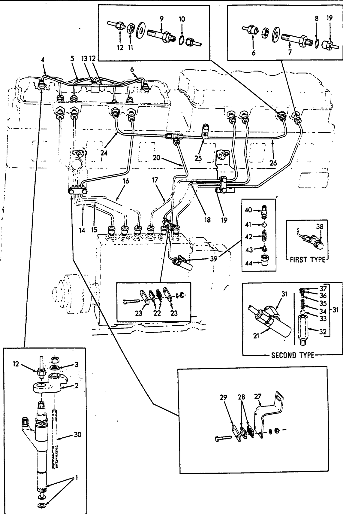
INJECTION NOZZLE LINES
