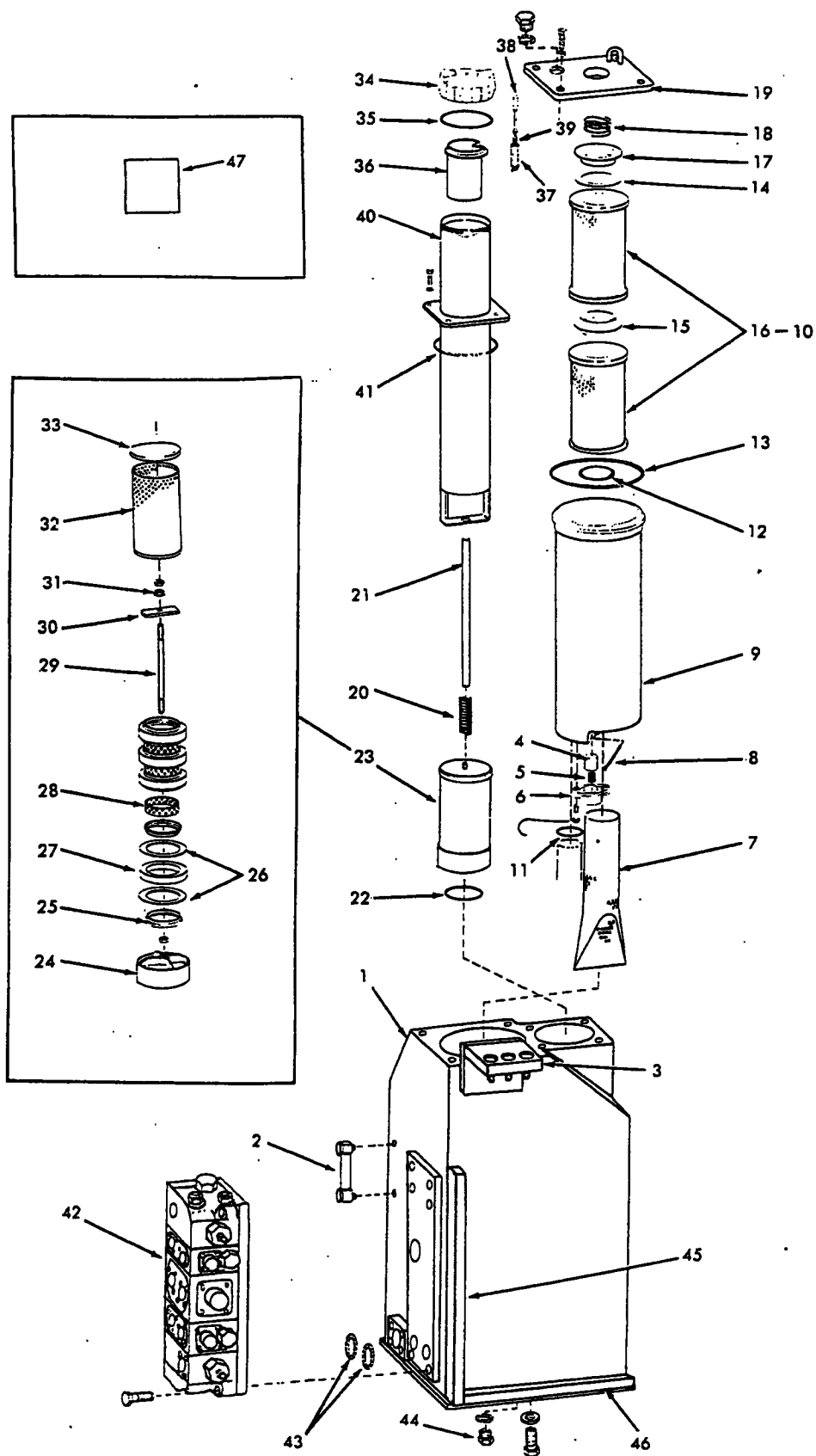
HYDRAULIC TANK
