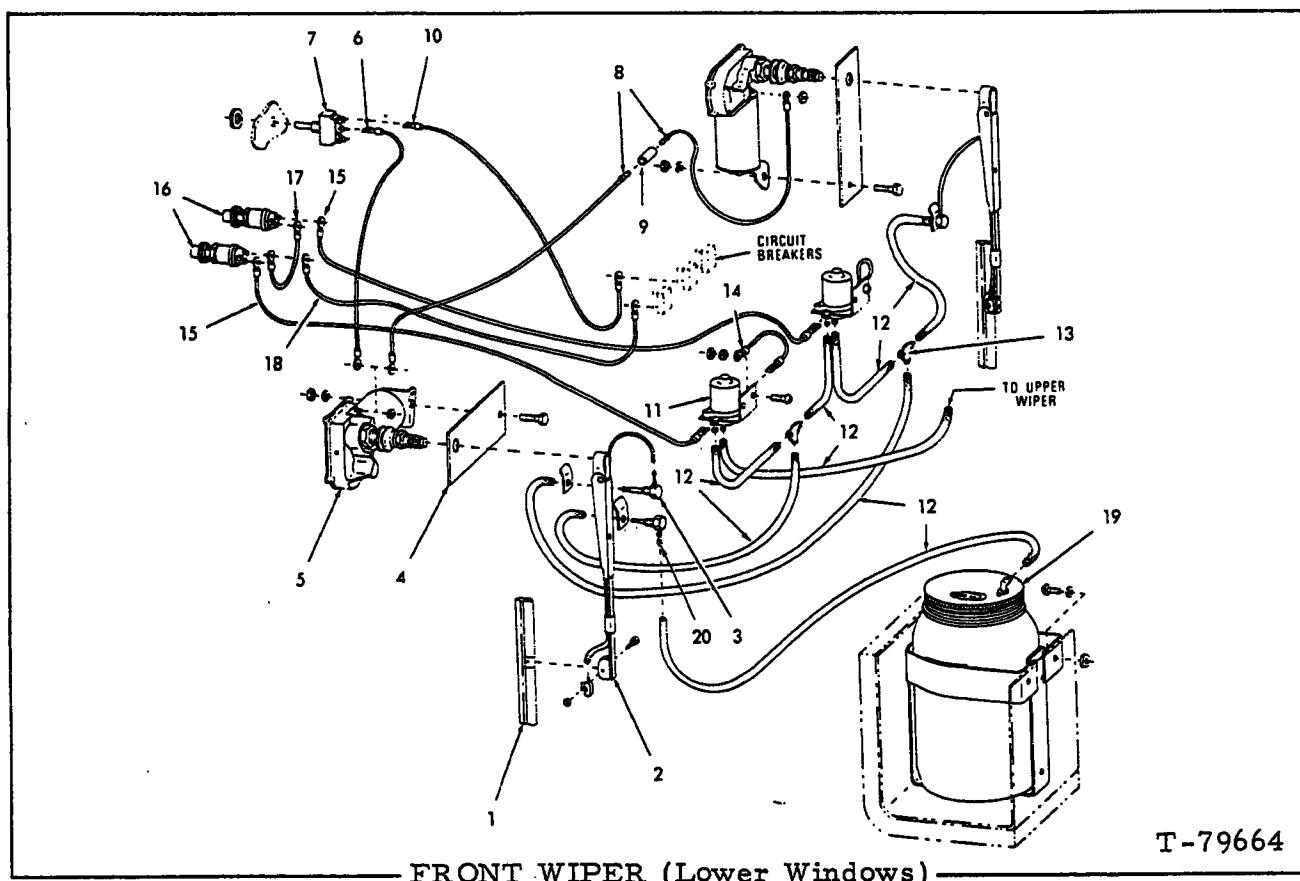
FRONT WIPER (Lower Windows)
