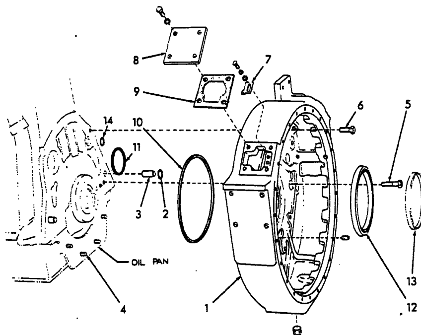
FLYWHEEL HOUSING
