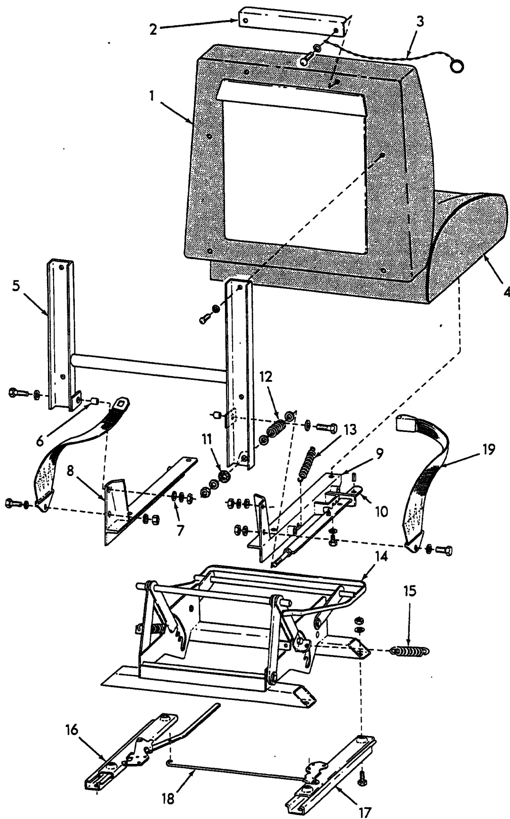
SEAT ASSEMBLY 191B
