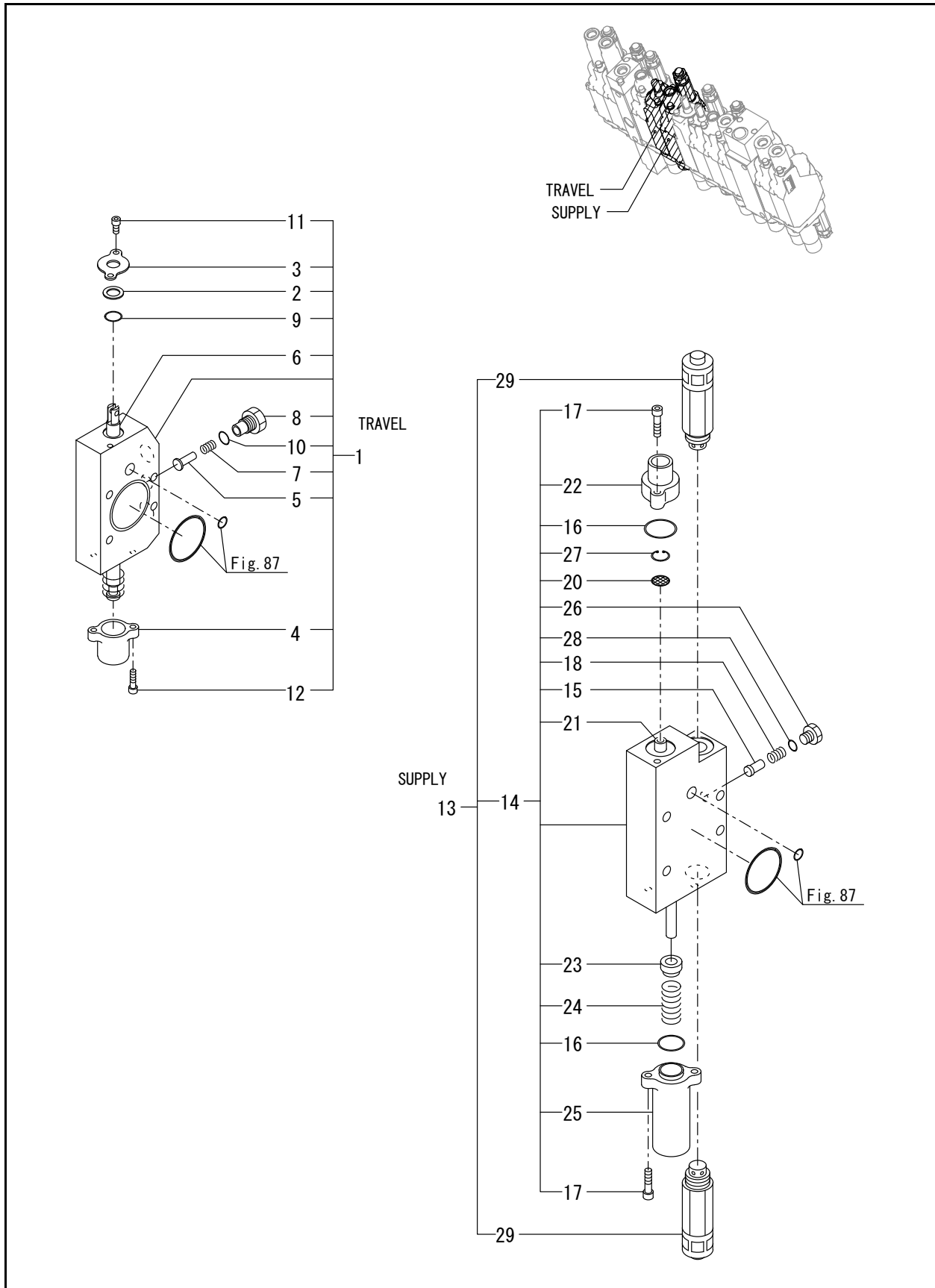
FIG. 89 - CONTROL VALVE (3/7)
