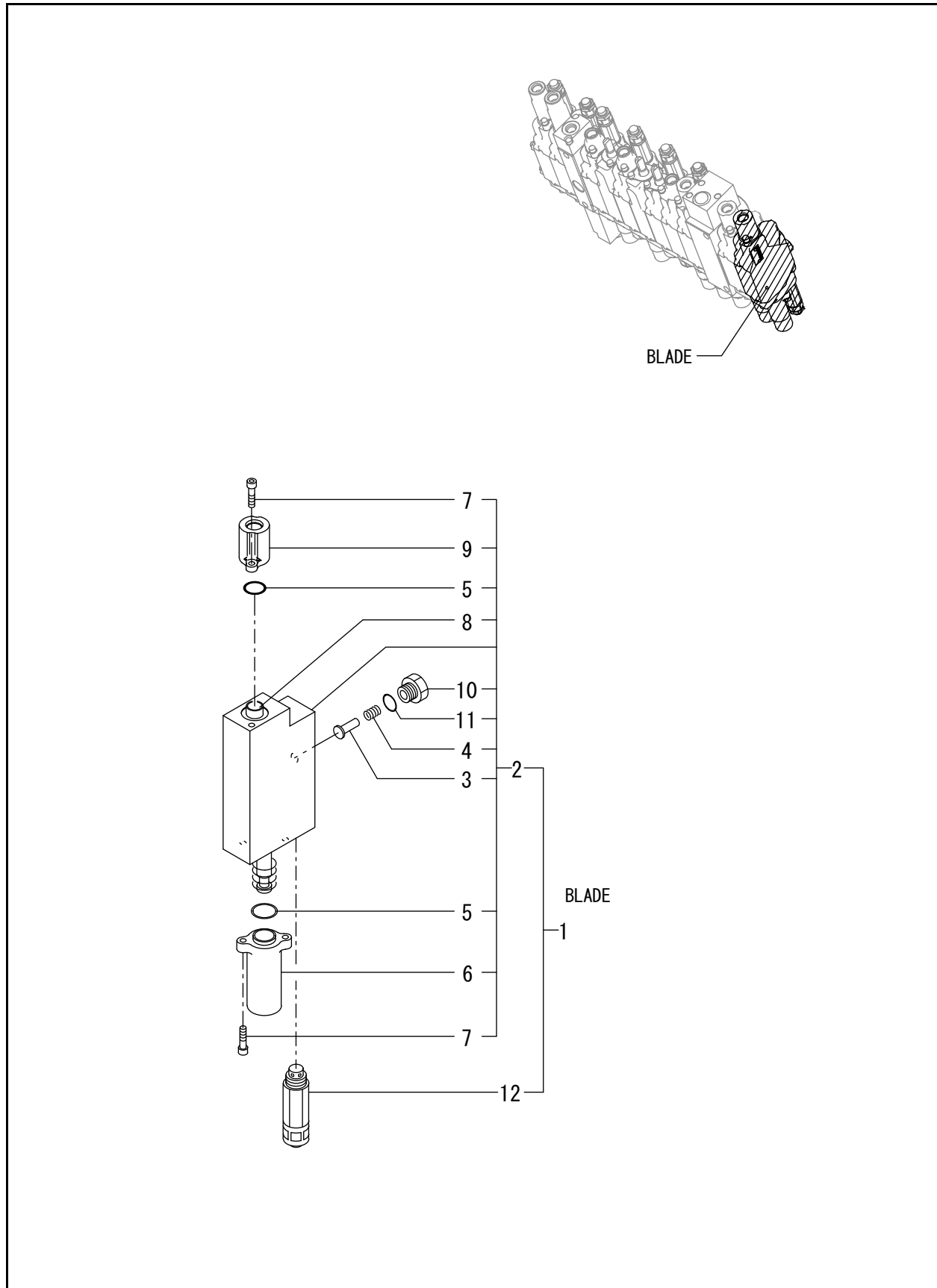
FIG. 93 - CONTROL VALVE (7/7)
