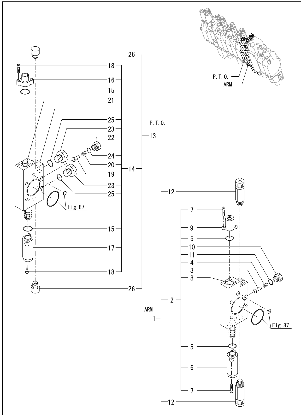
FIG. 91 - CONTROL VALVE (5/7)
