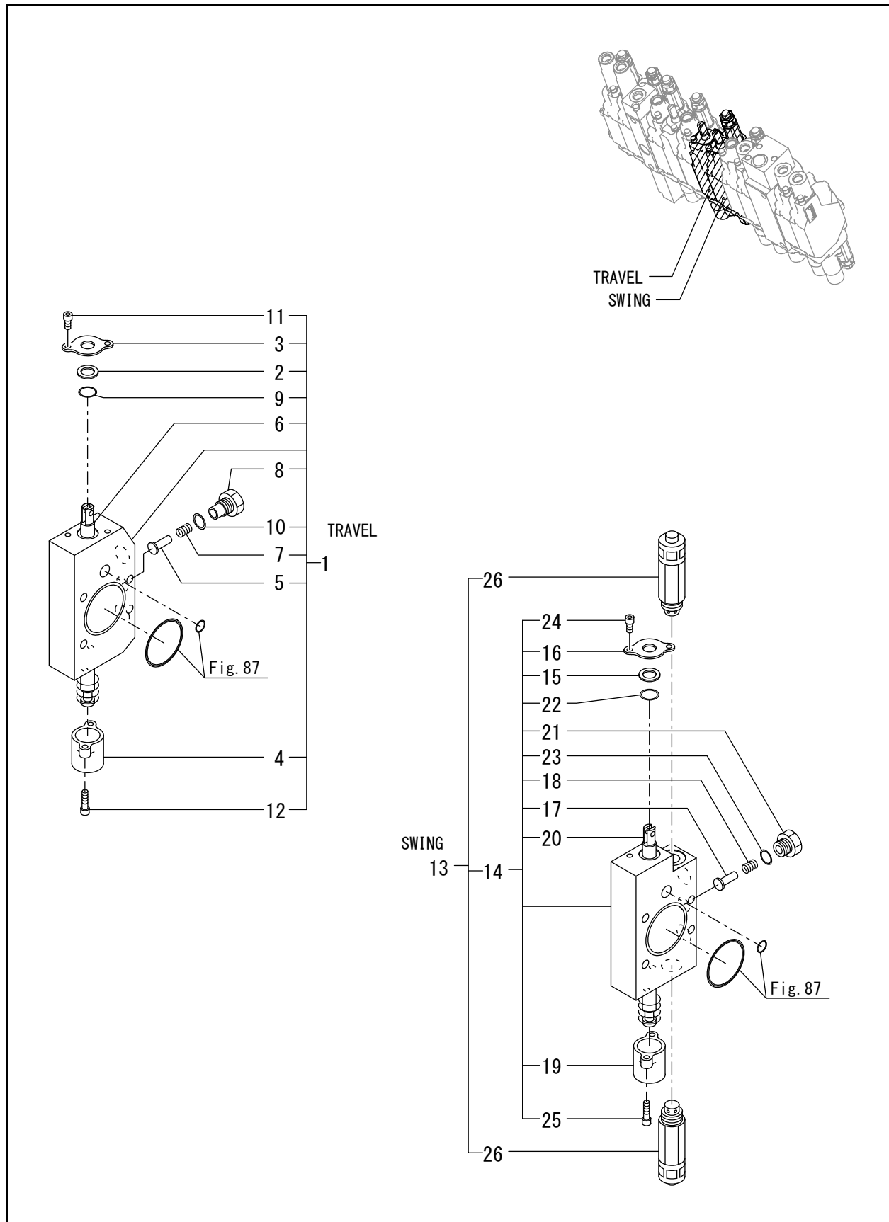
FIG. 90 - CONTROL VALVE (4/7)
