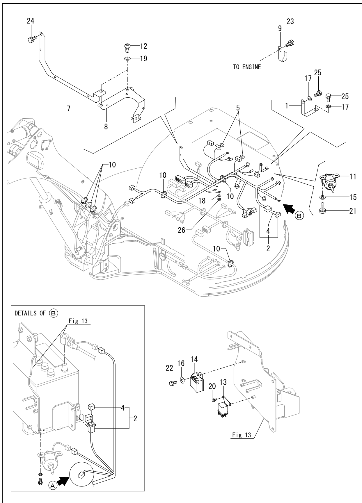
FIG. 14 - ELECTRIC PART (AROUND ENGINE)
