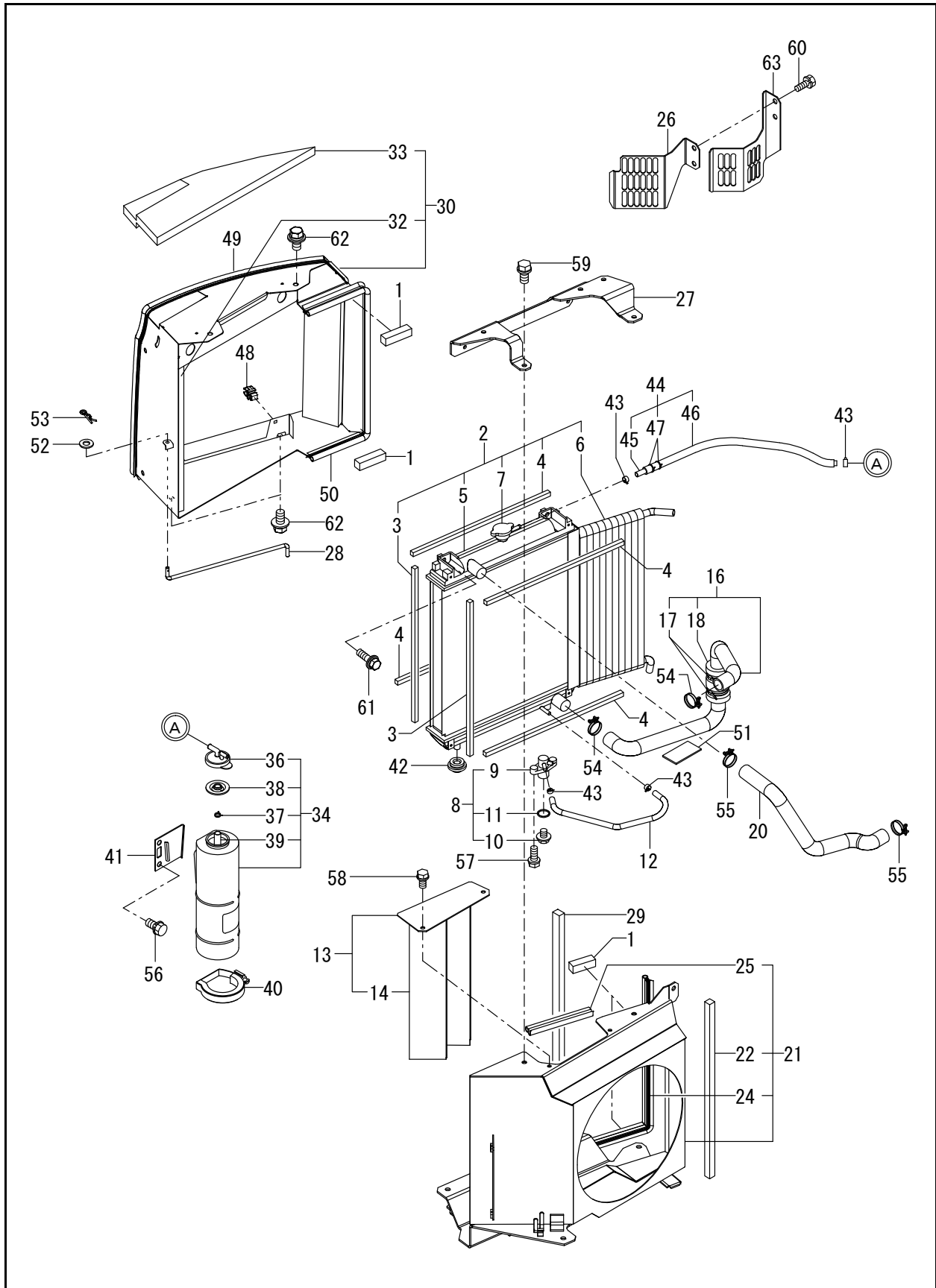
FIG. 10 - RADIATOR & MOUNT
