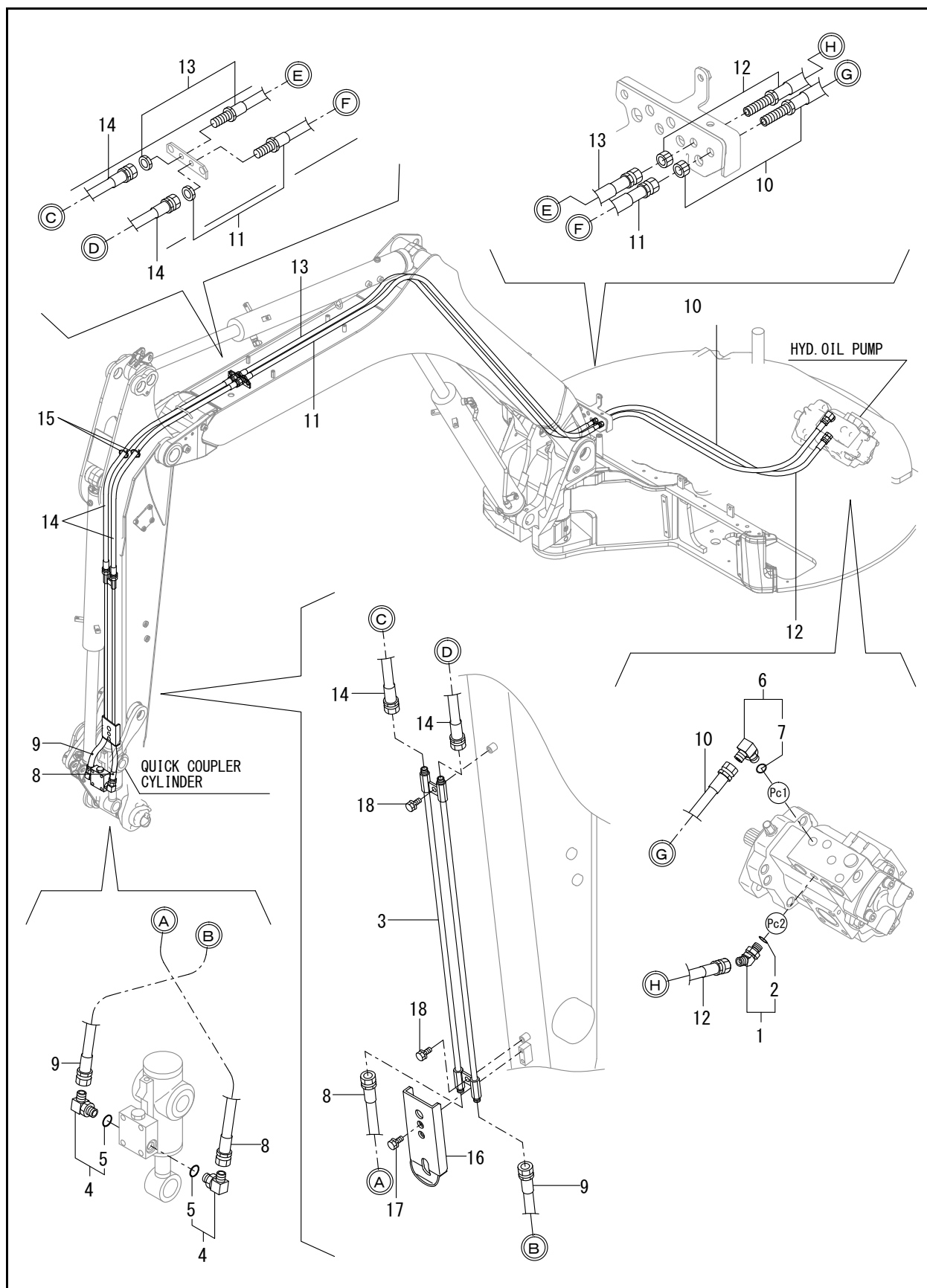
FIG. 110 - HYD. OIL PIPING (QUICK COUPLER)
