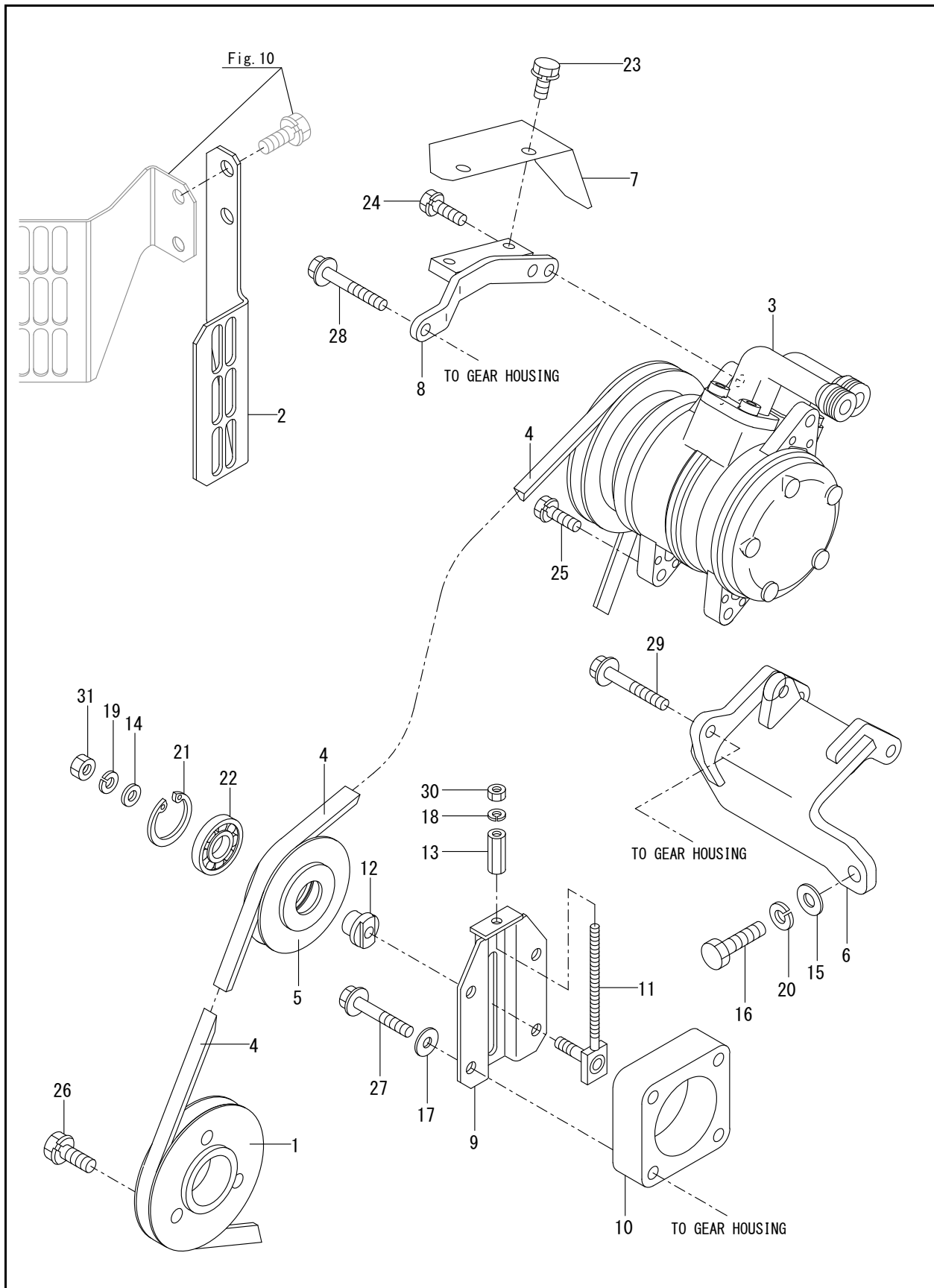
FIG. 26 - AIR CONDITIONER (ENGINE RELATED)
