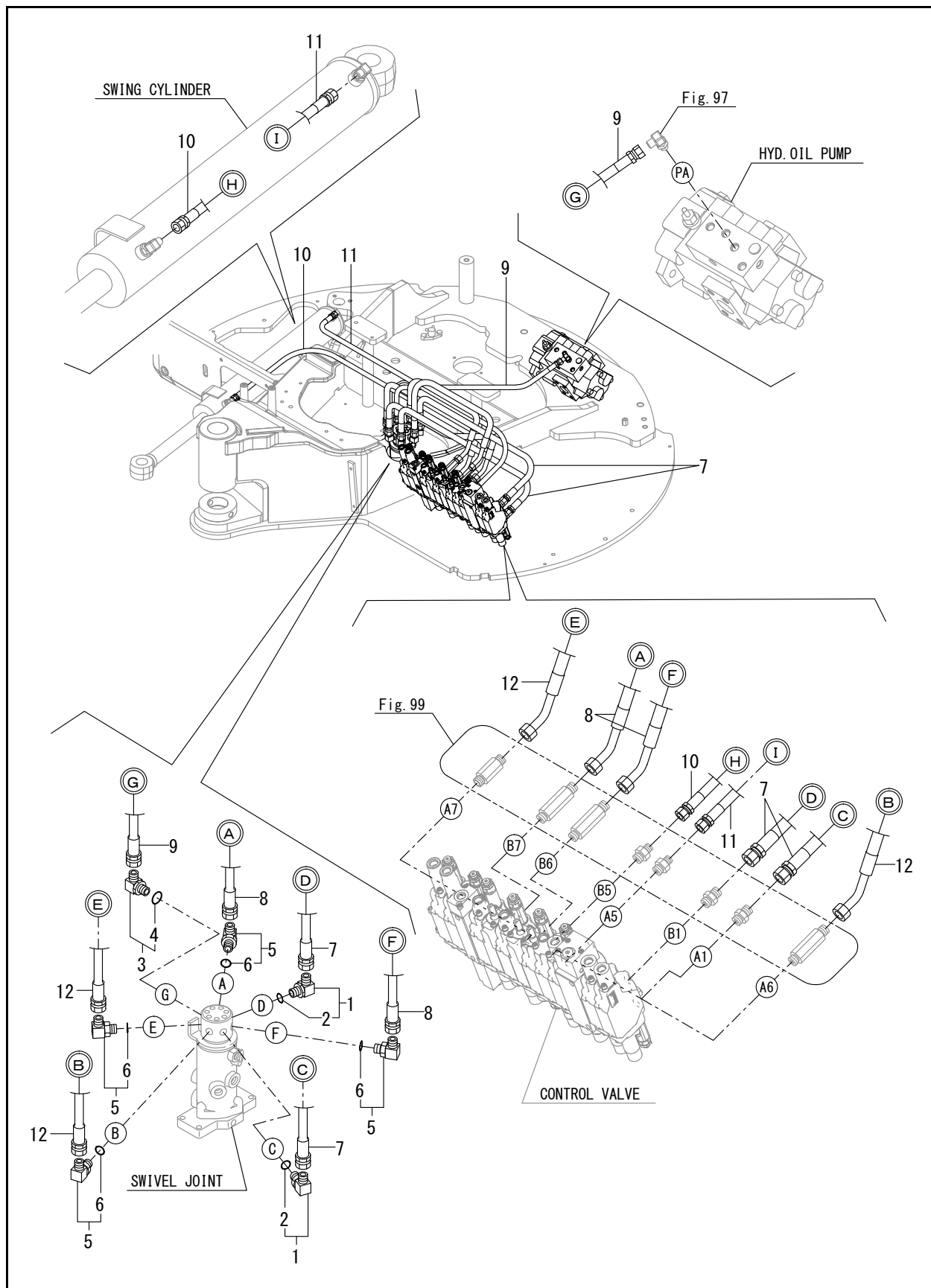
FIG. 102 - HYD. OIL PIPING (VALVE-SWIVEL-SWING CYLINDER)
