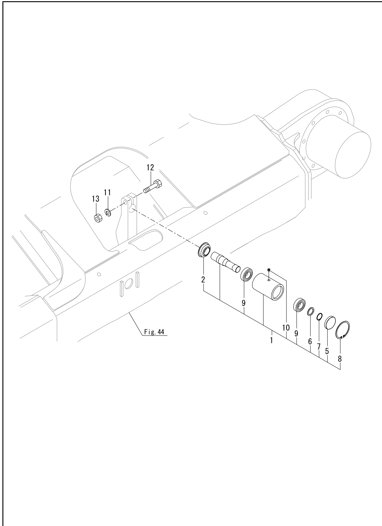
FIG. 33 - CARRIER ROLLER
