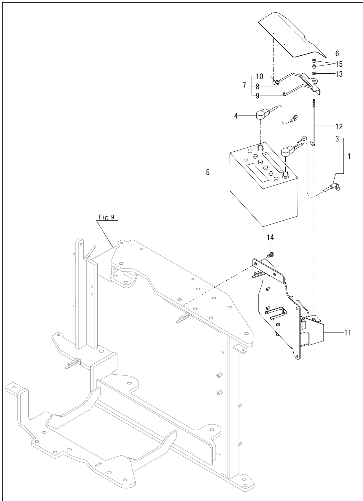
FIG. 13 - BATTERY
