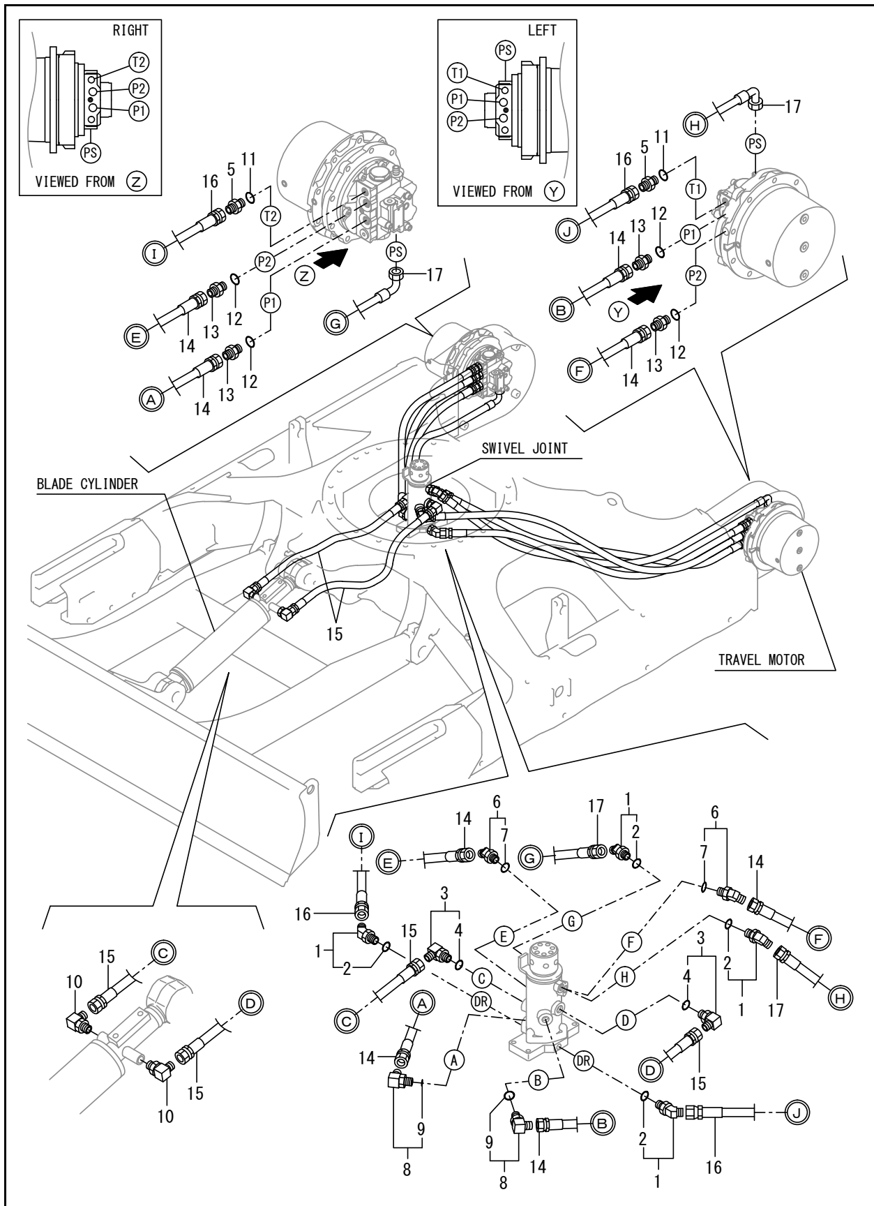
FIG. 106 - HYD. OIL PIPING (TRUCK FRAME)
