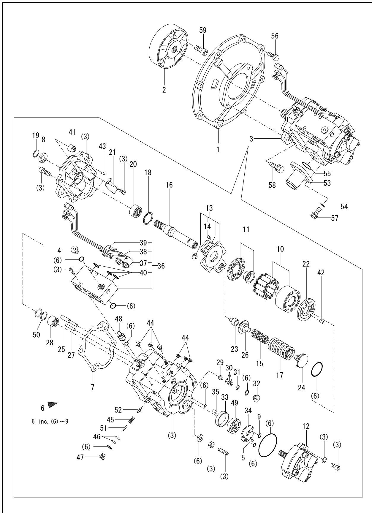
FIG. 77 - HYD. OIL PUMP & JOINT
