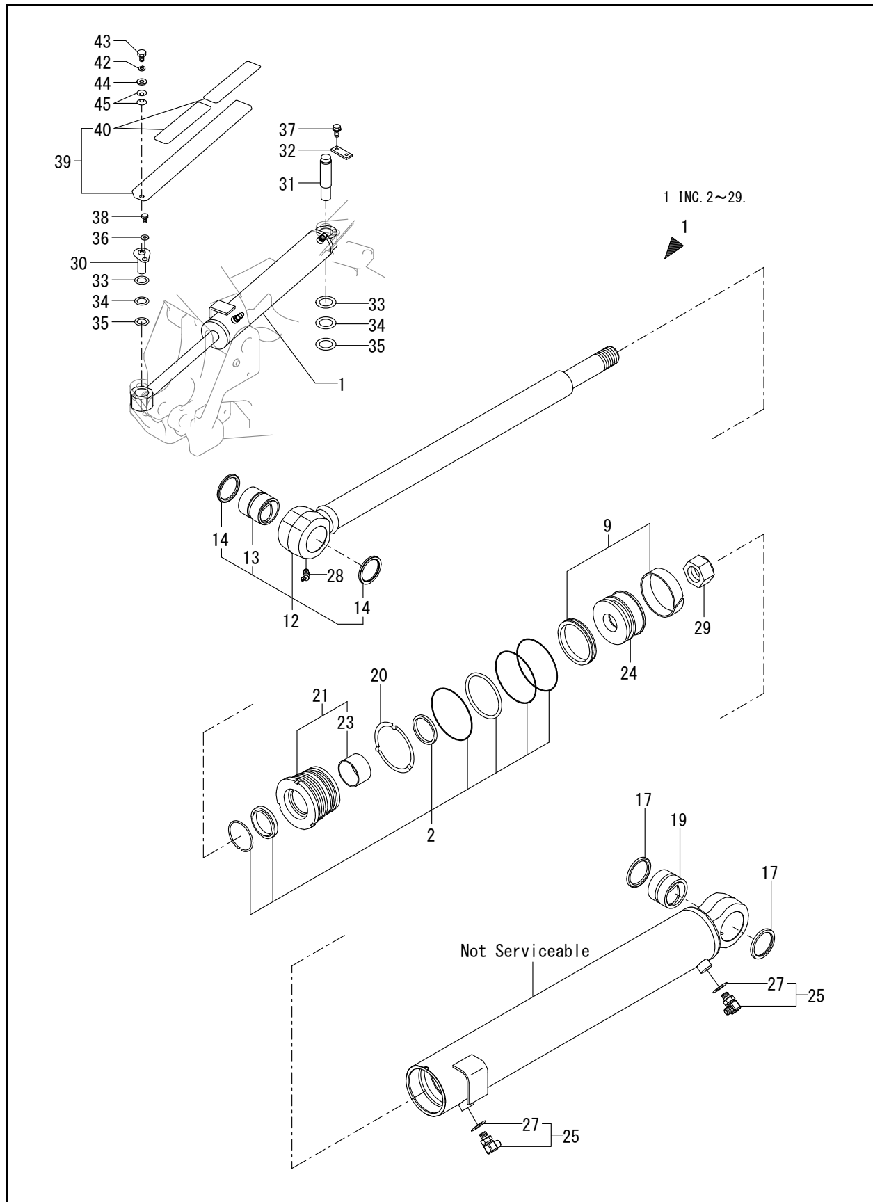
FIG. 81 - SWING CYLINDER
