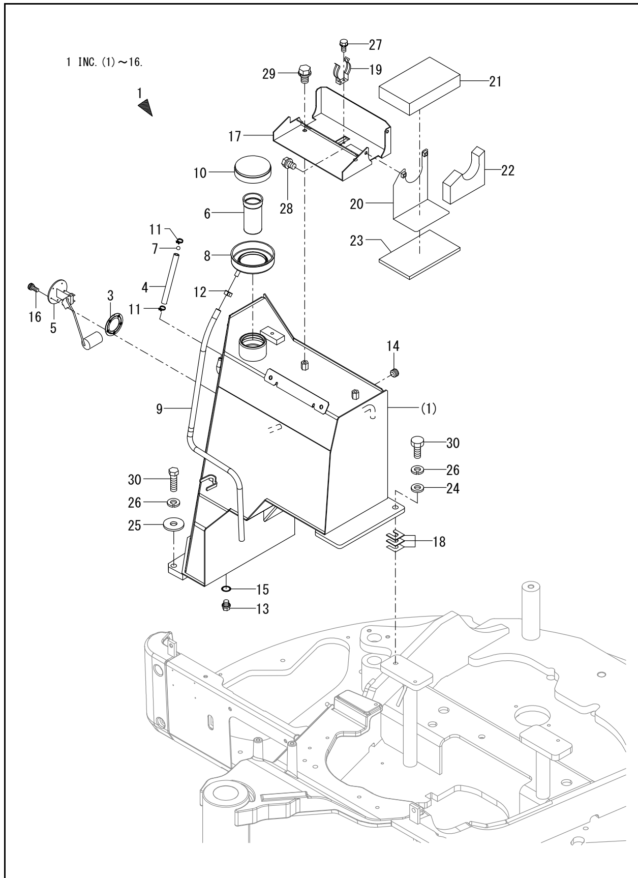
FIG. 11 - FUEL TANK
