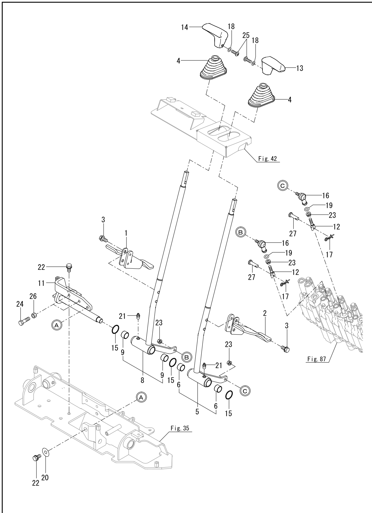
FIG. 36 - CONTROL EQUIPMENT (TRAVEL LEVER)
