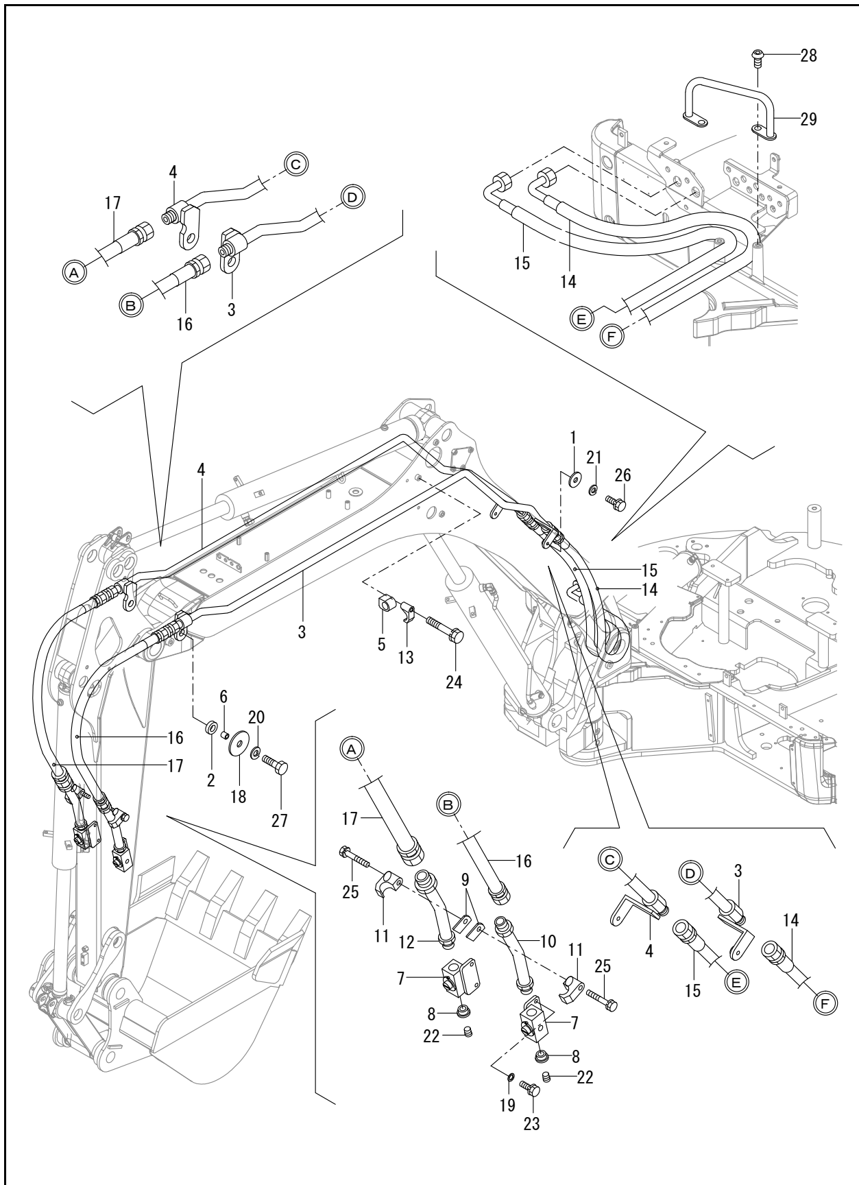
FIG. 108 - HYD. OIL PIPING (P.T.O. : BOOM-ARM)
