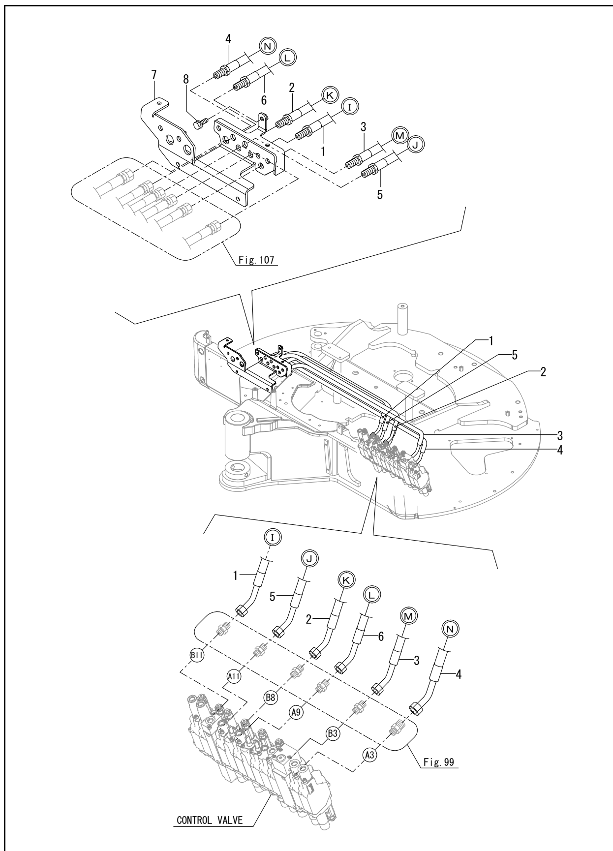
FIG. 105 - HYD. OIL PIPING (CONTROL VALVE-FRAME END)
