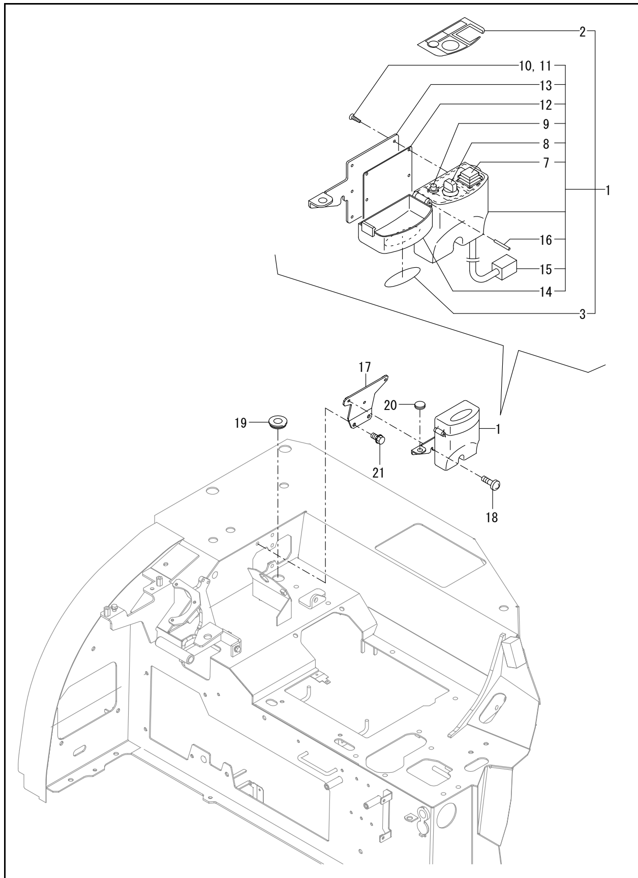
FIG. 18 - ELECTRIC PART (QUICK COUPLER : SWITCH BOX)
