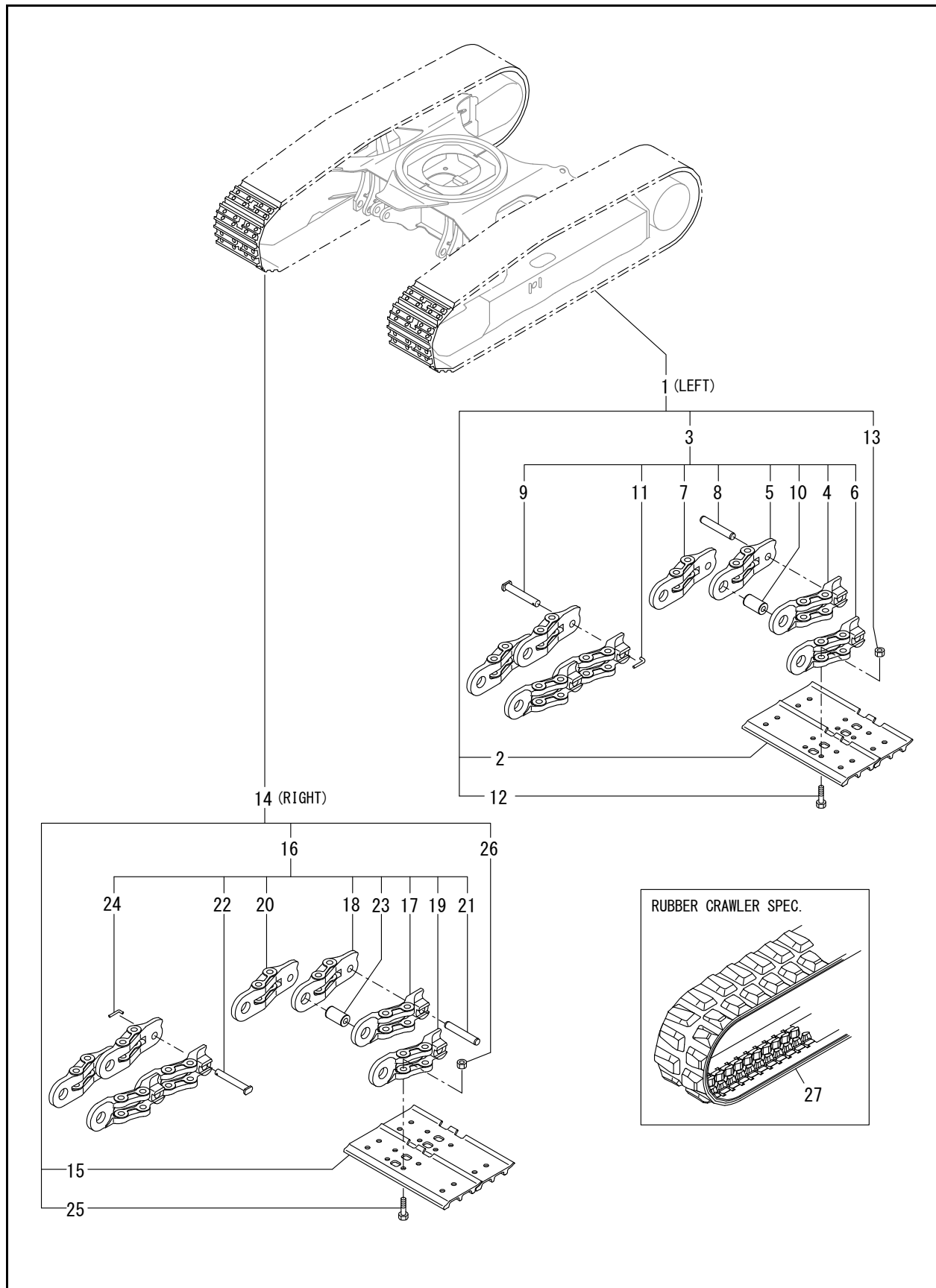
FIG. 34 - CRAWLER
