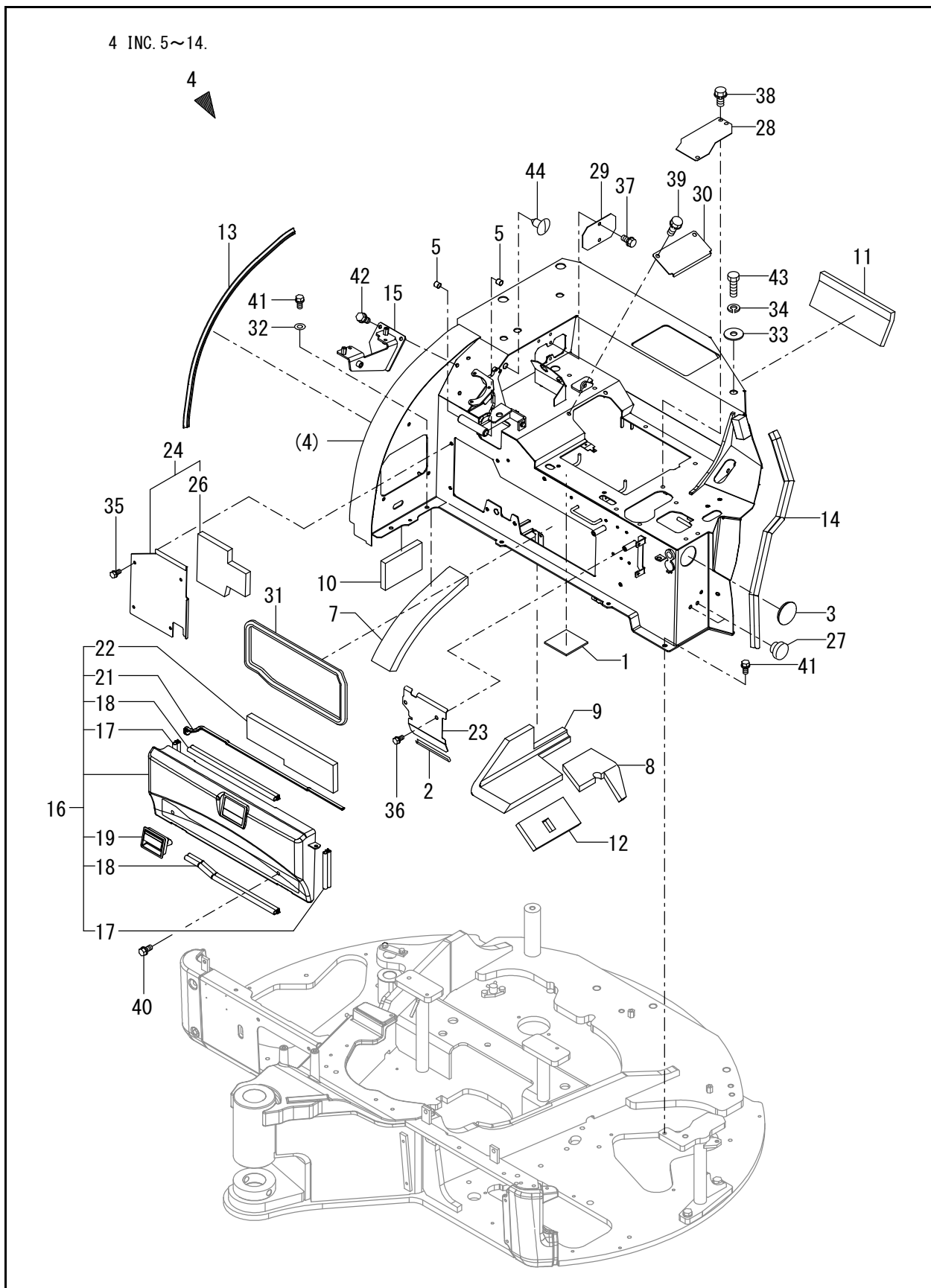
FIG. 56 - SEAT MOUNT
