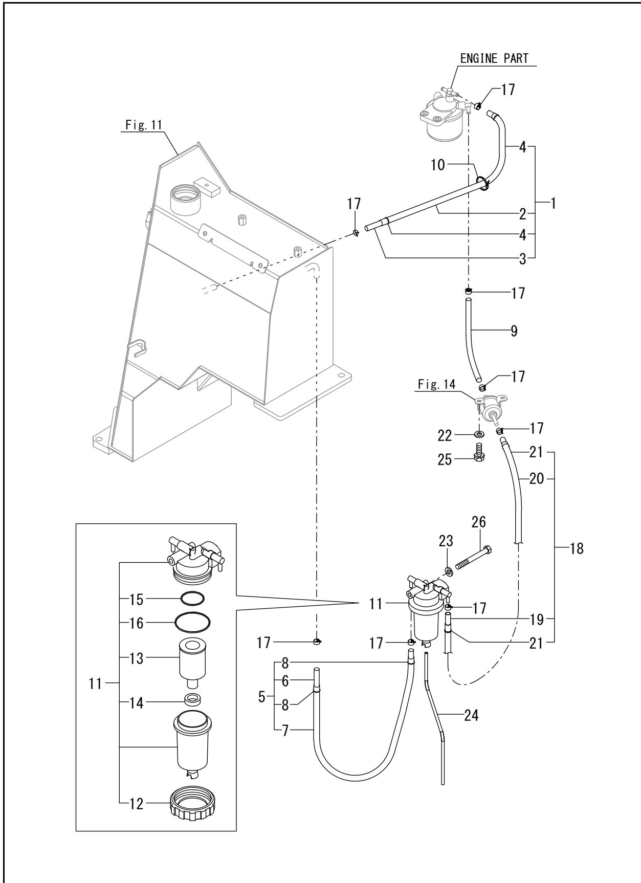
FIG. 12 - FUEL LINE
