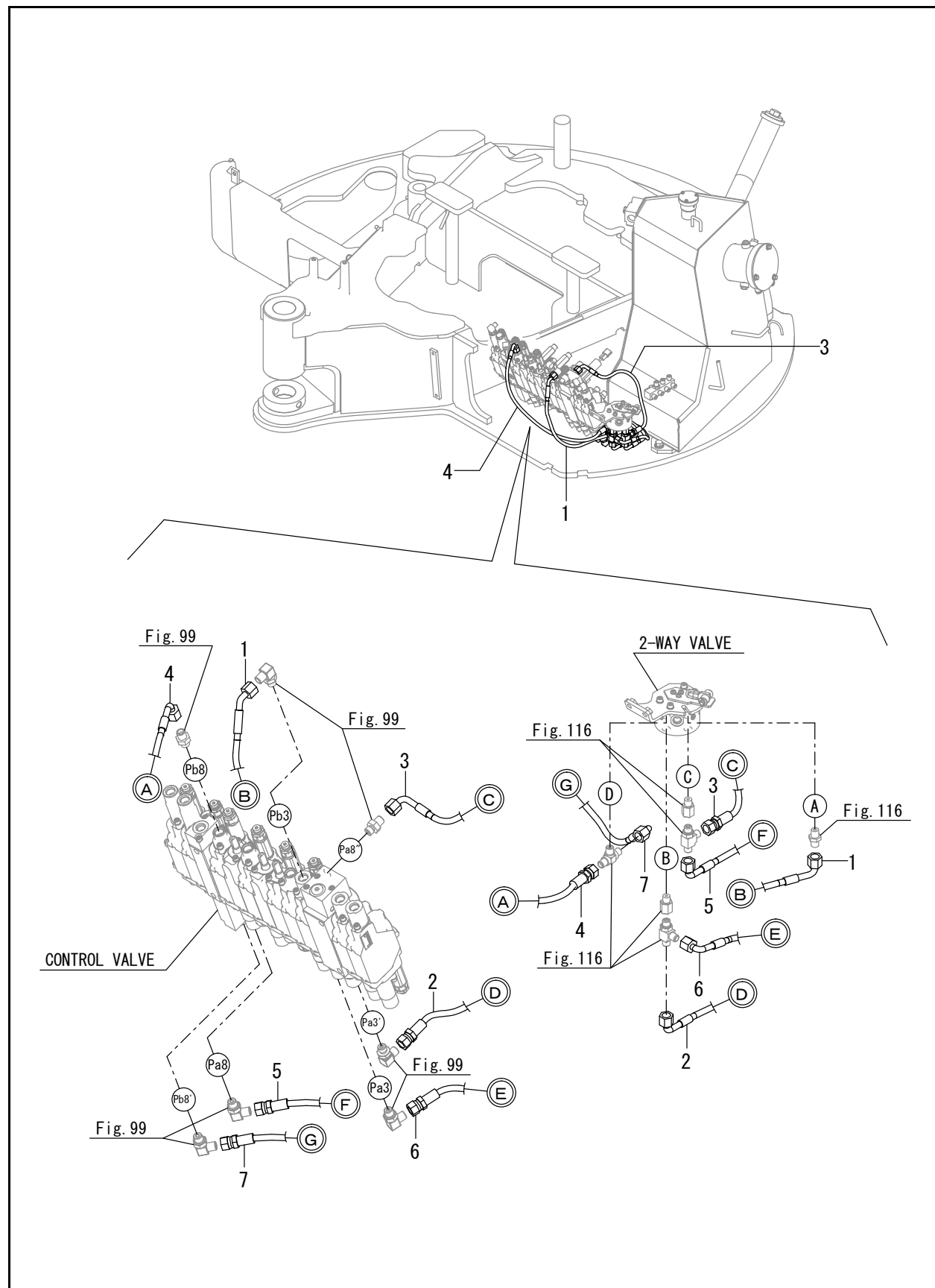
FIG. 114 - CONTROL PIPING (2-WAY VALVE : 2)
