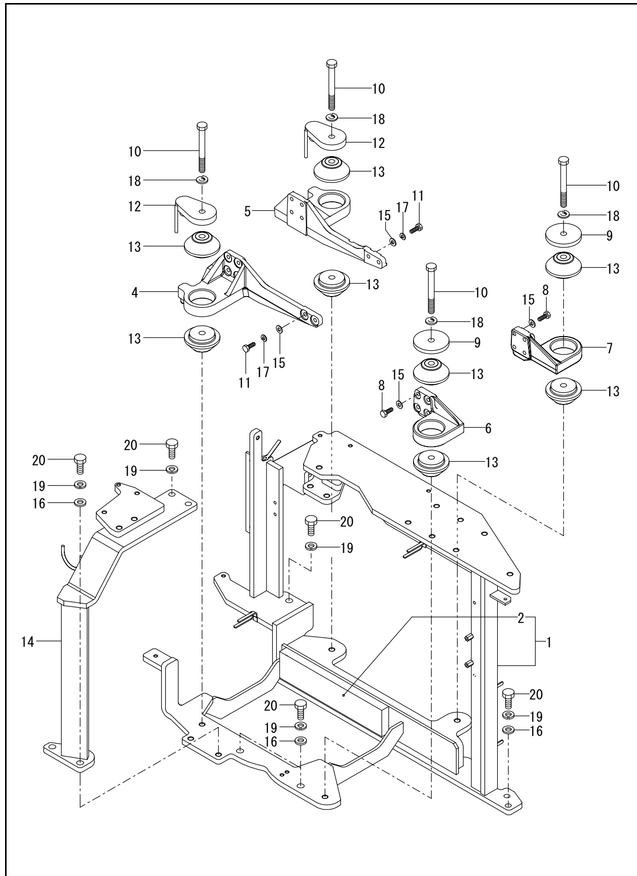
FIG. 9 - ENGINE MOUNT
