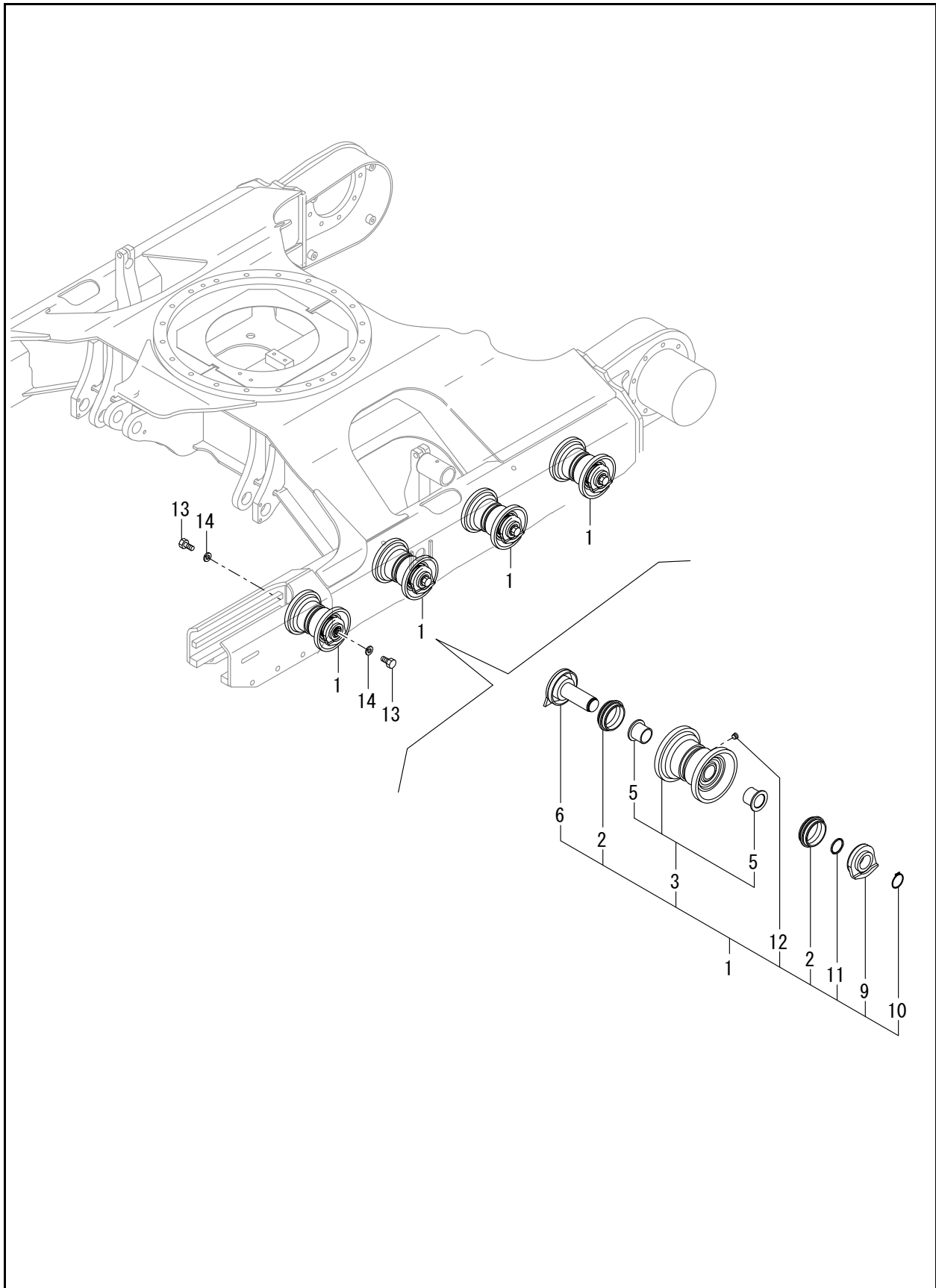
FIG. 32 - TRACK ROLLER
