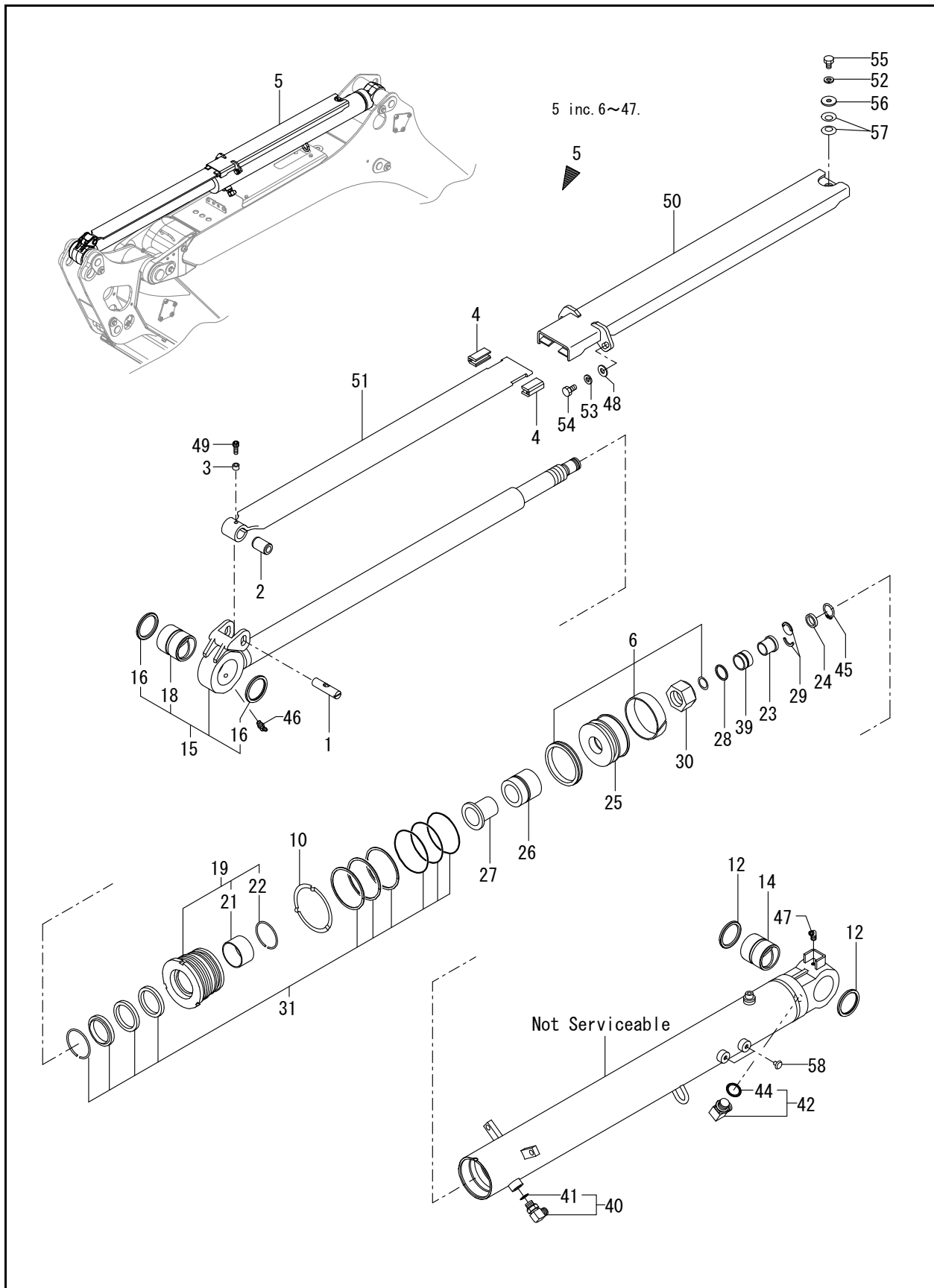
FIG. 79 - ARM CYLINDER
