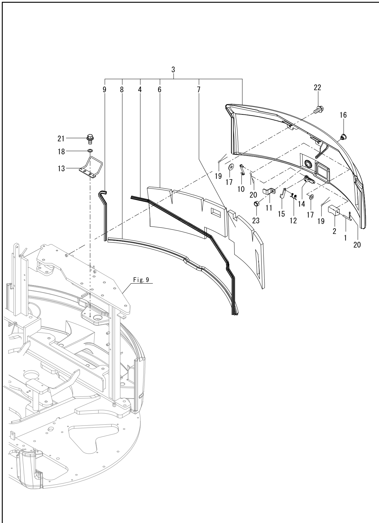
FIG. 59 - BONNET (REAR)
