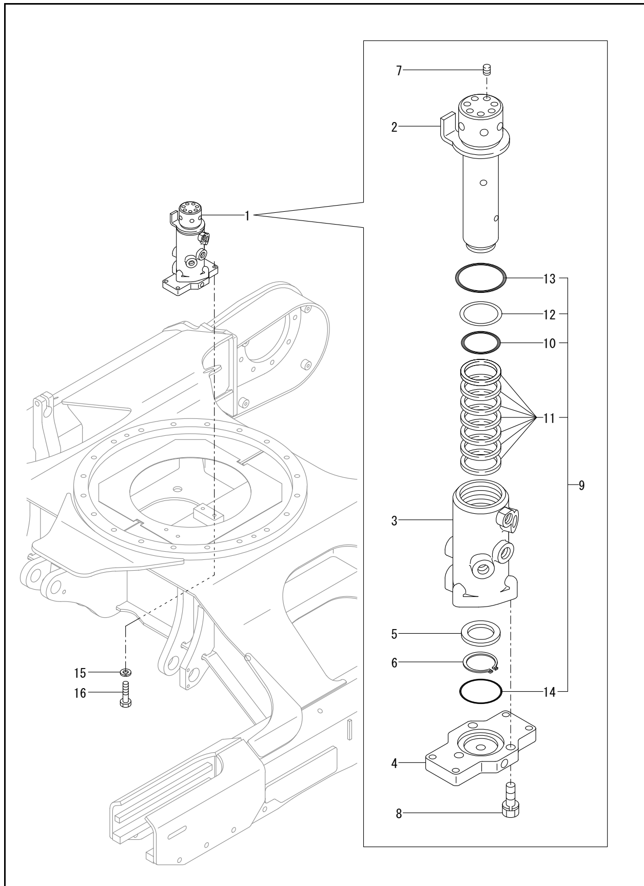
FIG. 86 - SWIVEL JOINT
