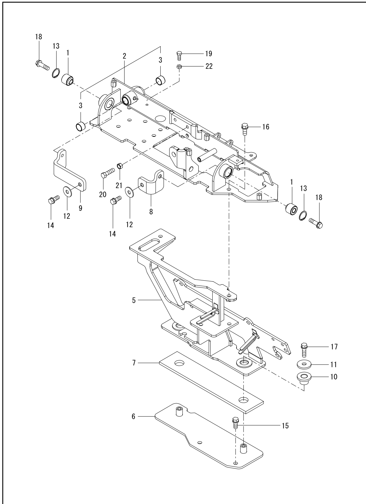
FIG. 35 - VALVE PLATE
