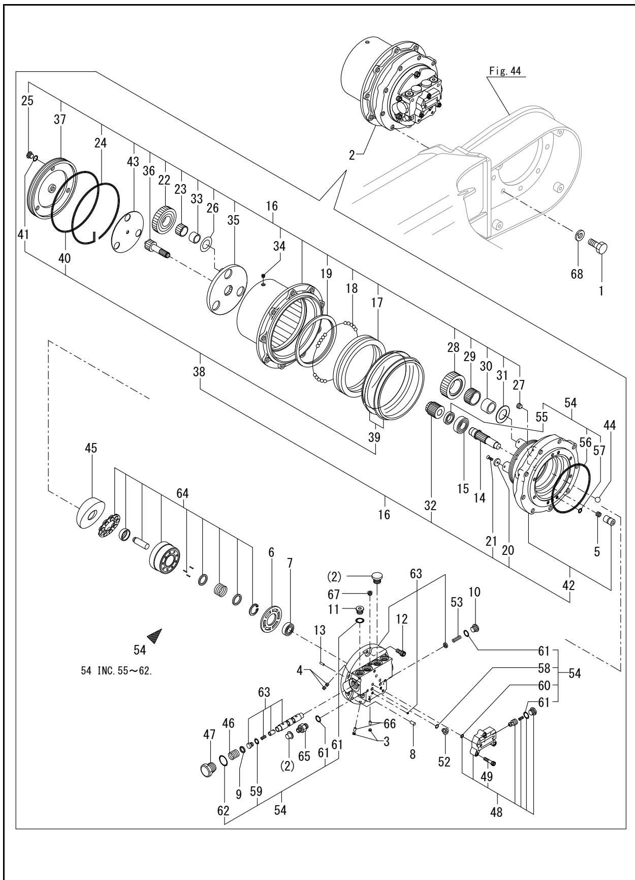
FIG. 84 - TRAVEL MOTOR
