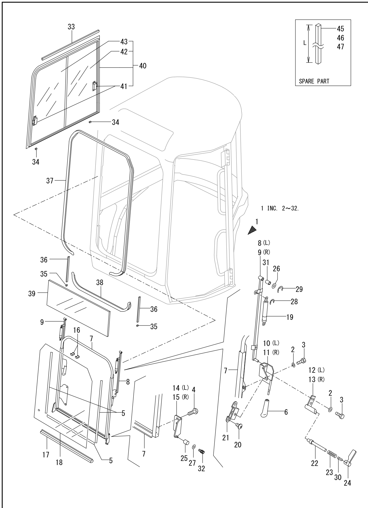
FIG. 69 - CABIN (GLASS)
