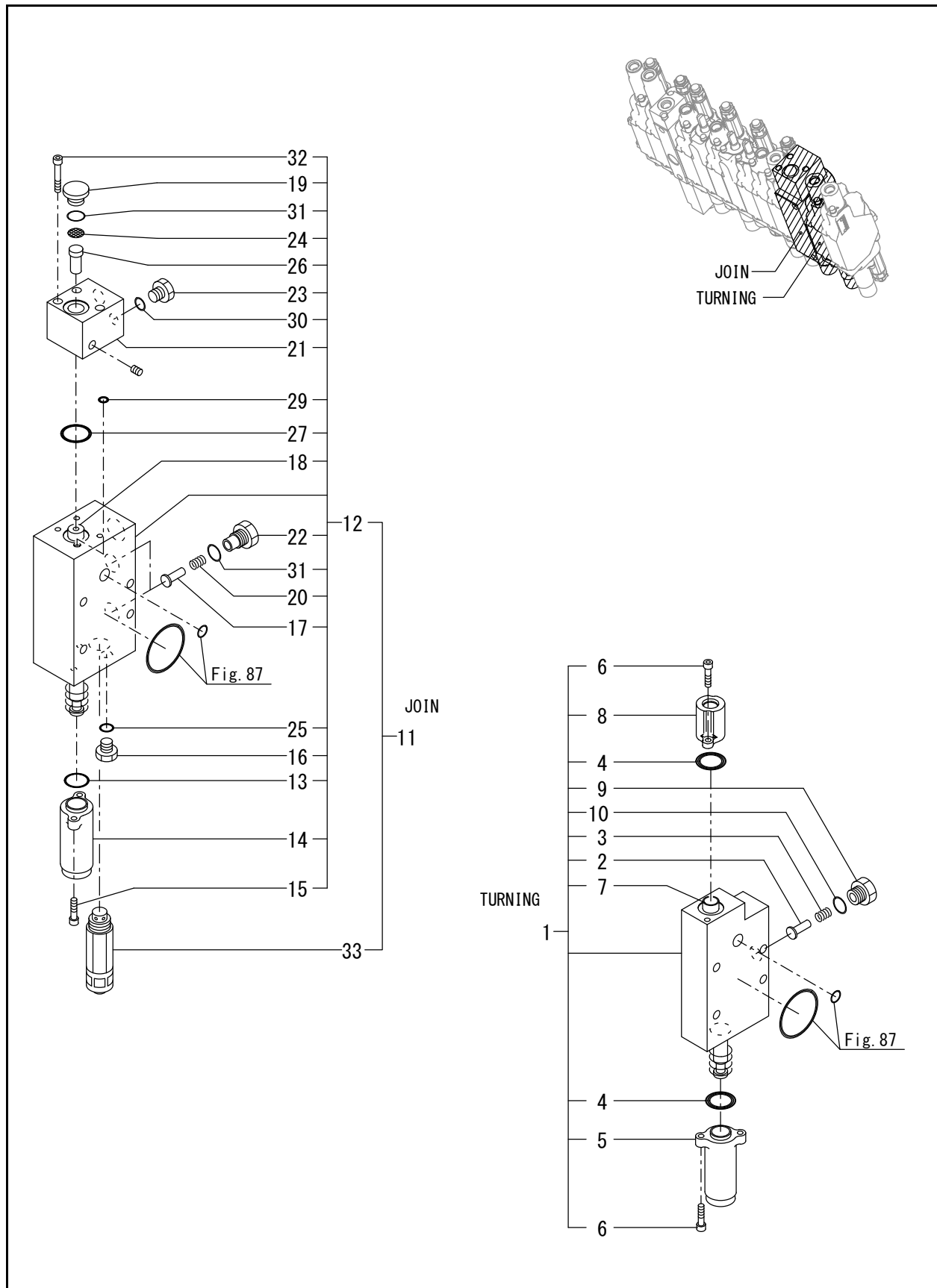
FIG. 92 - CONTROL VALVE (6/7)
