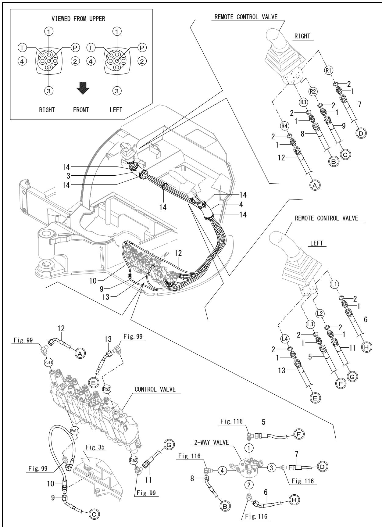
FIG. 113 - CONTROL PIPING (2-WAY VALVE : 1)
