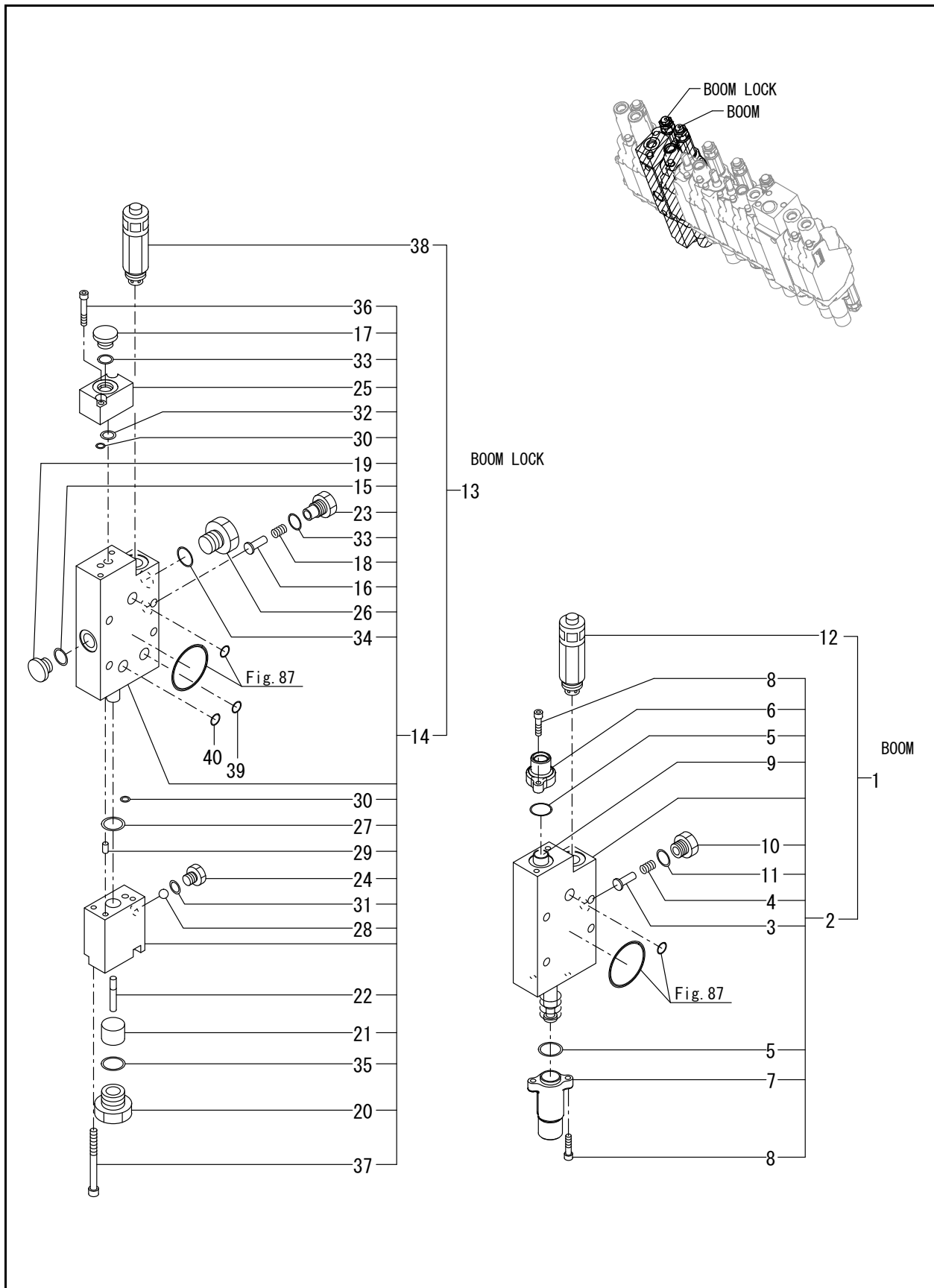
FIG. 88 - CONTROL VALVE (2/7)
