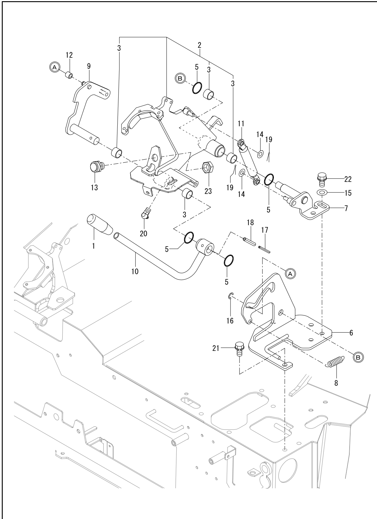
FIG. 39 - CONTROL EQUIPMENT (LOCK LEVER & STAND : LEFT)
