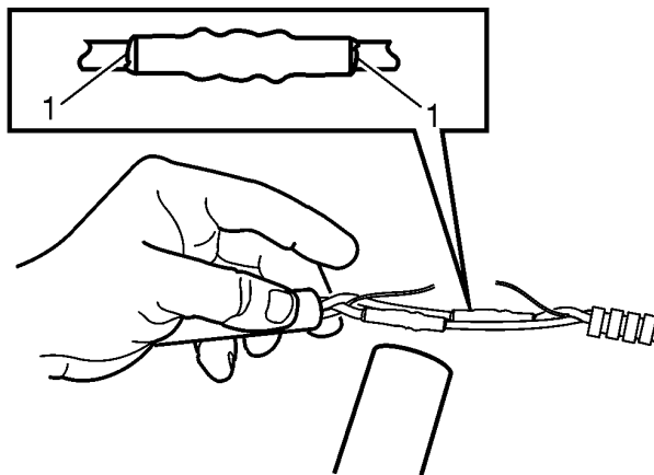
1 Visible sealant
