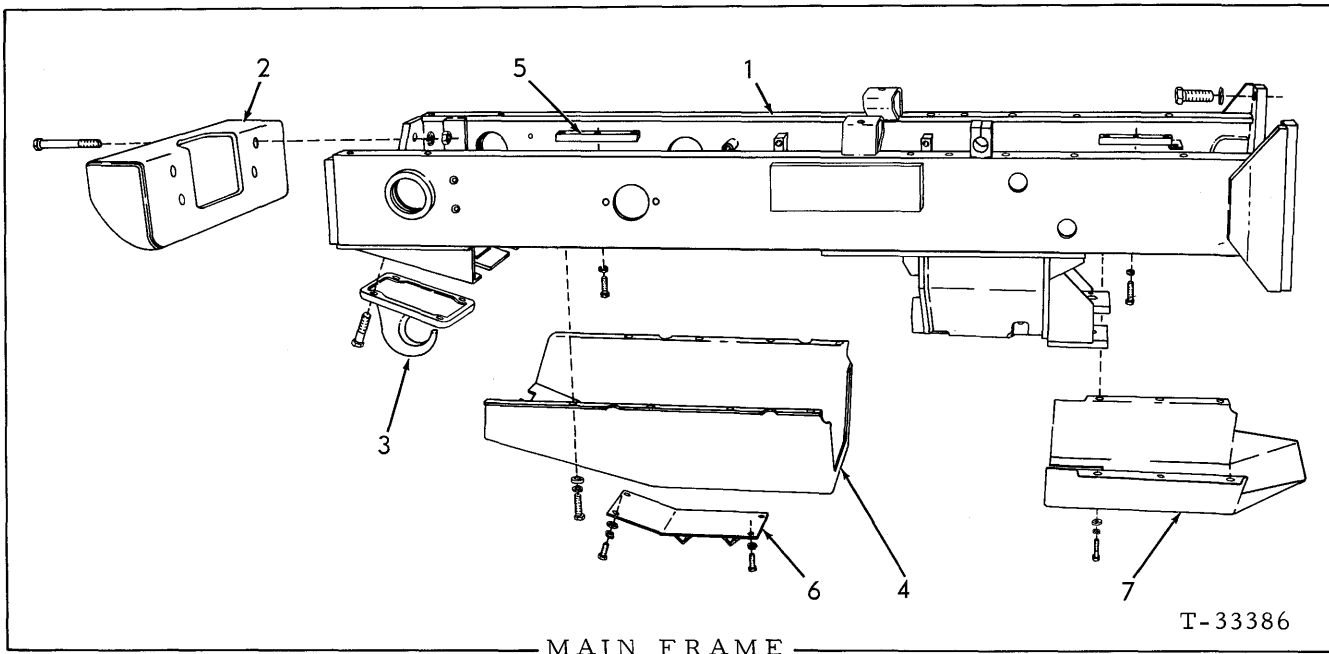
MAIN FRAME
