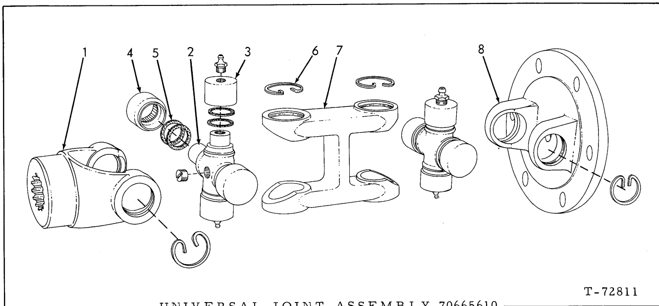
UNIVERSAL JOINT ASSEMBLY 70665610
