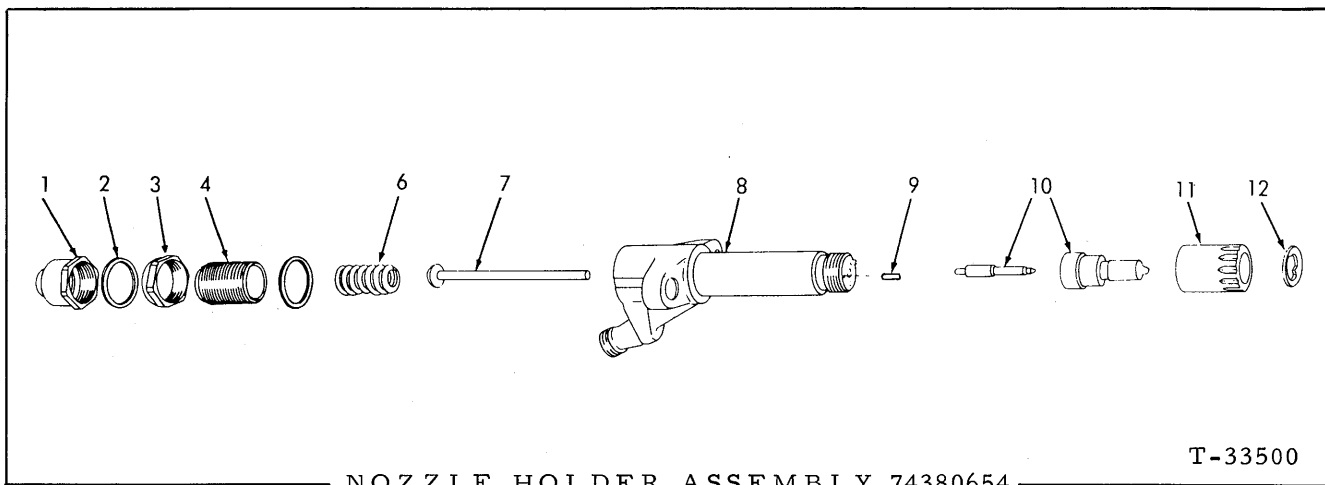
NOZZLE HOLDER ASSEMBLY 74380654
