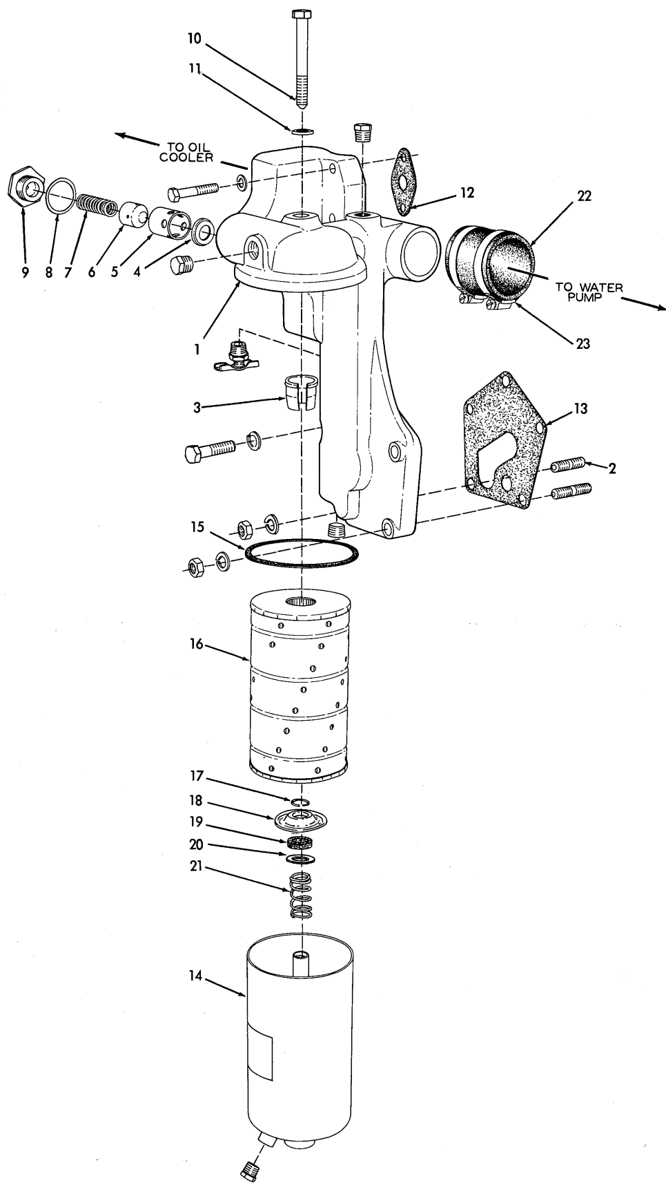
OIL FILTER
