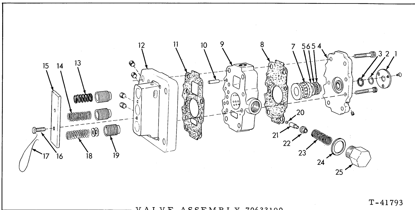
VALVE ASSEMBLY 70633190
