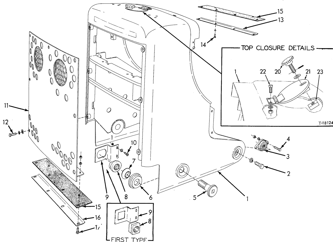
WRAP-AROUND RADIATOR GUARD
