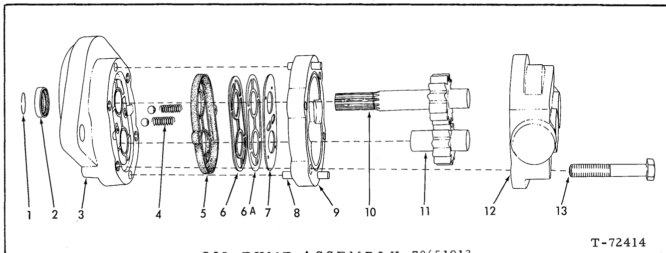
OIL PUMP ASSEMBLY 70651913
