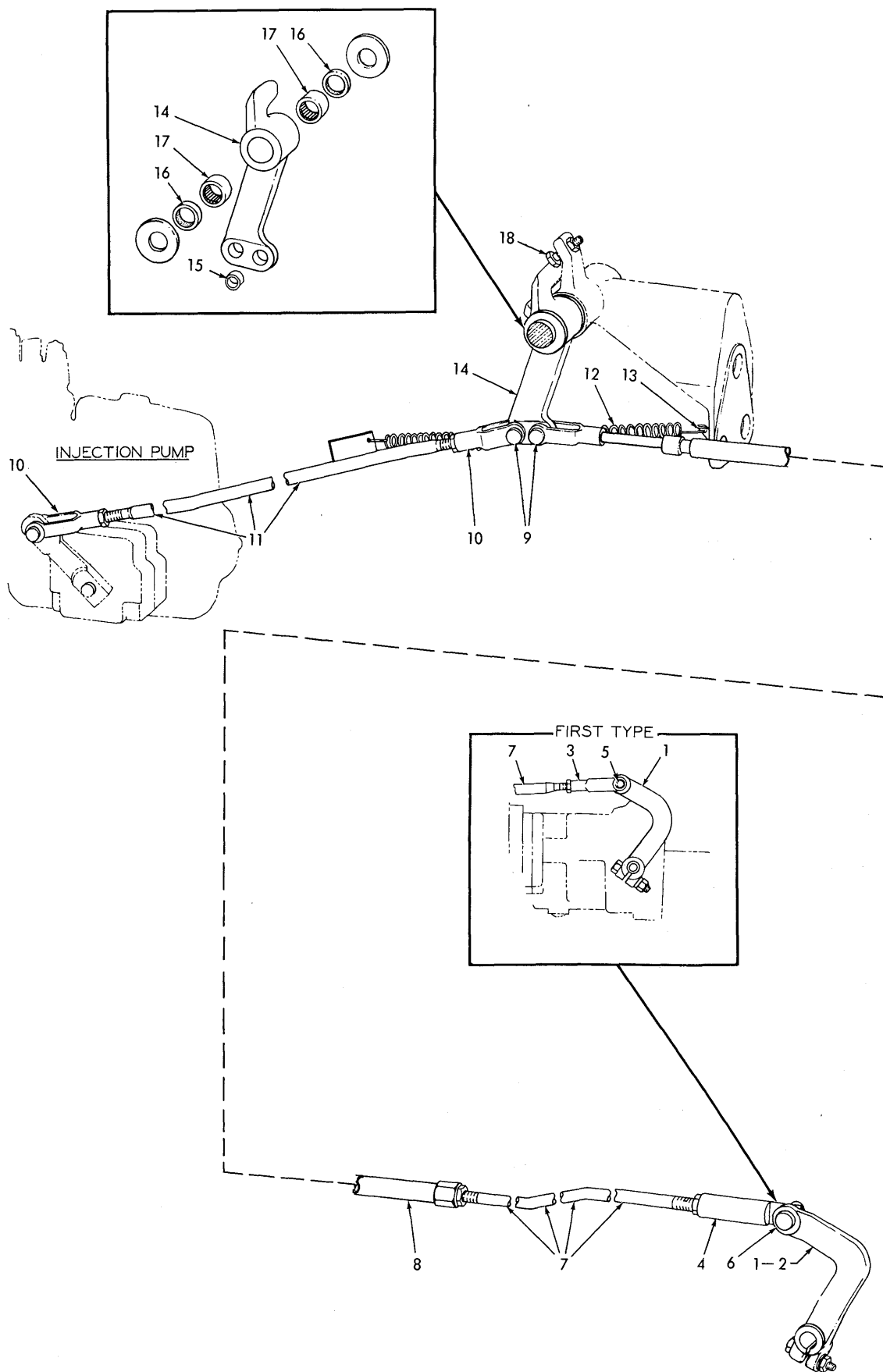
GOVERNOR LINKAGE
