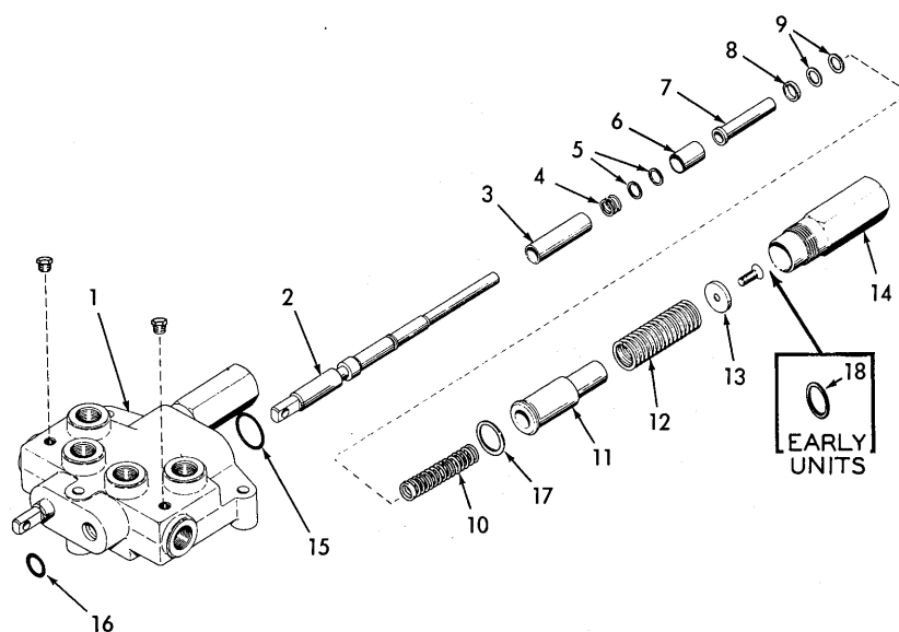
CONTROL VALVE ASSEMBLY 70651432 ("Cessna")
