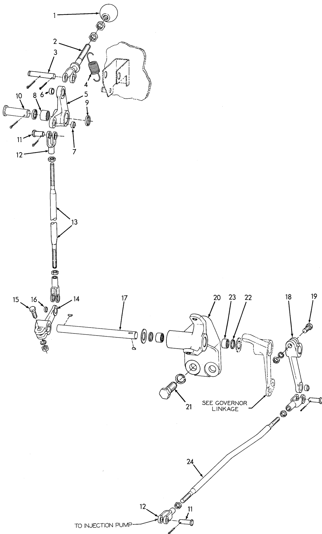
ENGINE SHUT-OFF CONTROL
