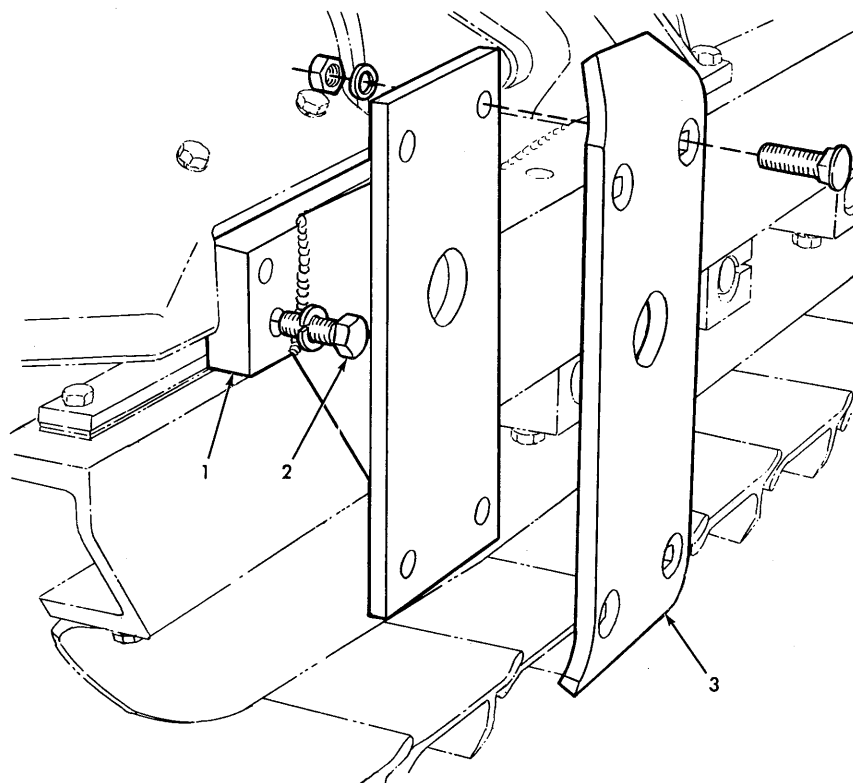
GUIDE BRACKETS
