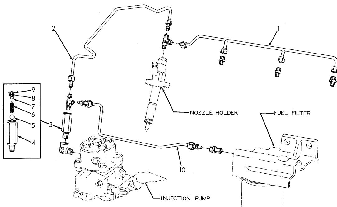
INJECTION FUEL RETURN LINES
