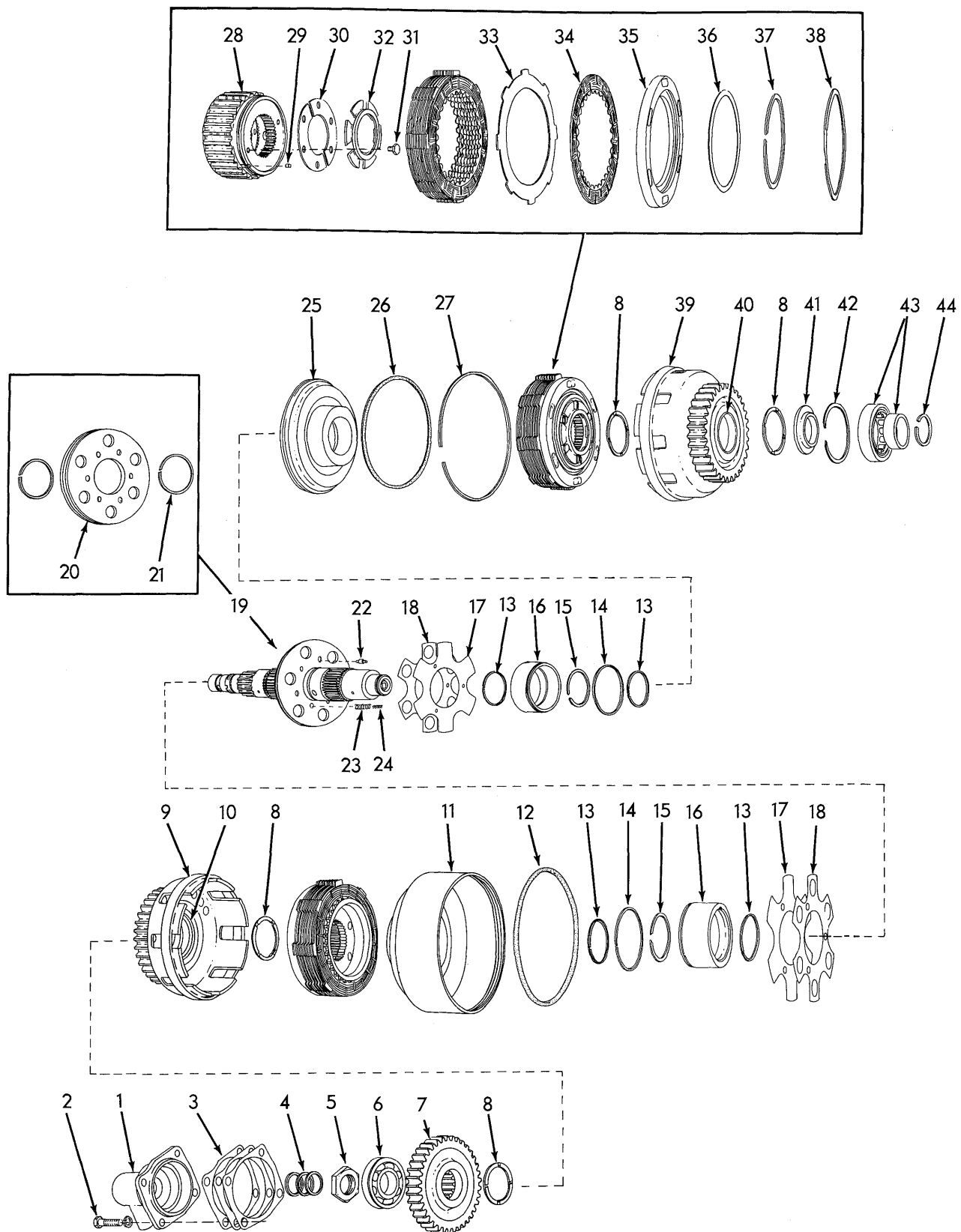
TRANSMISSION BOTTOM SHAFT
