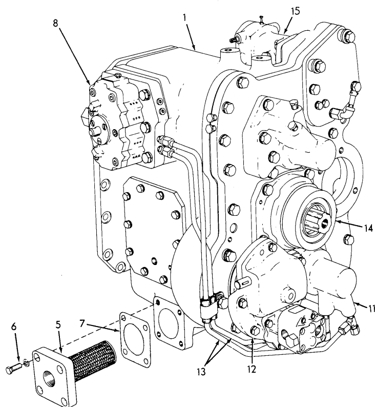
RIGHT FRONT VIEW
