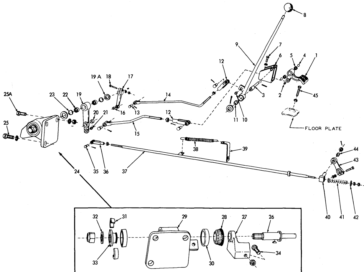
THROTTLE CONTROL (Second type)
