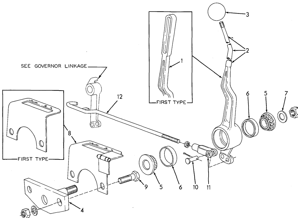
HAND THROTTLE
