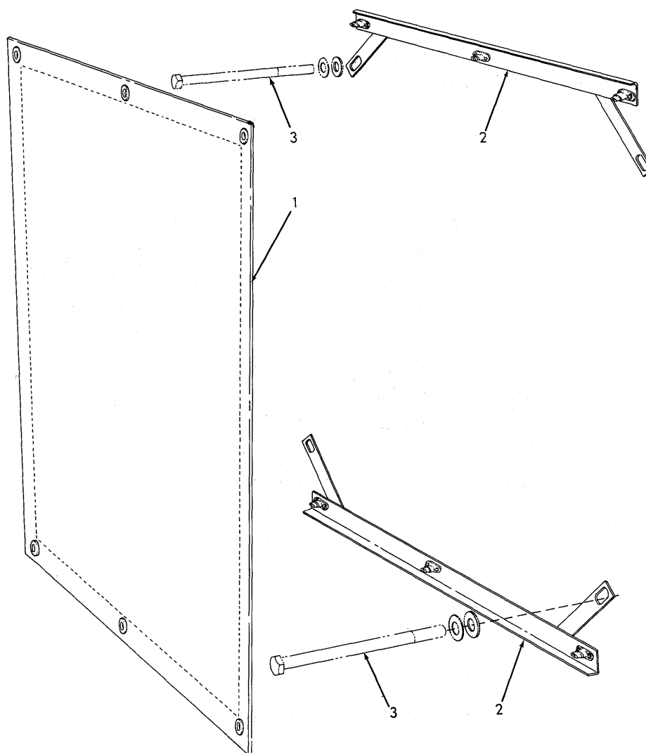
RADIATOR CURTAIN
