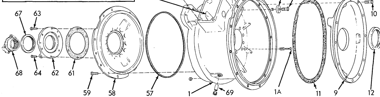
HOUSING
