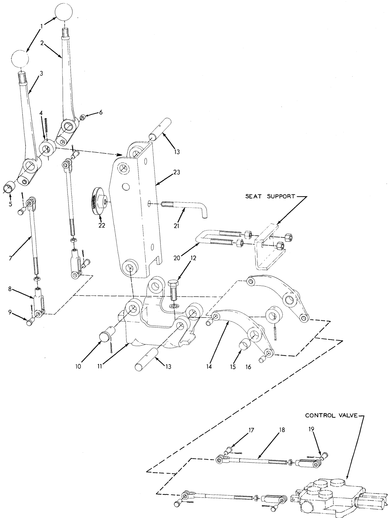
STEERING LEVERS AND LINKAGE
