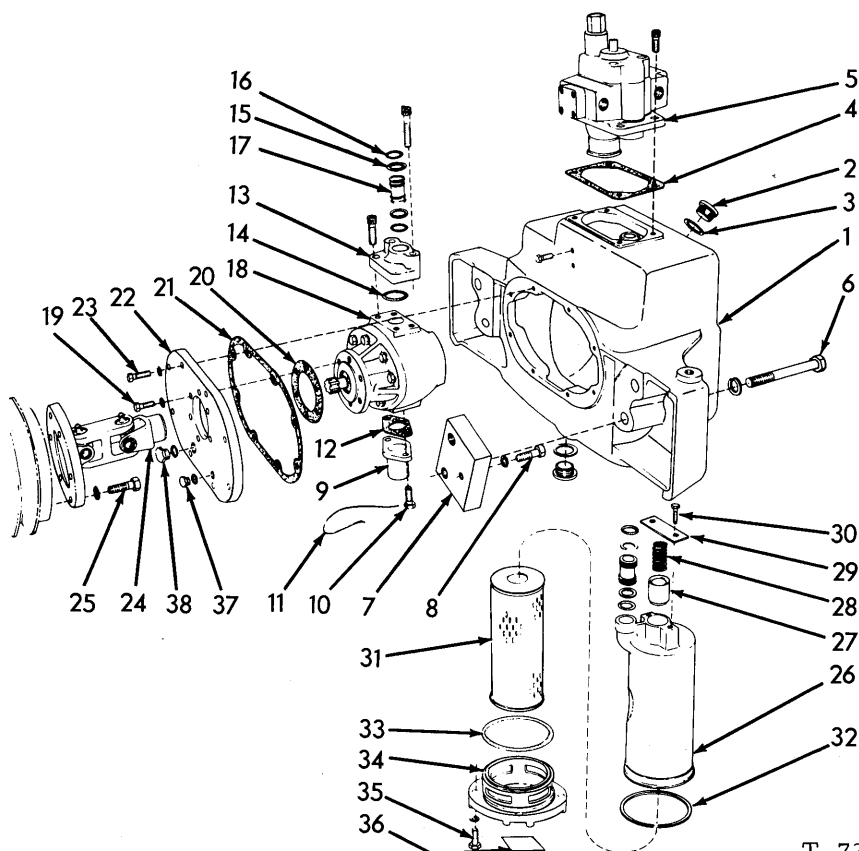
PUMP AND TANK (Second type)
