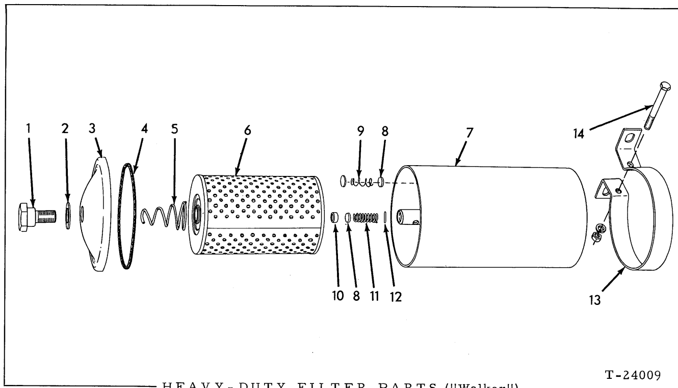
HEAVY-DUTY FILTER PARTS ("Walker")
