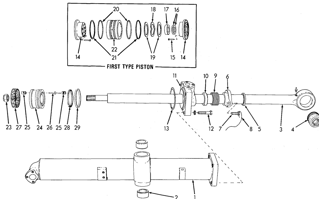
CYLINDER PARTS
