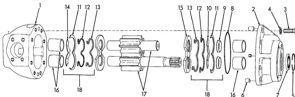
PUMP ASSEMBLY 70649349 ("Tyrone")
