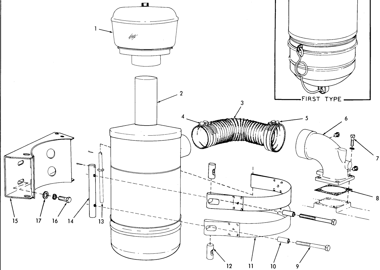
AIR CLEANER (Oil-bath)
