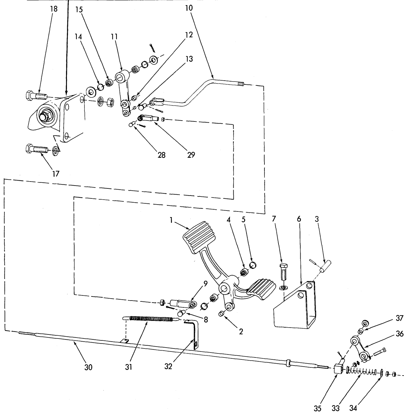
THROTTLE CONTROL (First type)
