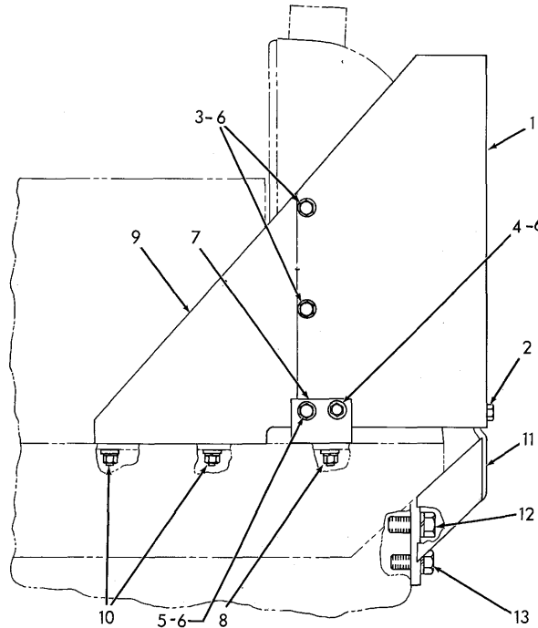
FUEL TANK GUARD
