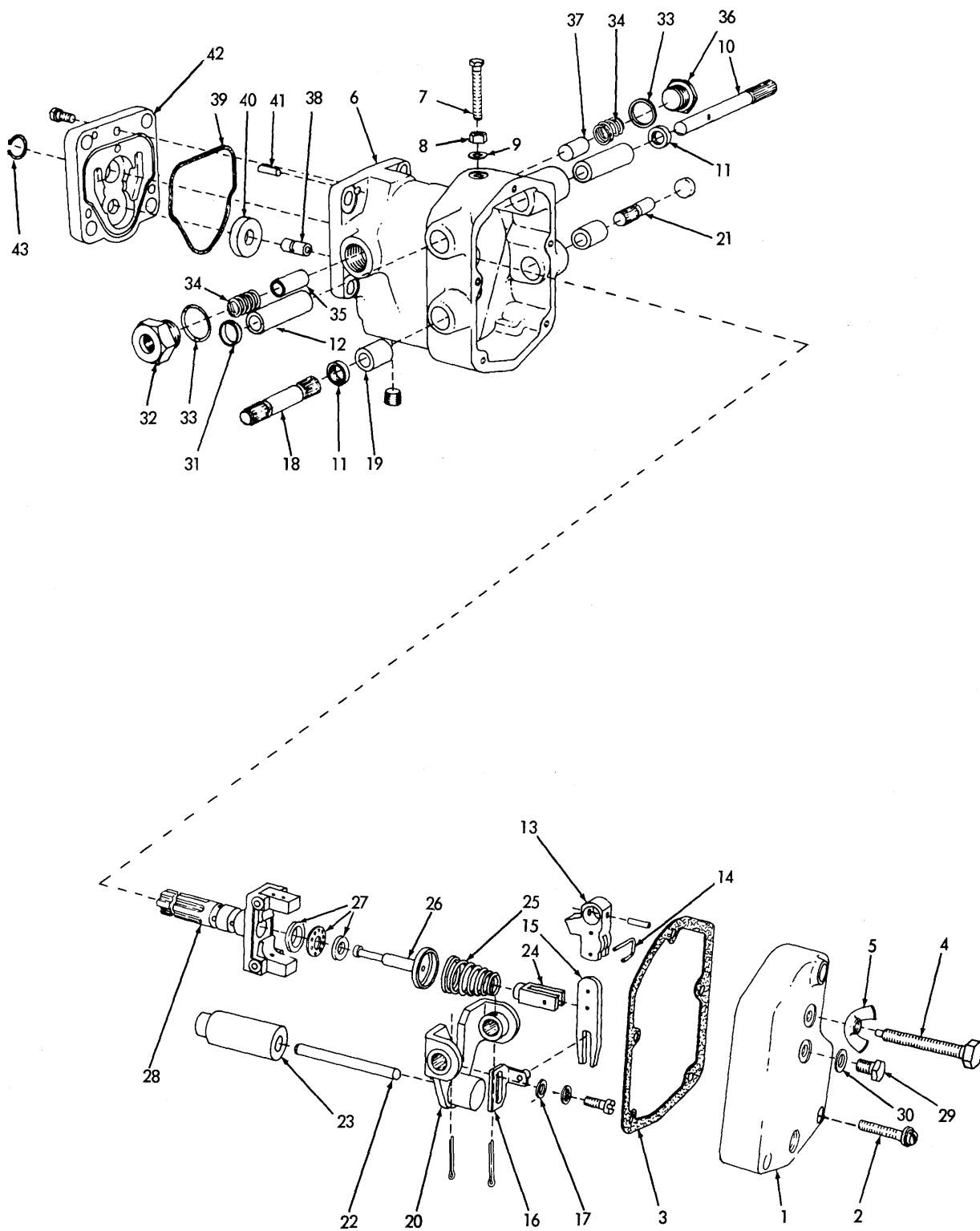
GOVERNOR ASSEMBLY 638088
