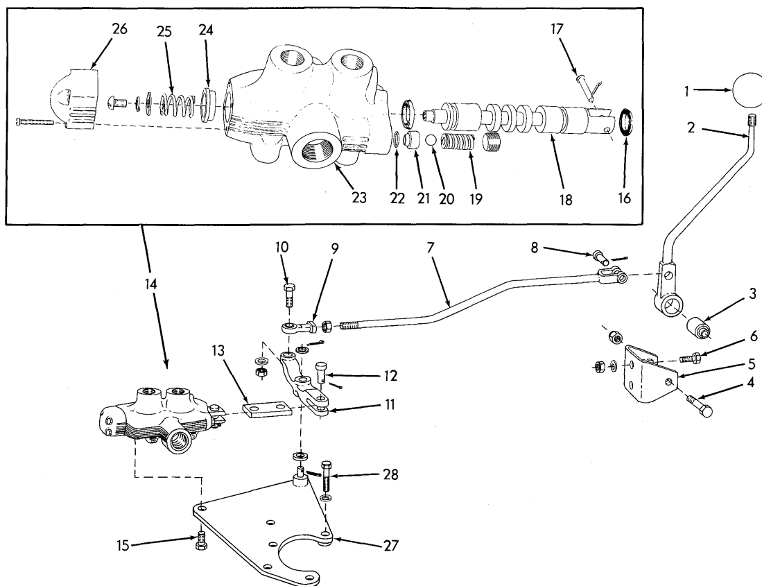
AUXILIARY CONTROL VALVE
