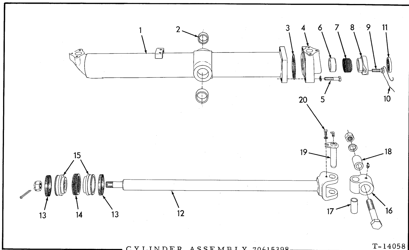
CYLINDER ASSEMBLY 70615398
