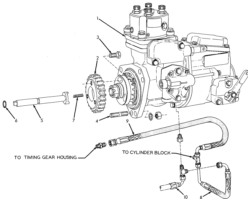
INJECTION PUMP
