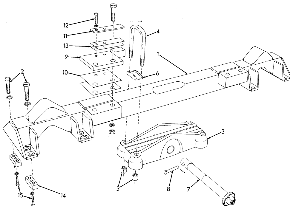
RIGID BEAM
