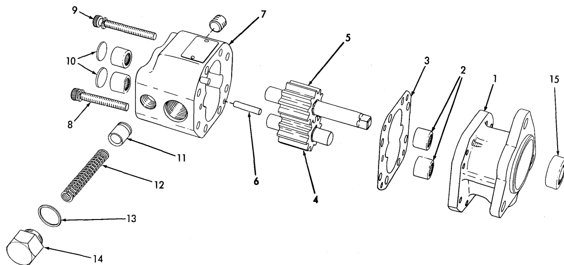
OIL PUMP ASSEMBLY
