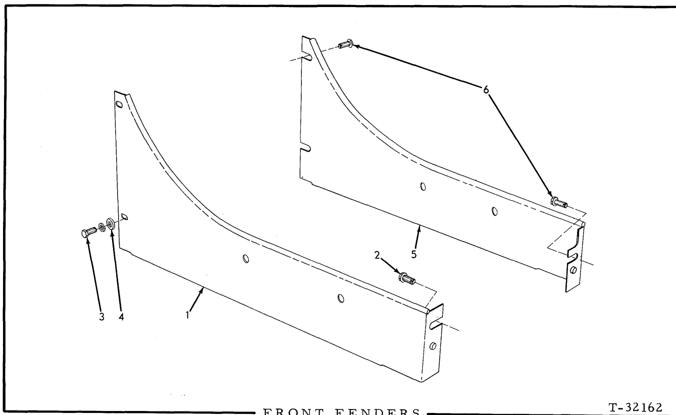
FRONT FENDERS
