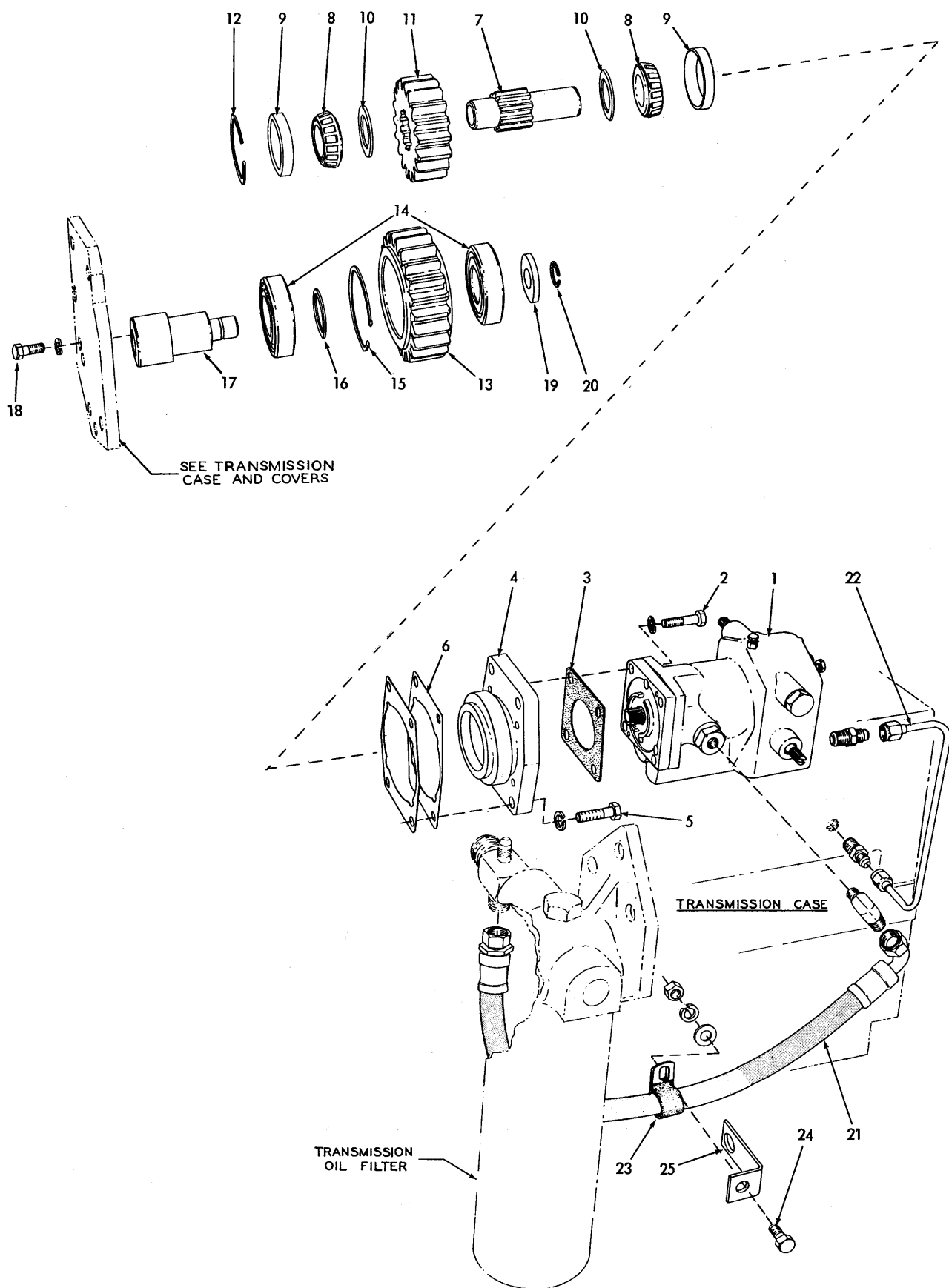
GROUND SPEED GOVERNOR
