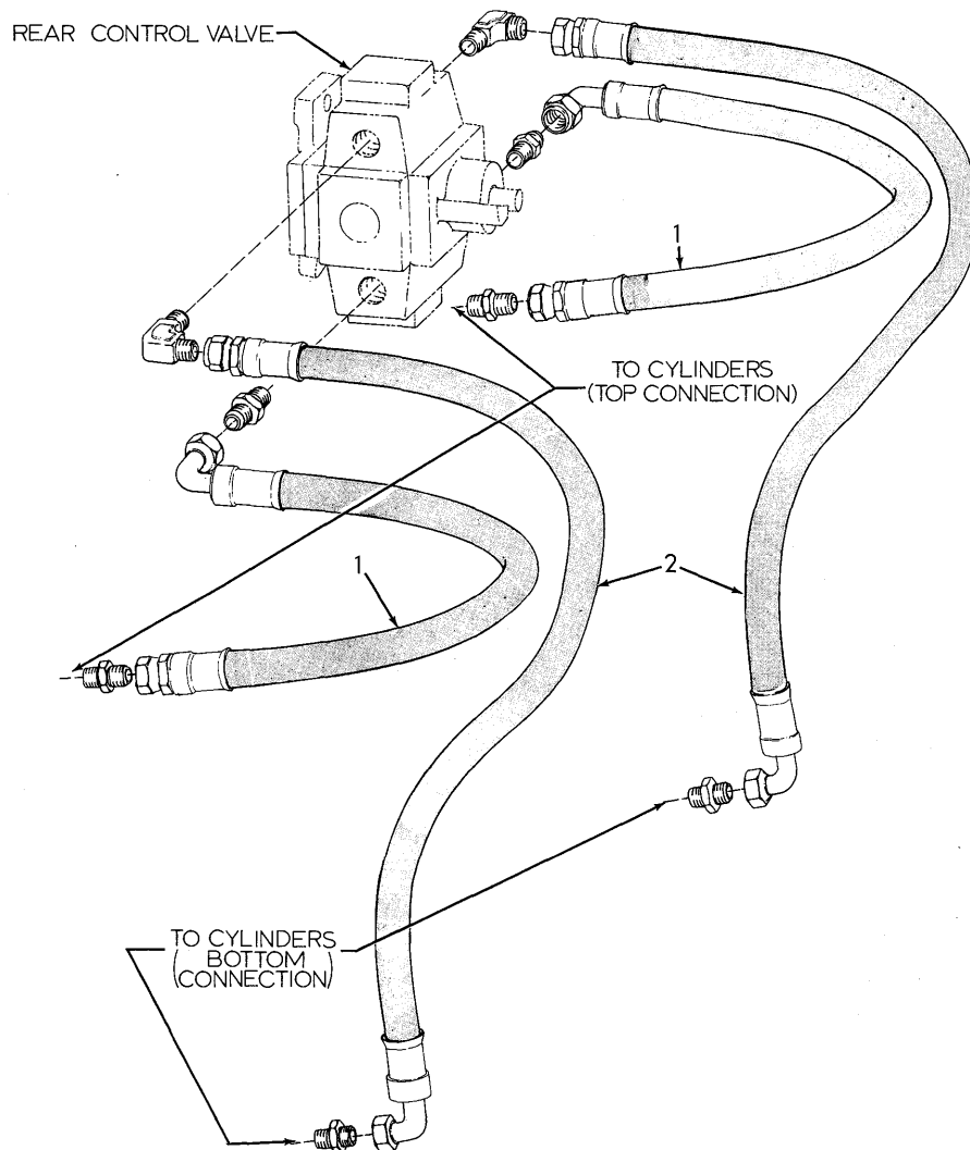
RIPPER CYLINDER PIPING (For dual cylinders)
