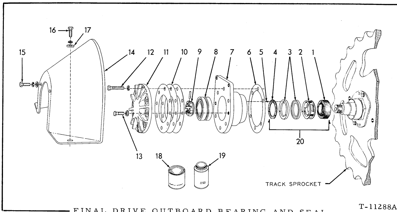
FINAL DRIVE OUTBOARD BEARING AND SEAL
