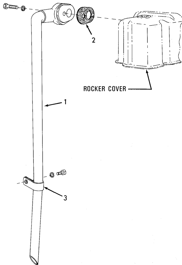
ENGINE BREATHER
