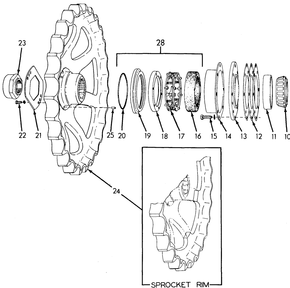
FINAL DRIVE SPROCKET, SHAFT AND
