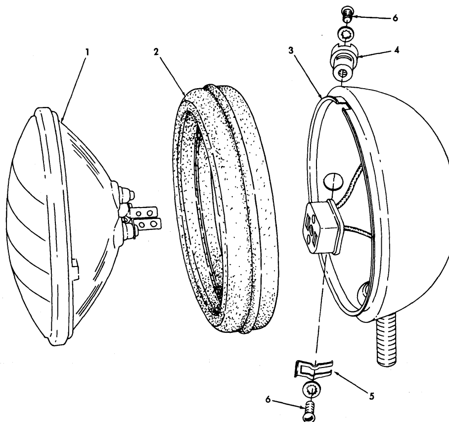
LIGHT ASSEMBLY 70638283
