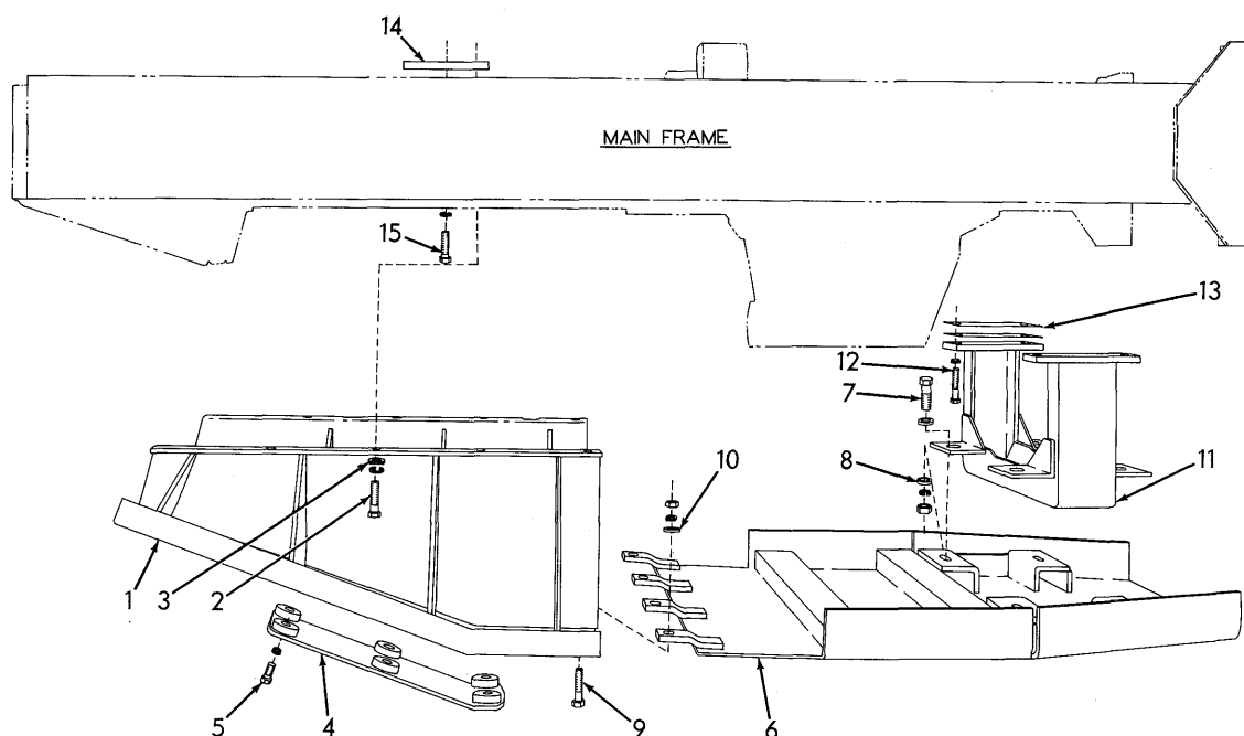
BOTTOM GUARDS
