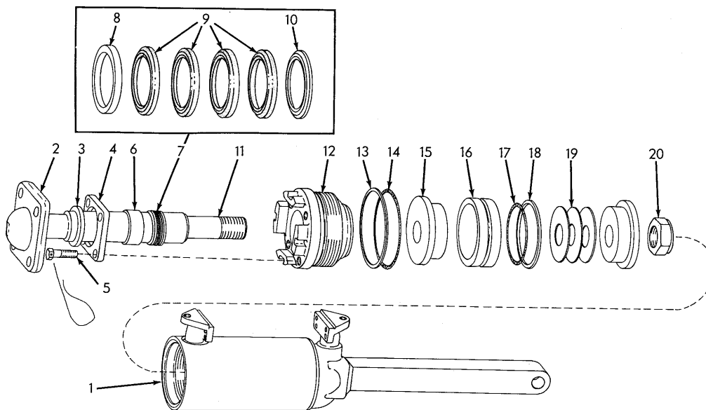
TILT CYLINDER ASSEMBLY 70659891
