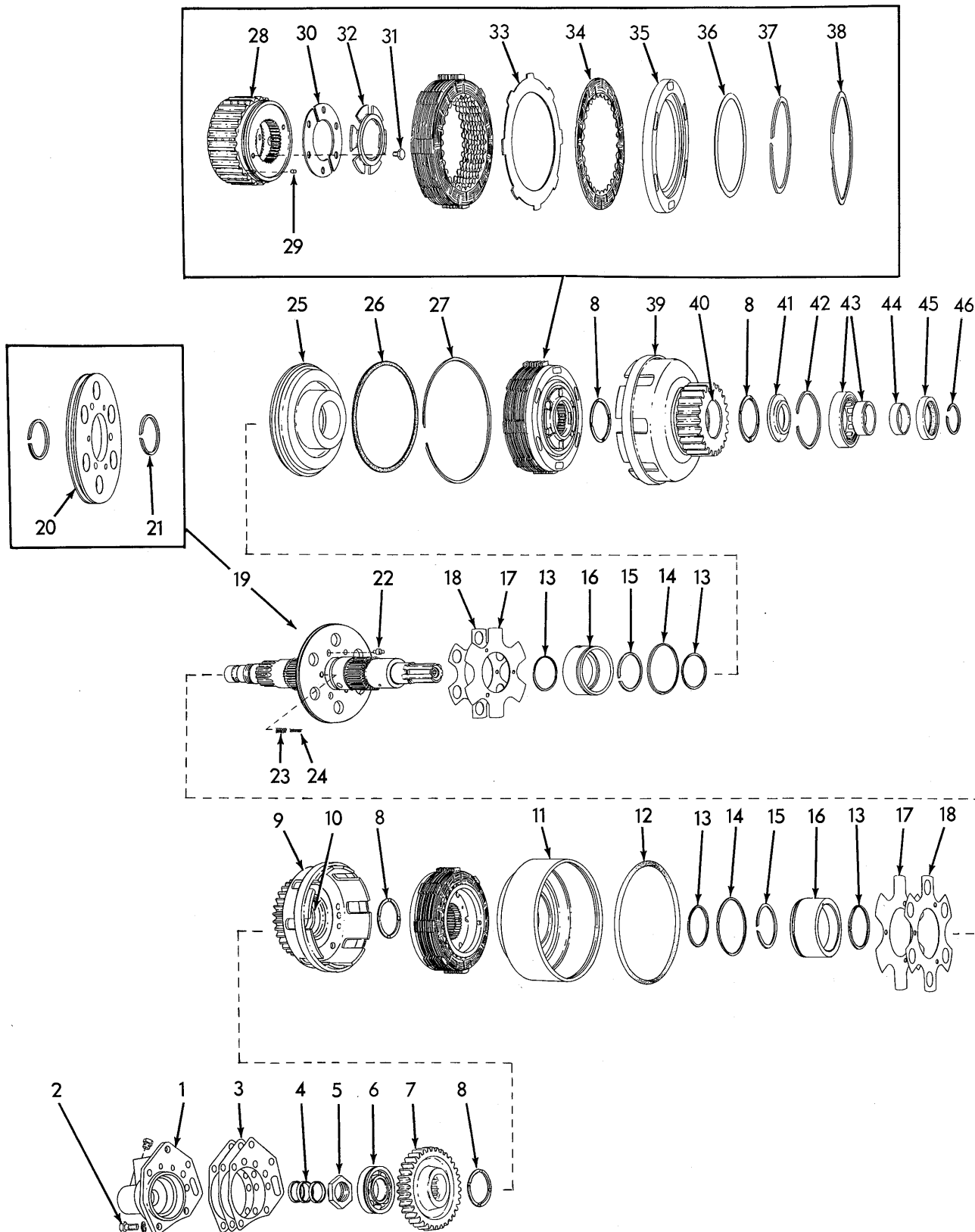
TRANSMISSION TOP SHAFT
