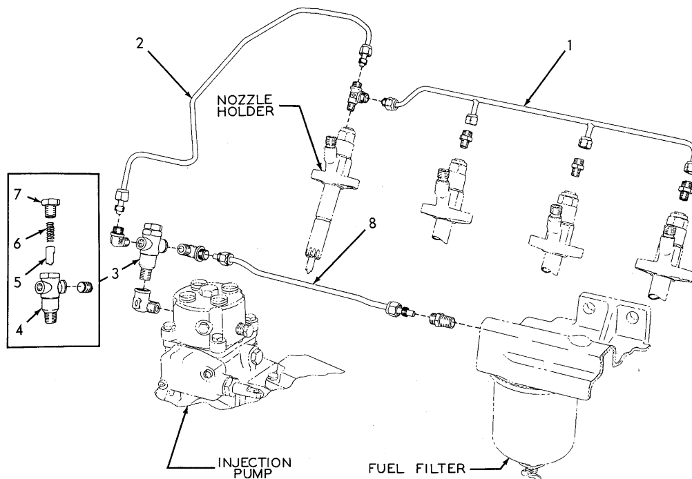
INJECTION FUEL RETURN LINES
