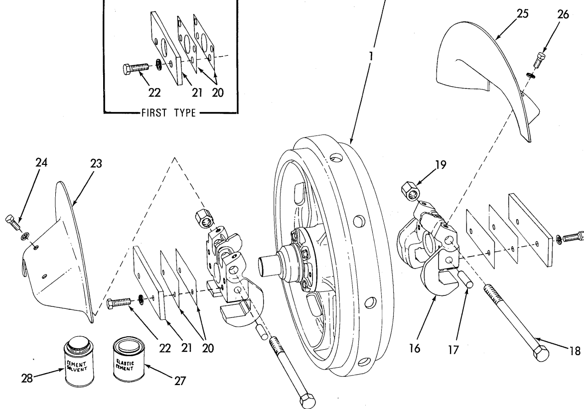
TRACK IDLER
