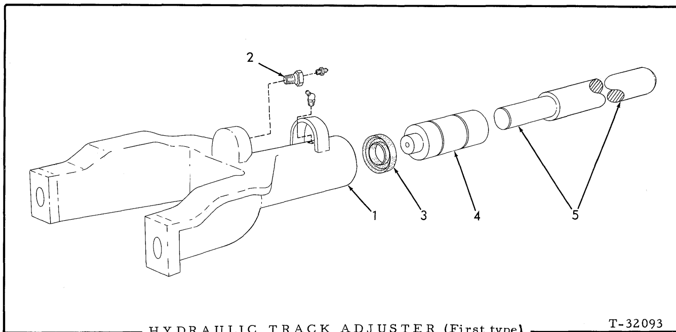
HYDRAULIC TRACK ADJUSTER (First type)
