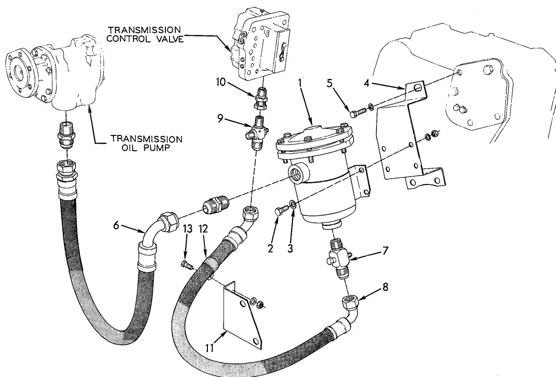
TRANSMISSION OIL FILTER (First type)
