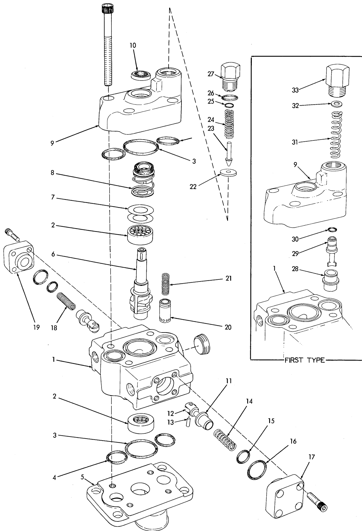
CONTROL VALVE PARTS
