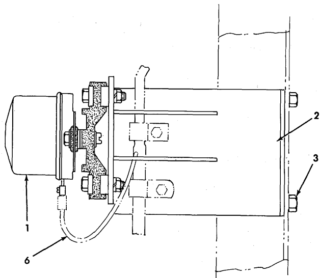
UNITS WITH OIL-BATH AIR CLEANER
