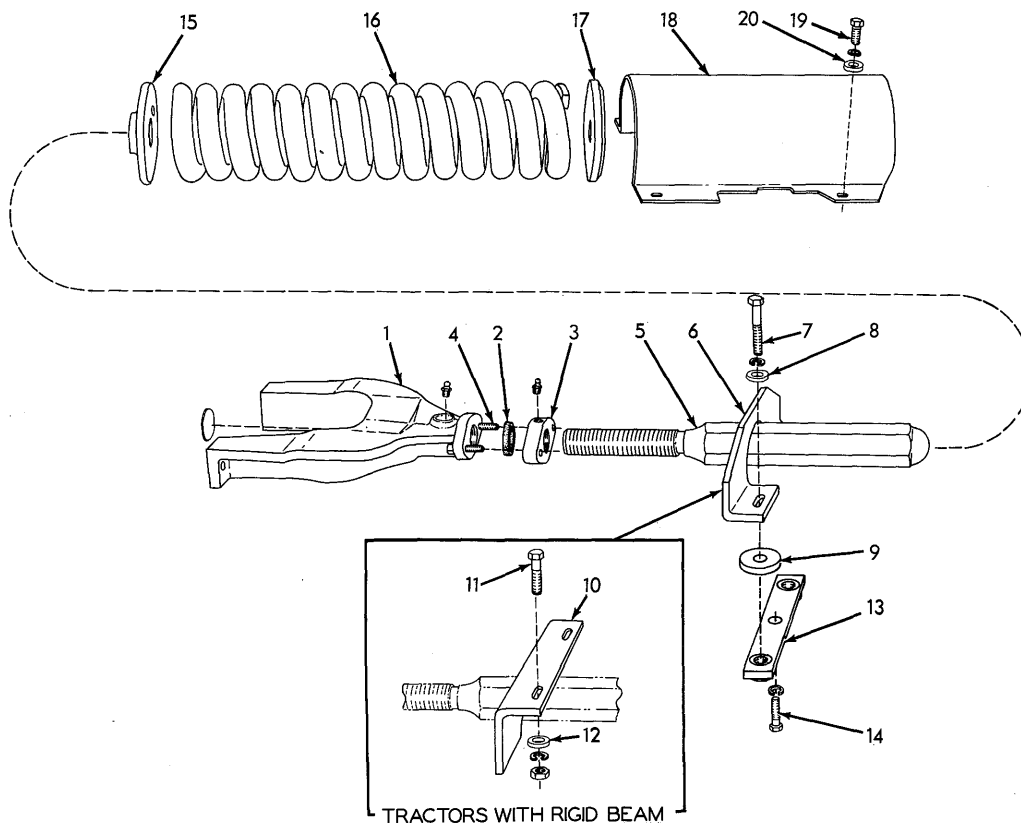
TRACK RELEASE
