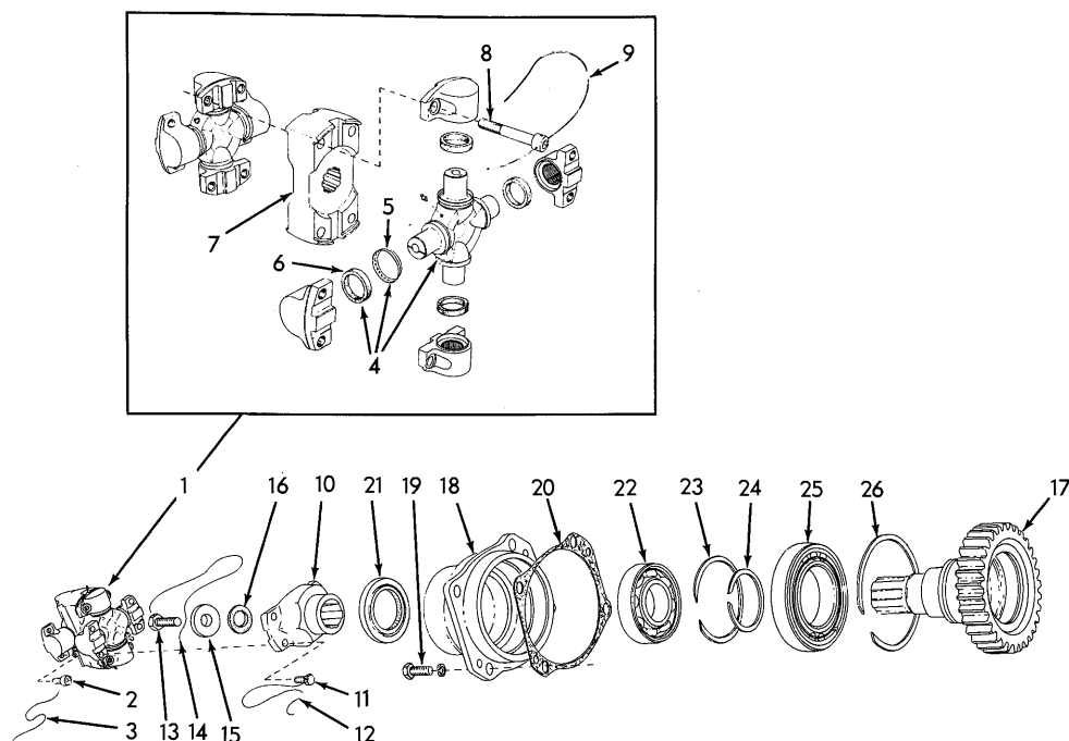
DRIVE SHAFT
