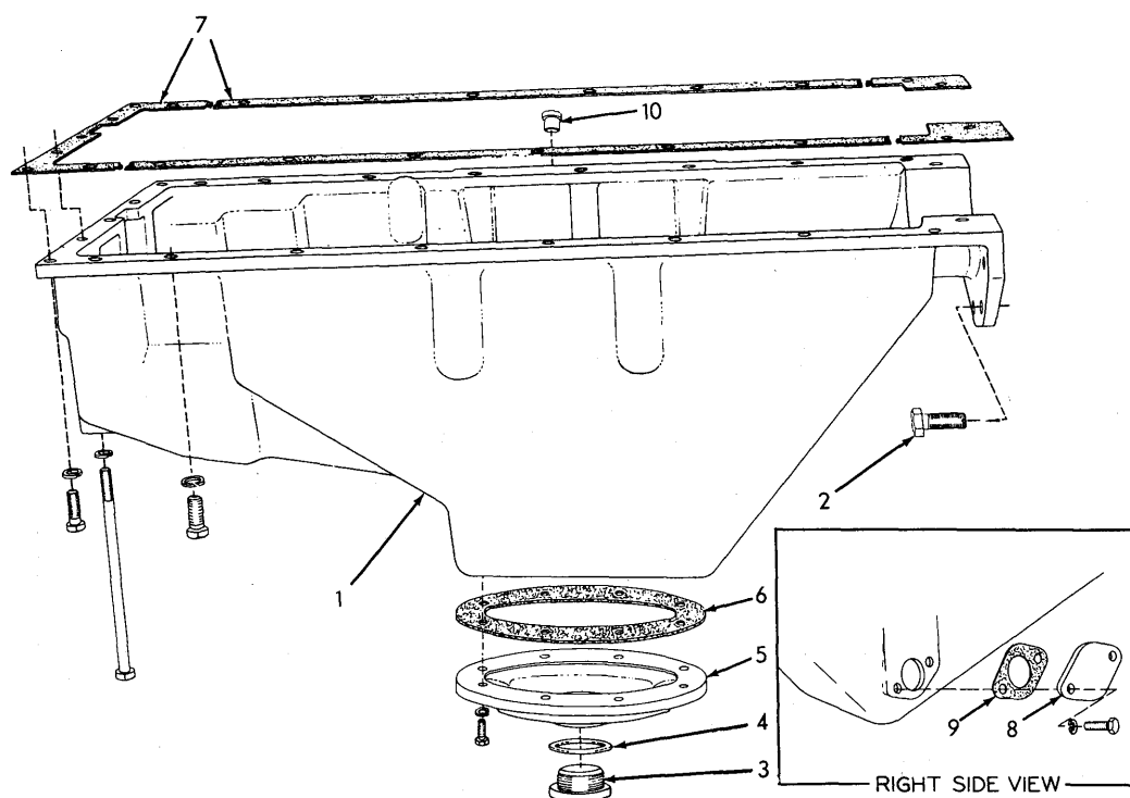
OIL PAN
