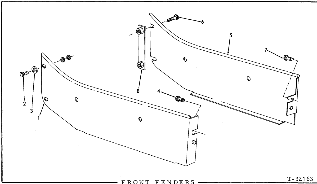
FRONT FENDERS
