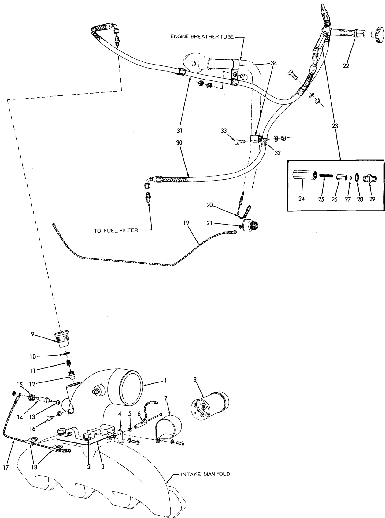
AIR HEATER (Model HD6E)
