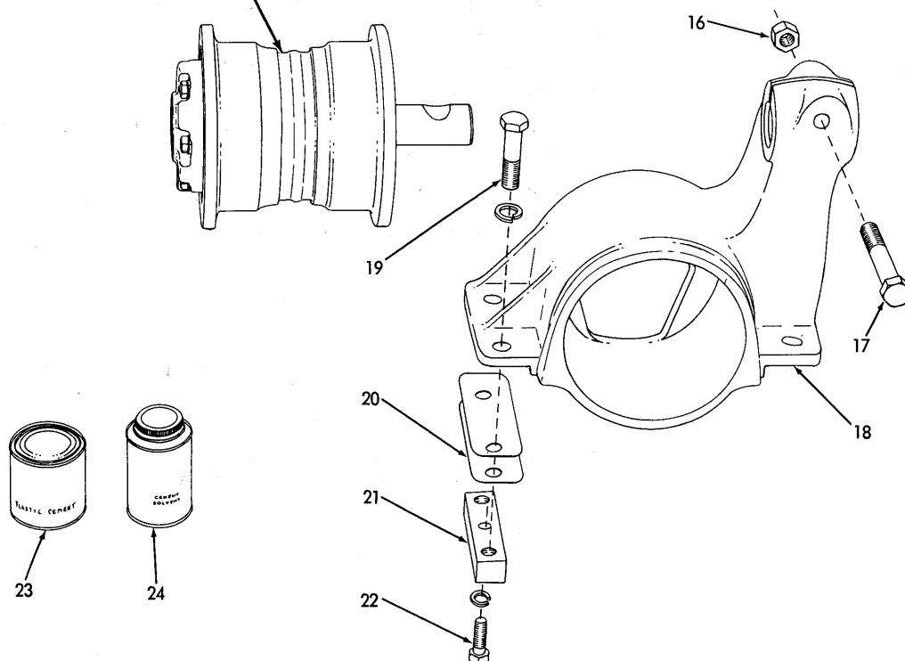
TRACK CARRIER ROLLER (First type)
