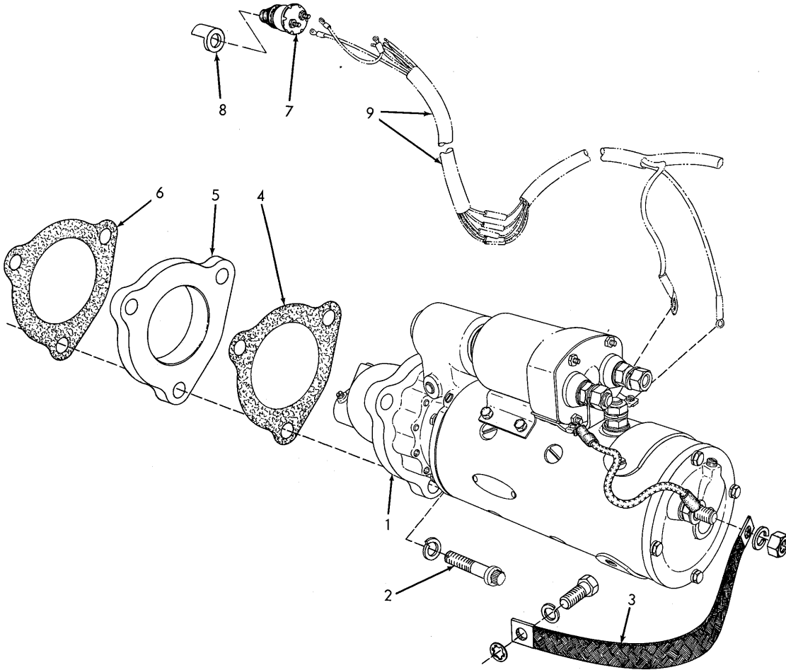
STARTER
