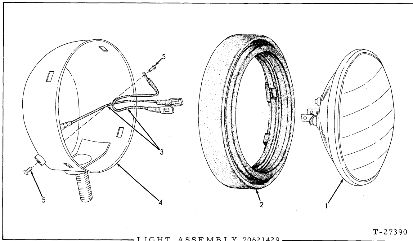
LIGHT ASSEMBLY 70621429
