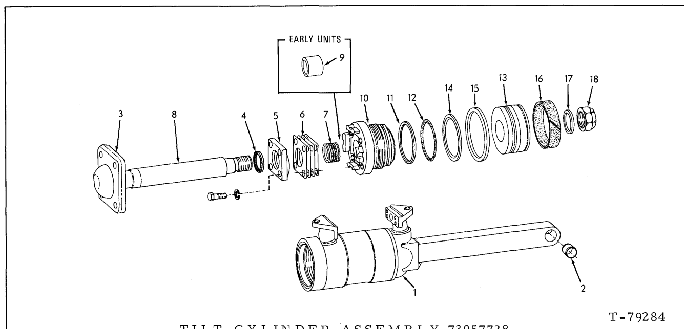
TILT CYLINDER ASSEMBLY 73057728
