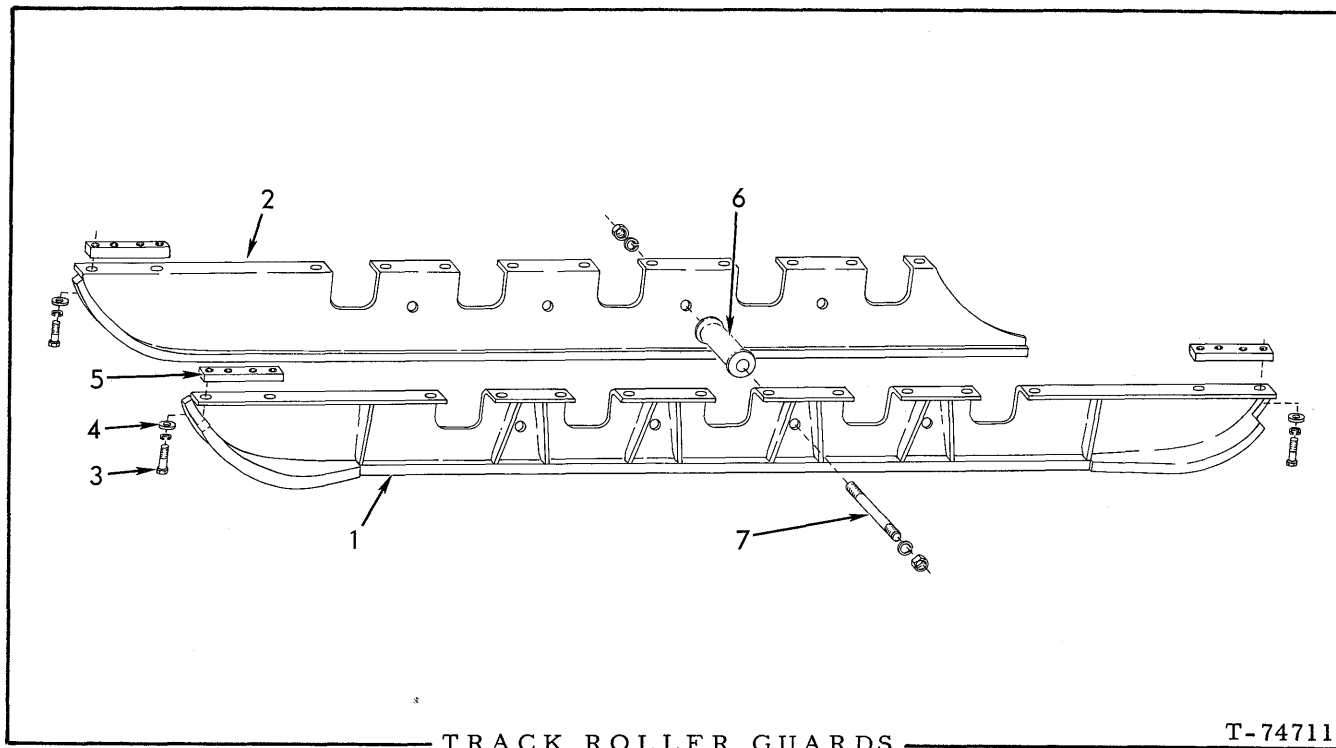
TRACK ROLLER GUARDS
