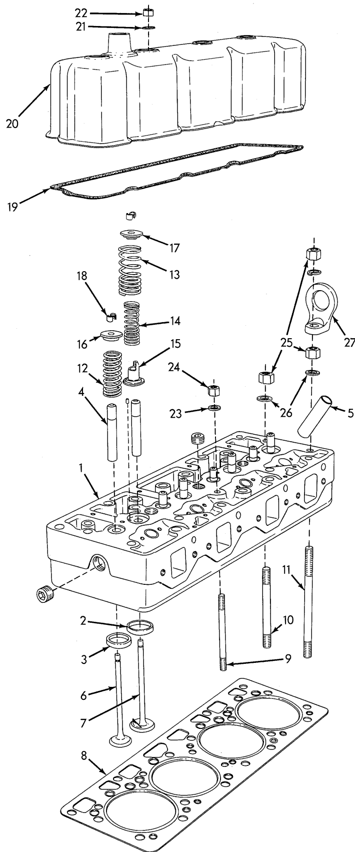
CYLINDER HEAD
