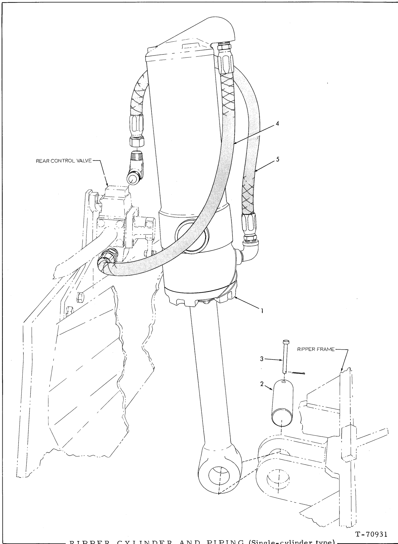
RIPPER CYLINDER AND PIPING (Single-cylinder type)
