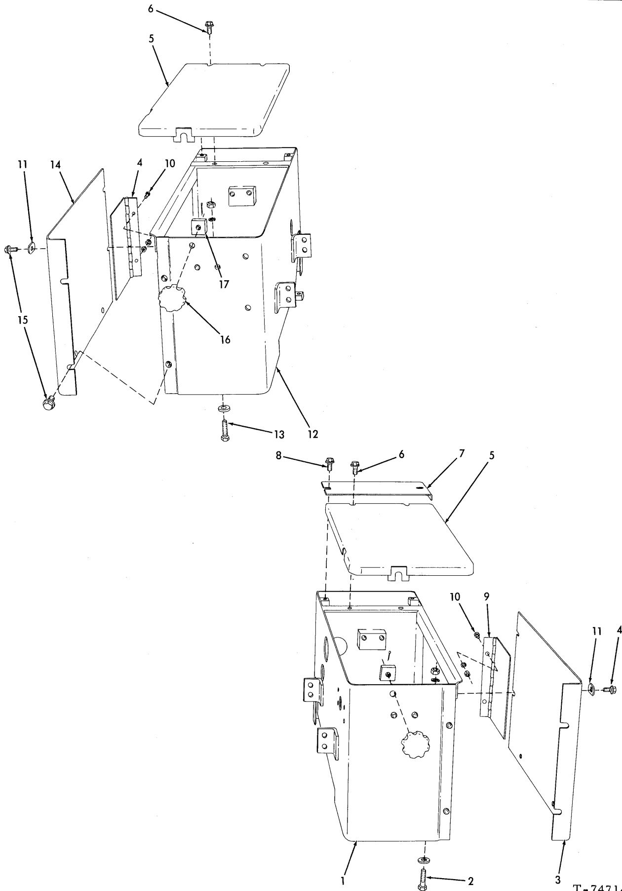
BATTERY BOXES
