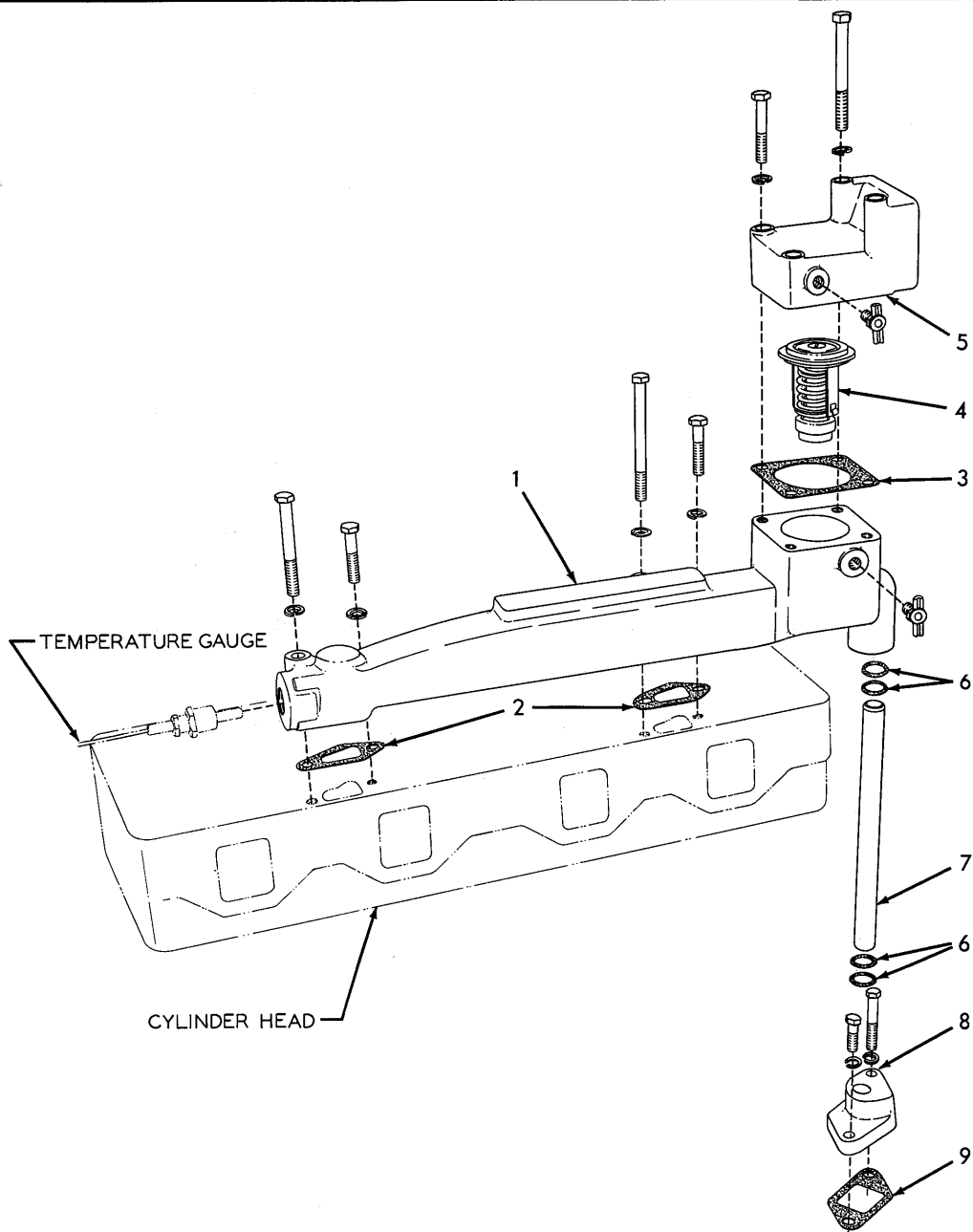
WATER OUTLET MANIFOLD
