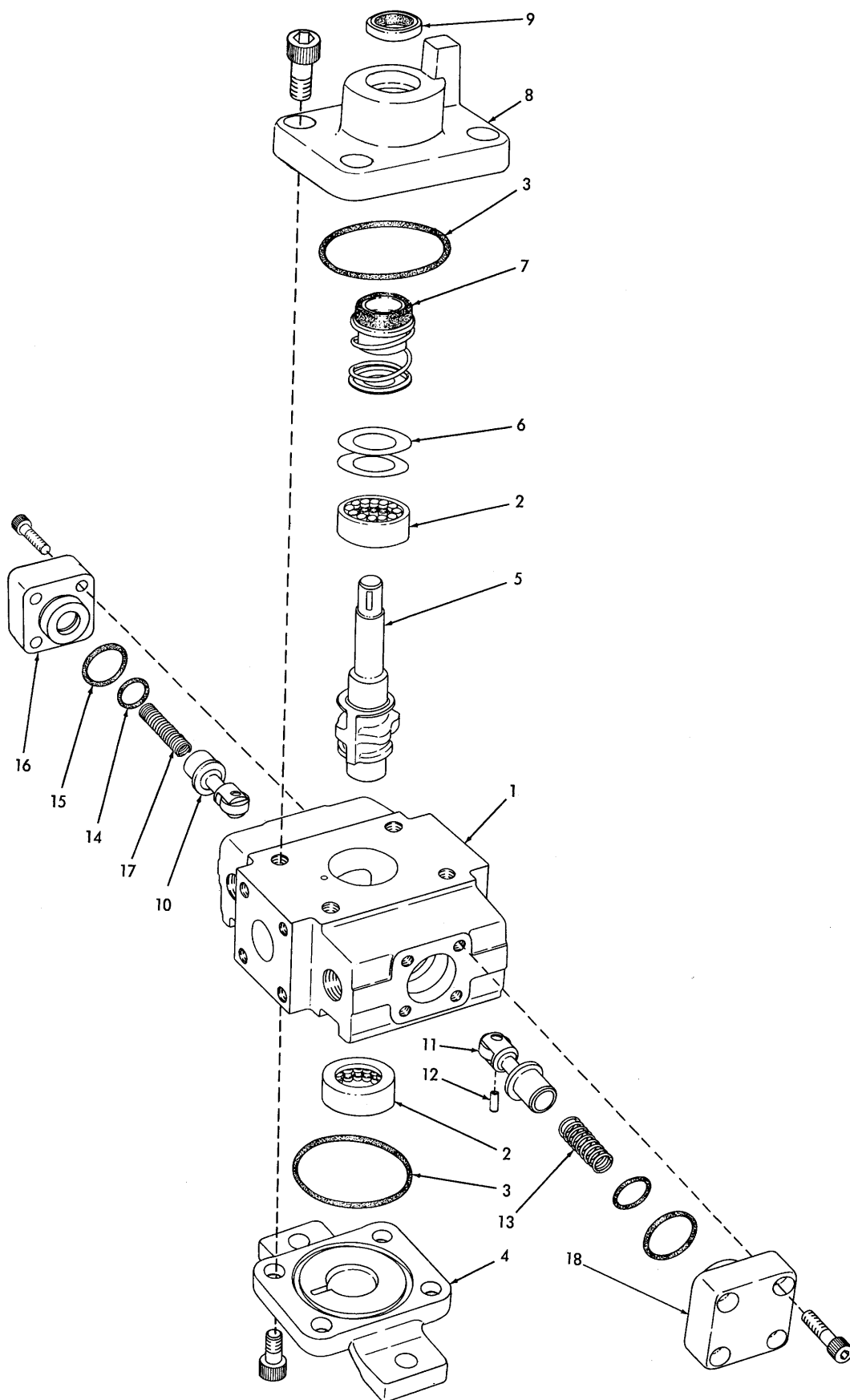
CONTROL VALVE ASSEMBLY 618911
