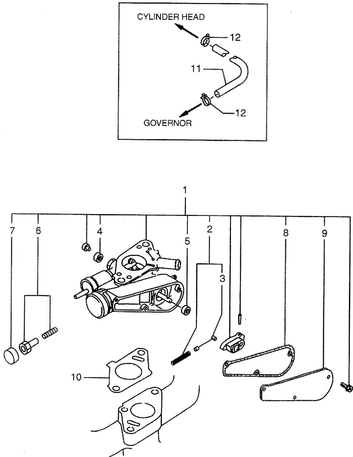
FIG. 42 GOVERNOR ガバナ
