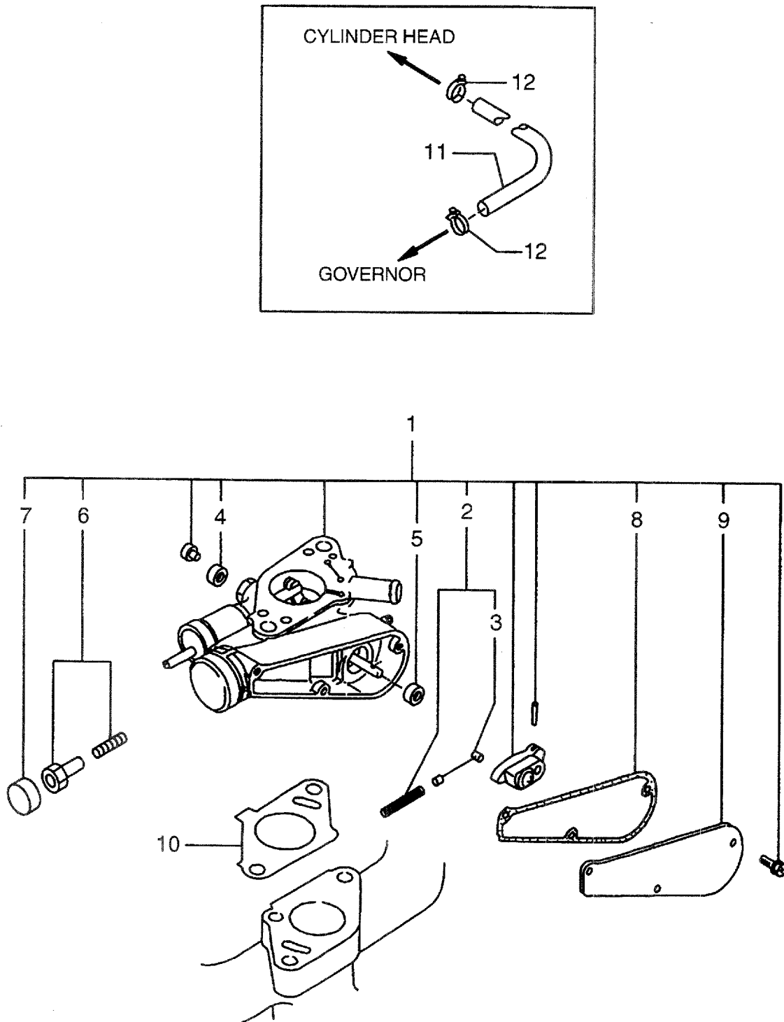
FIG. 41 GOVERNOR ガバナ
