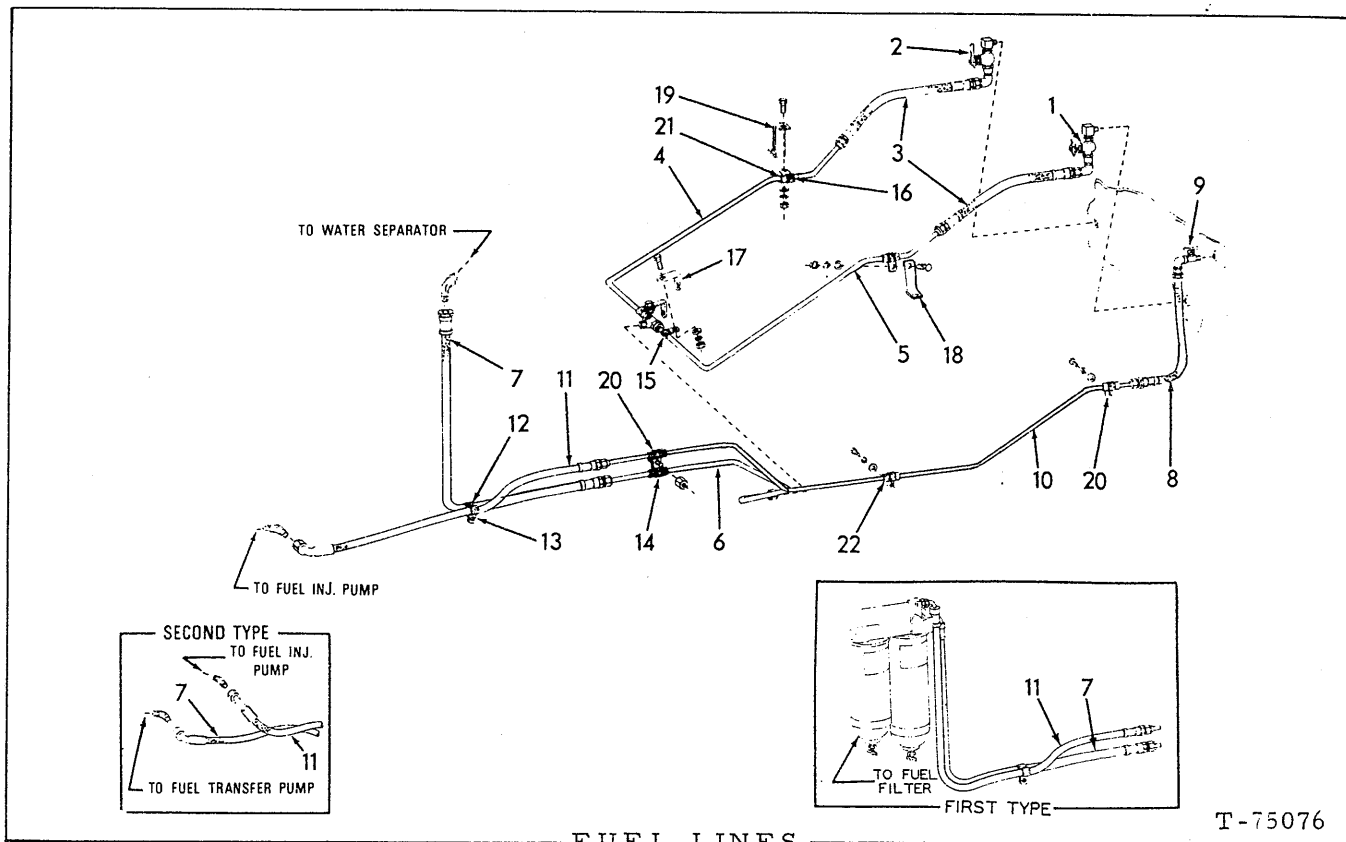
FUEL LINES
