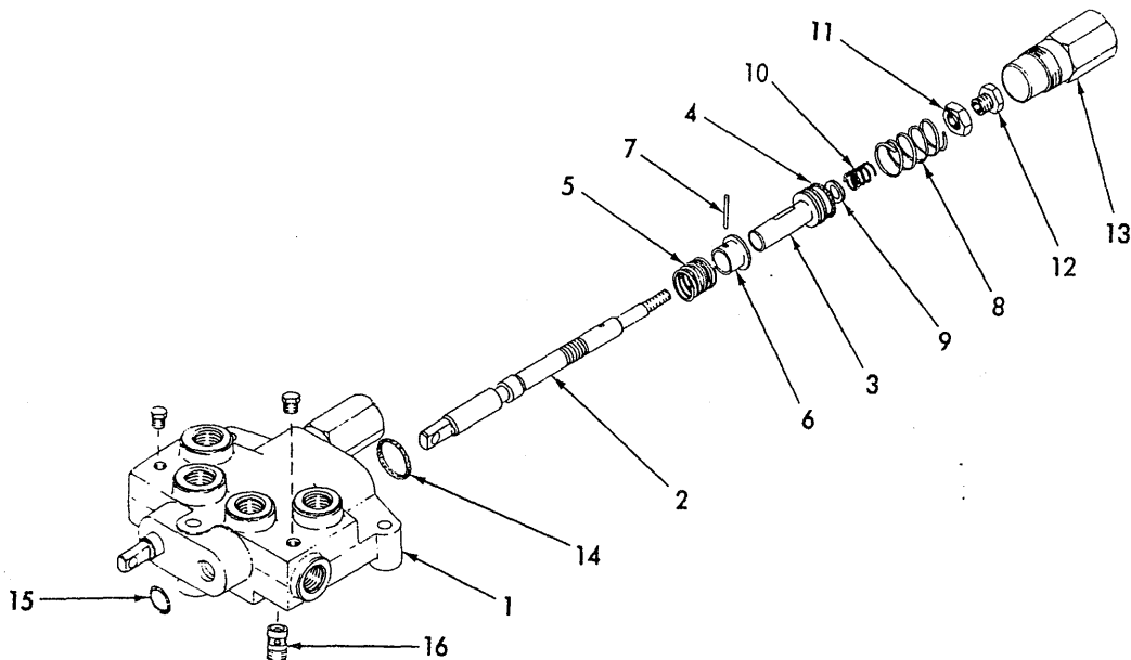
STEERING CONTROL VALVE
