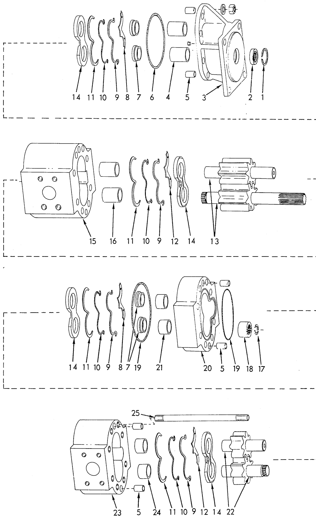
PUMP PARTS
