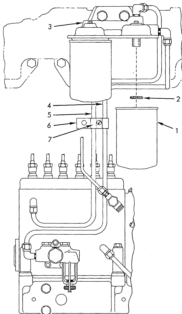
FUEL FILTER
