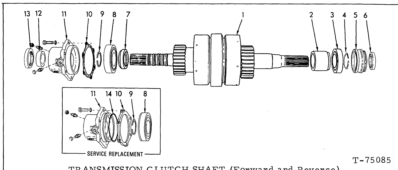
TRANSMISSION CLUTCH SHAFT (Forward and Reverse)
