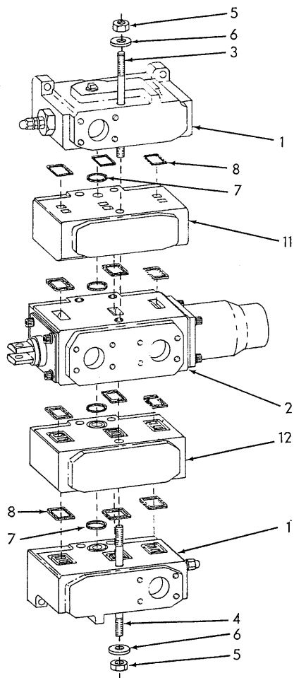
VALVE ASSY. 70686090
