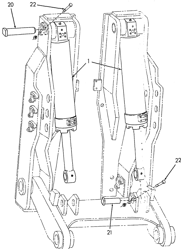
— RIPPER CYLINDERS —
