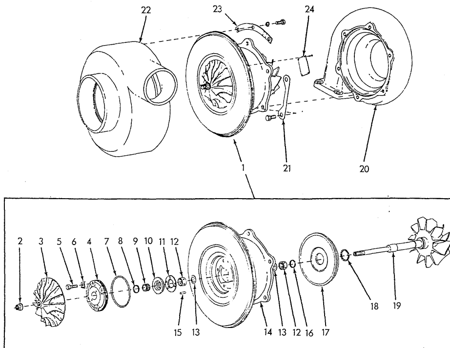
TURBOCHARGER ASSEMBLY
