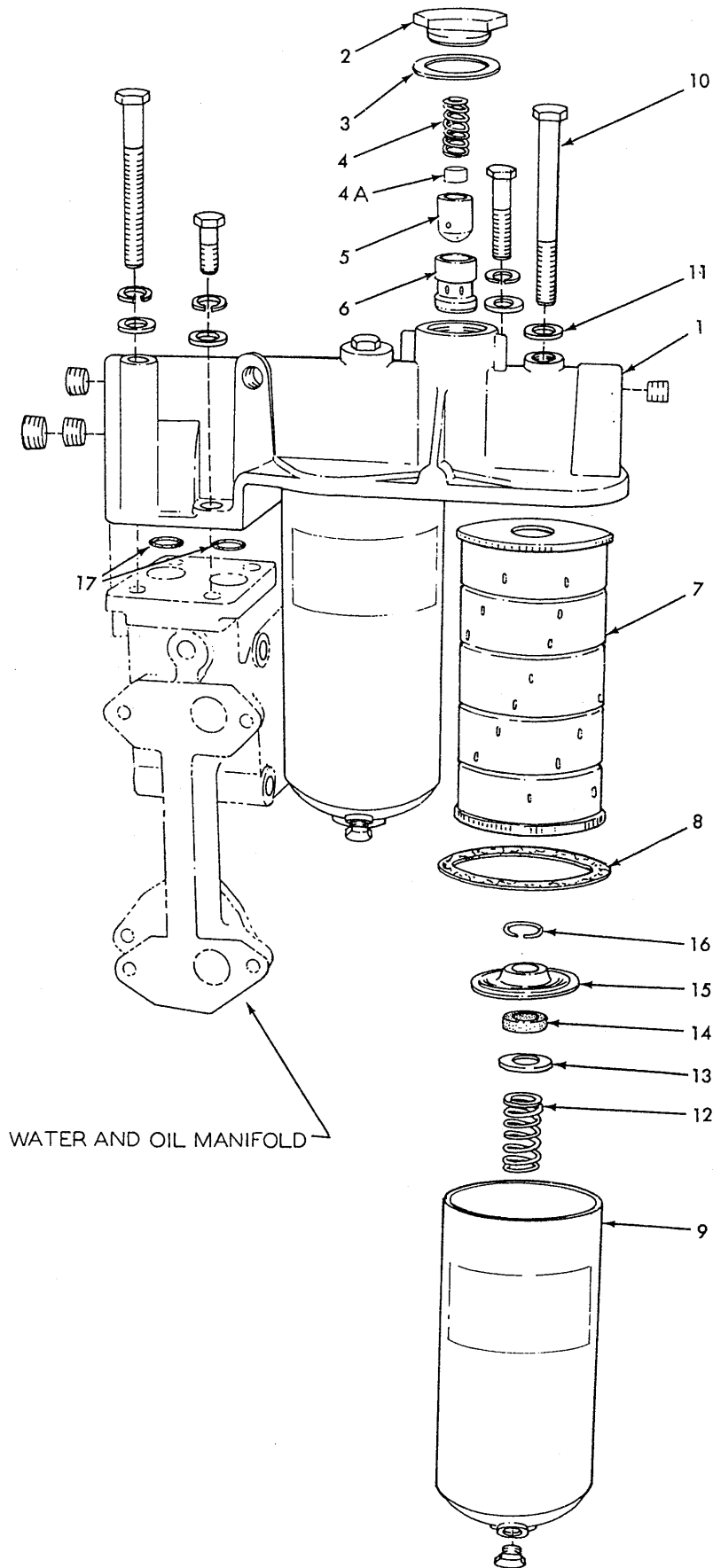
OIL FILTER (Full-flow type)
