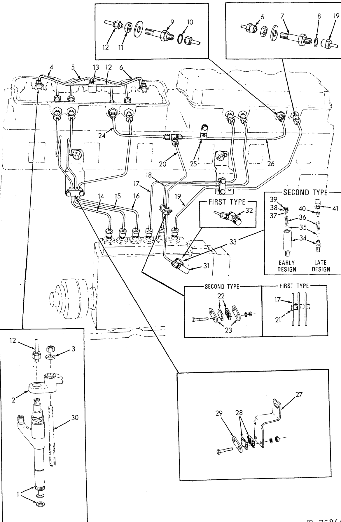
INJECTION NOZZLE LINES (Robert Bosch-Germany)
