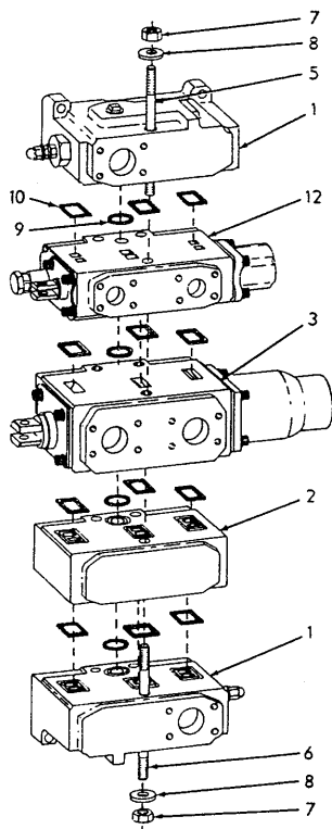
VALVE ASSY 70665121
