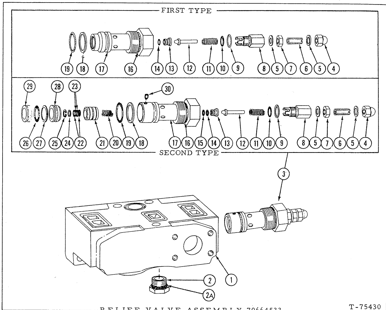
RELIEF VALVE ASSEMBLY 70664533
