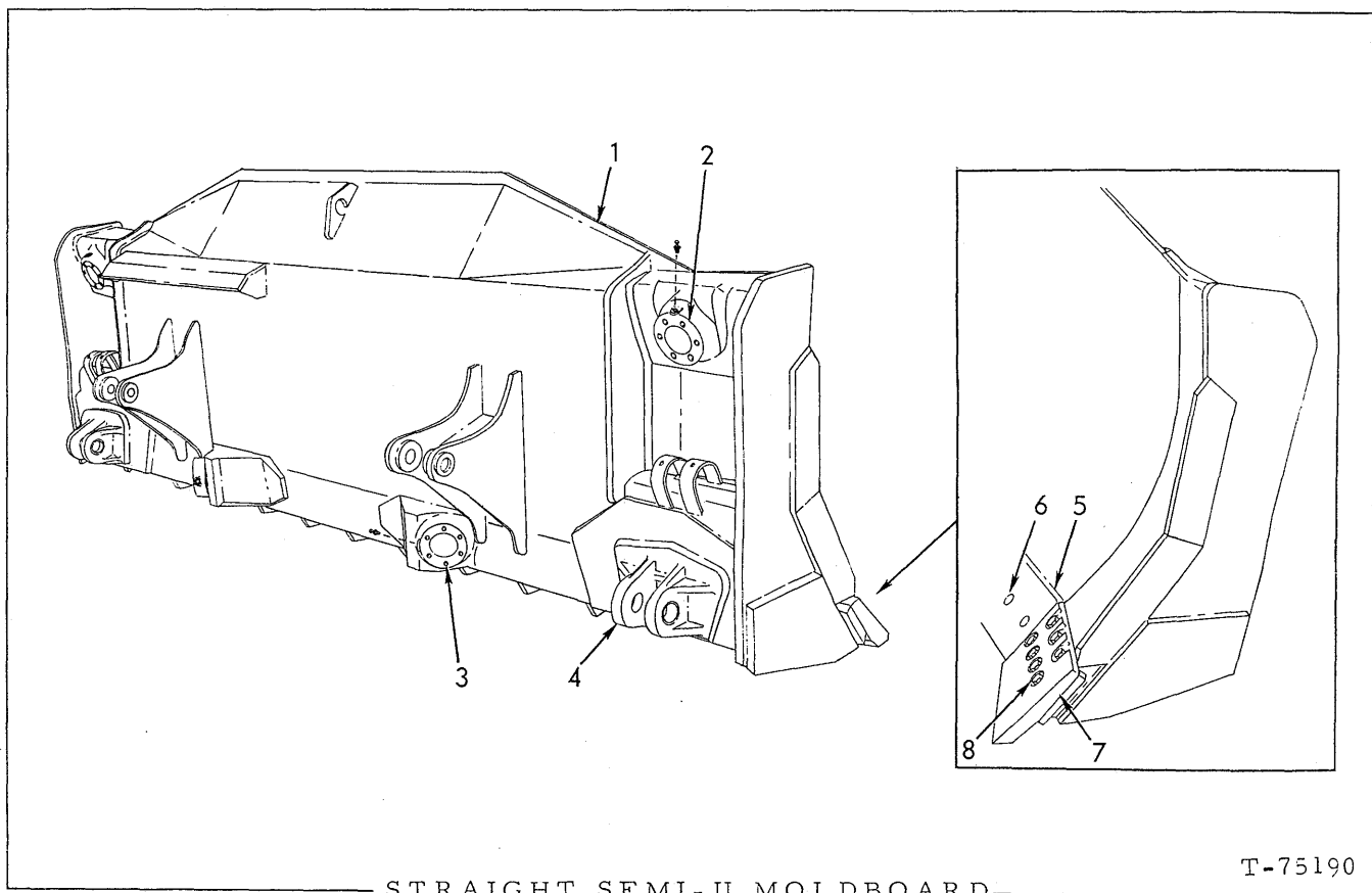
STRAIGHT SEMI- U MOLDBOARD
