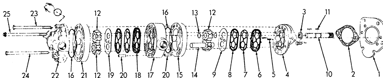
STEERING PUMP PARTS
