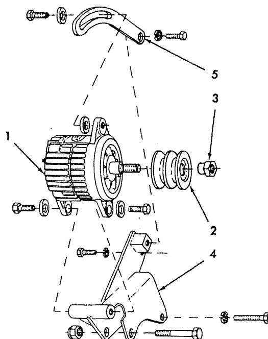
ALTERNATOR
