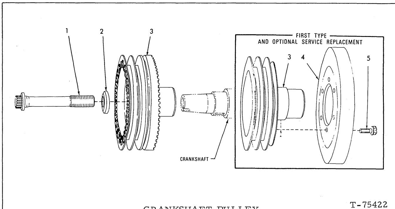
CRANKSHAFT PULLEY
