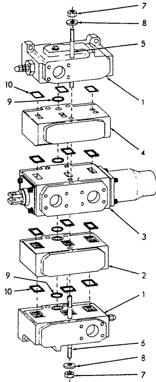
VALVE ASSY 70660647
