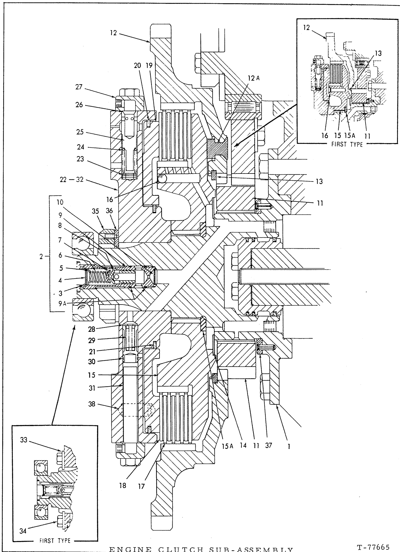
ENGINE CLUTCH SUB-ASSEMBLY
