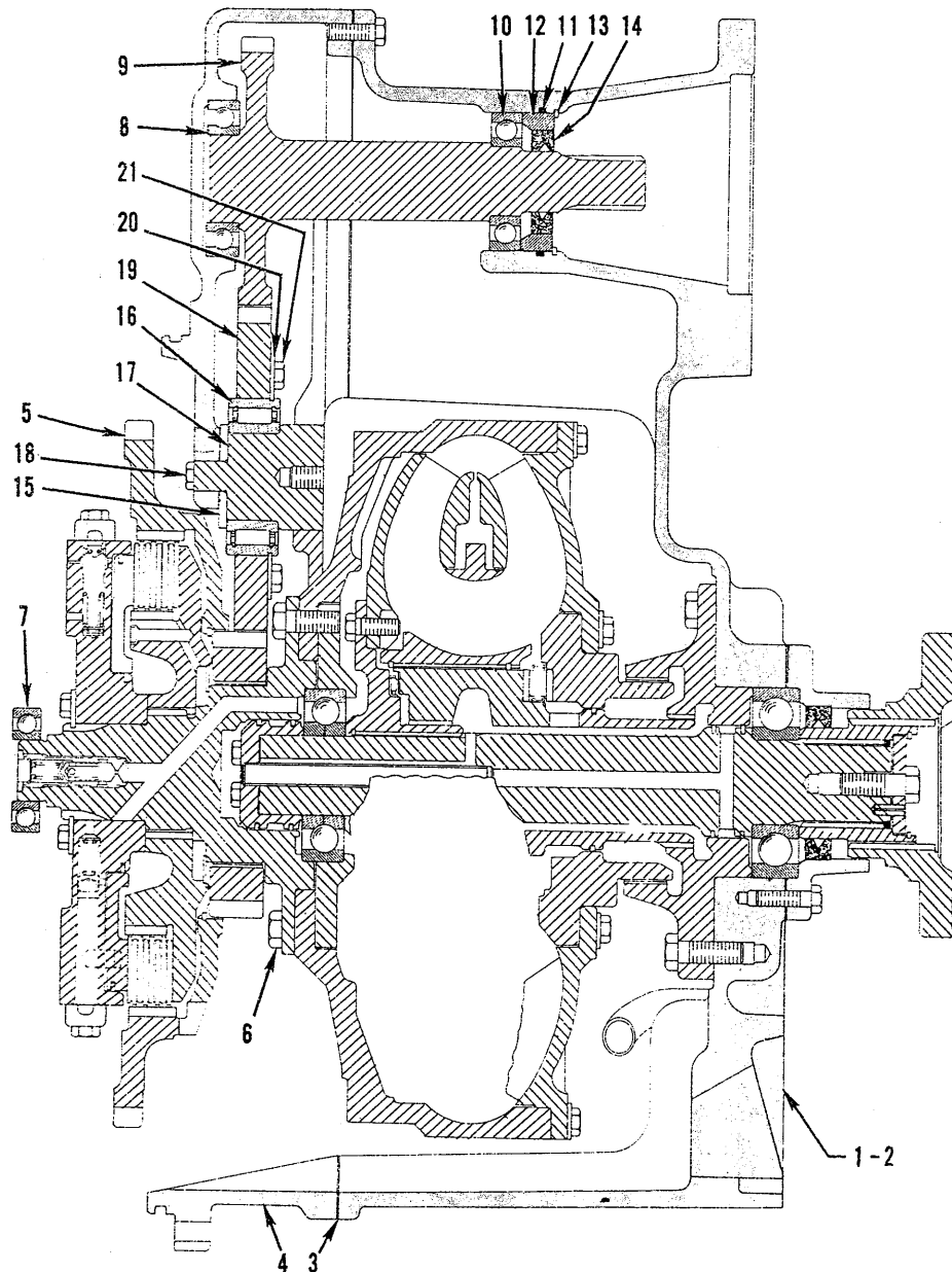
TORQUE CONVERTER ASSEMBLY 70654305
