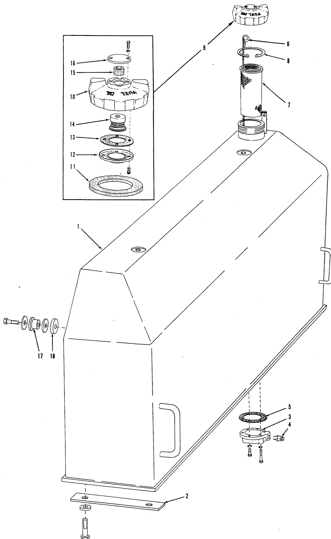
FUEL TANK
