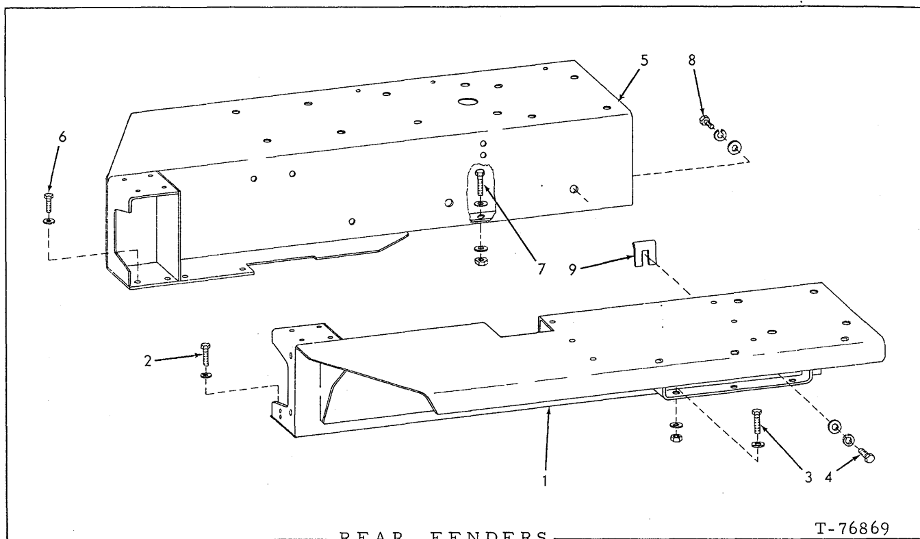
REAR FENDERS
