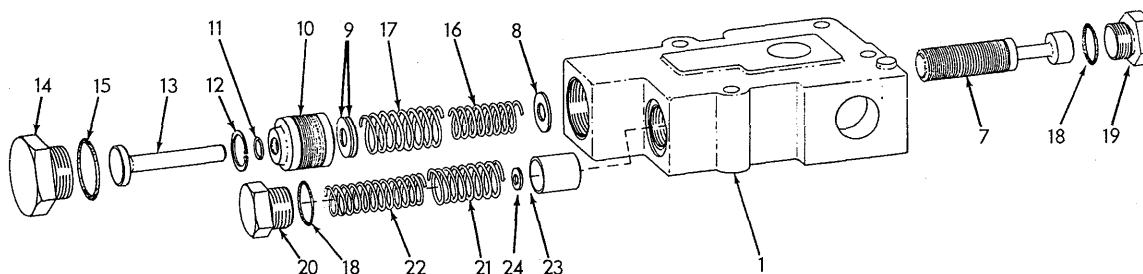
PRESSURE REGULATING VALVE ASSEMBLY 70677065 T-76866
