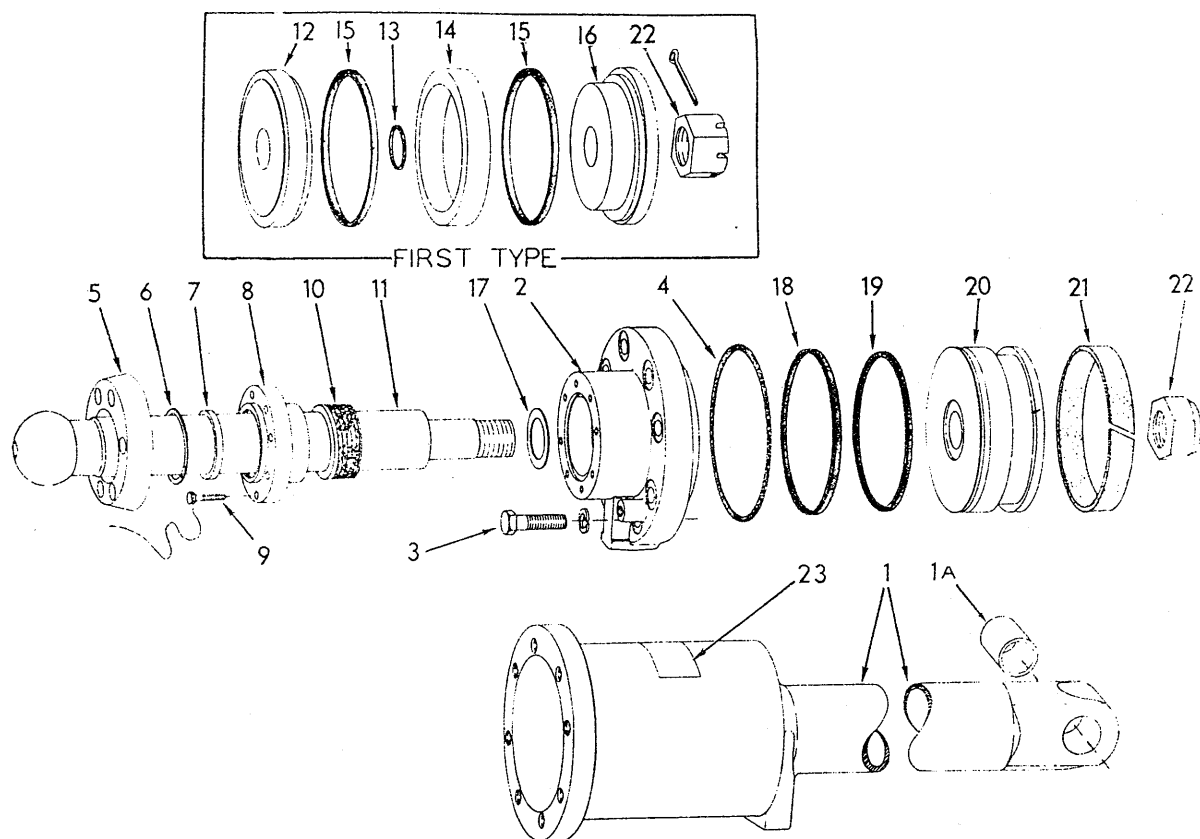
TILT CYLINDER
