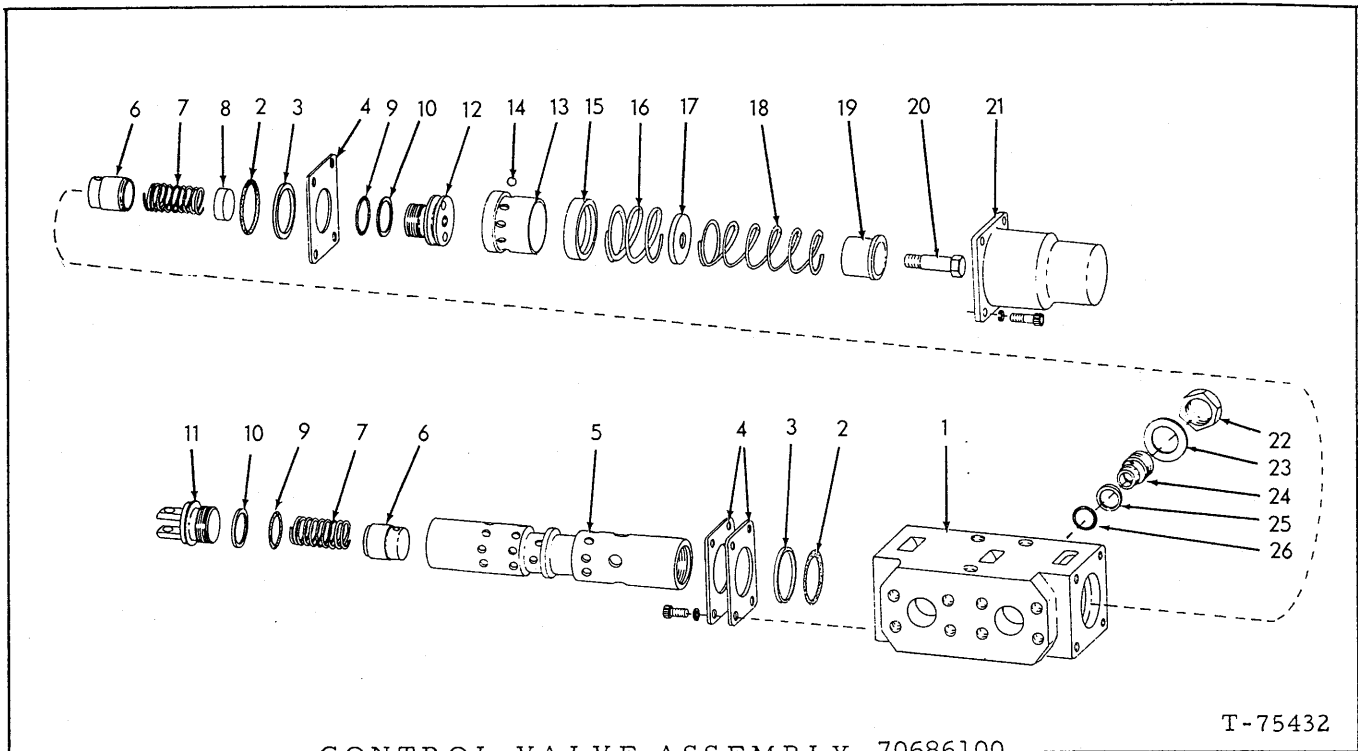
CONTROL VALVE ASSEMBLY 70686100
