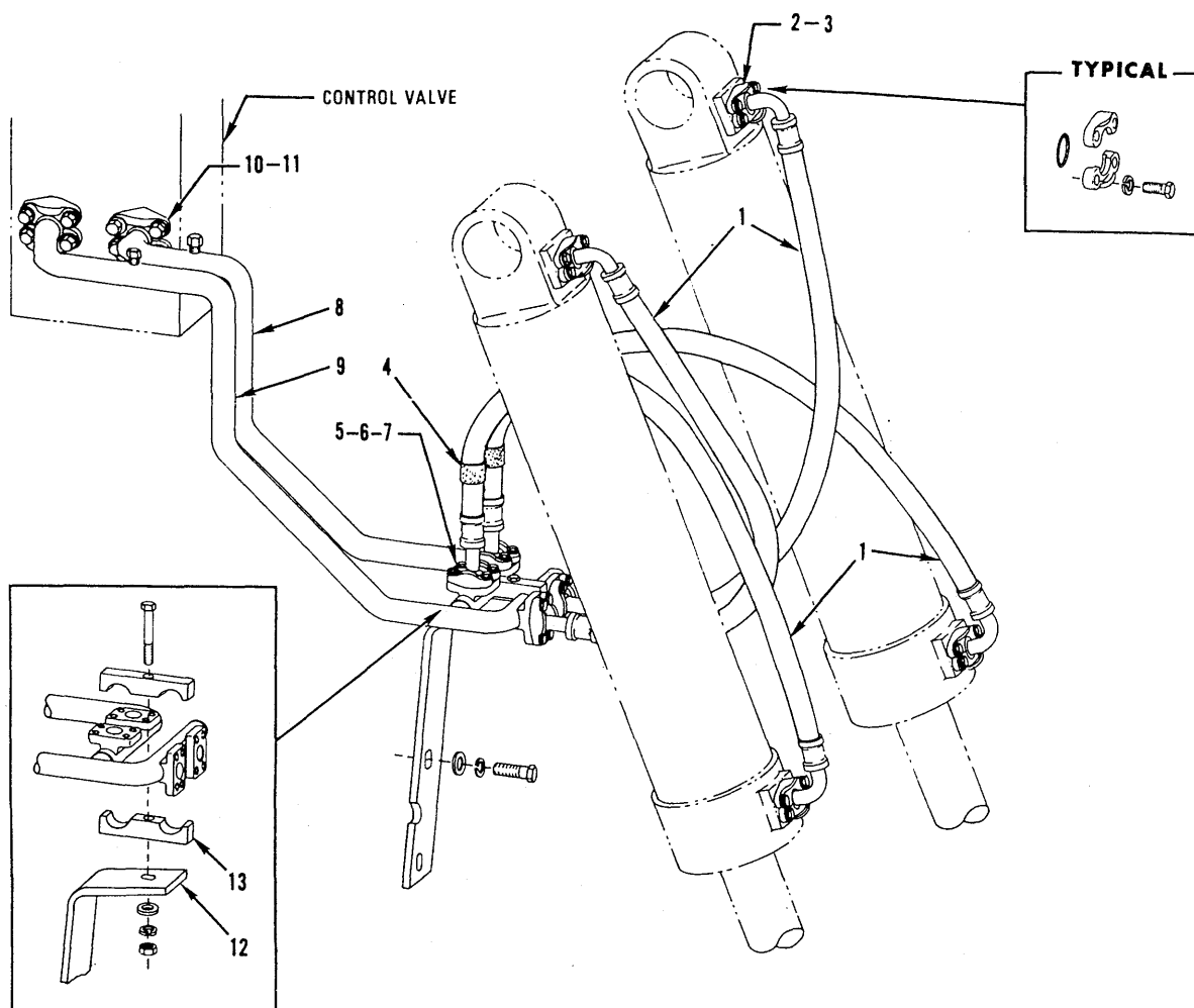
RIPPER PIPING
