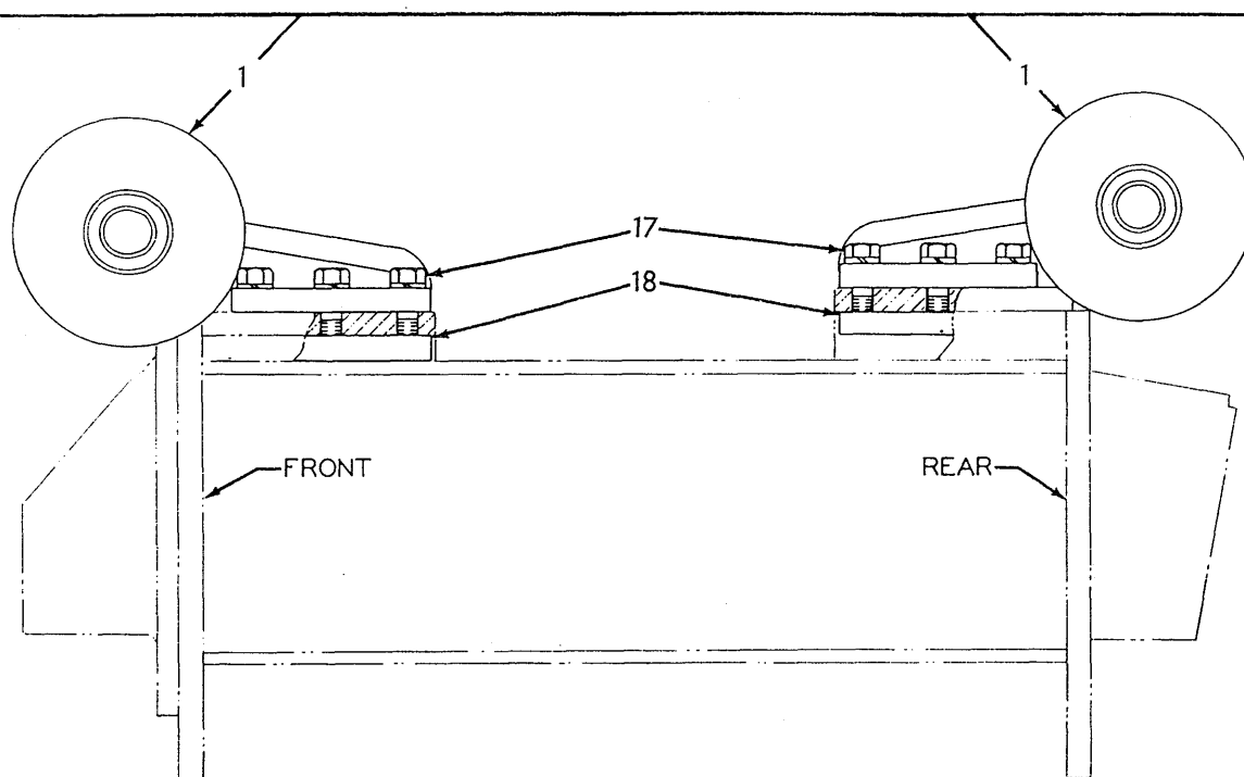
TRACK CARRIER ROLLER
