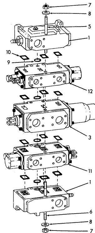
VALVE ASSY 70662085
