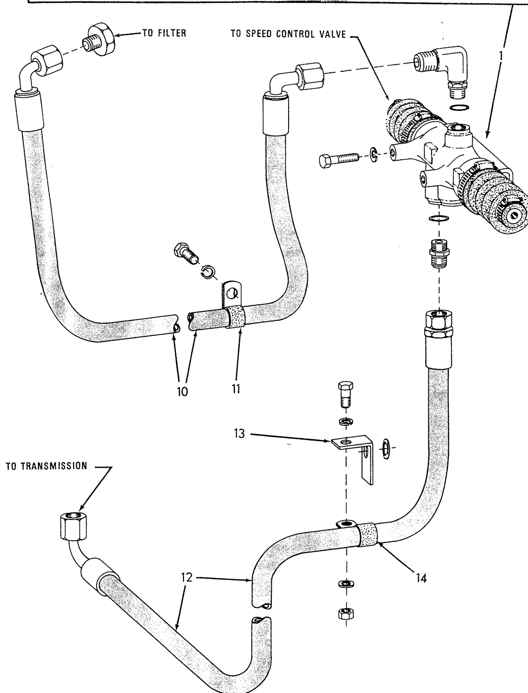
AUTOMATIC SAFETY BRAKE VALVE AND LINES
