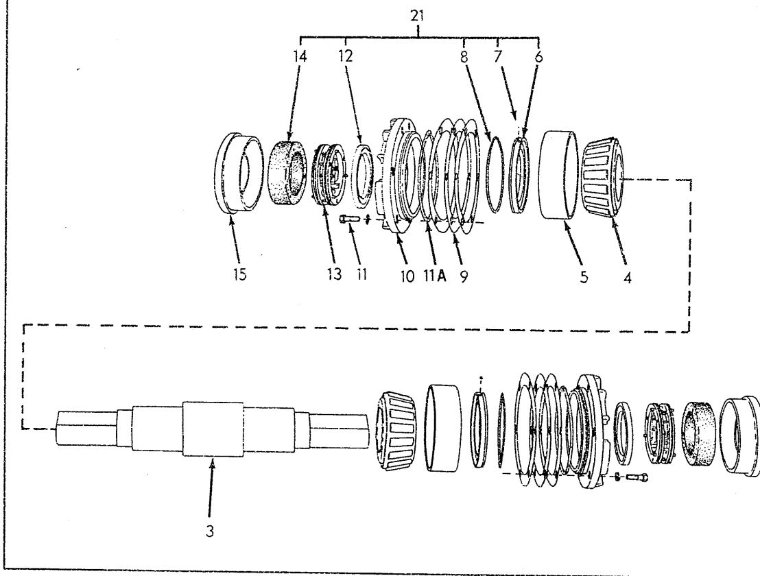
TRACK ROLLERS (First type)
