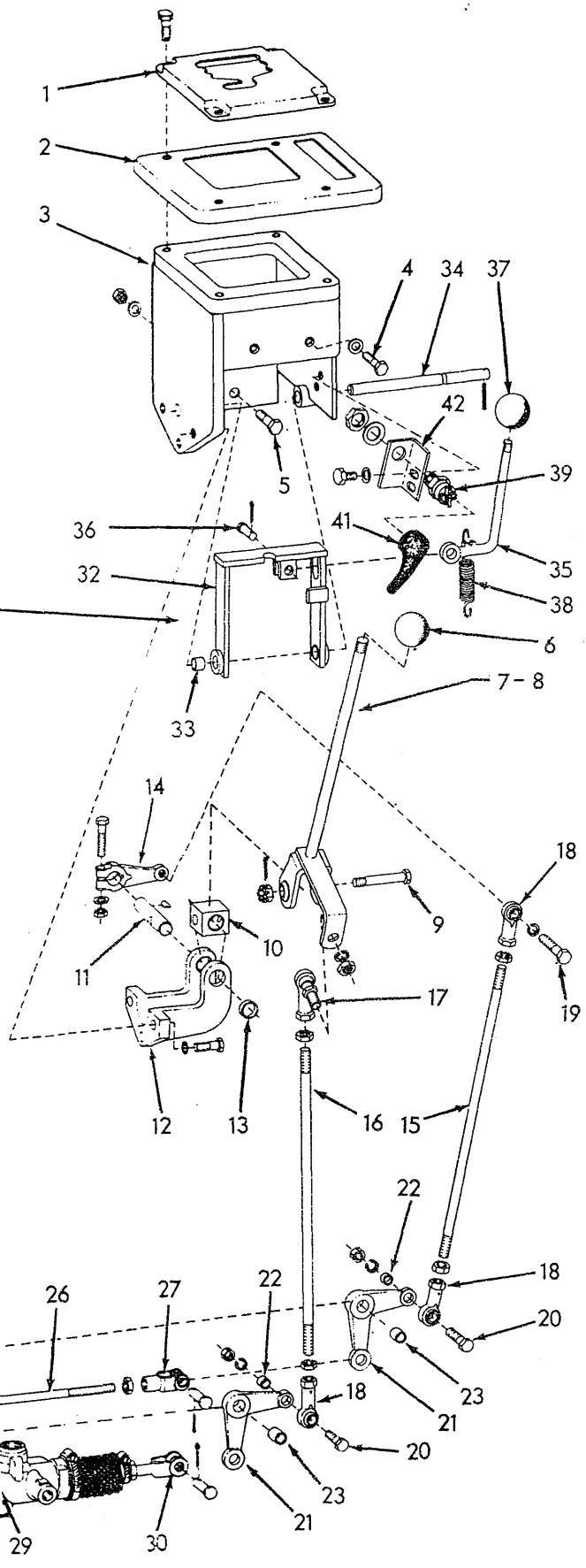
SPEED CONTROL LINKAGE
