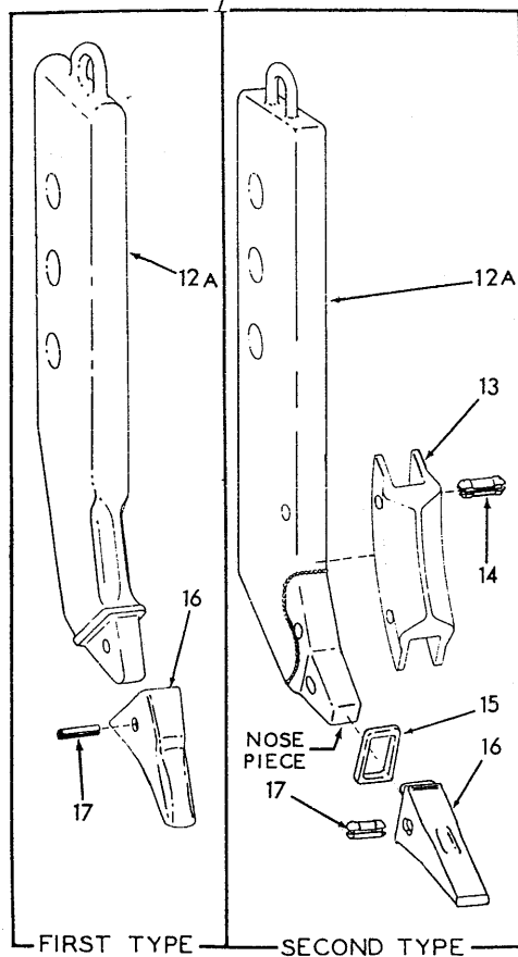
RIPPER TOOL BAR AND LINKAGE
