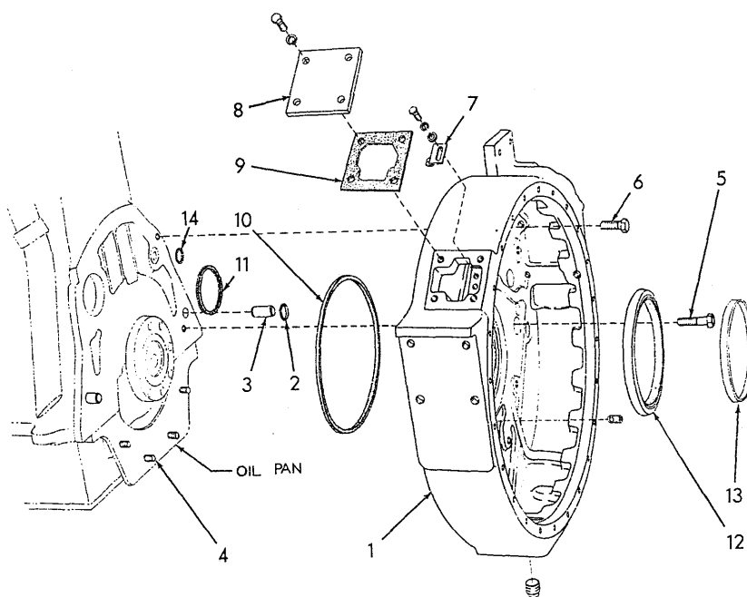
FLYWHEEL HOUSING
