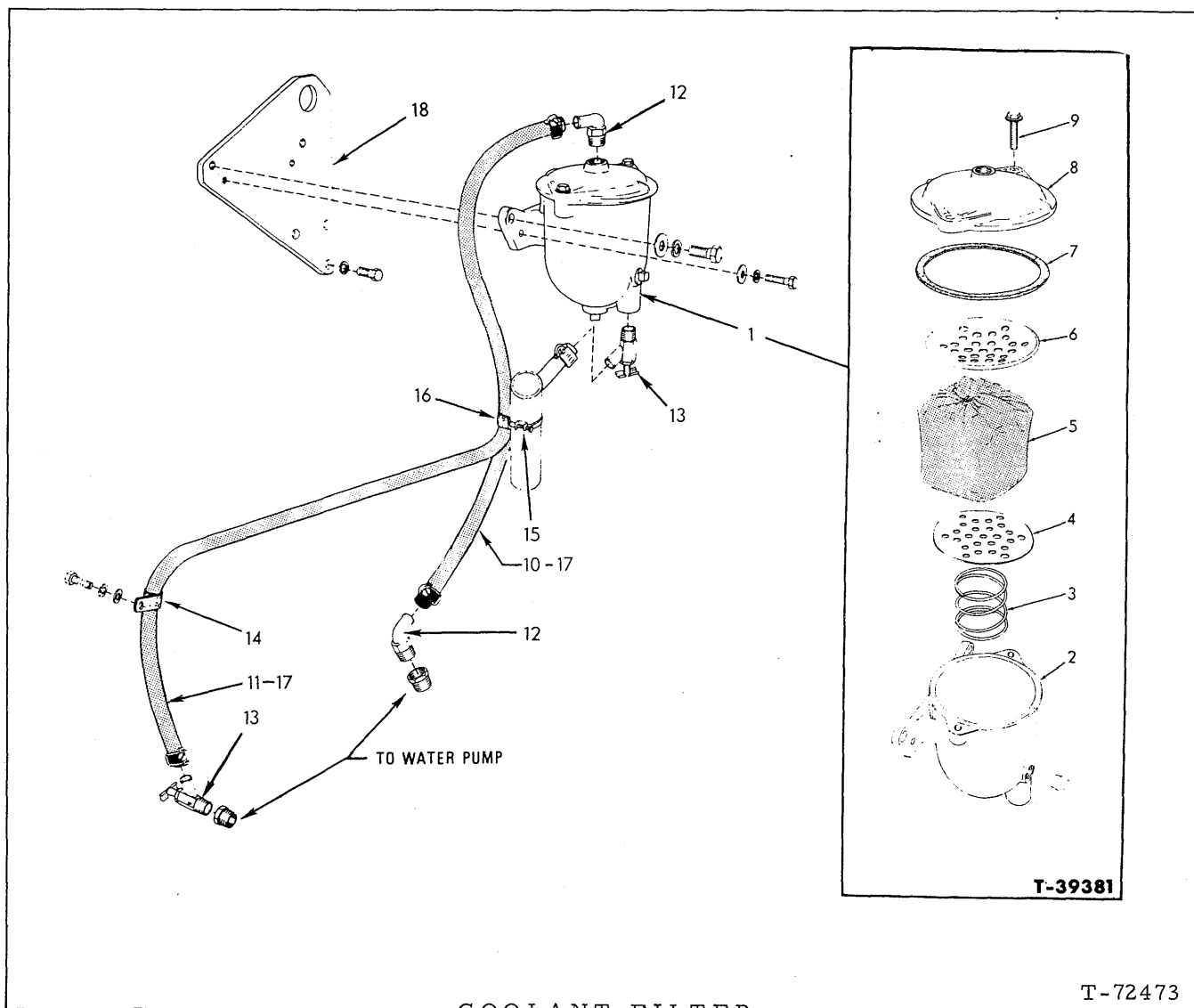
COOLANT FILTER
