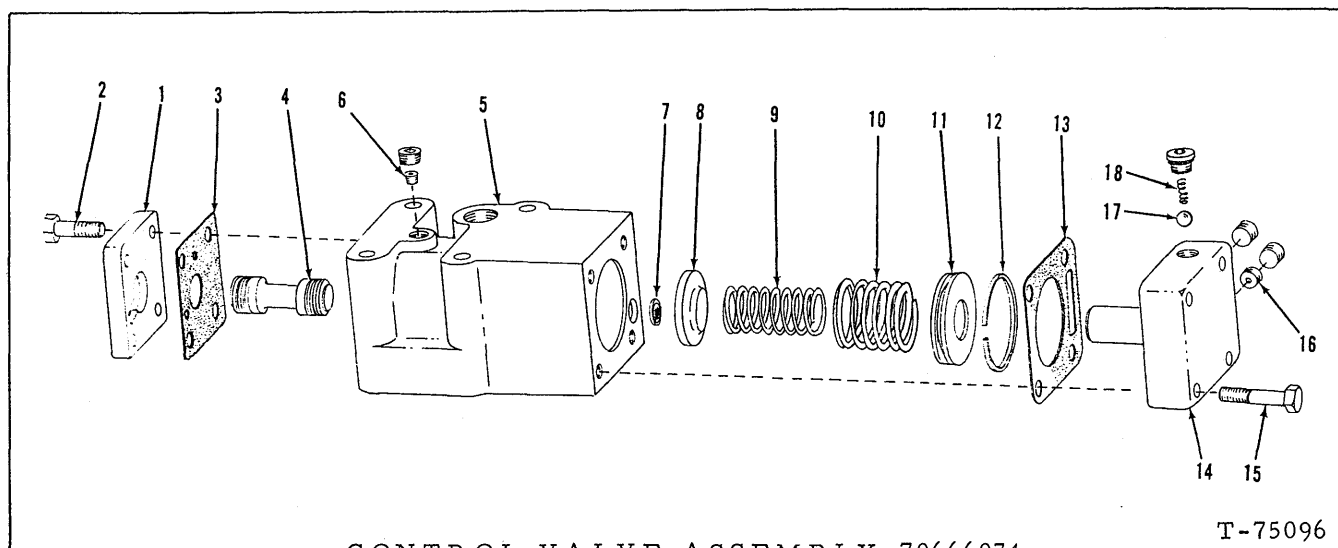
CONTROL VALVE ASSEMBLY 70666074
