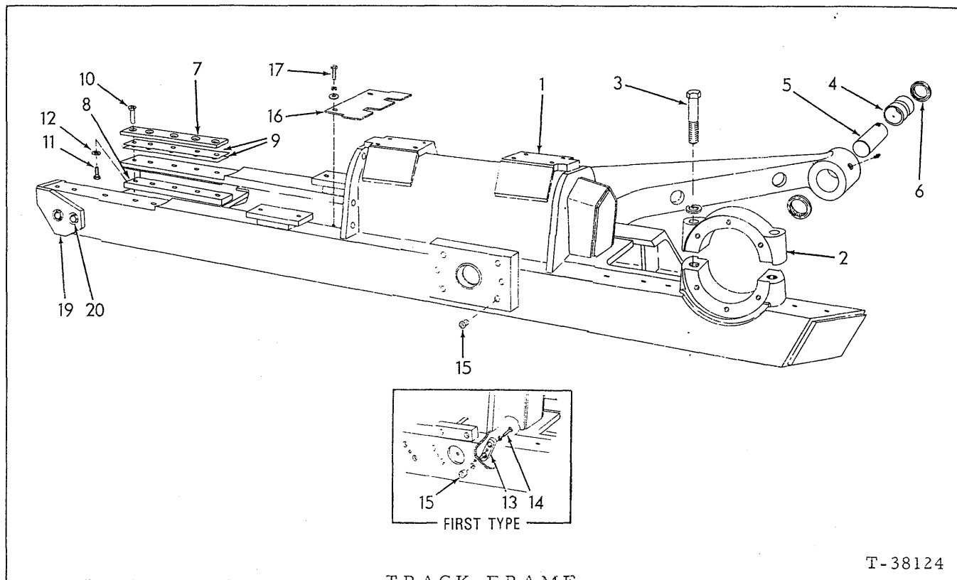
— TRACK FRAME —
