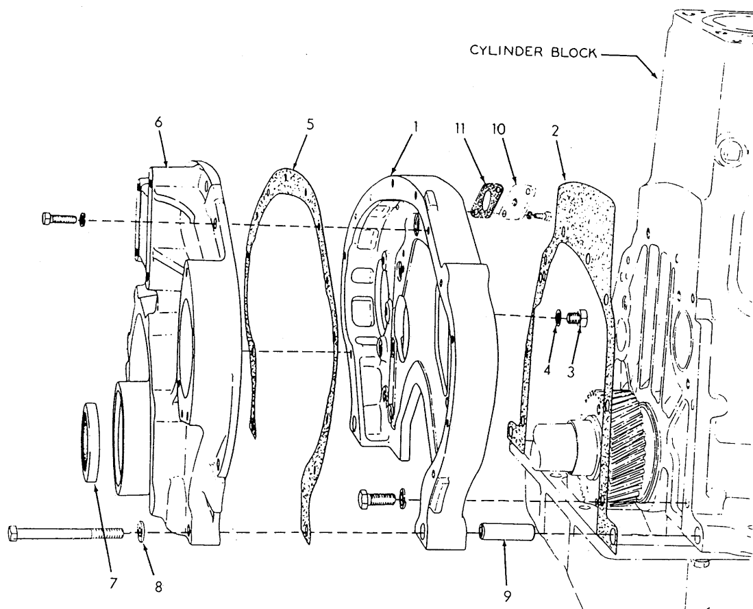
TIMING GEAR HOUSING
