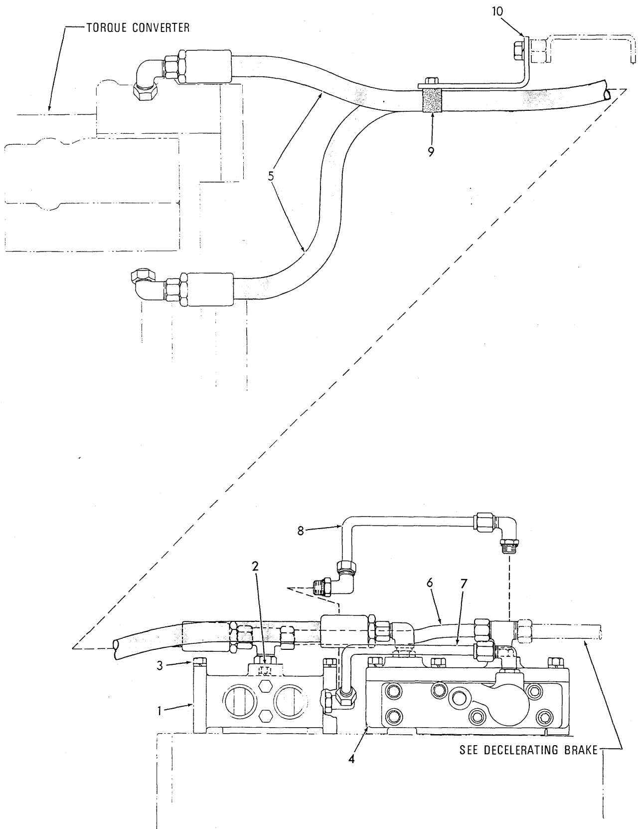
SPEED CONTROL VALVES AND LINES
