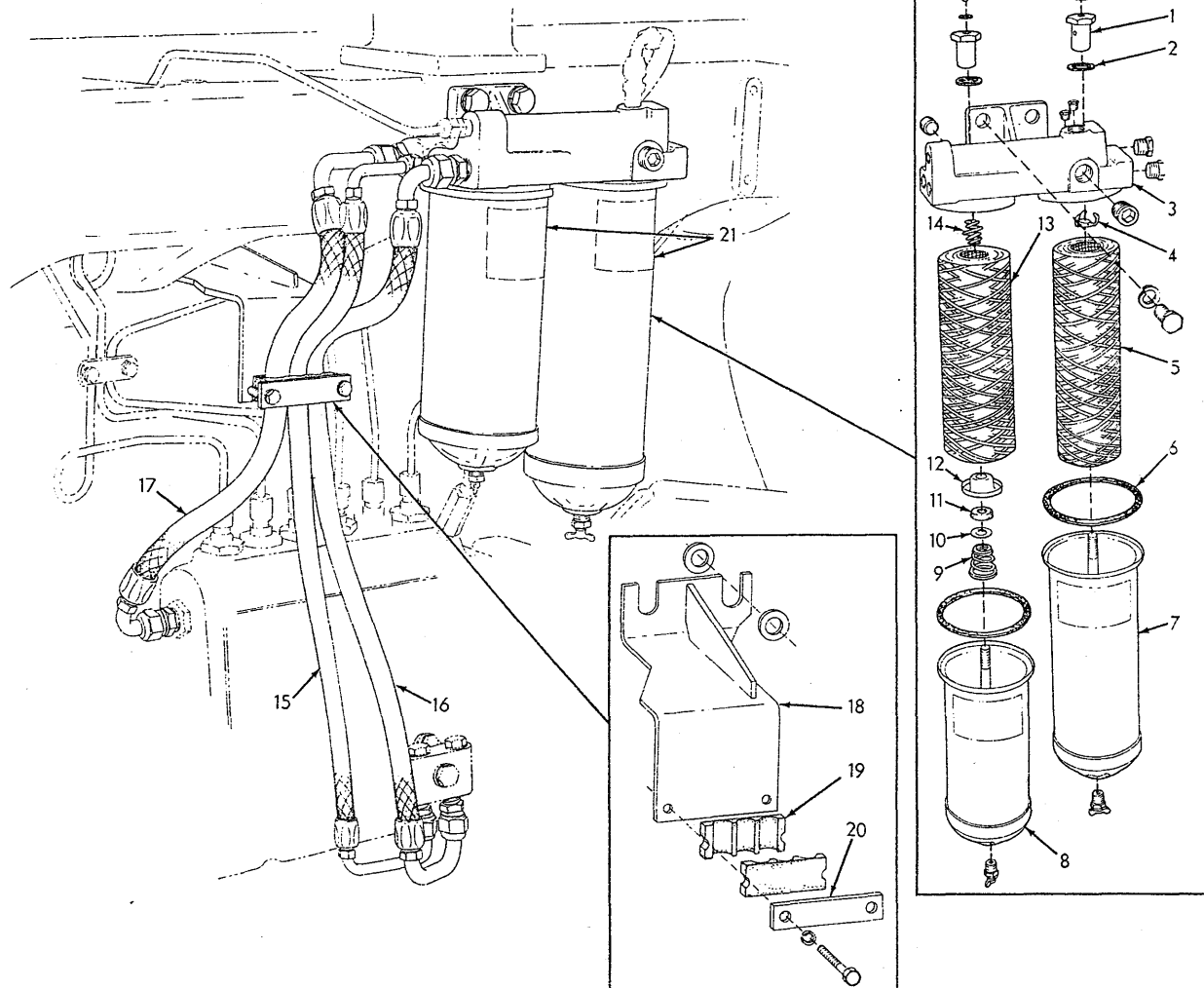
FUEL FILTER
