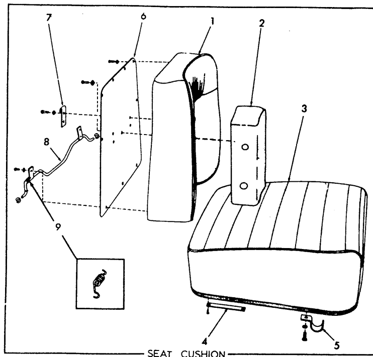
SEAT ASSEMBLY
