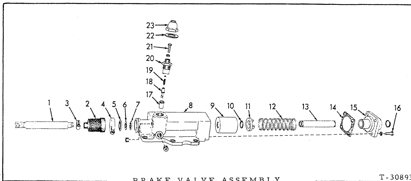
BRAKE VALVE ASSEMBLY
