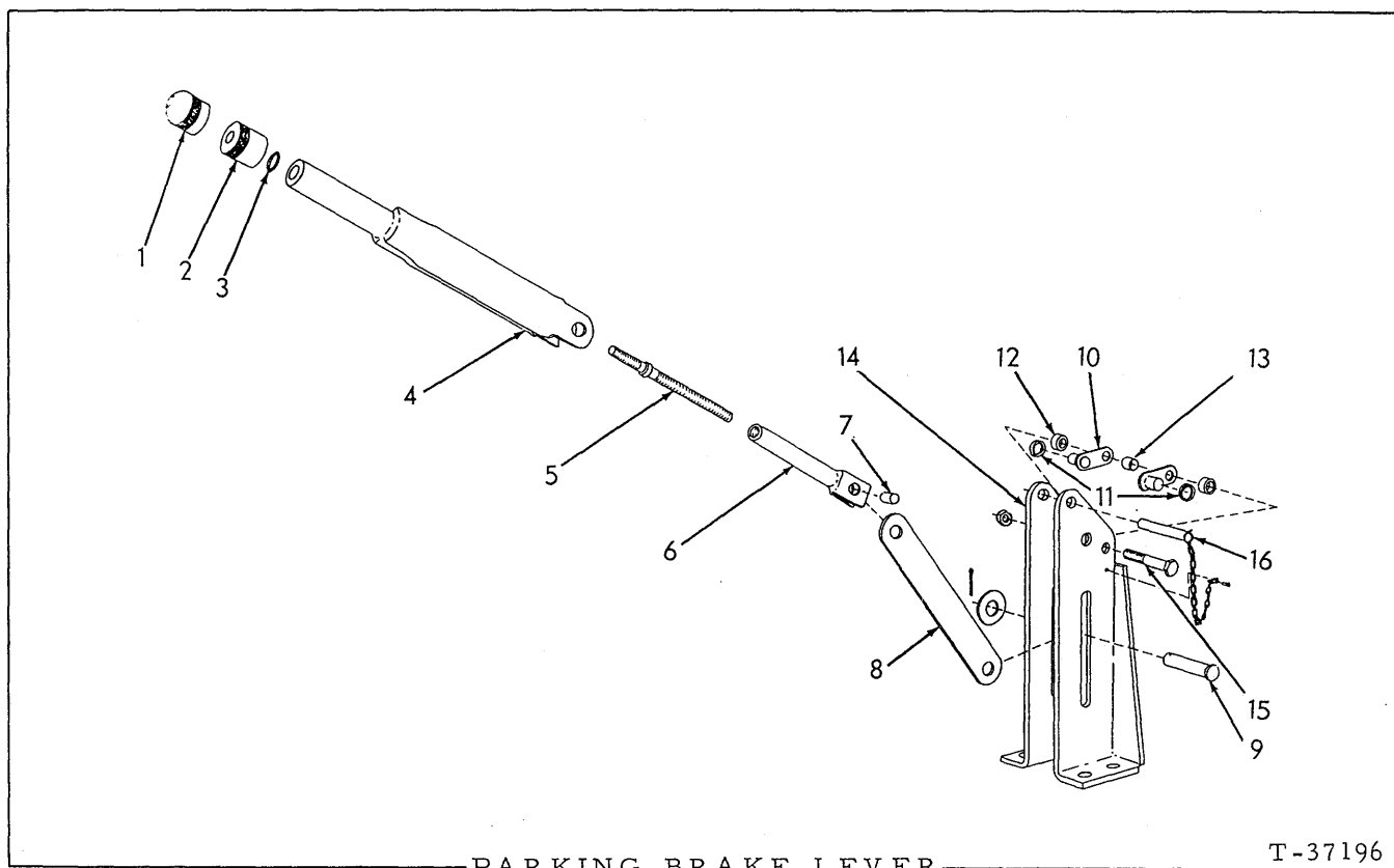
PARKING BRAKE LEVER
