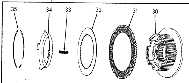
CLUTCH AND SHAFT ASSEMBLY 73118867
