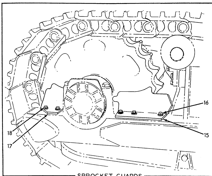
SPROCKET GUARDS
