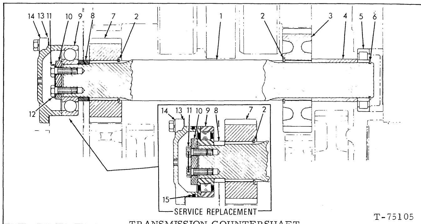
TRANSMISSION COUNTERSHAFT
