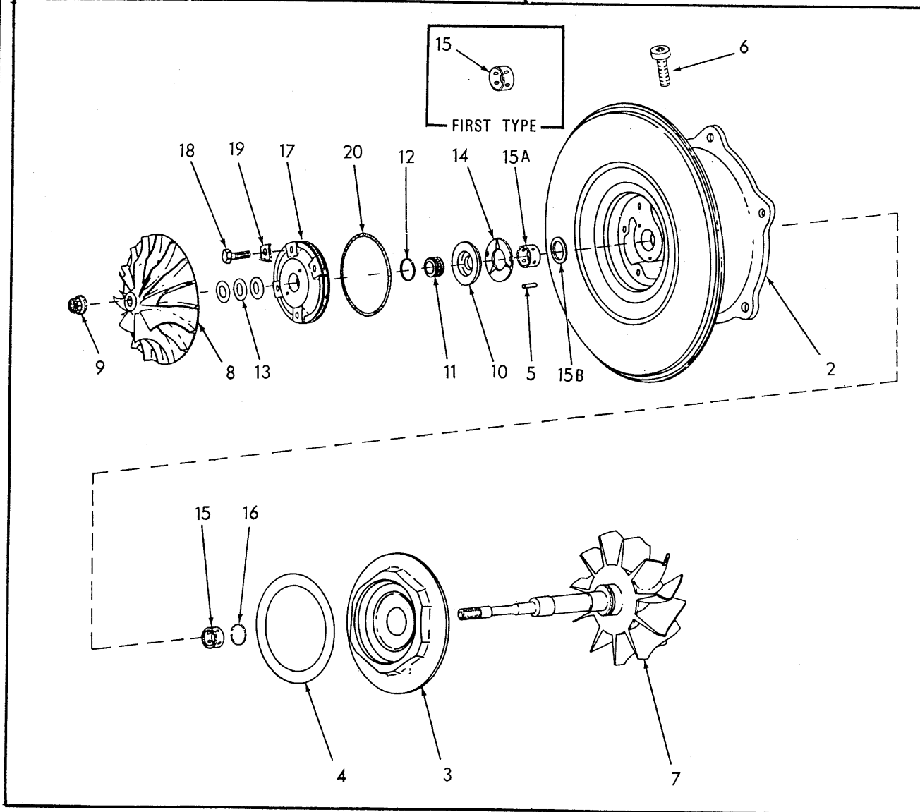
TURBOCHARGER ASSEMBLY (First Type)
