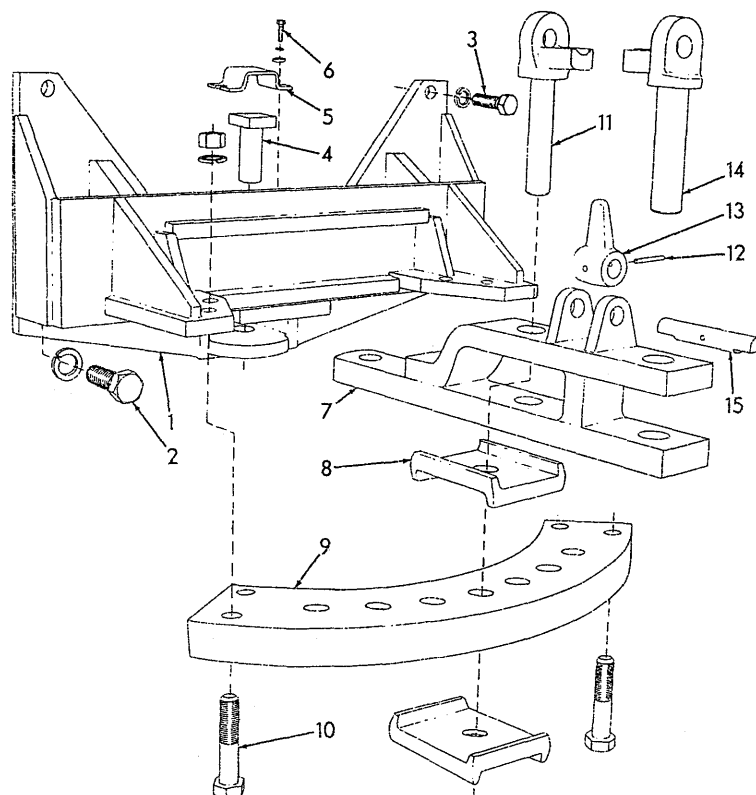
SWINGING DRAWBAR
