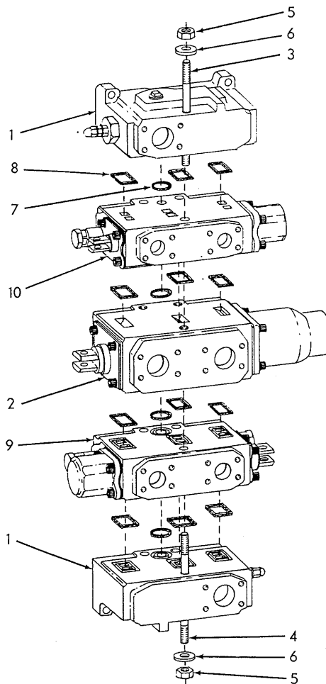
VALVE ASSY. 70686070
