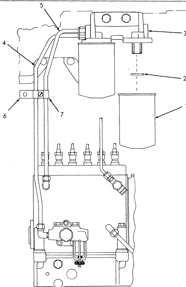
FUEL FILTER
