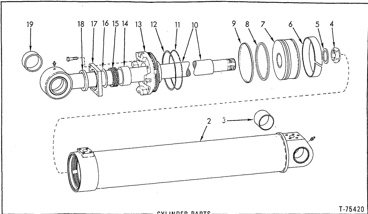
— CYLINDER PARTS —
