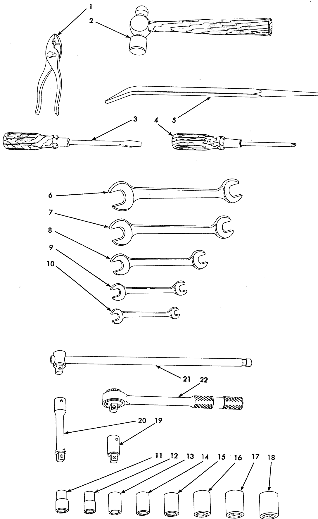
SPECIAL TOOLS
