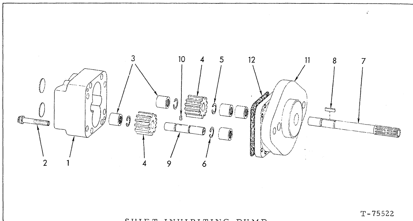
SHIFT INHIBITING PUMP
