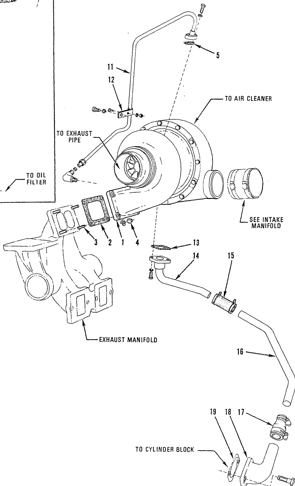
TURBOCHARGER
