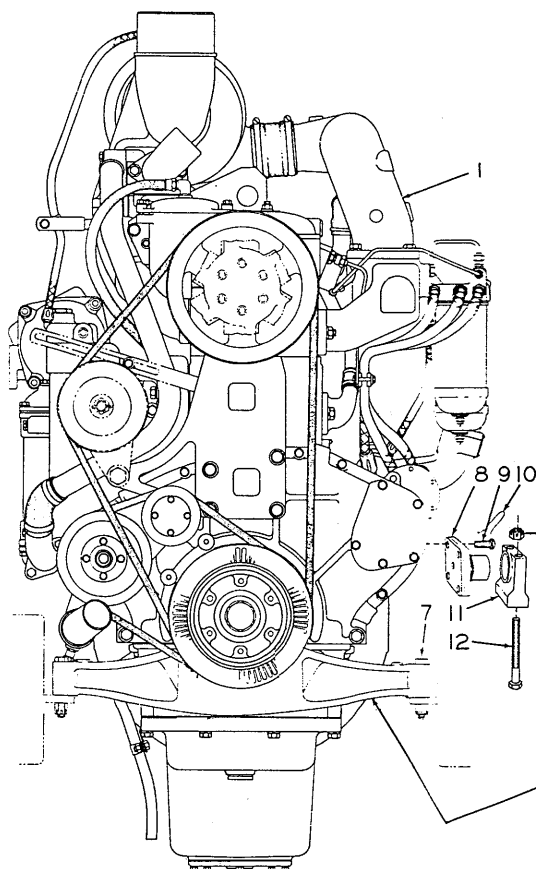
ENGINE AND MOUNTING
