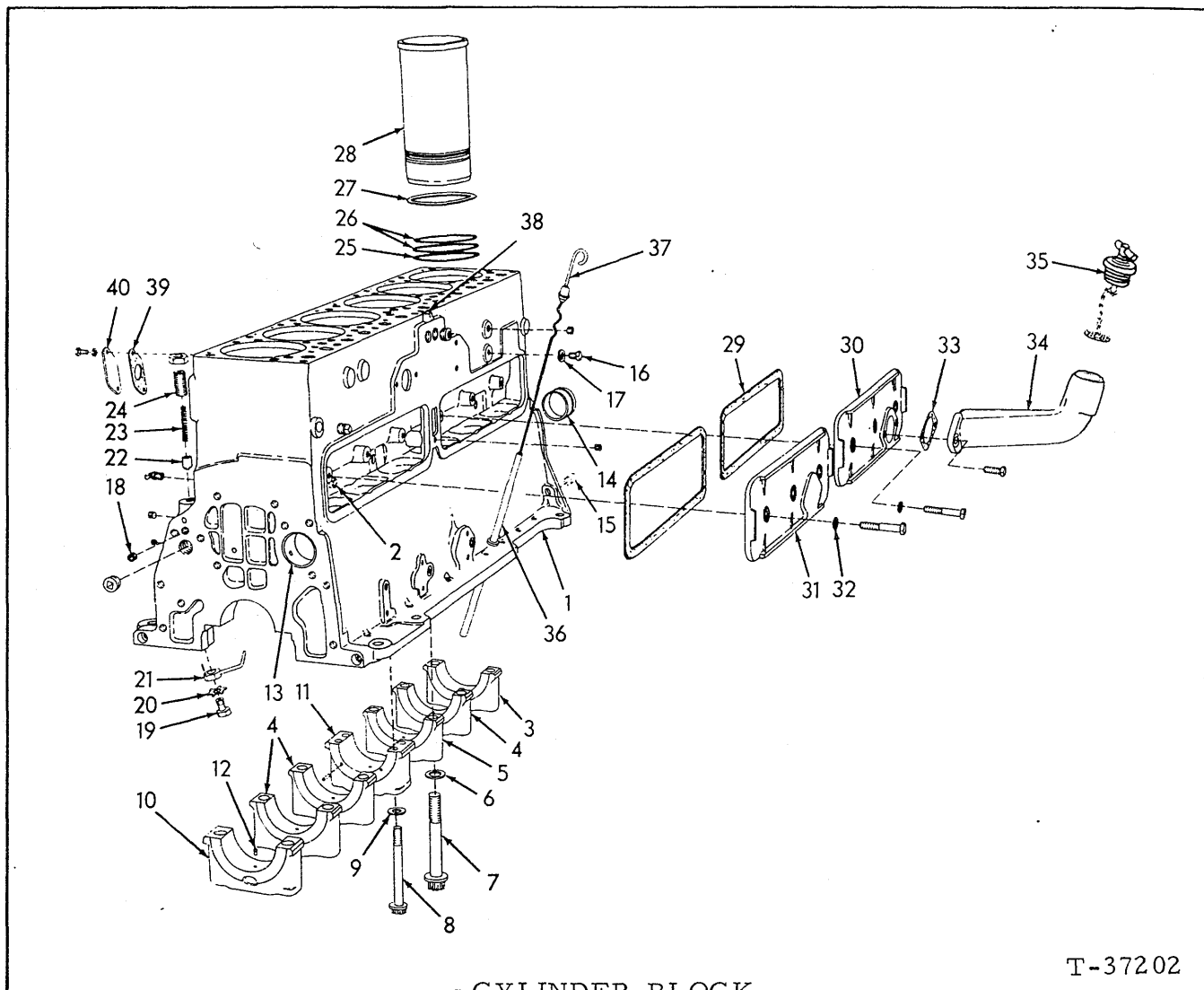
CYLINDER BLOCK
