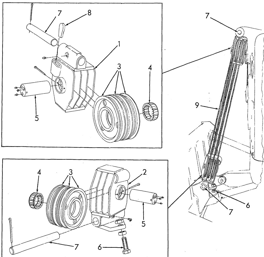
SHEAVE BLOCKS AND CABLE
