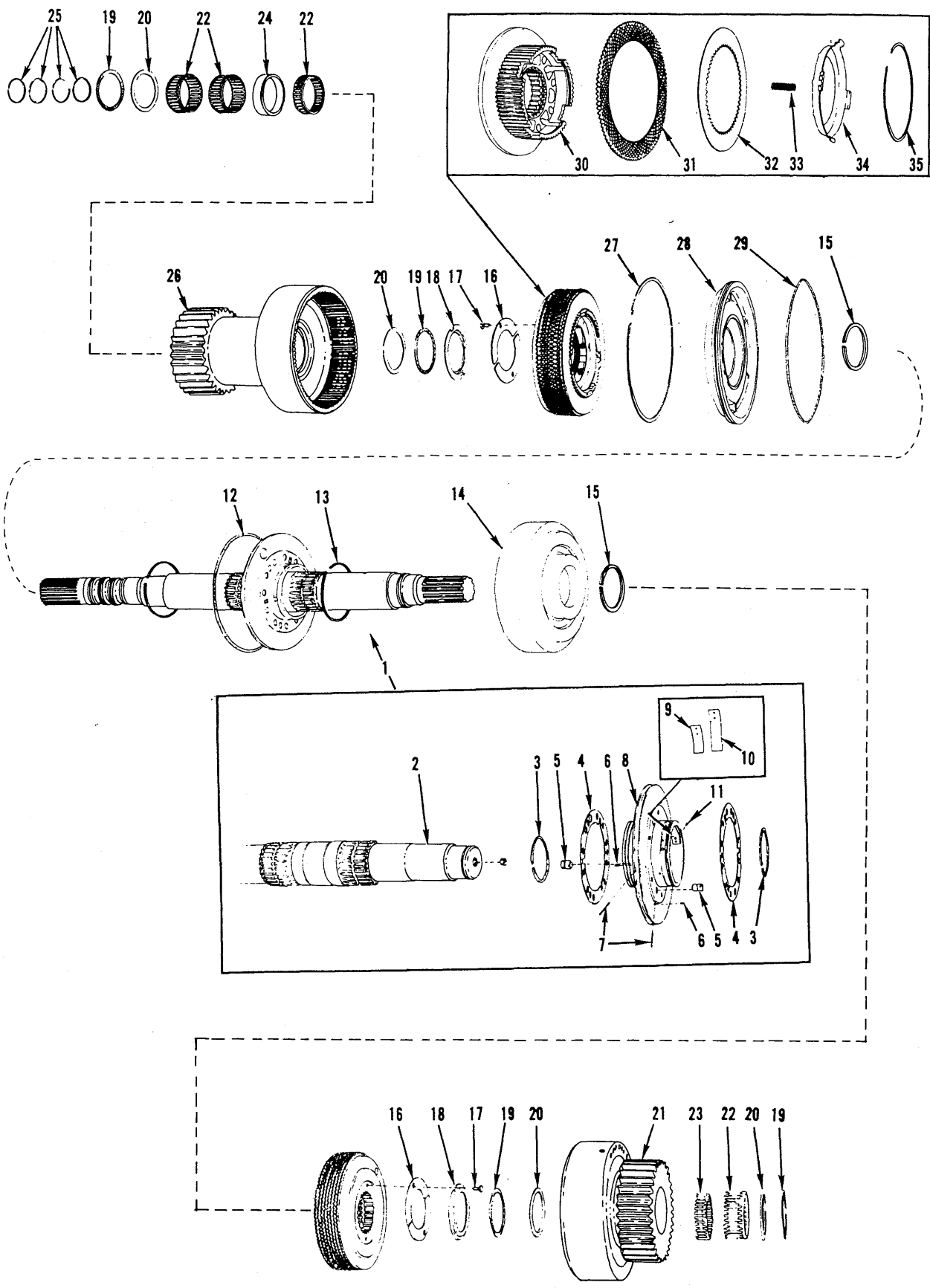
CLUTCH AND SHAFT ASSEMBLY 73118869
