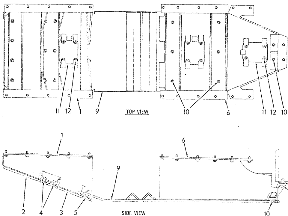
BOTTOM GUARDS
