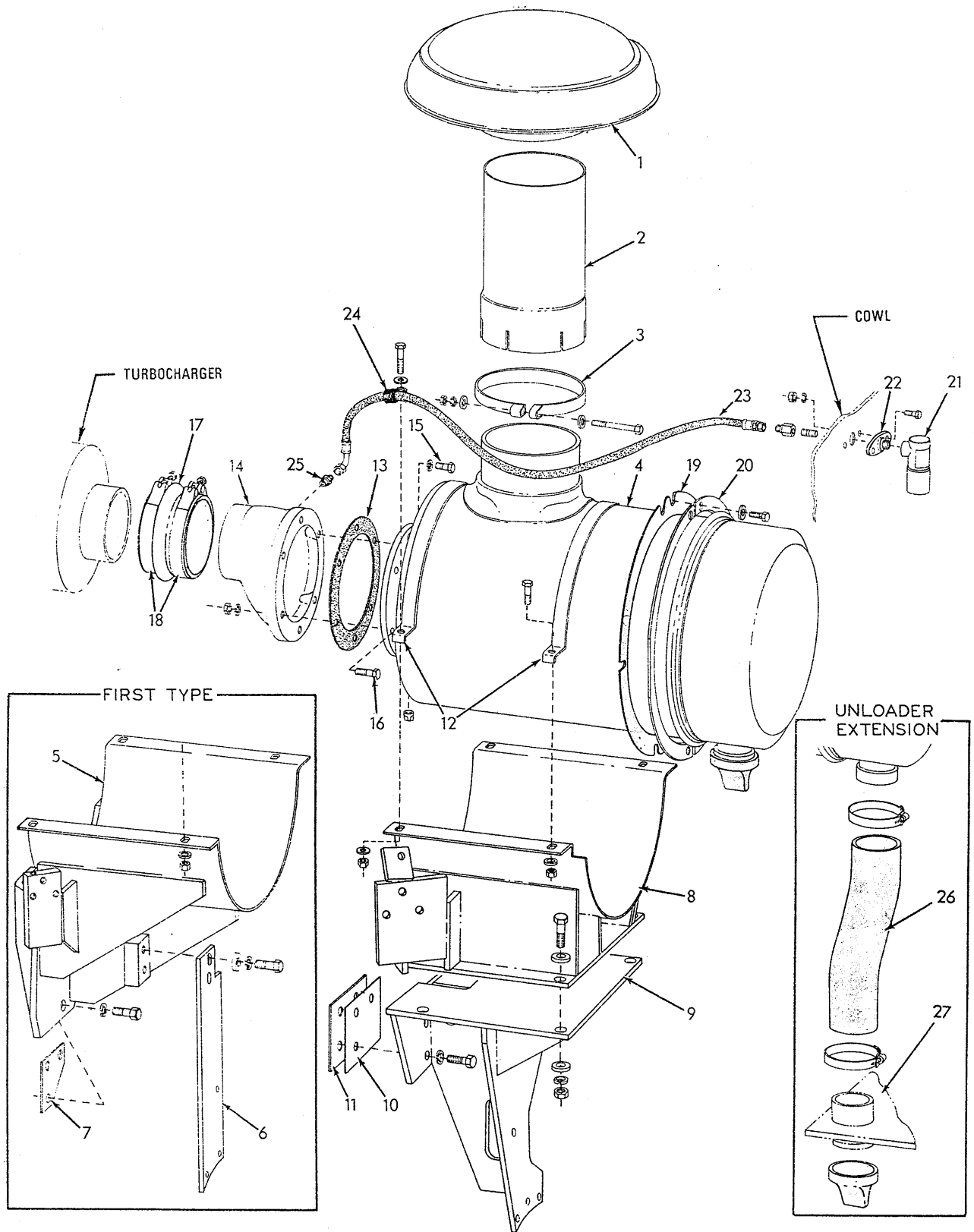
AIR CLEANER (Dry-type)
