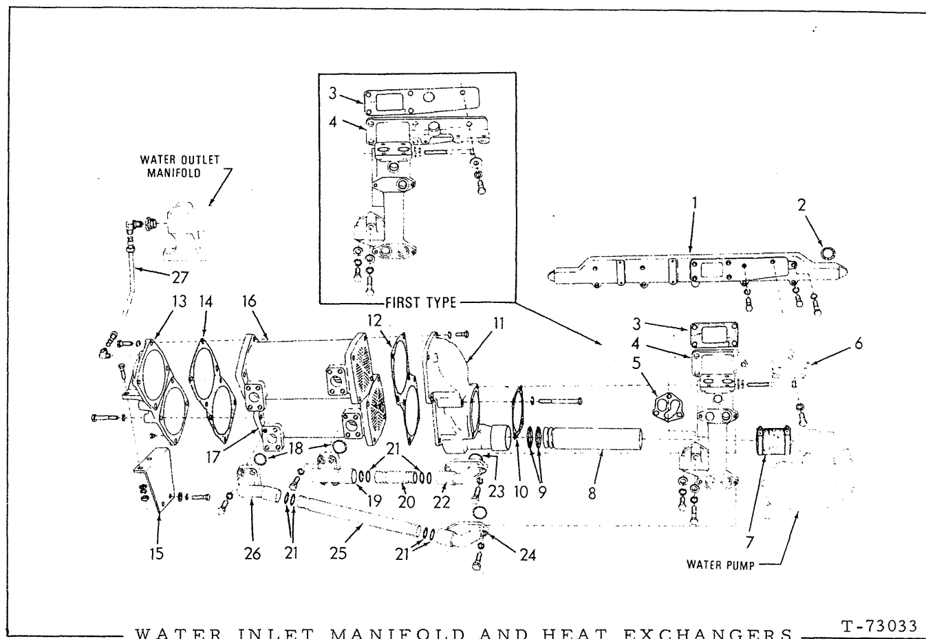
WATER INLET MANIFOLD AND HEAT EXCHANGERS
