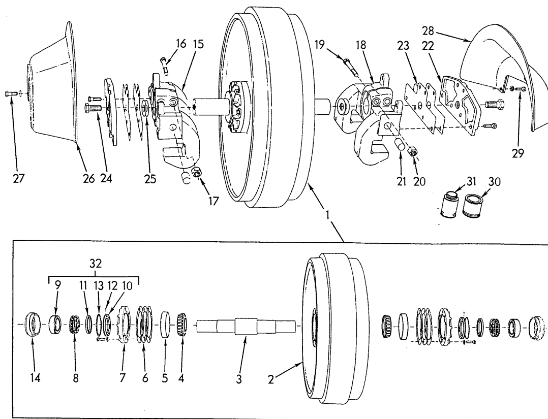
TRACK IDLER
