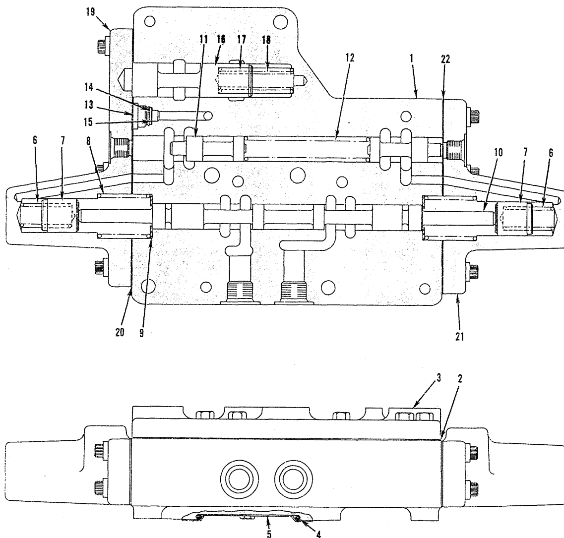
SHIFT INHIBITING VALVE ASSEMBLY 70662559
