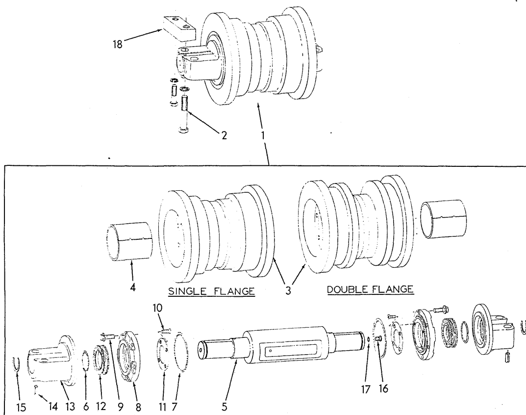
TRACK ROLLERS (Second Type)
