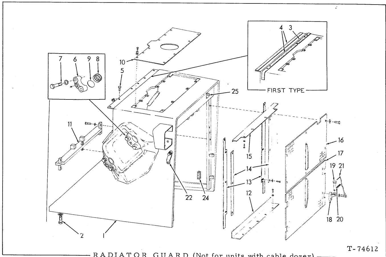
RADIATOR GUARD (Not for units with cable dozer)
