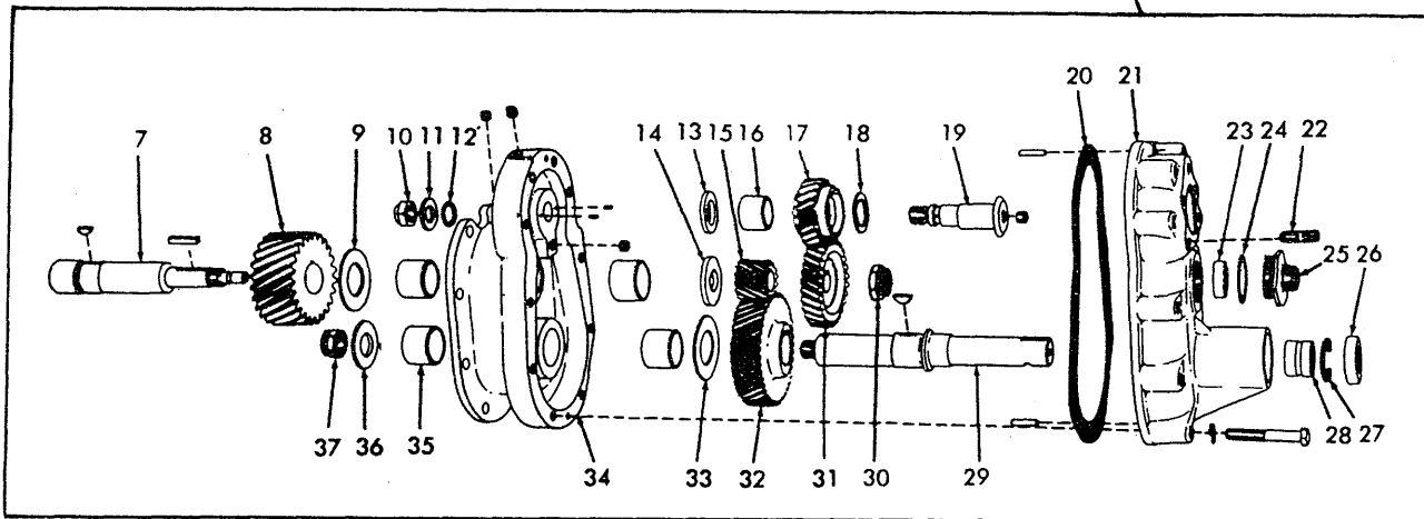
ACCESSORY DRIVE
