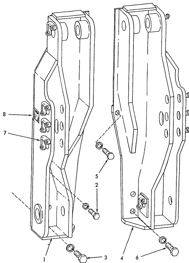
RIPPER MOUNTING FRAME
