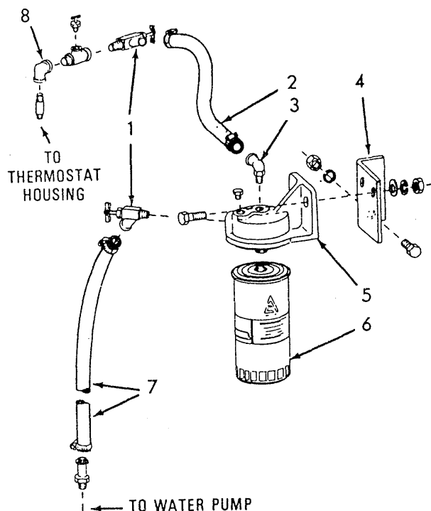
COOLANT FILTER
