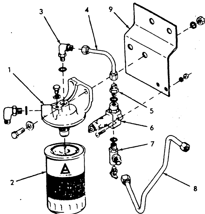
FUEL FILTER AND LINES
