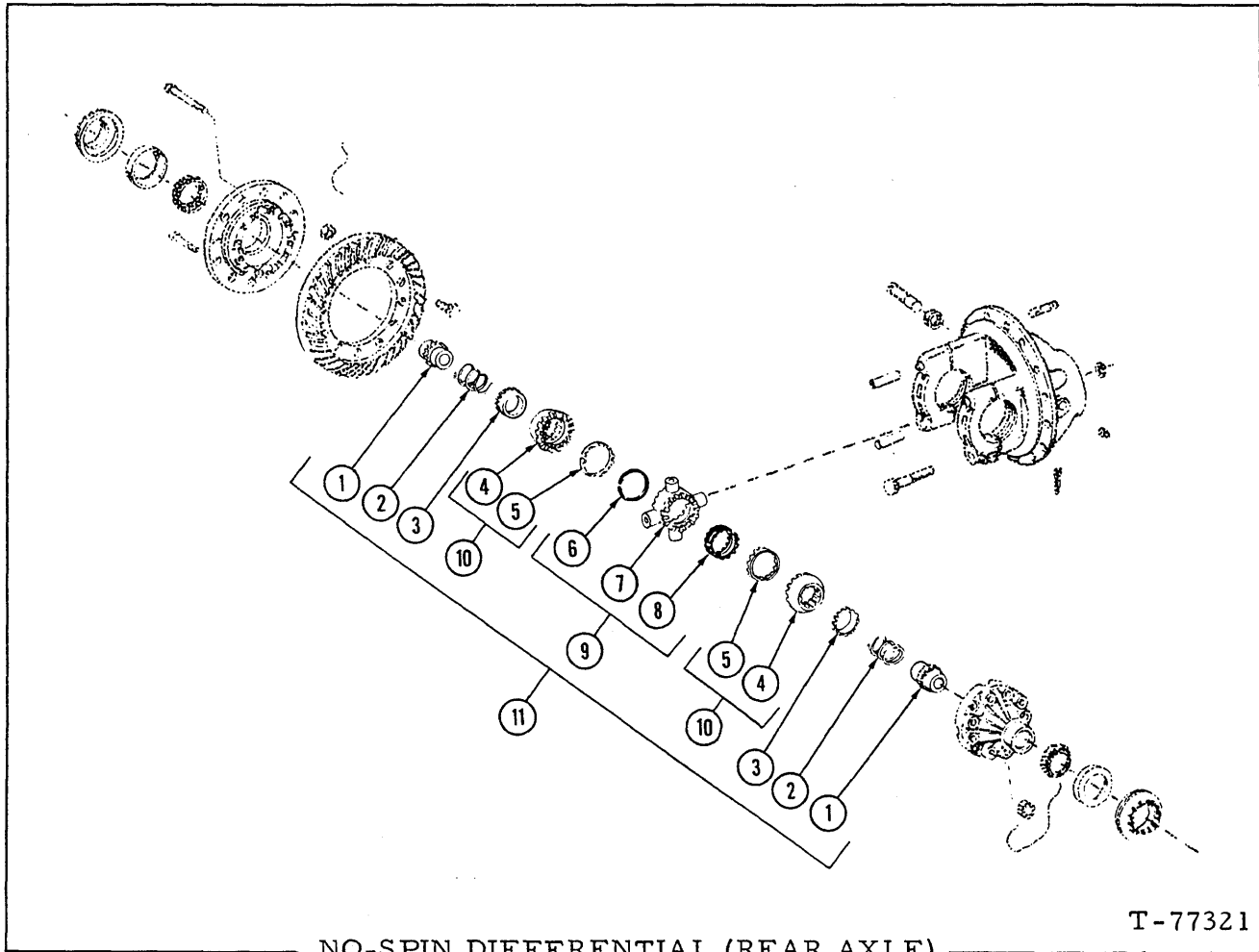
NO-SPIN DIFFERENTIAL (REAR AXLE)
