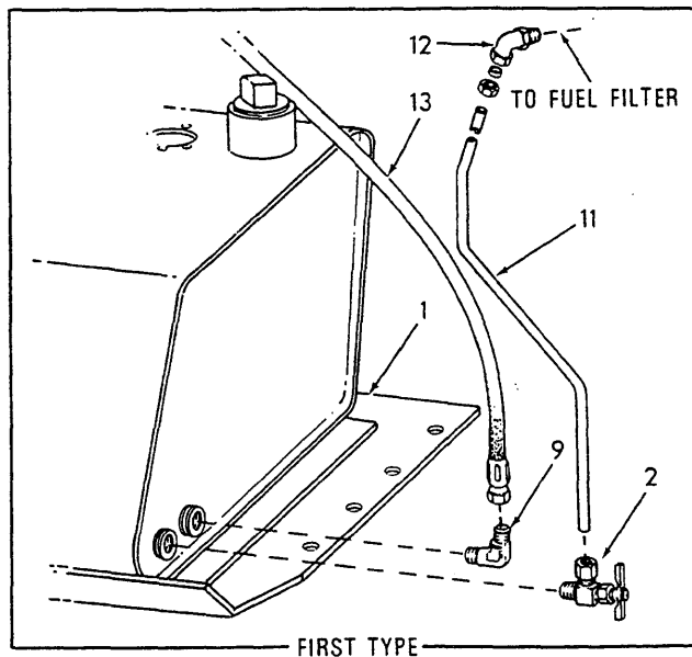
FUEL TANK GROUP
