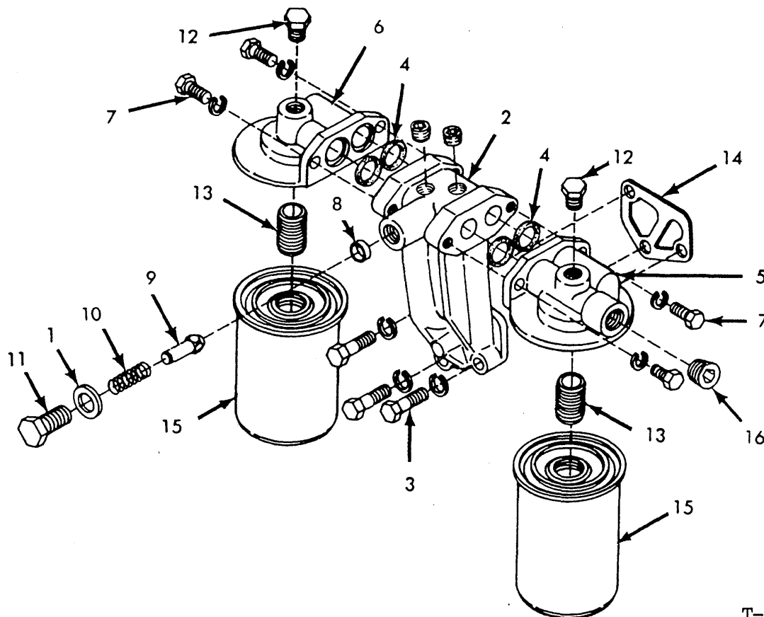
LUBE OIL FILTER
