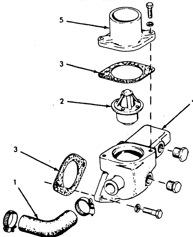
THERMOSTAT AND HOUSING
