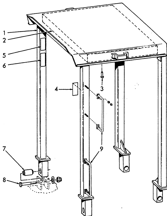
CANOPY ASSEMBLY (ROPS)
