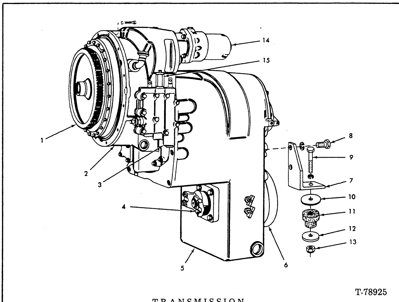
TRANSMISSION
