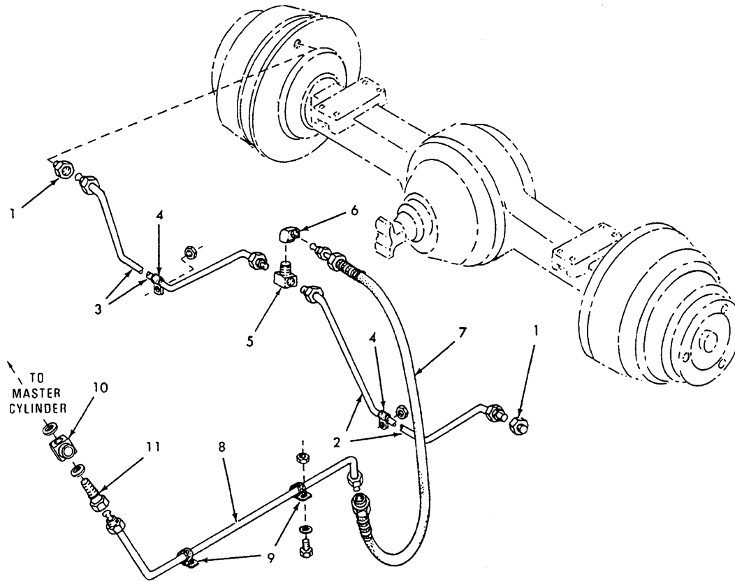
REAR BRAKE LINES
