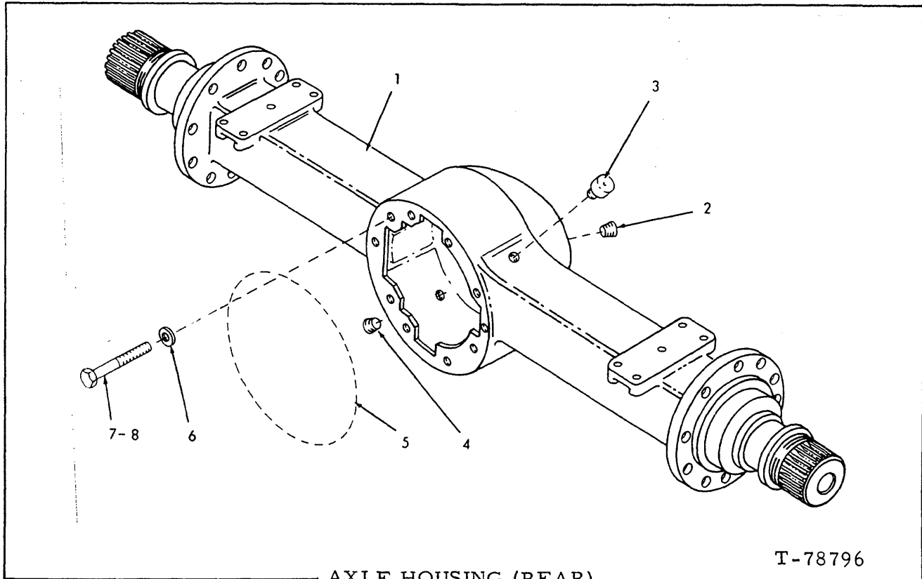
AXLE HOUSING (REAR)
