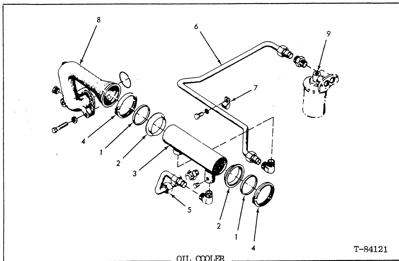
OIL COOLER
