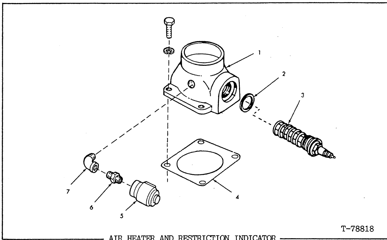
AIR HEATER AND RESTRICTION INDICATOR
