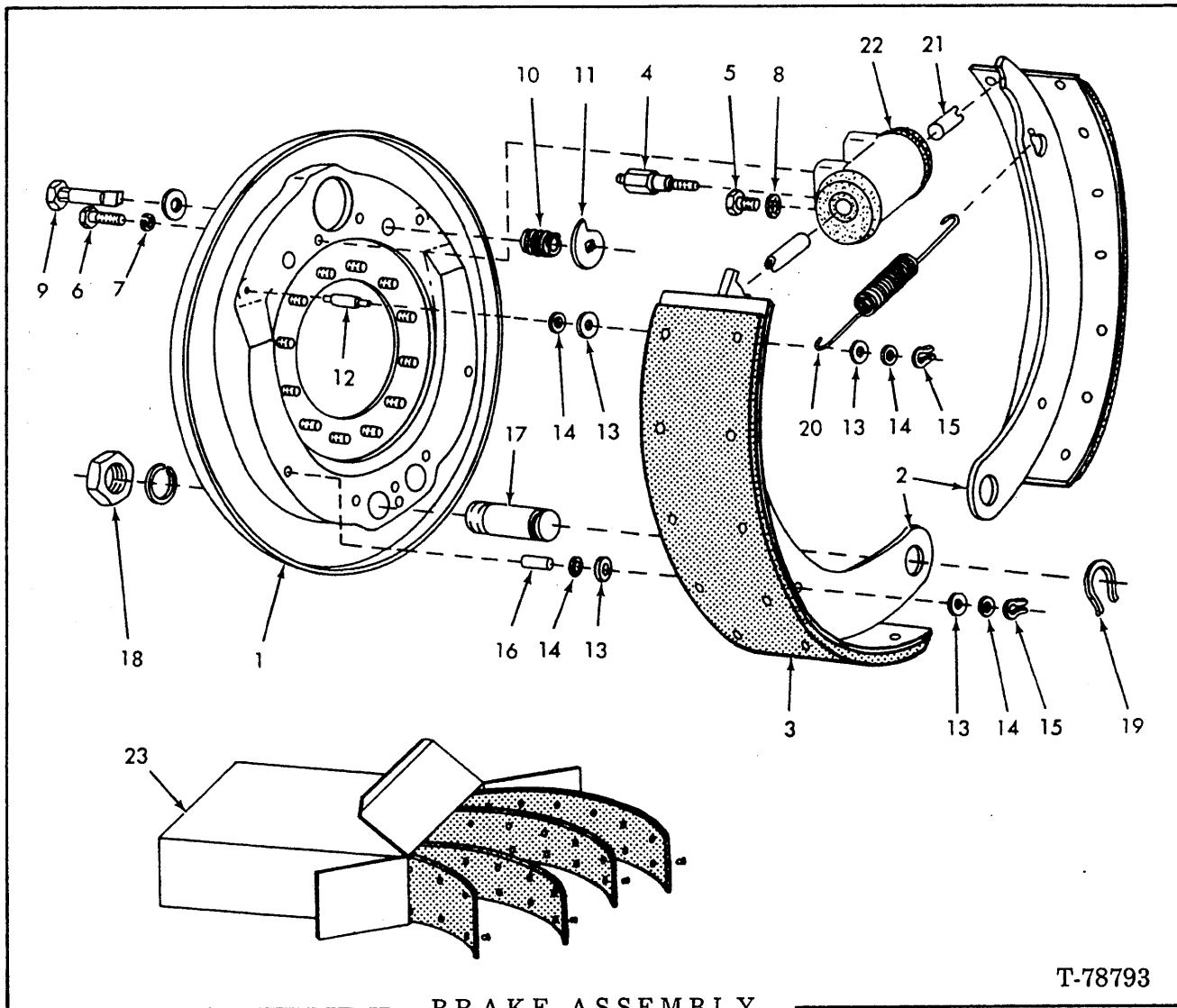
BRAKE ASSEMBLY
