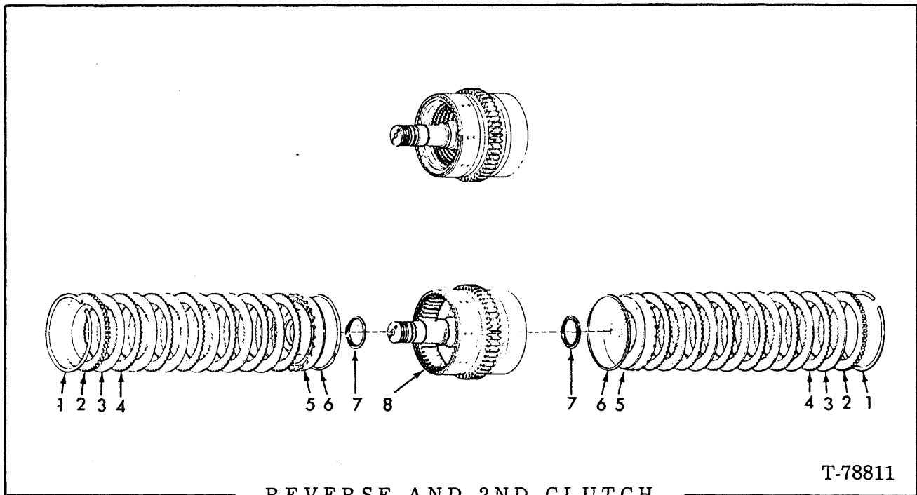
REVERSE AND 2ND CLUTCH
