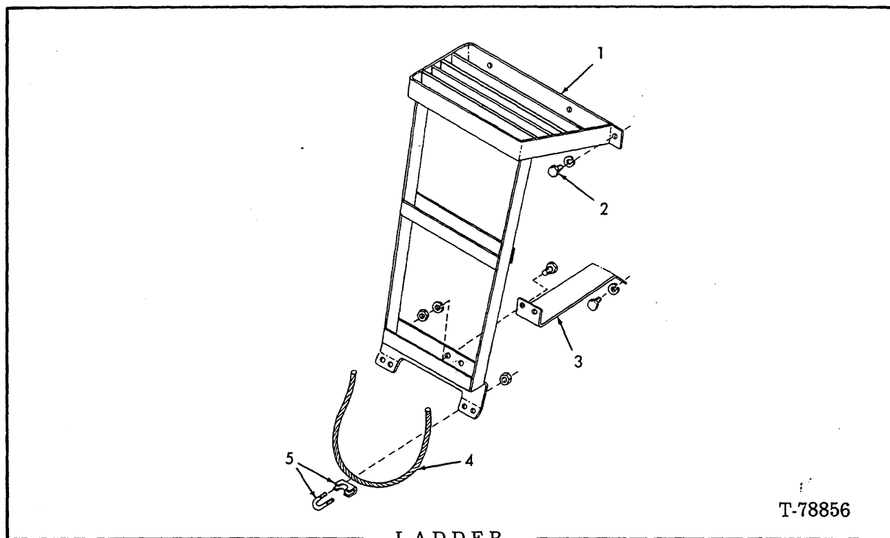
LADDER
