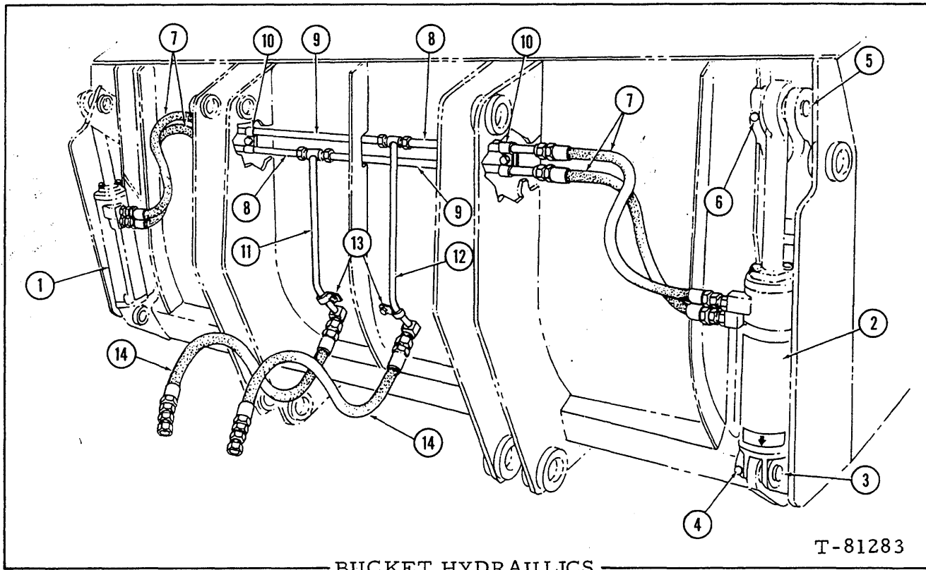
BUCKET HYDRAULICS
