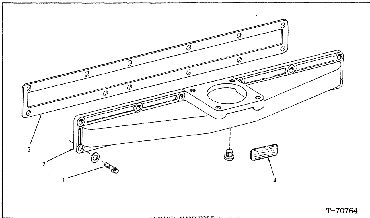
INTAKE MANIFOLD
