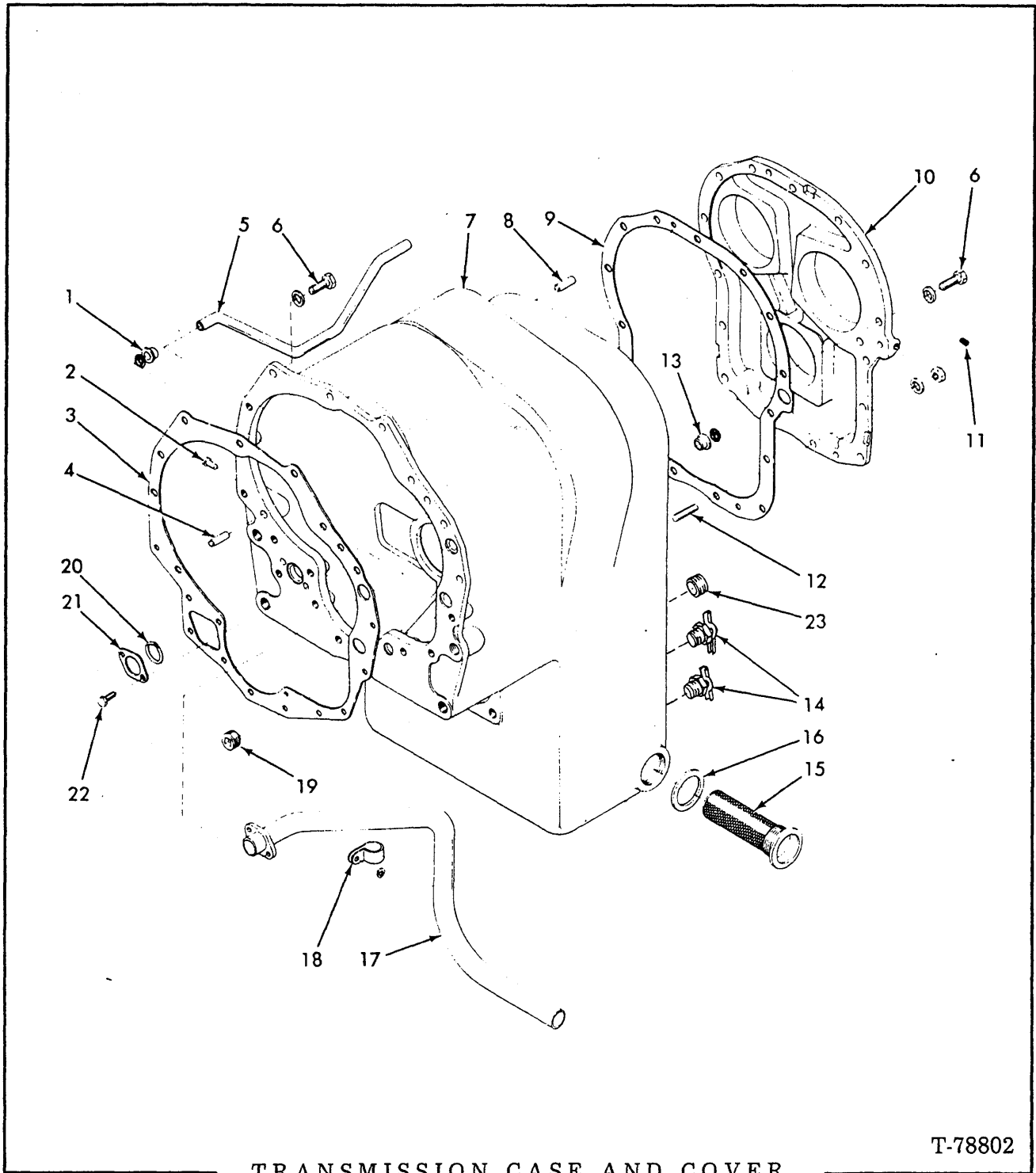
TRANSMISSION CASE AND COVER
