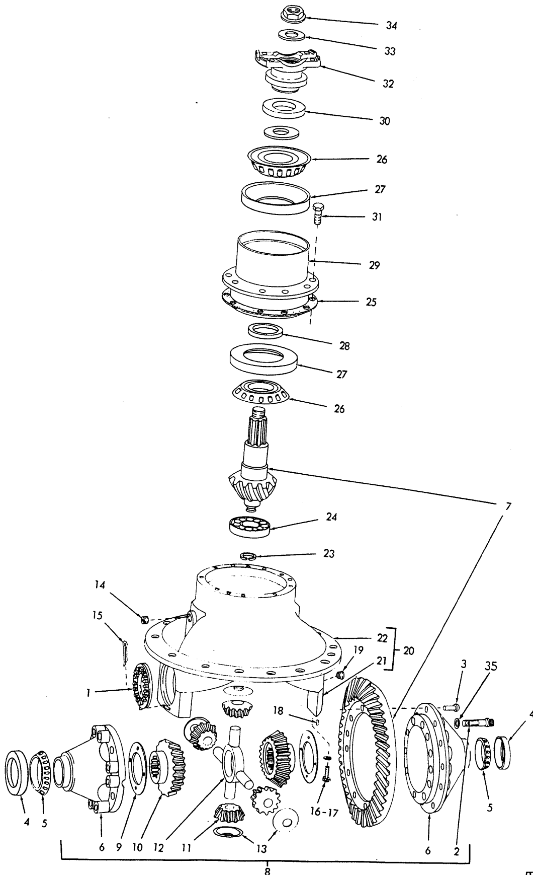
DIFFERENTIAL ASSEMBLY
