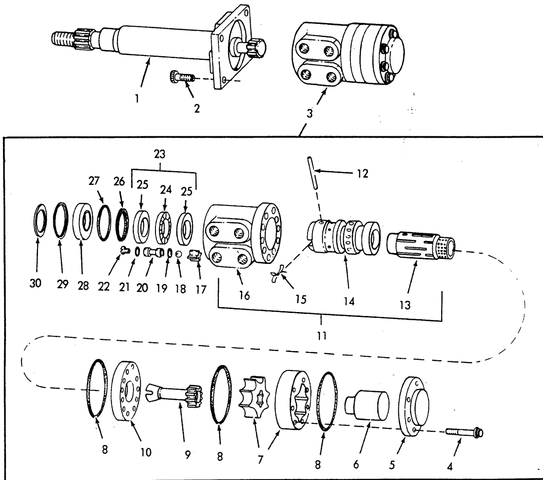
STEERING COLUMN AND VALVE ASSEMBLY
