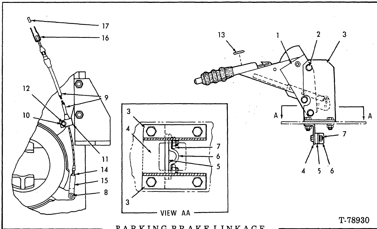
PARKING BRAKE LINKAGE
