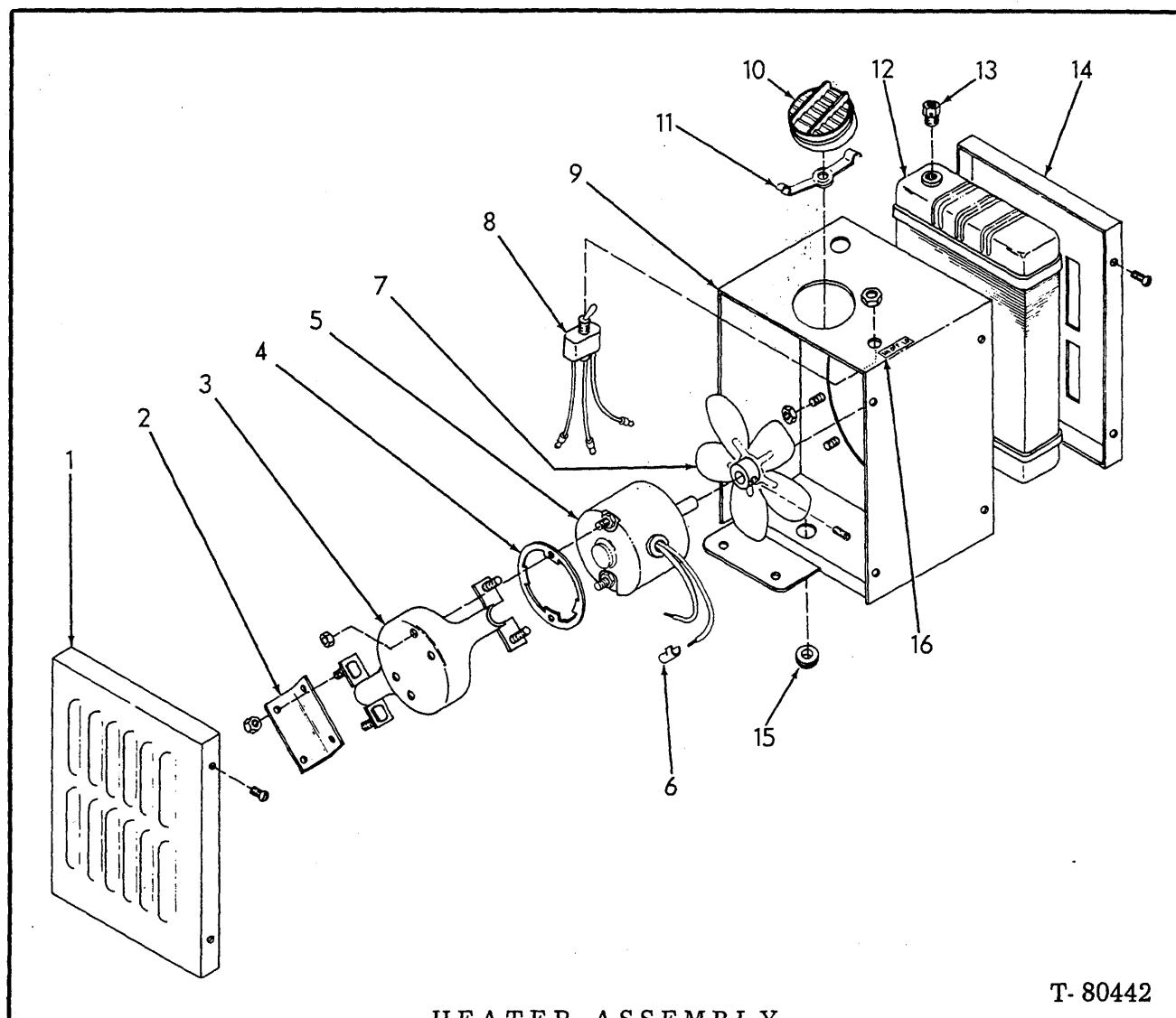
HEATER ASSEMBLY
