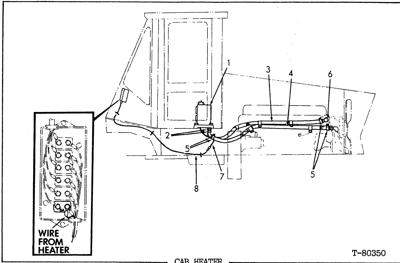
CAB HEATER
