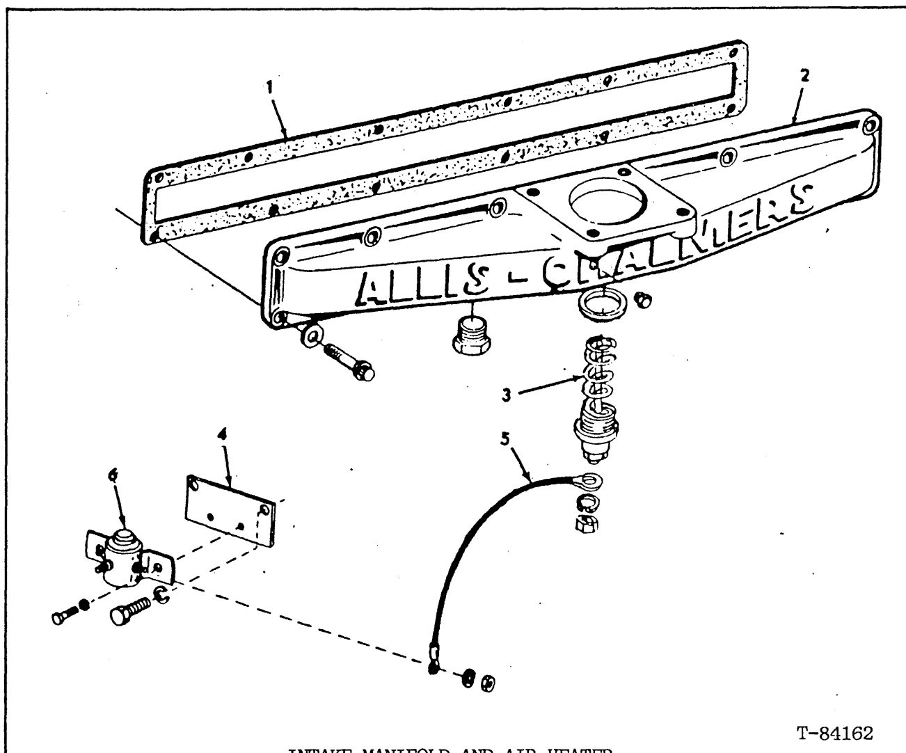
INTAKE MANIFOLD AND AIR HEATER
