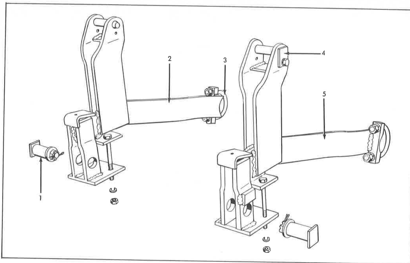
ANCHORS Inside Pushbeam Angle Dozers
