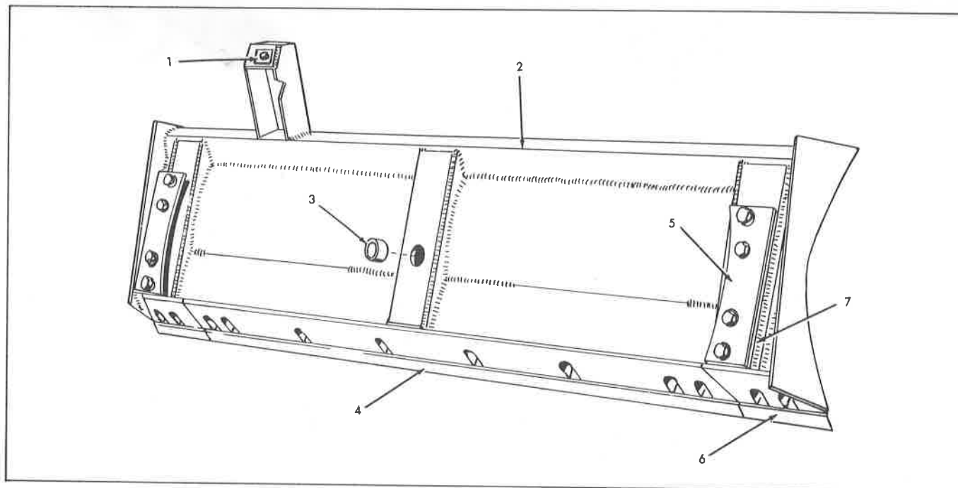
MOLDBOARD Outside Pushbeam Angle Dozer
