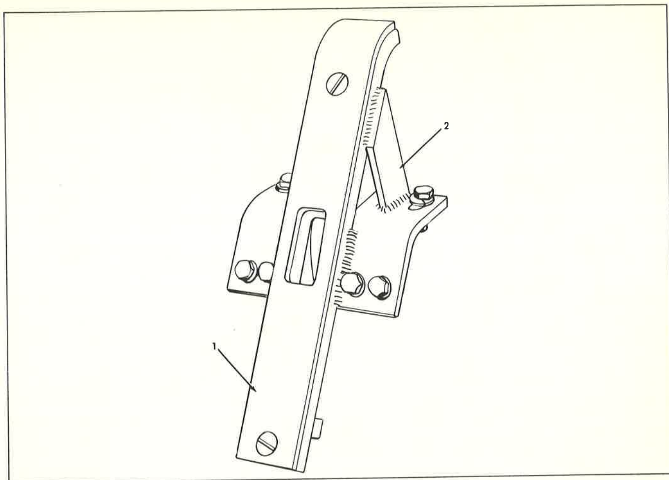
BUMPER Outside Pushbeam Angle Dozer
