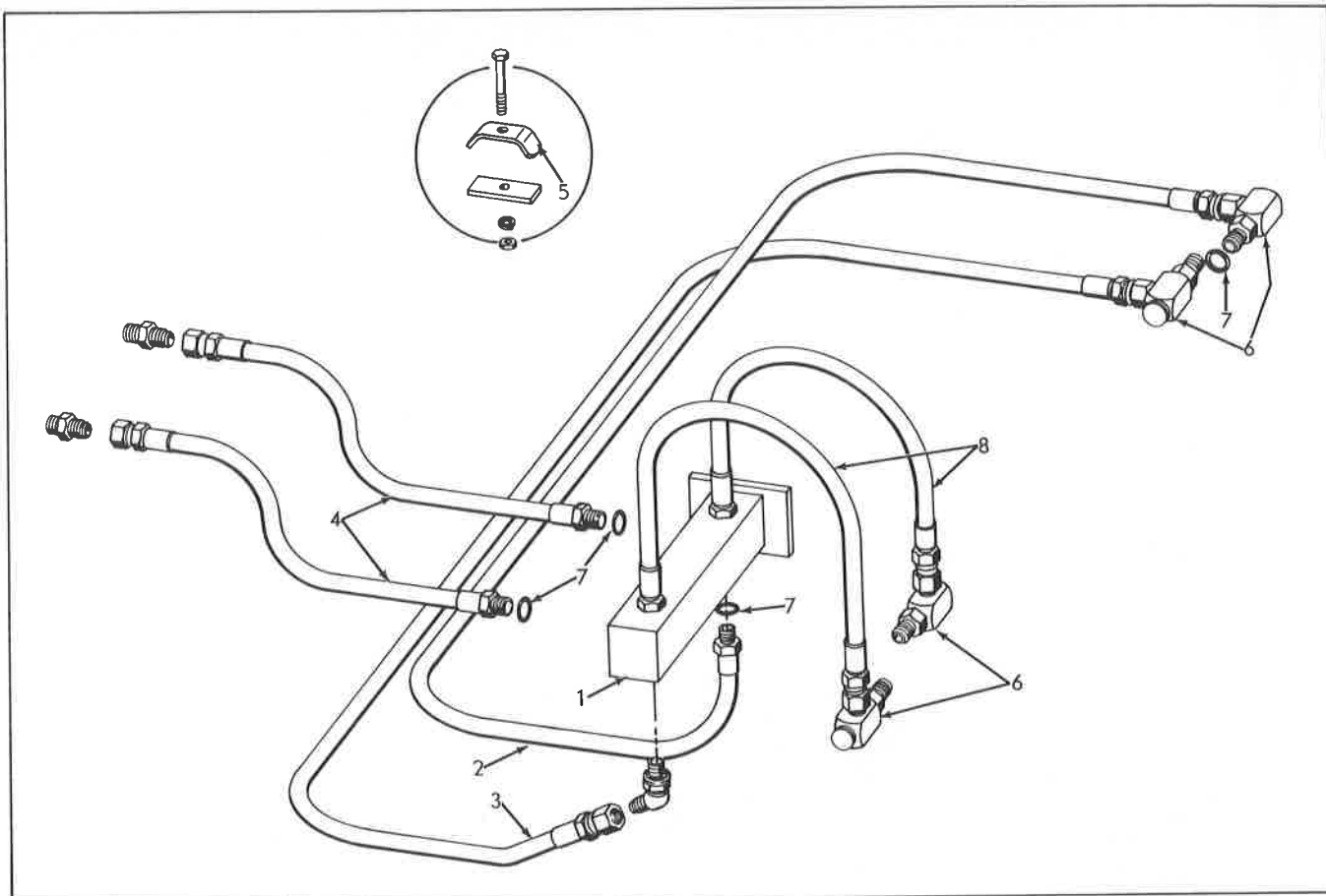
HYDRAULIC HOSES & MANIFOLD Inside & Outside Pushbeam Angle Dozers
