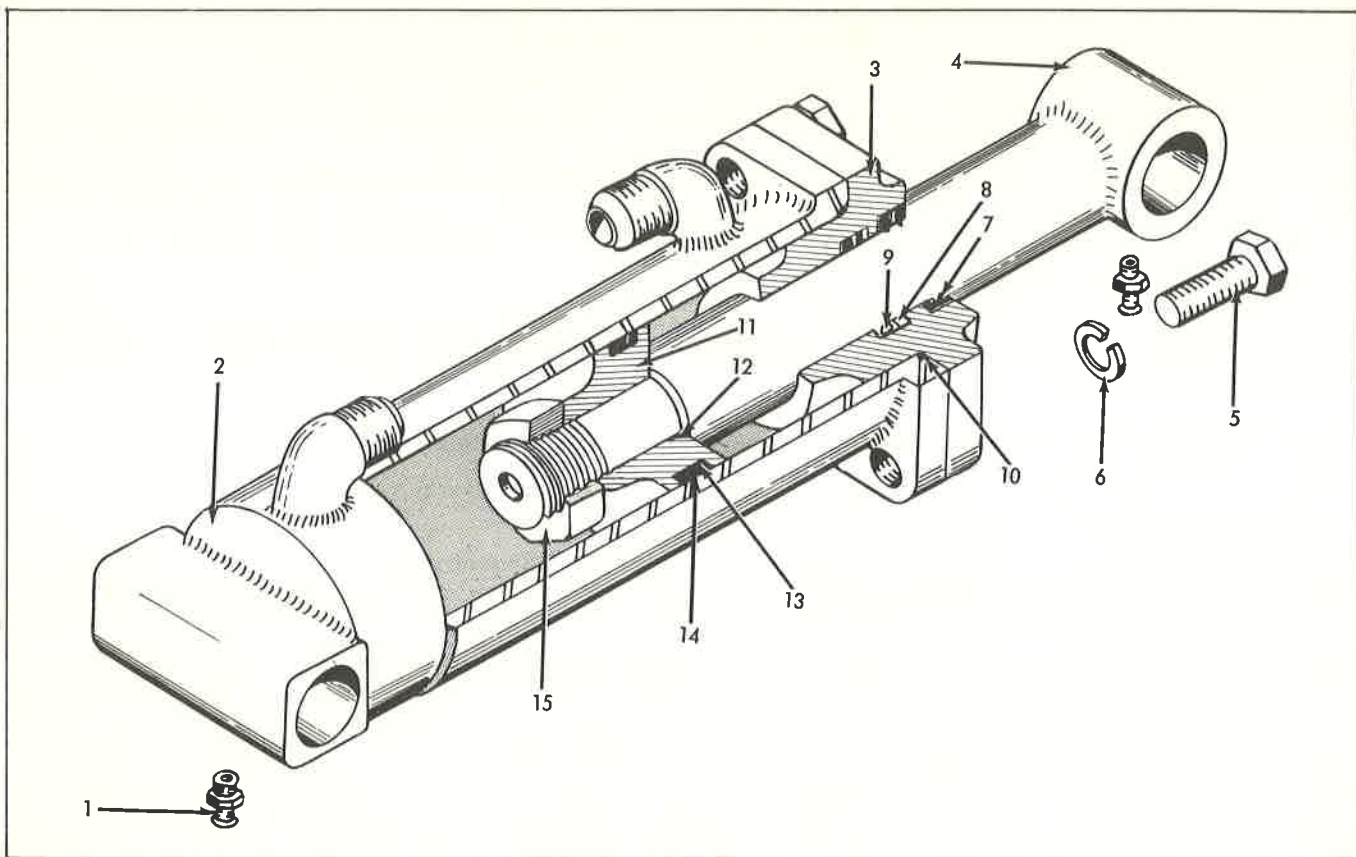
TILT CYLINDER Inside Pushbeams Angle Dozer 5" Stroke
