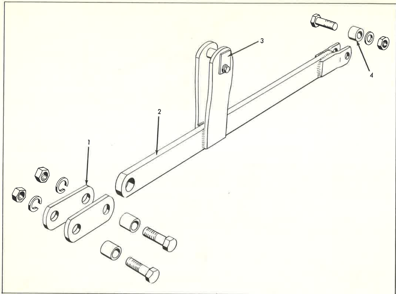
LIFT ARM Outside Pushbeam Angle Dozer
