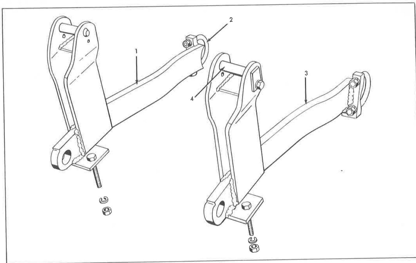
ANCHORS Outside Pushbeam Angle Dozer
