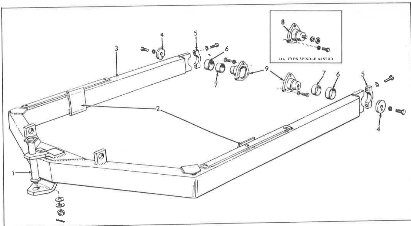
C-FRAME Outside Pushbeam Angle Dozer
