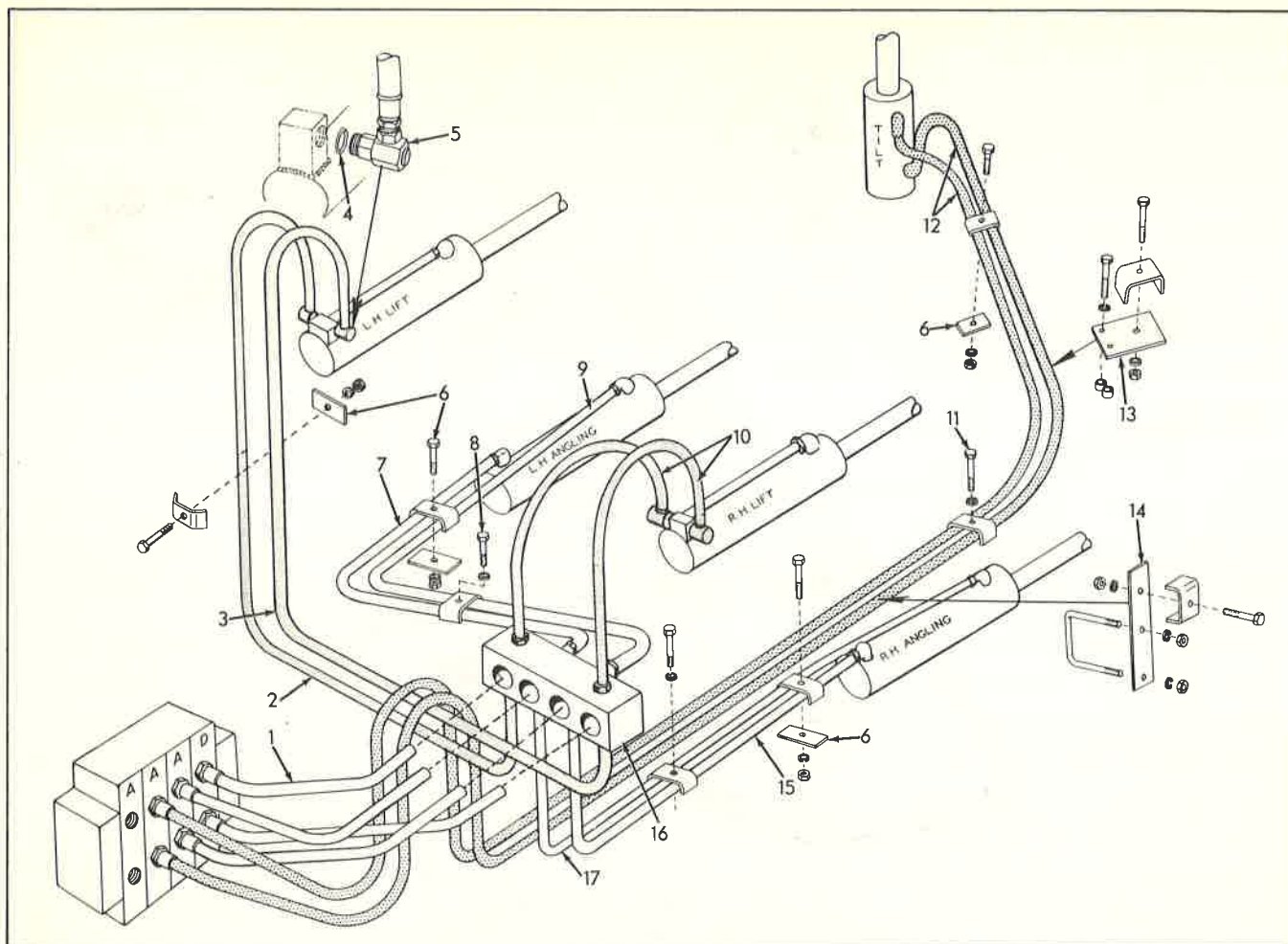
HYDRAULIC HOSES & MANIFOLD Inside Pushbeam Angle Dozers w/Hydraulic Lift, Angle & Tilt
