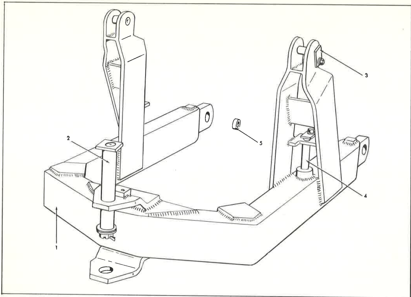
C-FRAME Inside Push Beam Angle Dozers
