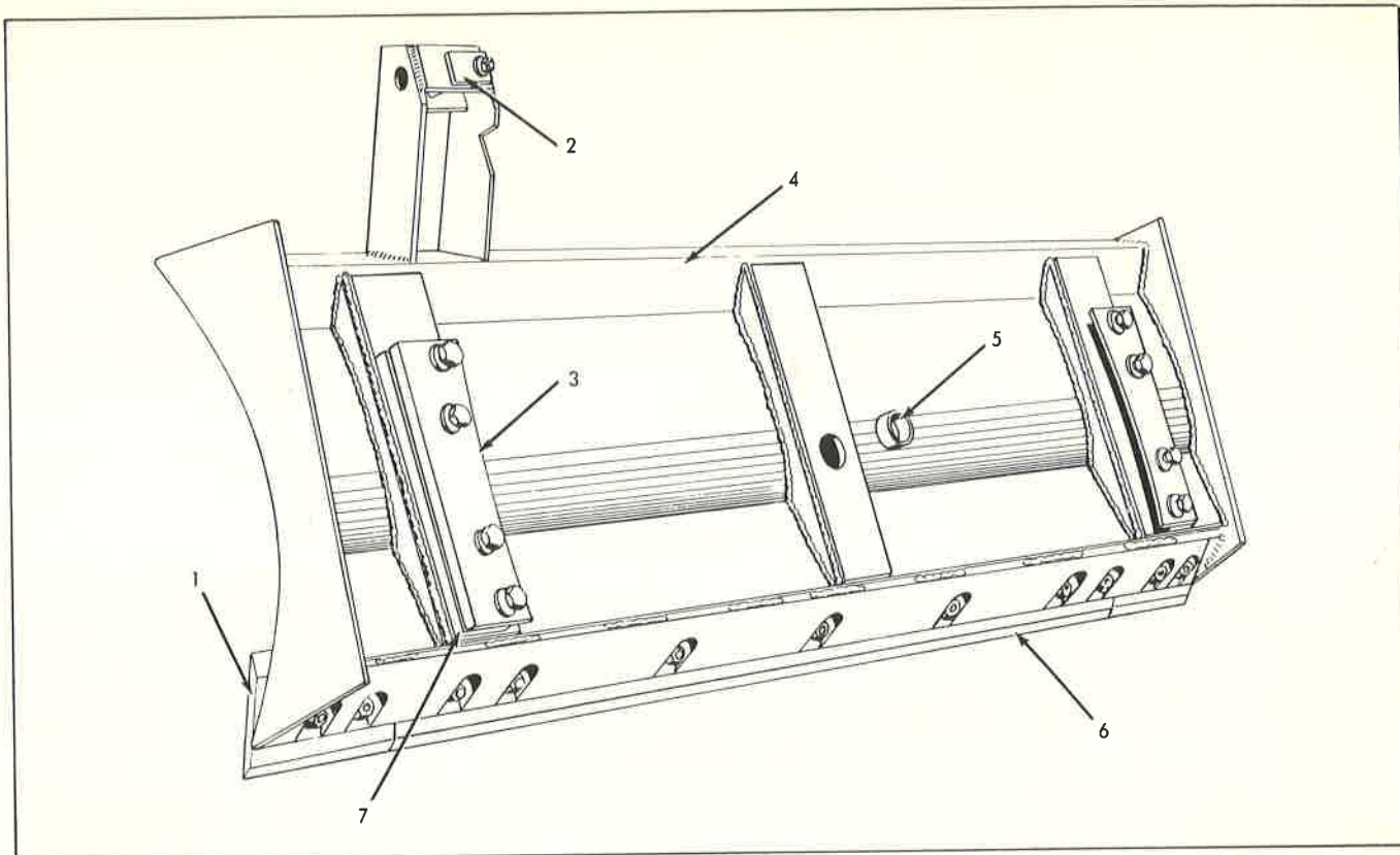
MOLDBOARD Inside Pushbeam Angle Dozer
