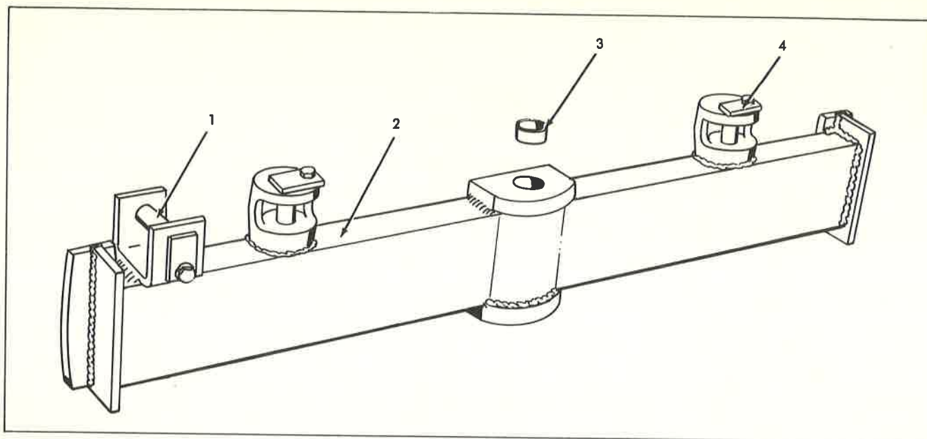
MOLDBOARD MOUNTING FRAME Inside Pushbeam Angle Dozers
