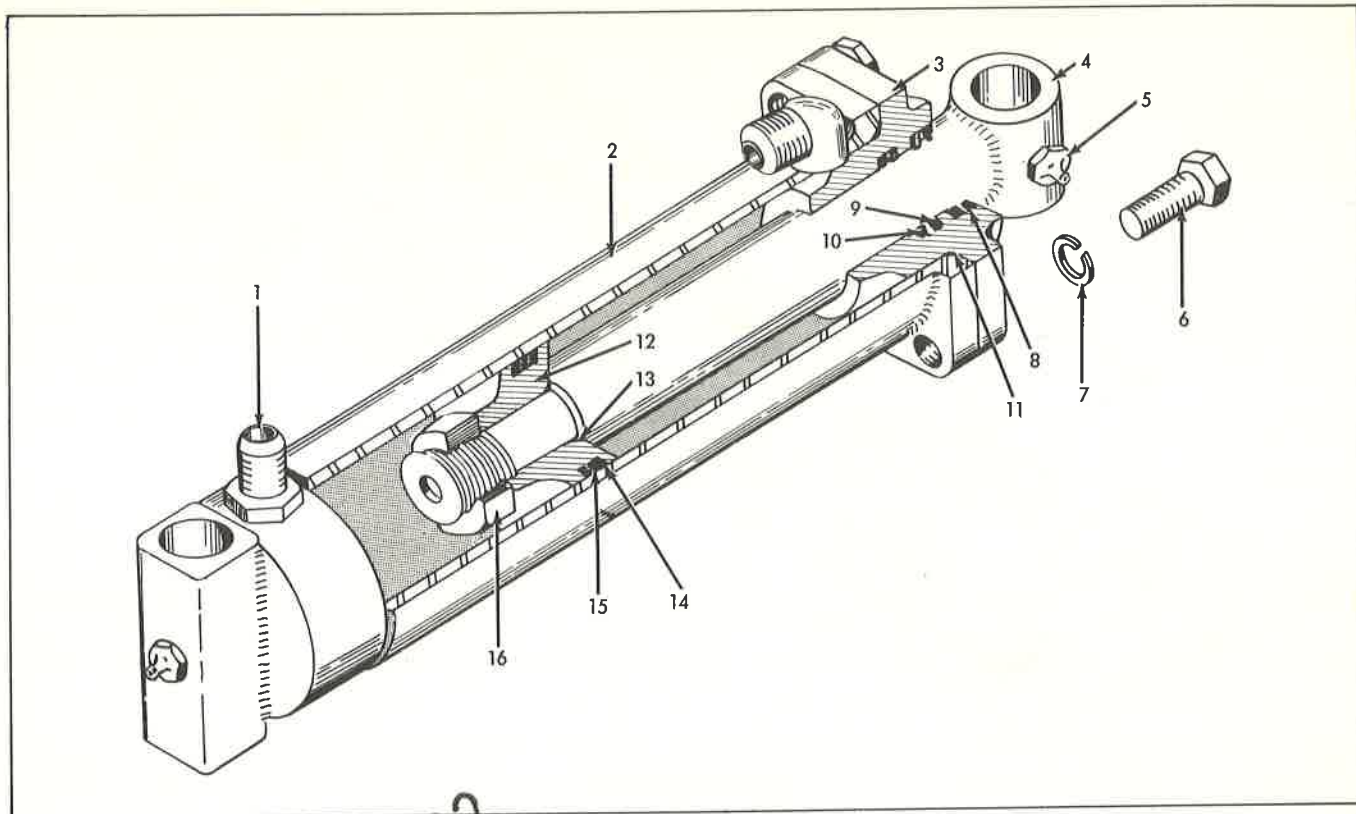
ANGLING CYLINDER Inside Pushbeam Angle Dozer 14" Stroke
