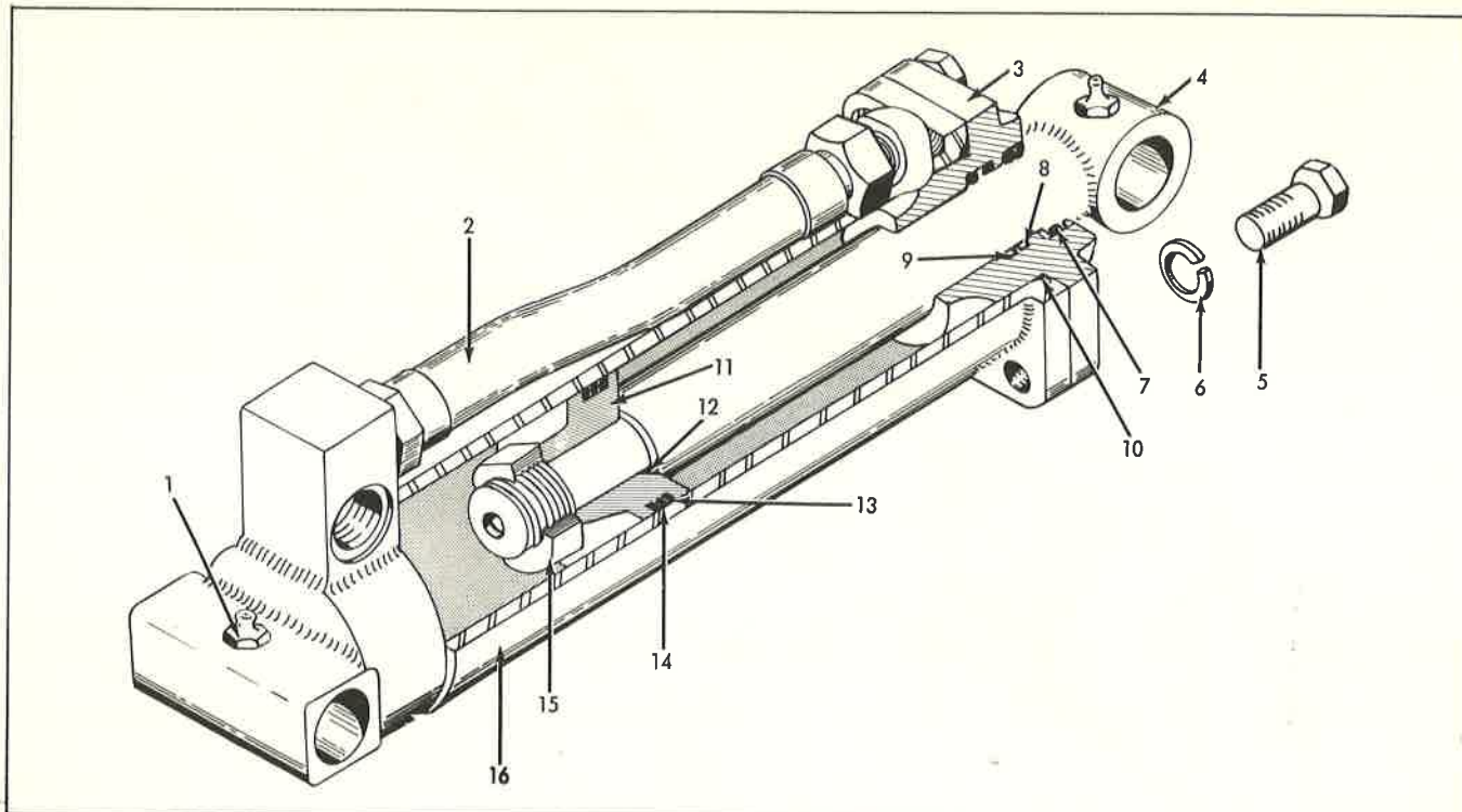
LIFT CYLINDER Inside & Outside Pushbeam Angle Dozers 16" Stroke
