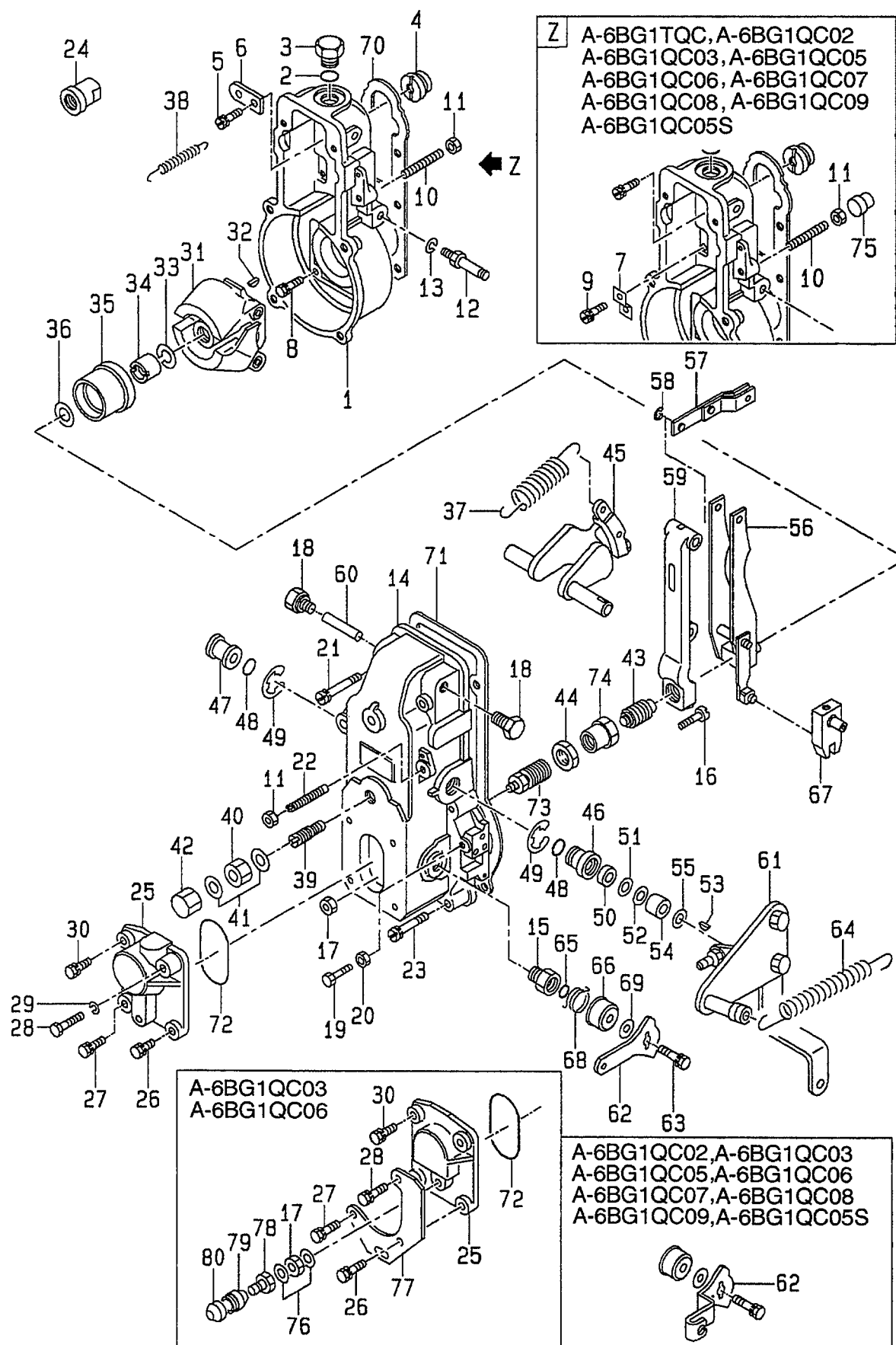
FIG. 32 GOVERNOR ガバナ
