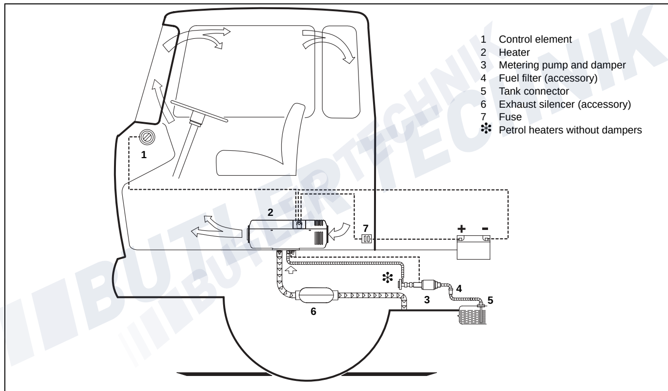
Fig. 7: Installation example for air heater
