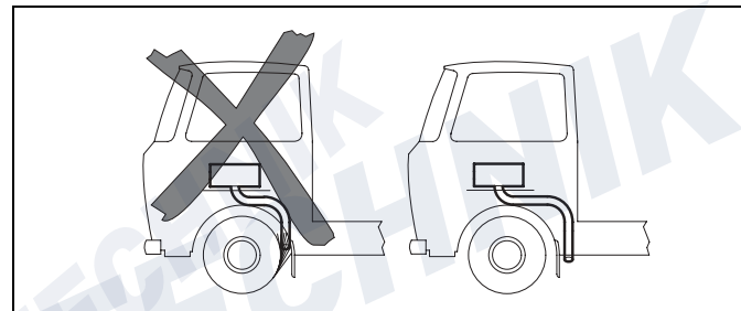
Fig. 21: Avoid the air outlet area
