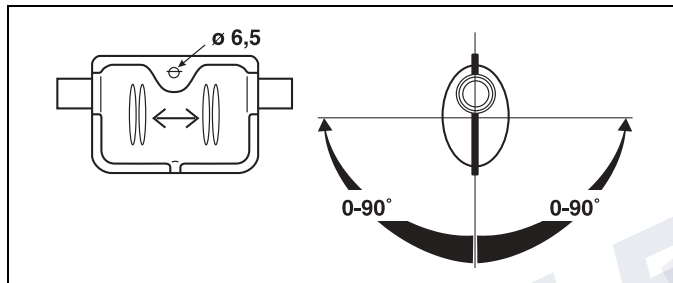
Fig. 18: Exhaust silencer
