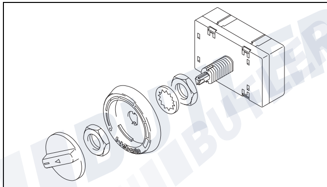
Fig. 26: Control element
