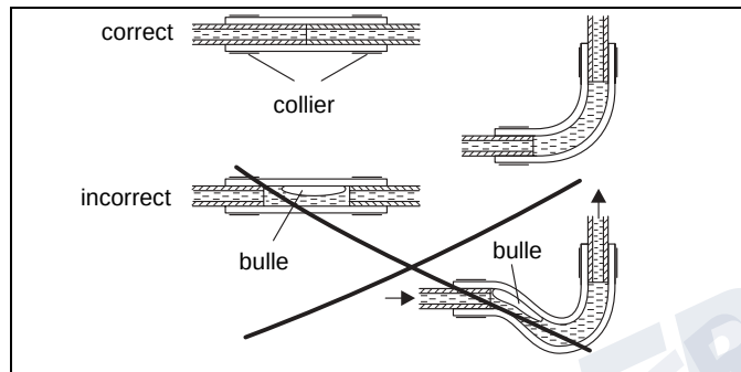
Fig. 14 Raccordement tube-tuyau
