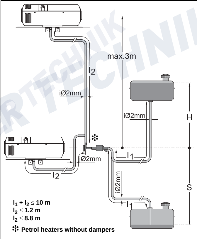
Fig. 9: Fuel supply
