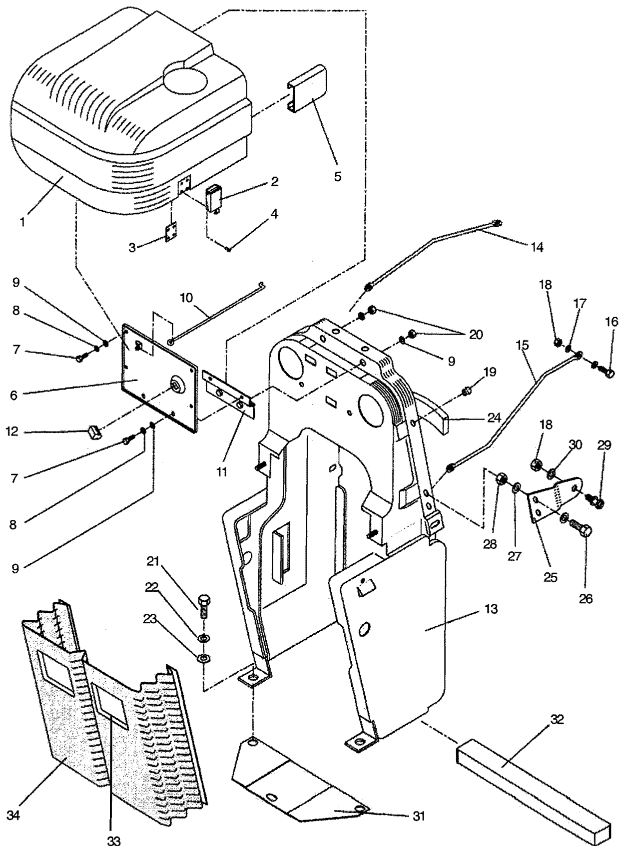
RADIATOR SHELL
