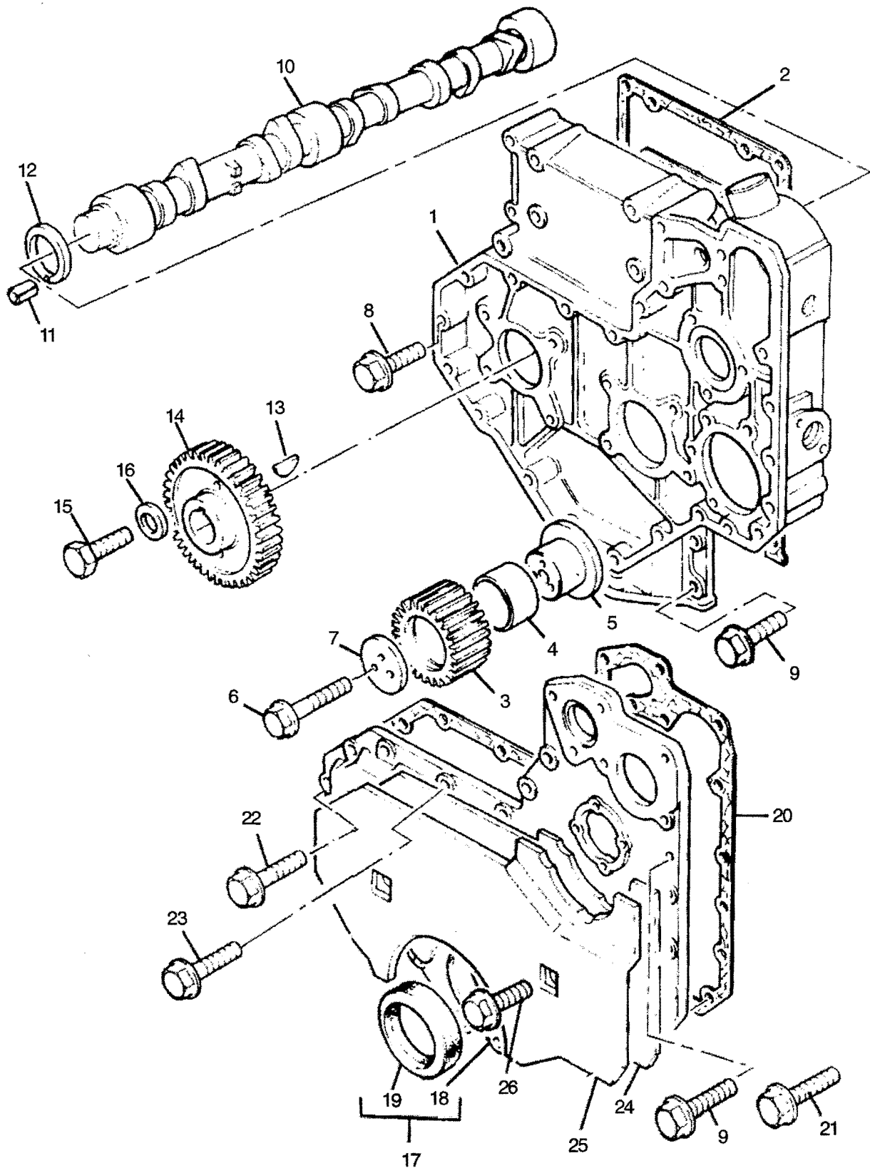
TIMING GEAR &amp; CAM SHAFT
