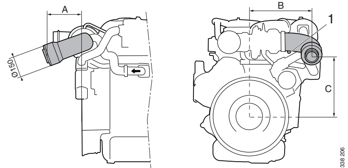
Example of a water-cooled exhaust pipe bend for DI09 and DI13.
