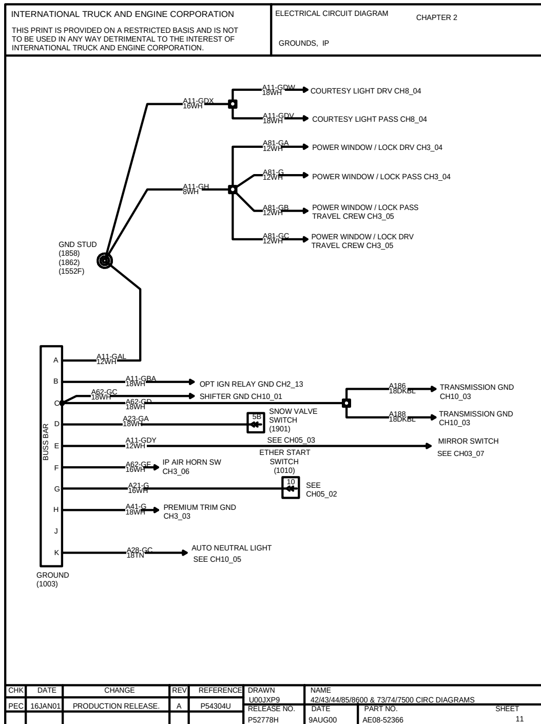
Figure 23 Grounds IP
