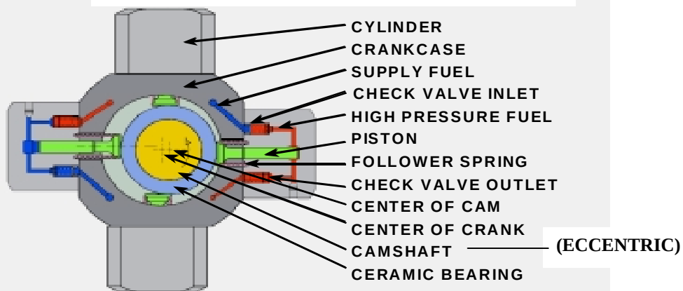
SIDE CUT AWAY VIEW (Fig. 17)
