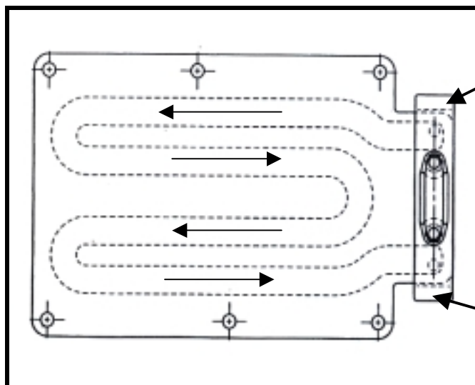
Fig. 92 Cold Plate Fuel Flow
