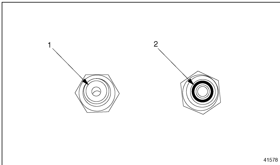
Figure 1 Improved Low-pressure Fuel Line Fitting
