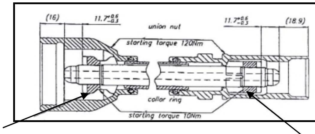
Fig. 61 High-pressure fuel line construction (cutaway).
