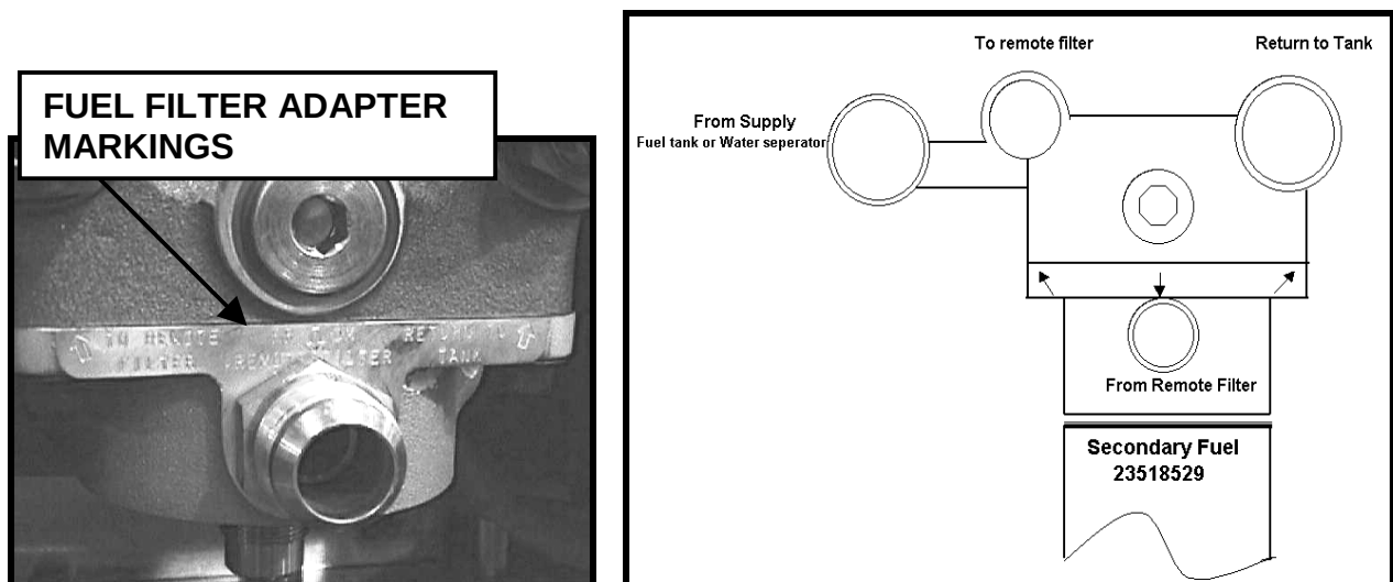
Fig. 105 C&I Fuel Junction Block Off-engine Fuel Line Connection Identification
