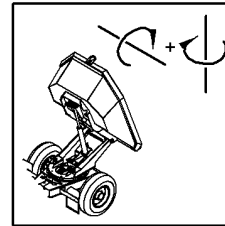
Drehkipper Swivel Tip Swivel Tip
