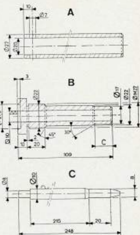
Guides de fabrication locale.
