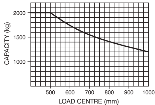
CAPACITY CHART
