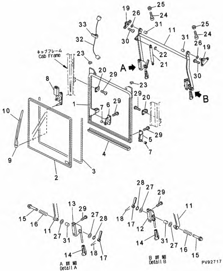
FIG. 224 CAB ASS'Y (2/3) (FRONT WINDOW AND RELATED PARTS) (APPLICABLE TO CAB SPEC.)
