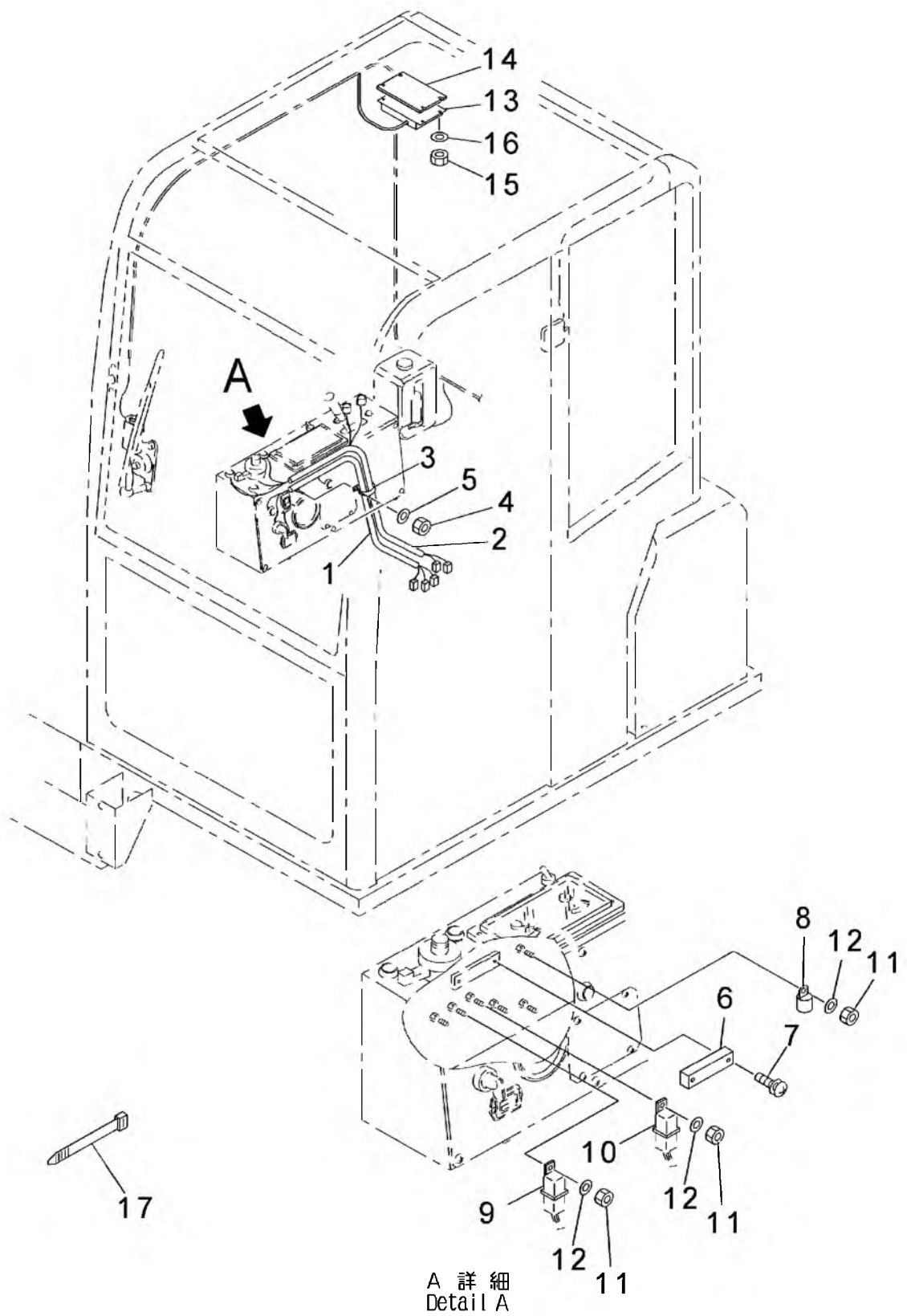
FIG. 705 ELECTRICAL SYSYTEM (CONSOLE BOX WIRING, BUZZER AND RELAY) (APPLICABLE TO CAB SPEC.)
