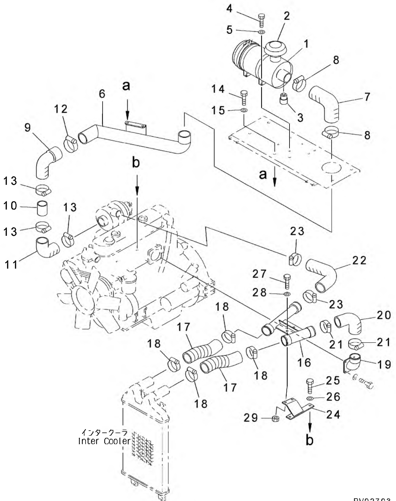
FIG. 111 ENGINE RELATED PARTS (AIR INTAKE SYSTEM) (SERIAL NO.4001-4011)
