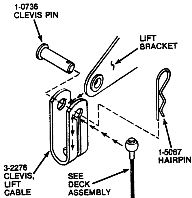
FRONT LIFT BRACKET
