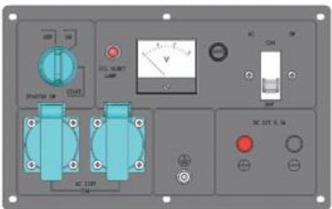
C:type-European standard
